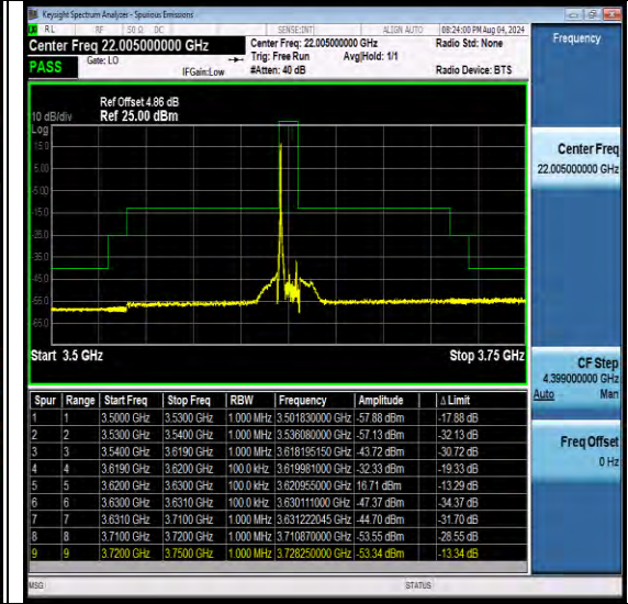
NTNV-N48-PC3-30-10-M-DFT-QPSK-Edge_1RB_Left-Ant1-PASS
