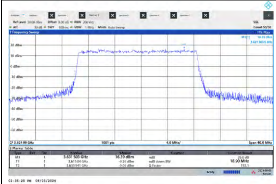
NTVN-N48-PC3-15-20-M-DFT-16QAM-Outer_Full-Ant5-PASS
