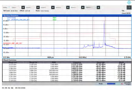
NTNV-N48-PC3-15-20-H-DFT-QPSK-Edge_1RB_Right-Ant5-PASS
