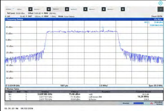
NTVN-N48-PC3-15-15-M-DFT-256QAM-Outer_Ful I-Ant5-PASS
