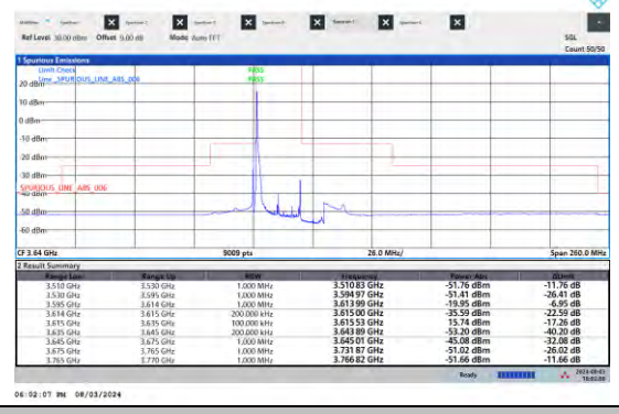
NTVN-N48-PC3-15-20-M-DFT-QPSK-Edge_1RB Left-Ant5-PASS
