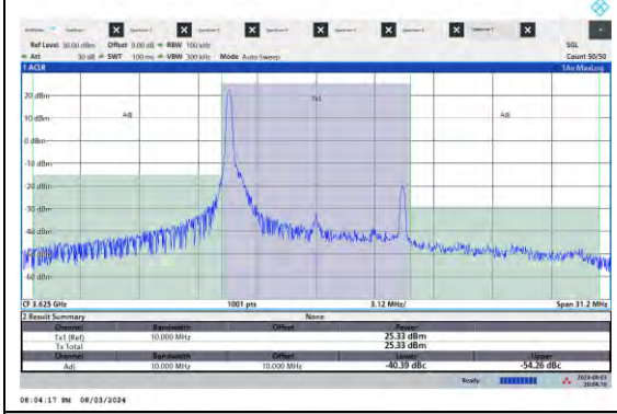
NTV-N48-PC3-15-10-M-DFT-QPSK-Edge_1RB_Left-Ant5-PASS
