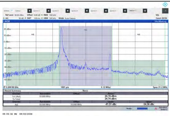
NTNV-N48-PC3-15-10-H-DFT-QPSK-Edge_1RB_Left-Ant5-PASS
