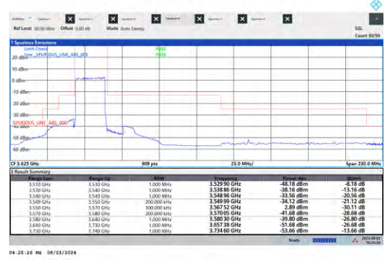
NTVN-N48-PC3-15-20-L-DFT-QPSK-Outer_Full-A nt5-PASS
