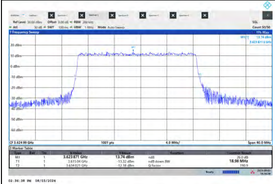
NTVN-N48-PC3-15-20-M-DFT-256QAM-Outer_Fu I-Ant5-PASS
