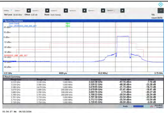
NTNV-N48-PC3-15-20-H-DFT-QPSK-Outer_Full-Ant5-PASS
