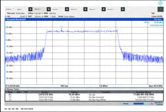
NTVN-N48-PC3-15-20-M-DFT-64QAM-Outer_Full-Ant5-PASS
