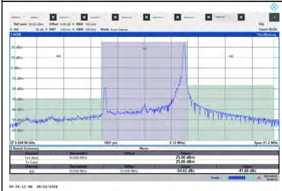
NTNV-N48-PC3-15-10-H-DFT-QPSK-Edge_1RB_Right-Ant5-PASS
