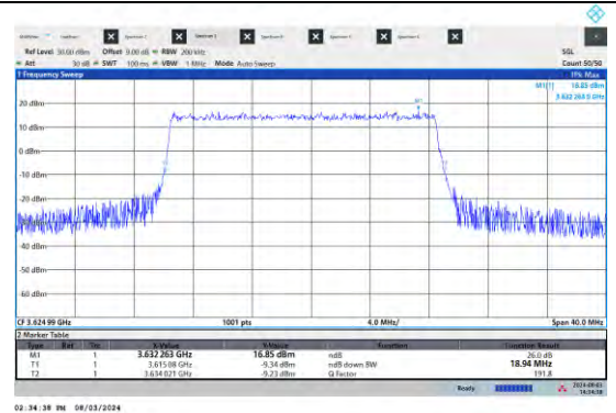
NTVN-N48-PC3-15-20-M-DFT-QPSK-Outer_Full-Ant5-PASS
