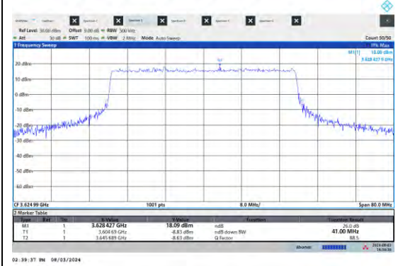
NTVN-N48-PC3-15-40-M-DFT-QPSK-Outer_Full-Ant5-PASS
