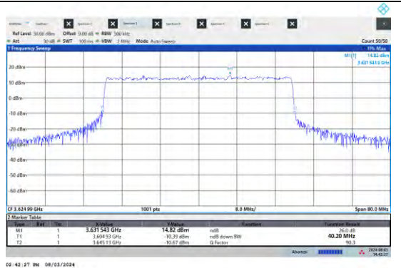
NTV-N48-PC3-15-40-M-DFT-256QAM-Outer_Ful-I-Ant5-PASS
