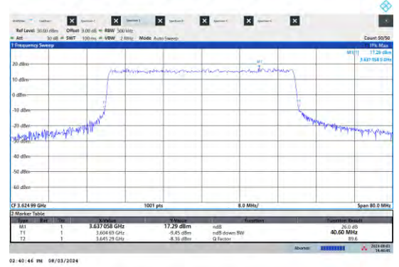
NTVN-N48-PC3-15-40-M-DFT-16QAM-Outer_Full-Ant5-PASS
