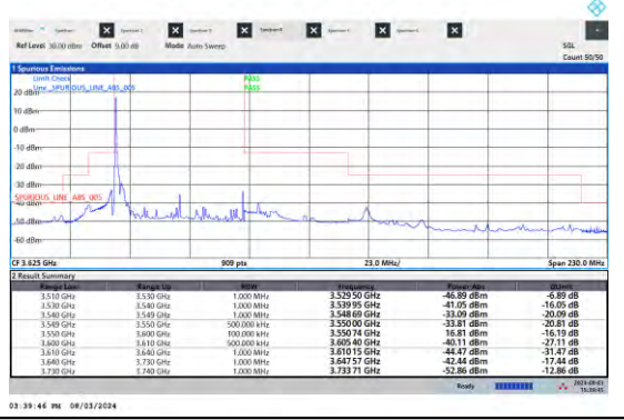
NTNV-N48-PC3-15-50-L-DFT-QPSK-Edge_1RB_Left-Ant5-PASS
