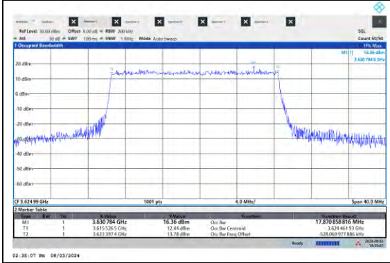
NTVN-N48-PC3-15-20-M-DFT-16QAM-Outer_Full-Ant5-PASS
