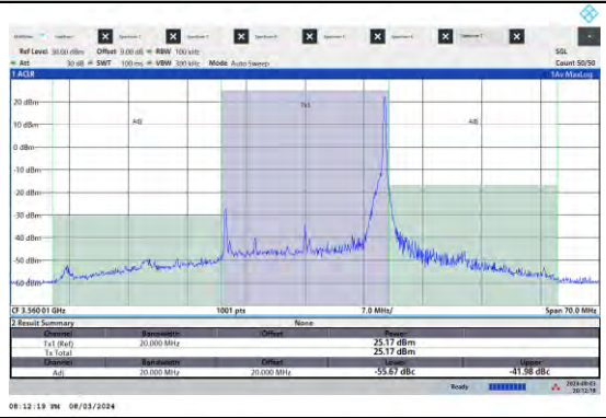
NTNV-N48-PC3-15-20-L-DFT-QPSK-Edge_1RB_Right-Ant5-PASS
