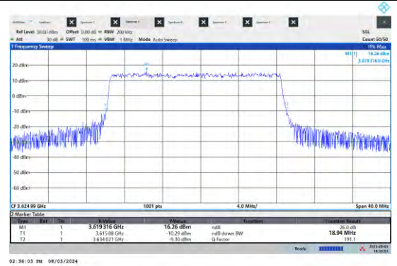
NTVN-N48-PC3-15-20-M-DFT-64QAM-Outer_Full-Ant5-PASS
