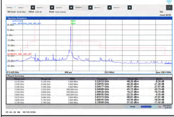
NTNV-N48-PC3-15-50-L-DFT-QPSK-Edge_1RB_Right-Ant5-PASS
