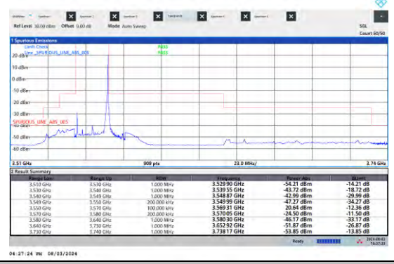
NTVN-N48-PC3-15-20-L-DFT-QPSK-Edge_1RB Right-Ant5-PASS
