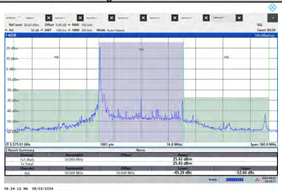
NTVN-N48-PC3-15-50-L-DFT-QPSK-Outer_Full-Ant5-PASS
