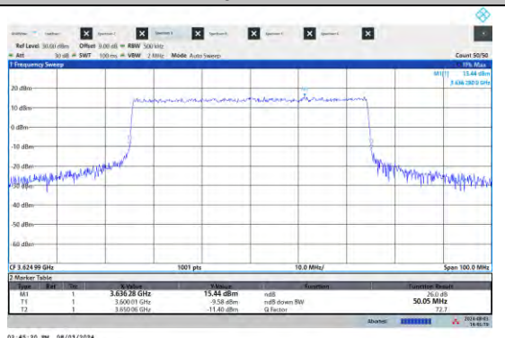
NTV-N48-PC3-50-M-DFT-PI2BPSK-Outer_Full-Ant5-PASS
