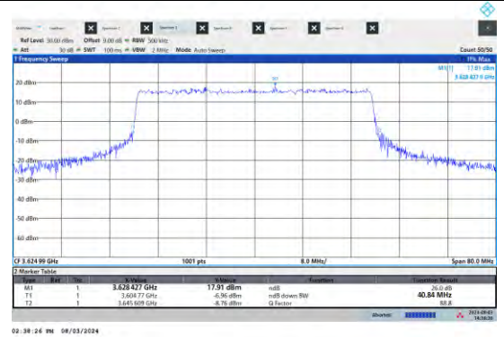
NTVN-N48-PC3-40-M-DFT-PI2BPSK-Outer_Full-Ant5-PASS
