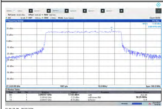
NTV-N48-PC3-15-50-M-DFT-QPSK-Outer_Full-Ant5-PASS
