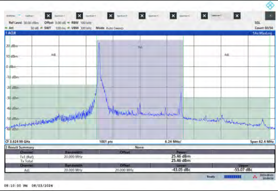
NTNV-N48-PC3-15-20-M-DFT-QPSK-Edge_1RB_Left-Ant5-PASS
