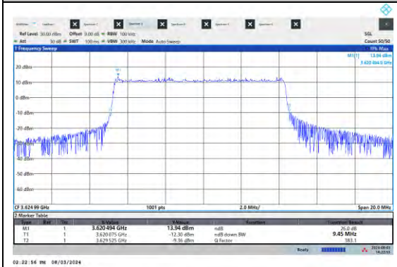
NTVN-N48-PC3-15-10-M-DFT-256QAM-Outer_Ful I-Ant5-PASS
