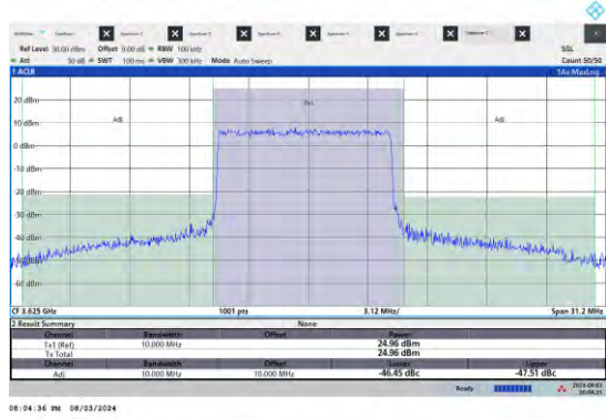
NTV-N48-PC3-15-10-M-DFT-QPSK-Outer_Full-Ant5-PASS
