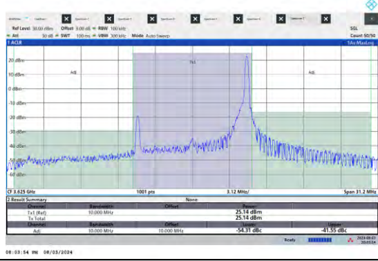
NTV-N48-PC3-15-10-M-DFT-QPSK-Edge_1RB_Right-Ant5-PASS
