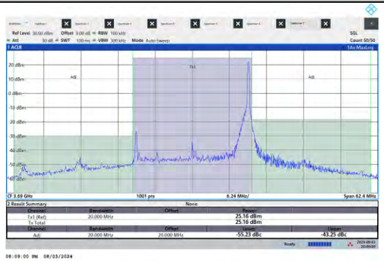
NTVN-N48-PC3-15-20-H-DFT-QPSK-Edge_1RB_Right-Ant5-PASS
