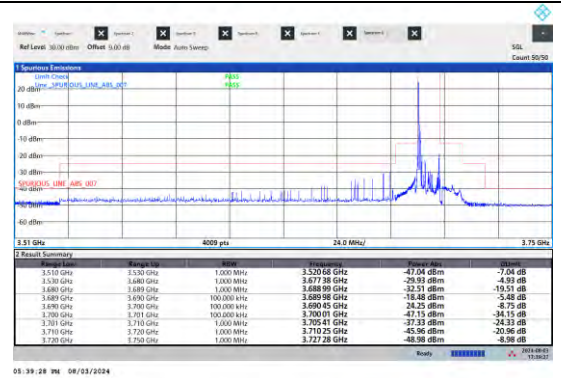
NTVN-N48-PC3-15-10-H-DFT-QPSK-Edge_1RB Left-Ant5-PASS
