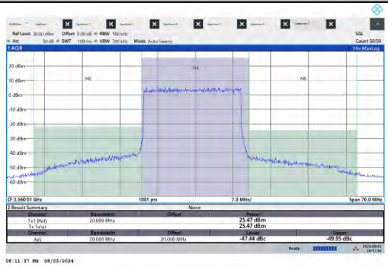
NTNV-N48-PC3-15-20-L-DFT-QPSK-Outer_Full-Ant5-PASS
