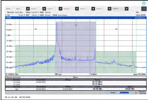
NTNV-N48-PC3-15-20-L-DFT-QPSK-Edge_1RB_Left-Ant5-PASS
