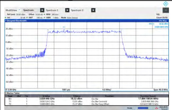
NTN-N77-3700-3980-PC2-15-20-M-DFT-64QAM-Outer Full-Ant5-PASS
