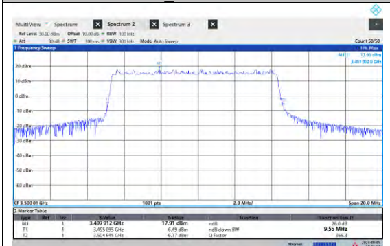
NTN-N77-3450-3550-PC2-15-10-M-DFT-16QAM
