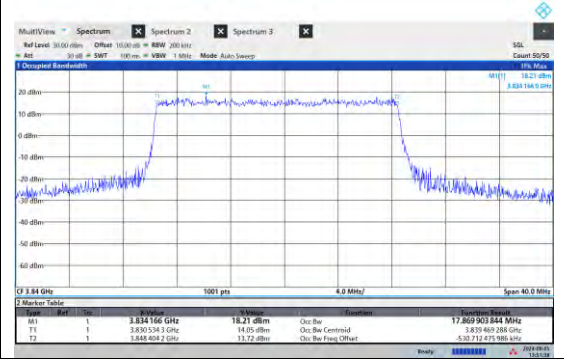
NTN-N77-3700-3980-PC2-15-20-M-DFT-QPSK-Outer Full-Ant5-PASS
