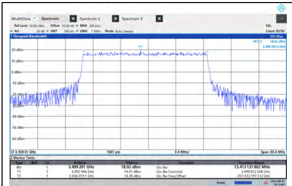
NTNV-N77-3450-3550-PC2-15-15-M-DFT-QPSK-Outer Full-Ant5-PASS
