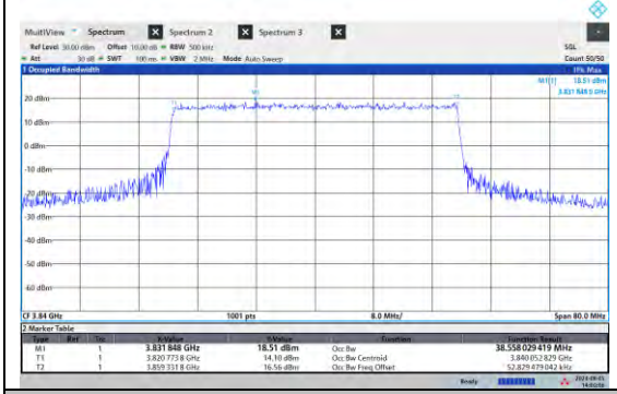
NTNV-N77-3700-3980-PC2-15-40-M-DFT-64QAM-Outer Full-Ant5-PASS
