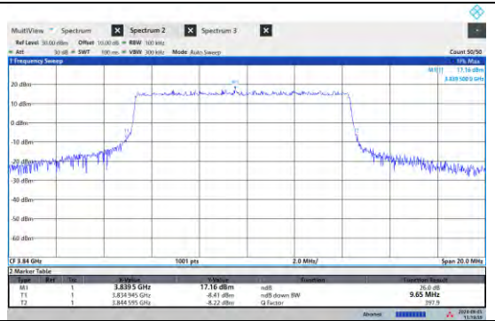
NTNV-N77-3700-3980-PC2-15-10-M-DFT-QPSK-Outer_Full-Ant5-PASS
