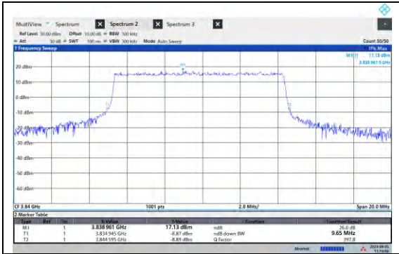
NTNV-N77-3700-3980-PC2-15-10-M-DFT-PI2BPS K-Outer_Full-Ant5-PASS
