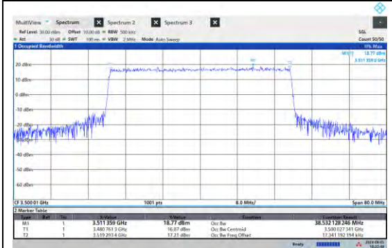
NTNV-N77-3450-3550-PC2-15-40-M-DFT-QPSK-Outer Full-Ant5-PASS
