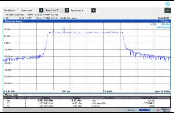
NTNV-N77-3700-3980-PC2-15-10-M-DFT-64QAM
