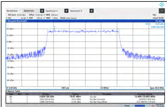
NTN-N77-3700-3980-PC2-15-15-M-DFT-QPSK-Outer Full-Ant5-PASS
