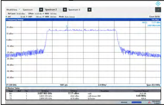
NTNV-N77-3700-3980-PC2-15-10-M-DFT-16QAM
