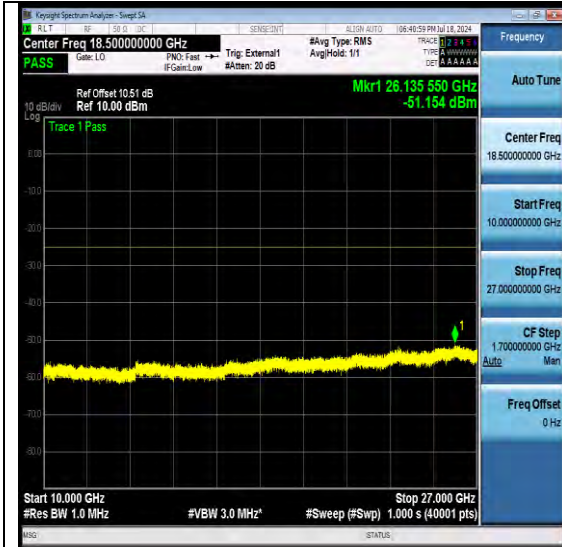
NTN-N41-PC3-30-100-L-DFT-QPSK-Edge_1RB Left-Ant1-PASS
