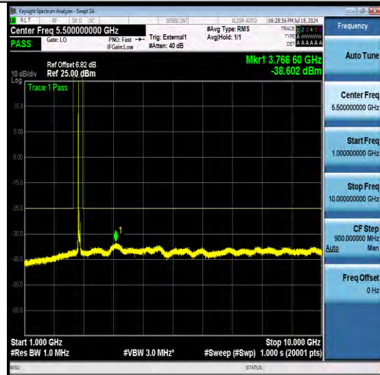
NTNV-N41-PC3-30-60-H-DFT-QPSK-Edge_1RB_Left-Ant1-PASS
