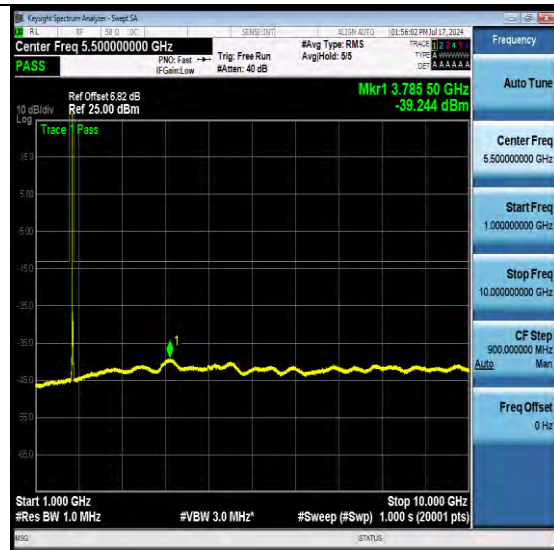
NTNV-N66-PC3-15-20-H-DFT-QPSK-Edge_1RB_Left-Ant1-PASS
