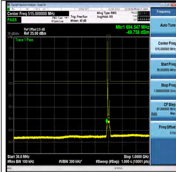
NTNV-N12-PC3-15-15-M-DFT-QPSK-Edge_1RB_Left-Ant1-PASS
