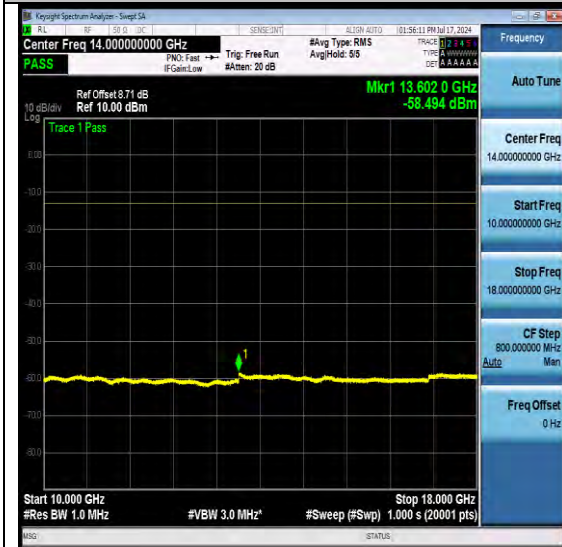
NTNV-N66-PC3-15-20-H-DFT-QPSK-Edge_1RB_Left-Ant1-PASS
