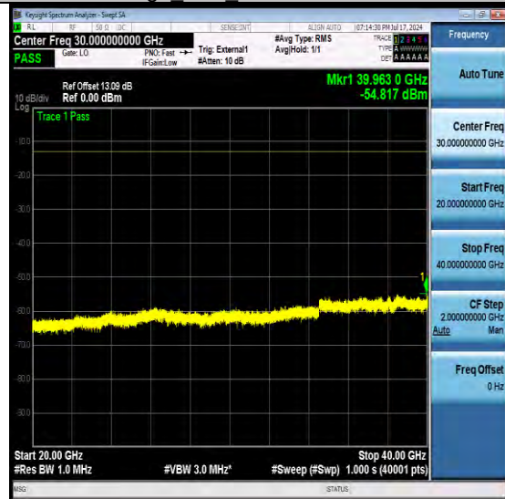
NTNV-N77-3700-3980-PC2-30-30-H-DFT-QPSK-Edge 1RB Left-Ant1-PASS
