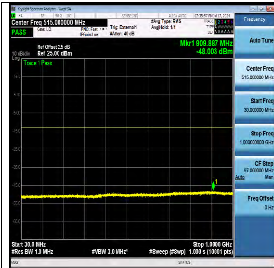
NTNV-N77-3700-3980-PC2-30-100-H-DFT-QPSK-Edge_1RB_Left-Ant1-PASS
