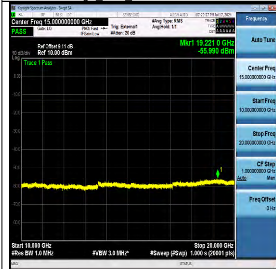
NTNV-N77-3700-3980-PC2-30-100-L-DFT-QPSK-Edge 1RB Left-Ant1-PASS
