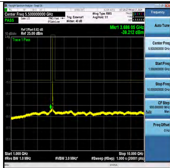
NTNV-N77-3700-3980-PC2-30-60-M-DFT-QPSK-Edge 1RB Left-Ant1-PASS
