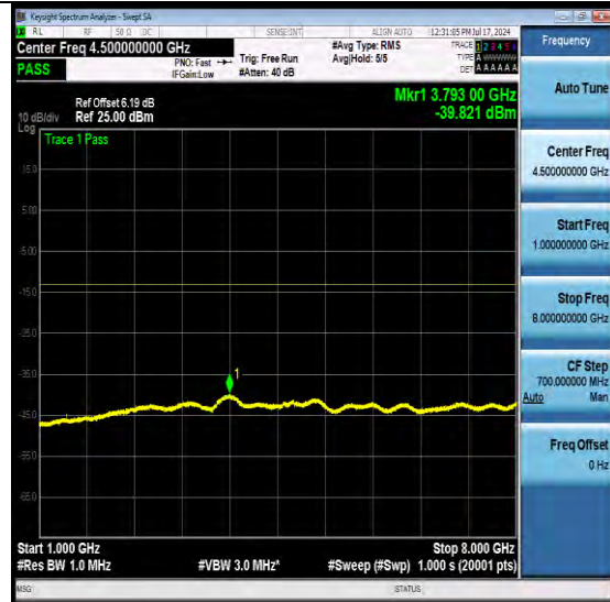
NTNV-N12-PC3-15-15-M-DFT-QPSK-Edge_1RB_Left-Ant1-PASS
