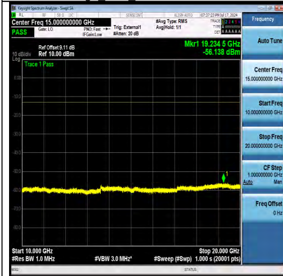
NTNV-N77-3700-3980-PC2-30-100-H-DFT-QPSK-Edge_1RB_Left-Ant1-PASS
