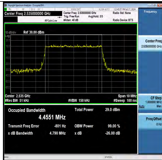
NTNV-N7-PC3-15-5-M-DFT-QPSK-Outer_Full-Ant1-PASS
