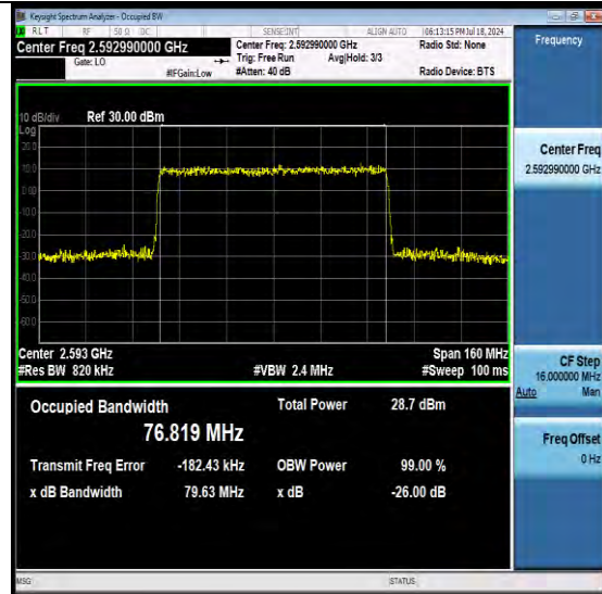
NTNV-N41-PC3-30-80-M-DFT-64QAM-Outer_Full-Ant1-PASS
