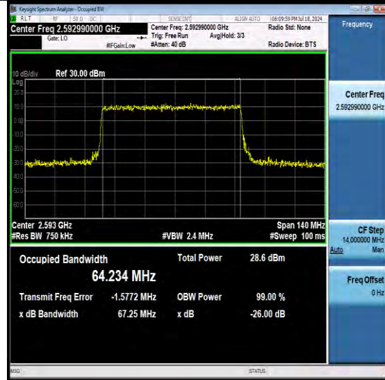
NTNV-N41-PC3-30-70-M-DFT-256QAM-Outer_Full-Ant1-PASS
