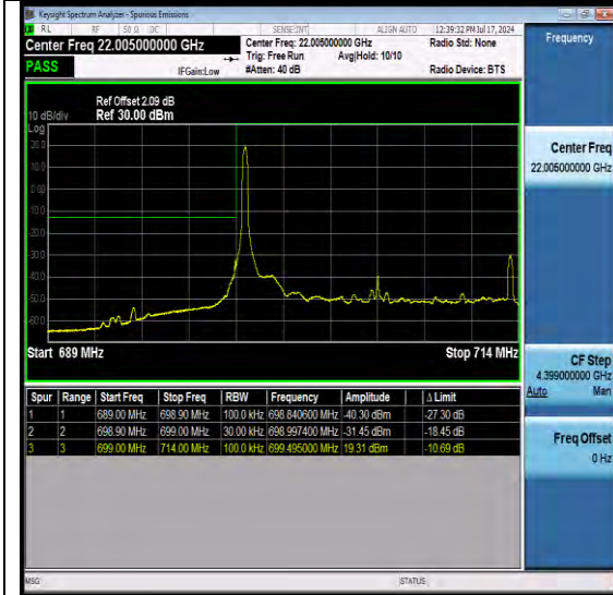
N12-PC3-15-15-L-DFT-QPSK-Edge_1RB_Left-Ant1-PASS
