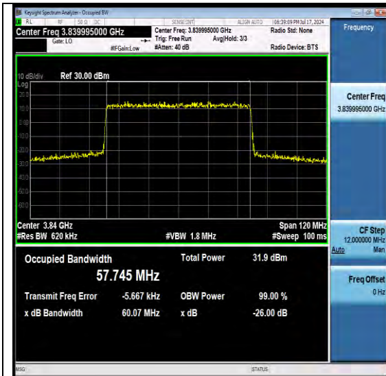
NTNV-N77-3700-3980-PC2-30-60-M-DFT-QPSK-Outer Full-Ant1-PASS
