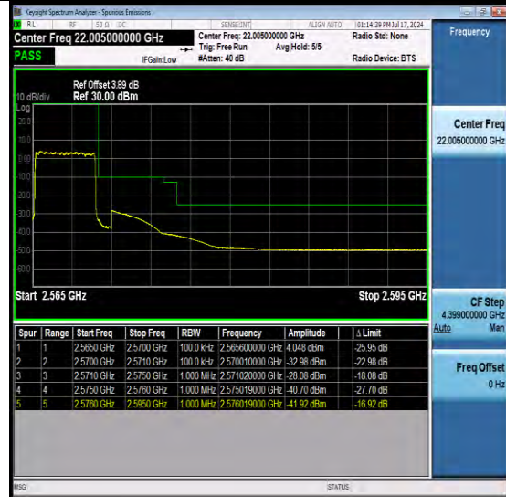
NTNV-N7-PC3-15-5-H-DFT-QPSK-Outer_Full-Ant1-PASS
