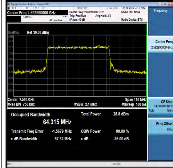
NTNV-N41-PC3-30-70-M-DFT-64QAM-Outer_Full-Ant1-PASS
