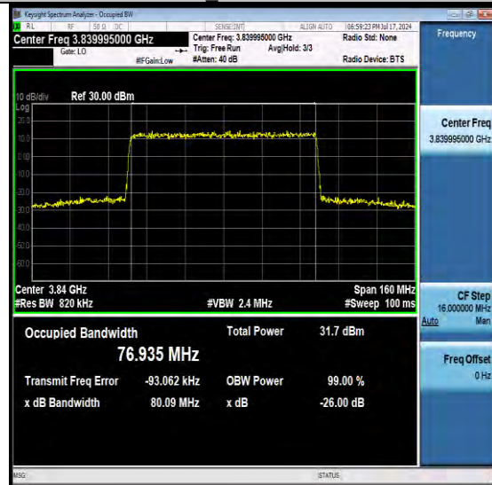
NTNV-N77-3700-3980-PC2-30-80-M-DFT-16QAM-Outer Full-Ant1-PASS
