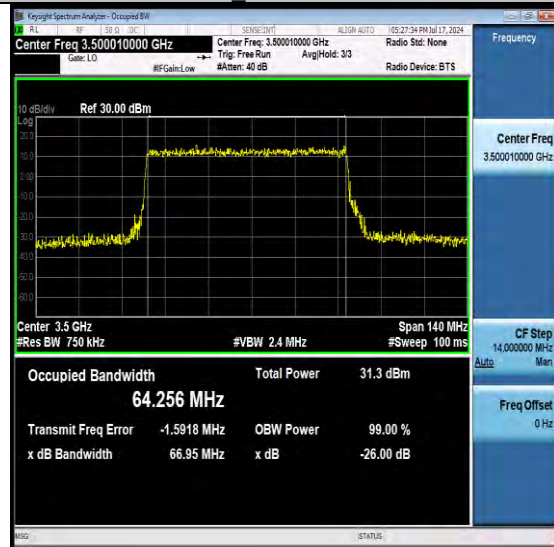
NTNV-N77-3450-3550-PC2-30-70-M-DFT-16QAM-Outer Full-Ant1-PASS
