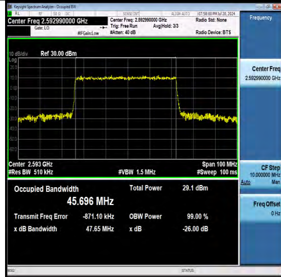
NTNV-N41-PC3-30-50-M-DFT-256QAM-Outer_Full-Ant1-PASS
