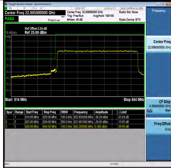
NTNV-N26-824-849-PC3-15-20-L-DFT-QPSK-Outer Full-Ant1-PASS
