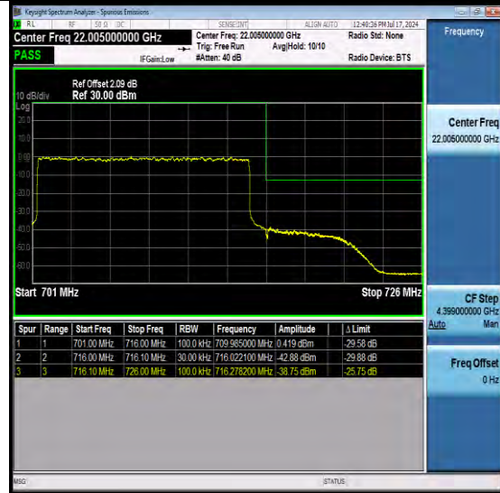
N12-PC3-15-15-H-DFT-QPSK-Outer_Full-Ant1-PASS
