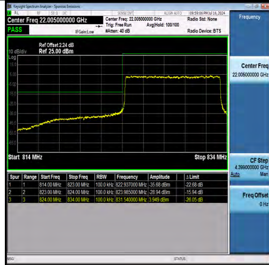
NTNV-N26-824-849-PC3-15-10-L-DFT-QPSK-Outer Full-Ant1-PASS
