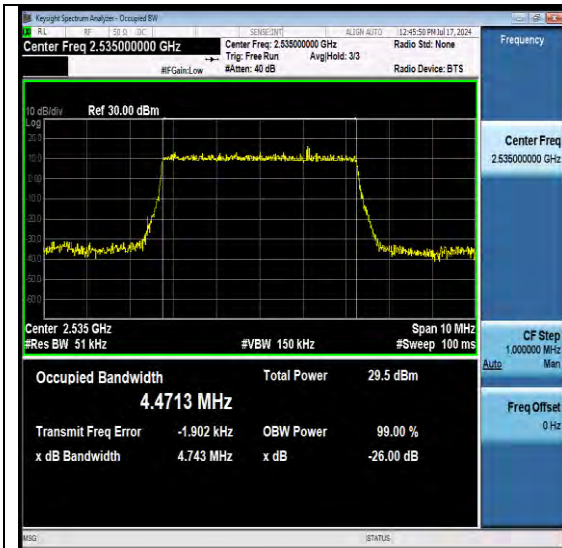
NTNV-N7-PC3-15-5-M-DFT-PI2BPSK-Outer_Full-Ant1-PASS
