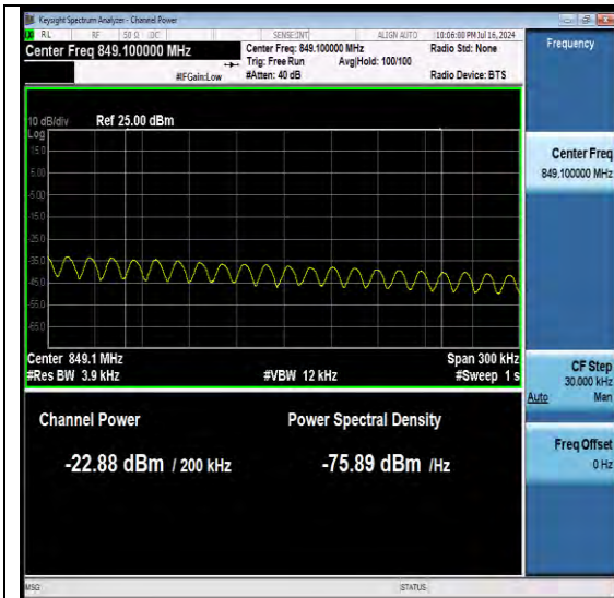
NTNV-N26-824-849-PC3-15-20-H-DFT-QPSK-Edge_1RB_Right-Ant1-PASS
