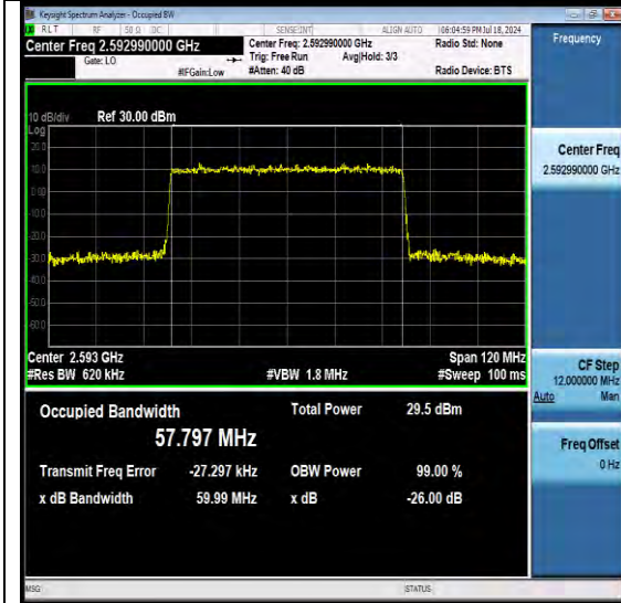
NTNV-N41-PC3-30-60-M-DFT-16QAM-Outer_Full-Ant1-PASS
