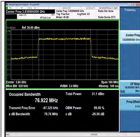
NTNV-N77-3700-3980-PC2-30-80-M-DFT-64QAM-Outer Full-Ant1-PASS
