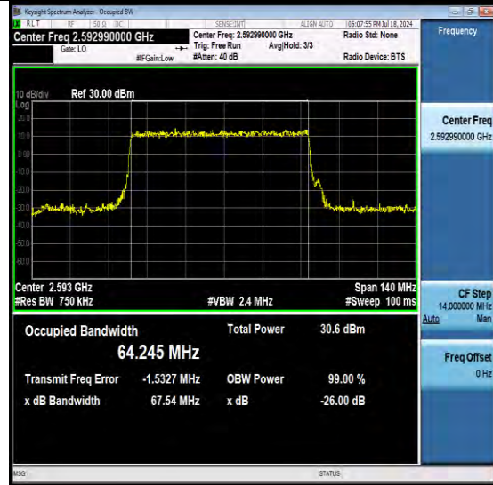
NTNV-N41-PC3-30-70-M-DFT-PI2BPSK-Outer_Fu II-Ant1-PASS
