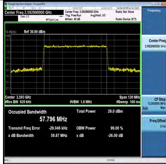
NTNV-N41-PC3-30-60-M-DFT-64QAM-Outer_Full-Ant1-PASS
