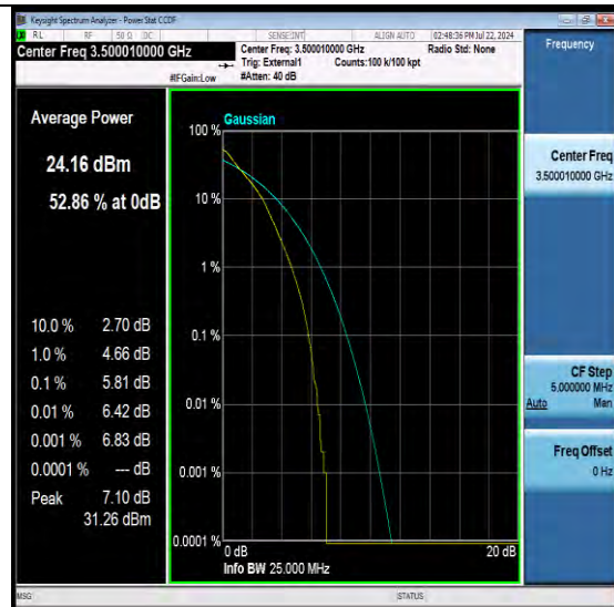
NTNV-N77-3450-3550-PC2-30-20-M-DFT-QPSK-Outer Full-PASS
