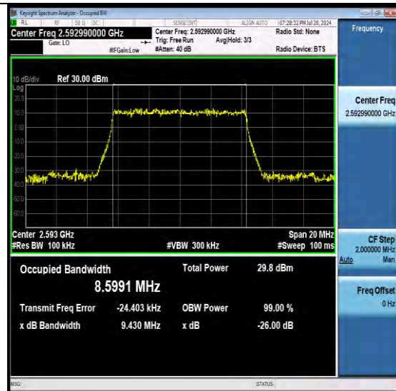
NTNV-N41-PC3-30-10-M-DFT-PI2BPSK-Outer_Fu II-Ant1-PASS
