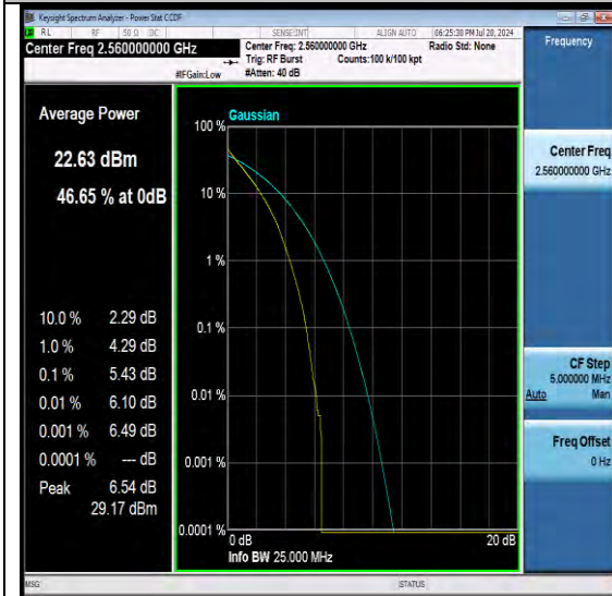
NTNV-N7-PC3-15-20-H-DFT-QPSK-Outer_Full-PA SS
