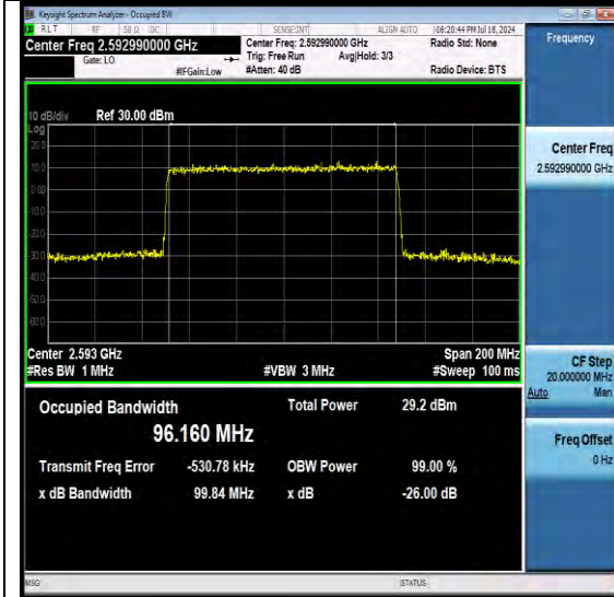
NTNV-N41-PC3-30-100-M-DFT-256QAM-Outer_Full-Ant1-PASS
