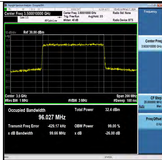
NTNV-N77-3450-3550-PC2-30-100-M-DFT-QPSK -Outer Full-Ant1-PASS
