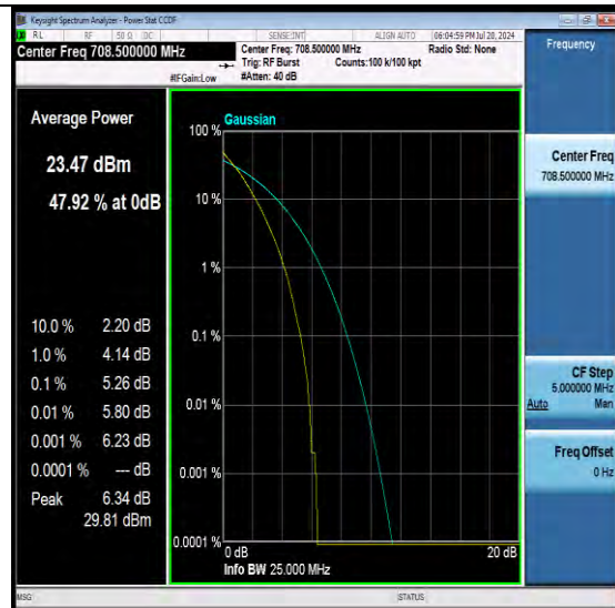
NTNV-N12-PC3-15-15-H-DFT-QPSK-Outer_Full-PASS
