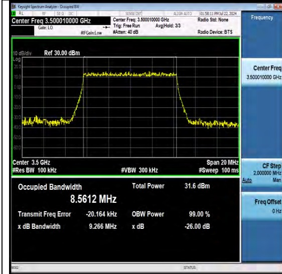
NTNV-N77-3450-3550-PC2-30-10-M-DFT-PI2BPS K-Outer_Full-Ant1-PASS
