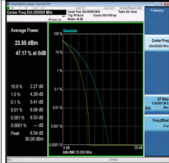
NTNV-N26-824-849-PC3-15-20-L-DFT-QPSK-Outer Full-PASS
