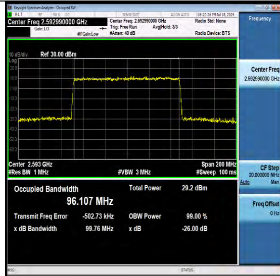
NTNV-N41-PC3-30-100-M-DFT-64QAM-Outer_Ful I-Ant1-PASS
