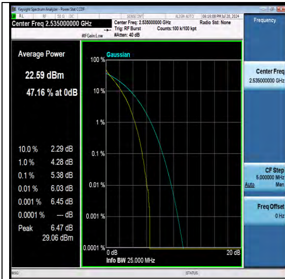
NTNV-N7-PC3-15-20-M-DFT-QPSK-Outer_Full-P ASS
