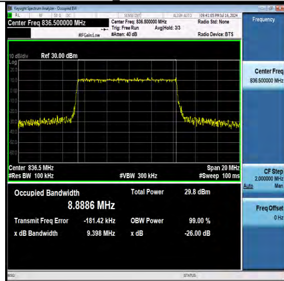
NTNV-N26-824-849-PC3-15-10-M-DFT-16QAM-Out er Full-Ant1-PASS
