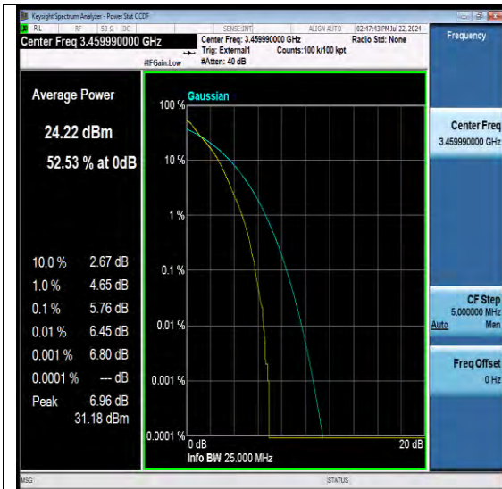
NTNV-N77-3450-3550-PC2-30-20-L-DFT-QPSK-Outer Full-PASS
