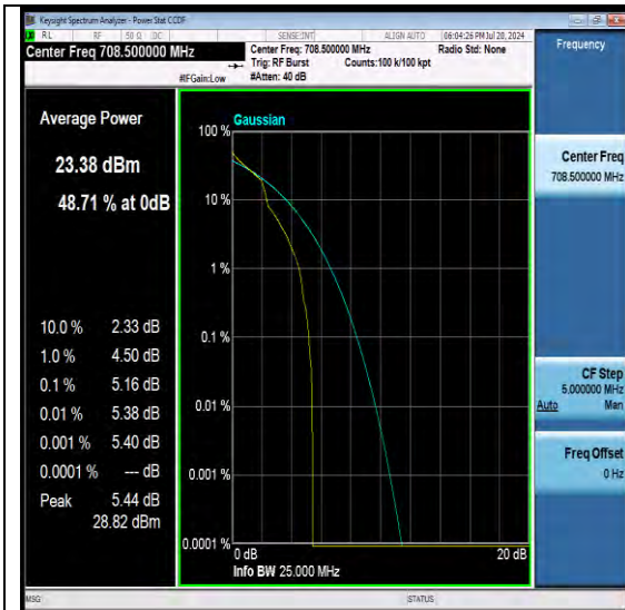
NTNV-N12-PC3-15-15-H-DFT-QPSK-Edge_1RB_Left-PASS
