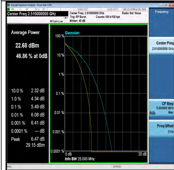
NTNV-N7-PC3-15-20-L-DFT-QPSK-Outer_Full-PASS
