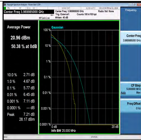
NTNV-N77-3700-3980-PC3-30-20-H-DFT-QPSK-Outer Full-PASS
