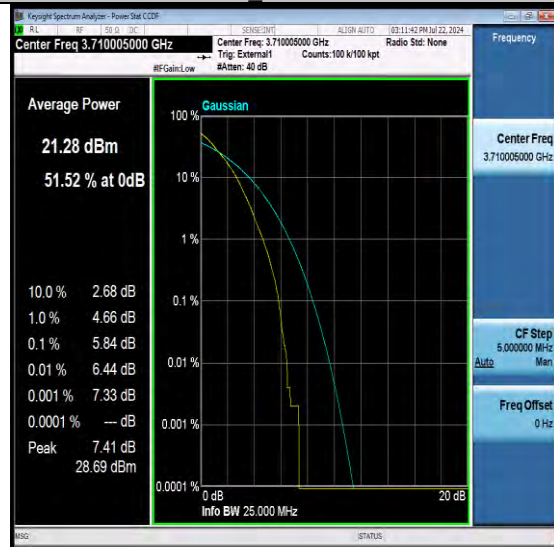
NTNV-N77-3700-3980-PC3-30-20-L-DFT-QPSK-Outer Full-PASS
