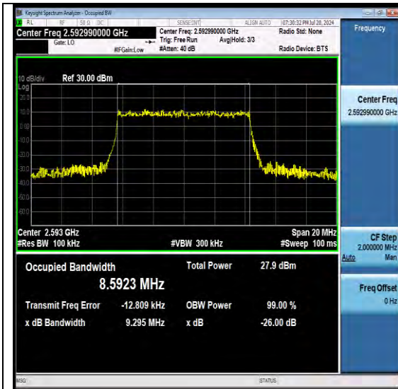
NTNV-N41-PC3-30-10-M-DFT-64QAM-Outer_Full-Ant1-PASS
