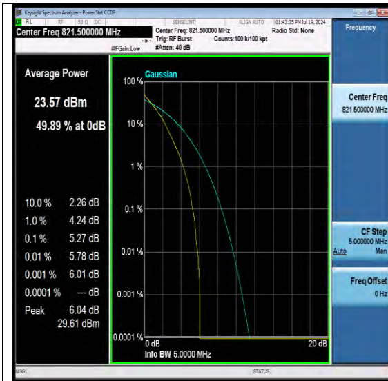
NTNV-N26-814-824-PC3-15-5-H-DFT-QPSK-Outer Full-PASS
