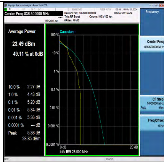
NTNV-N26-824-849-PC3-15-20-M-DFT-QPSK-Ed ge 1RB Left-PASS
