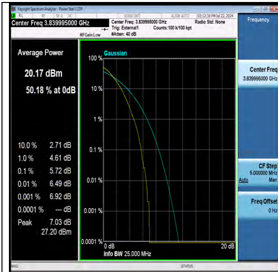
NTNV-N77-3700-3980-PC3-30-20-M-DFT-QPSK-Outer Full-PASS
