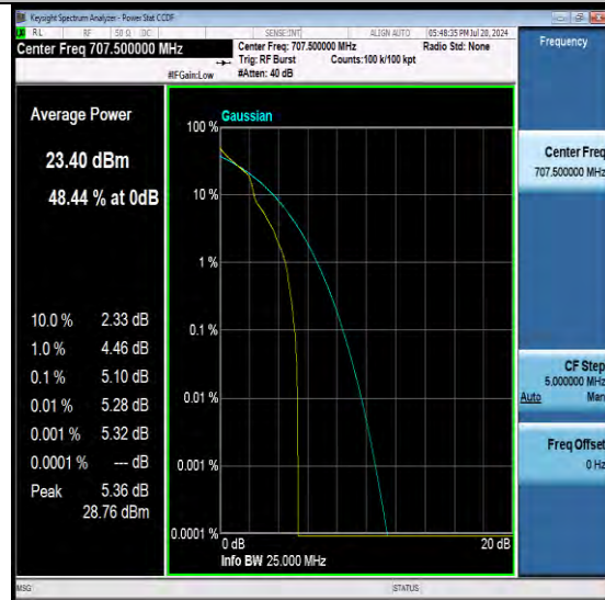
NTNV-N12-PC3-15-15-M-DFT-QPSK-Edge_1RB_Left-PASS
