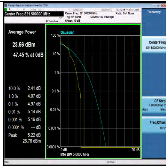
NTNV-N26-814-824-PC3-15-5-H-DFT-QPSK-Edge 1RB Left-PASS
