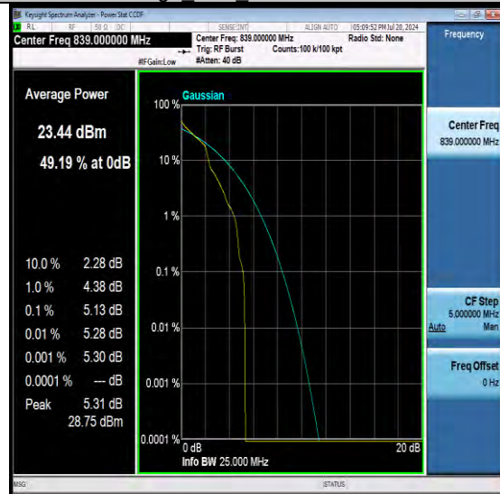
NTNV-N26-824-849-PC3-15-20-H-DFT-QPSK-Ed ge 1RB Left-PASS
