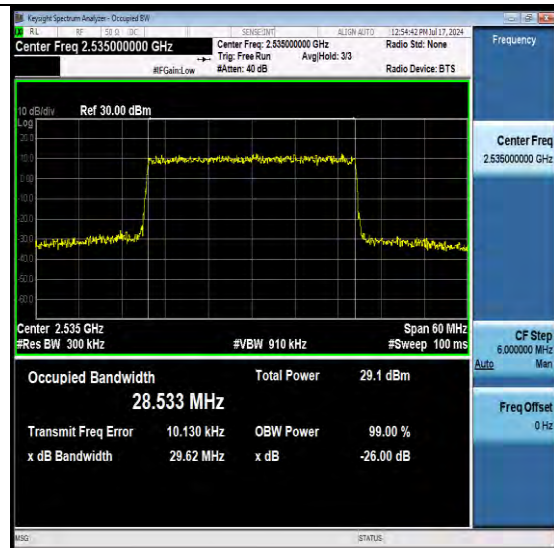
NTNV-N7-PC3-15-30-M-DFT-16QAM-Outer_Ant1-PASS
