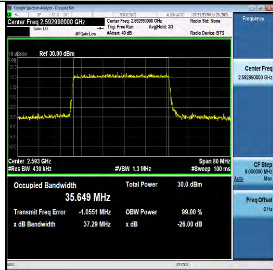
NTNV-N41-PC3-30-40-M-DFT-QPSK-Outer_Full-Ant1-PASS
