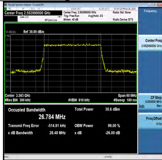
NTNV-N41-PC3-30-30-M-DFT-PI2BPSK-Outer_Fu II-Ant1-PASS
