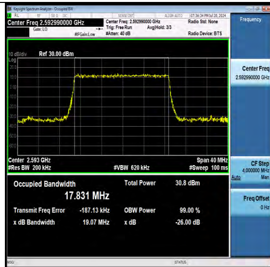
NTNV-N41-PC3-30-20-M-DFT-PI2BPSK-Outer_Fu II-Ant1-PASS
