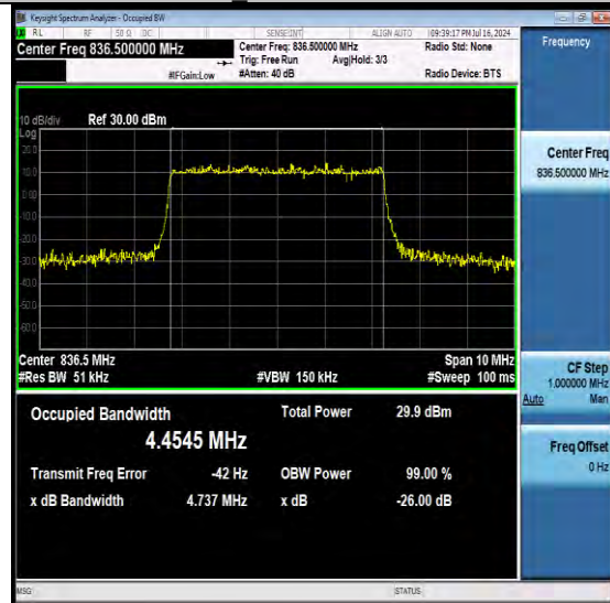
NTN-N26-824-849-PC3-15-5-M-DFT-QPSK-Outer Full-Ant1-PASS
