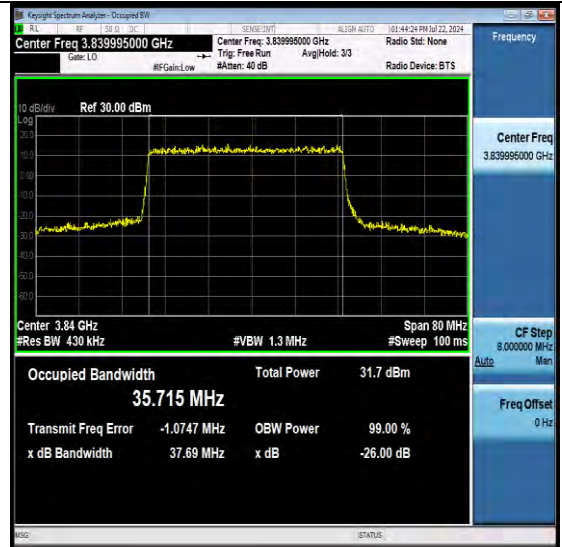
NTNV-N77-3700-3980-PC2-30-40-M-DFT-QPSK- Outer Full-Ant1-PASS
