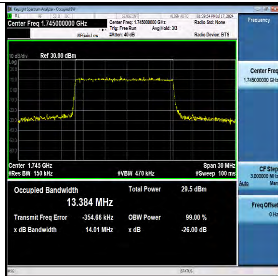
NTNV-N66-PC3-15-15-M-DFT-64QAM-Outer_Full-Ant1-PASS
