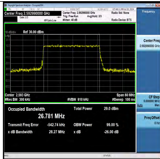
NTNV-N41-PC3-30-30-M-DFT-16QAM-Outer_Full-Ant1-PASS
