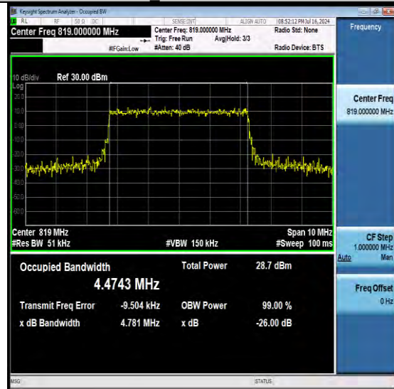
NTNV-N26-814-824-PC3-15-5-M-DFT-16QAM-Ou ter Full-Ant1-PASS
