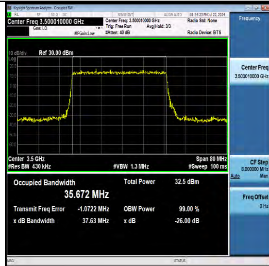
NTNV-N77-3450-3550-PC2-30-40-M-DFT-PI2BPS K-Outer_Full-Ant1-PASS
