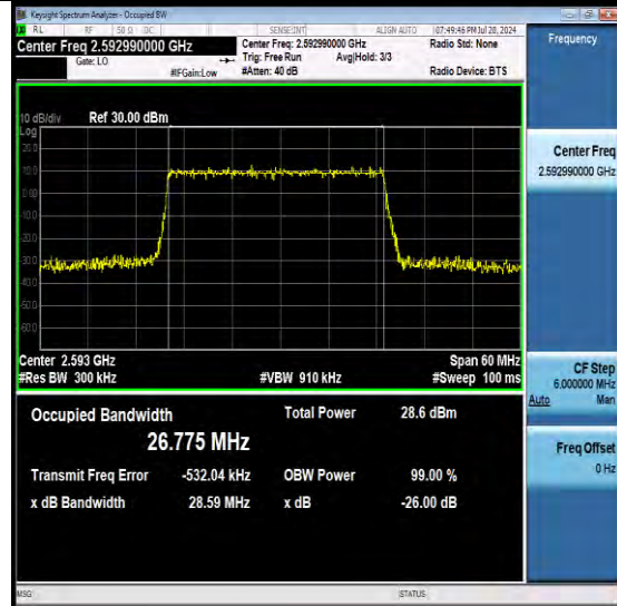
NTNV-N41-PC3-30-30-M-DFT-256QAM-Outer_Full-Ant1-PASS
