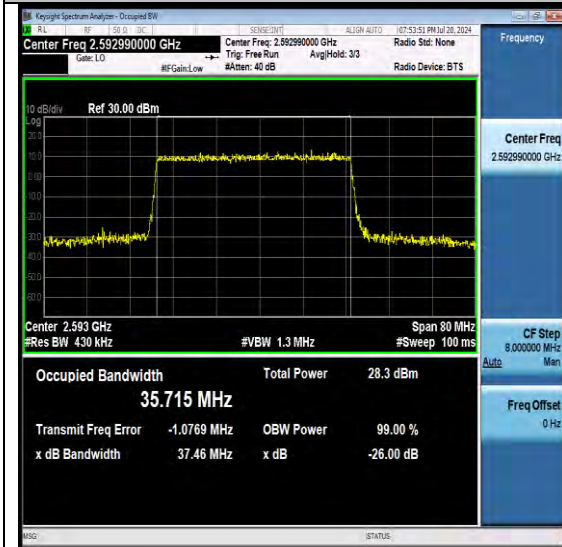
NTNV-N41-PC3-30-40-M-DFT-256QAM-Outer_Full-Ant1-PASS
