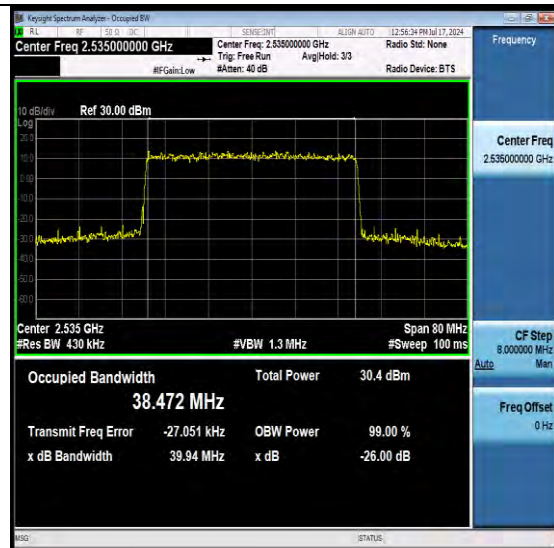
NTNV-N7-PC3-15-40-M-DFT-QPSK-Outer_Full-Ant1-PASS
