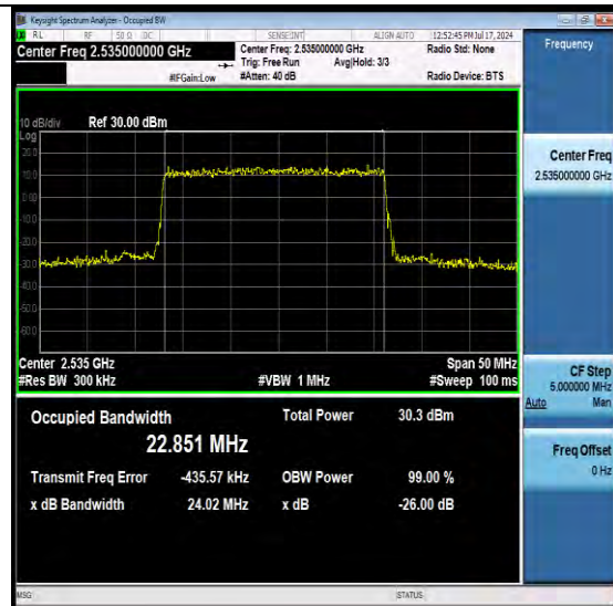
NTNV-N7-PC3-15-25-M-DFT-QPSK-Outer_Full-Ant1-PASS
