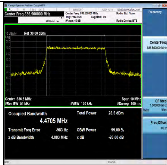
NTNV-N26-824-849-PC3-15-5-M-DFT-64QAM-Outer Full-Ant1-PASS
