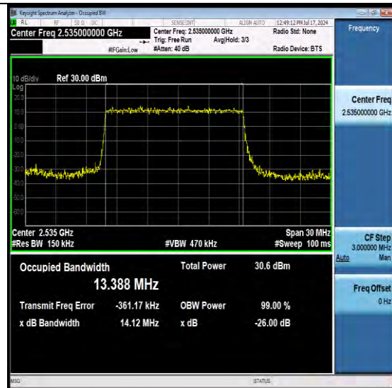
NTNV-N7-PC3-15-15-M-DFT-PI2BPSK-Outer_Full -Ant1-PASS
