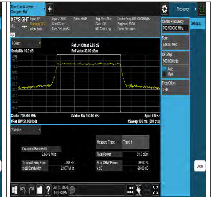
Band12-3MHz-16QAM-23025-15RB#0-PASS
