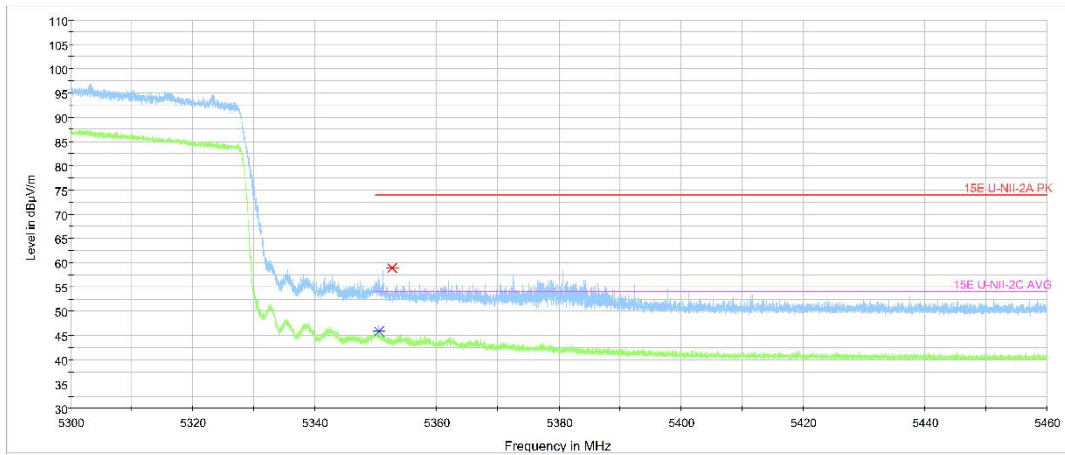
Fig. 22 Band Edges (802.11ac-HT80 Ch58, 5290MHz)
