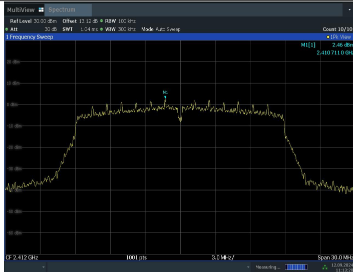
11N20SISO_2412_0~Reference
