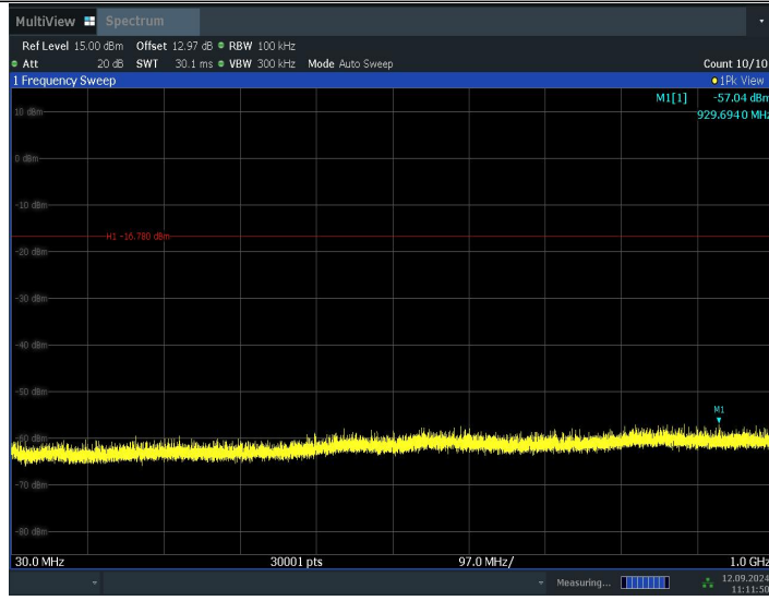
11G_2462_30~1000
