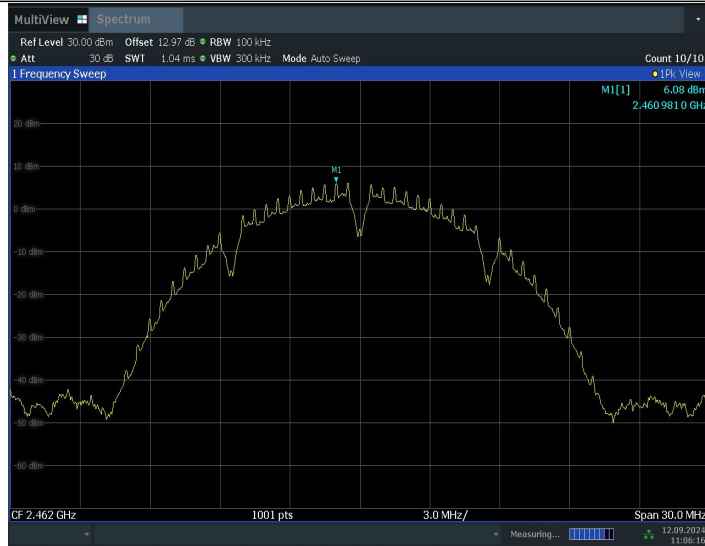
11B_2462_0~Reference
