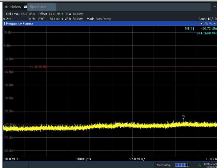
11G_2412_30~1000
