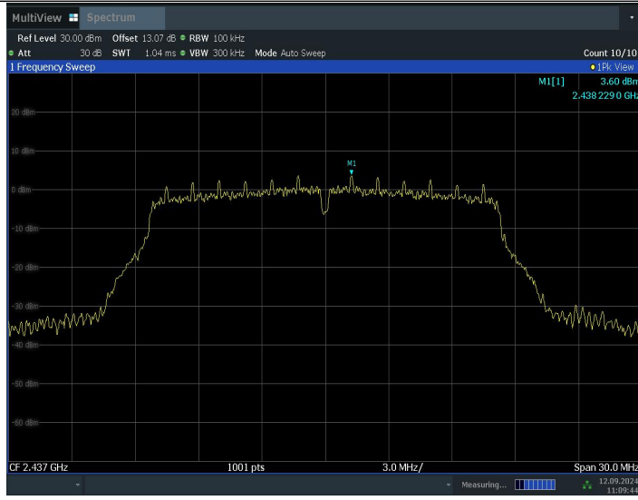
11G_2437_0~Reference
