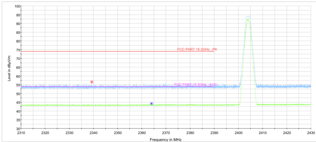
Fig.24. Frequency Band Edges: GFSK, 2404 MHz, Hopping Off, 2.31 GHz – 2.43GHz
