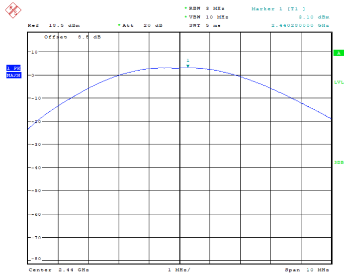
Fig.5. Peak Output Power -Conducted:2Mbps, Channel 19
