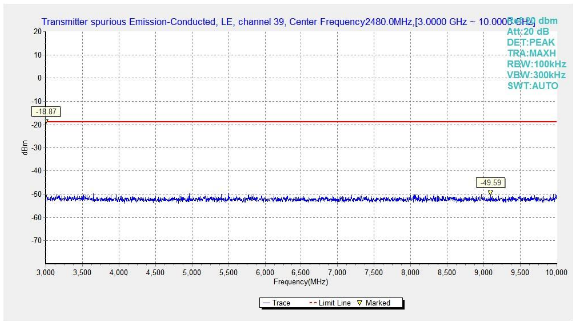
Fig.22. Transmitter Spurious Emission -Conducted:GFSK, 2480 MHz,3GHz - 10GHz
