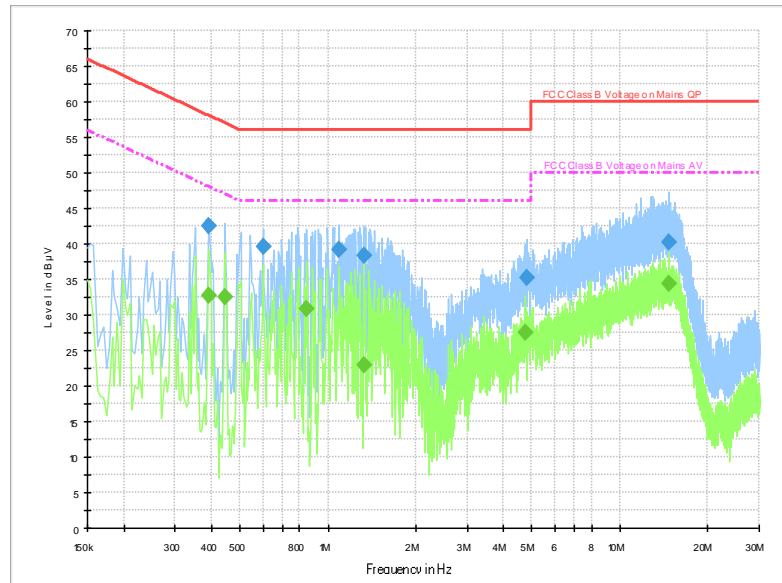
Fig.B.8.2 AC Powerline Conducted Emission-Idle
