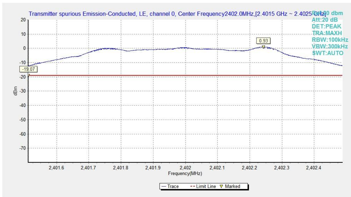
Fig.9. Transmitter Spurious Emission -Conducted: GFSK,2402MHz
