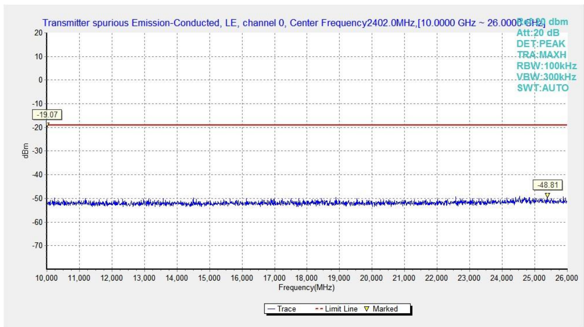
Fig.13. Transmitter Spurious Emission -Conducted: GFSK, 2402 MHz,10GHz - 26GHz
