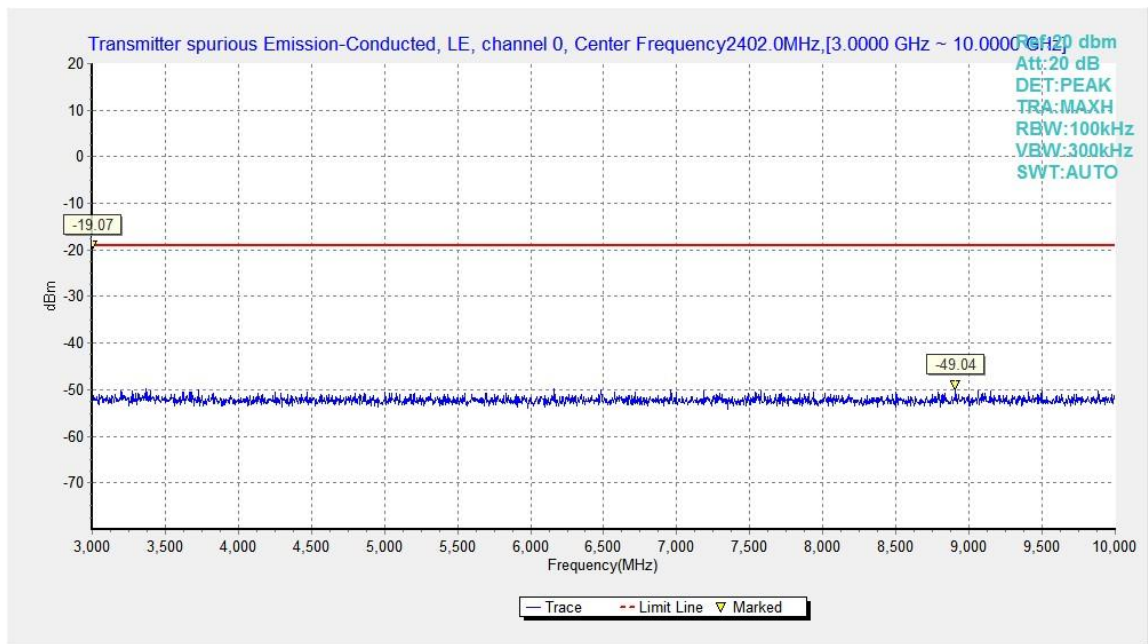
Fig.12. Transmitter Spurious Emission -Conducted: GFSK, 2402 MHz,3GHz - 10GHz
