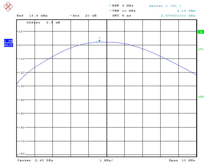
Fig.3. Peak Output Power -Conducted: 1Mbps, Channel 39
