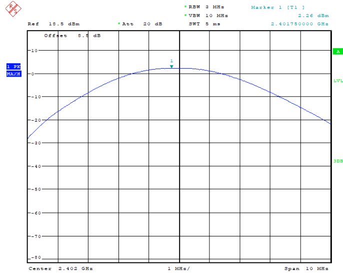
Fig.1. Peak Output Power -Conducted: 1Mbps, Channel 0
