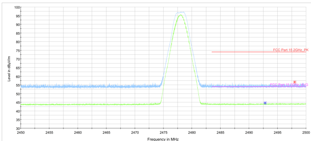
Fig.25. Frequency Band Edges: GFSK, 2478 MHz, Hopping Off, 2.45 GHz - 2.50GHz
