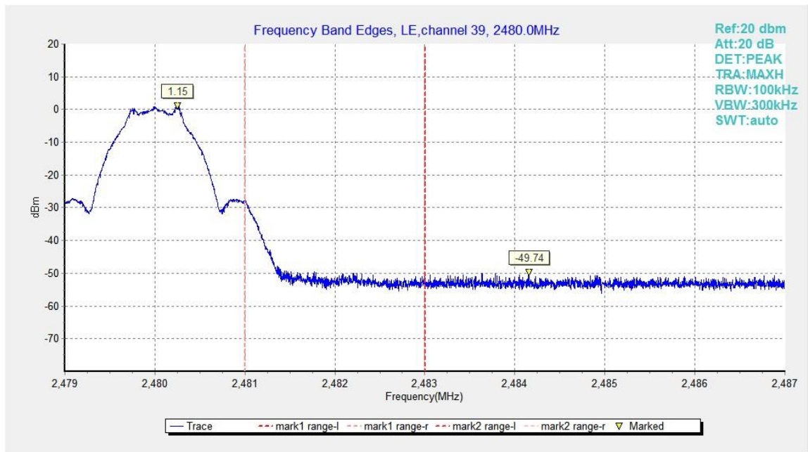
Fig.8. Frequency Band Edges: GFSK, 2480 MHz, Hopping Off
