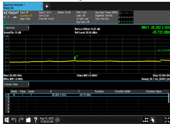
N77(60M)_DFT-s-OFDM_BPSK_Edge_1RB_Left_Mid_CH
