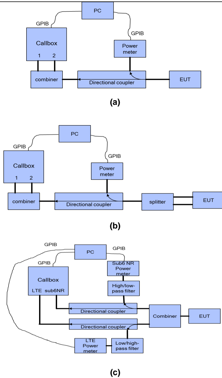
Figure 5-1 Conducted power measurement setup
