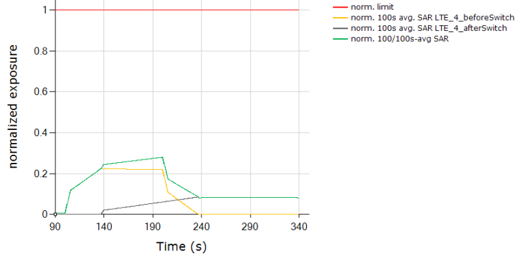
Total Normalized Time-averaged RF Exposure Tech: LTE, Band 4
