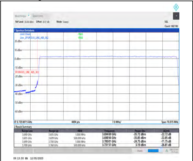
1-N78-3700-3800-PC3-30-60-L-3-DFT-PI2BPSK-Outer_Full-162@0-Ant1-1--PASS-see graph
