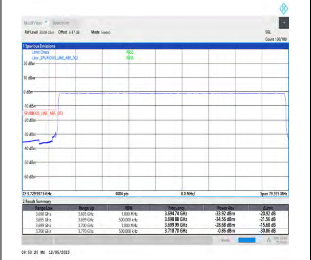
1-N78-3700-3800-PC3-30-70-L-6-CP-QPSK-Outer_Full-189@0-Ant1-1--PASS-see graph
