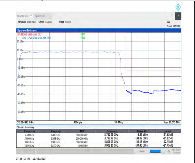
1-N78-3700-3800-PC3-30-20-H-3-DFT-PI2BPSK-Outer_Full-50@0-Ant1-1--PASS-see graph
