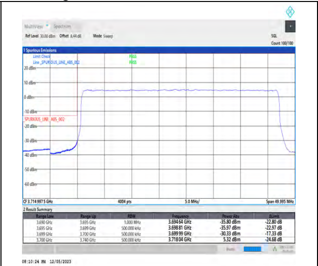
1-N78-3700-3800-PC3-30-40-L-3-DFT-PI2BPSK-Outer_Full-100@0-Ant1-1--PASS-see graph
