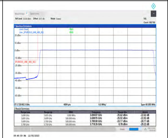
1-N78-3700-3800-PC3-30-50-L-6-CP-QPSK-Outer_Full-133@0-Ant1-1--PASS-see graph
