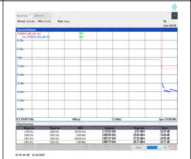
1-N78-3700-3800-PC3-30-100-H-6-CP-QPSK-Outer_Full-273@0-Ant1-1--PASS-see graph
