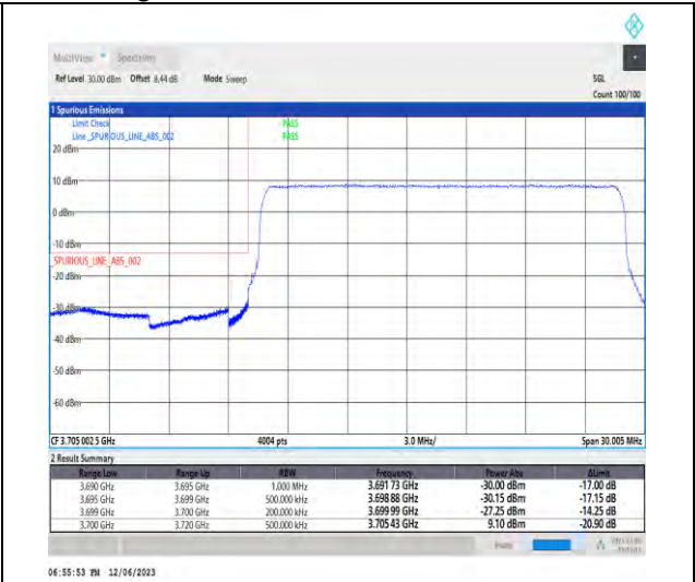
1-N78-3700-3800-PC3-30-20-L-3-DFT-PI2BPSK-Outer_Full-50@0-Ant1-1--PASS-see graph
