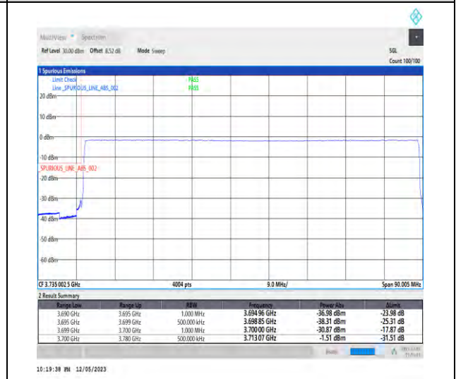
1-N78-3700-3800-PC3-30-80-L-6-CP-QPSK-Outer_Full-217@0-Ant1-1--PASS-see graph
