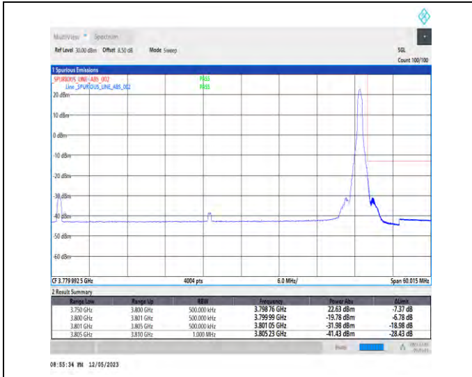
1-N78-3700-3800-PC3-30-50-H-2-DFT-PI2BPSK-Edge_1RB_Right-1@132-Ant1-1--PASS-see graph
