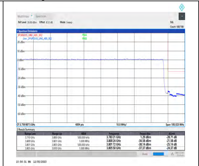
1-N78-3700-3800-PC3-30-90-H-3-DFT-PI2BPSK-Outer_Full-240@0-Ant1-1--PASS-see graph
