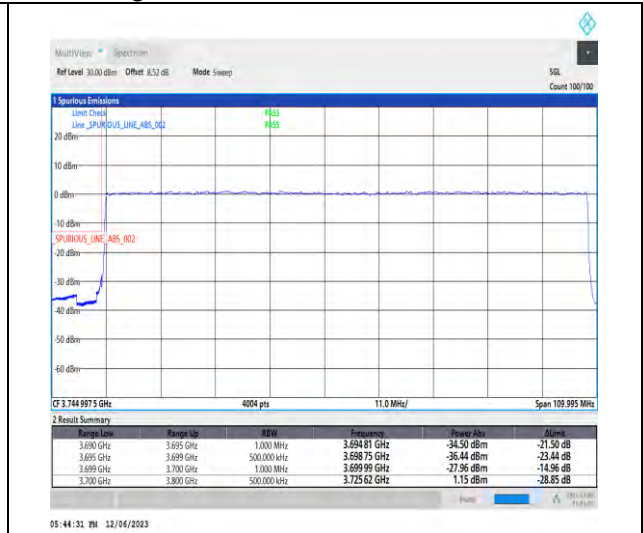
1-N78-3700-3800-PC3-30-100-L-3-DFT-PI2BPSK-Outer_Full-270@0-Ant1-1--PASS-see graph
