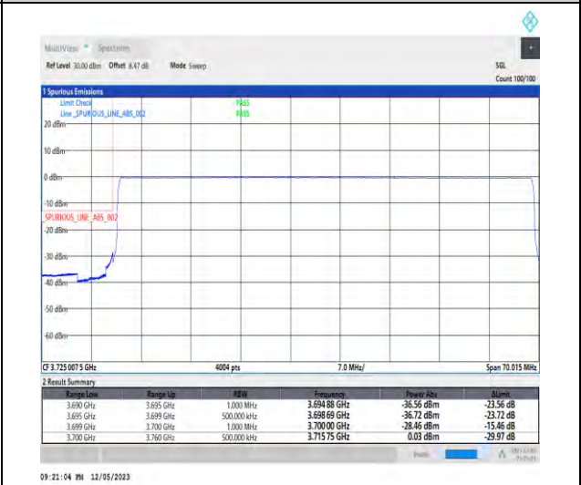
1-N78-3700-3800-PC3-30-60-L-6-CP-QPSK-Outer_Full-162@0-Ant1-1--PASS-see graph
