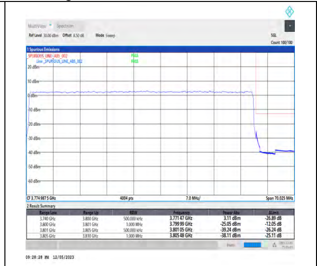
1-N78-3700-3800-PC3-30-60-H-3-DFT-PI2BPSK-Outer_Full-162@0-Ant1-1--PASS-see graph
