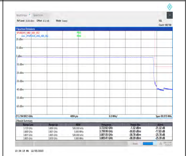
1-N78-3700-3800-PC3-30-80-H-6-CP-QPSK-Outer_Full-217@0-Ant1-1--PASS-see graph
