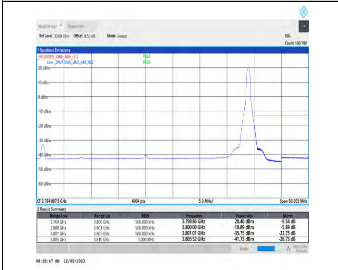
1-N78-3700-3800-PC3-30-40-H-5-CP-QPSK-Edge_1RB_Right-1@105-Ant1-1--PASS-see graph
