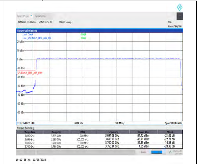
1-N78-3700-3800-PC3-30-80-L-3-DFT-PI2BPSK-Outer_Full-216@0-Ant1-1--PASS-see graph
