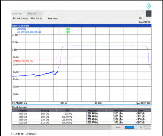
1-N78-3700-3800-PC3-30-20-L-6-CP-QPSK-Outer_Full-51@0-Ant1-1--PASS-see graph
