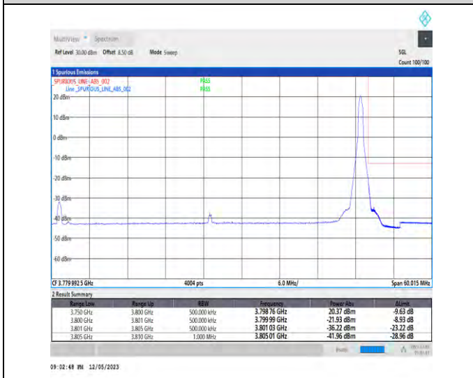
1-N78-3700-3800-PC3-30-50-H-5-CP-QPSK-Edge_1RB_Right-1@132-Ant1-1--PASS-see graph
