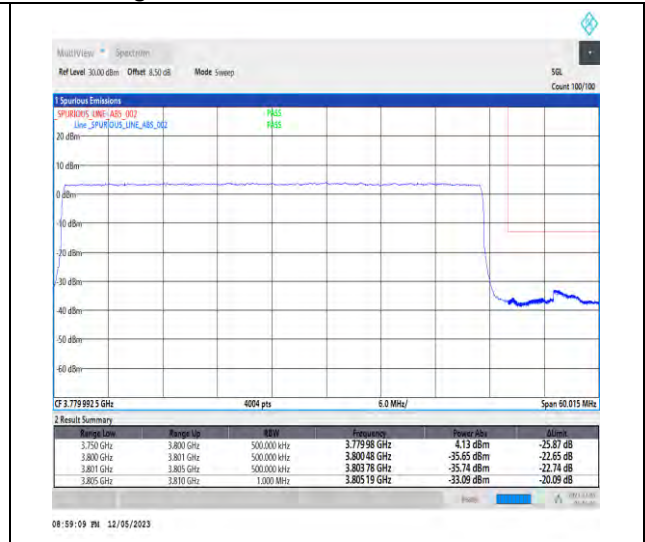
1-N78-3700-3800-PC3-30-50-H-3-DFT-PI2BPSK-Outer_Full-128@0-Ant1-1--PASS-see graph
