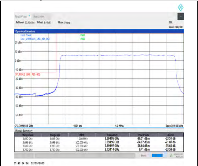
1-N78-3700-3800-PC3-30-30-L-3-DFT-PI2BPSK-Outer_Full-75@0-Ant1-1--PASS-see graph
