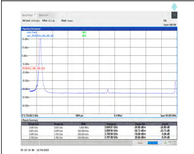
1-N78-3700-3800-PC3-30-80-L-4-CP-QPSK-Edge_1RB_Left-1@0-Ant1-1--PASS-see graph
