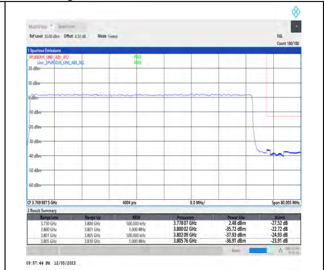
1-N78-3700-3800-PC3-30-70-H-3-DFT-PI2BPSK-Outer_Full-180@0-Ant1-1--PASS-see graph
