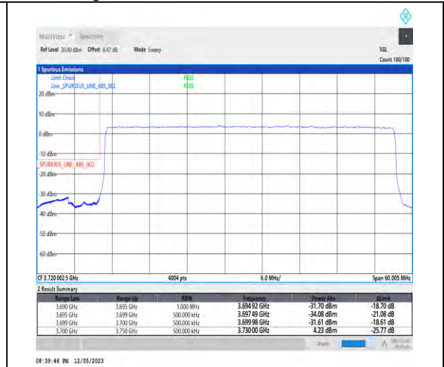
1-N78-3700-3800-PC3-30-50-L-3-DFT-PI2BPSK-Outer_Full-128@0-Ant1-1--PASS-see graph
