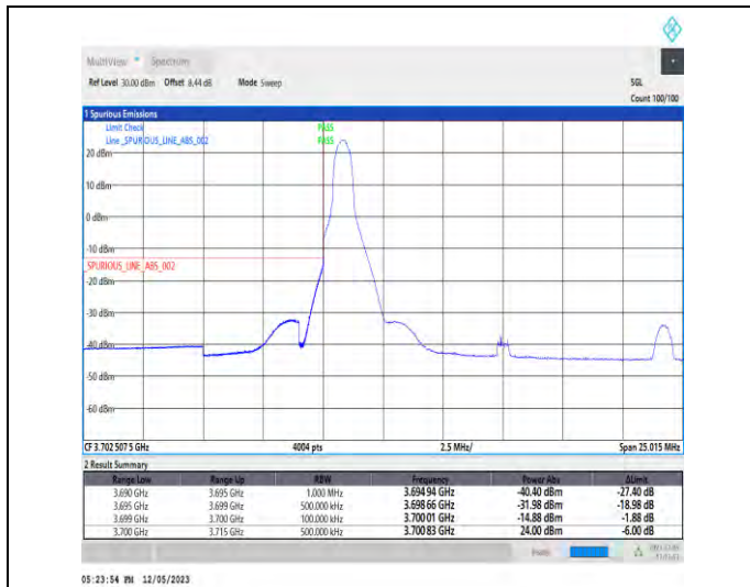
1-N78-3700-3800-PC3-30-15-L-1-DFT-PI2BPSK-Edge_1RB_Left-1@0-Ant1-1--PASS-see graph
