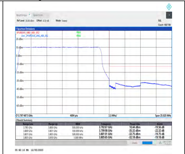
1-N78-3700-3800-PC3-30-15-H-3-DFT-PI2BPSK-Outer_Full-36@0-Ant1-1--PASS-see graph
