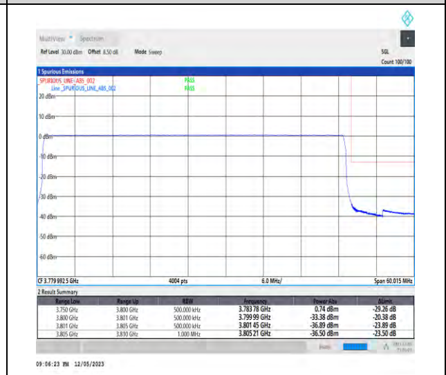
1-N78-3700-3800-PC3-30-50-H-6-CP-QPSK-Outer_Full-133@0-Ant1-1--PASS-see graph
