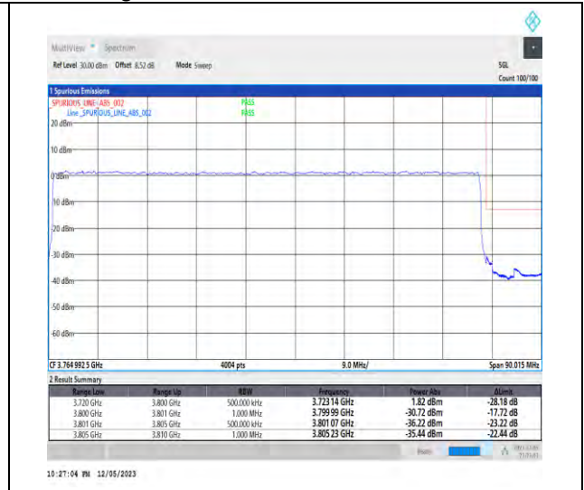
1-N78-3700-3800-PC3-30-80-H-3-DFT-PI2BPSK-Outer_Full-216@0-Ant1-1--PASS-see graph
