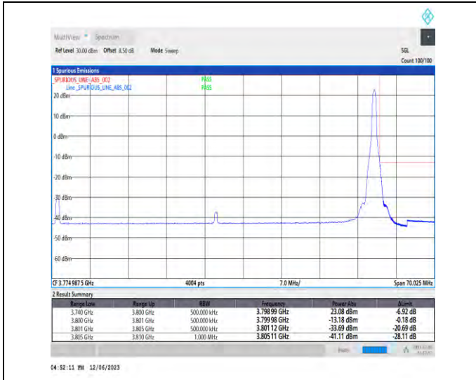
1-N78-3700-3800-PC3-30-60-H-2-DFT-PI2BPSK-Edge_1RB_Right-1@161-Ant1-1--PASS-see graph
