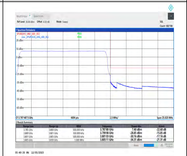
1-N78-3700-3800-PC3-30-15-H-6-CP-QPSK-Outer_Full-38@0-Ant1-1--PASS-see graph
