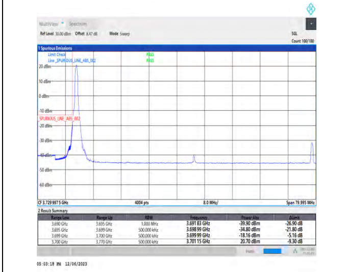
1-N78-3700-3800-PC3-30-70-L-4-CP-QPSK-Edge_1RB_Left-1@0-Ant1-1--PASS-see graph
