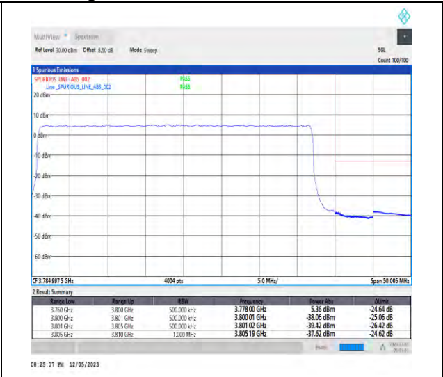
1-N78-3700-3800-PC3-30-40-H-3-DFT-PI2BPSK-Outer_Full-100@0-Ant1-1--PASS-see graph
