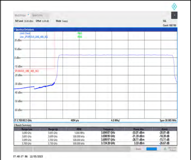
1-N78-3700-3800-PC3-30-30-L-6-CP-QPSK-Outer_Full-78@0-Ant1-1--PASS-see graph
