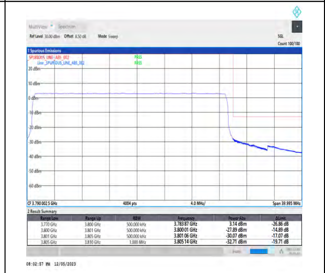
1-N78-3700-3800-PC3-30-30-H-6-CP-QPSK-Outer_Full-78@0-Ant1-1--PASS-see graph
