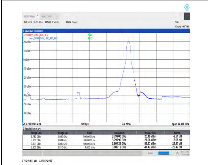
1-N78-3700-3800-PC3-30-20-H-5-CP-QPSK-Edge_1RB_Right-1@50-Ant1-1--PASS-see graph
