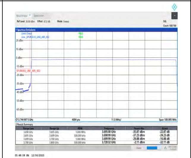
1-N78-3700-3800-PC3-30-100-L-6-CP-QPSK-Outer_Full-273@0-Ant1-1--PASS-see graph
