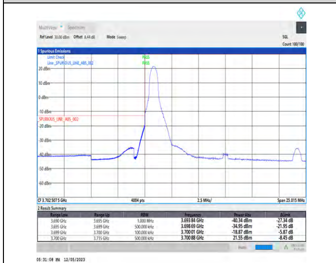
1-N78-3700-3800-PC3-30-15-L-4-CP-QPSK-Edge_1RB_Left-1@0-Ant1-1--PASS-see graph
