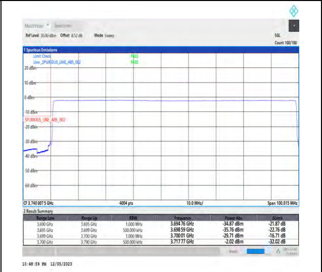
1-N78-3700-3800-PC3-30-90-L-6-CP-QPSK-Outer_Full-245@0-Ant1-1--PASS-see graph
