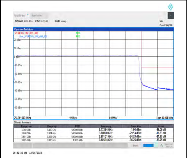
1-N78-3700-3800-PC3-30-40-H-6-CP-QPSK-Outer_Full-106@0-Ant1-1--PASS-see graph
