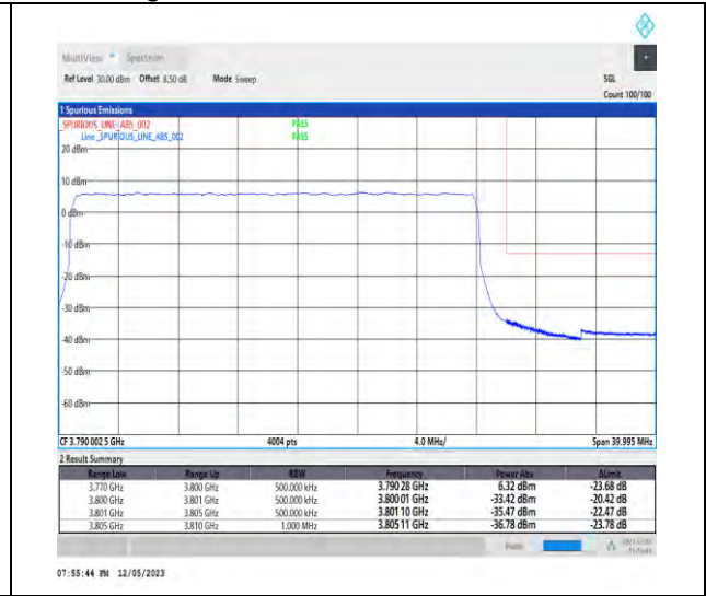
1-N78-3700-3800-PC3-30-30-H-3-DFT-PI2BPSK-Outer_Full-75@0-Ant1-1--PASS-see graph
