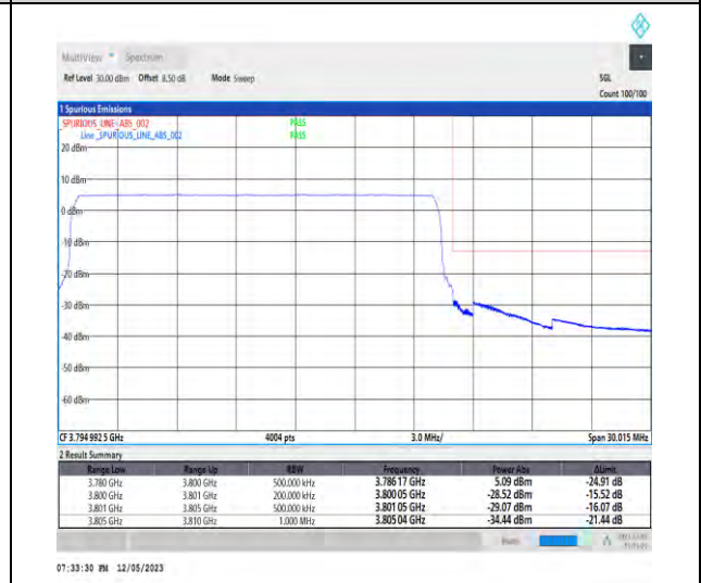
1-N78-3700-3800-PC3-30-20-H-6-CP-QPSK-Outer_Full-51@0-Ant1-1--PASS-see graph
