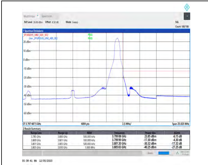
1-N78-3700-3800-PC3-30-15-H-2-DFT-PI2BPSK-Edge_1RB_Right-1@37-Ant1-1--PASS-see graph
