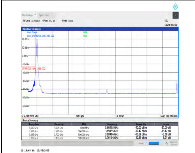
1-N78-3700-3800-PC3-30-100-L-4-CP-QPSK-Edge_1_RB_Left-1@0-Ant1-1--PASS-see graph
