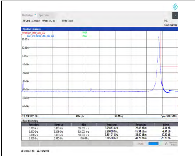
1-N78-3700-3800-PC3-30-80-H-2-DFT-PI2BPSK-Edge_1RB_Right-1@216-Ant1-1--PASS-see graph
