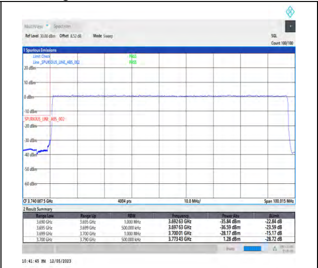
1-N78-3700-3800-PC3-30-90-L-3-DFT-PI2BPSK-Outer_Full-240@0-Ant1-1--PASS-see graph
