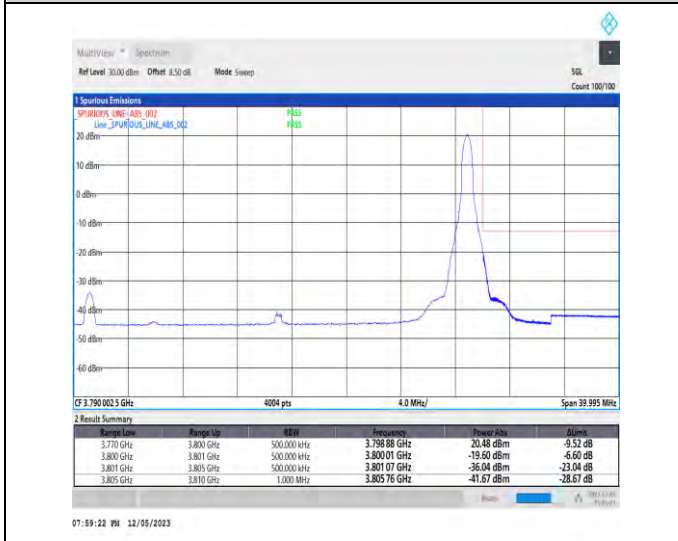
1-N78-3700-3800-PC3-30-30-H-5-CP-QPSK-Edge_1RB_Right-1@77-Ant1-1--PASS-see graph
