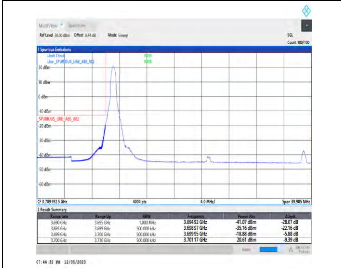
1-N78-3700-3800-PC3-30-30-L-4-CP-QPSK-Edge_1RB_Left-1@0-Ant1-1--PASS-see graph
