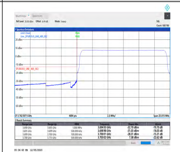
1-N78-3700-3800-PC3-30-15-L-6-CP-QPSK-Outer_Full-38@0-Ant1-1--PASS-see graph
