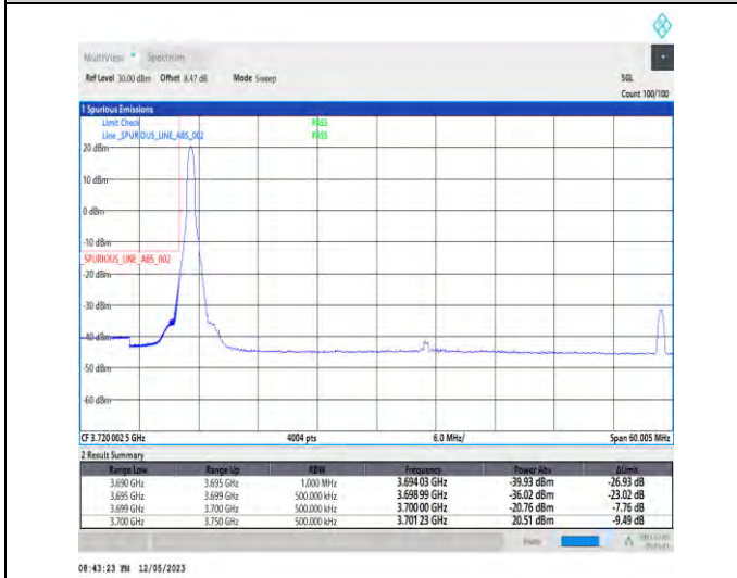
1-N78-3700-3800-PC3-30-50-L-4-CP-QPSK-Edge_1RB_Left-1@0-Ant1-1--PASS-see graph
