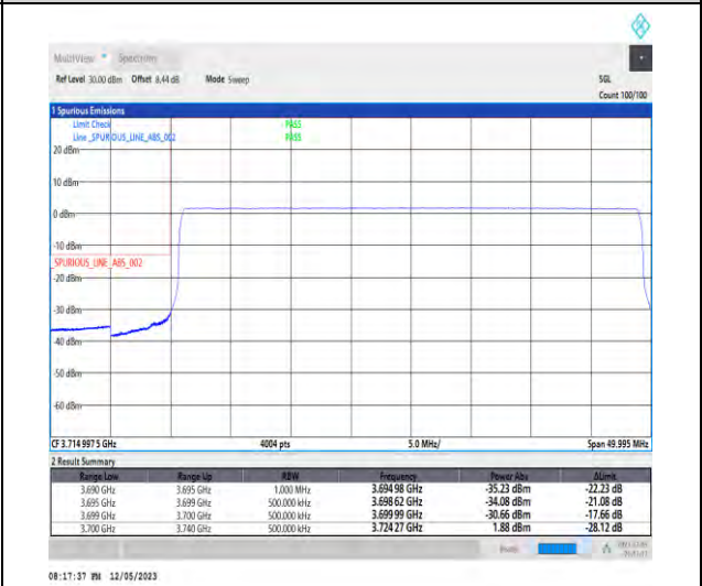
1-N78-3700-3800-PC3-30-40-L-6-CP-QPSK-Outer_Full-106@0-Ant1-1--PASS-see graph
