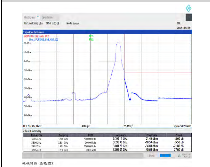
1-N78-3700-3800-PC3-30-15-H-5-CP-QPSK-Edge_1RB_Right-1@37-Ant1-1--PASS-see graph
