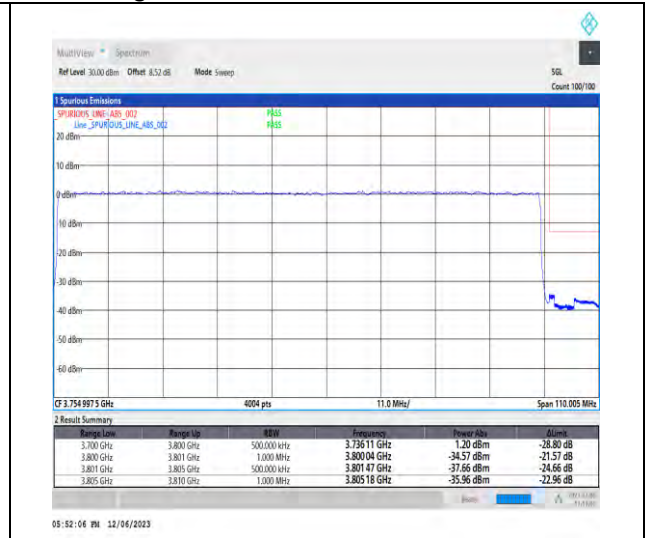
1-N78-3700-3800-PC3-30-100-H-3-DFT-PI2BPSK-Outer_Full-270@0-Ant1-1--PASS-see graph
