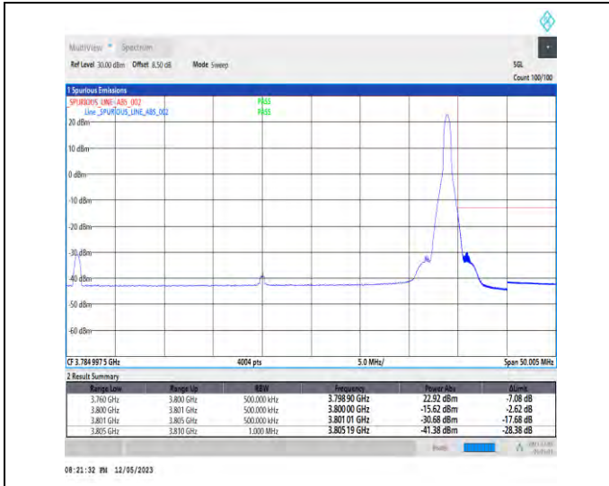
1-N78-3700-3800-PC3-30-40-H-2-DFT-PI2BPSK-Edge_1RB_Right-1@105-Ant1-1--PASS-see graph
