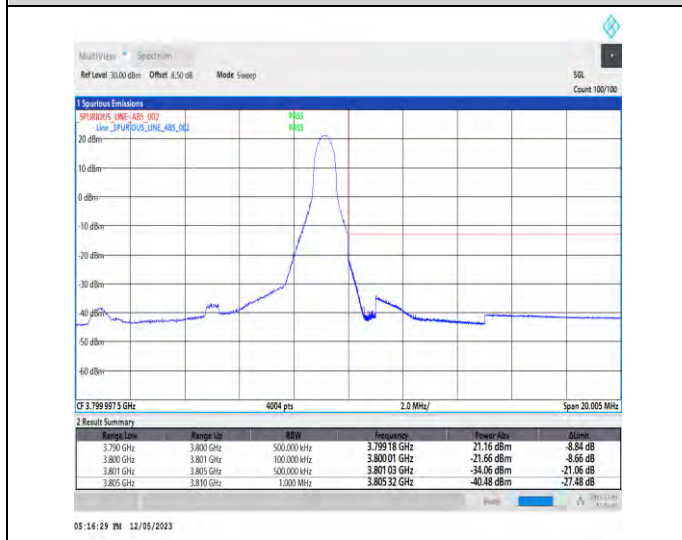
1-N78-3700-3800-PC3-30-10-H-5-CP-QPSK-Edge_1RB_Right-1@23-Ant1-1--PASS-see graph
