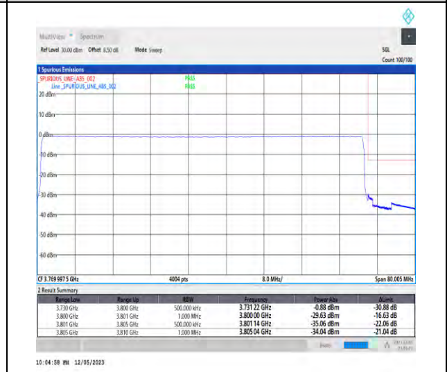
1-N78-3700-3800-PC3-30-70-H-6-CP-QPSK-Outer_Full-189@0-Ant1-1--PASS-see graph
