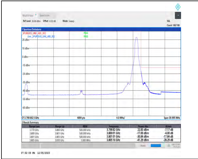
1-N78-3700-3800-PC3-30-30-H-2-DFT-PI2BPSK-Edge_1RB_Right-1@77-Ant1-1--PASS-see graph
