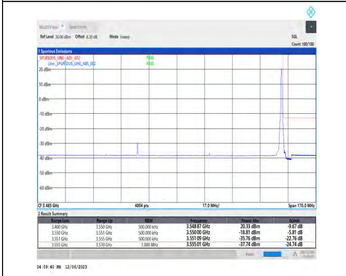
1-N78-3450-3550-PC3-30-90-H-5-CP-QPSK-Edge_1RB_Right-1@244-Ant1-1--PASS-see graph
