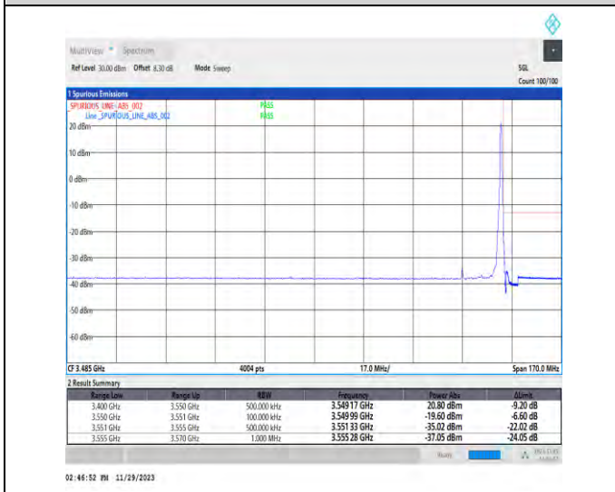
1-N78-3450-3550-PC3-30-15-H-5-CP-QPSK-Edge_1RB_Right-1@37-Ant1-1--PASS-see graph
