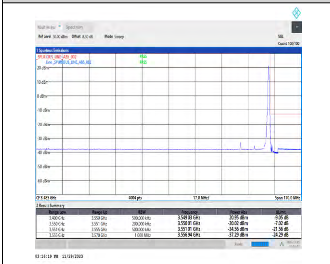
1-N78-3450-3550-PC3-30-20-H-5-CP-QPSK-Edge_1R_B_Right-1@50-Ant1-1--PASS-see graph
