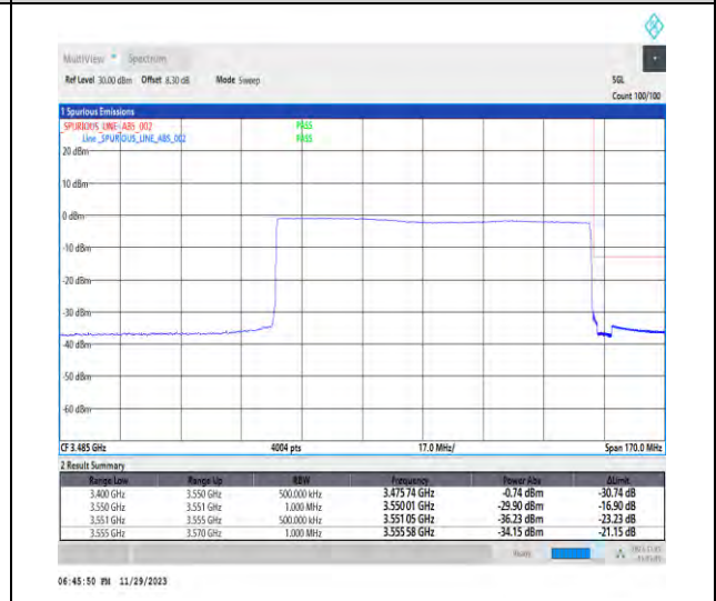
1-N78-3450-3550-PC3-30-90-H-6-CP-QPSK-Outer_Full-245@0-Ant1-1--PASS-see graph
