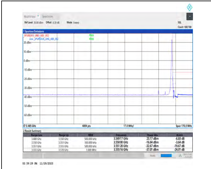
1-N78-3450-3550-PC3-30-15-H-2-DFT-PI2BPSK-Edge_1RB_Right-1@37-Ant1-1--PASS-see graph
