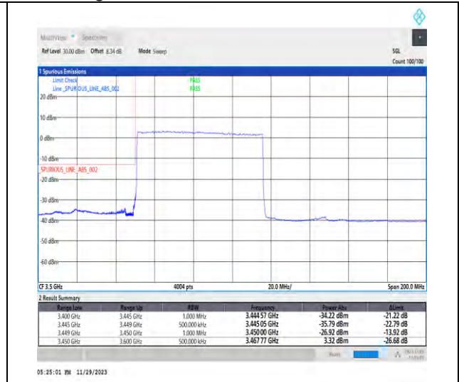
1-N78-3450-3550-PC3-30-70-L-3-DFT-PI2BPSK-Outer_Full-180@0-Ant1-1--PASS-see graph
