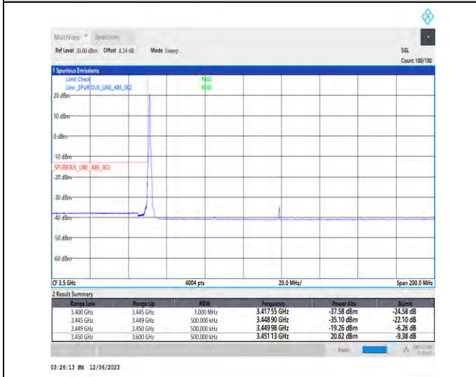
1-N78-3450-3550-PC3-30-70-L-4-CP-QPSK-Edge_1RB_Left-1@0-Ant1-1--PASS-see graph
