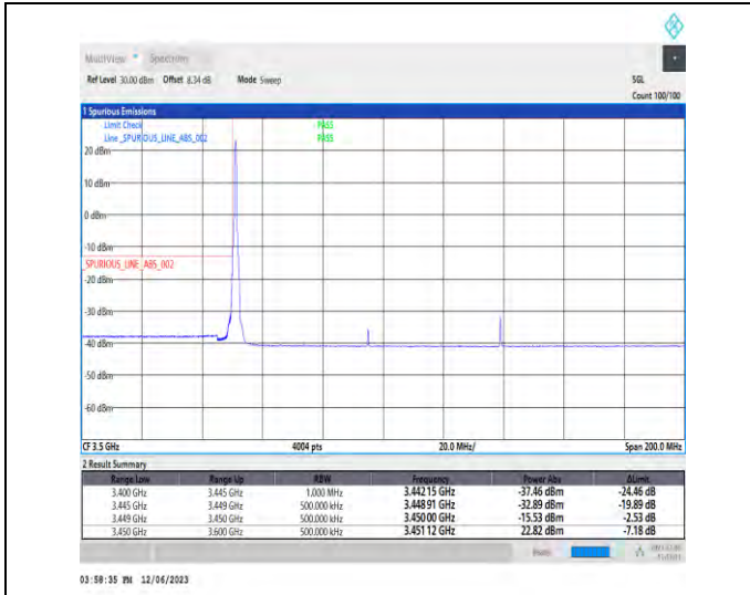
1-N78-3450-3550-PC3-30-90-L-1-DFT-PI2BPSK-Edge_1RB_Left-1@0-Ant1-1--PASS-see graph
