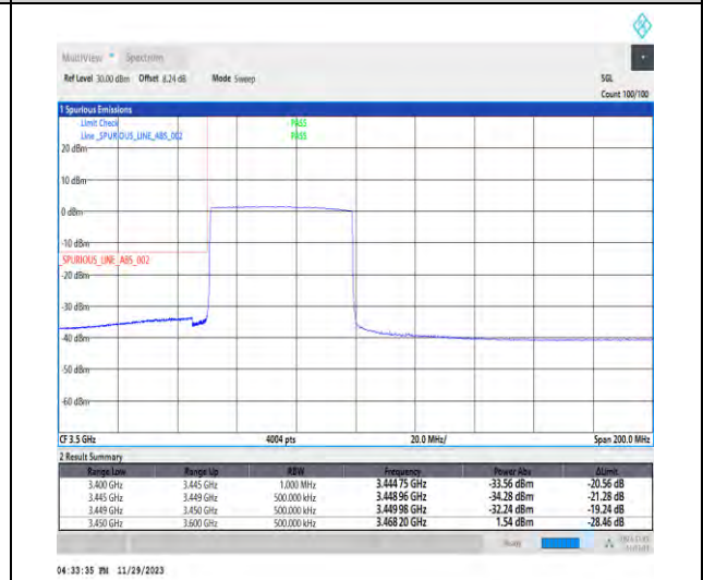
1-N78-3450-3550-PC3-30-50-L-6-CP-QPSK-Outer_Full-133@0-Ant1-1--PASS-see graph
