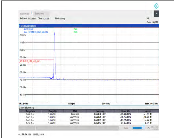
1-N78-3450-3550-PC3-30-15-L-1-DFT-PI2BPSK-Edge_1RB_Left-1@0-Ant1-1--PASS-see graph
