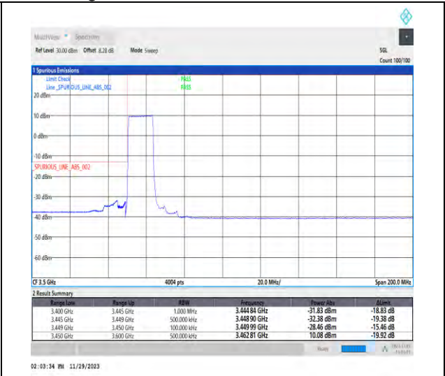
1-N78-3450-3550-PC3-30-15-L-3-DFT-PI2BPSK-Outer_Full-36@0-Ant1-1--PASS-see graph
