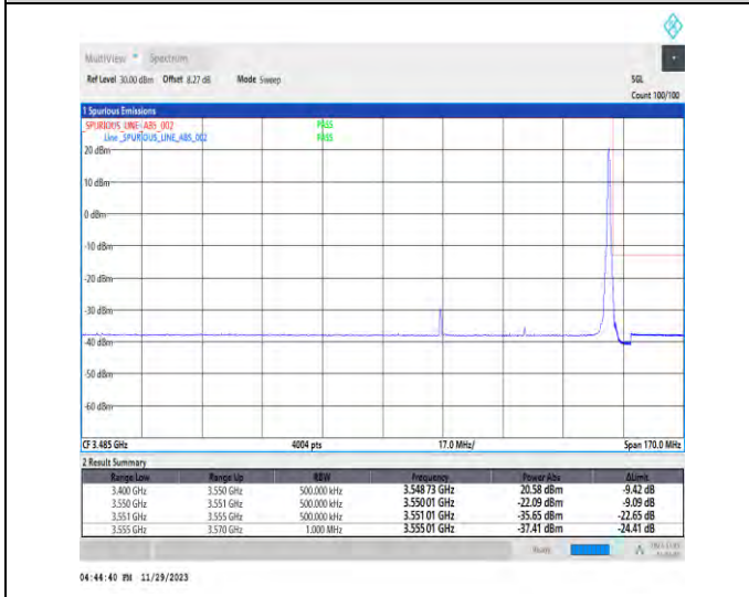
1-N78-3450-3550-PC3-30-50-H-5-CP-QPSK-Edge_1RB_Right-1@132-Ant1-1--PASS-see graph
