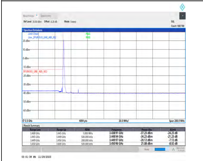
1-N78-3450-3550-PC3-30-20-L-4-CP-QPSK-Edge_1RB_Left-1@0-Ant1-1--PASS-see graph
