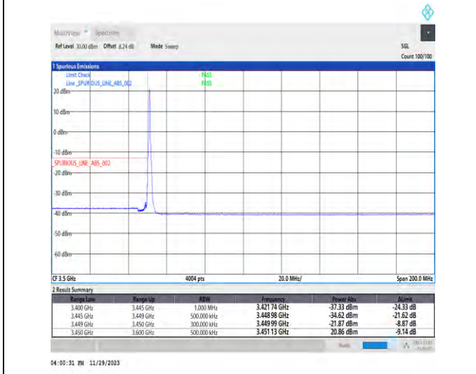
1-N78-3450-3550-PC3-30-40-L-4-CP-QPSK-Edge_1RB_Left-1@0-Ant1-1--PASS-see graph
