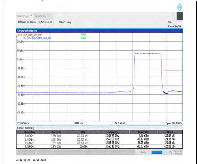
1-N78-3450-3550-PC3-30-30-H-3-DFT-PI2BPSK-Outer_Full-75@0-Ant1-1--PASS-see graph
