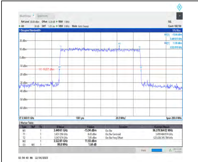
1-N78-3450-3550-PC3-30-100-M-3-DFT-16QAM-Out er_Full-270@0-Ant1-96.378-99.800-≤100-PASS
