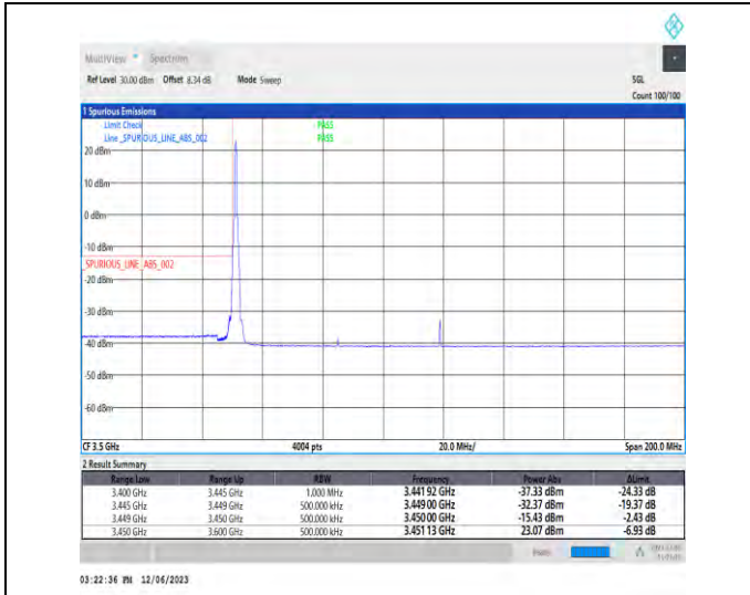
1-N78-3450-3550-PC3-30-70-L-1-DFT-PI2BPSK-Edge_1RB_Left-1@0-Ant1-1--PASS-see graph
