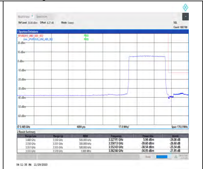
1-N78-3450-3550-PC3-30-40-H-3-DFT-PI2BPSK-Outer_Full-100@0-Ant1-1--PASS-see graph
