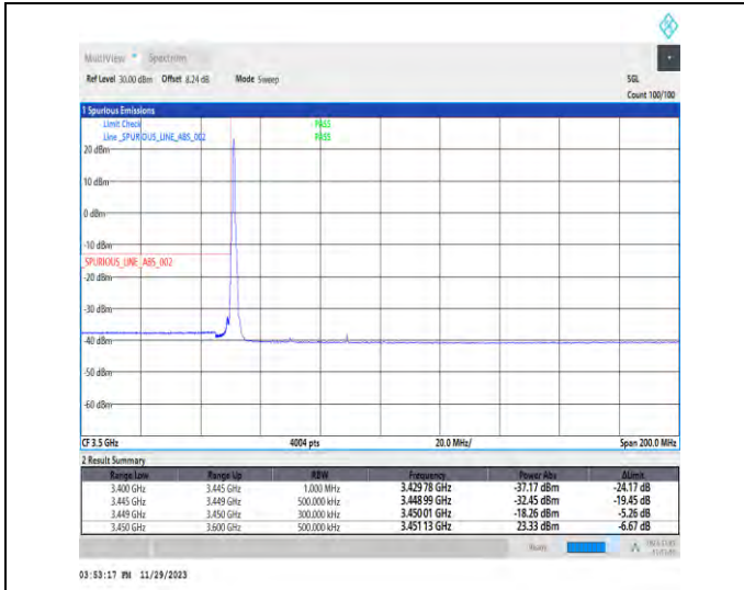
1-N78-3450-3550-PC3-30-40-L-1-DFT-PI2BPSK-Edge_1RB_Left-1@0-Ant1-1--PASS-see graph
