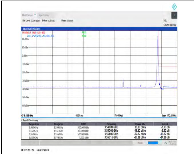
1-N78-3450-3550-PC3-30-40-H-2-DFT-PI2BPSK-Edge_1RB_Right-1@105-Ant1-1--PASS-see graph
