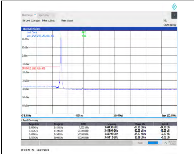
1-N78-3450-3550-PC3-30-30-L-1-DFT-PI2BPSK-Edge_1RB_Left-1@0-Ant1-1--PASS-see graph
