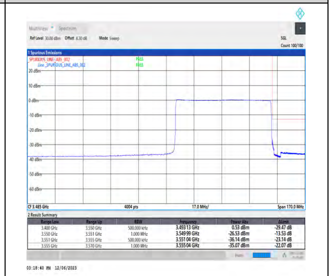
1-N78-3450-3550-PC3-30-60-H-6-CP-QPSK-Outer_Full-162@0-Ant1-1--PASS-see graph
