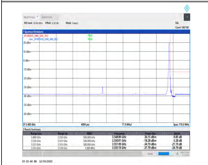
1-N78-3450-3550-PC3-30-70-H-5-CP-QPSK-Edge_1RB_Right-1@188-Ant1-1--PASS-see graph
