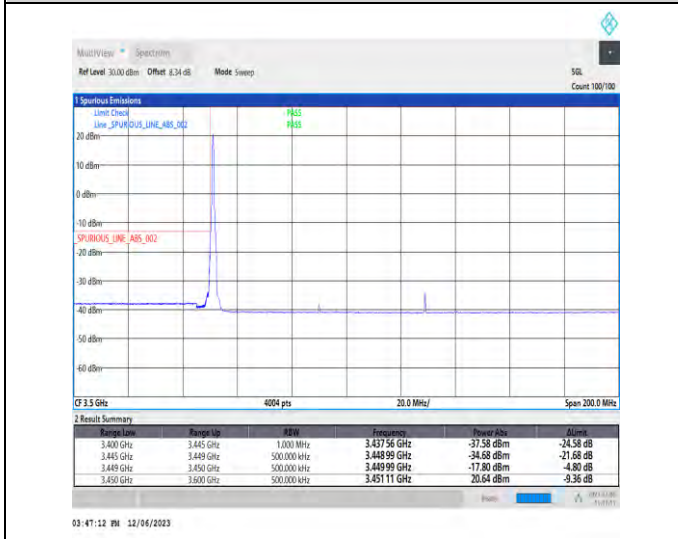
1-N78-3450-3550-PC3-30-80-L-4-CP-QPSK-Edge_1RB_Left-1@0-Ant1-1--PASS-see graph
