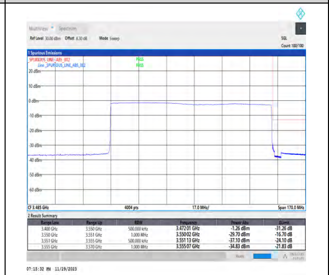
1-N78-3450-3550-PC3-30-100-H-6-CP-QPSK-Outer_Full-273@0-Ant1-1--PASS-see graph
