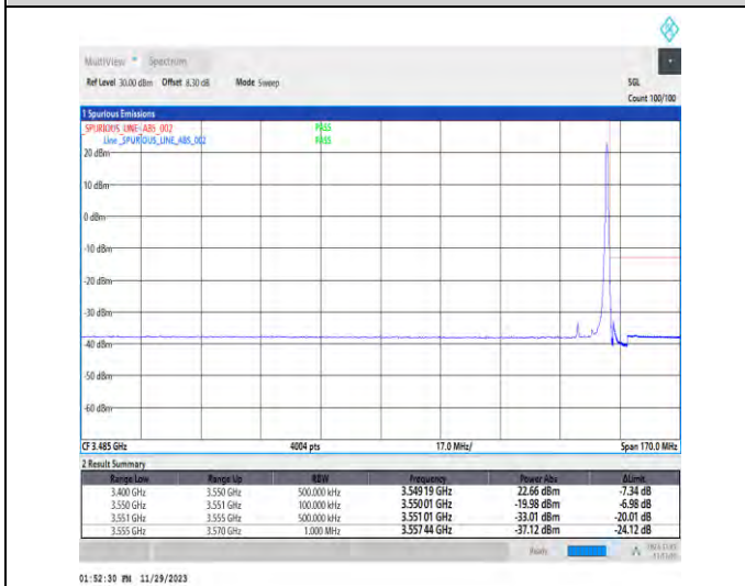
1-N78-3450-3550-PC3-30-10-H-5-CP-QPSK-Edge_1RB_Right-1@23-Ant1-1--PASS-see graph
