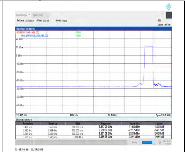
1-N78-3450-3550-PC3-30-10-H-3-DFT-PI2BPSK-Outer_Full-24@0-Ant1-1--PASS-see graph
