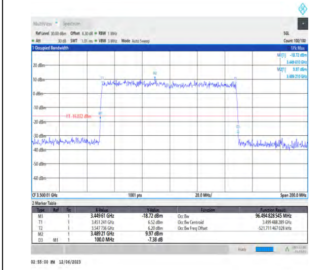
1-N78-3450-3550-PC3-30-100-M-5-DFT-256QAM-Out er_Full-270@0-Ant1-96.495-100.000-≤100-PASS
