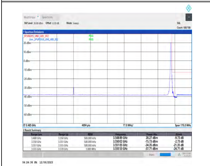
1-N78-3450-3550-PC3-30-100-H-5-CP-QPSK-Edge_1_RB_Right-1@272-Ant1-1--PASS-see graph
