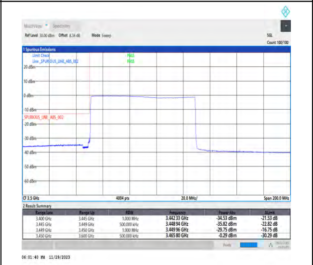
1-N78-3450-3550-PC3-30-80-L-6-CP-QPSK-Outer_Full-217@0-Ant1-1--PASS-see graph
