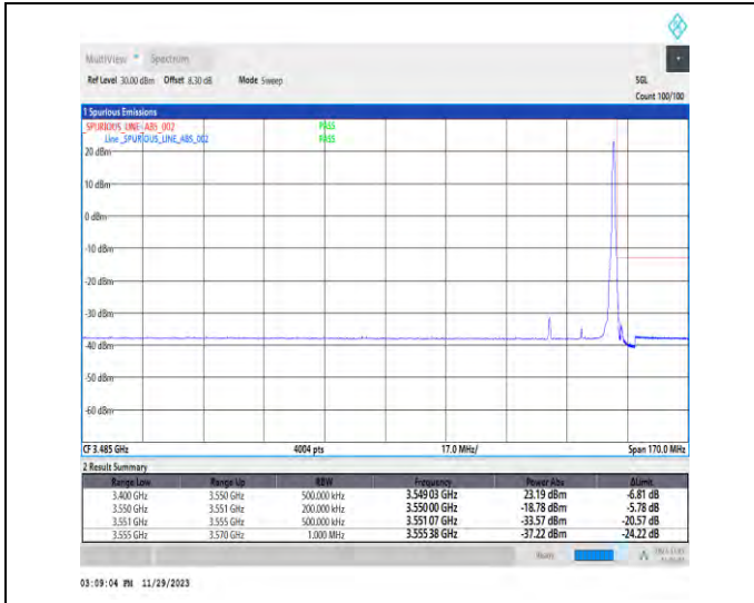
1-N78-3450-3550-PC3-30-20-H-2-DFT-PI2BPSK-Edge_1RB_Right-1@50-Ant1-1--PASS-see graph
