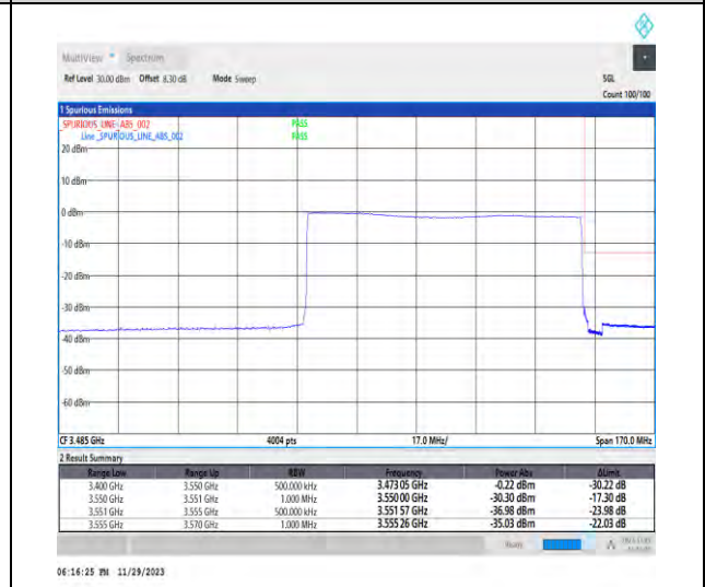
1-N78-3450-3550-PC3-30-80-H-6-CP-QPSK-Outer_Full-217@0-Ant1-1--PASS-see graph
