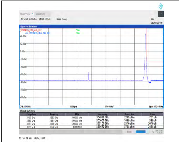
1-N78-3450-3550-PC3-30-70-H-2-DFT-PI2BPSK-Edge_1RB_Right-1@188-Ant1-1--PASS-see graph
