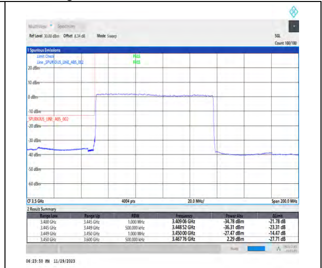
1-N78-3450-3550-PC3-30-90-L-3-DFT-PI2BPSK-Outer_Full-240@0-Ant1-1--PASS-see graph
