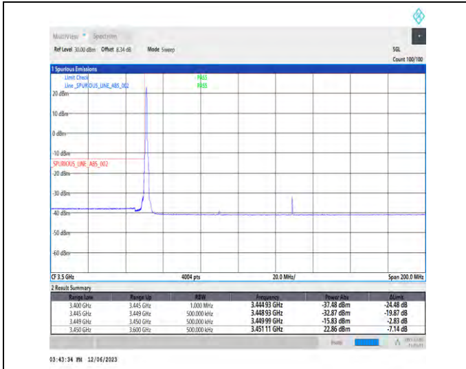
1-N78-3450-3550-PC3-30-80-L-1-DFT-PI2BPSK-Edge_1RB_Left-1@0-Ant1-1--PASS-see graph
