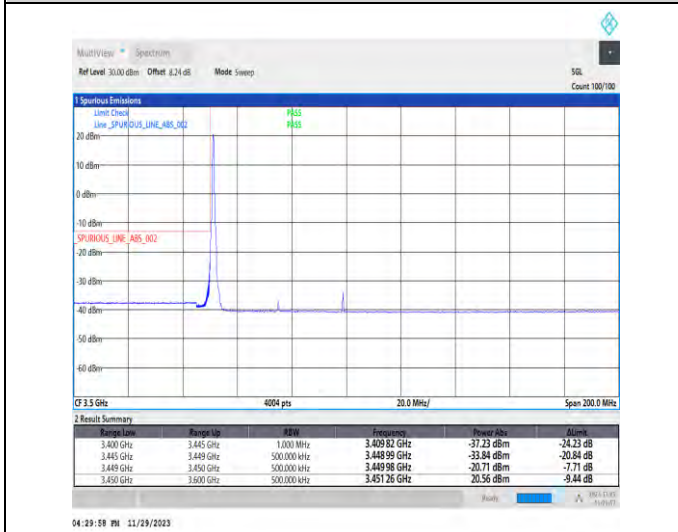
1-N78-3450-3550-PC3-30-50-L-4-CP-QPSK-Edge_1RB_Left-1@0-Ant1-1--PASS-see graph
