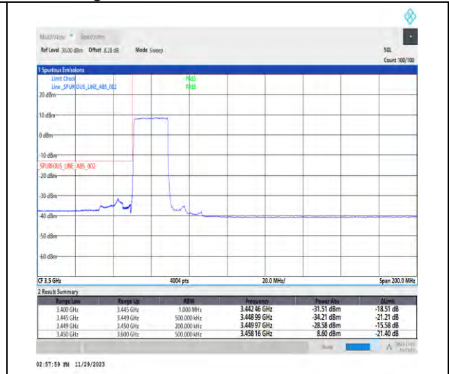
1-N78-3450-3550-PC3-30-20-L-3-DFT-PI2BPSK-Outer_Full-50@0-Ant1-1--PASS-see graph
