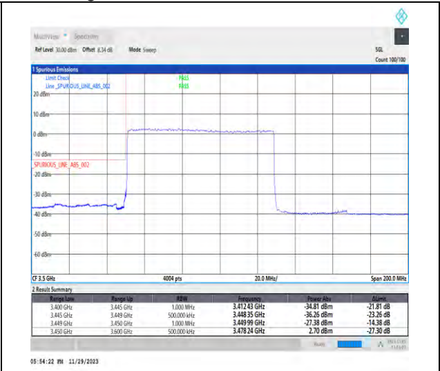
1-N78-3450-3550-PC3-30-80-L-3-DFT-PI2BPSK-Outer_Full-216@0-Ant1-1--PASS-see graph
