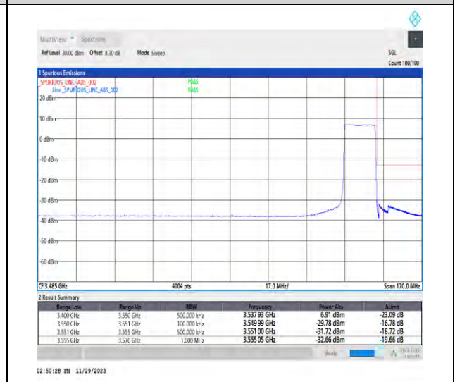
1-N78-3450-3550-PC3-30-15-H-6-CP-QPSK-Outer_Full-38@0-Ant1-1--PASS-see graph
