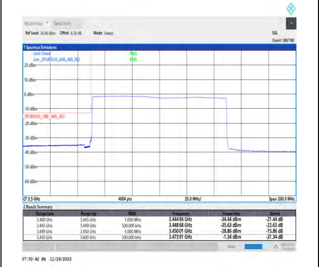
1-N78-3450-3550-PC3-30-100-L-6-CP-QPSK-Outer_Full-273@0-Ant1-1--PASS-see graph
