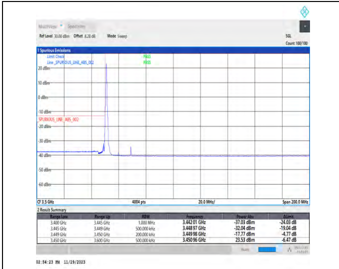
1-N78-3450-3550-PC3-30-20-L-1-DFT-PI2BPSK-Edge_1RB_Left-1@0-Ant1-1--PASS-see graph
