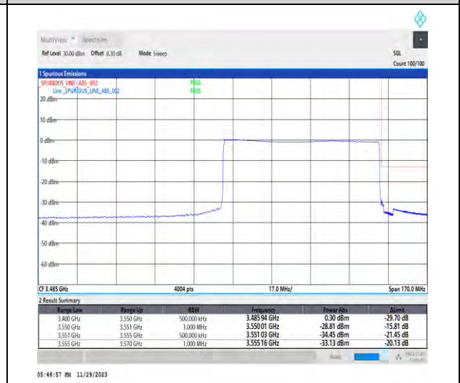
1-N78-3450-3550-PC3-30-70-H-6-CP-QPSK-Outer_Full-189@0-Ant1-1--PASS-see graph
