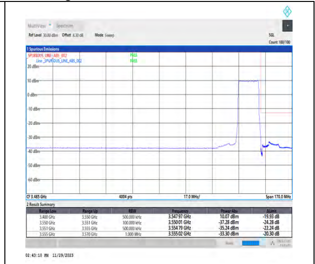
1-N78-3450-3550-PC3-30-15-H-3-DFT-PI2BPSK-Outer_Full-36@0-Ant1-1--PASS-see graph
