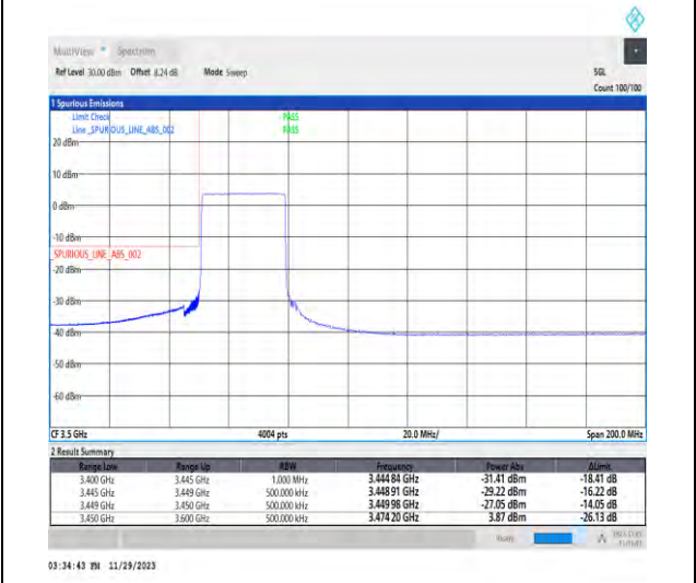
1-N78-3450-3550-PC3-30-30-L-6-CP-QPSK-Outer_Full-78@0-Ant1-1--PASS-see graph
