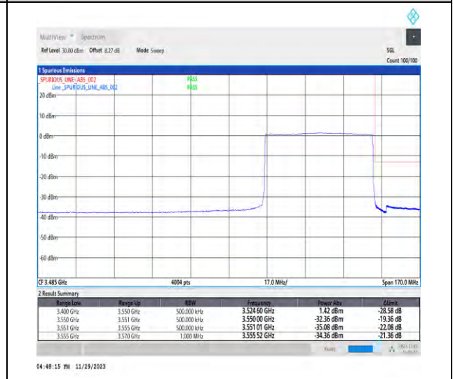
1-N78-3450-3550-PC3-30-50-H-6-CP-QPSK-Outer_Full-133@0-Ant1-1--PASS-see graph
