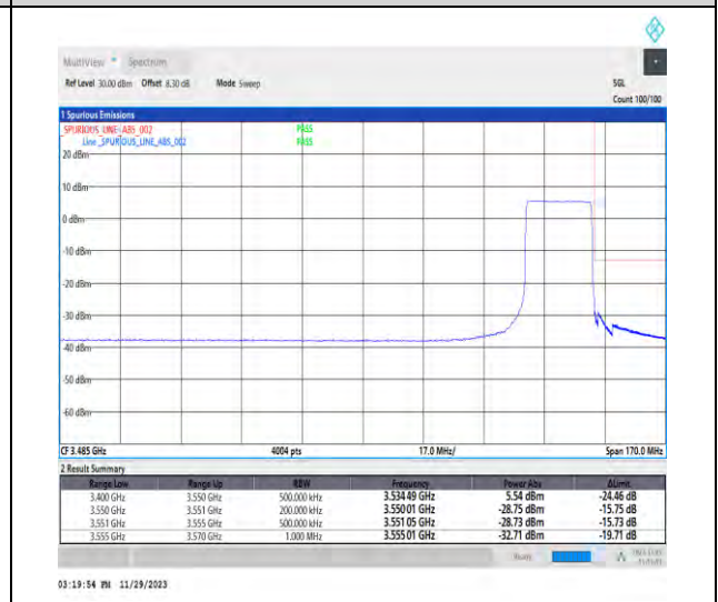
1-N78-3450-3550-PC3-30-20-H-6-CP-QPSK-Outer_Full-51@0-Ant1-1--PASS-see graph
