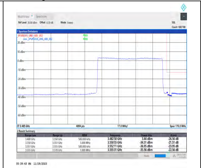
1-N78-3450-3550-PC3-30-70-H-3-DFT-PI2BPSK-Outer_Full-180@0-Ant1-1--PASS-see graph
