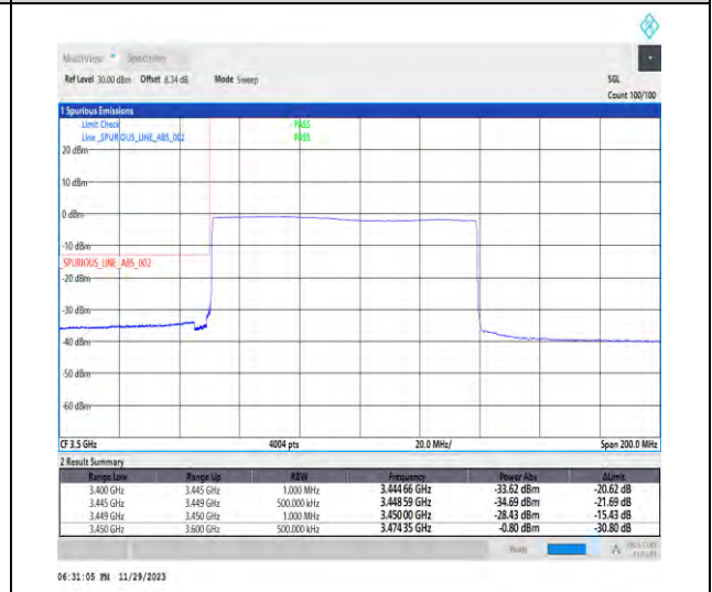
1-N78-3450-3550-PC3-30-90-L-6-CP-QPSK-Outer_Full-245@0-Ant1-1--PASS-see graph
