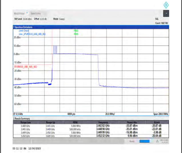
1-N78-3450-3550-PC3-30-60-L-6-CP-QPSK-Outer_Full-162@0-Ant1-1--PASS-see graph
