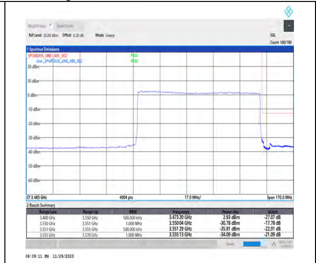
1-N78-3450-3550-PC3-30-80-H-3-DFT-PI2BPSK-Outer_Full-216@0-Ant1-1--PASS-see graph
