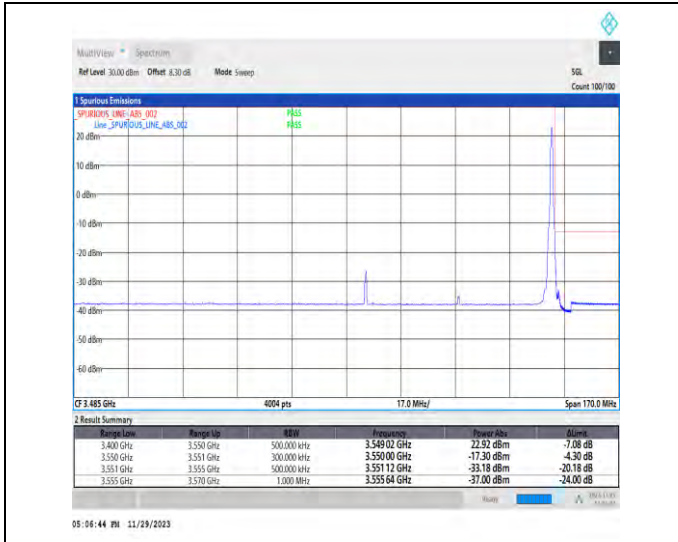
1-N78-3450-3550-PC3-30-60-H-2-DFT-PI2BPSK-Edge_1RB_Right-1@161-Ant1-1--PASS-see graph
