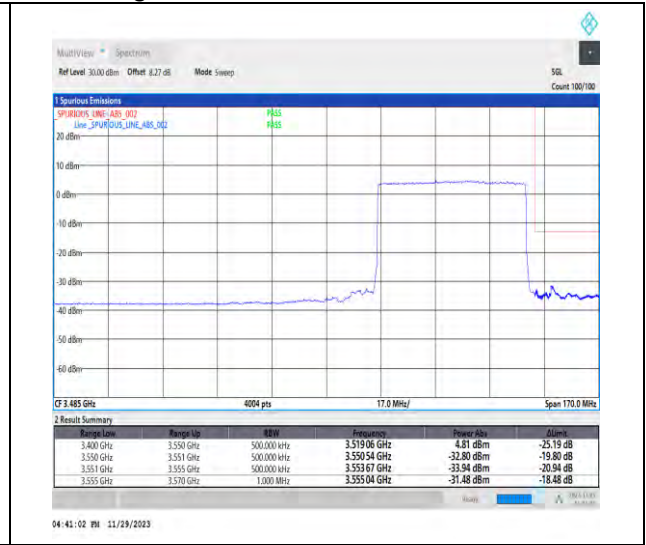
1-N78-3450-3550-PC3-30-50-H-3-DFT-PI2BPSK-Outer_Full-128@0-Ant1-1--PASS-see graph
