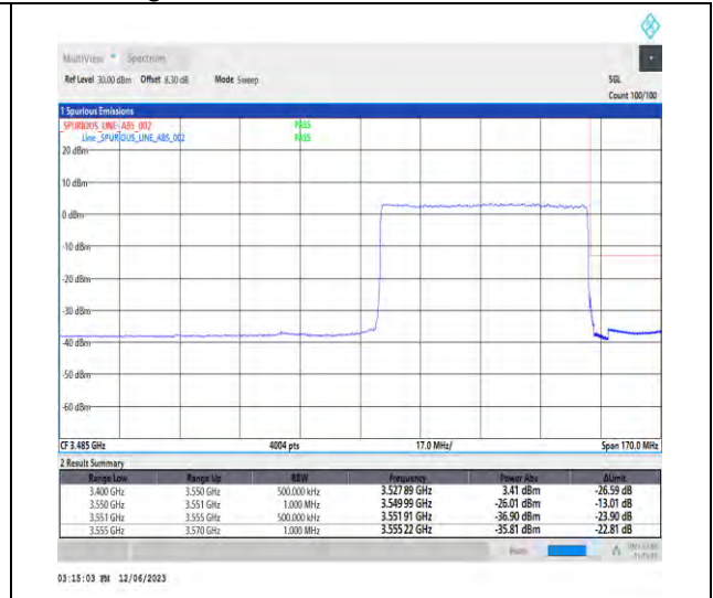
1-N78-3450-3550-PC3-30-60-H-3-DFT-PI2BPSK-Outer_Full-162@0-Ant1-1--PASS-see graph
