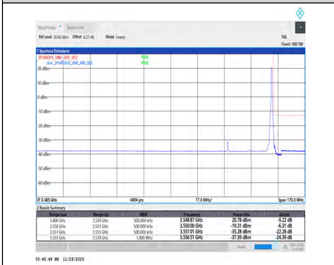
1-N78-3450-3550-PC3-30-30-H-5-CP-QPSK-Edge_1RB_Right-1@77-Ant1-1--PASS-see graph
