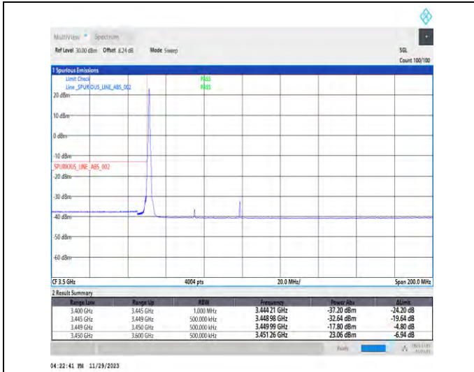
1-N78-3450-3550-PC3-30-50-L-1-DFT-PI2BPSK-Edge_1RB_Left-1@0-Ant1-1--PASS-see graph
