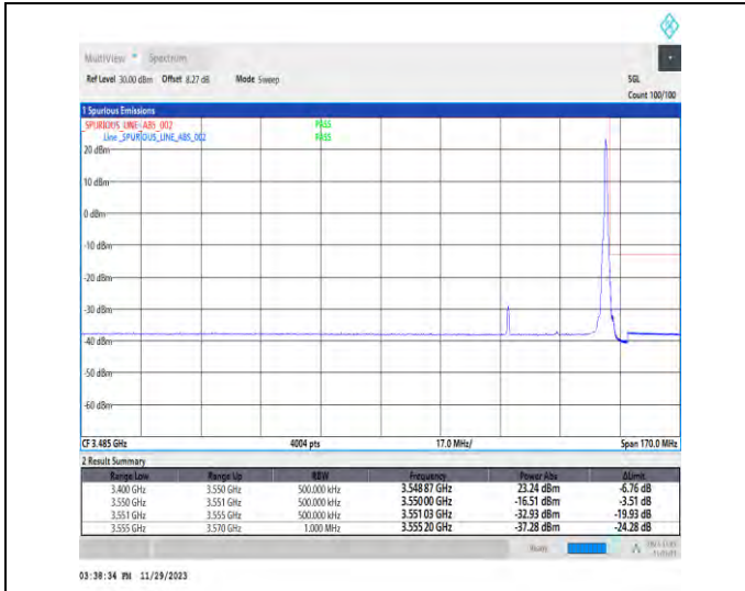
1-N78-3450-3550-PC3-30-30-H-2-DFT-PI2BPSK-Edge_1RB_Right-1@77-Ant1-1--PASS-see graph
