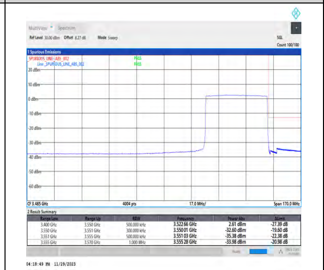
1-N78-3450-3550-PC3-30-40-H-6-CP-QPSK-Outer_Full-106@0-Ant1-1--PASS-see graph
