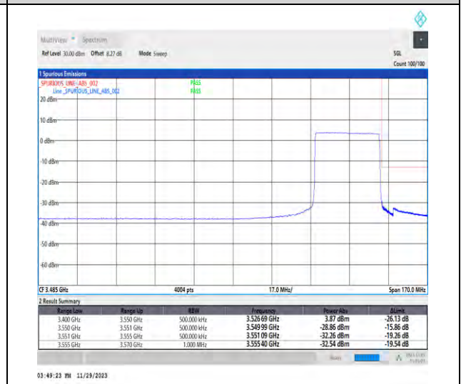
1-N78-3450-3550-PC3-30-30-H-6-CP-QPSK-Outer_Full-78@0-Ant1-1--PASS-see graph
