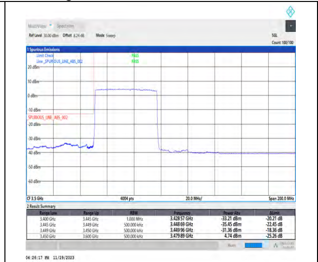
1-N78-3450-3550-PC3-30-50-L-3-DFT-PI2BPSK-Outer_Full-128@0-Ant1-1--PASS-see graph
