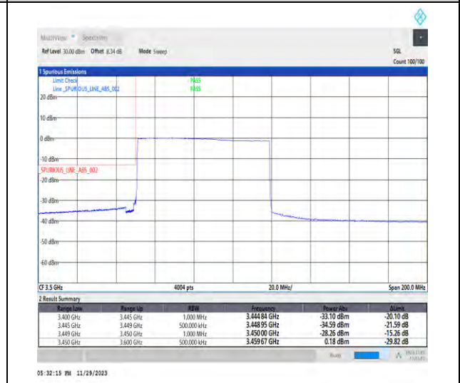
1-N78-3450-3550-PC3-30-70-L-6-CP-QPSK-Outer_Full-189@0-Ant1-1--PASS-see graph
