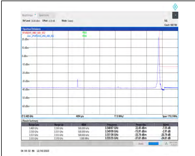
1-N78-3450-3550-PC3-30-90-H-2-DFT-PI2BPSK-Edge_1RB_Right-1@244-Ant1-1--PASS-see graph
