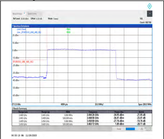
1-N78-3450-3550-PC3-30-100-L-3-DFT-PI2BPSK-Outer_Full-270@0-Ant1-1--PASS-see graph
