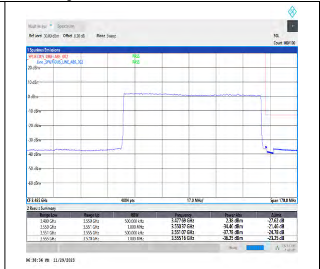
1-N78-3450-3550-PC3-30-90-H-3-DFT-PI2BPSK-Outer_Full-240@0-Ant1-1--PASS-see graph
