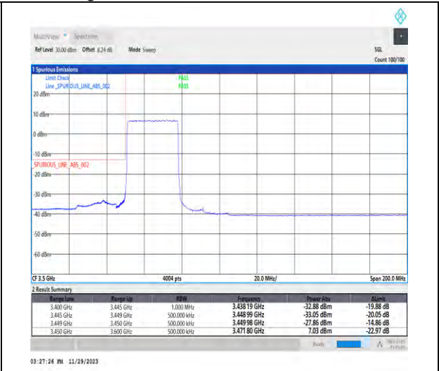
1-N78-3450-3550-PC3-30-30-L-3-DFT-PI2BPSK-Outer_Full-75@0-Ant1-1--PASS-see graph
