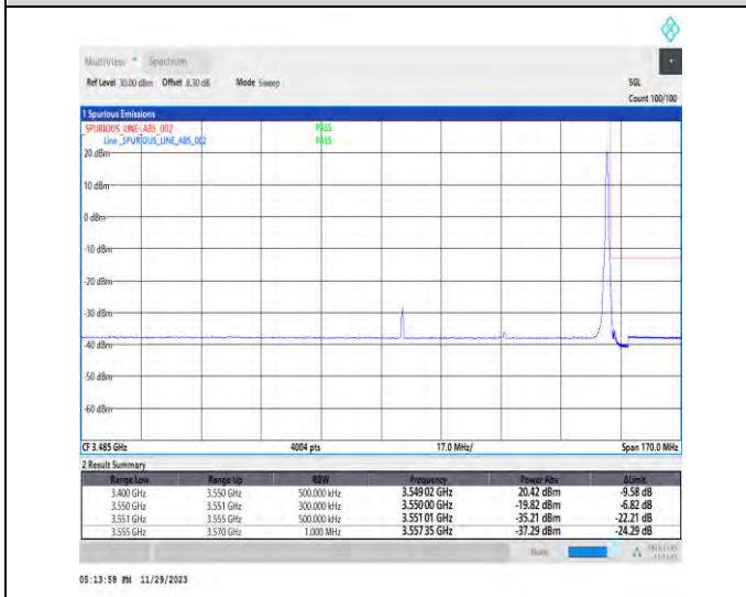
1-N78-3450-3550-PC3-30-60-H-5-CP-QPSK-Edge_1RB_Right-1@161-Ant1-1--PASS-see graph
