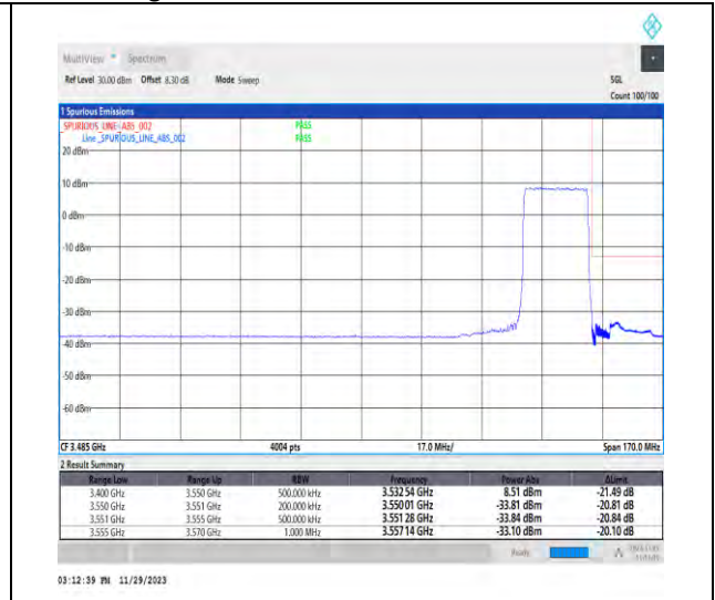
1-N78-3450-3550-PC3-30-20-H-3-DFT-PI2BPSK-Outer_Full-50@0-Ant1-1--PASS-see graph
