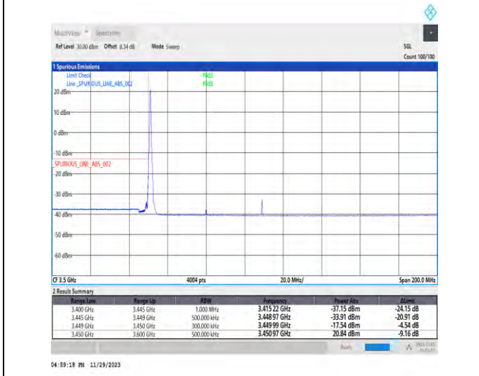
1-N78-3450-3550-PC3-30-60-L-4-CP-QPSK-Edge_1RB_Left-1@0-Ant1-1--PASS-see graph
