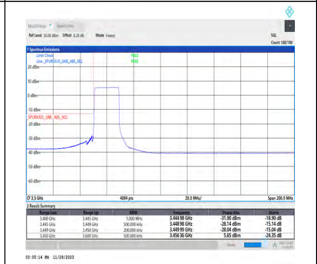
1-N78-3450-3550-PC3-30-20-L-6-CP-QPSK-Outer_Full-51@0-Ant1-1--PASS-see graph
