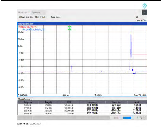
1-N78-3450-3550-PC3-30-80-H-5-CP-QPSK-Edge_1RB_Right-1@216-Ant1-1--PASS-see graph
