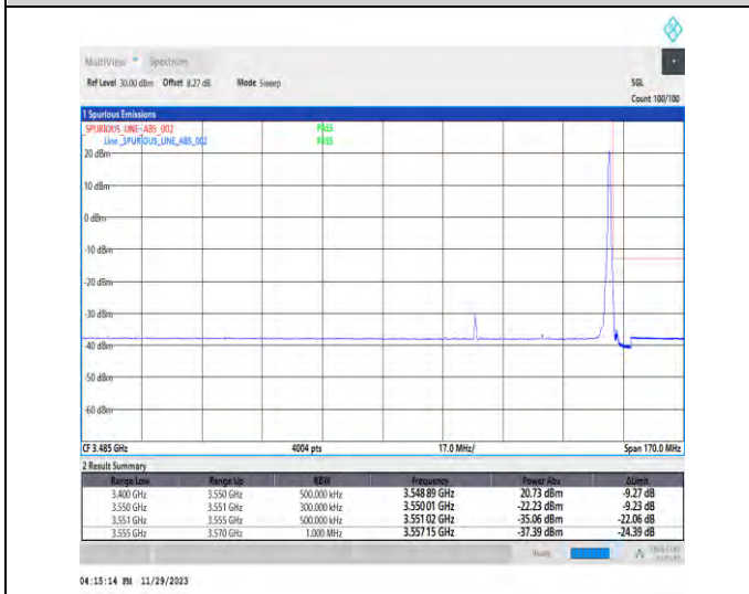
1-N78-3450-3550-PC3-30-40-H-5-CP-QPSK-Edge_1RB_Right-1@105-Ant1-1--PASS-see graph
