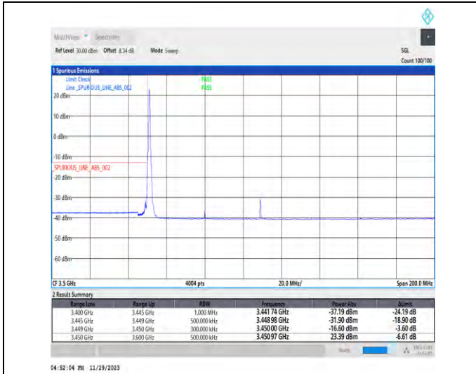
1-N78-3450-3550-PC3-30-60-L-1-DFT-PI2BPSK-Edge_1RB_Left-1@0-Ant1-1--PASS-see graph
