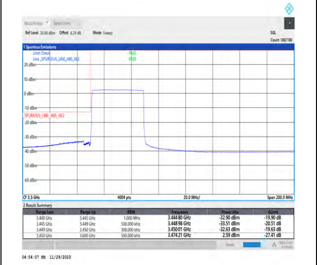
1-N78-3450-3550-PC3-30-40-L-6-CP-QPSK-Outer_Full-106@0-Ant1-1--PASS-see graph
