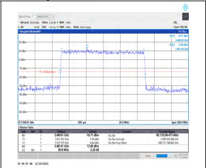
1-N78-3450-3550-PC3-30-100-M-4-DFT-64QAM-Out er_Full-270@0-Ant1-96.118-99.800-≤100-PASS
