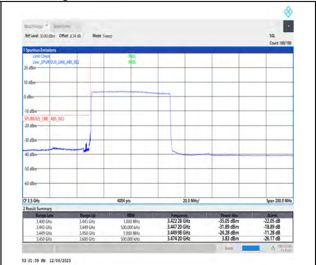
1-N78-3450-3550-PC3-30-60-L-3-DFT-PI2BPSK-Outer_Full-162@0-Ant1-1--PASS-see graph
