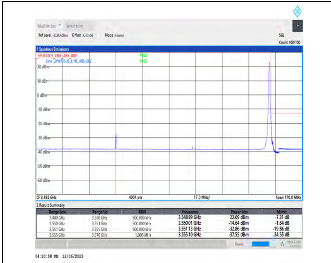
1-N78-3450-3550-PC3-30-100-H-2-DFT-PI2BPSK-Edge_1_RB_Right-1@272-Ant1-1--PASS-see graph
