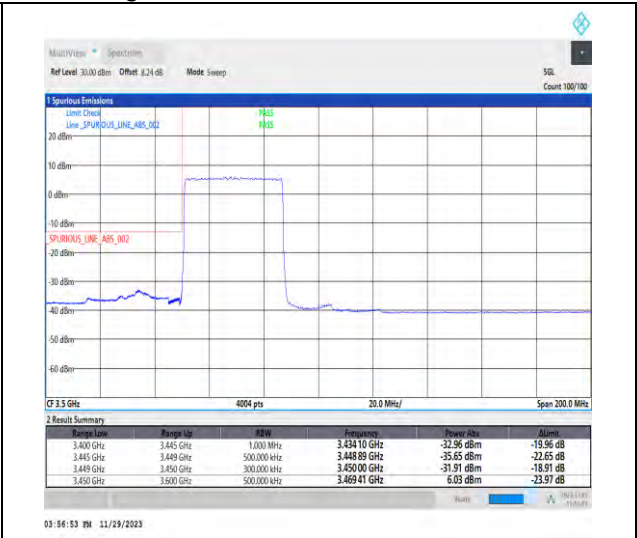
1-N78-3450-3550-PC3-30-40-L-3-DFT-PI2BPSK-Outer_Full-100@0-Ant1-1--PASS-see graph
