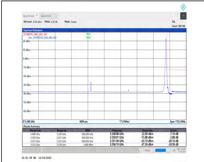
1-N78-3450-3550-PC3-30-80-H-2-DFT-PI2BPSK-Edge_1RB_Right-1@216-Ant1-1--PASS-see graph
