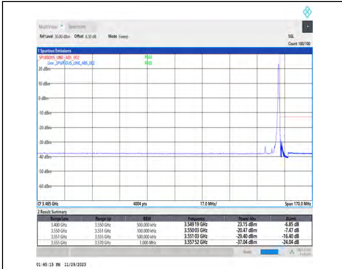
1-N78-3450-3550-PC3-30-10-H-2-DFT-PI2BPSK-Edge_1RB_Right-1@23-Ant1-1--PASS-see graph
