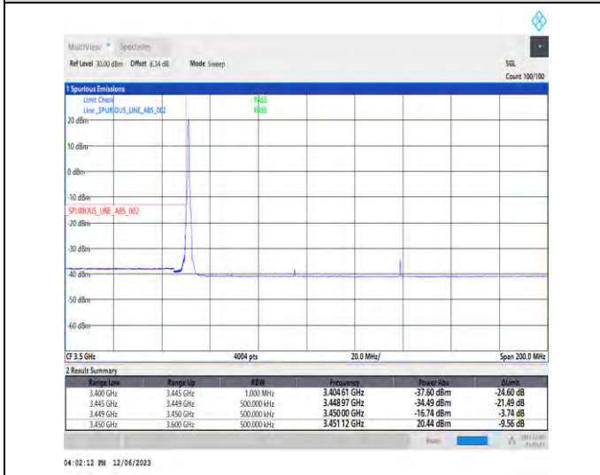
1-N78-3450-3550-PC3-30-90-L-4-CP-QPSK-Edge_1RB_Left-1@0-Ant1-1--PASS-see graph
