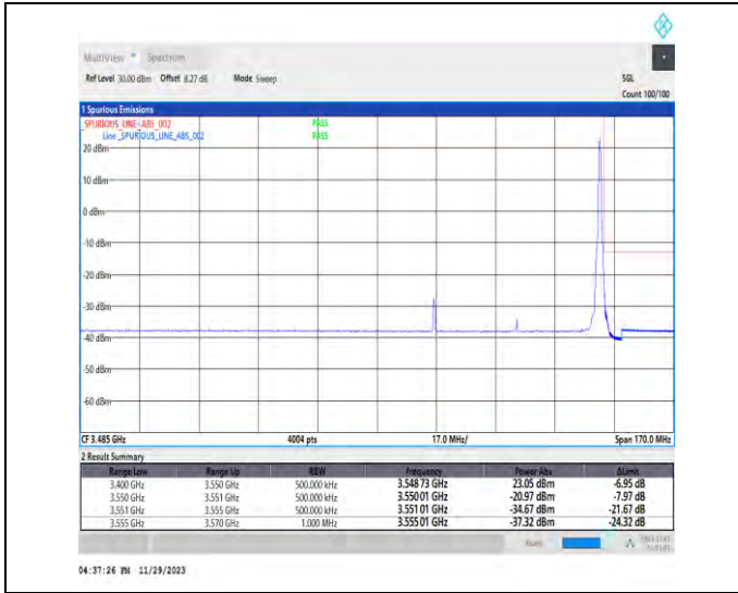
1-N78-3450-3550-PC3-30-50-H-2-DFT-PI2BPSK-Edge_1RB_Right-1@132-Ant1-1--PASS-see graph
