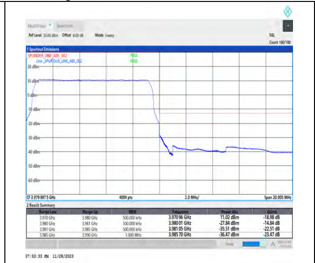
1-N77-3700-3980-PC3-30-10-H-3-DFT-PI2BPSK-Outer_Full-24@0-Ant1-1--PASS-see graph
