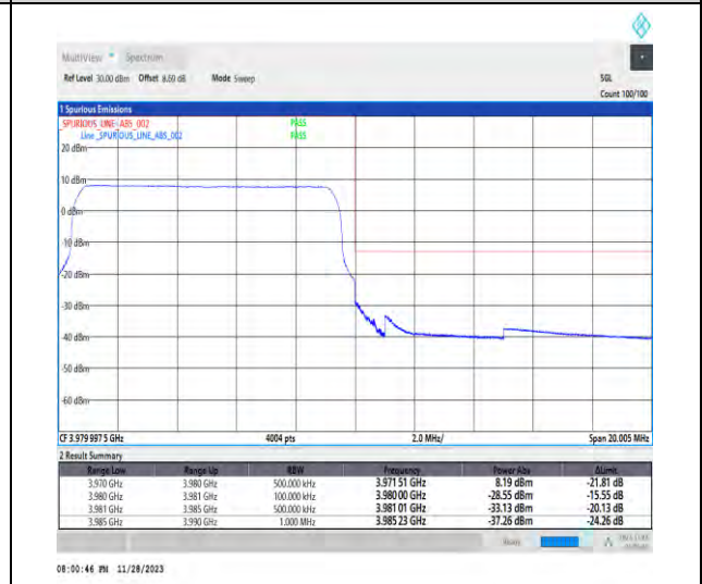
1-N77-3700-3980-PC3-30-10-H-6-CP-QPSK-Outer_Full-24@0-Ant1-1--PASS-see graph
