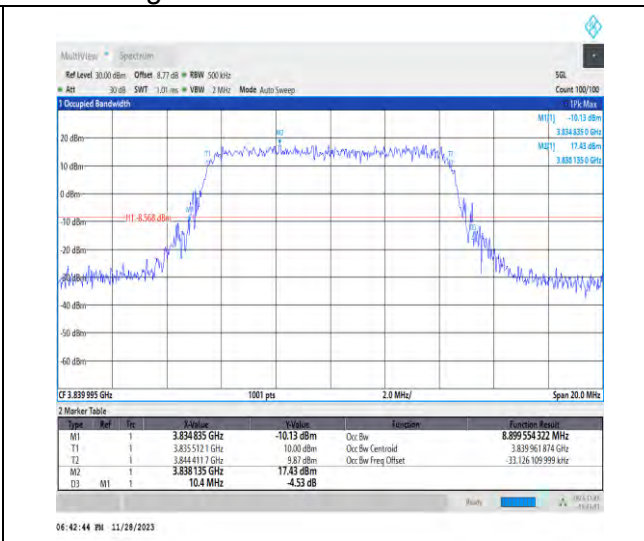
1-N77-3700-3980-PC3-30-10-M-6-CP-QPSK-Outer Full-24@0-Ant1-8.9-10.400-≤10-PASS
