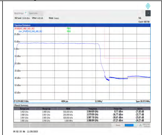
1-N77-3700-3980-PC3-30-20-H-3-DFT-PI2BPSK-Outer_Full-50@0-Ant1-1--PASS-see graph
