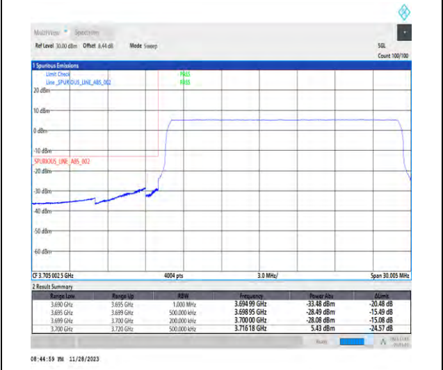
1-N77-3700-3980-PC3-30-20-L-6-CP-QPSK-Outer_Full-51@0-Ant1-1--PASS-see graph
