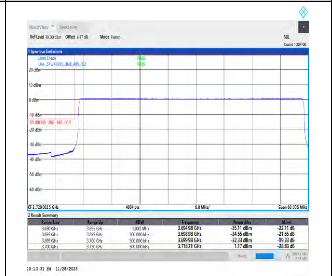
1-N77-3700-3980-PC3-30-50-L-6-CP-QPSK-Outer_Full-133@0-Ant1-1--PASS-see graph
