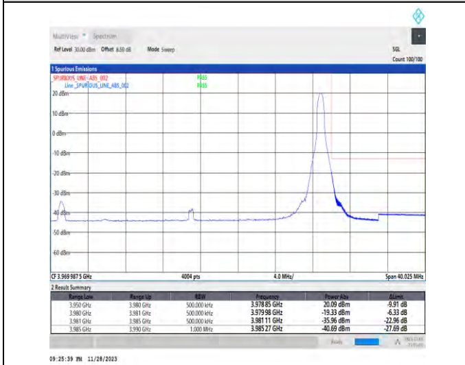
1-N77-3700-3980-PC3-30-30-H-5-CP-QPSK-Edge_1RB_Right-1@77-Ant1-1--PASS-see graph
