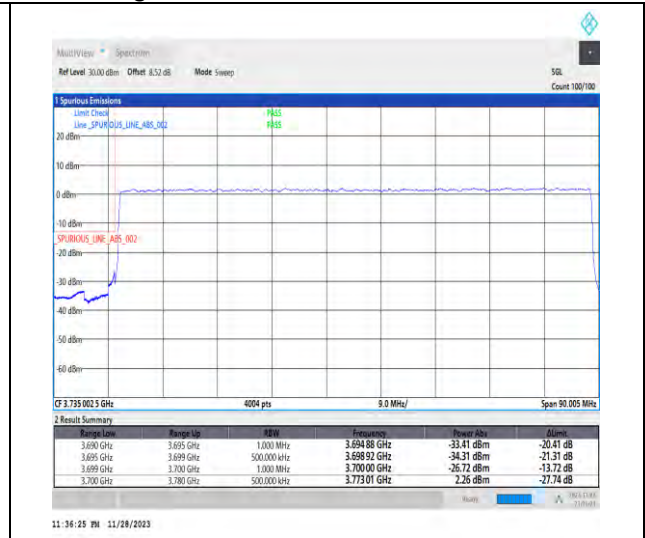
1-N77-3700-3980-PC3-30-80-L-3-DFT-PI2BPSK-Outer_Full-216@0-Ant1-1--PASS-see graph
