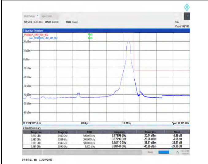
1-N77-3700-3980-PC3-30-20-H-5-CP-QPSK-Edge_1RB_Right-1@50-Ant1-1--PASS-see graph
