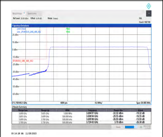
1-N77-3700-3980-PC3-30-30-L-6-CP-QPSK-Outer_Full-78@0-Ant1-1--PASS-see graph
