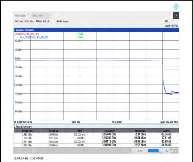
1-N77-3700-3980-PC3-30-100-H-6-CP-QPSK-Outer_Full-273@0-Ant1-1--PASS-see graph
