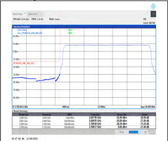
1-N77-3700-3980-PC3-30-20-L-3-DFT-PI2BPSK-Outer_Full-50@0-Ant1-1--PASS-see graph
