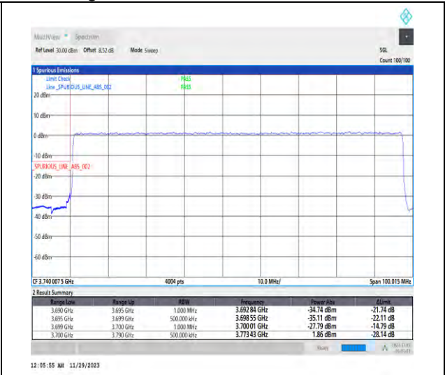
1-N77-3700-3980-PC3-30-90-L-3-DFT-PI2BPSK-Outer_Full-240@0-Ant1-1--PASS-see graph
