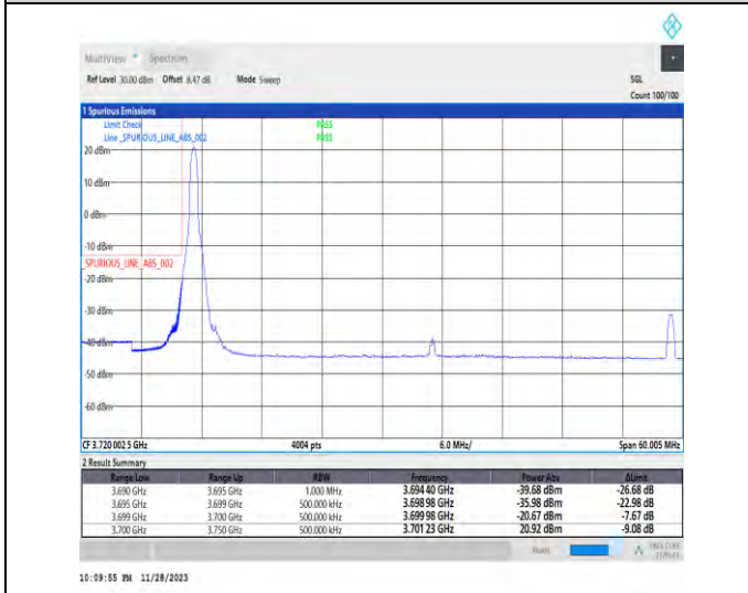
1-N77-3700-3980-PC3-30-50-L-4-CP-QPSK-Edge_1RB_Left-1@0-Ant1-1--PASS-see graph
