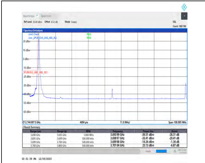
1-N77-3700-3980-PC3-30-100-L-1-DFT-PI2BPSK-Edge_1_RB_Left-1@0-Ant1-1--PASS-see graph
