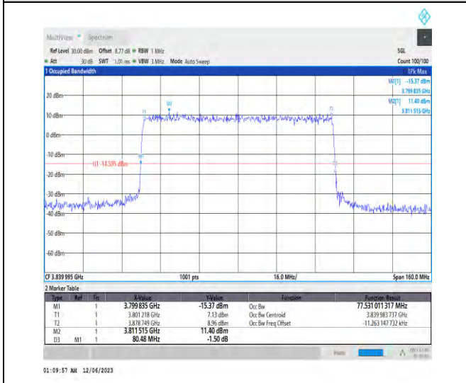
1-N77-3700-3980-PC3-30-80-M-7-CP-16QAM-Outer_Full-217@0-Ant1-77.531-80.480-≤80-PASS
