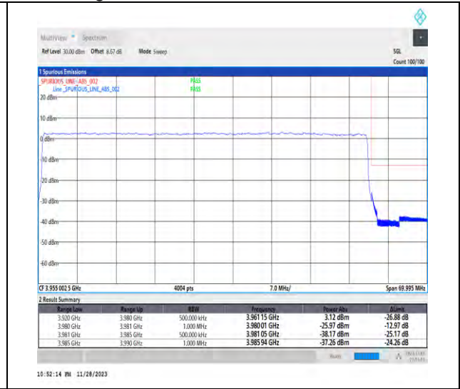
1-N77-3700-3980-PC3-30-60-H-3-DFT-PI2BPSK-Outer_Full-162@0-Ant1-1--PASS-see graph
