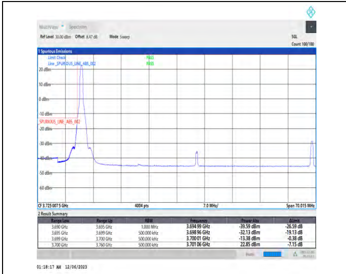
1-N77-3700-3980-PC3-30-60-L-1-DFT-PI2BPSK-Edge_1RB_Left-1@0-Ant1-1--PASS-see graph
