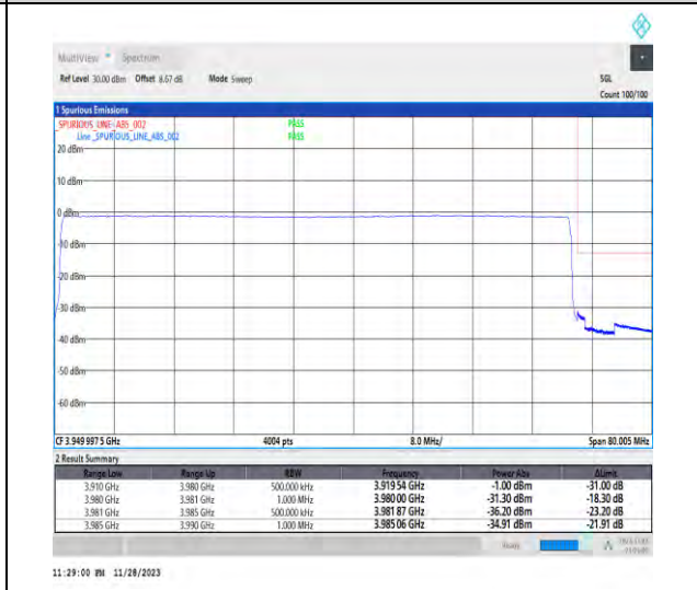
1-N77-3700-3980-PC3-30-70-H-6-CP-QPSK-Outer_Full-189@0-Ant1-1--PASS-see graph
