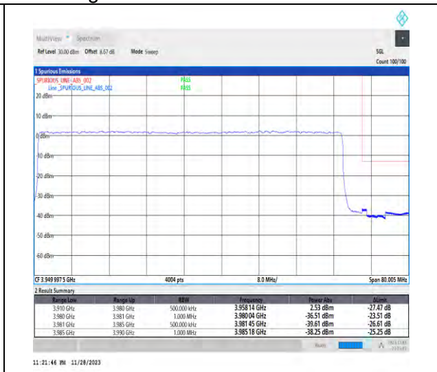
1-N77-3700-3980-PC3-30-70-H-3-DFT-PI2BPSK-Outer_Full-180@0-Ant1-1--PASS-see graph
