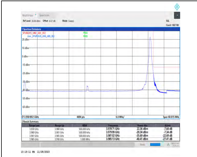
1-N77-3700-3980-PC3-30-50-H-2-DFT-PI2BPSK-Edge_1RB_Right-1@132-Ant1-1--PASS-see graph
