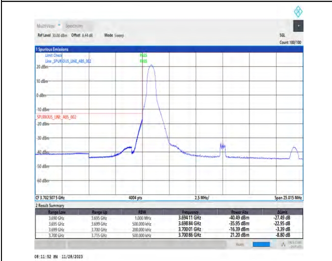
1-N77-3700-3980-PC3-30-15-L-4-CP-QPSK-Edge_1RB_Left-1@0-Ant1-1--PASS-see graph
