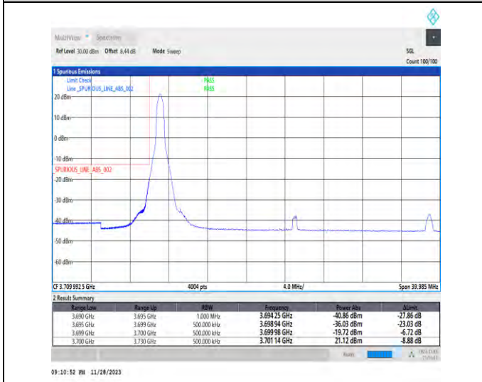
1-N77-3700-3980-PC3-30-30-L-4-CP-QPSK-Edge_1RB_Left-1@0-Ant1-1--PASS-see graph
