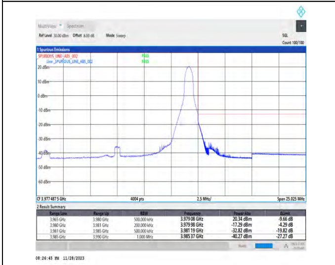
1-N77-3700-3980-PC3-30-15-H-5-CP-QPSK-Edge_1RB_Right-1@37-Ant1-1--PASS-see graph
