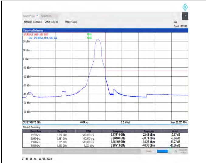
1-N77-3700-3980-PC3-30-10-H-2-DFT-PI2BPSK-Edge_1RB_Right-1@23-Ant1-1--PASS-see graph
