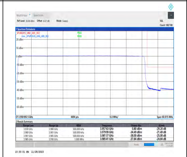
1-N77-3700-3980-PC3-30-50-H-6-CP-QPSK-Outer_Full-133@0-Ant1-1--PASS-see graph
