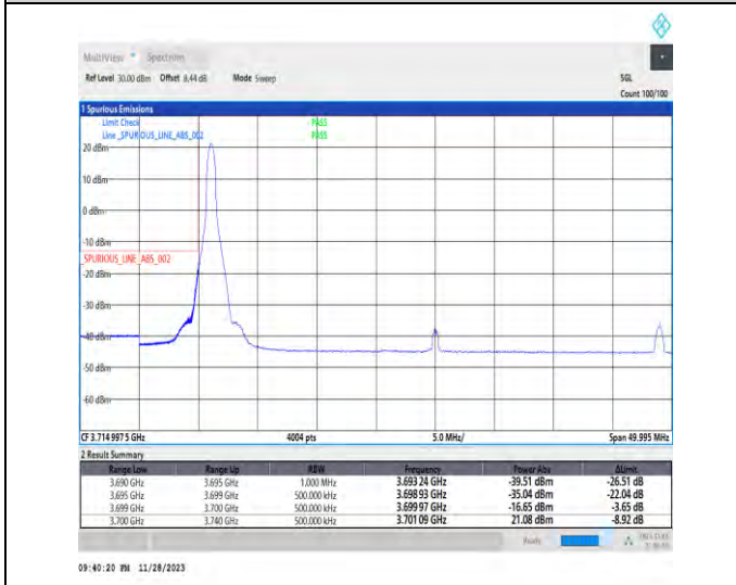
1-N77-3700-3980-PC3-30-40-L-4-CP-QPSK-Edge_1RB_Left-1@0-Ant1-1--PASS-see graph
