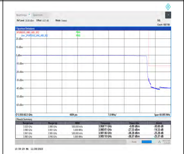
1-N77-3700-3980-PC3-30-60-H-6-CP-QPSK-Outer_Full-162@0-Ant1-1--PASS-see graph
