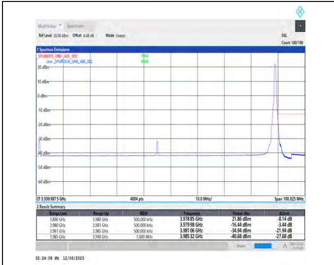
1-N77-3700-3980-PC3-30-90-H-2-DFT-PI2BPSK-Edge_1RB_Right-1@244-Ant1-1--PASS-see graph
