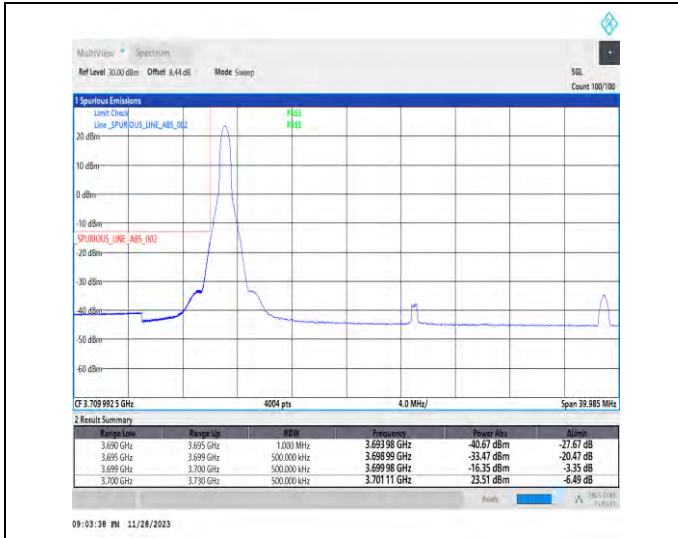
1-N77-3700-3980-PC3-30-30-L-1-DFT-PI2BPSK-Edge_1RB_Left-1@0-Ant1-1--PASS-see graph
