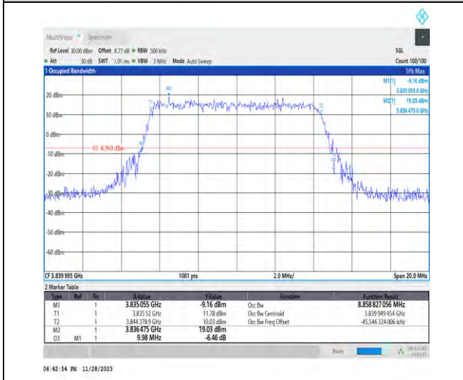
1-N77-3700-3980-PC3-30-10-M-7-CP-16QAM-Outer _Full-24@0-Ant1-8.859-9.980-≤10-PASS
