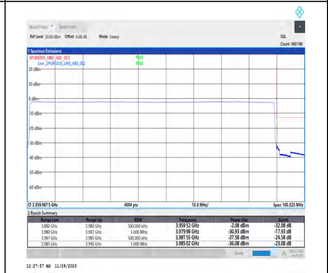
1-N77-3700-3980-PC3-30-90-H-6-CP-QPSK-Outer_Full-245@0-Ant1-1--PASS-see graph
