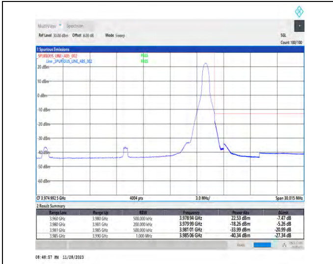
1-N77-3700-3980-PC3-30-20-H-2-DFT-PI2BPSK-Edge_1RB_Right-1@50-Ant1-1--PASS-see graph
