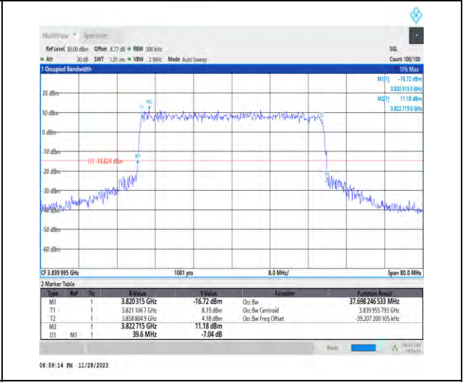
1-N77-3700-3980-PC3-30-40-M-8-CP-64QAM-Outer _Full-106@0-Ant1-37.698-39.600-≤40-PASS
