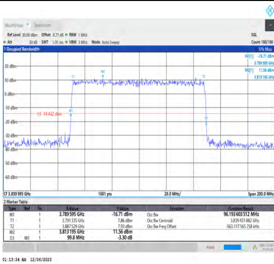
1-N77-3700-3980-PC3-30-100-M-3-DFT-16QAM-Out er_Full-270@0-Ant1-96.194-99.800-≤100-PASS
