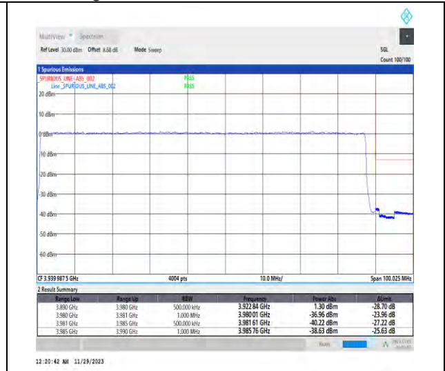
1-N77-3700-3980-PC3-30-90-H-3-DFT-PI2BPSK-Outer_Full-240@0-Ant1-1--PASS-see graph
