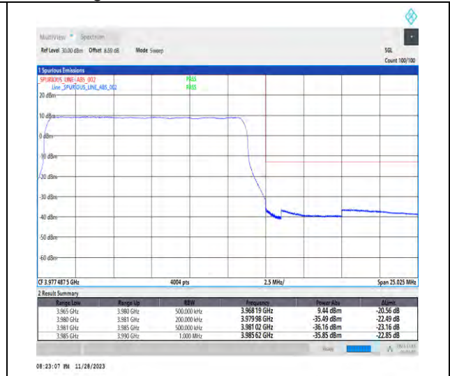
1-N77-3700-3980-PC3-30-15-H-3-DFT-PI2BPSK-Outer_Full-36@0-Ant1-1--PASS-see graph
