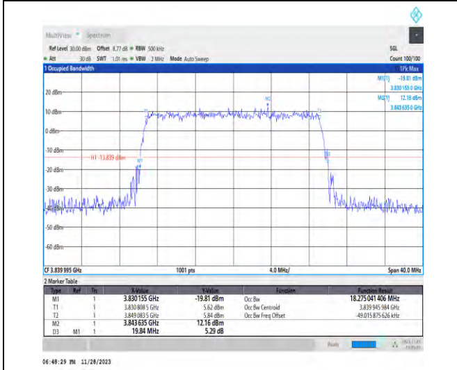
1-N77-3700-3980-PC3-30-20-M-9-CP-256QAM-Outer_Full-51@0-Ant1-18.275-19.840-≤20-PASS
