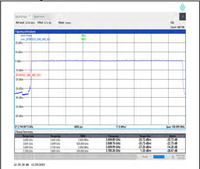
1-N77-3700-3980-PC3-30-100-L-3-DFT-PI2BPSK-Outer_Full-270@0-Ant1-1--PASS-see graph
