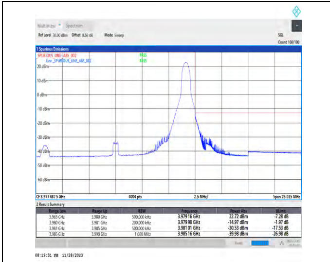
1-N77-3700-3980-PC3-30-15-H-2-DFT-PI2BPSK-Edge_1RB_Right-1@37-Ant1-1--PASS-see graph
