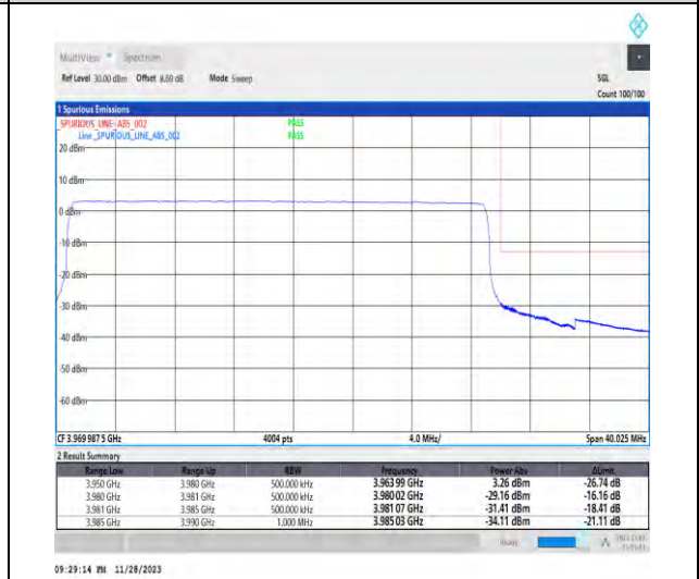
1-N77-3700-3980-PC3-30-30-H-6-CP-QPSK-Outer_Full-78@0-Ant1-1--PASS-see graph
