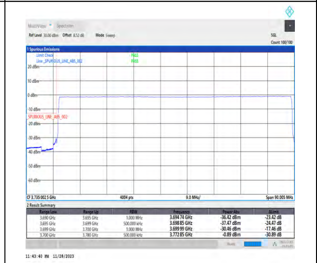
1-N77-3700-3980-PC3-30-80-L-6-CP-QPSK-Outer_Full-217@0-Ant1-1--PASS-see graph
