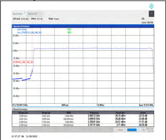
1-N77-3700-3980-PC3-30-60-L-3-DFT-PI2BPSK-Outer_Full-162@0-Ant1-1--PASS-see graph
