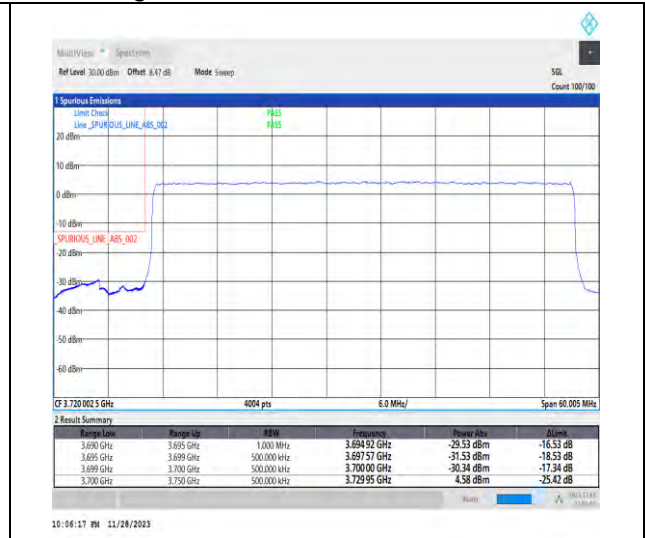
1-N77-3700-3980-PC3-30-50-L-3-DFT-PI2BPSK-Outer_Full-128@0-Ant1-1--PASS-see graph
