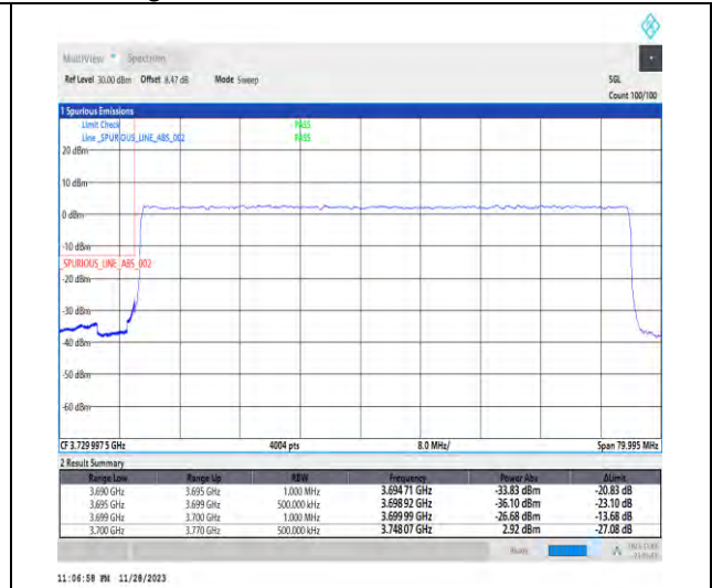
1-N77-3700-3980-PC3-30-70-L-3-DFT-PI2BPSK-Outer_Full-180@0-Ant1-1--PASS-see graph
