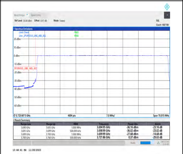
1-N77-3700-3980-PC3-30-60-L-6-CP-QPSK-Outer_Full-162@0-Ant1-1--PASS-see graph
