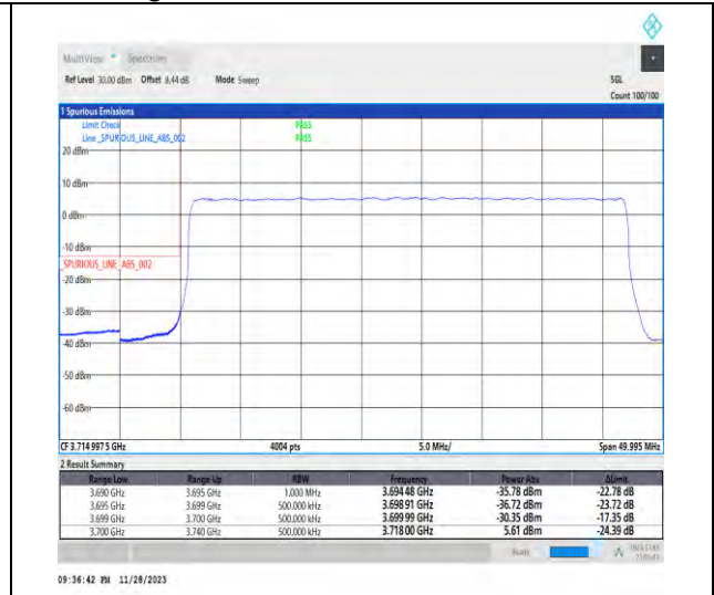
1-N77-3700-3980-PC3-30-40-L-3-DFT-PI2BPSK-Outer_Full-100@0-Ant1-1--PASS-see graph
