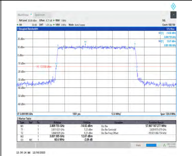
1-N77-3700-3980-PC3-30-60-M-6-CP-QPSK-Outer_Full-162@0-Ant1-57.907-60.600-≤60-PASS
