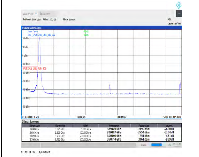
1-N77-3700-3980-PC3-30-90-L-4-CP-QPSK-Edge_1RB_Left-1@0-Ant1-1--PASS-see graph
