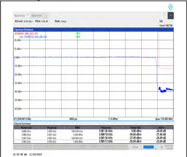
1-N77-3700-3980-PC3-30-100-H-3-DFT-PI2BPSK-Outer_Full-270@0-Ant1-1--PASS-see graph
