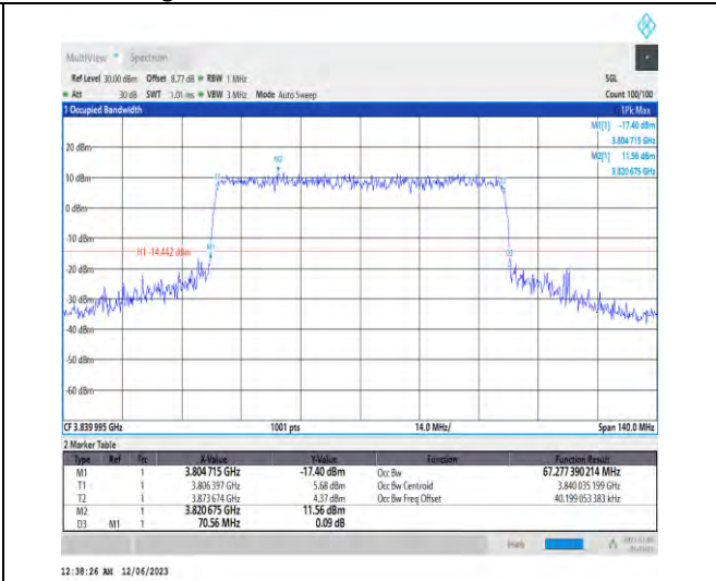
1-N77-3700-3980-PC3-30-70-M-7-CP-16QAM-Outer_Full-189@0-Ant1-67.277-70.560-≤70-PASS
