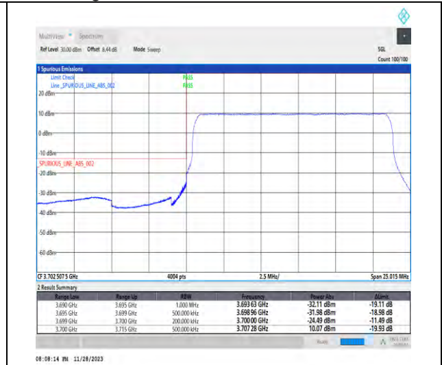
1-N77-3700-3980-PC3-30-15-L-3-DFT-PI2BPSK-Outer_Full-36@0-Ant1-1--PASS-see graph
