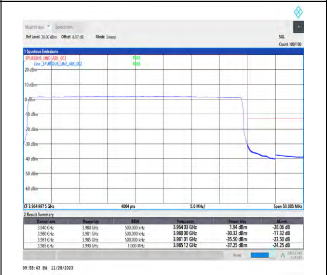
1-N77-3700-3980-PC3-30-40-H-6-CP-QPSK-Outer_Full-106@0-Ant1-1--PASS-see graph
