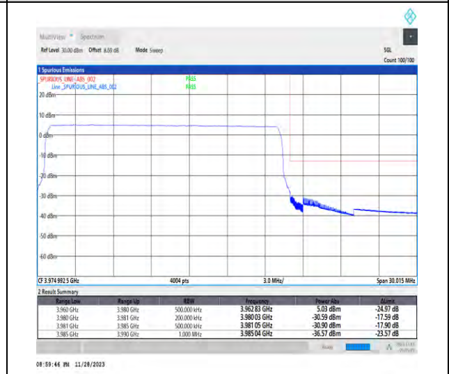
1-N77-3700-3980-PC3-30-20-H-6-CP-QPSK-Outer_Full-51@0-Ant1-1--PASS-see graph
