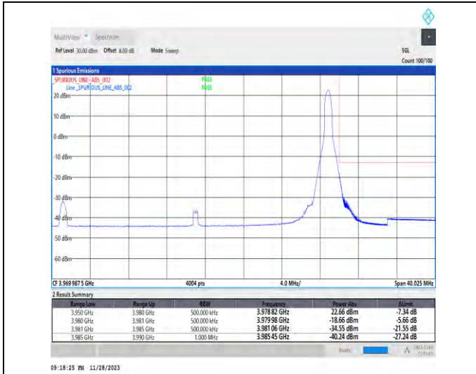
1-N77-3700-3980-PC3-30-30-H-2-DFT-PI2BPSK-Edge_1RB_Right-1@77-Ant1-1--PASS-see graph
