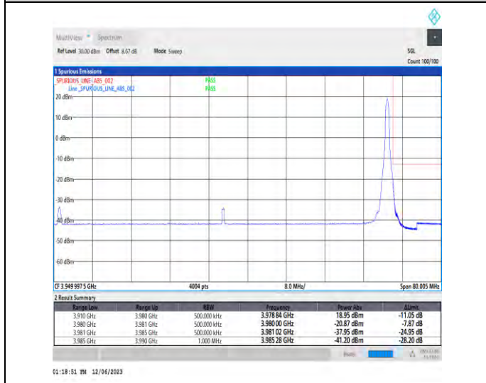
1-N77-3700-3980-PC3-30-70-H-5-CP-QPSK-Edge_1RB_Right-1@188-Ant1-1--PASS-see graph
