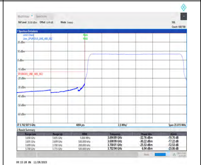
1-N77-3700-3980-PC3-30-15-L-6-CP-QPSK-Outer_Full-38@0-Ant1-1--PASS-see graph
