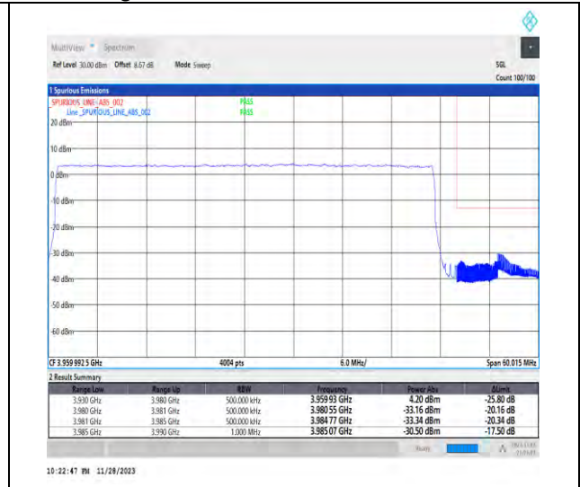
1-N77-3700-3980-PC3-30-50-H-3-DFT-PI2BPSK-Outer_Full-128@0-Ant1-1--PASS-see graph
