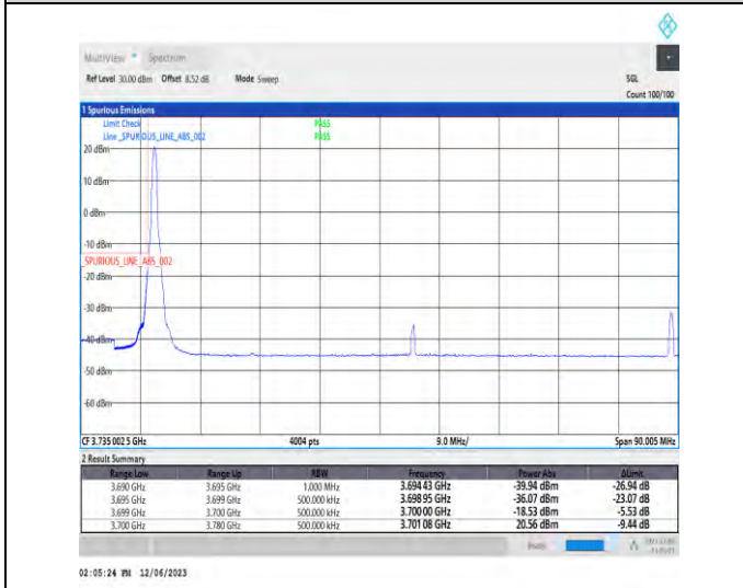
1-N77-3700-3980-PC3-30-80-L-4-CP-QPSK-Edge_1RB_Left-1@0-Ant1-1--PASS-see graph
