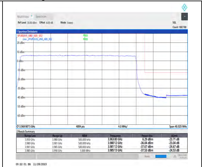
1-N77-3700-3980-PC3-30-30-H-3-DFT-PI2BPSK-Outer_Full-75@0-Ant1-1--PASS-see graph
