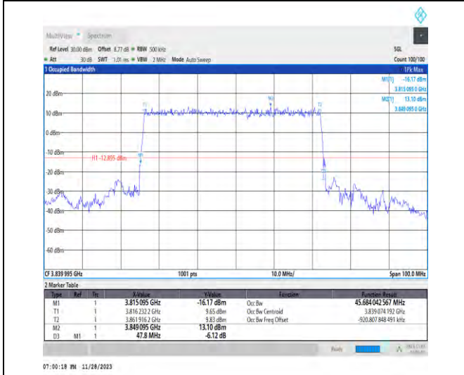
1-N77-3700-3980-PC3-30-50-M-2-DFT-PI2BPSK-Outer_Full-128@0-Ant1-45.684-47.800-≤50-PASS
