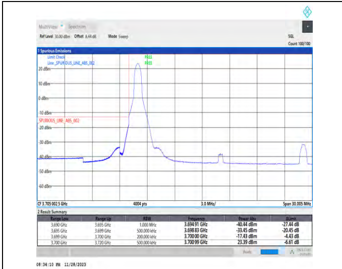
1-N77-3700-3980-PC3-30-20-L-1-DFT-PI2BPSK-Edge_1RB_Left-1@0-Ant1-1--PASS-see graph
