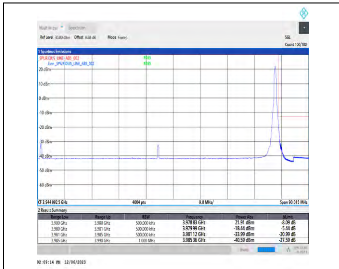
1-N77-3700-3980-PC3-30-80-H-2-DFT-PI2BPSK-Edge_1RB_Right-1@216-Ant1-1--PASS-see graph
