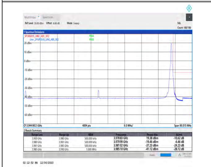
1-N77-3700-3980-PC3-30-80-H-5-CP-QPSK-Edge_1RB_Right-1@216-Ant1-1--PASS-see graph
