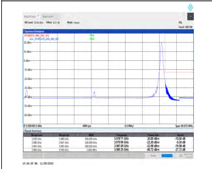
1-N77-3700-3980-PC3-30-50-H-5-CP-QPSK-Edge_1RB_Right-1@132-Ant1-1--PASS-see graph
