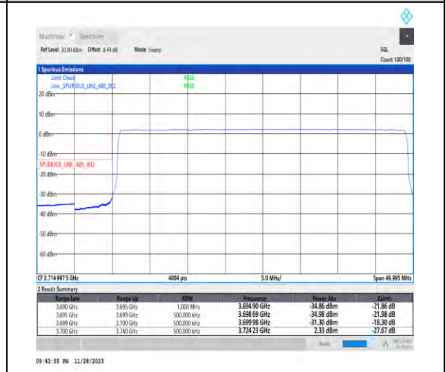
1-N77-3700-3980-PC3-30-40-L-6-CP-QPSK-Outer_Full-106@0-Ant1-1--PASS-see graph
