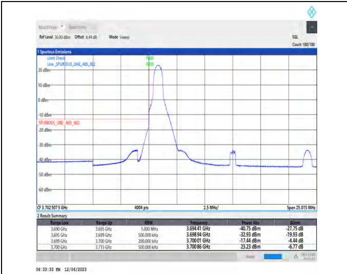
1-N77-3700-3980-PC3-30-15-L-1-DFT-PI2BPSK-Edge_1RB_Left-1@0-Ant1-1--PASS-see graph
