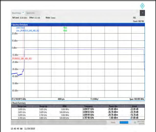
1-N77-3700-3980-PC3-30-100-L-6-CP-QPSK-Outer_Full-273@0-Ant1-1--PASS-see graph
