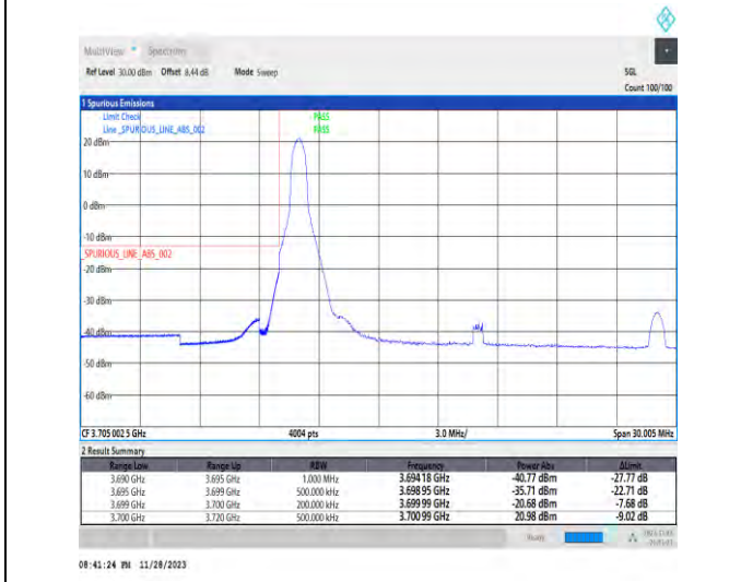
1-N77-3700-3980-PC3-30-20-L-4-CP-QPSK-Edge_1RB_Left-1@0-Ant1-1--PASS-see graph
