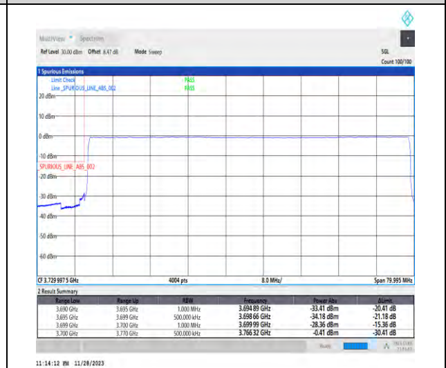
1-N77-3700-3980-PC3-30-70-L-6-CP-QPSK-Outer_Full-189@0-Ant1-1--PASS-see graph
