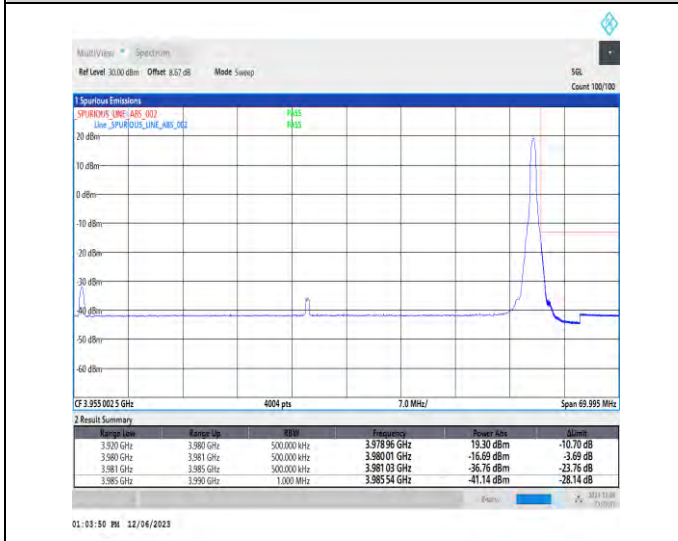
1-N77-3700-3980-PC3-30-60-H-5-CP-QPSK-Edge_1RB_Right-1@161-Ant1-1--PASS-see graph
