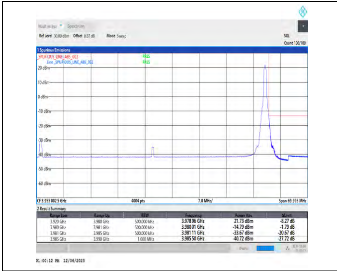
1-N77-3700-3980-PC3-30-60-H-2-DFT-PI2BPSK-Edge_1RB_Right-1@161-Ant1-1--PASS-see graph
