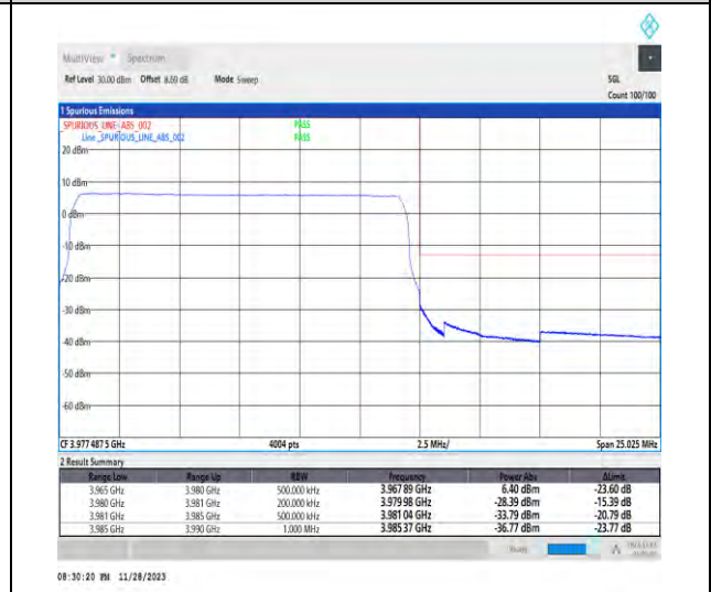
1-N77-3700-3980-PC3-30-15-H-6-CP-QPSK-Outer_Full-38@0-Ant1-1--PASS-see graph
