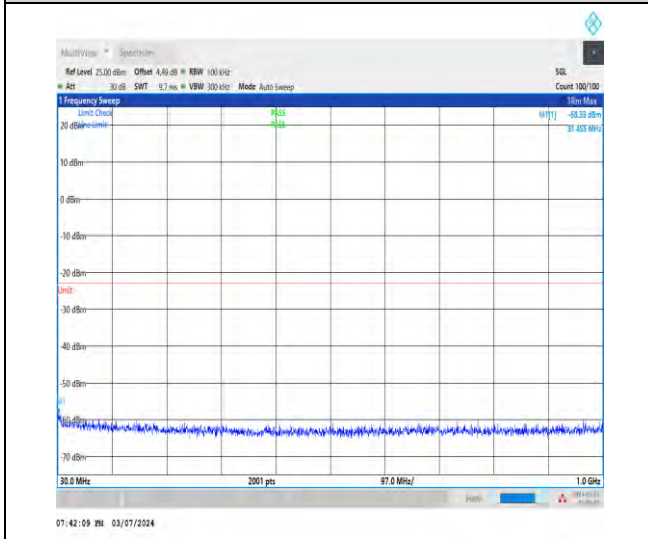
1-N66-15-40-H-1-DFT-PI2BPSK-Inner_1RB_Left-1 @ 1-30-1000-Ant1-31.46--58.33--23-PASS
