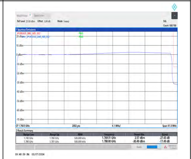
1-N66-15-40-H-6-CP-QPSK-Outer_Full-216@0-Ant1-1-seegraph-PASS-see graph
