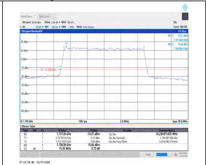
1-N66-15-15-M-8-CP-64QAM-Outer_Full-79@0-Ant1 -14.231-15.450-≤15-PASS
