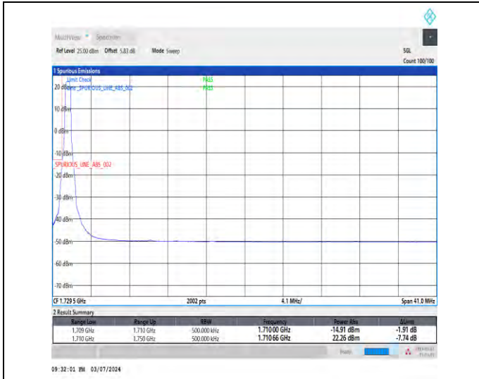
1-N66-15-40-L-1-DFT-PI2BPSK-Edge_1RB_Left-1@0-Ant1-1-seegraph-PASS-see graph
