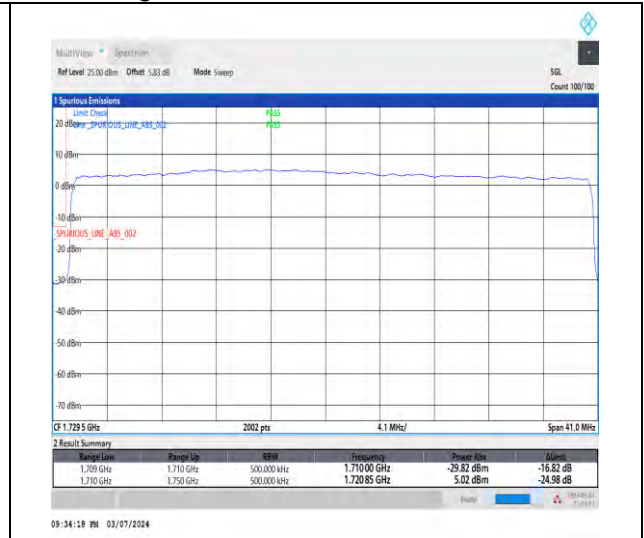
1-N66-15-40-L-3-DFT-PI2BPSK-Outer_Full-216@0-Ant1-1-seegraph-PASS-see graph
