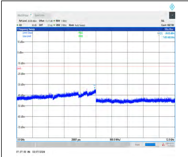
1-N66-15-40-L-1-DFT-PI2BPSK-Inner_1RB_Left-1 @ 1-3000-12000-Ant1-7431.60--34.02--13-PASS
