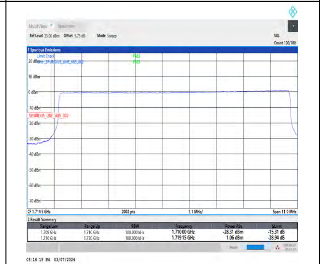
1-N66-15-10-L-6-CP-QPSK-Outer_Full-52@0-Ant1-1-seegraph-PASS-see graph
