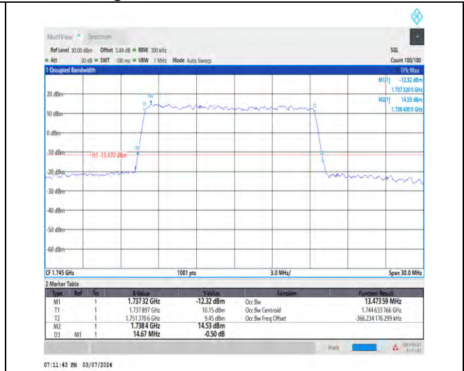
1-N66-15-15-M-4-DFT-64QAM-Outer_Full-75@0-Ant 1-13.474-14.670-≤15-PASS
