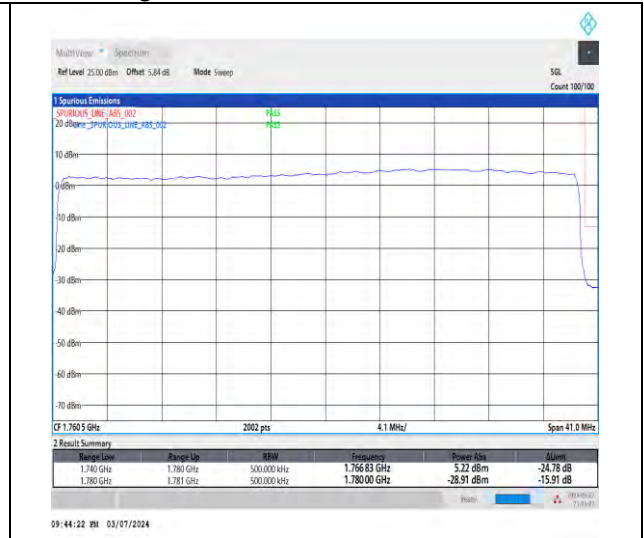
1-N66-15-40-H-3-DFT-PI2BPSK-Outer_Full-216@0-Ant1-1-seegraph-PASS-see graph
