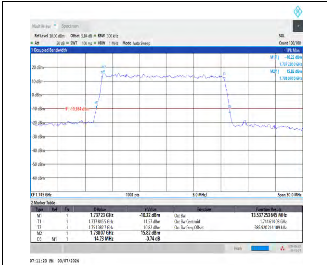
1-N66-15-15-M-3-DFT-16QAM-Outer_Full-75@0-Ant 1-13.537-14.730-≤15-PASS
