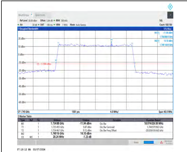
1-N66-15-20-M-6-CP-QPSK-Outer_Full-106@0-Ant1 -18.974-20.240-≤20-PASS
