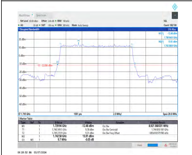
1-N66-15-10-M-2-DFT-PI2BPSK-Outer_Full-50@0-Ant1 -8.921-9.700-≤10-PASS
