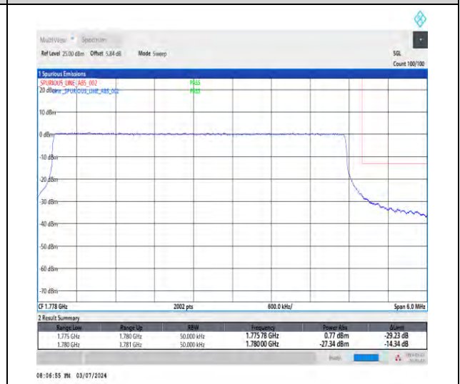
1-N66-15-5-H-6-CP-QPSK-Outer_Full-25@0-Ant1-1-seegraph-PASS-see graph
