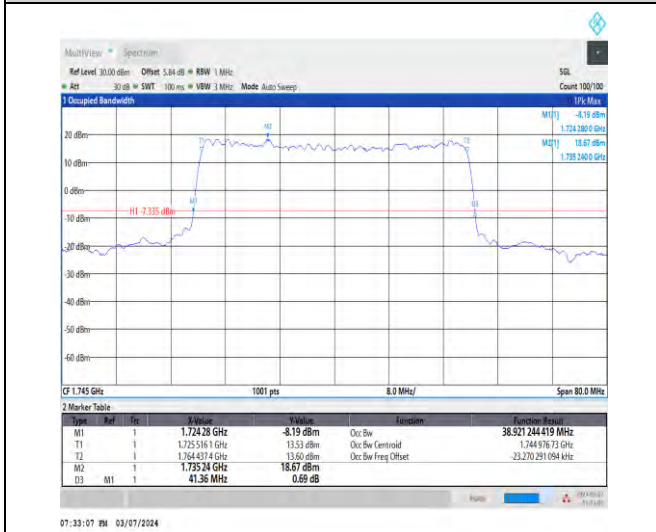
1-N66-15-40-M-2-DFT-PI2BPSK-Outer_Full-216@0-Ant1 Ant1-38.921-41.360-≤40-PASS
