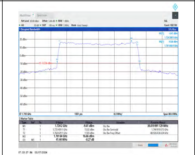
1-N66-15-40-M-3-DFT-16QAM-Outer_Full-216@0-A nt1-39.02-41.440-≤40-PASS
