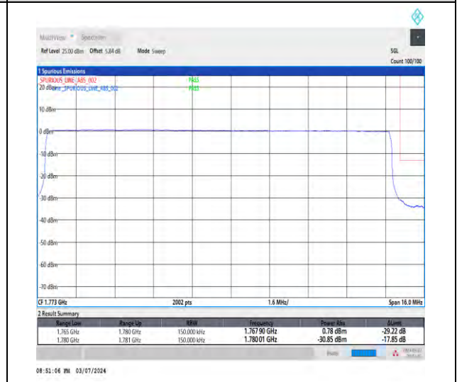
1-N66-15-15-H-6-CP-QPSK-Outer_Full-79@0-Ant1-1-seegraph-PASS-see graph
