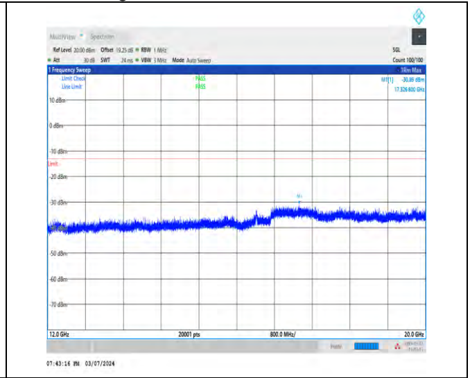
1-N66-15-40-H-1-DFT-PI2BPSK-Inner_1RB_Left-1@ 1-12000-20000-Ant1-17326.80--30.89--13-PASS
