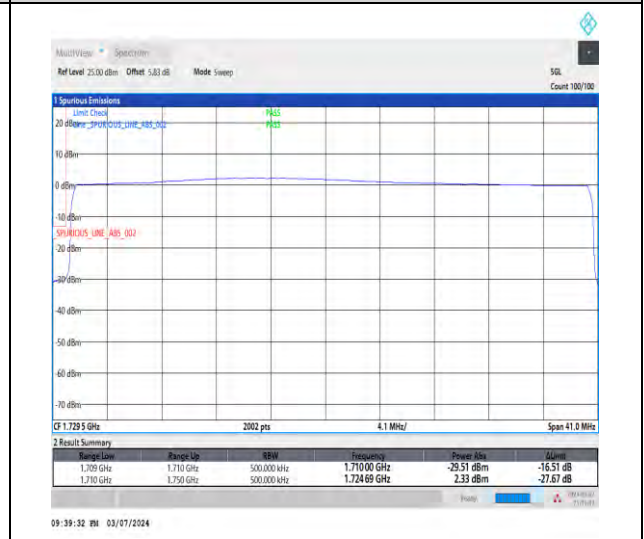
1-N66-15-40-L-6-CP-QPSK-Outer_Full-216@0-Ant1-1-seegraph-PASS-see graph
