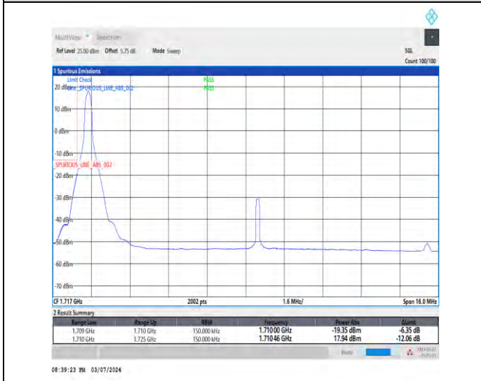
1-N66-15-15-L-4-CP-QPSK-Edge_1RB_Left-1@0-Ant1-1-seegraph-PASS-see graph
