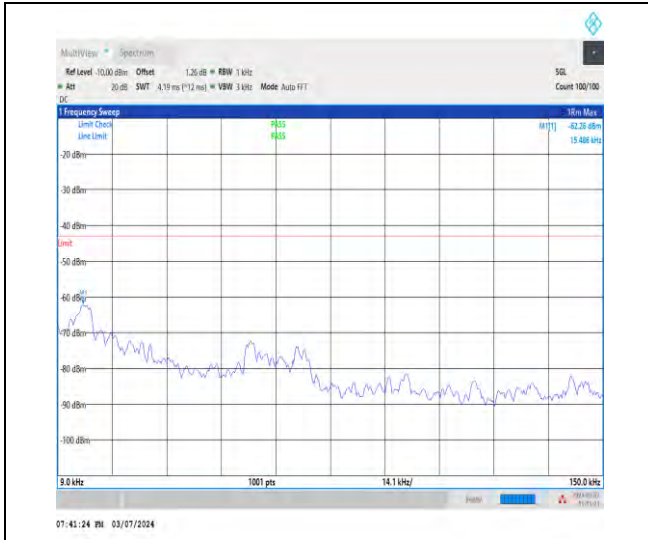
1-N66-15-40-H-1-DFT-PI2BPSK-Inner_1RB_Left-1 @ 1-0.009-0.15-Ant1-0.02--62.26--43-PASS
