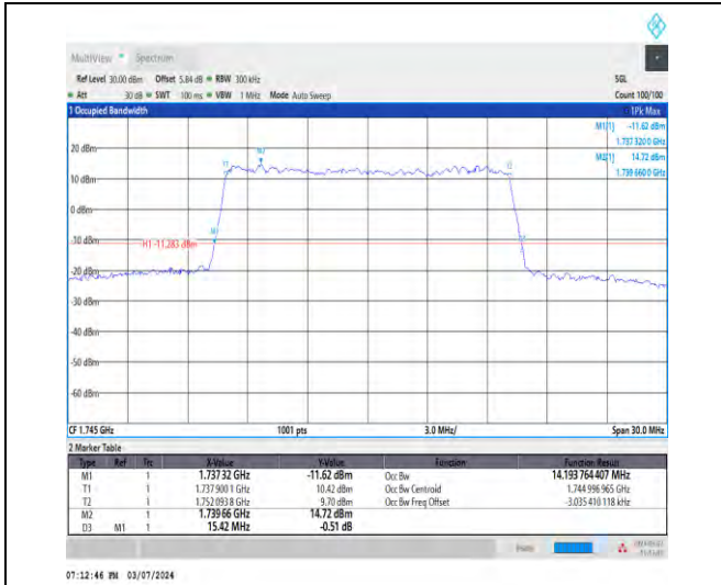
1-N66-15-15-M-7-CP-16QAM-Outer_Full-79@0-Ant1 -14.194-15.420-≤15-PASS
