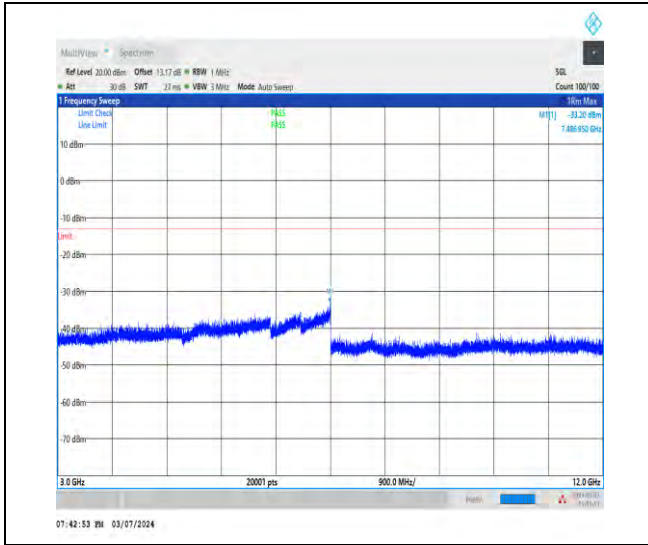
1-N66-15-40-H-1-DFT-PI2BPSK-Inner_1RB_Left-1 @ 1-3000-12000-Ant1-7486.95--33.20--13-PASS
