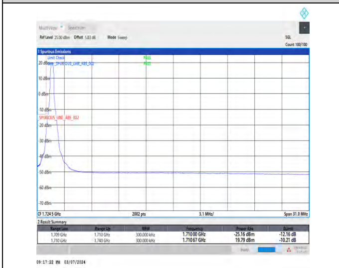
1-N66-15-30-L-4-CP-QPSK-Edge_1RB_Left-1@0-Ant1-1-seegraph-PASS-see graph
