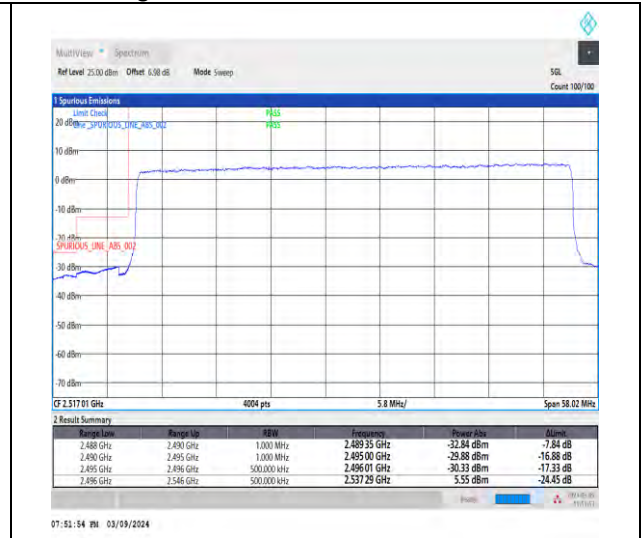
1-N41-30-50-L-3-DFT-PI2BPSK-Outer_Full-128@0-Ant1-1--PASS-see graph
