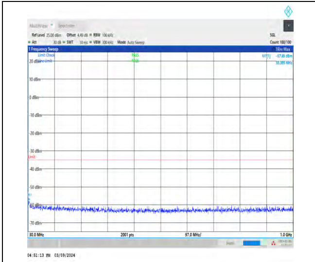
1-N41-30-100-M-1-DFT-PI2BPSK-Inner_1RB_Left-1 @1-30-1000-Ant1-33.40--57.89--35-PASS
