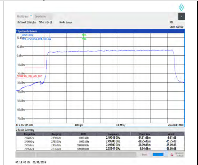
1-N41-30-40-L-3-DFT-PI2BPSK-Outer_Full-100@0-Ant1-1--PASS-see graph
