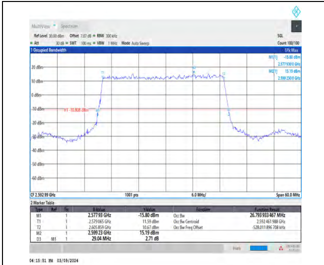
1-N41-30-30-M-2-DFT-PI2BPSK-Outer_Full-75@0-A nt1-26.794-29.040-≤30-PASS
