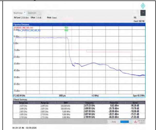
1-N41-30-20-H-3-DFT-PI2BPSK-Outer_Full-50@0-Ant1-1--PASS-see graph
