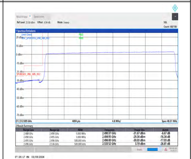
1-N41-30-40-L-6-CP-QPSK-Outer_Full-106@0-Ant1-1--PASS-see graph
