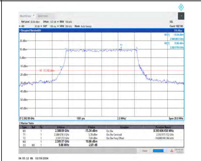
1-N41-30-10-M-8-CP-64QAM-Outer_Full-24@0-Ant1 -8.594-9.880-≤10-PASS
