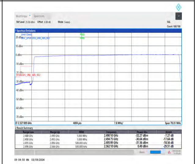
1-N41-30-70-L-6-CP-QPSK-Outer_Full-189@0-Ant1-1--PASS-see graph
