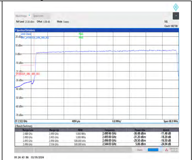
1-N41-30-60-L-3-DFT-PI2BPSK-Outer_Full-162@0-Ant1-1--PASS-see graph
