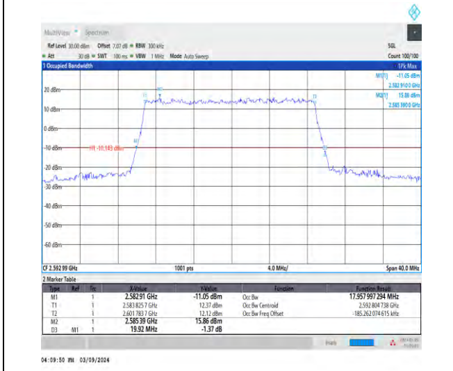
1-N41-30-20-M-1-DFT-QPSK-Outer_Full-50@0-Ant1 -17.958-19.920-≤20-PASS
