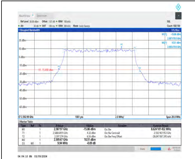
1-N41-30-10-M-5-DFT-256QAM-Outer_Full-24@0-A nt1-8.624-9.940-≤10-PASS
