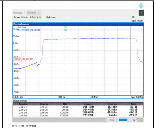
1-N41-30-30-L-3-DFT-PI2BPSK-Outer_Full-75@0-Ant1-1--PASS-see graph
