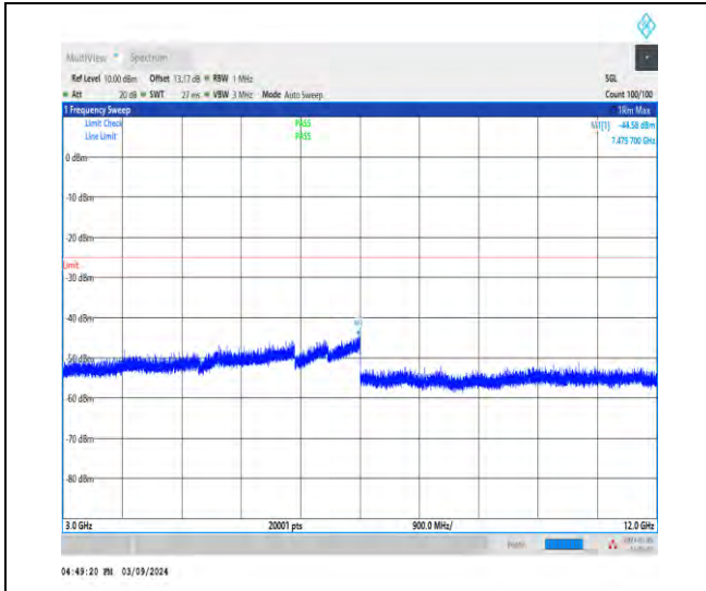
1-N41-30-100-L-1-DFT-PI2BPSK-Inner_1RB_Left-1 @ 1-3000-12000-Ant1-7475.70--44.58--25-PASS
