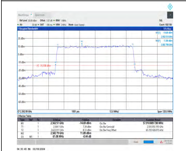
1-N41-30-60-M-9-CP-256QAM-Outer_Full-162@0-A nt1-57.911-61.080-<60-PASS
