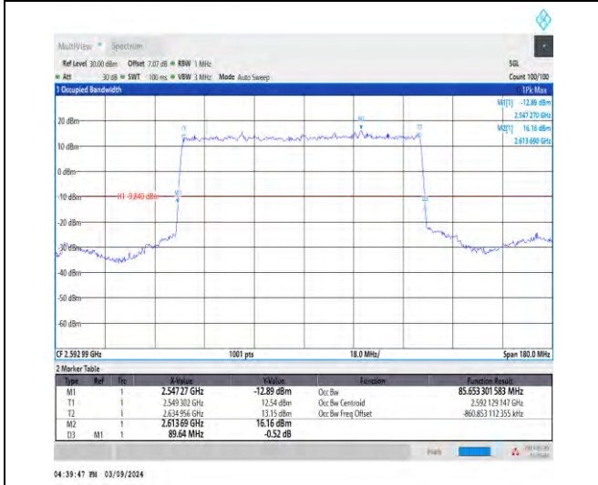
1-N41-30-90-M-2-DFT-PI2BPSK-Outer_Full-240@0-Ant1 1-85.653-89.640-≤90-PASS
