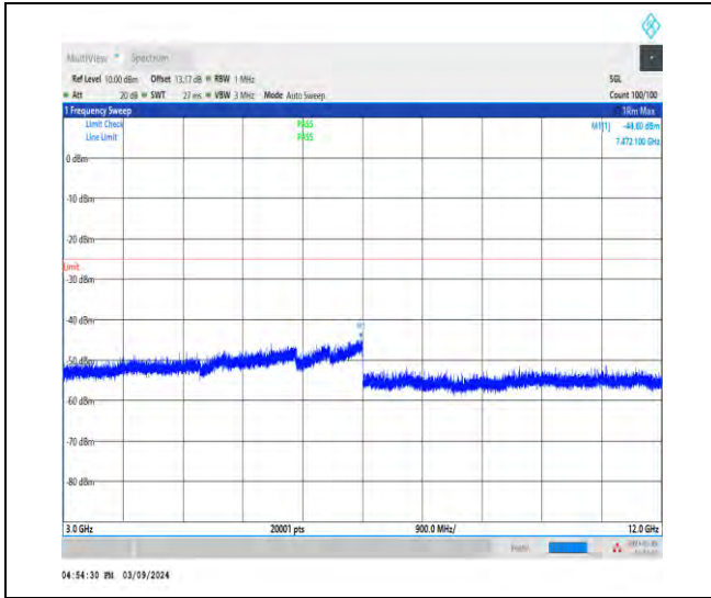
1-N41-30-100-H-1-DFT-PI2BPSK-Inner_1RB_Left-1 @1-3000-12000-Ant1-7472.10--44.80--25-PASS
