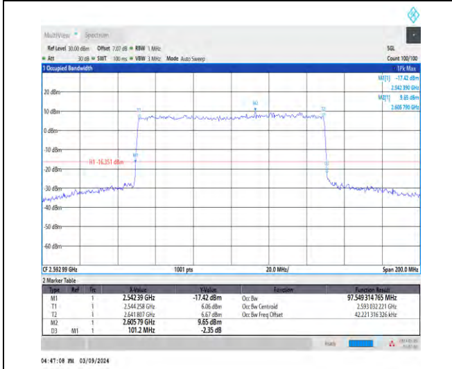
1-N41-30-100-M-9-CP-256QAM-Outer_Full-273@0-A Ant1-97.549-101.200-≤100-PASS
