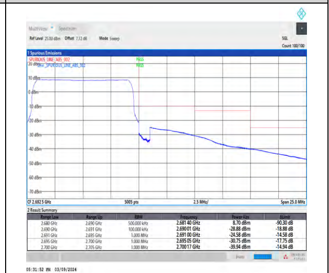
1-N41-30-10-H-6-CP-QPSK-Outer_Full-24@0-Ant1-1--PASS-see graph
