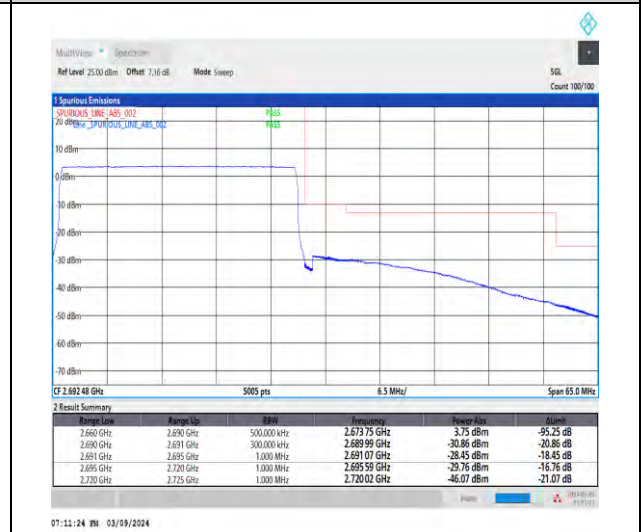
1-N41-30-30-H-6-CP-QPSK-Outer_Full-78@0-Ant1-1--PASS-see graph
