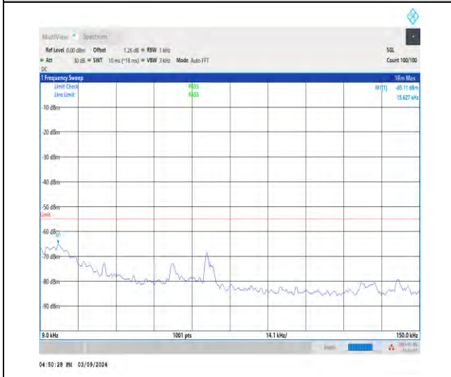
1-N41-30-100-M-1-DFT-PI2BPSK-Inner_1RB_Left-1 @ 1-0.009-0.15-Ant1-0.02--65.11--55-PASS
