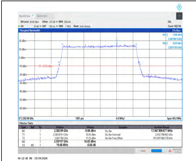
1-N41-30-20-M-3-DFT-16QAM-Outer_Full-50@0-Ant 1-17.968-19.680-≤20-PASS
