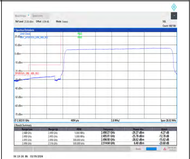
1-N41-30-20-L-6-CP-QPSK-Outer_Full-51@0-Ant1-1--PASS-see graph
