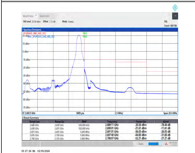
1-N41-30-10-H-5-CP-QPSK-Edge_1RB_Right-1@23-Ant1-1--PASS-see graph
