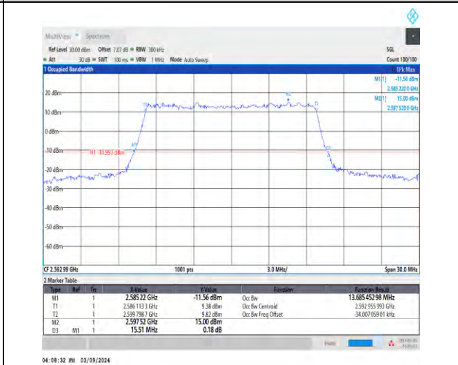
1-N41-30-15-M-7-CP-16QAM-Outer_Full-38@0-Ant1 -13.685-15.510-≤15-PASS
