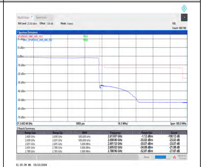
1-N41-30-90-H-6-CP-QPSK-Outer_Full-245@0-Ant1-1--PASS-see graph
