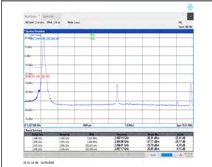
1-N41-30-70-L-4-CP-QPSK-Edge_1RB_Left-1@0-Ant1-1--PASS-see graph
