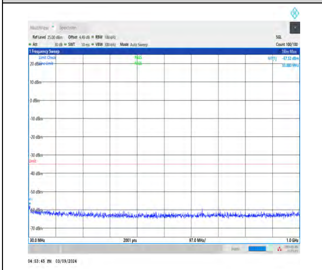
1-N41-30-100-H-1-DFT-PI2BPSK-Inner_1RB_Left-1 @1-30-1000-Ant1-33.88--57.52--35-PASS
