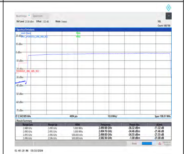
1-N41-30-100-L-6-CP-QPSK-Outer_Full-273@0-Ant1-1--PASS-see graph
