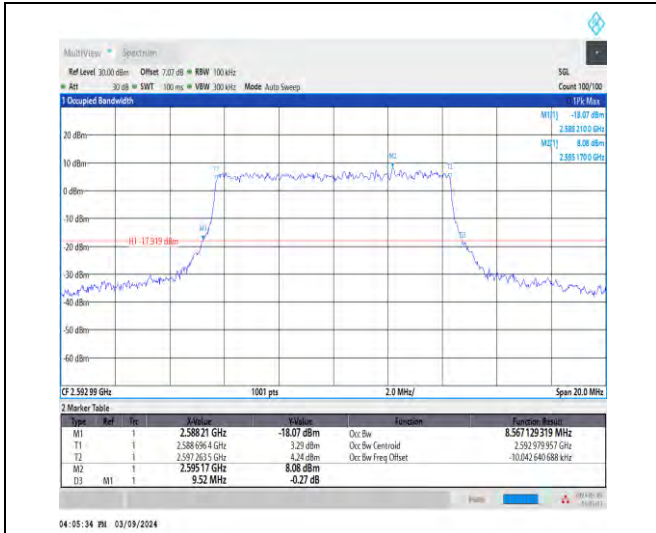
1-N41-30-10-M-9-CP-256QAM-Outer_Full-24@0-An t1-8.567-9.520-≤10-PASS
