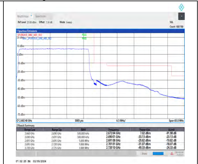
1-N41-30-30-H-3-DFT-PI2BPSK-Outer_Full-75@0-Ant1-1--PASS-see graph
