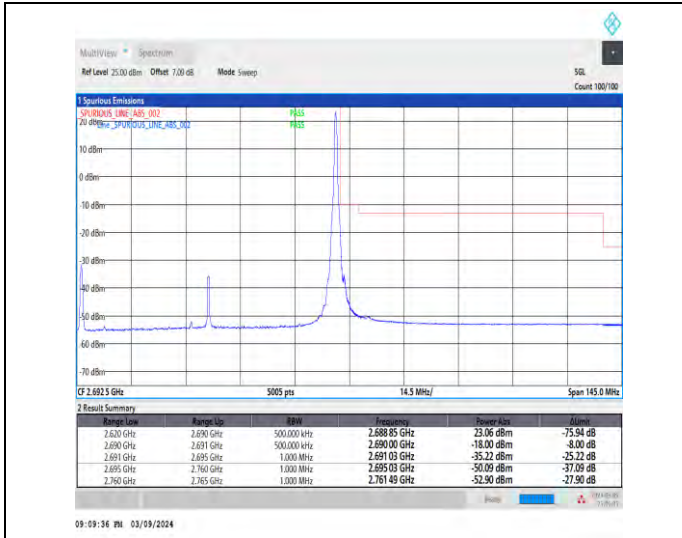
1-N41-30-70-H-2-DFT-PI2BPSK-Edge_1RB_Right-1@188-Ant1-1--PASS-see graph
