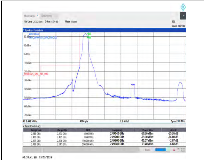
1-N41-30-15-L-1-DFT-PI2BPSK-Edge_1RB_Left-1@0-Ant1-1--PASS-see graph
