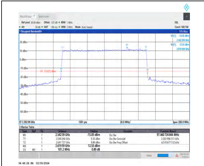
1-N41-30-100-M-7-CP-16QAM-Outer_Full-273@0-A Ant1-97.461-101.200-≤100-PASS
