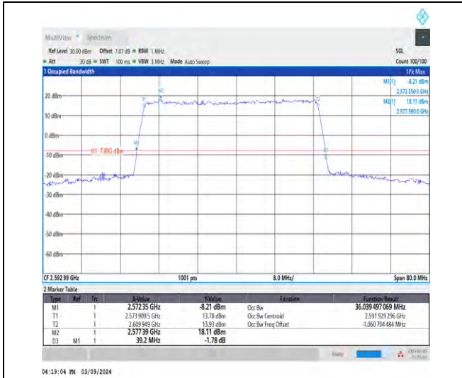
1-N41-30-40-M-1-DFT-QPSK-Outer_Full-100@0-Ant 1-36.039-39.200-≤40-PASS
