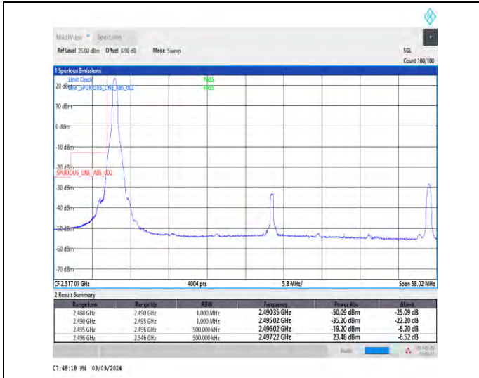
1-N41-30-50-L-1-DFT-PI2BPSK-Edge_1RB_Left-1@0-Ant1-1--PASS-see graph
