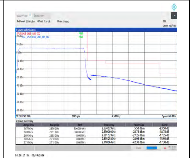
1-N41-30-20-H-6-CP-QPSK-Outer_Full-51@0-Ant1-1--PASS-see graph
