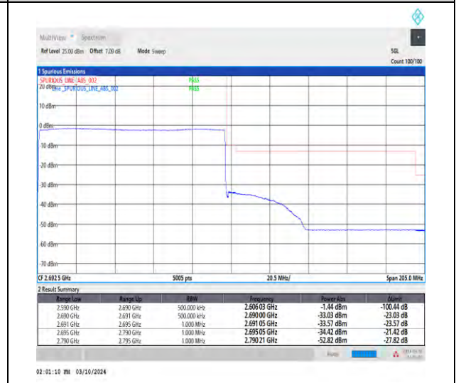
1-N41-30-100-H-6-CP-QPSK-Outer_Full-273@0-Ant1-1--PASS-see graph
