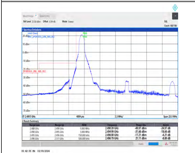
1-N41-30-15-L-4-CP-QPSK-Edge_1RB_Left-1@0-Ant1-1--PASS-see graph
