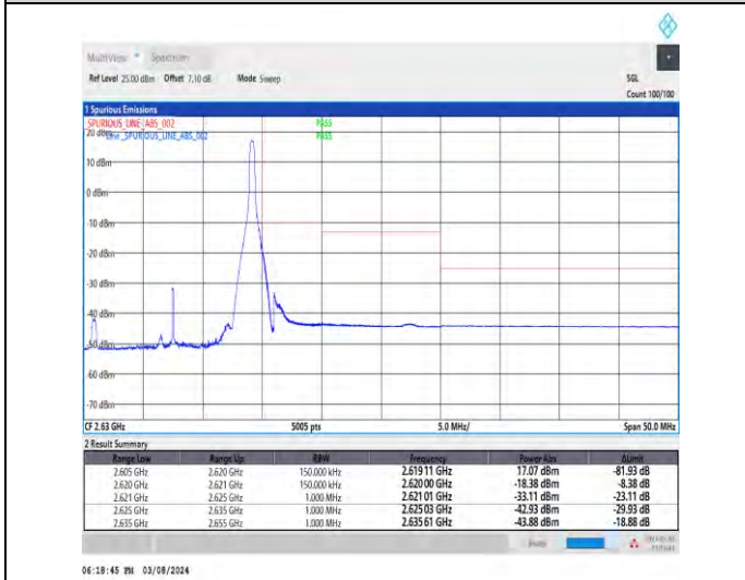
1-N38-30-15-H-5-CP-QPSK-Edge_1RB_Right-1@37-Ant1-1--PASS-see graph
