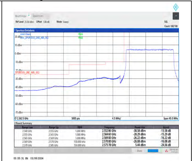
1-N38-30-15-L-3-DFT-PI2BPSK-Outer_Full-36@0-Ant1-1--PASS-see graph
