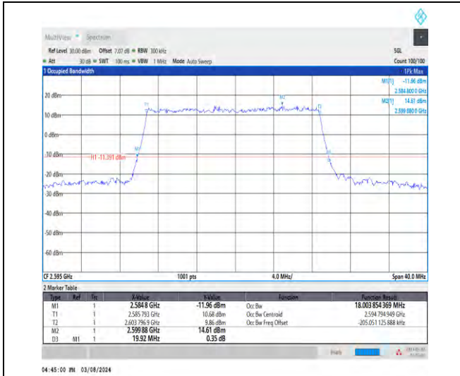
1-N38-30-20-M-3-DFT-16QAM-Outer_Full-50@0-Ant 1-18.004-19.920-≤20-PASS
