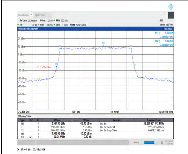
1-N38-30-20-M-9-CP-256QAM-Outer_Full-51@0-An t1-18.239-20.040-≤20-PASS
