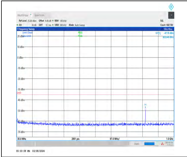
1-N38-30-40-M-1-DFT-PI2BPSK-Inner_1RB_Left-1 @ 1-30-1000-Ant1-823.95--47.79--35-PASS
