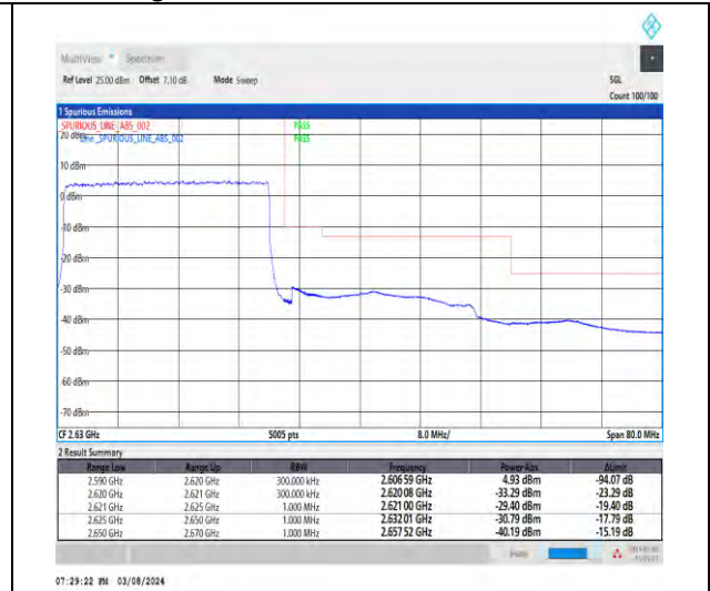
1-N38-30-30-H-3-DFT-PI2BPSK-Outer_Full-75@0-Ant1-1--PASS-see graph
