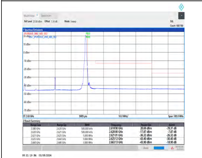
1-N38-30-40-H-5-CP-QPSK-Edge_1RB_Right-1@105-Ant1-1--PASS-see graph
