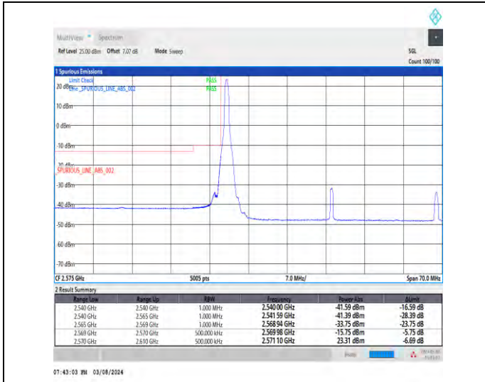
1-N38-30-40-L-1-DFT-PI2BPSK-Edge_1RB_Left-1@0-Ant1-1--PASS-see graph
