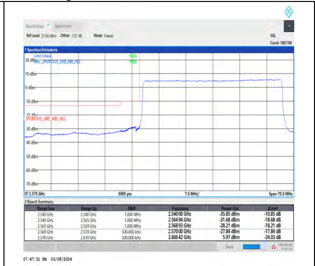
1-N38-30-40-L-3-DFT-PI2BPSK-Outer_Full-100@0-Ant1-1--PASS-see graph
