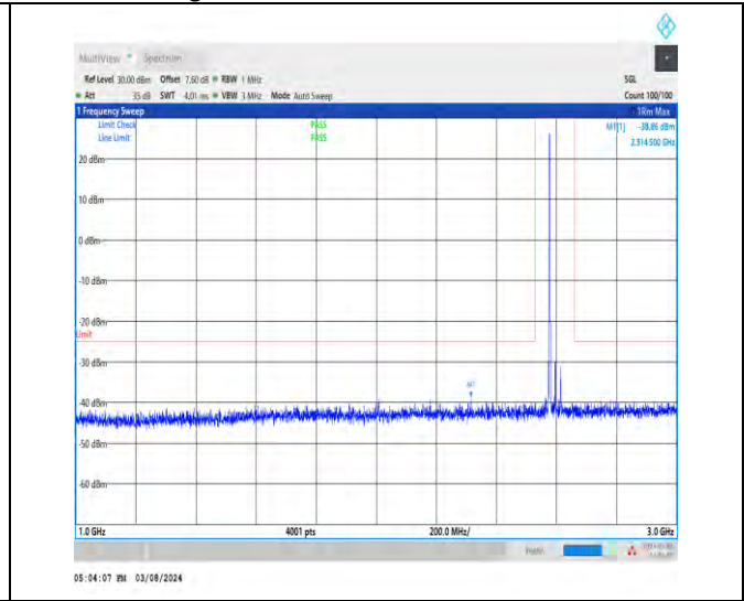
1-N38-30-40-M-1-DFT-PI2BPSK-Inner_1RB_Left-1@ 1-1000-3000-Ant1-2314.50--38.86--25-PASS
