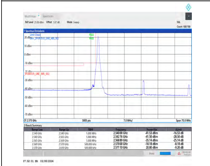
1-N38-30-40-L-4-CP-QPSK-Edge_1RB_Left-1@0-Ant1-1--PASS-see graph
