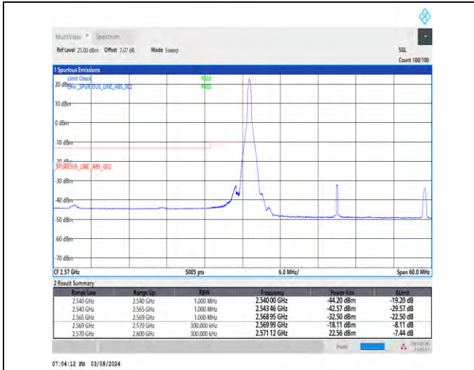
1-N38-30-30-L-1-DFT-PI2BPSK-Edge_1RB_Left-1@0-Ant1-1--PASS-see graph
