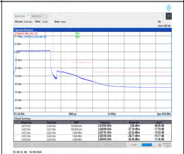
1-N38-30-10-H-6-CP-QPSK-Outer_Full-24@0-Ant1-1--PASS-see graph
