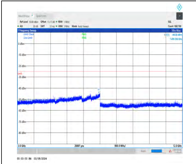
1-N38-30-40-L-1-DFT-PI2BPSK-Inner_1RB_Left-1 @ 1-3000-12000-Ant1-7439.25--44.58--25-PASS
