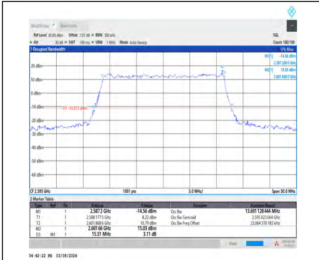
1-N38-30-15-M-8-CP-64QAM-Outer_Full-38@0-Ant 1-13.691-15.510-≤15-PASS
