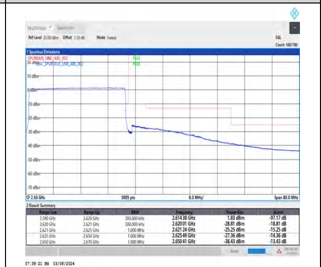
1-N38-30-30-H-6-CP-QPSK-Outer_Full-78@0-Ant1-1--PASS-see graph
