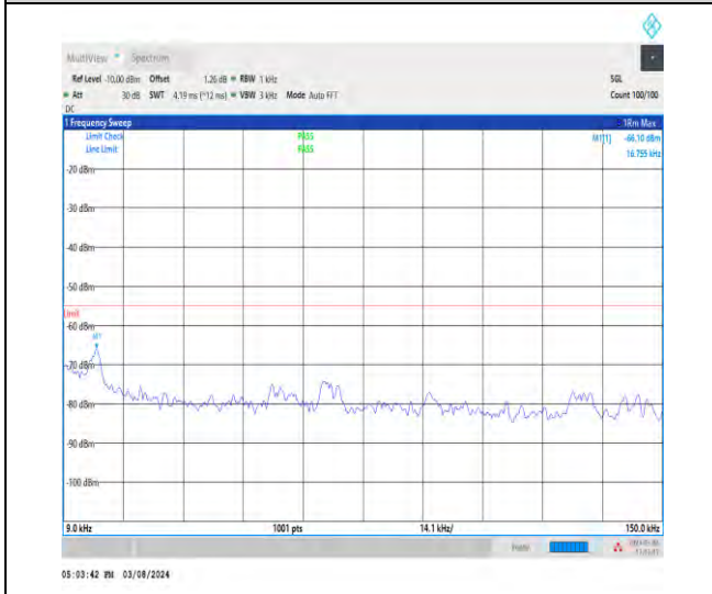
1-N38-30-40-M-1-DFT-PI2BPSK-Inner_1RB_Left-1 @ 1-0.009-0.15-Ant1-0.02--66.10--55-PASS
