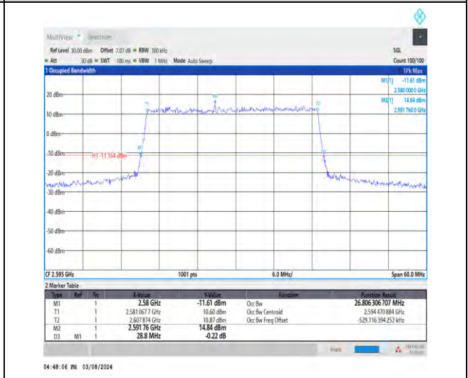
1-N38-30-30-M-1-DFT-QPSK-Outer_Full-75@0-Ant1 -26.806-28.800-≤30-PASS
