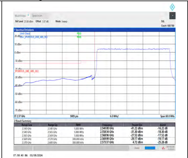
1-N38-30-30-L-3-DFT-PI2BPSK-Outer_Full-75@0-Ant1-1--PASS-see graph
