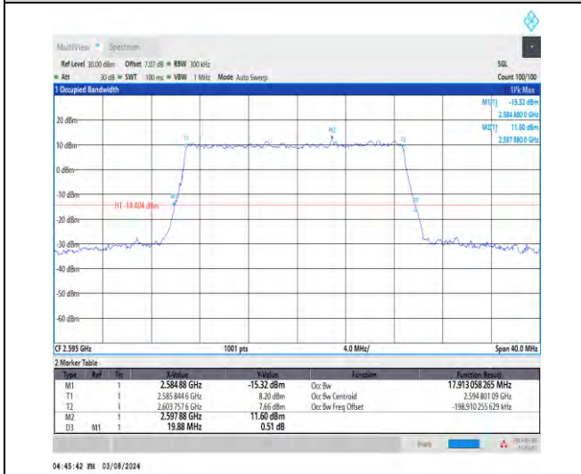
1-N38-30-20-M-5-DFT-256QAM-Outer_Full-50@0-Ant 1-17.913-19.880-≤20-PASS
