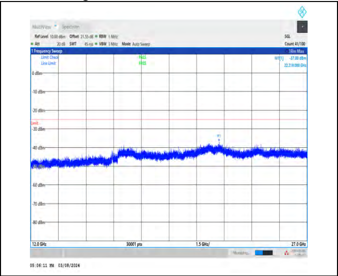
1-N38-30-40-H-1-DFT-PI2BPSK-Inner_1RB_Left-1@ 1-12000-27000-Ant1-22218.00--37.00--25-PASS
