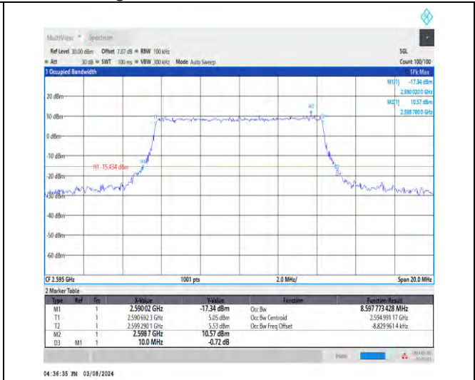
1-N38-30-10-M-6-CP-QPSK-Outer_Full-24@0-Ant1- 8.598-10.000-≤10-PASS
