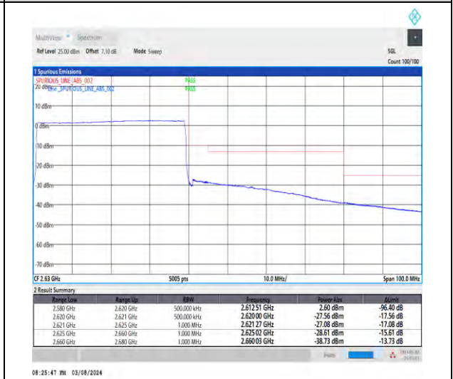
1-N38-30-40-H-6-CP-QPSK-Outer_Full-106@0-Ant1-1--PASS-see graph
