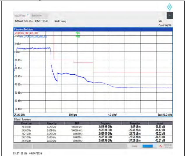
1-N38-30-10-H-3-DFT-PI2BPSK-Outer_Full-24@0-Ant1-1--PASS-see graph
