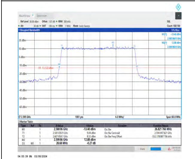
1-N38-30-30-M-4-DFT-64QAM-Outer_Full-75@0-Ant 1-26.822-28.680-≤30-PASS
