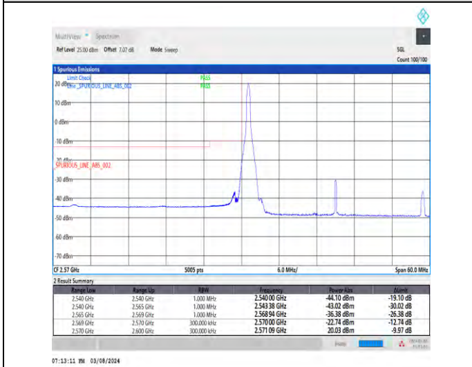
1-N38-30-30-L-4-CP-QPSK-Edge_1RB_Left-1@0-Ant1-1--PASS-see graph
