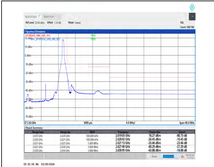
1-N38-30-10-H-2-DFT-PI2BPSK-Edge_1RB_Right-1@23-Ant1-1--PASS-see graph
