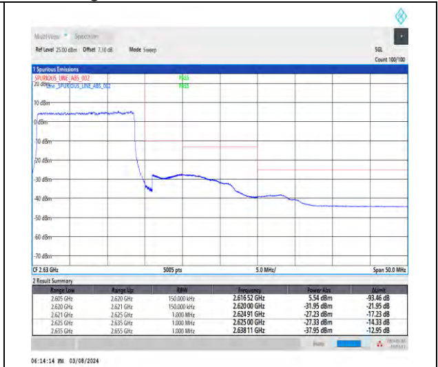
1-N38-30-15-H-3-DFT-PI2BPSK-Outer_Full-36@0-Ant1-1--PASS-see graph
