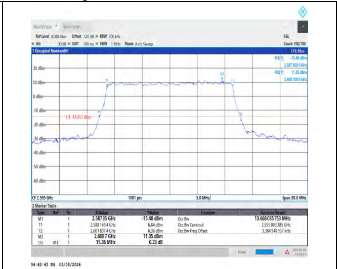
1-N38-30-15-M-9-CP-256QAM-Outer_Full-38@0-Ant 1-13.668-15.360-≤15-PASS
