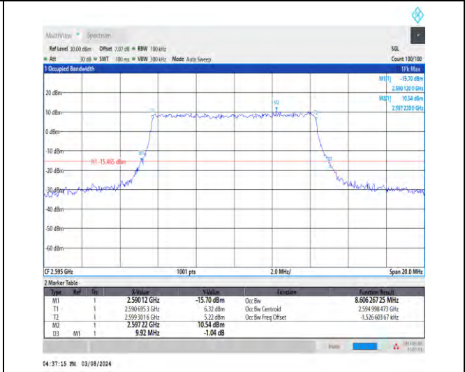
1-N38-30-10-M-8-CP-64QAM-Outer_Full-24@0-Ant1 -8.606-9.920-≤10-PASS
