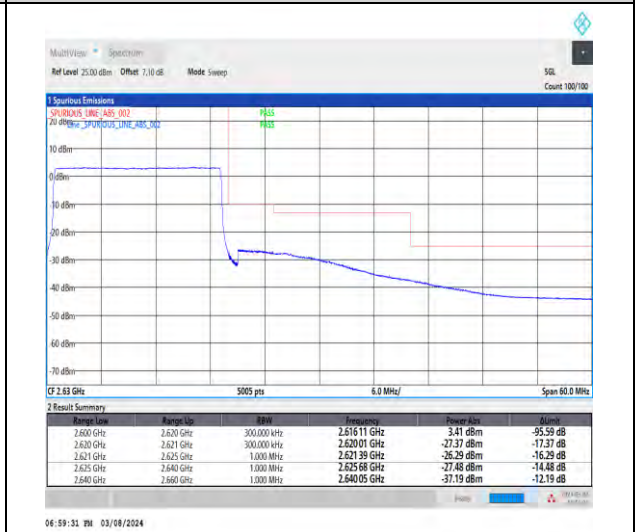
1-N38-30-20-H-6-CP-QPSK-Outer_Full-51@0-Ant1-1--PASS-see graph
