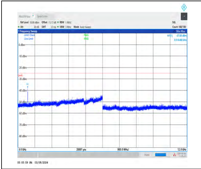
1-N38-30-40-H-1-DFT-PI2BPSK-Inner_1RB_Left-1 @ 1-3000-12000-Ant1-3518.40--37.93--25-PASS
