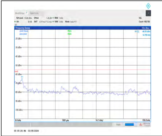
1-N38-30-40-H-1-DFT-PI2BPSK-Inner_1RB_Left-1 @ 1-0.009-0.15-Ant1-0.02--66.50--55-PASS
