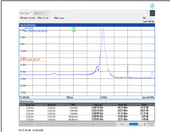
1-N38-30-20-L-1-DFT-PI2BPSK-Edge_1RB_Left-1@0-Ant1-1--PASS-see graph
