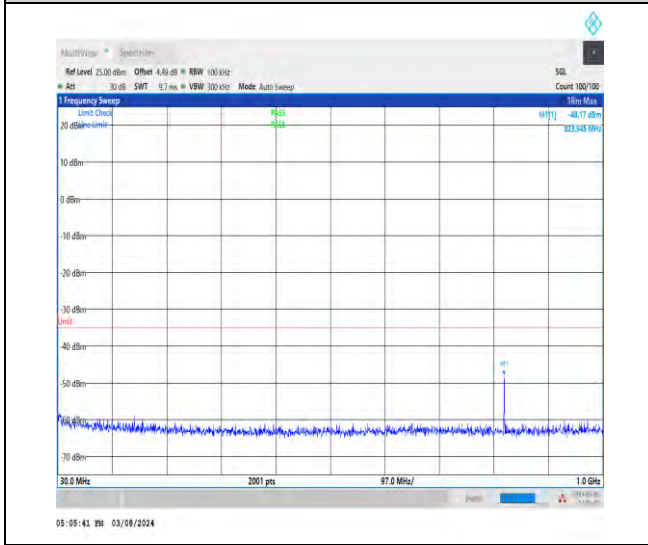
1-N38-30-40-H-1-DFT-PI2BPSK-Inner_1RB_Left-1 @ 1-30-1000-Ant1-823.95--48.17--35-PASS
