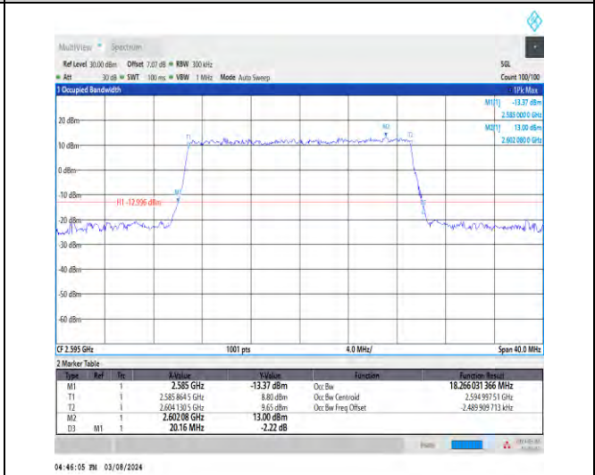
1-N38-30-20-M-6-CP-QPSK-Outer_Full-51@0-Ant 1-18.266-20.160-≤20-PASS
