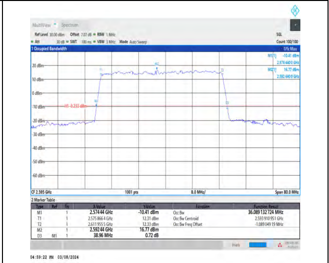
1-N38-30-40-M-4-DFT-64QAM-Outer_Full-100@0-A nt1-36.089-38.960-≤40-PASS
