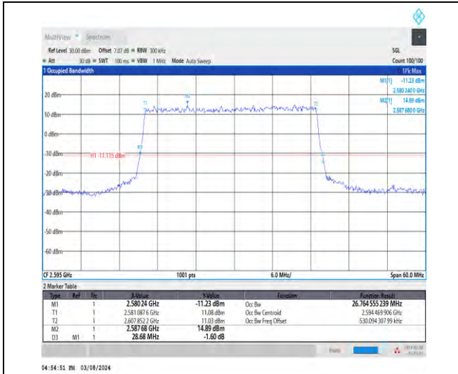
1-N38-30-30-M-2-DFT-PI2BPSK-Outer_Full-75@0-A nt1-26.765-28.680-≤30-PASS
