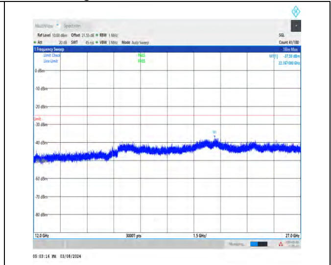
1-N38-30-40-L-1-DFT-PI2BPSK-Inner_1RB_Left-1@ 1-12000-27000-Ant1-22167.00--37.59--25-PASS
