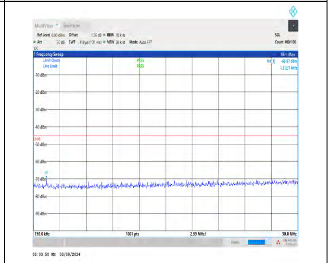
1-N38-30-40-M-1-DFT-PI2BPSK-Inner_1RB_Left-1@ 1-0.15-30-Ant1-1.61--69.87--45-PASS
