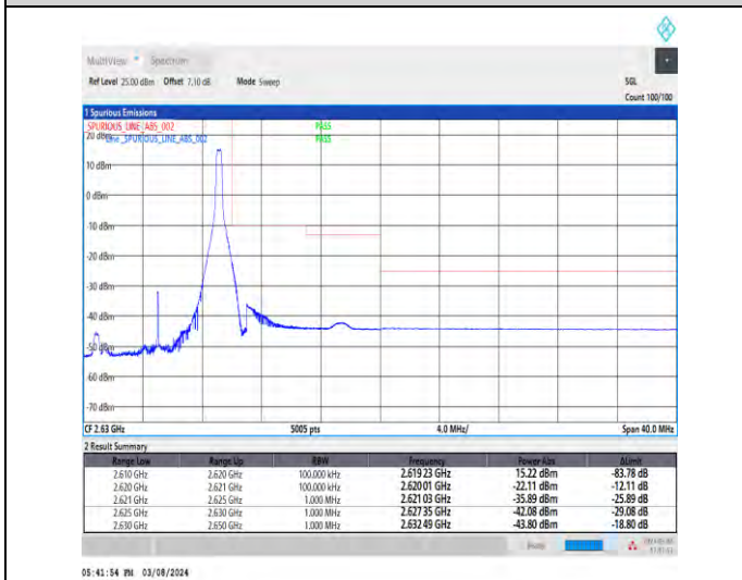
1-N38-30-10-H-5-CP-QPSK-Edge_1RB_Right-1@23-Ant1-1--PASS-see graph
