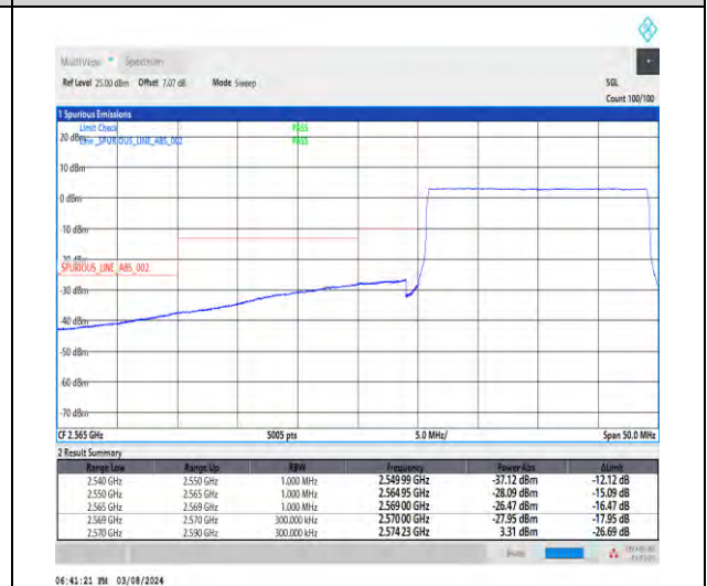
1-N38-30-20-L-6-CP-QPSK-Outer_Full-51@0-Ant1-1--PASS-see graph
