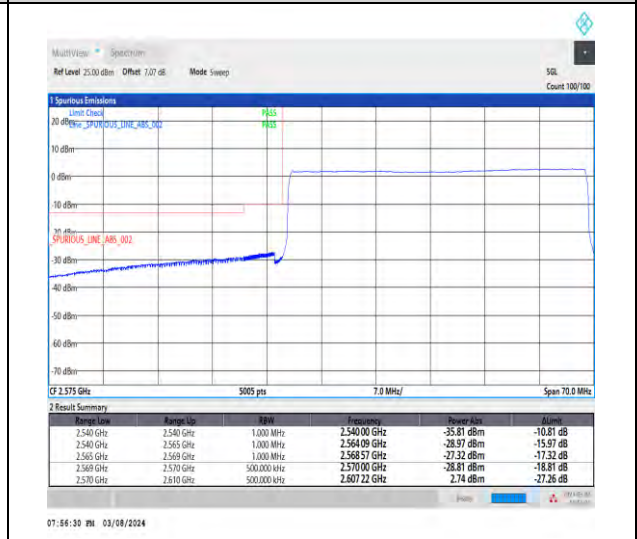
1-N38-30-40-L-6-CP-QPSK-Outer_Full-106@0-Ant1-1--PASS-see graph
