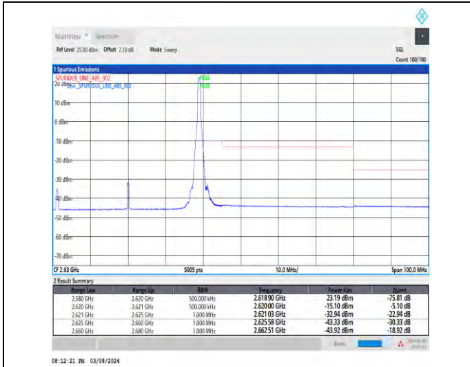
1-N38-30-40-H-2-DFT-PI2BPSK-Edge_1RB_Right-1@105-Ant1-1--PASS-see graph
