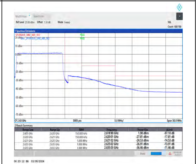
1-N38-30-15-H-6-CP-QPSK-Outer_Full-38@0-Ant1-1--PASS-see graph
