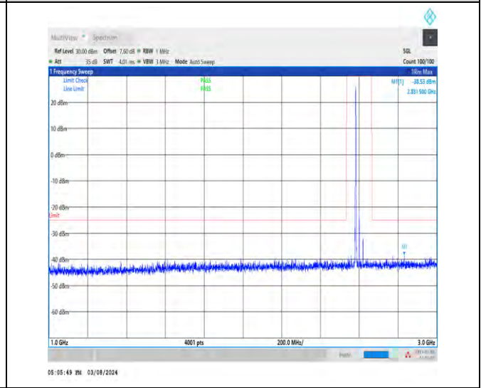
1-N38-30-40-H-1-DFT-PI2BPSK-Inner_1RB_Left-1 @ 1-1000-3000-Ant1-2831.50--38.53--25-PASS
