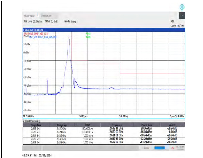
1-N38-30-15-H-2-DFT-PI2BPSK-Edge_1RB_Right-1@37-Ant1-1--PASS-see graph
