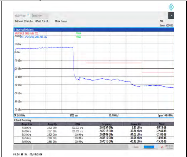
1-N38-30-40-H-3-DFT-PI2BPSK-Outer_Full-100@0-Ant1-1--PASS-see graph
