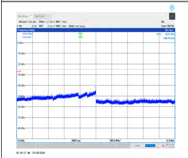
1-N38-30-40-M-1-DFT-PI2BPSK-Inner_1RB_Left-1 @ 1-3000-12000-Ant1-7488.75--44.62--25-PASS
