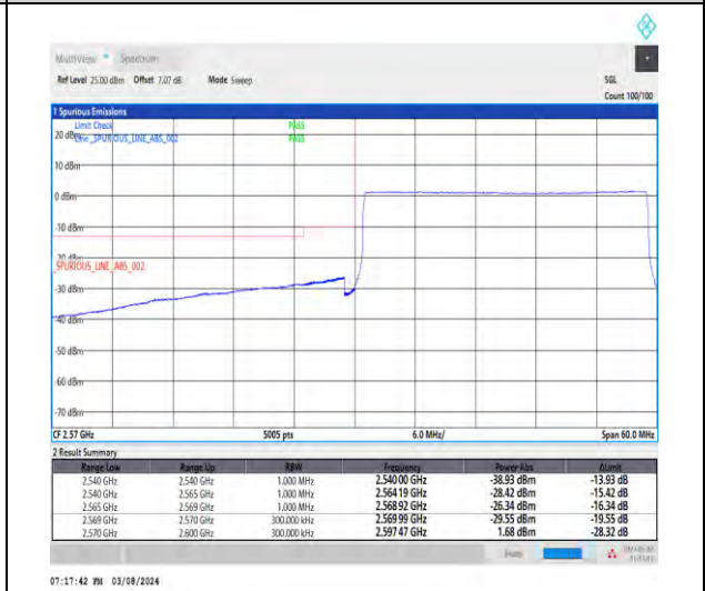
1-N38-30-30-L-6-CP-QPSK-Outer_Full-78@0-Ant1-1--PASS-see graph
