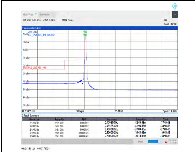
1-N7-15-30-L-4-CP-QPSK-Edge_1RB_Left-1@0-Ant1-1--PASS-see graph
