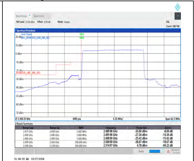
1-N7-15-25-L-3-DFT-PI2BPSK-Outer_Full-128@0 -Ant1-1--PASS-see graph
