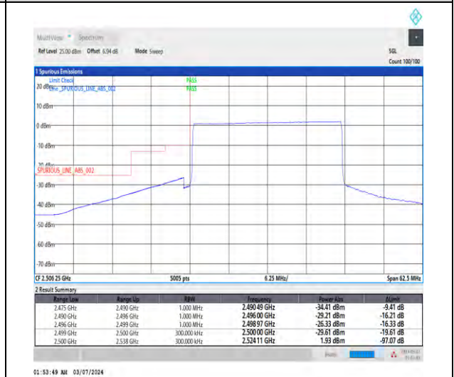
1-N7-15-25-L-6-CP-QPSK-Outer_Full-133@0-Ant1-1--PASS-see graph
