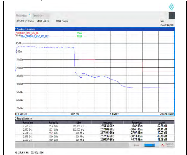
1-N7-15-20-H-3-DFT-PI2BPSK-Outer_Full-100@0-Ant1-1--PASS-see graph
