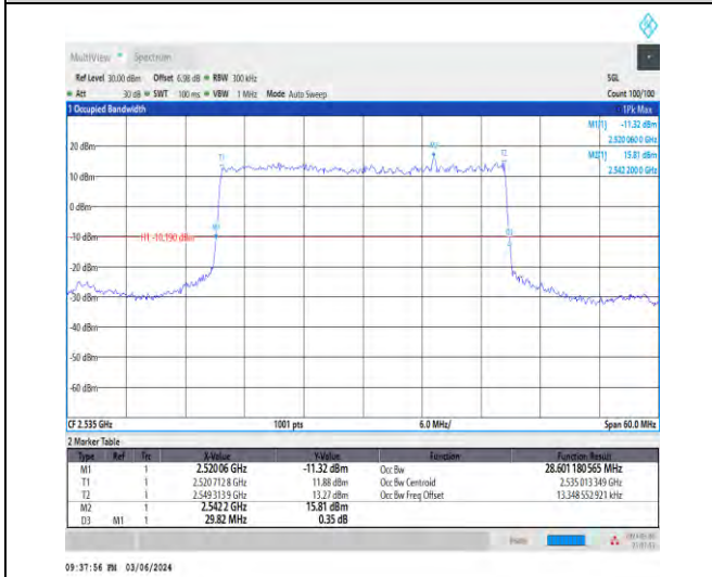
1-N7-15-30-M-2-DFT-PI2BPSK-Outer_Full-160@0-A nt1-28.601-29.820-≤30-PASS
