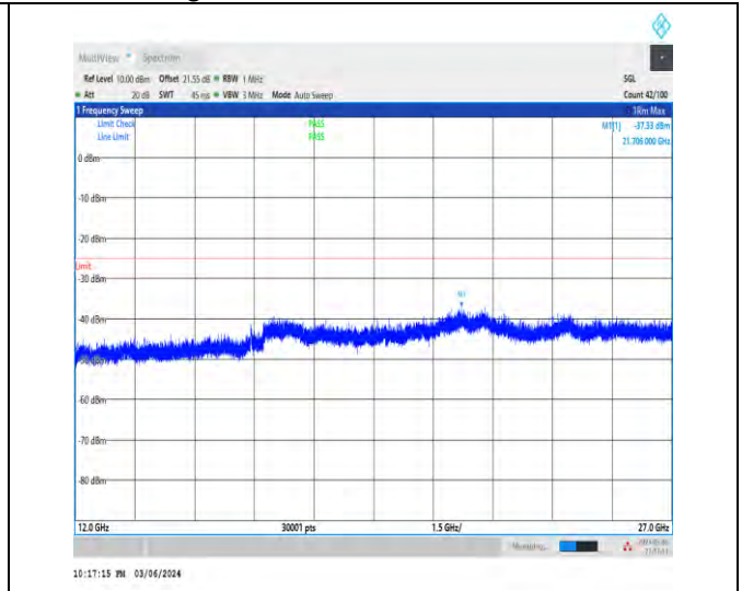
1-N7-15-40-L-1-DFT-PI2BPSK-Inner_1RB_Left-1@1- 12000-27000-Ant1-21162.00--37.33--25-PASS
