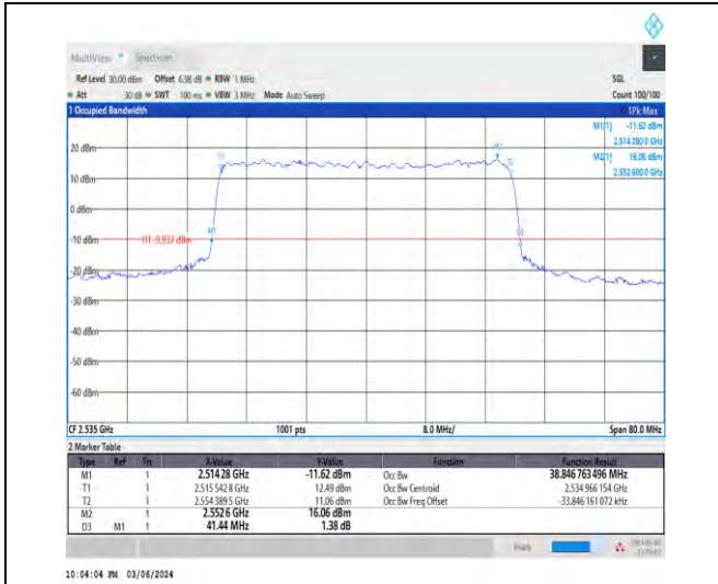
1-N7-15-40-M-7-CP-16QAM-Outer_Full-216@0-Ant1 -38.847-41.440-≤40-PASS
