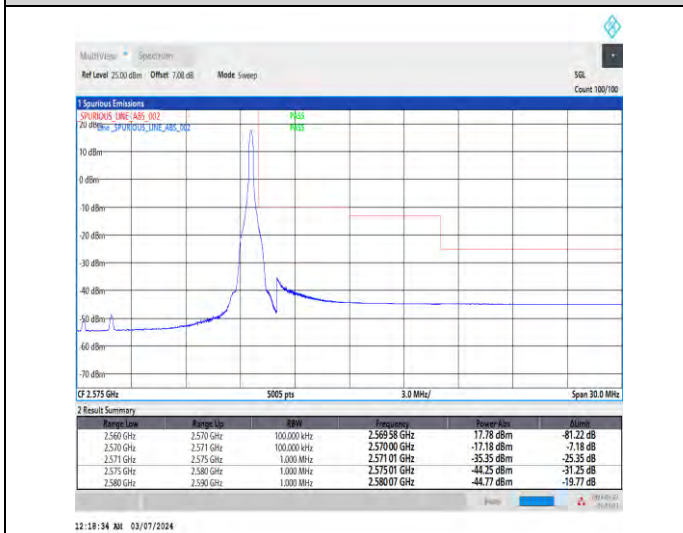
1-N7-15-10-H-5-CP-QPSK-Edge_1RB_Right-1@51-Ant1-1--PASS-see graph
