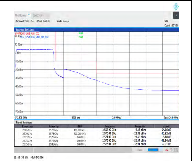
1-N7-15-5-H-6-CP-QPSK-Outer_Full-25@0-Ant1-1--PASS-see graph
