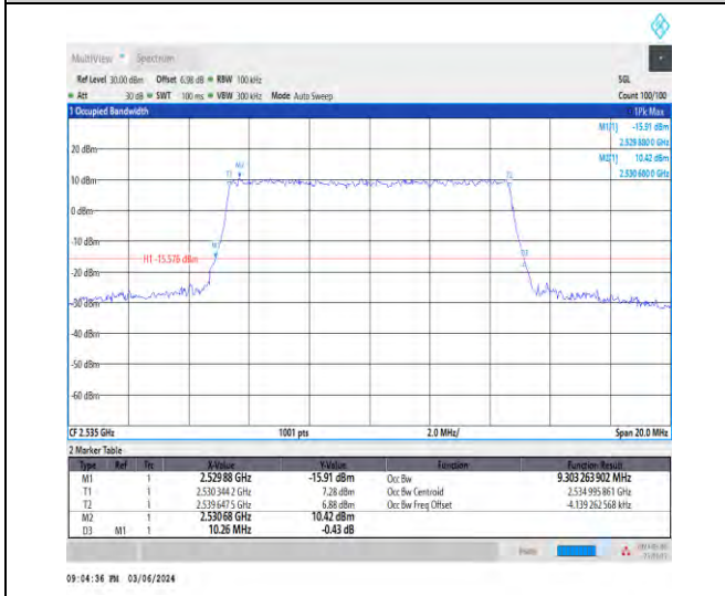
1-N7-15-10-M-6-CP-QPSK-Outer_Full-52@0-Ant1-9. 303-10.260-≤10-PASS
