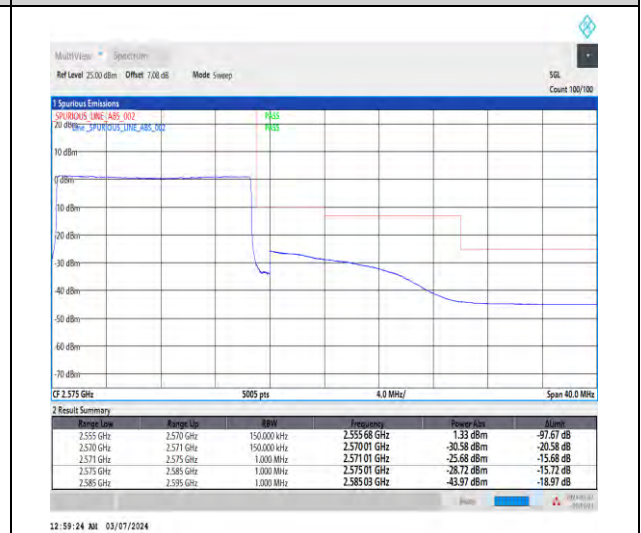
1-N7-15-15-H-6-CP-QPSK-Outer_Full-79@0-Ant1-1--PASS-see graph
