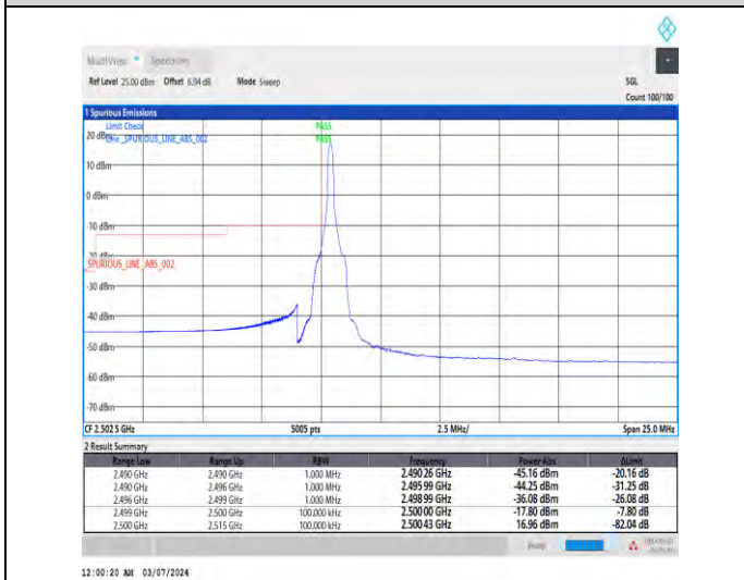
1-N7-15-10-L-4-CP-QPSK-Edge_1RB_Left-1@0-A nt1-1--PASS-see graph
