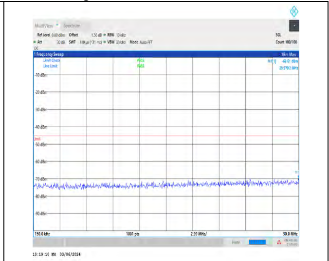
1-N7-15-40-H-1-DFT-PI2BPSK-Inner_1RB_Left-1@ -0.15-30-Ant1-29.97--69.61--45-PASS
