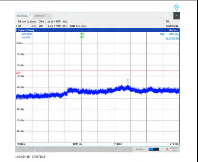
1-N7-15-40-M-1-DFT-PI2BPSK-Inner_1RB_Left-1@ -12000-27000-Ant1-22283.50--37.04--25-PASS
