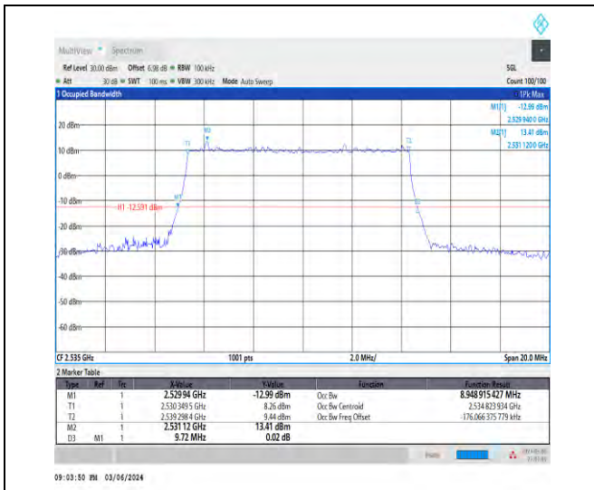
1-N7-15-10-M-4-DFT-64QAM-Outer_Full-50@0-Ant1 -8.949-9.720-≤10-PASS
