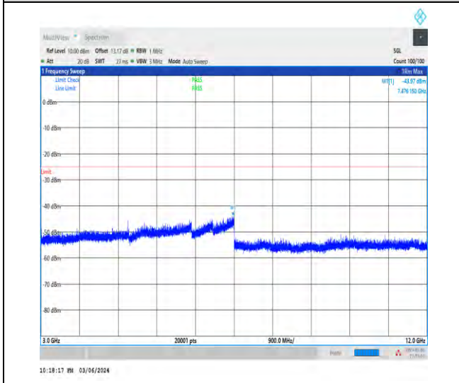
1-N7-15-40-M-1-DFT-PI2BPSK-Inner_1RB_Left-1@ 1-3000-12000-Ant1-7476.15--43.97--25-PASS
