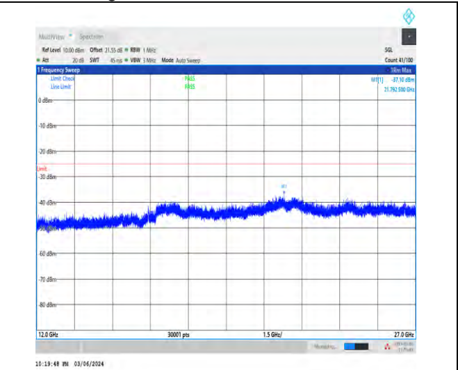
1-N7-15-40-H-1-DFT-PI2BPSK-Inner_1RB_Left-1@ -12000-27000-Ant1-21792.50--37.10--25-PASS
