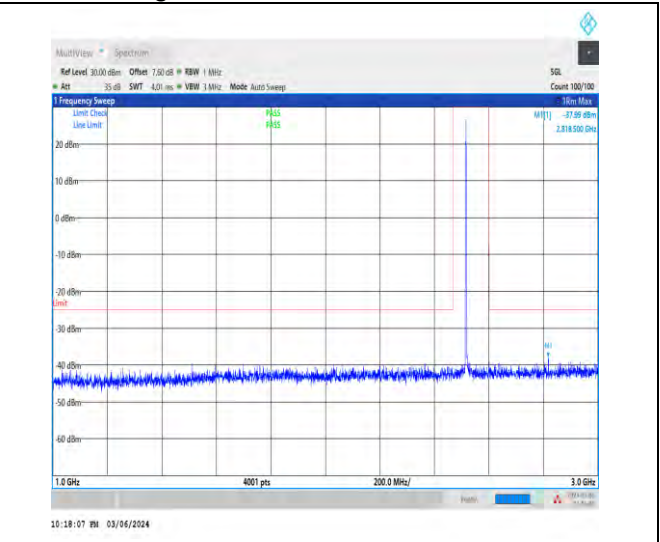
1-N7-15-40-M-1-DFT-PI2BPSK-Inner_1RB_Left-1@ -1000-3000-Ant1-2117.00--37.99--25-PASS
