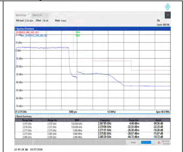
1-N7-15-15-H-3-DFT-PI2BPSK-Outer_Full-75@0- Ant1-1--PASS-see graph
