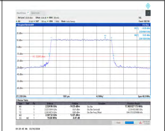
1-N7-15-20-M-5-DFT-256QAM-Outer_Full-100@0-A nt1-17.903-19.040-≤20-PASS
