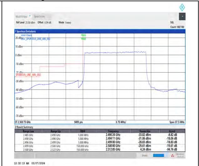
1-N7-15-15-L-3-DFT-PI2BPSK-Outer_Full-75@0-A nt1-1--PASS-see graph
