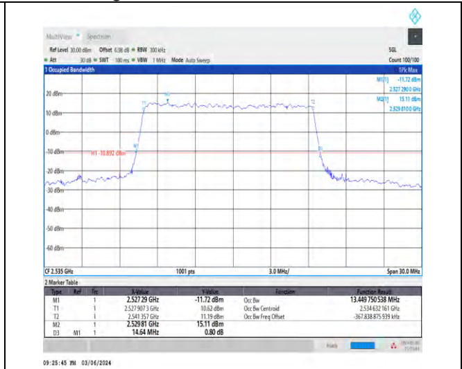
1-N7-15-15-M-4-DFT-64QAM-Outer_Full-75@0-Ant1 -13.45-14.640-≤15-PASS
