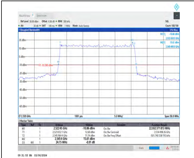
1-N7-15-25-M-1-DFT-QPSK-Outer_Full-128@0-Ant1 -22.932-24.150-≤25-PASS
