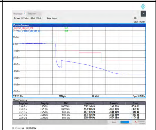
1-N7-15-10-H-6-CP-QPSK-Outer_Full-52@0-Ant1-1--PASS-see graph
