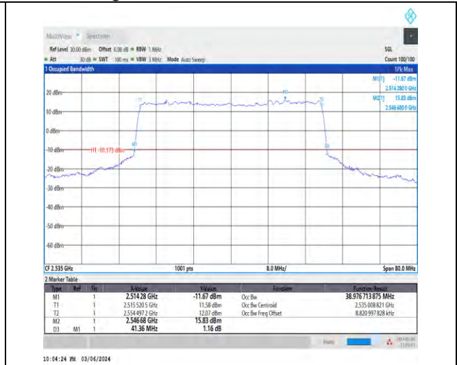
1-N7-15-40-M-8-CP-64QAM-Outer_Full-216@0-Ant1 -38.977-41.360-≤40-PASS
