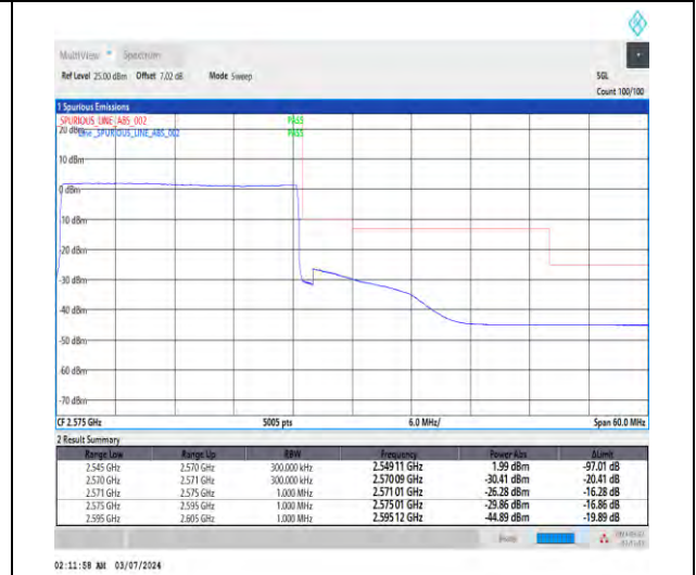
1-N7-15-25-H-6-CP-QPSK-Outer_Full-133@0-Ant 1-1--PASS-see graph
