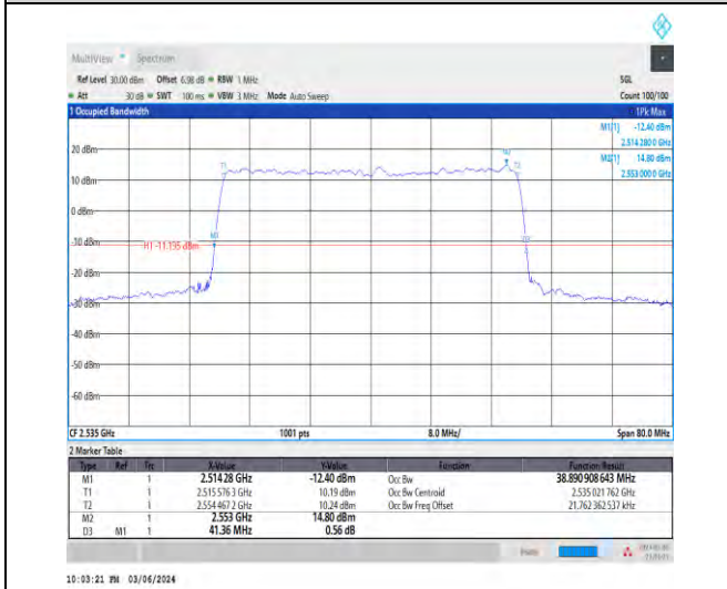
1-N7-15-40-M-5-DFT-256QAM-Outer_Full-216@0-A nt1-38.891-41.360-≤40-PASS
