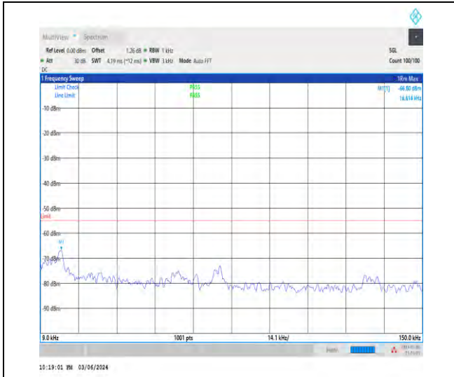
1-N7-15-40-H-1-DFT-PI2BPSK-Inner_1RB_Left-1@ 1-0.009-0.15-Ant1-0.02--66.80--55-PASS
