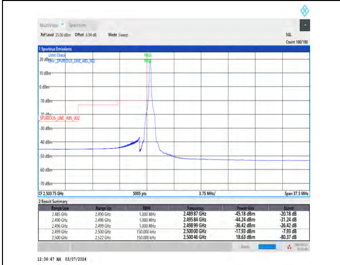
1-N7-15-15-L-4-CP-QPSK-Edge_1RB_Left-1@0-A nt1-1--PASS-see graph
