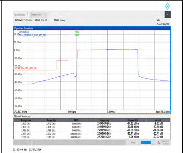
1-N7-15-30-L-6-CP-QPSK-Outer_Full-160@0-Ant1-1--PASS-see graph
