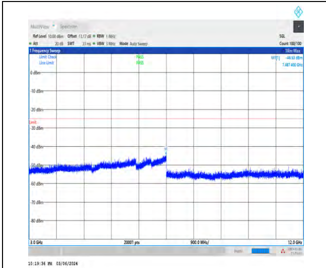
1-N7-15-40-H-1-DFT-PI2BPSK-Inner_1RB_Left-1@ 1-3000-12000-Ant1-7487.40--44.63--25-PASS
