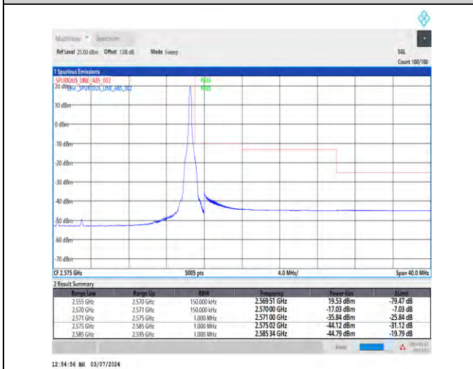
1-N7-15-15-H-5-CP-QPSK-Edge_1RB_Right-1@78-Ant1-1--PASS-see graph
