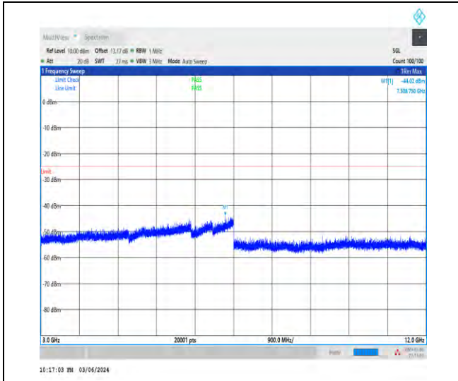
1-N7-15-40-L-1-DFT-PI2BPSK-Inner_1RB_Left-1@ 1-3000-12000-Ant1-7496.40--44.02--25-PASS
