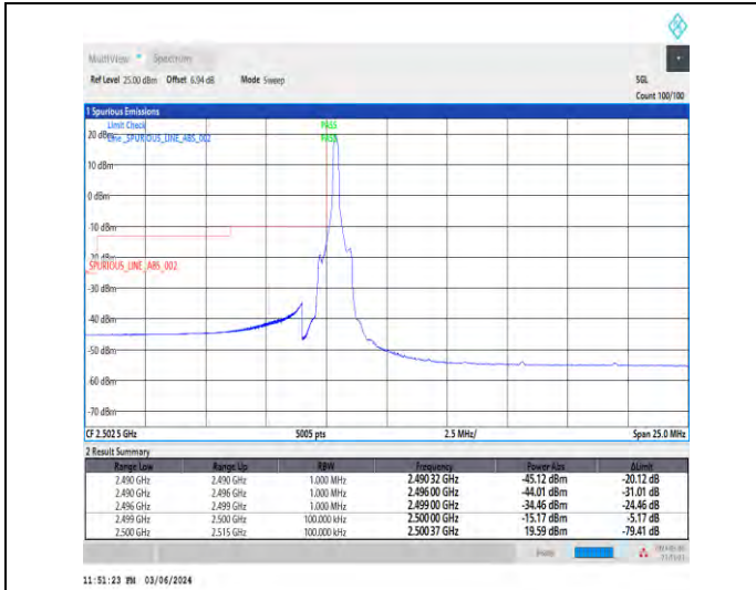
1-N7-15-10-L-1-DFT-PI2BPSK-Edge_1RB_Left-1@0-A nt1-1--PASS-see graph
