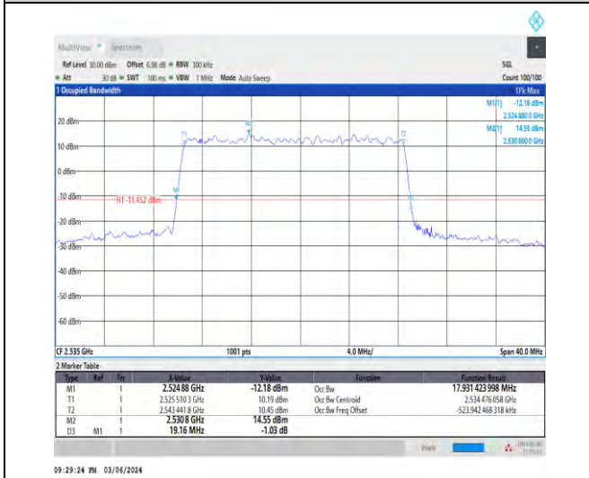
1-N7-15-20-M-4-DFT-64QAM-Outer_Full-100@0-Ant 1-17.931-19.160-≤20-PASS
