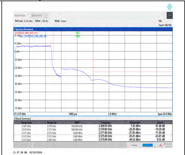
1-N7-15-5-H-3-DFT-PI2BPSK-Outer_Full-25@0-Ant1-1--PASS-see graph
