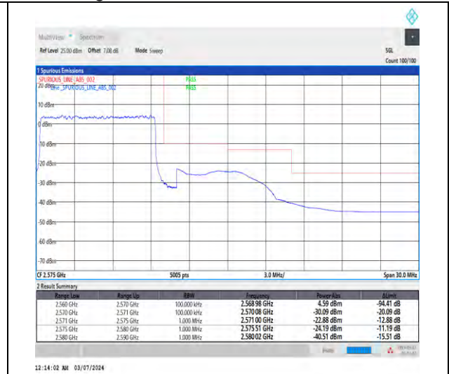
1-N7-15-10-H-3-DFT-PI2BPSK-Outer_Full-50@0- Ant1-1--PASS-see graph
