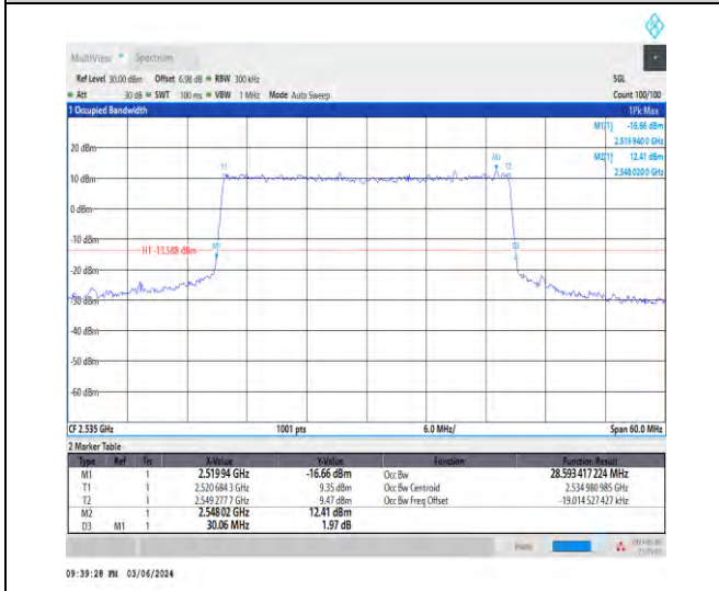
1-N7-15-30-M-6-CP-QPSK-Outer_Full-160@0-Ant1 28.593-30.060-≤30-PASS
