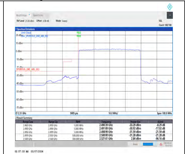
1-N7-15-40-L-3-DFT-PI2BPSK-Outer_Full-216@0 -Ant1-1--PASS-see graph
