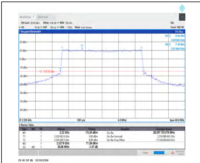
1-N7-15-30-M-8-CP-64QAM-Outer_Full-160@0-Ant1 -28.592-30.060-≤30-PASS
