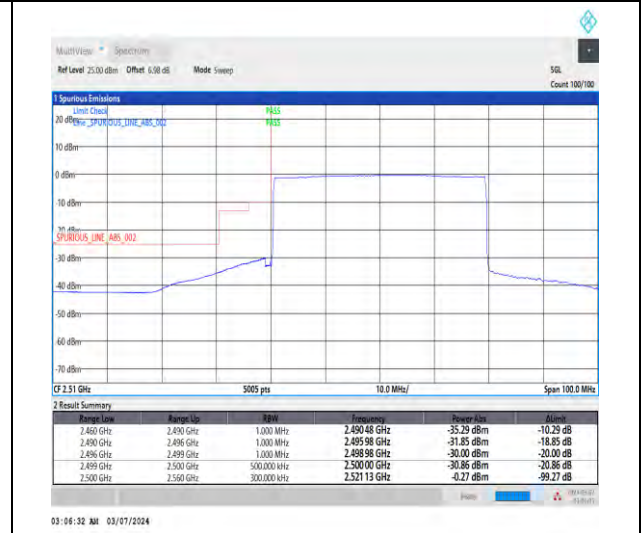
1-N7-15-40-L-6-CP-QPSK-Outer_Full-216@0-Ant 1-1--PASS-see graph
