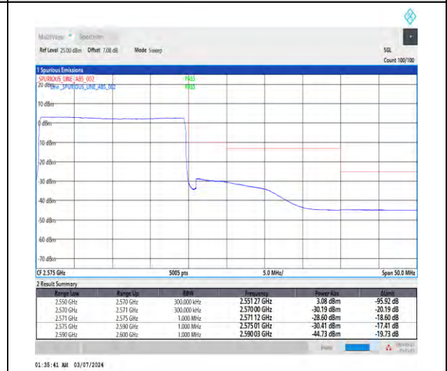
1-N7-15-20-H-6-CP-QPSK-Outer_Full-106@0-Ant1-1--PASS-see graph
