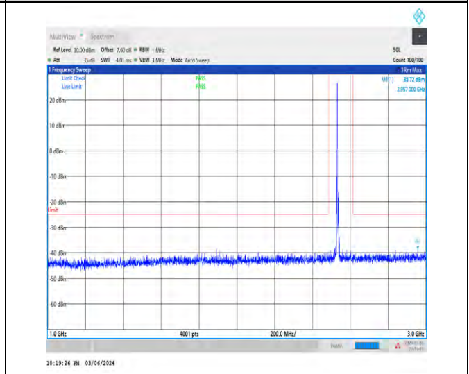
1-N7-15-40-H-1-DFT-PI2BPSK-Inner_1RB_Left-1@ -1000-3000-Ant1-2957.00--38.72--25-PASS
