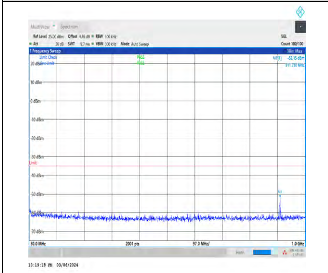
1-N7-15-40-H-1-DFT-PI2BPSK-Inner_1RB_Left-1@ 1-30-1000-Ant1-911.73--52.15--35-PASS
