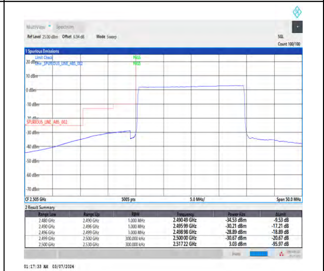
1-N7-15-20-L-6-CP-QPSK-Outer_Full-106@0-Ant1-1--PASS-see graph
