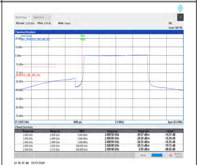
1-N7-15-10-L-6-CP-QPSK-Outer_Full-52@0-A nt1-1--PASS-see graph
