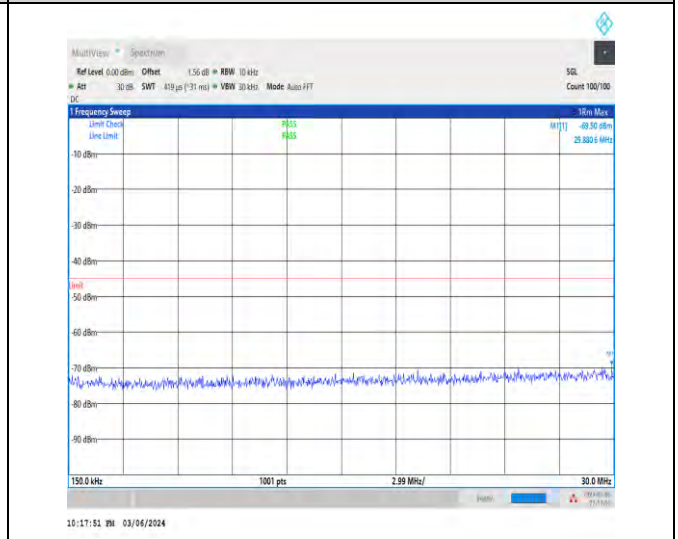
1-N7-15-40-M-1-DFT-PI2BPSK-Inner_1RB_Left-1@1 -0.15-30-Ant1-28.45--69.50--45-PASS
