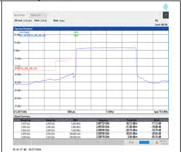
1-N7-15-30-L-3-DFT-PI2BPSK-Outer_Full-160@0 -Ant1-1--PASS-see graph
