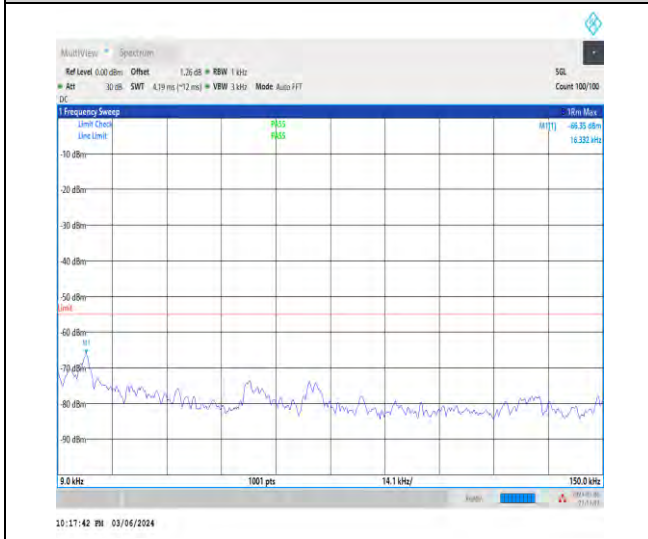
1-N7-15-40-M-1-DFT-PI2BPSK-Inner_1RB_Left-1@ 1-0.009-0.15-Ant1-0.02--66.35--55-PASS
