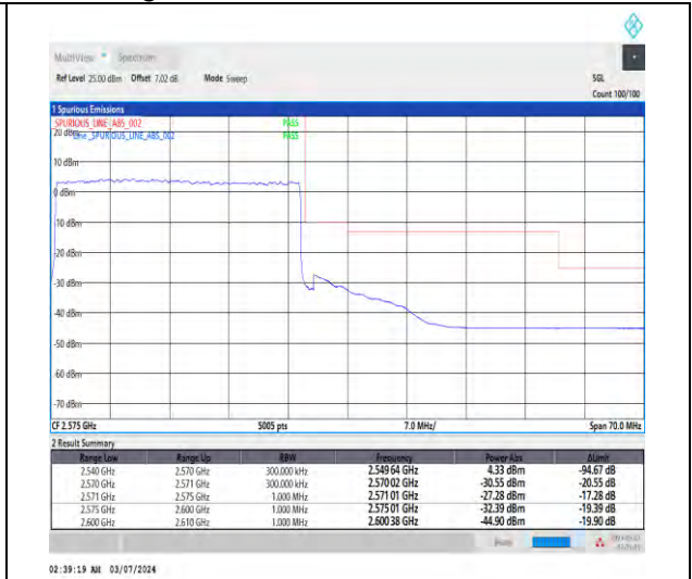
1-N7-15-30-H-3-DFT-PI2BPSK-Outer_Full-160@0 -Ant1-1--PASS-see graph
