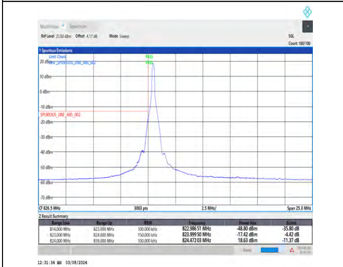
1-N5-15-15-L-4-CP-QPSK-Edge_1RB_Left-1@0-Ant1-1--PASS-see graph
