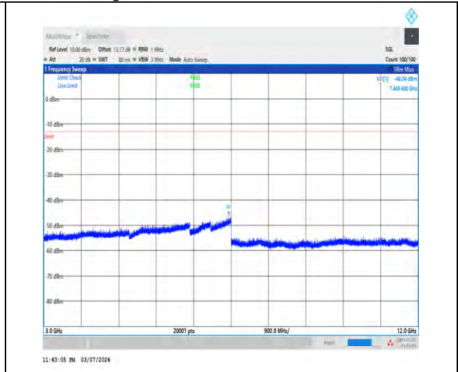
1-N5-15-20-M-1-DFT-PI2BPSK-Inner_1RB_Left-1@ 1-3000-12000-Ant1-7449.60--46.04--13-PASS
