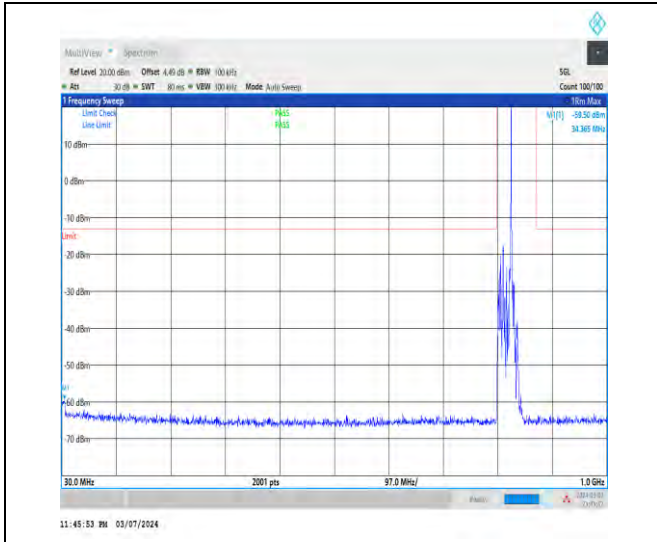
1-N5-15-20-H-1-DFT-PI2BPSK-Inner_1RB_Left-1@1 -30-1000-Ant1-34.37--59.50--13-PASS
