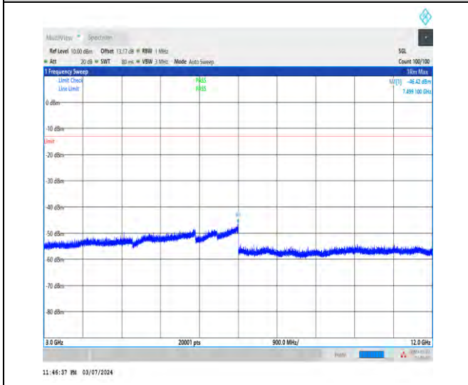
1-N5-15-20-H-1-DFT-PI2BPSK-Inner_1RB_Left-1@1 -3000-12000-Ant1-7499.10--46.42--13-PASS
