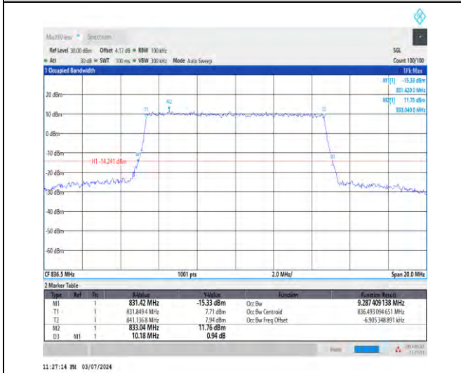
1-N5-15-10-M-6-CP-QPSK-Outer_Full-52@0-Ant1-9. 287-10.180-≤10-PASS
