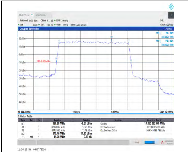
1-N5-15-20-M-2-DFT-PI2BPSK-Outer_Full-100@0-A nt1-17.855-19.080-≤20-PASS
