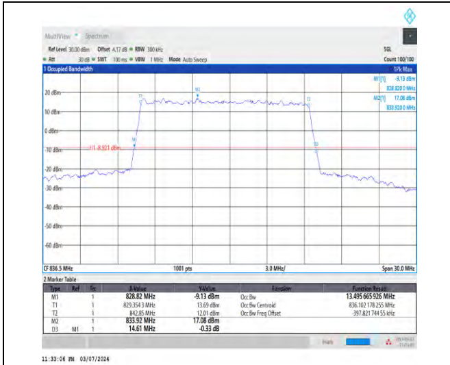
1-N5-15-15-M-3-DFT-16QAM-Outer_Full-75@0-Ant1 -13.496-14.610-≤15-PASS
