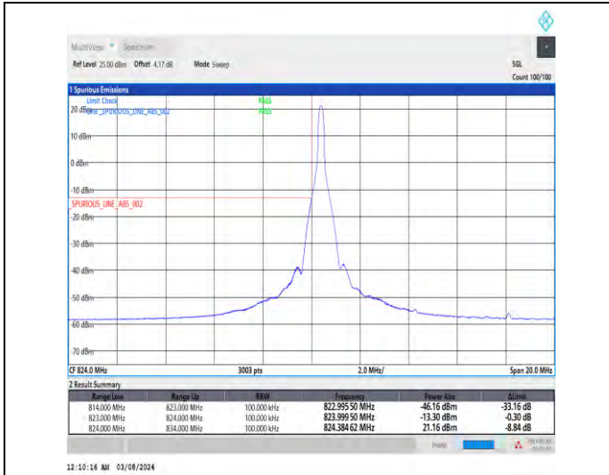
1-N5-15-10-L-1-DFT-PI2BPSK-Edge_1RB_Left-1@0-Ant1-1--PASS-see graph
