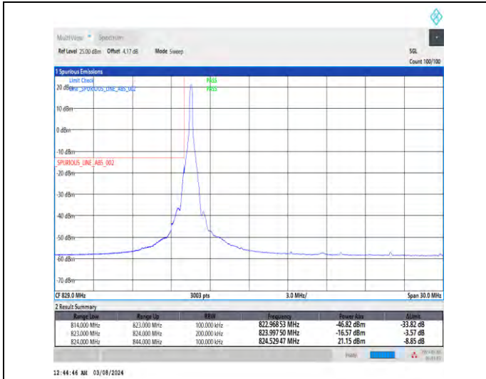
1-N5-15-20-L-1-DFT-PI2BPSK-Edge_1RB_Left-1@0-Ant1-1--PASS-see graph
