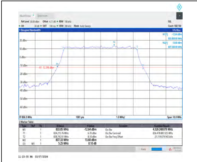
1-N5-15-5-M-5-DFT-256QAM-Outer_Full-25@0-Ant1 -4.526-5.250-≤5-PASS
