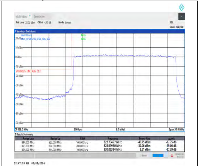
1-N5-15-20-L-3-DFT-PI2BPSK-Outer_Full-100@0-Ant1-1--PASS-see graph
