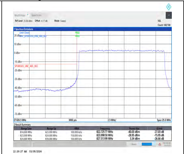
1-N5-15-15-L-3-DFT-PI2BPSK-Outer_Full-75@0-Ant1-1--PASS-see graph
