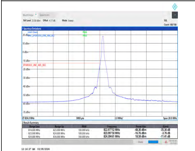
1-N5-15-10-L-4-CP-QPSK-Edge_1RB_Left-1@0-Ant1-1--PASS-see graph
