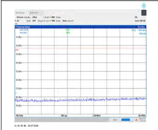
1-N5-15-20-M-1-DFT-PI2BPSK-Inner_1RB_Left-1@ 1-0.15-30-Ant1-0.15--78.62--23-PASS
