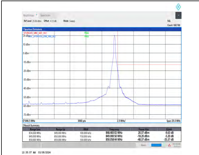
1-N5-15-15-H-2-DFT-PI2BPSK-Edge_1RB_Right-1@78-Ant1-1--PASS-see graph
