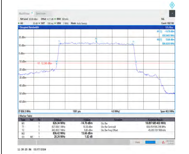
1-N5-15-20-M-8-CP-64QAM-Outer_Full-106@0-Ant1-18.898-20.240-≤20-PASS
