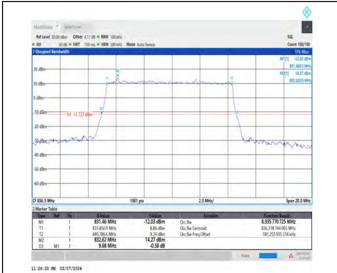
1-N5-15-10-M-4-DFT-64QAM-Outer_Full-50@0-Ant1 -8.936-9.680-≤10-PASS
