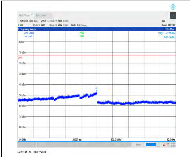
1-N5-15-20-L-1-DFT-PI2BPSK-Inner_1RB_Left-1@1 -3000-12000-Ant1-7482.45--47.00--13-PASS
