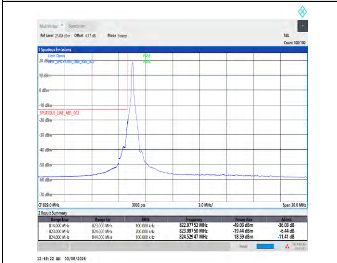
1-N5-15-20-L-4-CP-QPSK-Edge_1RB_Left-1@0-Ant1-1--PASS-see graph
