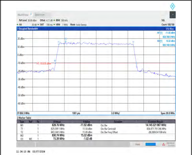
1-N5-15-15-M-6-CP-QPSK-Outer_Full-79@0-Ant1-1 4.145-15.390-≤15-PASS
