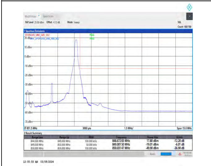
1-N5-15-5-H-5-CP-QPSK-Edge_1RB_Right-1@24-Ant1-1--PASS-see graph
