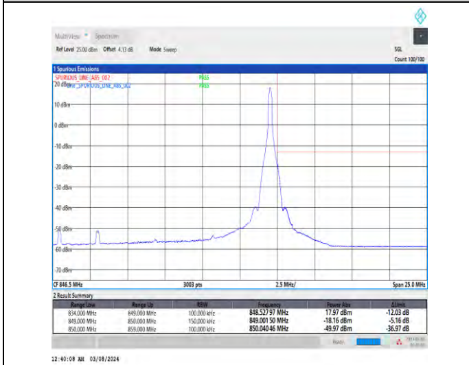
1-N5-15-15-H-5-CP-QPSK-Edge_1RB_Right-1@78-Ant1-1--PASS-see graph
