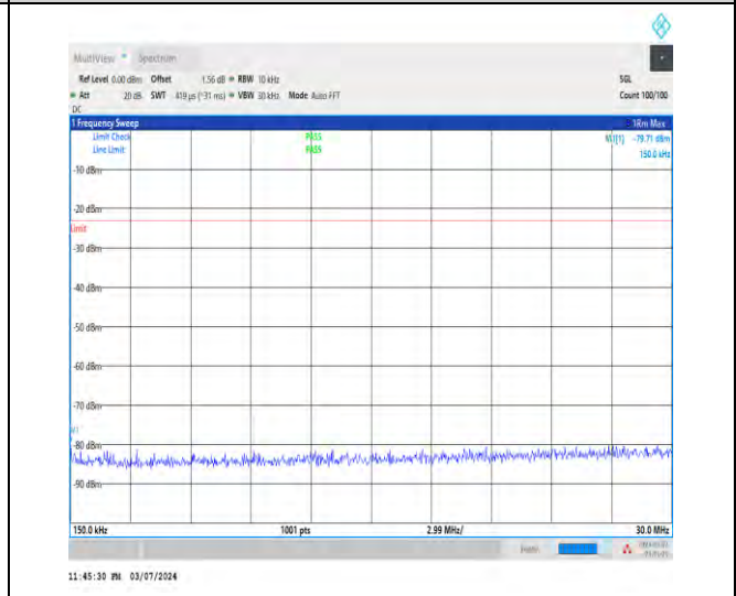
1-N5-15-20-H-1-DFT-PI2BPSK-Inner_1RB_Left-1@1 -0.15-30-Ant1-0.15--79.71--23-PASS
