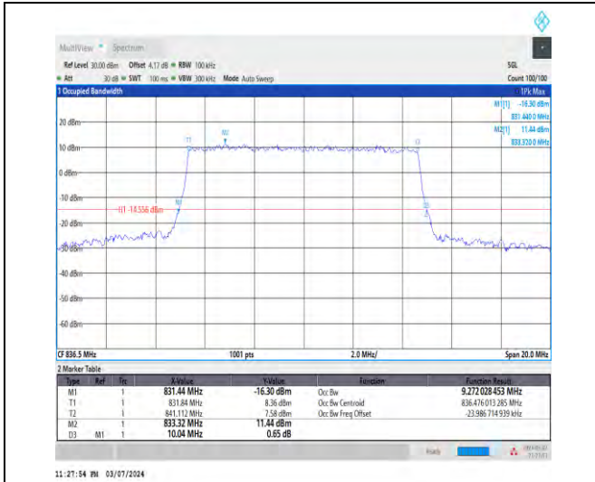
1-N5-15-10-M-8-CP-64QAM-Outer_Full-52@0-Ant1-9.272-10.040-≤10-PASS
