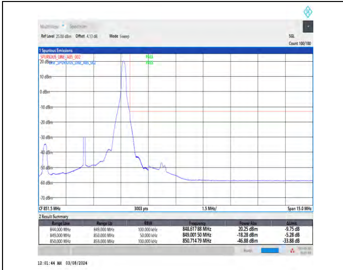
1-N5-15-5-H-2-DFT-PI2BPSK-Edge_1RB_Right-1@24-Ant1-1--PASS-see graph
