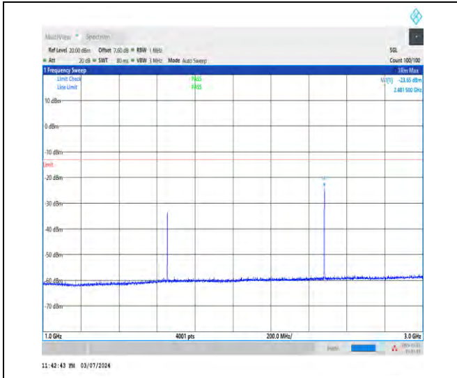
1-N5-15-20-M-1-DFT-PI2BPSK-Inner_1RB_Left-1@ 1-1000-3000-Ant1-2481.50--23.65--13-PASS
