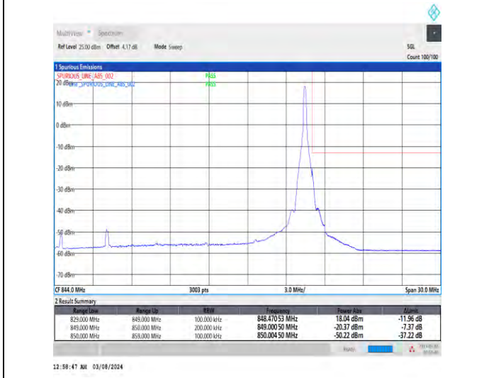
1-N5-15-20-H-5-CP-QPSK-Edge_1RB_Right-1@105-Ant1-1--PASS-see graph
