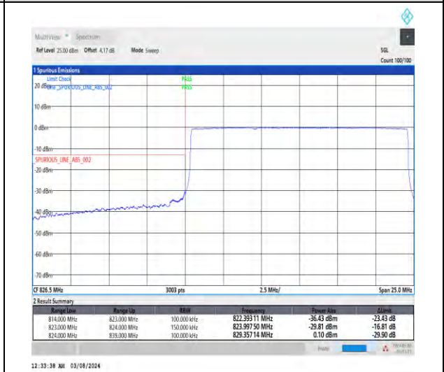
1-N5-15-15-L-6-CP-QPSK-Outer_Full-79@0-Ant1-1--PASS-see graph
