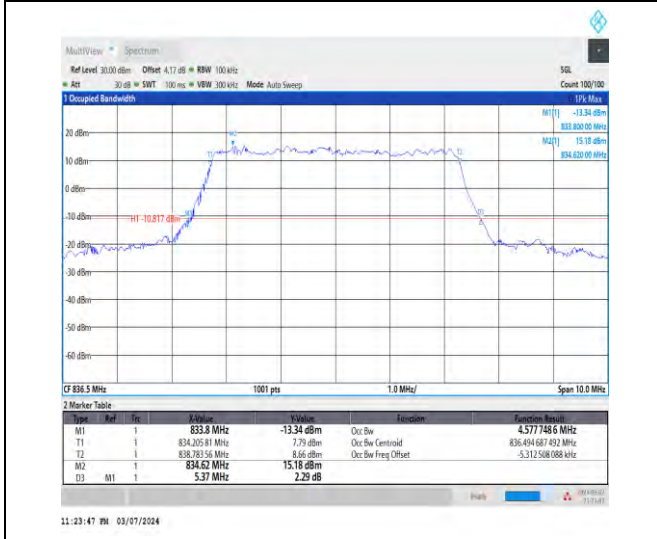
1-N5-15-5-M-7-CP-16QAM-Outer_Full-25@0-Ant1-4. 578-5.370-≤5-PASS
