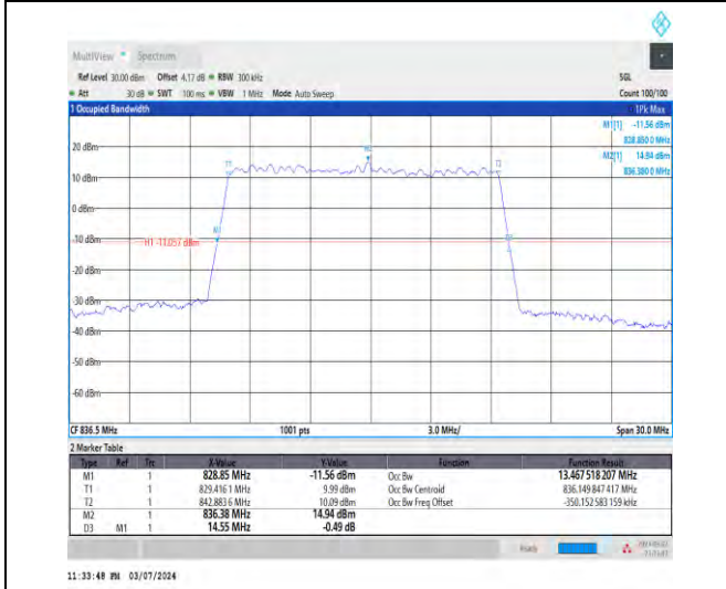
1-N5-15-15-M-5-DFT-256QAM-Outer_Full-75@0-Ant 1-13.468-14.550-≤15-PASS
