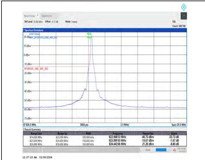
1-N5-15-15-L-1-DFT-PI2BPSK-Edge_1RB_Left-1@0-Ant1-1--PASS-see graph
