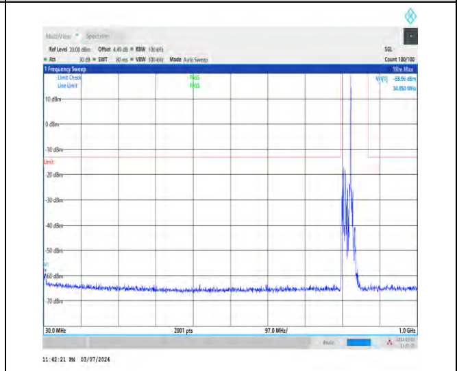
1-N5-15-20-M-1-DFT-PI2BPSK-Inner_1RB_Left-1@ 1-30-1000-Ant1-34.85--58.96--13-PASS
