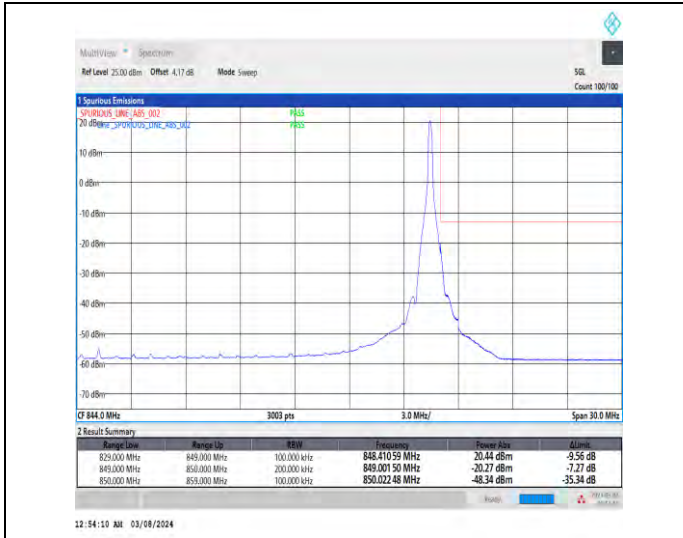
1-N5-15-20-H-2-DFT-PI2BPSK-Edge_1RB_Right-1@105-Ant1-1--PASS-see graph
