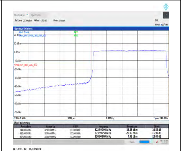
1-N5-15-10-L-6-CP-QPSK-Outer_Full-52@0-Ant1-1--PASS-see graph
