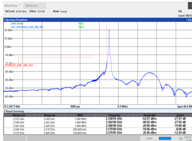
38-38-15MHz-15MHz-QPSK-QPSK-37825-37975-75RB#0-75RB#0
