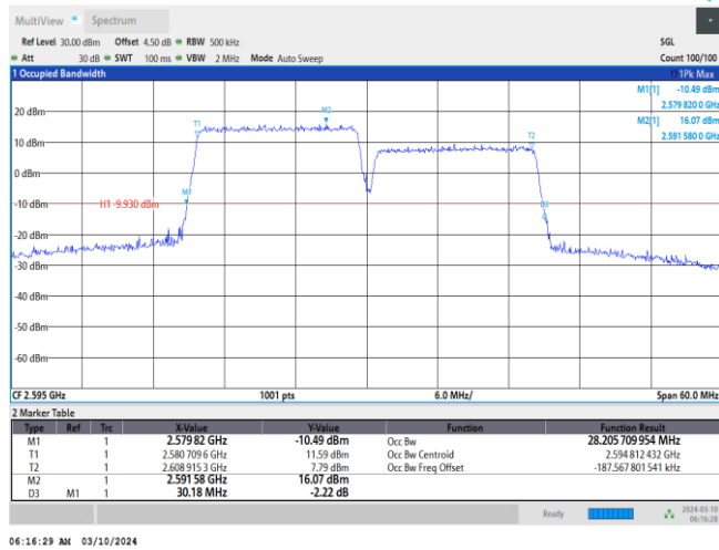
38-38-15MHz-15MHz-16QAM-16QAM-37925-38075-75RB#0-75RB#0
