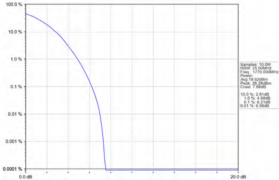
Band66_20MHz_64QAM_HCH_1770MHz_RB_100_0_NTNV
