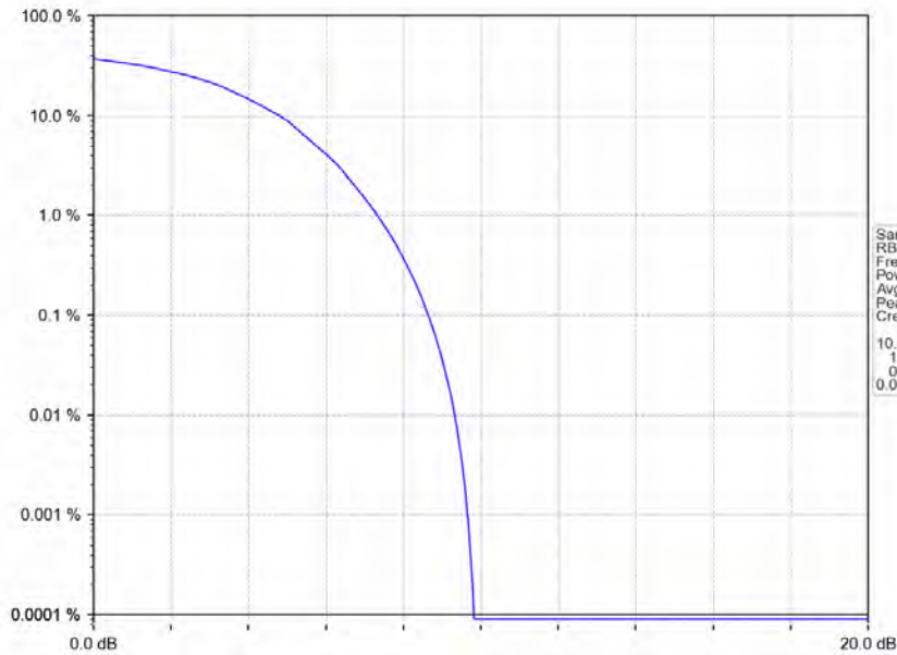
Band38_5MHz_64QAM_HCH_2617.5MHz_RB_25_0_NTNV
