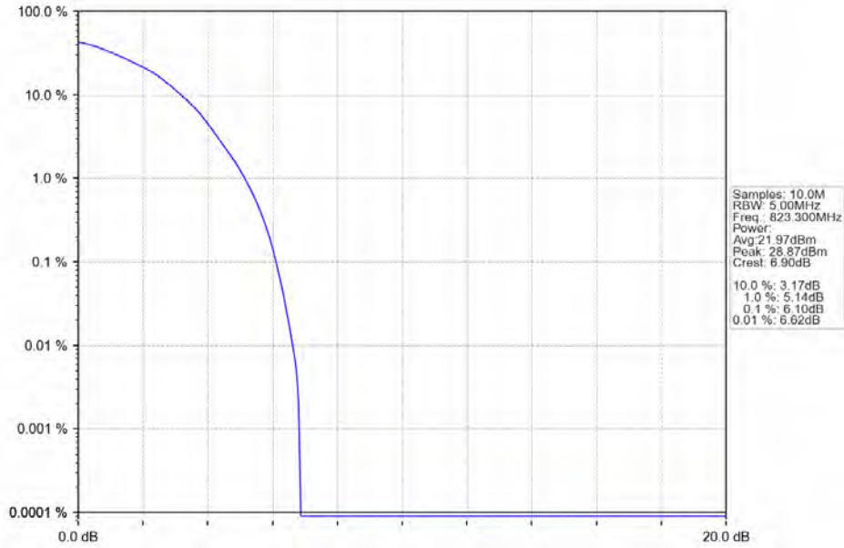
Band26a_1.4MHz_64QAM_HCH_823.3MHz_RB_6_0_NTNV
