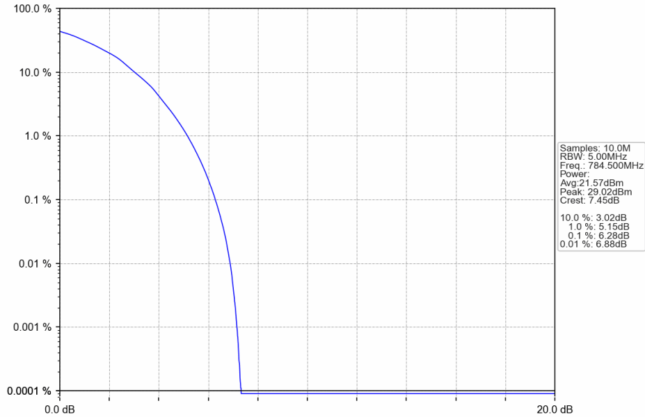
Band13_5MHz_64QAM_HCH_784.5MHz_RB_25_0_NTNV
