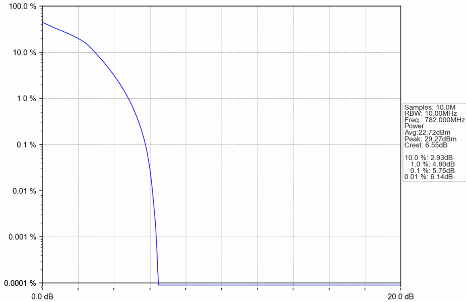
Band13_10MHz_16QAM_MCH_782MHz_RB_50_0_NTNV
