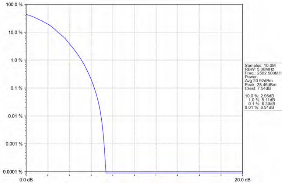
Band7_5MHz_64QAM_LCH_2502.5MHz_RB_25_0_NTNV
