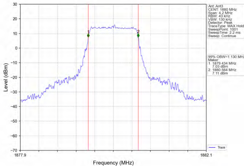
Band2_1.4MHz_64QAM_MCH_1880MHz_RB_6_0_NTNV
