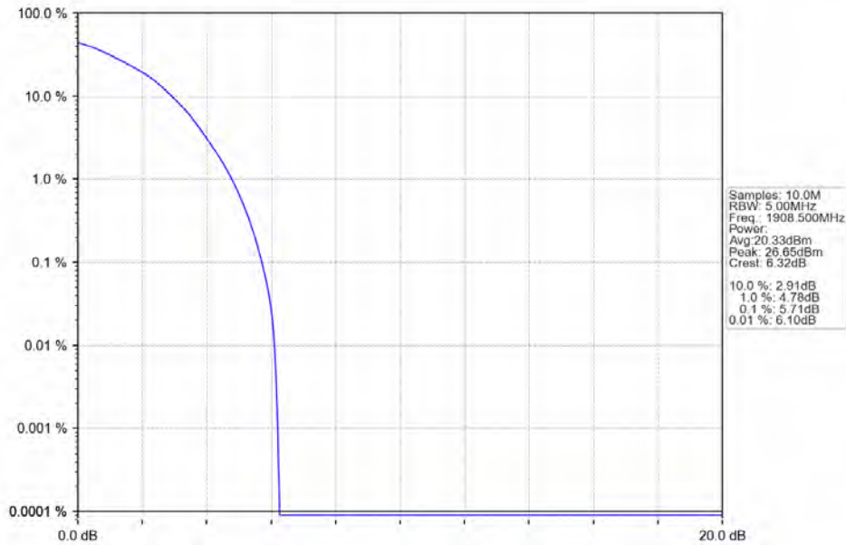
Band2_3MHz_64QAM_HCH_1908.5MHz_RB_15_0_NTNV
