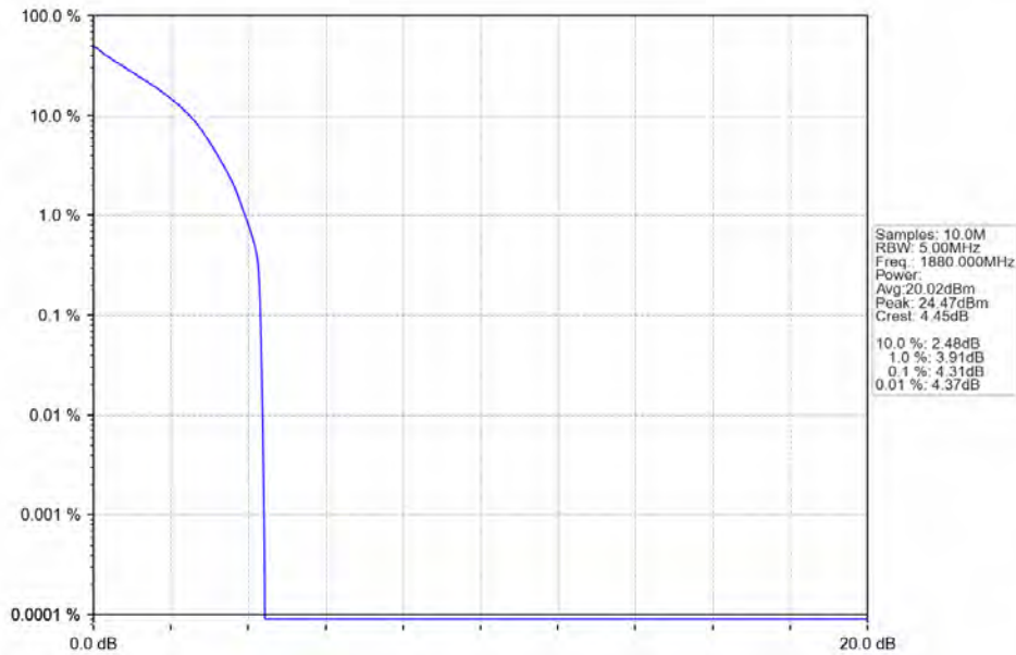
Band2_1.4MHz_QPSK_MCH_1880MHz_RB_6_0_NTNV
