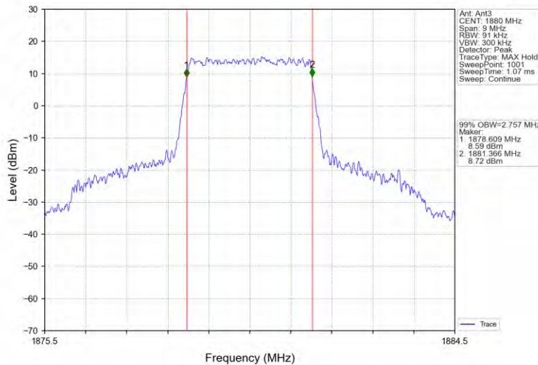
Band2_3MHz_16QAM_MCH_1880MHz_RB_15_0_NTNV
