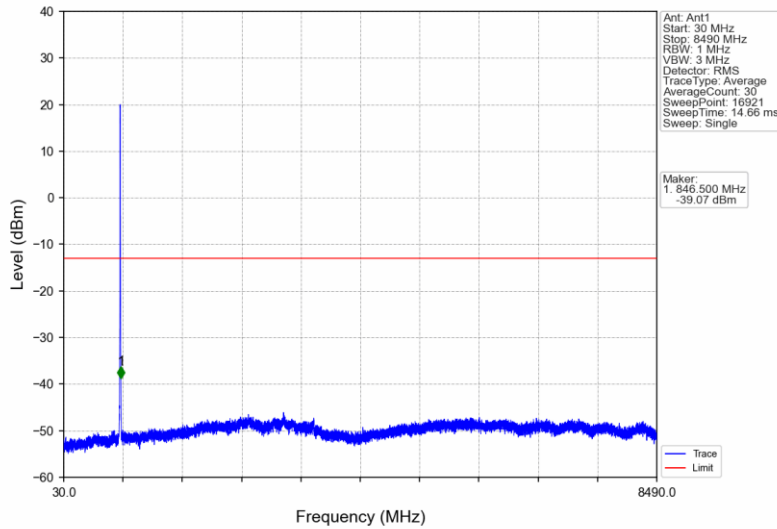
Band5_RMC_HCH_846.6MHz_12.2kbps RMC_NTNV
