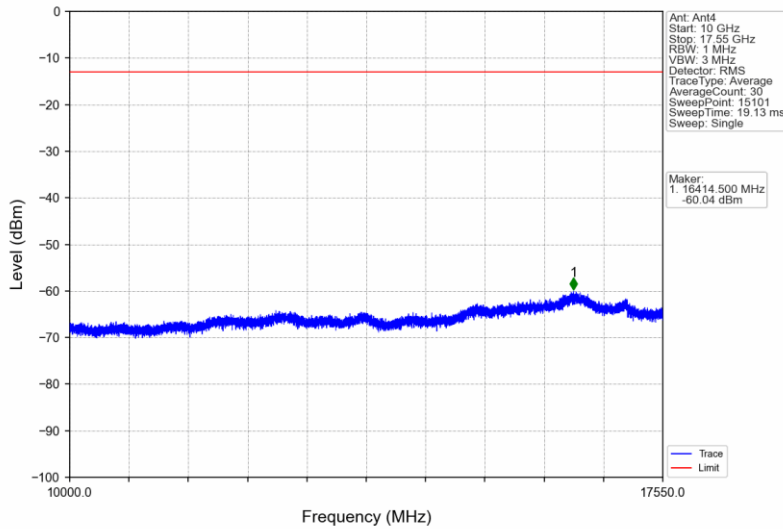
BandIV_RMC_HCH_1752.6MHz_12.2kbps RMC_NTNV
