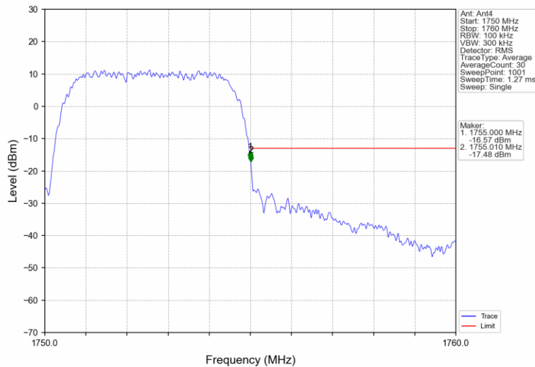
BandIV_RMC_HCH_1752.6MHz_12.2kbps RMC_NTNV
