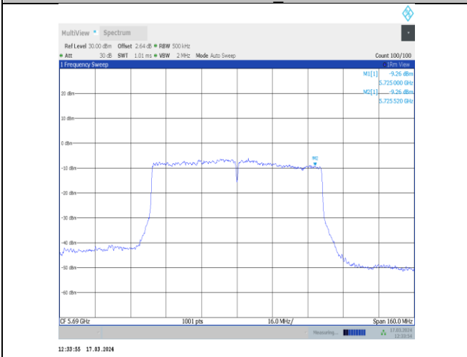
11ac80MIMO-Ant11-5690_UNII-3-PASS
