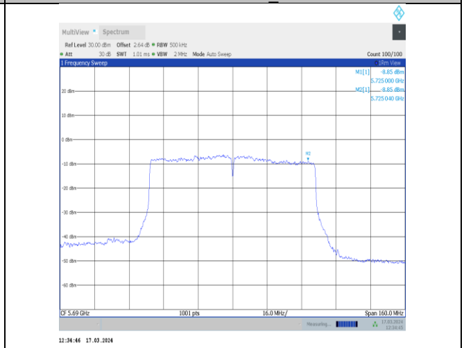
11ac80MIMO-Ant12-5690_UNII-3-PASS
