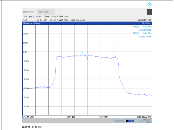
11ac80MIMO-Ant12-5690_UNII-2C-PASS
