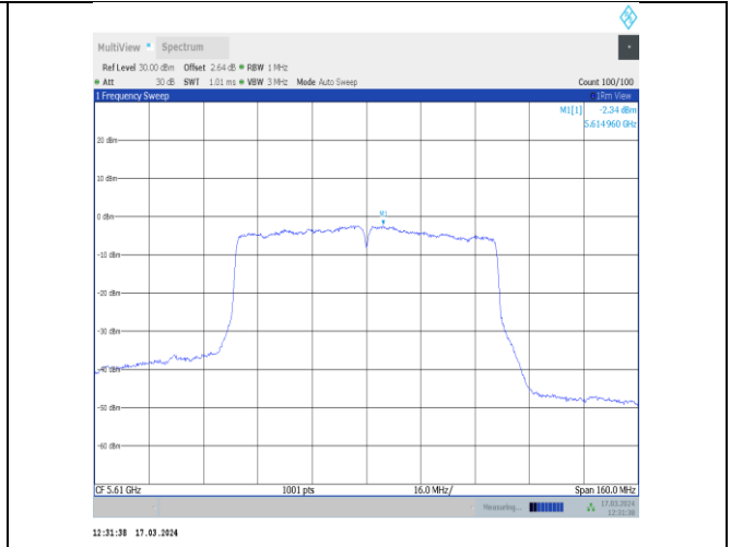
11ac80MIMO-Ant12-5610-PASS
