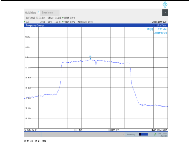
11ac80MIMO-Ant11-5610-PASS
