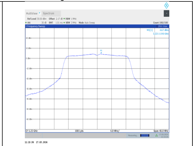
11ac20MIMO-Ant12-5220-PASS
