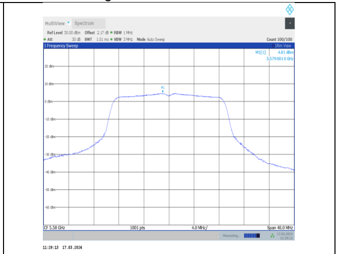
11ac20MIMO-Ant12-5580-PASS
