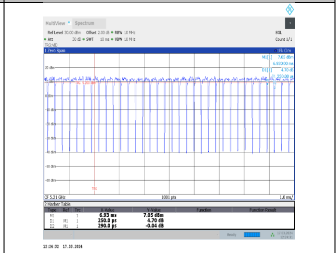
NTVN-11ac80MIMO-Ant12-5210
