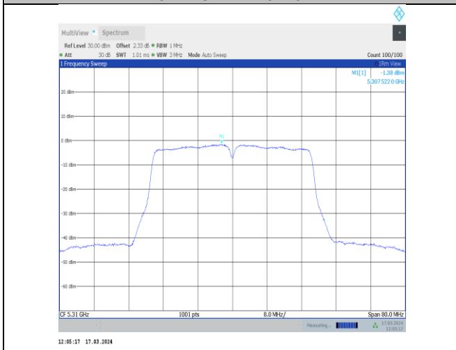
11ac40MIMO-Ant11-5310-PASS
