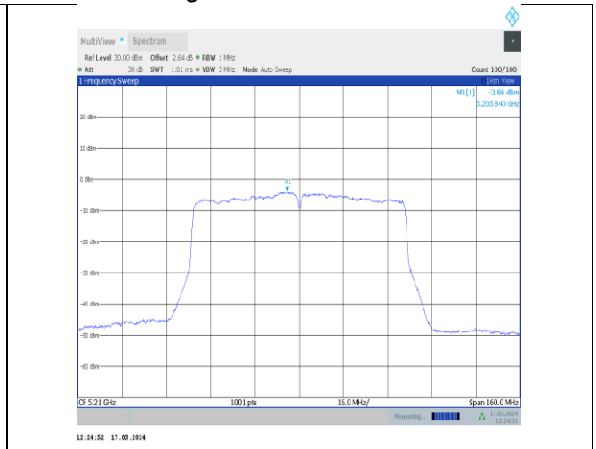
11ac80MIMO-Ant12-5210-PASS
