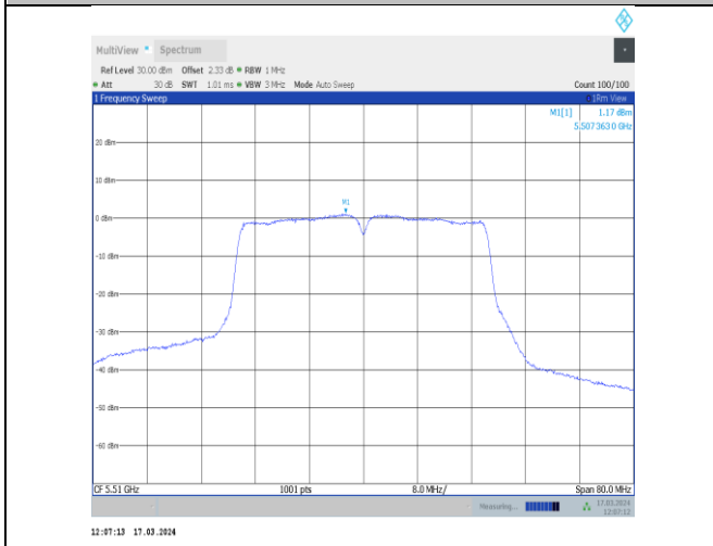
11ac40MIMO-Ant11-5510-PASS
