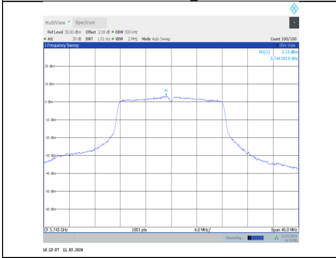
11a-CDD-Ant11-5745-PASS
