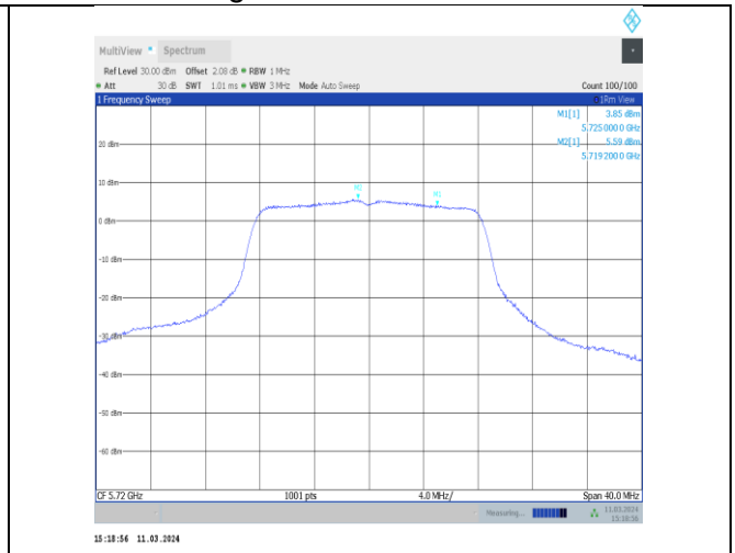
11a-CDD-Ant12-5720 UNII-2C-PASS
