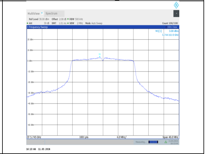
11a-CDD-Ant12-5745-PASS
