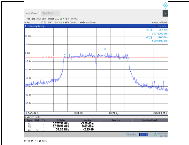
11ac40MIMO-Ant11-5755-PASS
