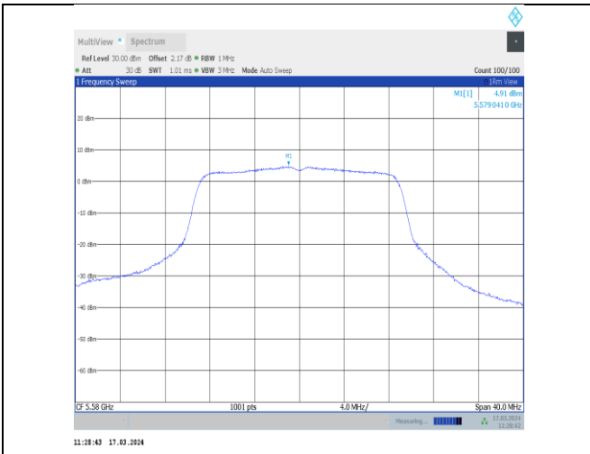
11ac20MIMO-Ant11-5580-PASS
