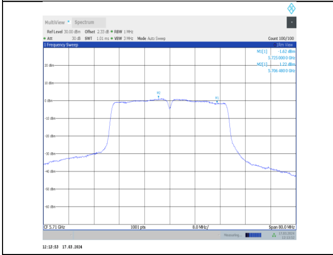
11ac40MIMO-Ant11-5710 UNII-2C-PASS
