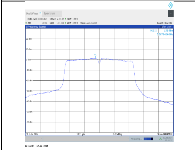
11ac40MIMO-Ant11-5670-PASS
