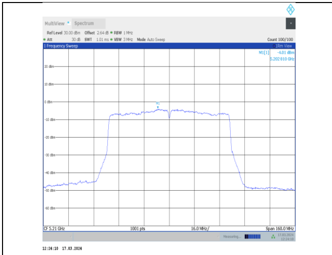
11ac80MIMO-Ant11-5210-PASS
