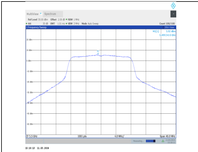
11a-CDD-Ant11-5500-PASS
