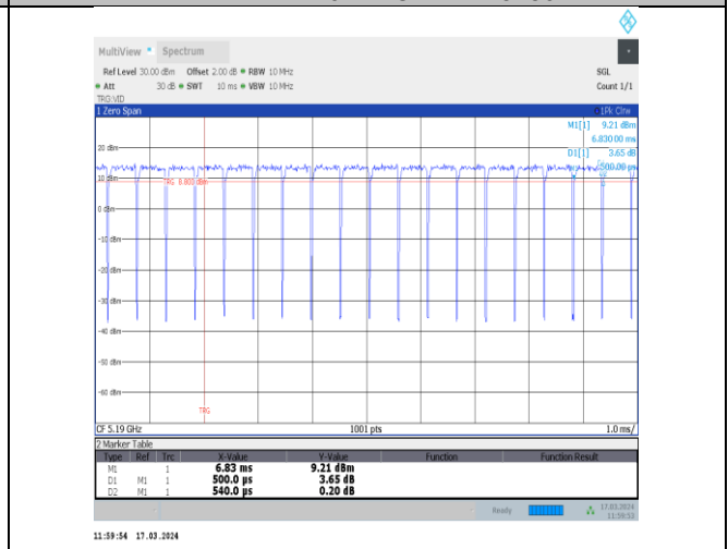
NTVN-11ac40MIMO-Ant12-5190
