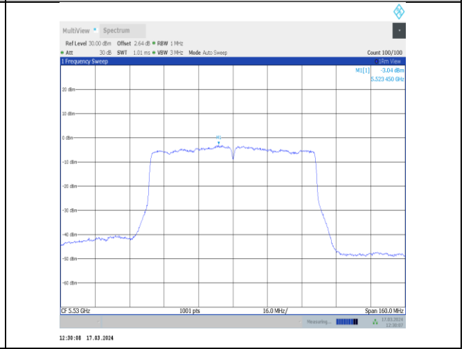
11ac80MIMO-Ant12-5530-PASS
