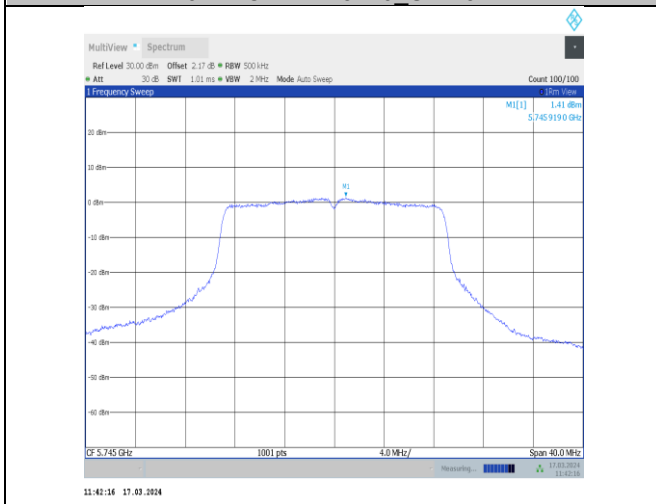
11ac20MIMO-Ant11-5745-PASS
