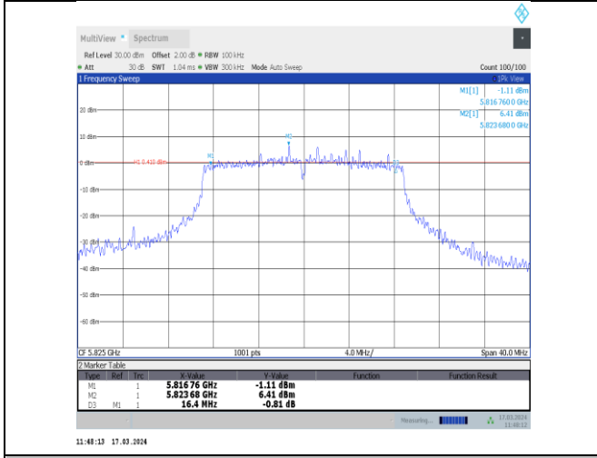
11ac20MIMO-Ant11-5825-PASS
