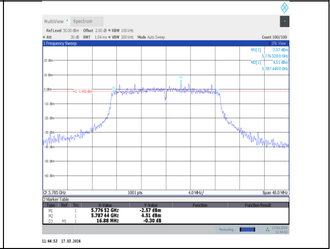
11ac20MIMO-Ant12-5785-PASS
