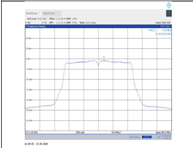
11ac40MIMO-Ant11-5190-PASS
