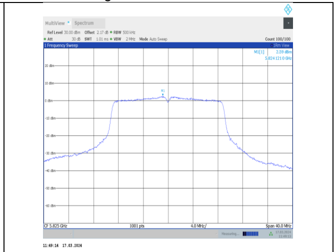
11ac20MIMO-Ant12-5825-PASS
