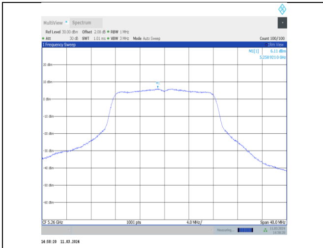
11a-CDD-Ant11-5260-PASS
