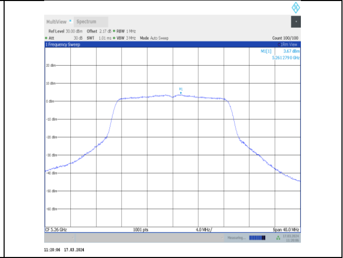
11ac20MIMO-Ant12-5260-PASS
