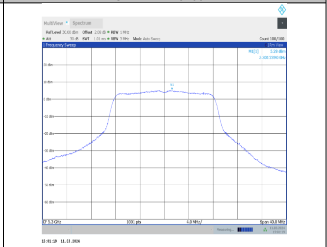
11a-CDD-Ant12-5300-PASS
