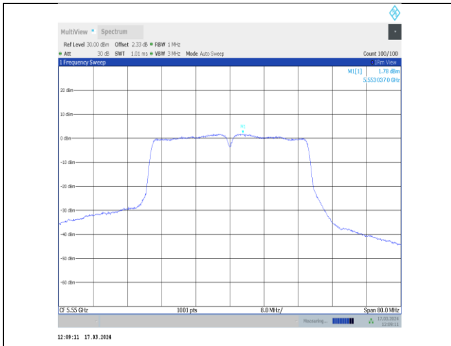
11ac40MIMO-Ant11-5550-PASS
