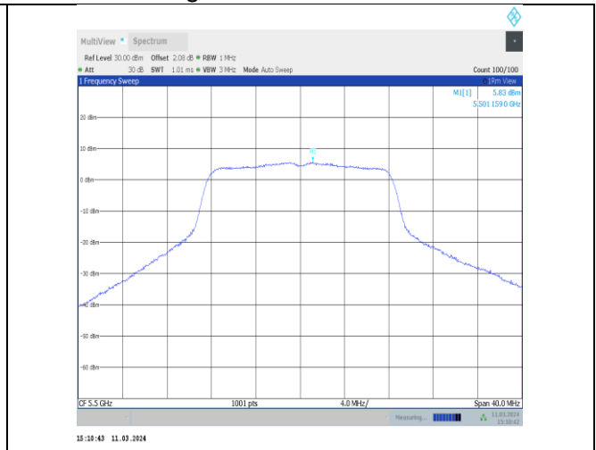
11a-CDD-Ant12-5500-PASS
