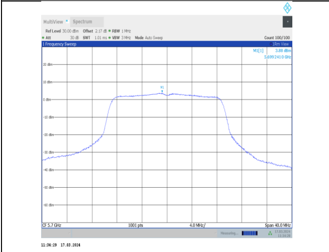
11ac20MIMO-Ant11-5700-PASS
