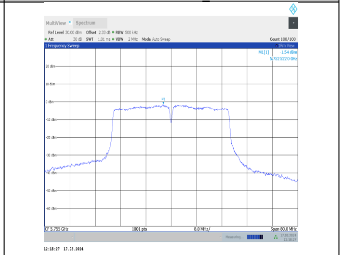
11ac40MIMO-Ant12-5755-PASS
