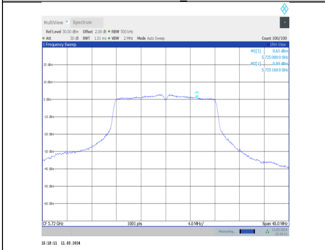
11a-CDD-Ant11-5720 UNII-3-PASS
