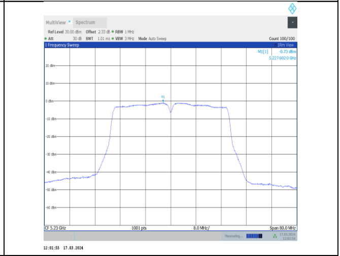
11ac40MIMO-Ant12-5230-PASS
