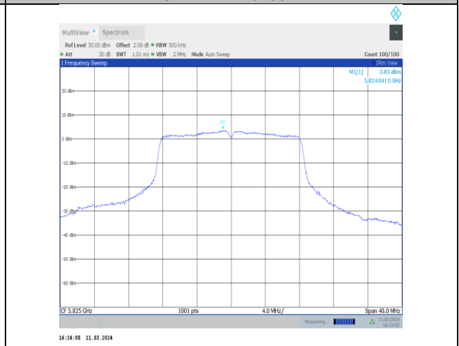
11a-CDD-Ant12-5825-PASS
