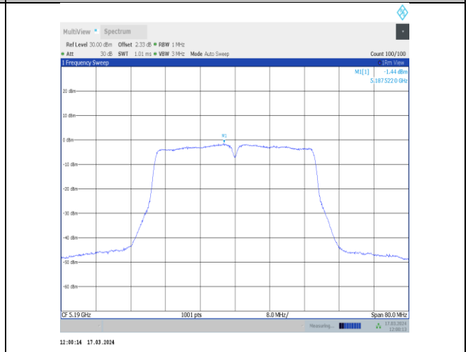
11ac40MIMO-Ant12-5190-PASS
