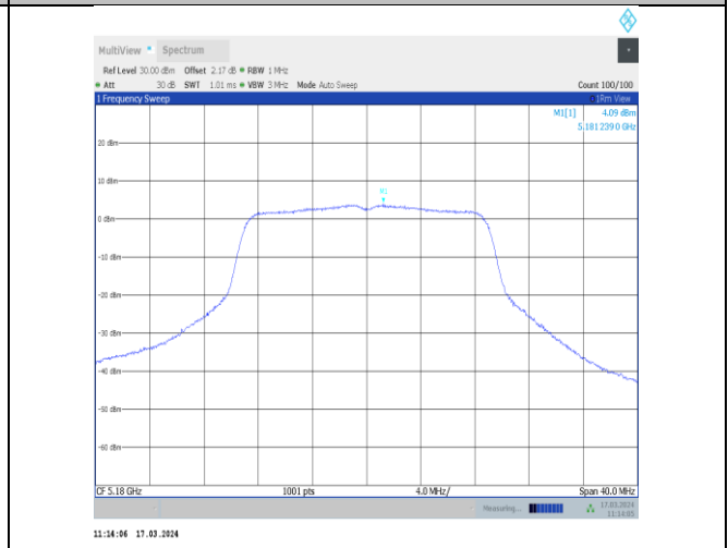
11ac20MIMO-Ant12-5180-PASS
