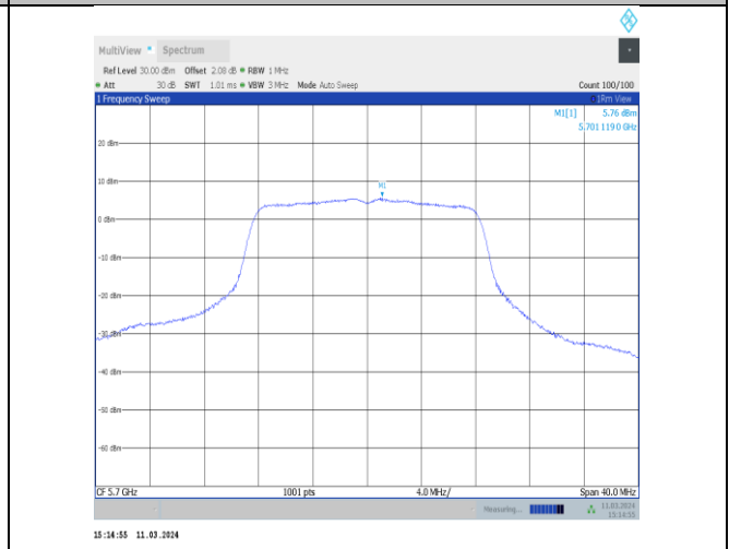
11a-CDD-Ant12-5700-PASS
