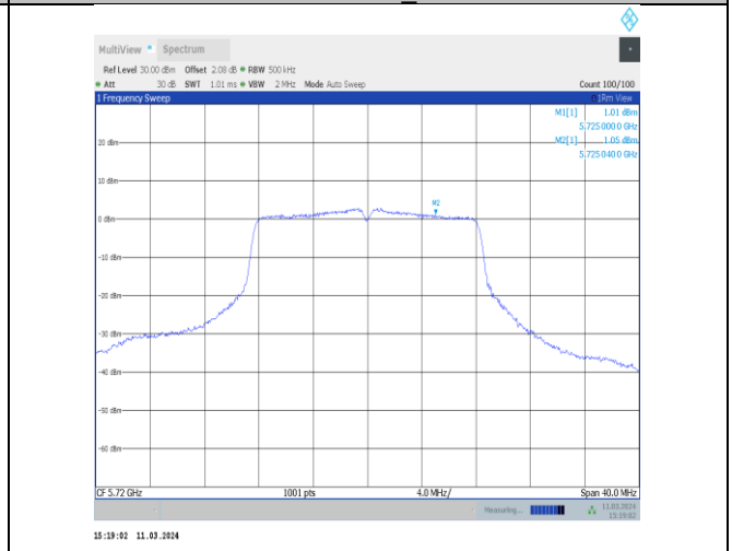
11a-CDD-Ant12-5720 UNII-3-PASS
