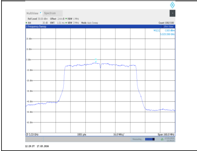
11ac80MIMO-Ant11-5530-PASS
