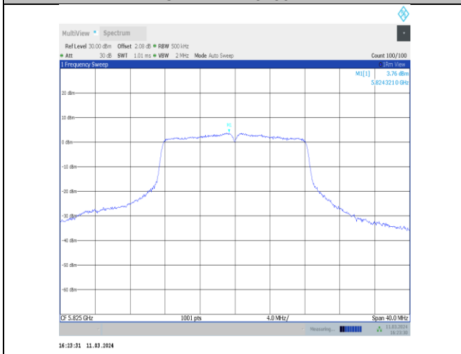
11a-CDD-Ant11-5825-PASS
