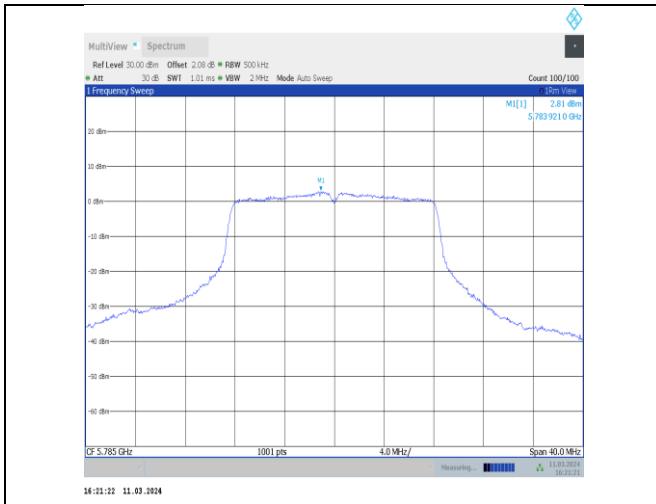
11a-CDD-Ant11-5785-PASS
