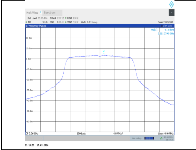
11ac20MIMO-Ant11-5260-PASS
