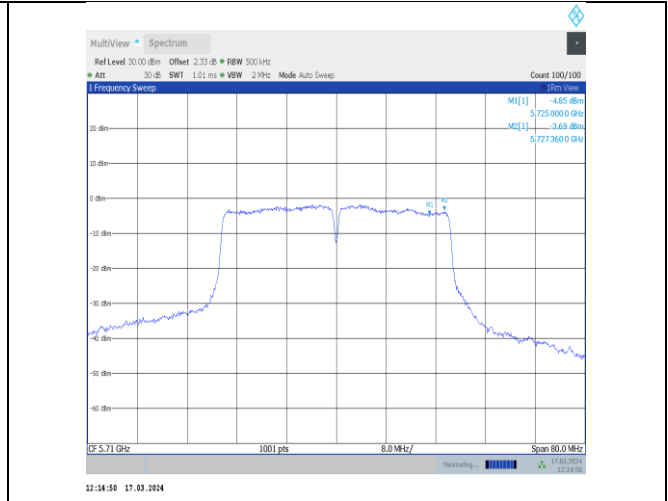
11ac40MIMO-Ant12-5710_UNII-3-PASS
