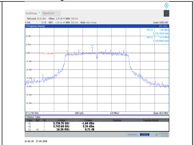
11ac20MIMO-Ant12-5745-PASS
