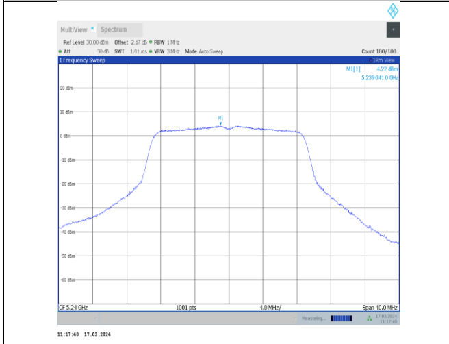
11ac20MIMO-Ant11-5240-PASS
