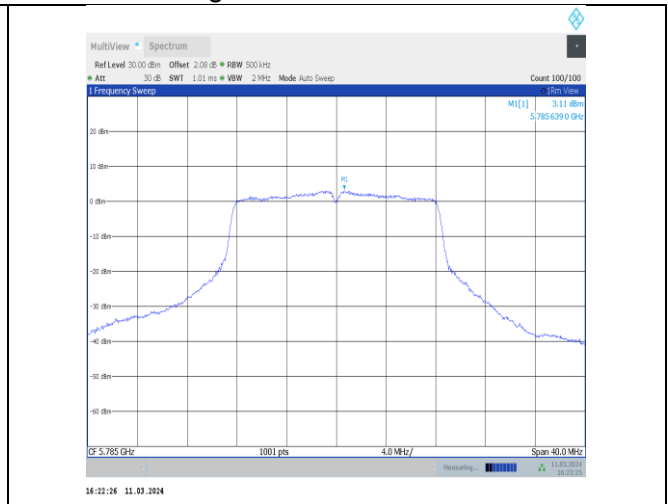
11a-CDD-Ant12-5785-PASS
