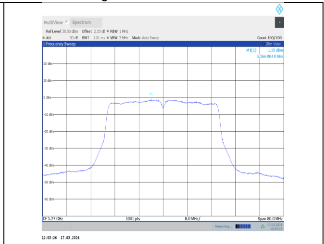
11ac40MIMO-Ant12-5270-PASS
