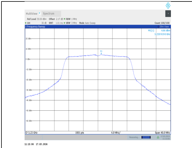
11ac20MIMO-Ant11-5220-PASS
