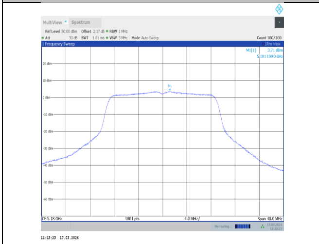
11ac20MIMO-Ant11-5180-PASS
