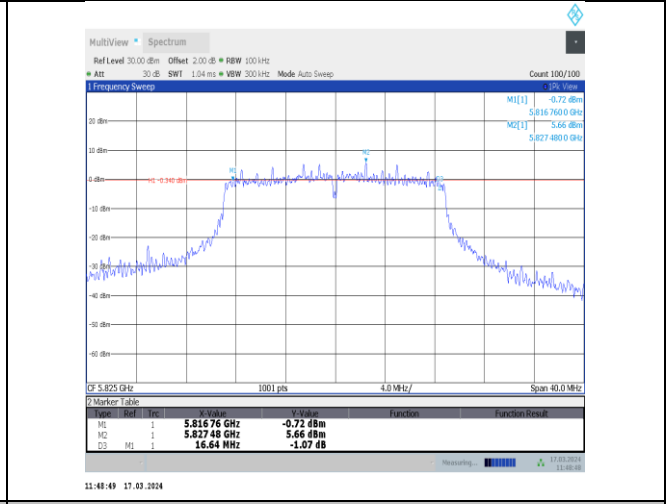
11ac20MIMO-Ant12-5825-PASS
