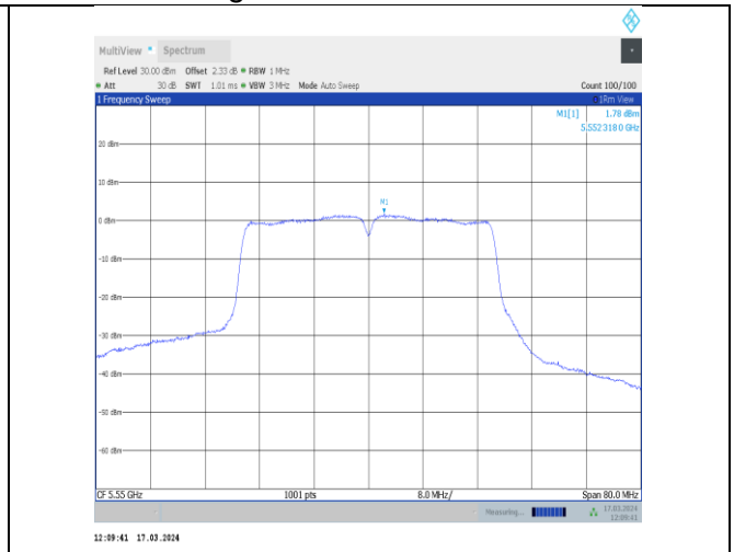
11ac40MIMO-Ant12-5550-PASS
