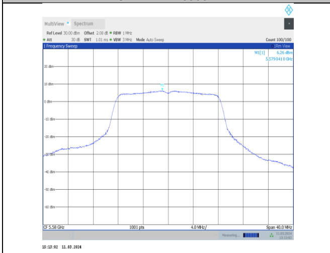
11a-CDD-Ant11-5580-PASS
