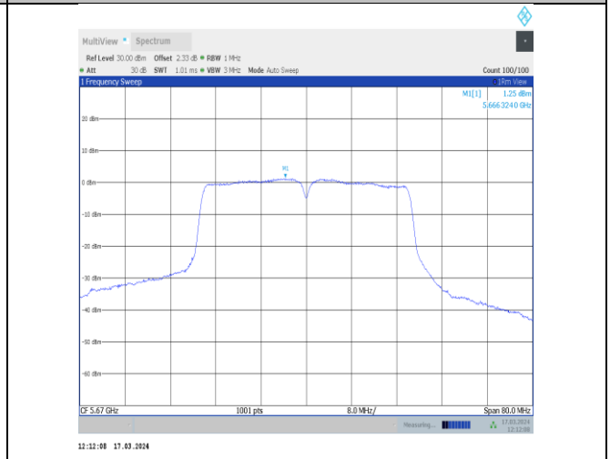
11ac40MIMO-Ant12-5670-PASS
