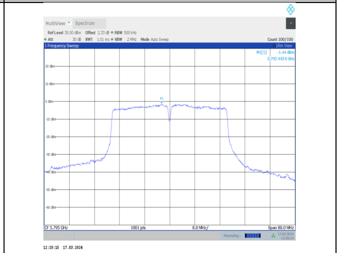
11ac40MIMO-Ant12-5795-PASS
