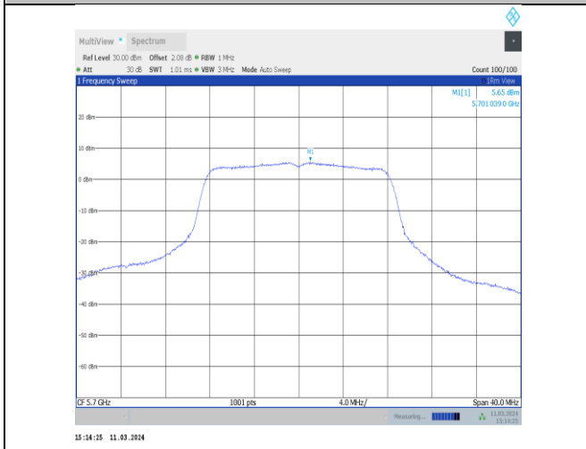
11a-CDD-Ant11-5700-PASS
