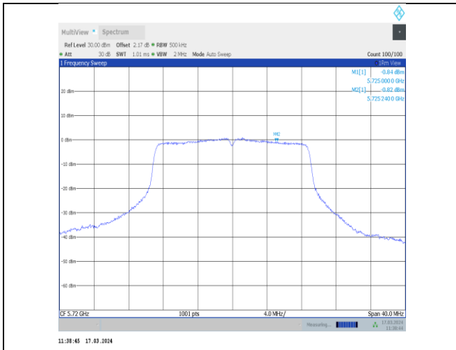
11ac20MIMO-Ant11-5720_UNII-3-PASS
