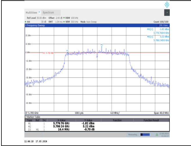
11ac20MIMO-Ant11-5785-PASS
