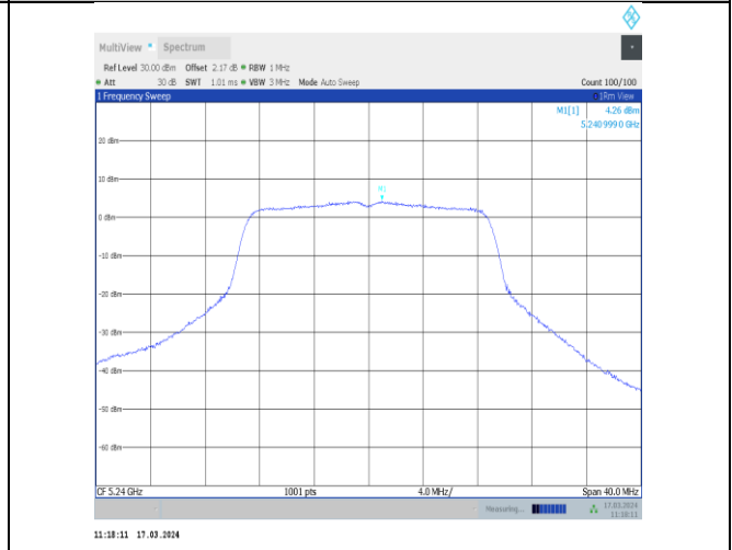
11ac20MIMO-Ant12-5240-PASS
