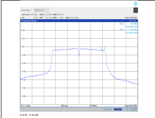
11ac40MIMO-Ant11-5710_UNII-3-PASS
