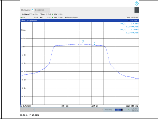
11ac20MIMO-Ant12-5720 UNII-2C-PASS
