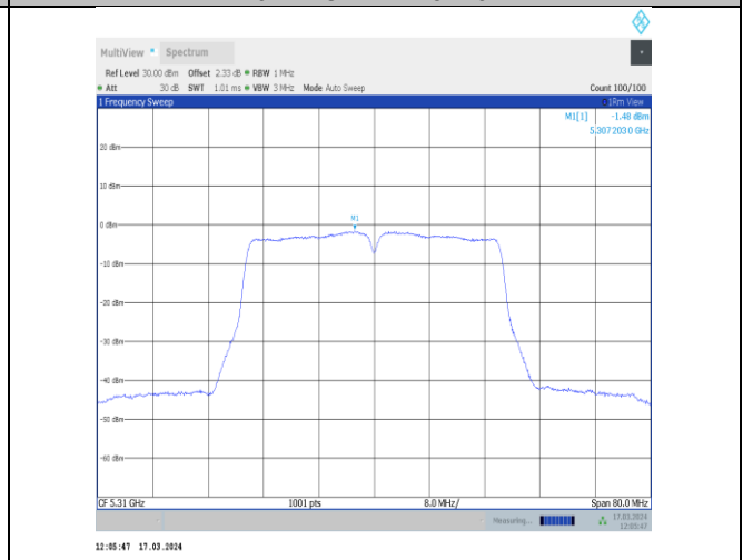
11ac40MIMO-Ant12-5310-PASS
