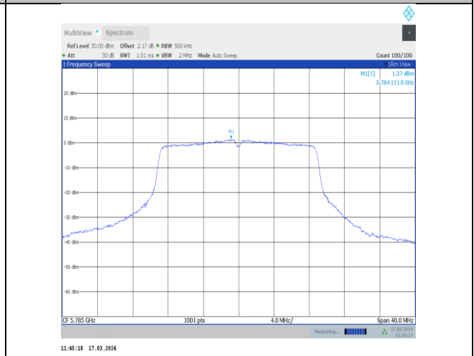
11ac20MIMO-Ant12-5785-PASS
