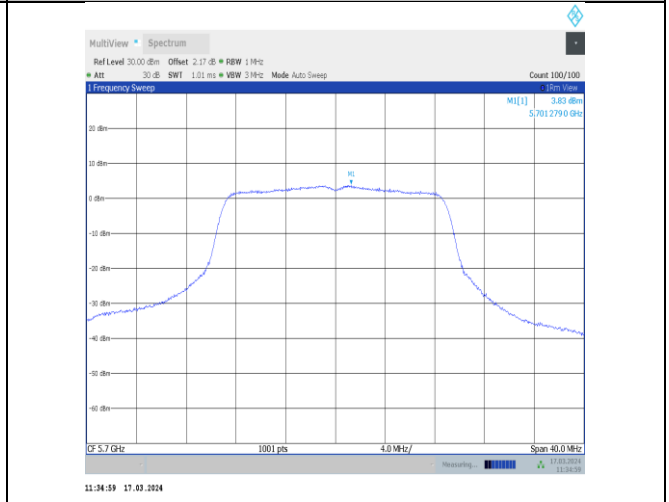
11ac20MIMO-Ant12-5700-PASS
