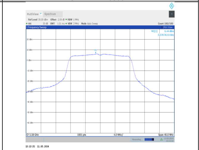
11a-CDD-Ant12-5580-PASS
