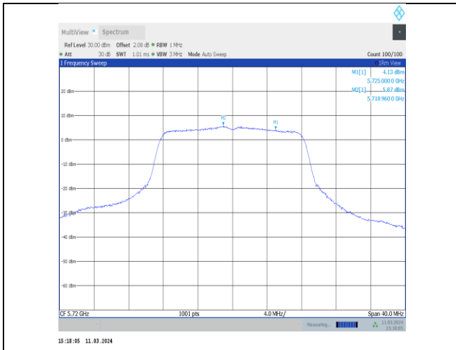
11a-CDD-Ant11-5720 UNII-2C-PASS
