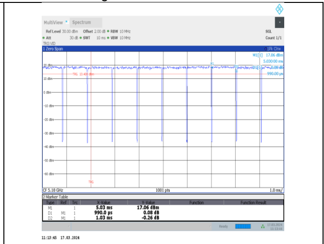
NTVN-11ac20MIMO-Ant12-5180
