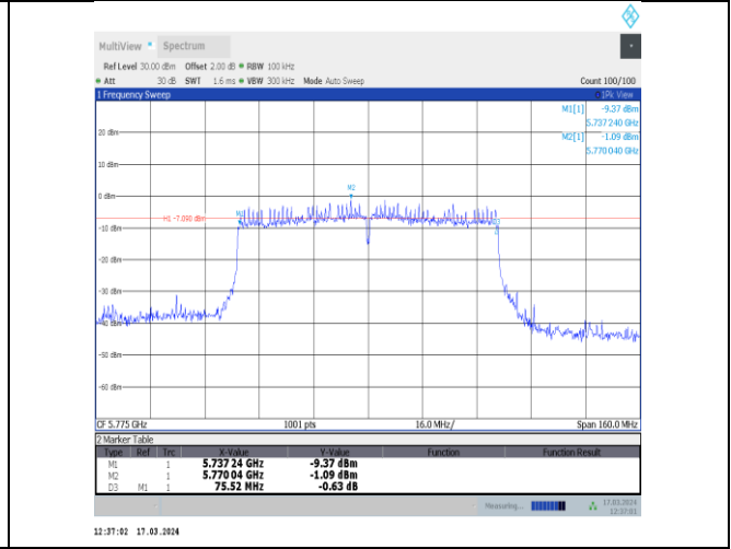
11ac80MIMO-Ant12-5775-PASS
