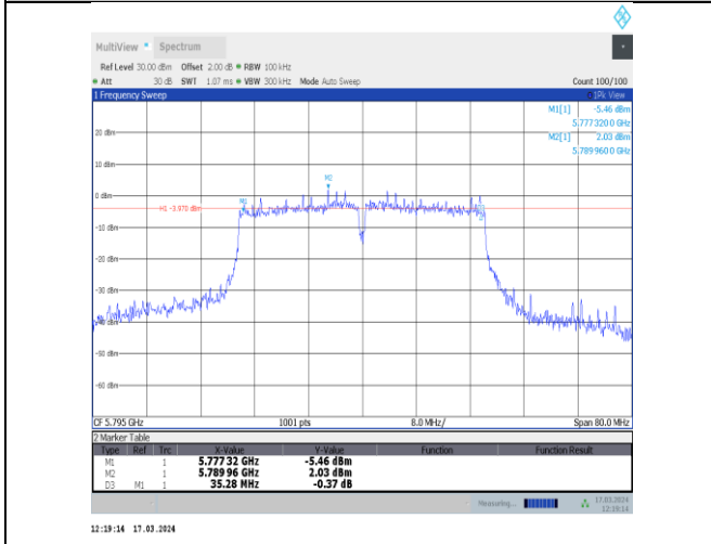
11ac40MIMO-Ant11-5795-PASS
