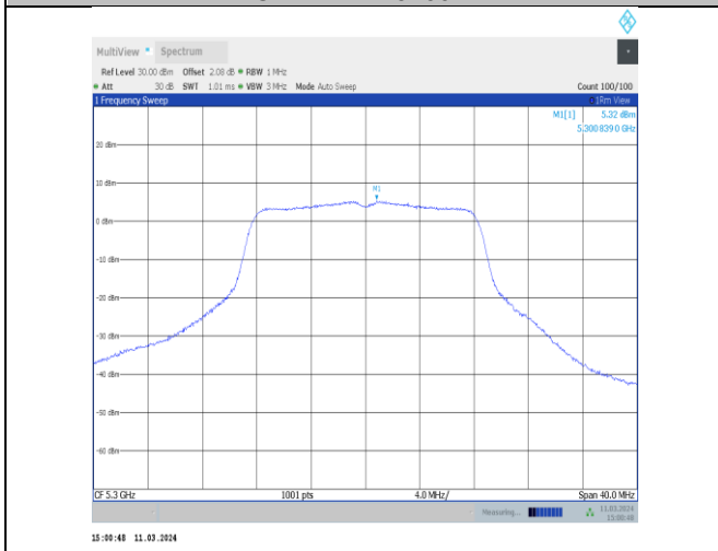
11a-CDD-Ant11-5300-PASS
