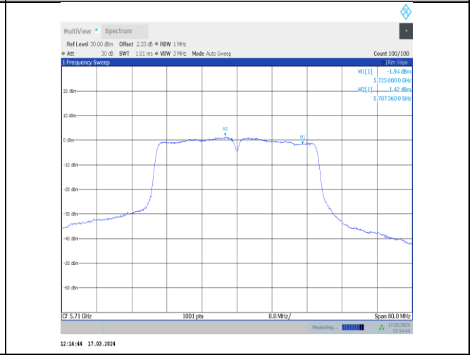
11ac40MIMO-Ant12-5710 UNII-2C-PASS
