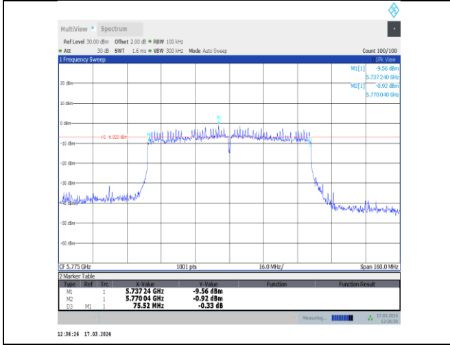
11ac80MIMO-Ant11-5775-PASS
