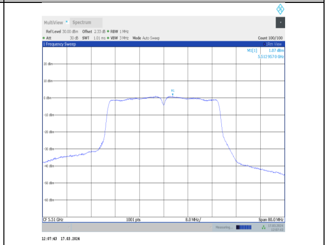
11ac40MIMO-Ant12-5510-PASS
