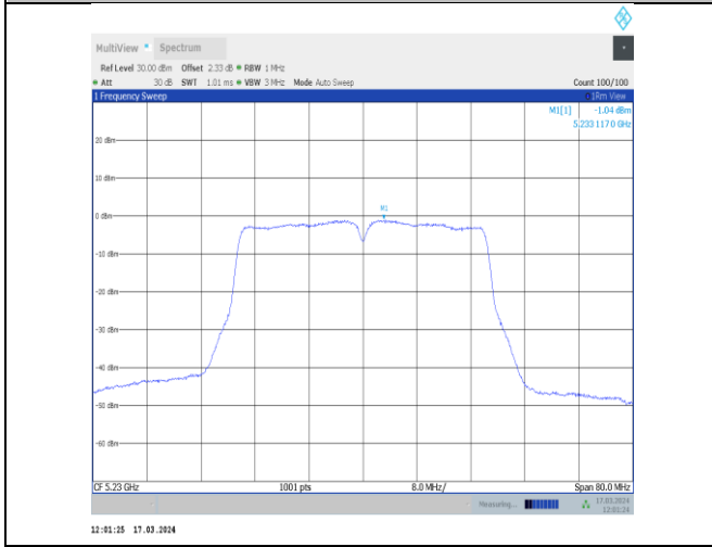
11ac40MIMO-Ant11-5230-PASS
