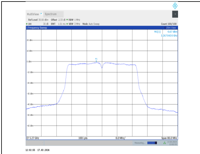
11ac40MIMO-Ant11-5270-PASS
