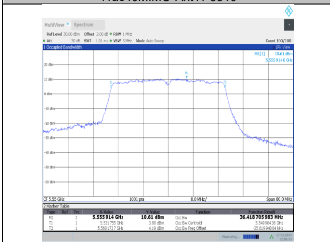
11ac40MIMO-Ant11-5550
