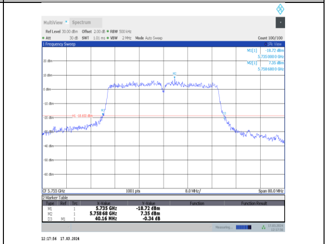
11ac40MIMO-Ant12-5755
