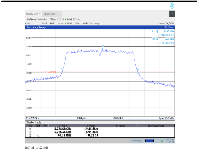
11ac40MIMO-Ant11-5755
