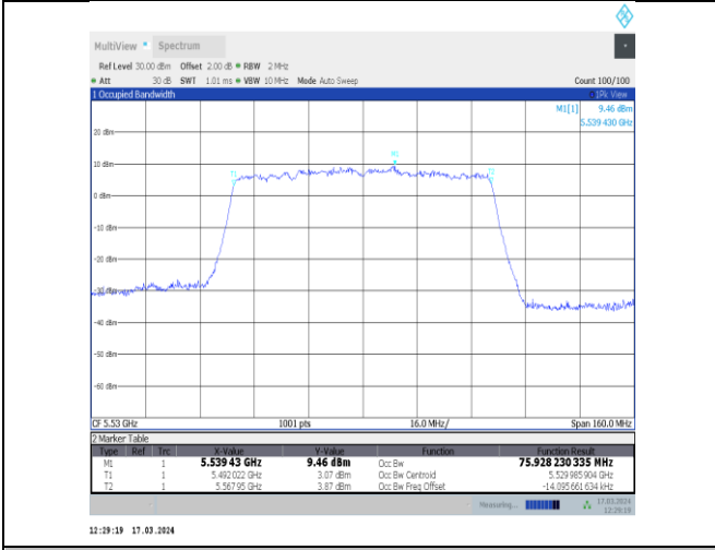
11ac80MIMO-Ant11-5530
