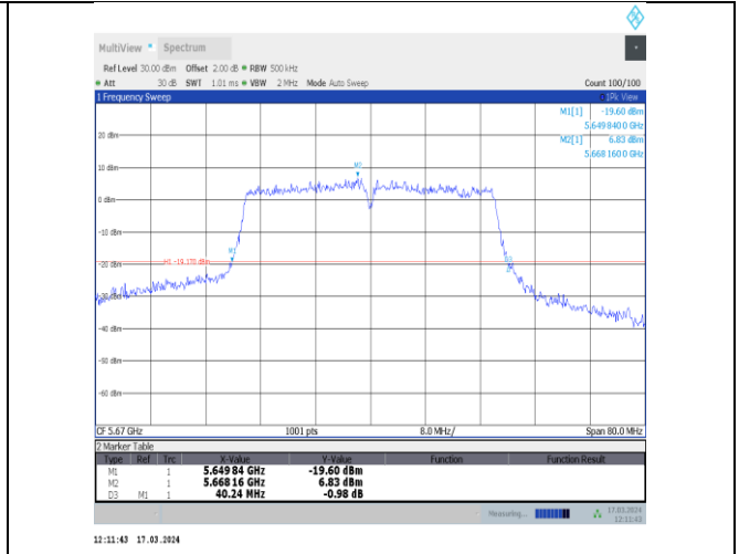
11ac40MIMO-Ant12-5670
