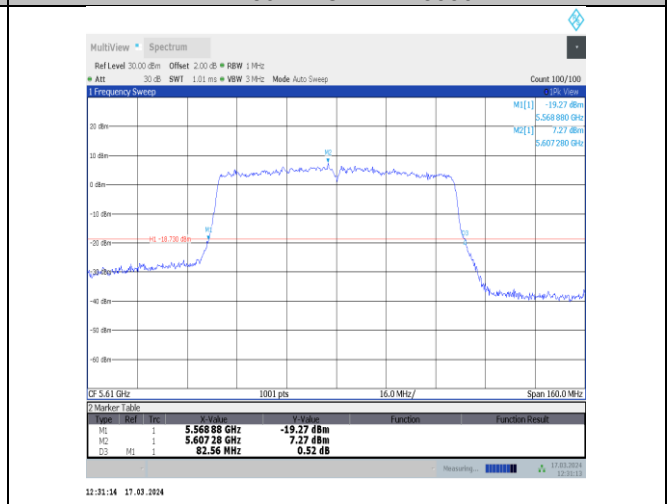
11ac80MIMO-Ant12-5610
