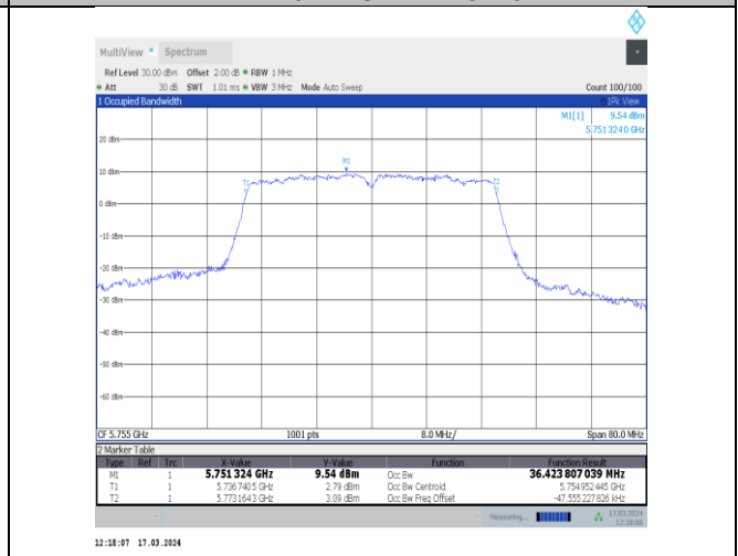
11ac40MIMO-Ant12-5755
