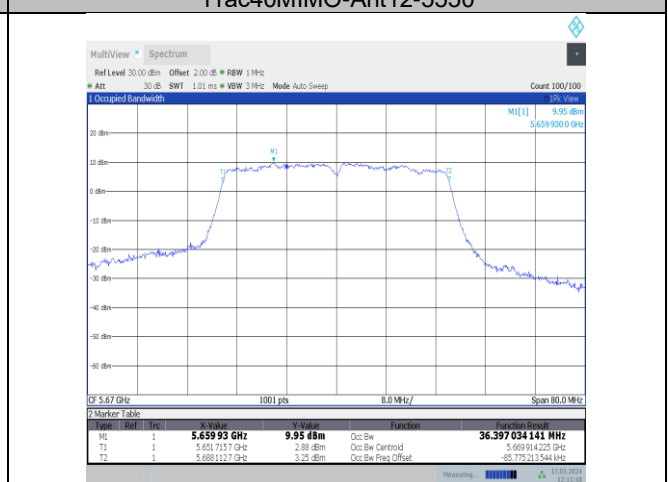
11ac40MIMO-Ant12-5670
