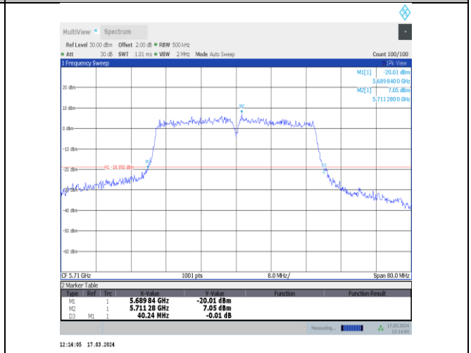
11ac40MIMO-Ant12-5710
