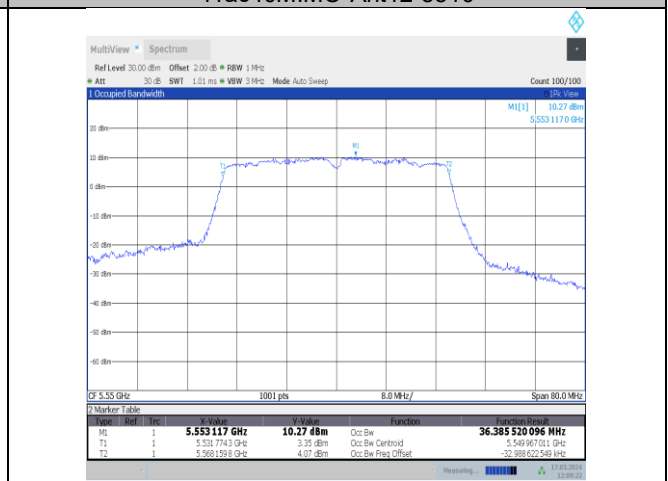
11ac40MIMO-Ant12-5550
