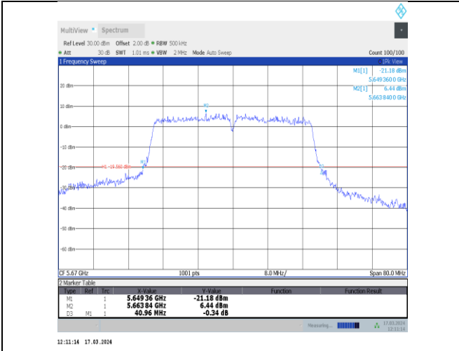
11ac40MIMO-Ant11-5670
