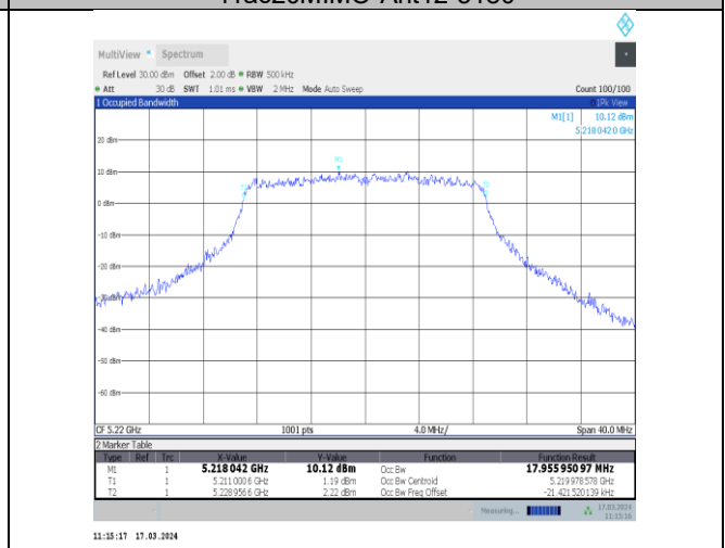
11ac20MIMO-Ant12-5220
