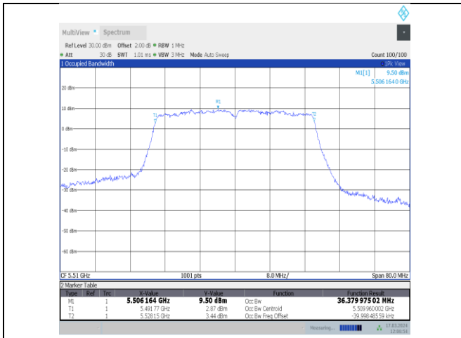
11ac40MIMO-Ant11-5510
