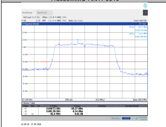
11ac80MIMO-Ant11-5690
