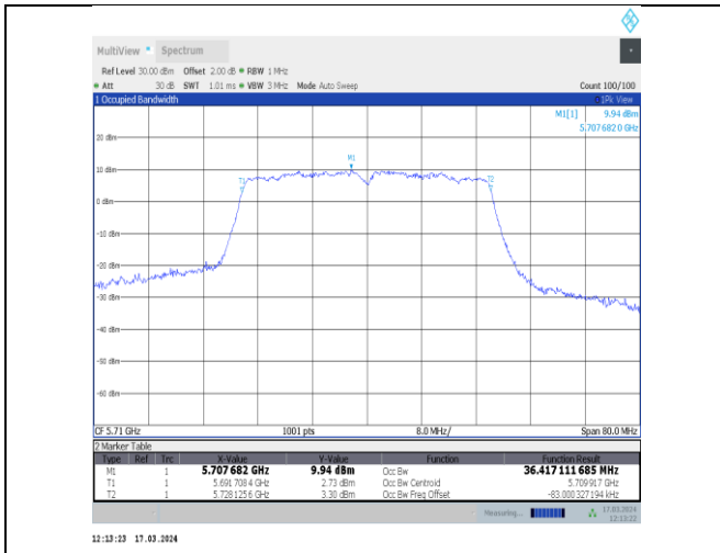
11ac40MIMO-Ant11-5710
