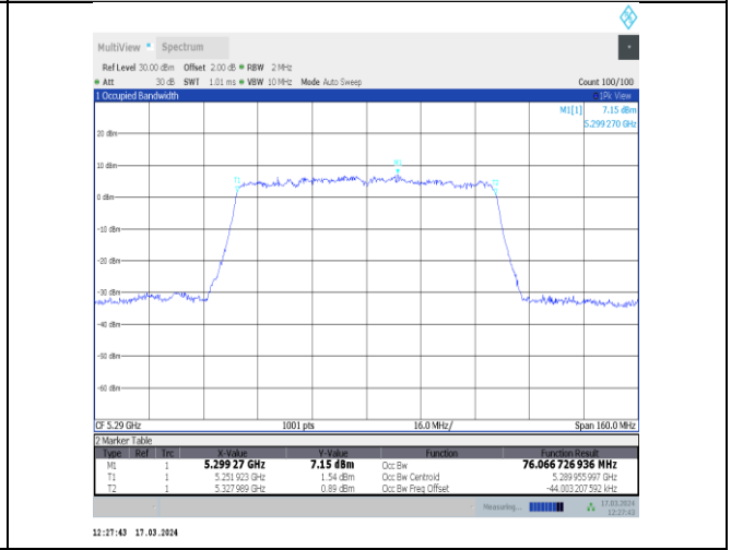
11ac80MIMO-Ant12-5290
