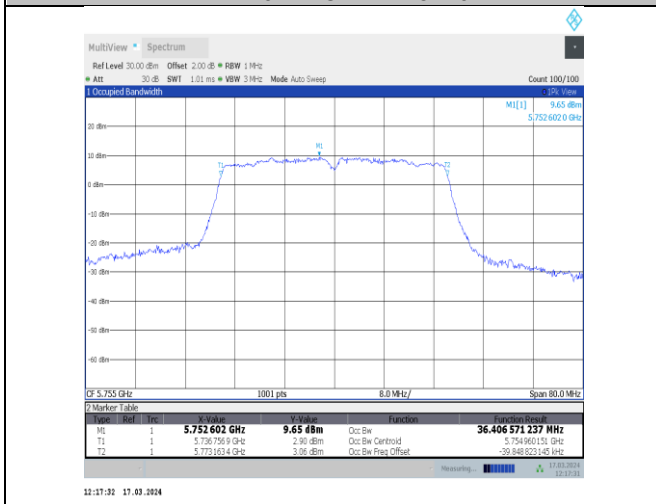
11ac40MIMO-Ant11-5755
