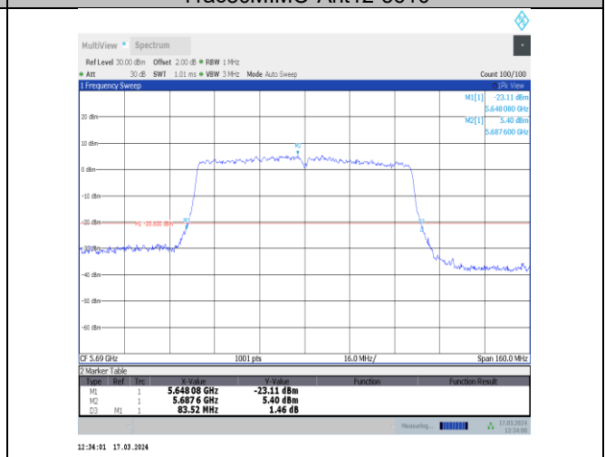
11ac80MIMO-Ant12-5690
