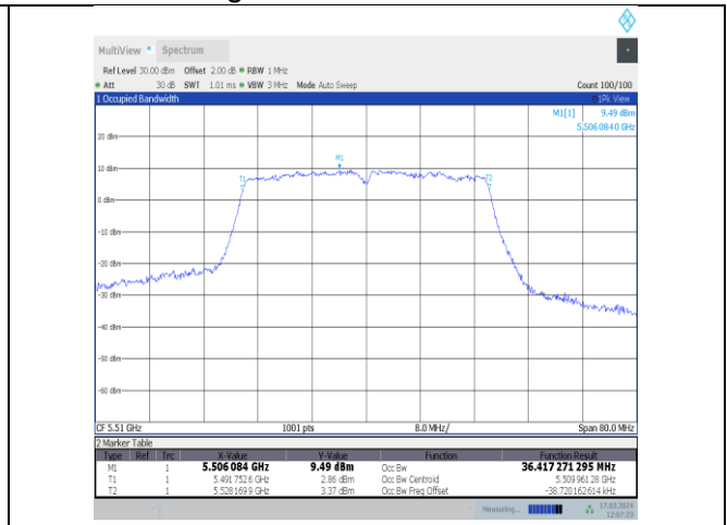
11ac40MIMO-Ant12-5510
