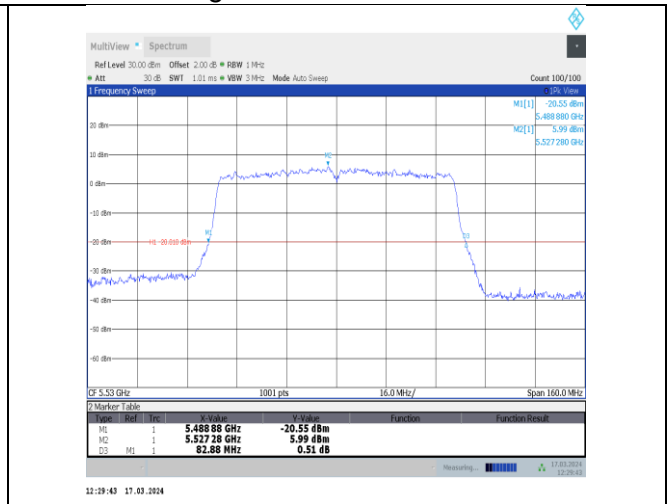
11ac80MIMO-Ant12-5530
