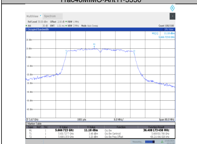
11ac40MIMO-Ant11-5670
