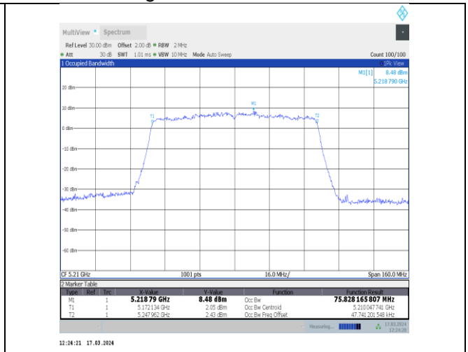
11ac80MIMO-Ant12-5210
