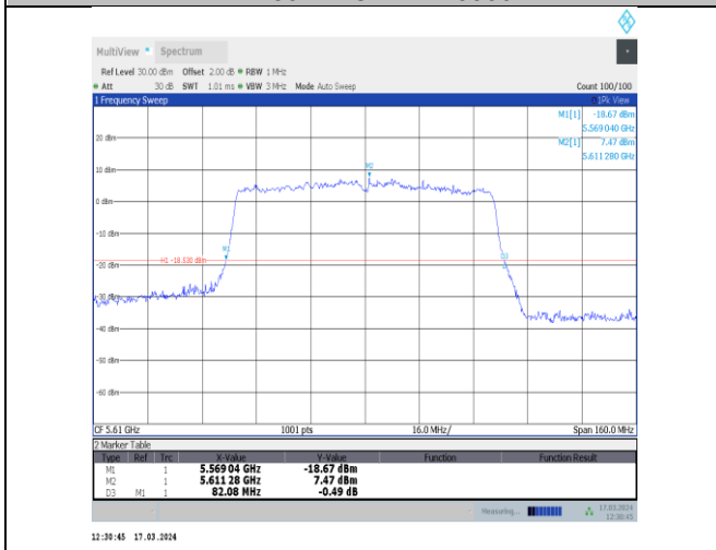
11ac80MIMO-Ant11-5610
