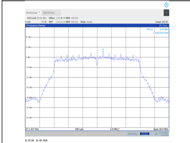
11n20MIMO-Ant10-2437-0~Reference-PASS
