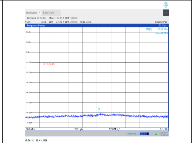
11b-CDD-Ant10-2437-30~1000-PASS
