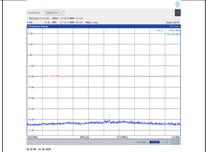
11n40MIMO-Ant10-2452-30~1000-PASS
