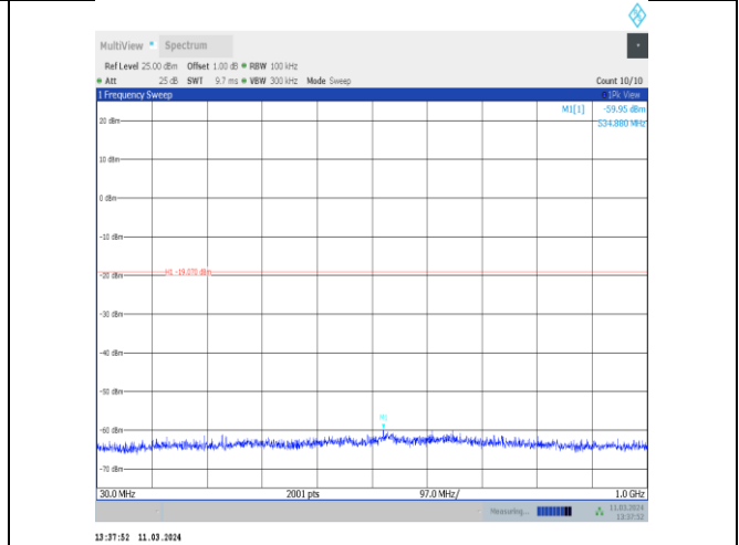
11n40MIMO-Ant10-2437-30~1000-PASS
