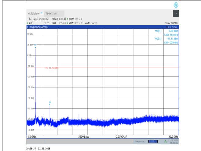
11b-CDD-Ant10-2437-1000~26500-PASS
