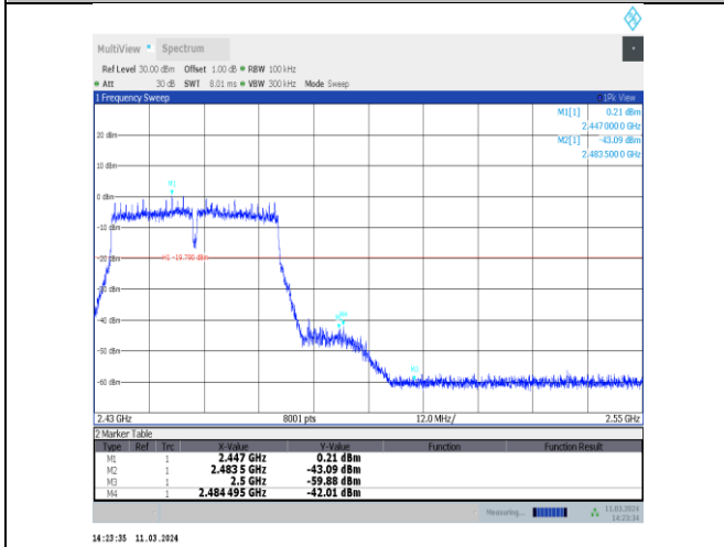
11n40MIMO-Ant10-2452-PASS
