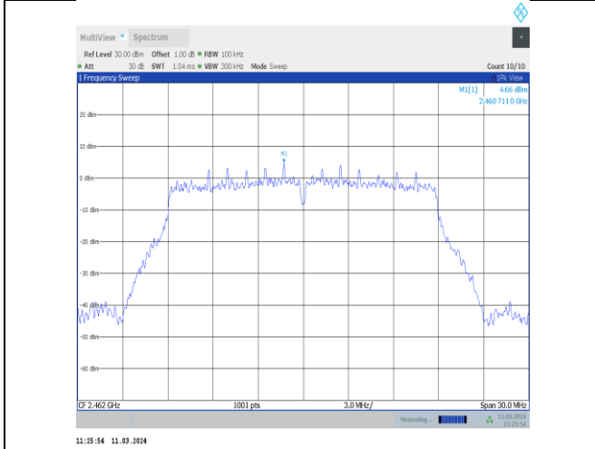
11n20MIMO-Ant10-2462-0~Reference-PASS
