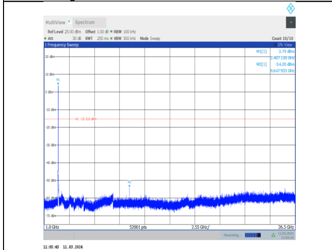
11g-CDD-Ant10-2412-1000~26500-PASS
