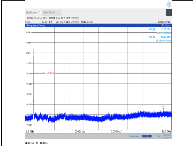
11n40MIMO-Ant10-2452-1000~26500-PASS
