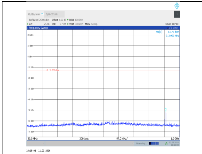
11b-CDD-Ant8-2412-30~1000-PASS
