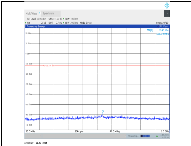
11b-CDD-Ant8-2437-30~1000-PASS
