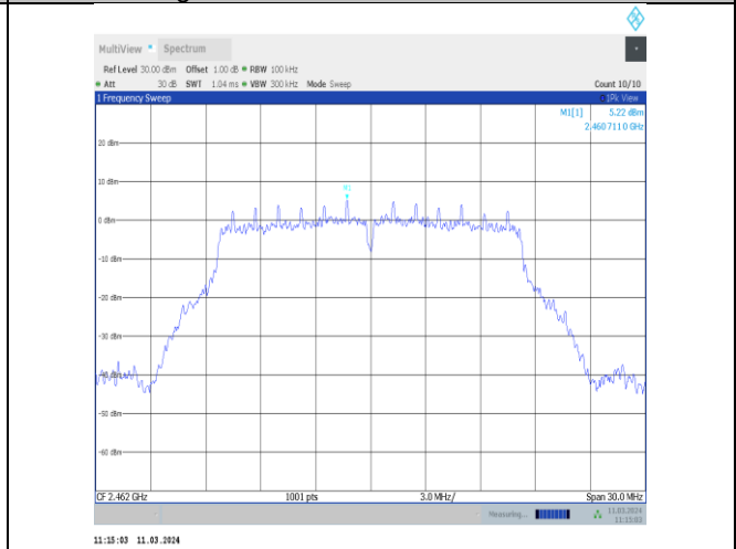
11g-CDD-Ant8-2462-0~Reference-PASS
