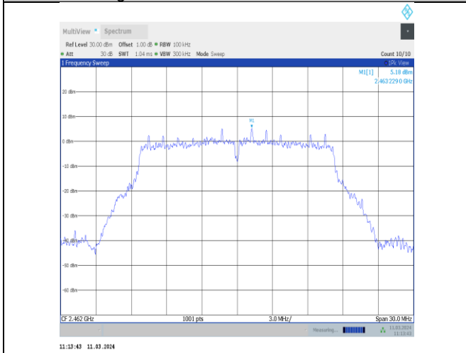
11g-CDD-Ant10-2462-0~Reference-PASS
