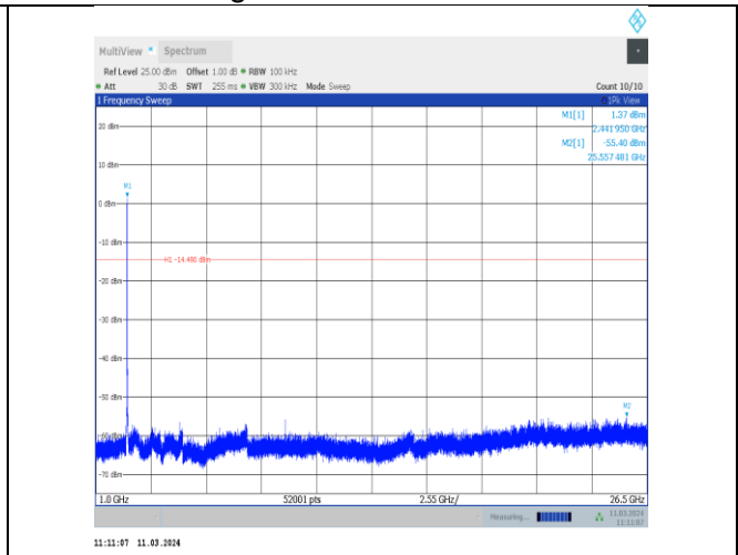
11g-CDD-Ant8-2437-1000~26500-PASS
