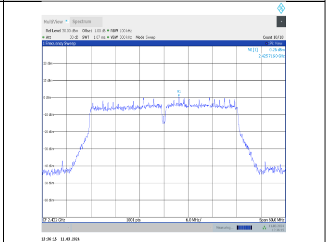
11n40MIMO-Ant8-2422-0~Reference-PASS
