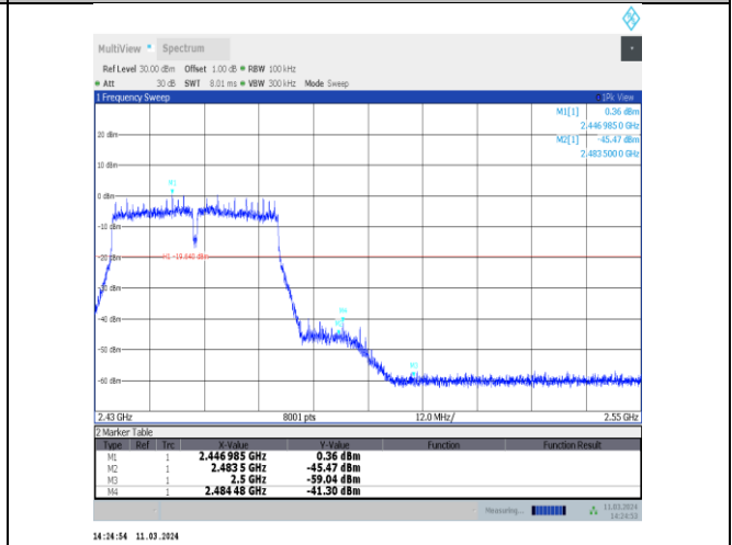
11n40MIMO-Ant8-2452-PASS
