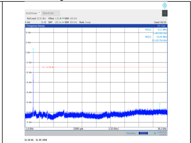
11g-CDD-Ant8-2462-1000~26500-PASS
