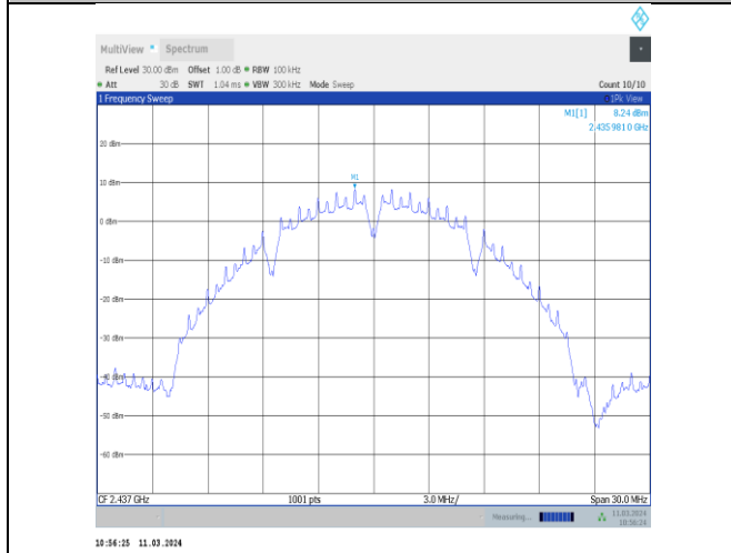
11b-CDD-Ant10-2437-0~Reference-PASS
