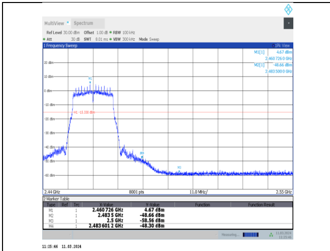
11n20MIMO-Ant10-2462-PASS
