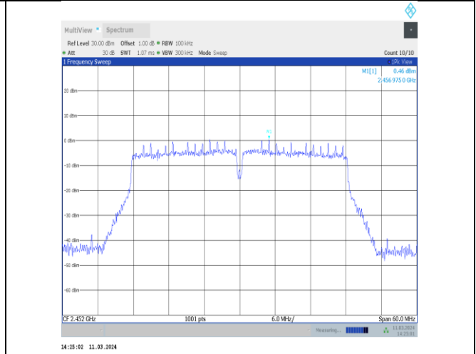
11n40MIMO-Ant8-2452-0~Reference-PASS
