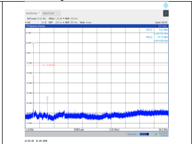
11b-CDD-Ant8-2462-1000~26500-PASS
