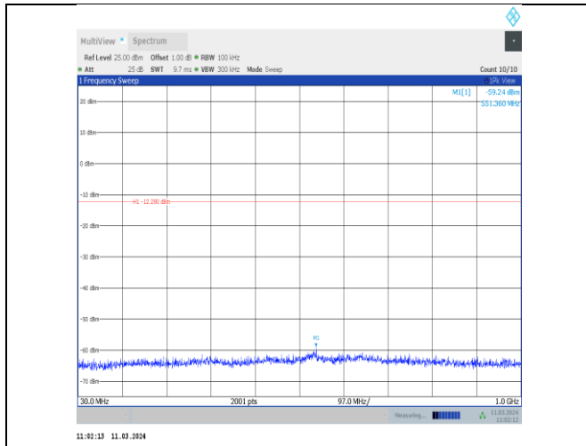
11b-CDD-Ant8-2462-30~1000-PASS
