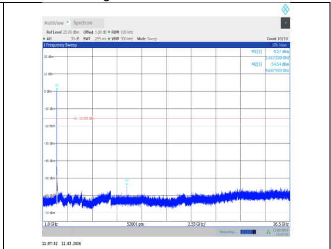
11g-CDD-Ant8-2412-1000~26500-PASS
