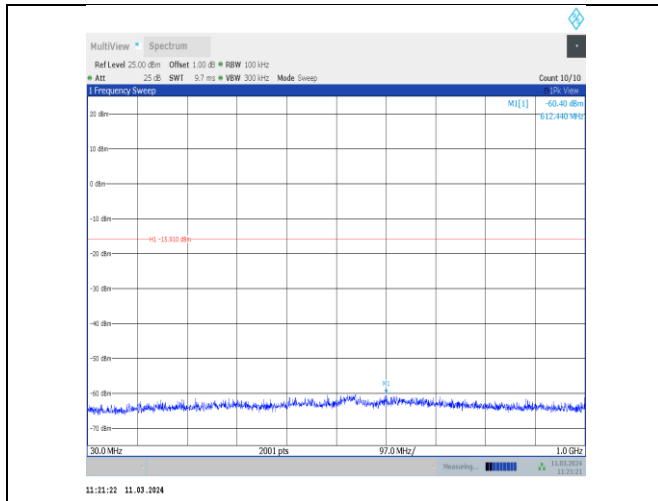
11n20MIMO-Ant8-2412-30~1000-PASS
