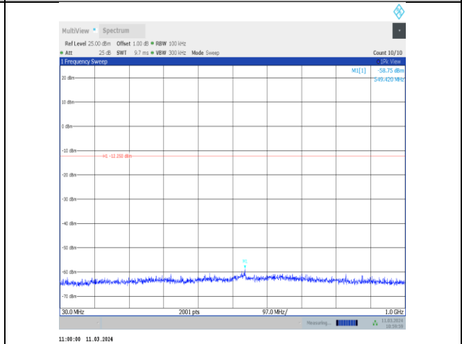
11b-CDD-Ant10-2462-30~1000-PASS
