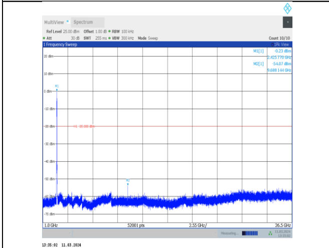
11n40MIMO-Ant10-2422-1000~26500-PASS
