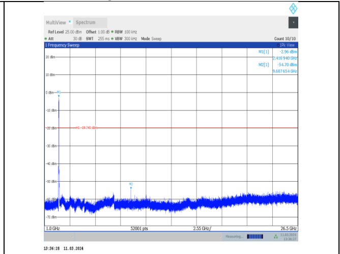
11n40MIMO-Ant8-2422-1000~26500-PASS
