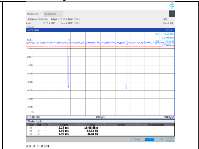
NTVN-11n20MIMO-Ant8-2412
