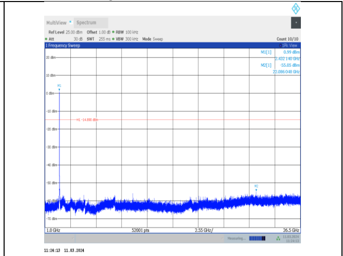
11n20MIMO-Ant8-2437-1000~26500-PASS
