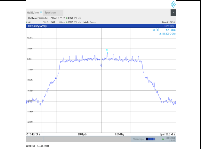
11g-CDD-Ant8-2437-0~Reference-PASS
