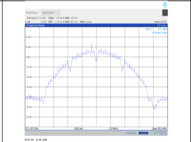
11b-CDD-Ant8-2437-0~Reference-PASS
