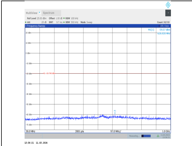
11n40MIMO-Ant8-2422-30~1000-PASS
