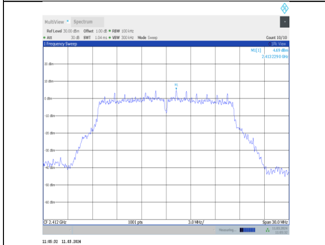
11g-CDD-Ant10-2412-0~Reference-PASS
