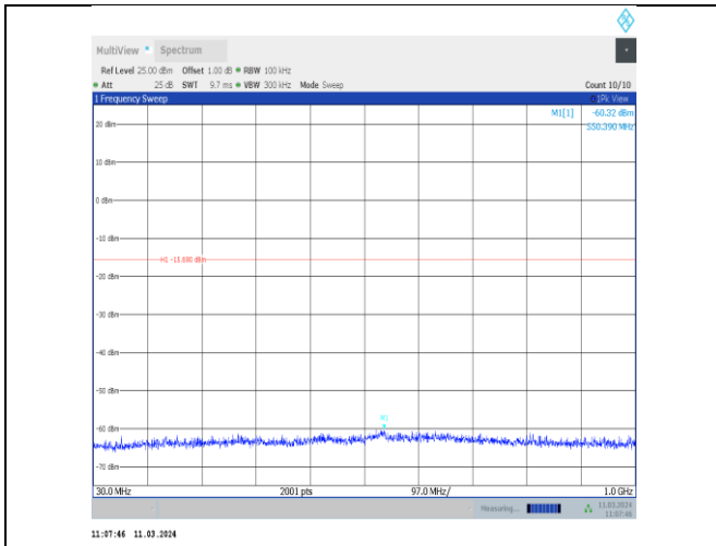
11g-CDD-Ant8-2412-30~1000-PASS
