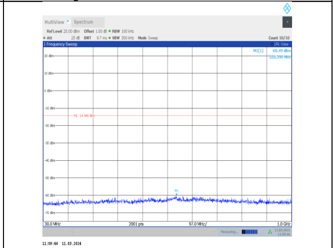
11g-CDD-Ant10-2437-30~1000-PASS
