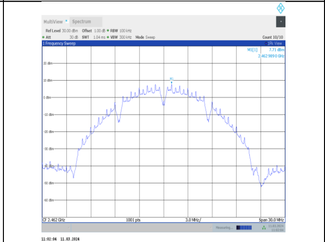
11b-CDD-Ant8-2462-0~Reference-PASS
