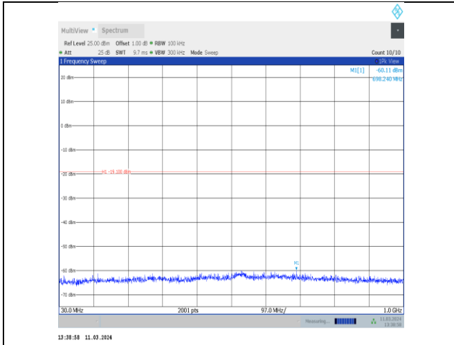
11n40MIMO-Ant8-2437-30~1000-PASS
