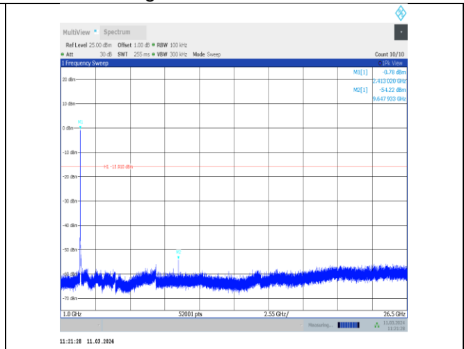
11n20MIMO-Ant8-2412-1000~26500-PASS
