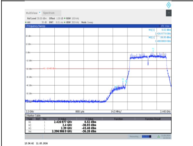
11n40MIMO-Ant10-2422-PASS
