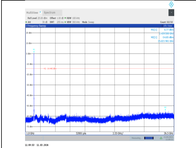
11g-CDD-Ant10-2437-1000~26500-PASS
