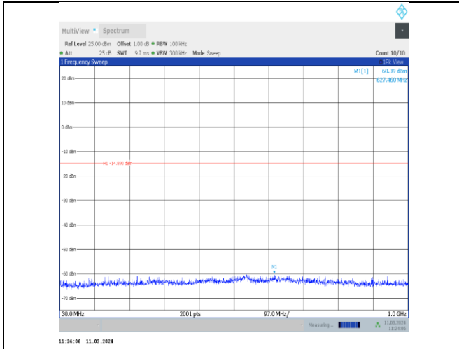
11n20MIMO-Ant8-2437-30~1000-PASS
