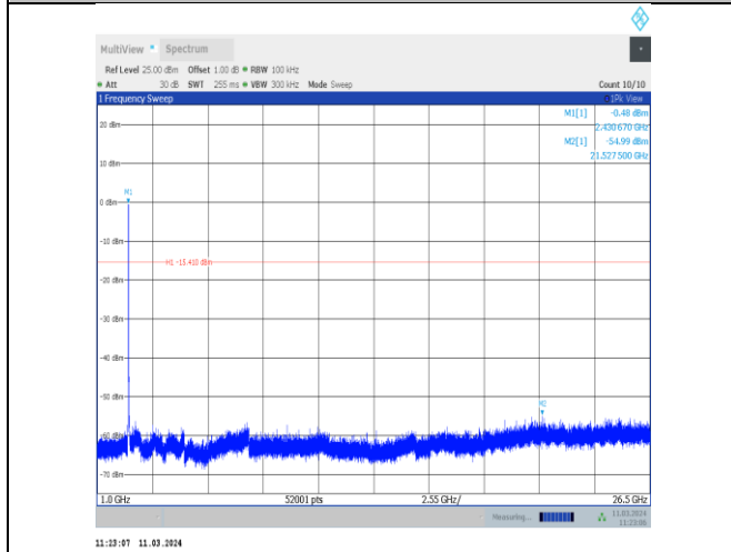
11n20MIMO-Ant10-2437-1000~26500-PASS
