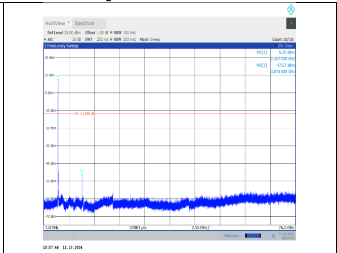
11b-CDD-Ant8-2437-1000~26500-PASS
