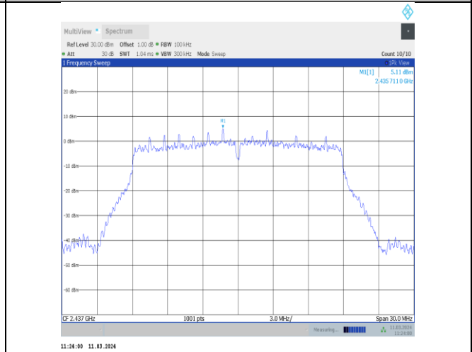
11n20MIMO-Ant8-2437-0~Reference-PASS
