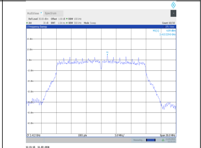
11n20MIMO-Ant8-2412-0~Reference-PASS
