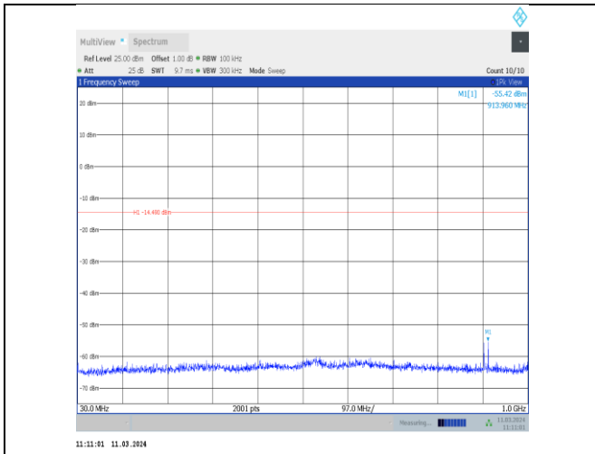
11g-CDD-Ant8-2437-30~1000-PASS
