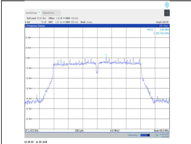
11n40MIMO-Ant10-2422-0~Reference-PASS
