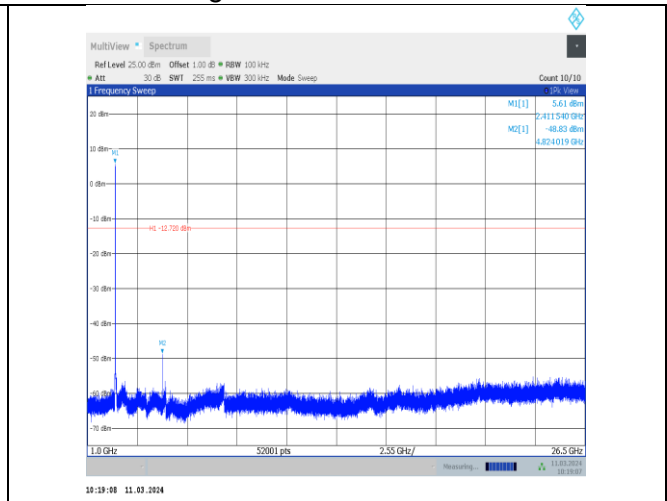
11b-CDD-Ant8-2412-1000~26500-PASS
