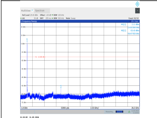
11n20MIMO-Ant10-2412-1000~26500-PASS
