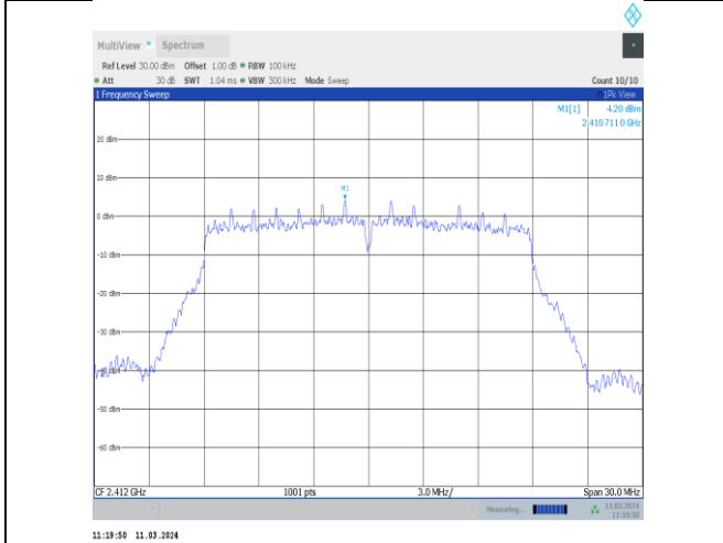
11n20MIMO-Ant10-2412-0~Reference-PASS
