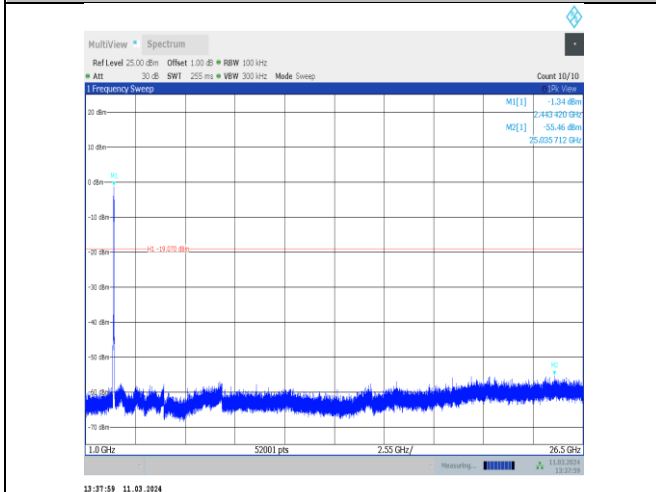
11n40MIMO-Ant10-2437-1000~26500-PASS
