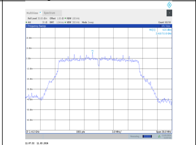
11g-CDD-Ant8-2412-0~Reference-PASS
