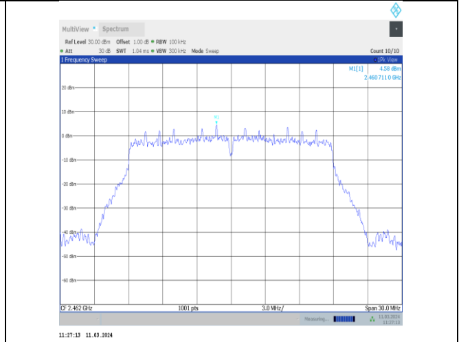
11n20MIMO-Ant8-2462-0~Reference-PASS
