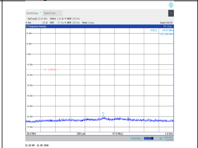
11g-CDD-Ant10-2462-30~1000-PASS
