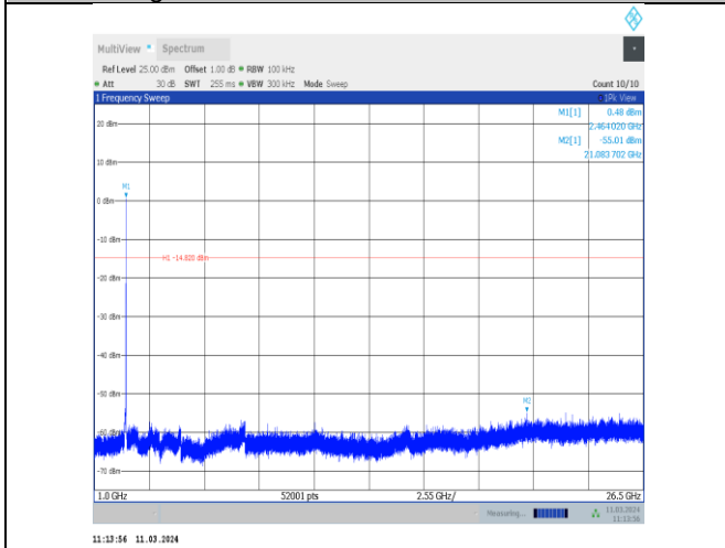
11g-CDD-Ant10-2462-1000~26500-PASS
