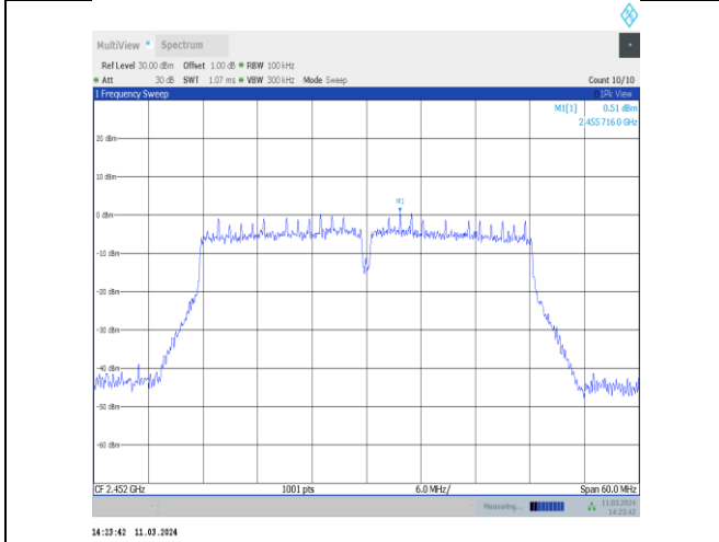
11n40MIMO-Ant10-2452-0~Reference-PASS
