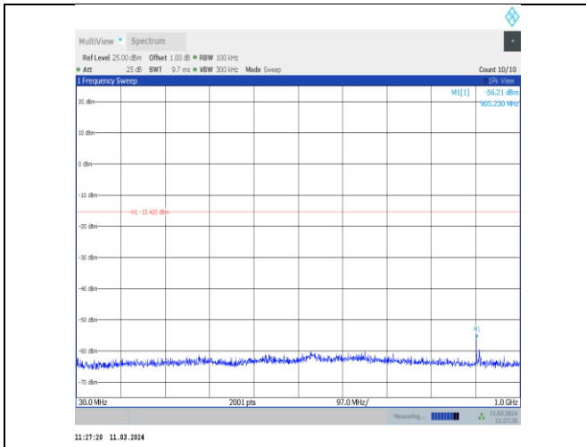
11n20MIMO-Ant8-2462-30~1000-PASS
