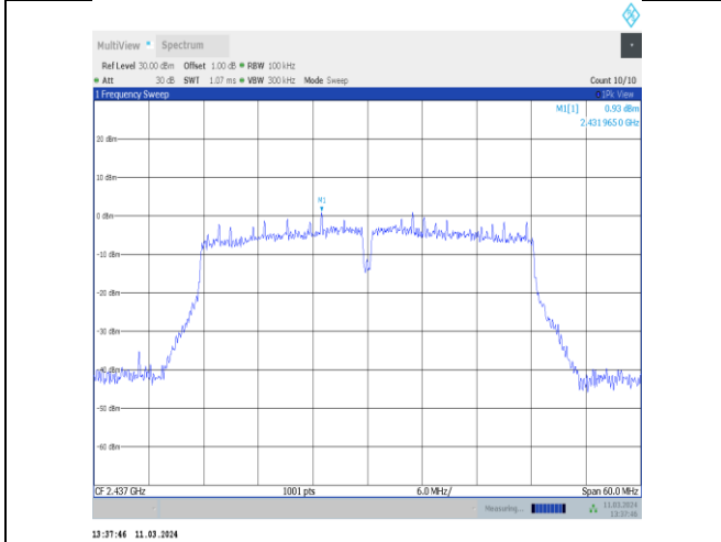
11n40MIMO-Ant10-2437-0~Reference-PASS
