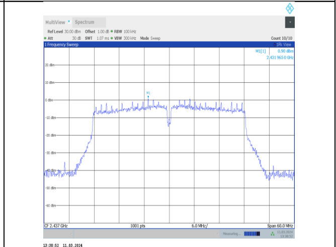
11n40MIMO-Ant8-2437-0~Reference-PASS
