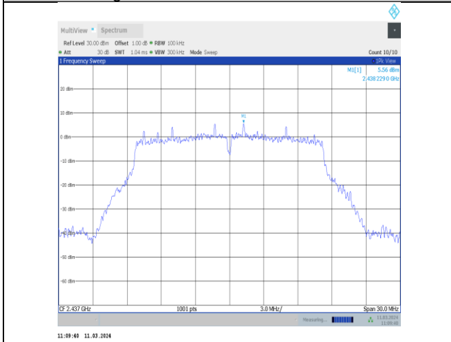
11g-CDD-Ant10-2437-0~Reference-PASS
