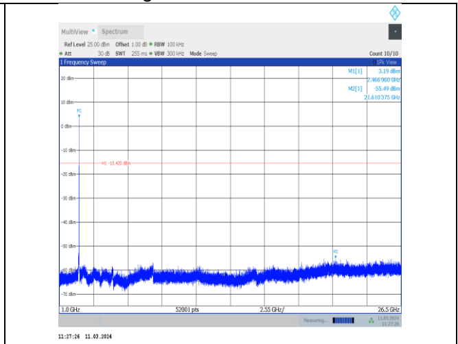
11n20MIMO-Ant8-2462-1000~26500-PASS
