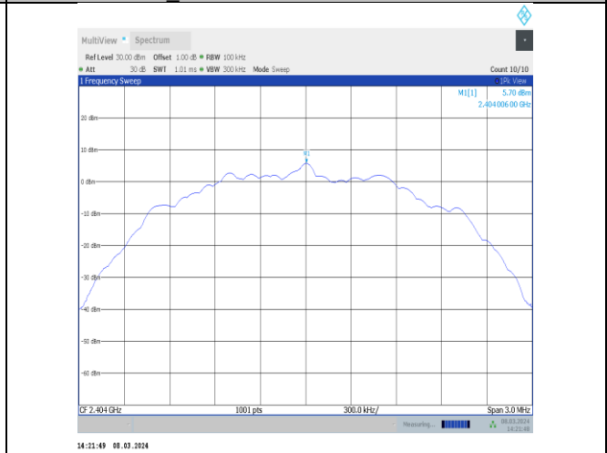
BLE_2M-Ant10-2404-0~Reference-PASS
