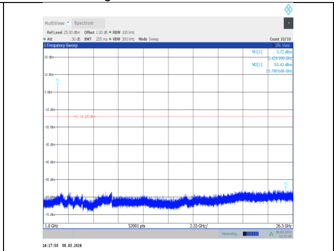
BLE_1M-Ant10-2440-1000~26500-PASS
