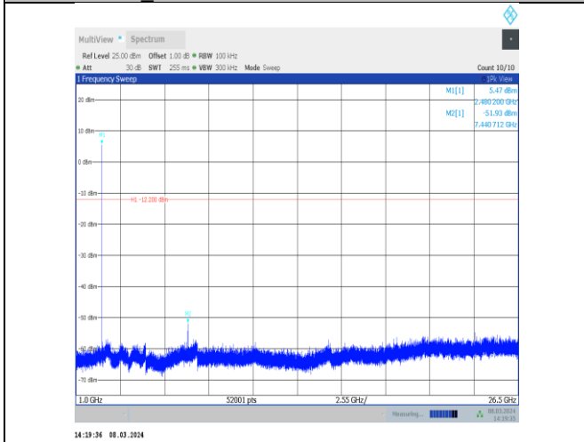
BLE_1M-Ant10-2480-1000~26500-PASS
