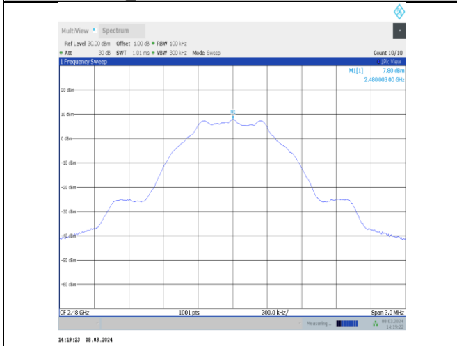
BLE_1M-Ant10-2480-0~Reference-PASS
