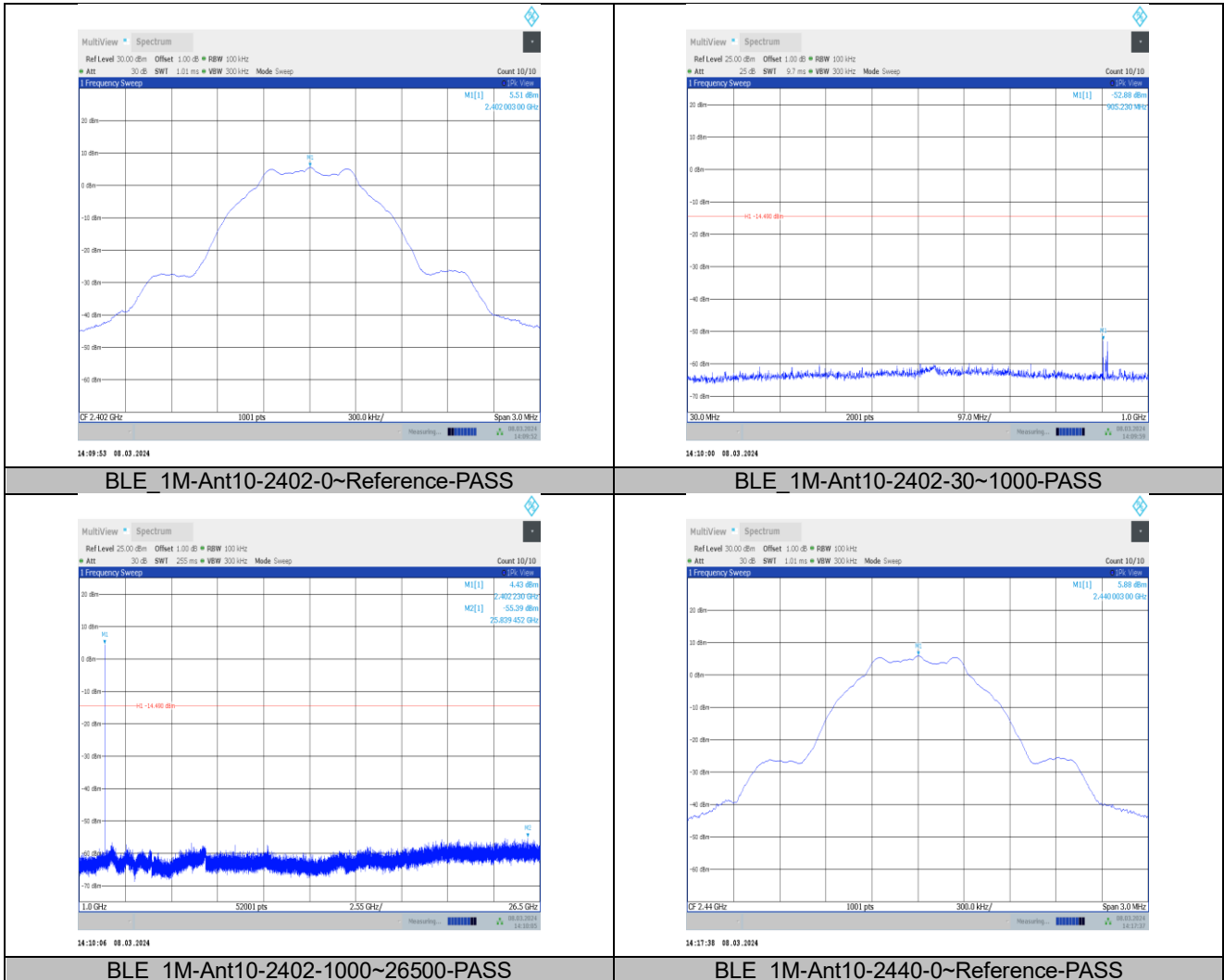
BLE_1M-Ant10-2402-1000~26500-PASS
