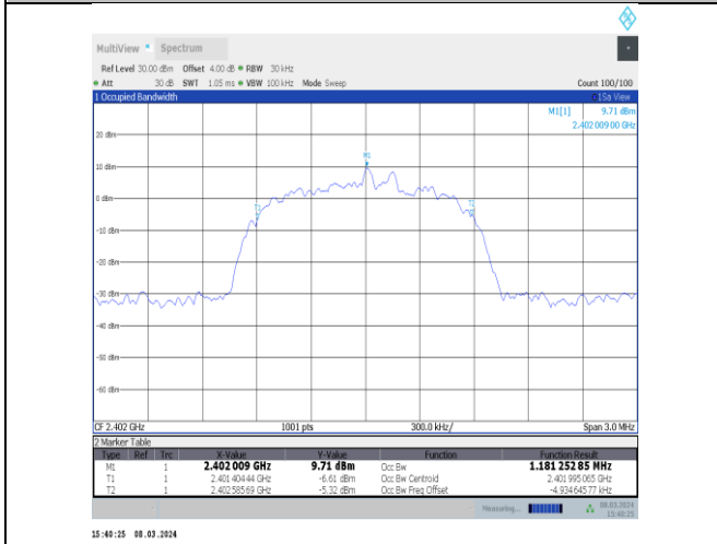
3DH5-Ant10-2402
