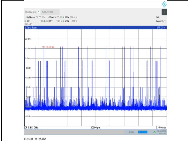
2DH3-Ant10-Hop-PASS
