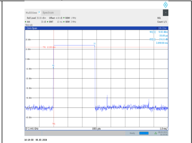
DH5-Ant10-Hop-PASS
