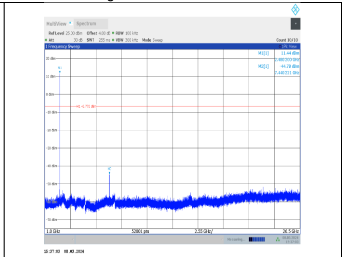
2DH5-Ant10-2480-1000~26500-PASS
