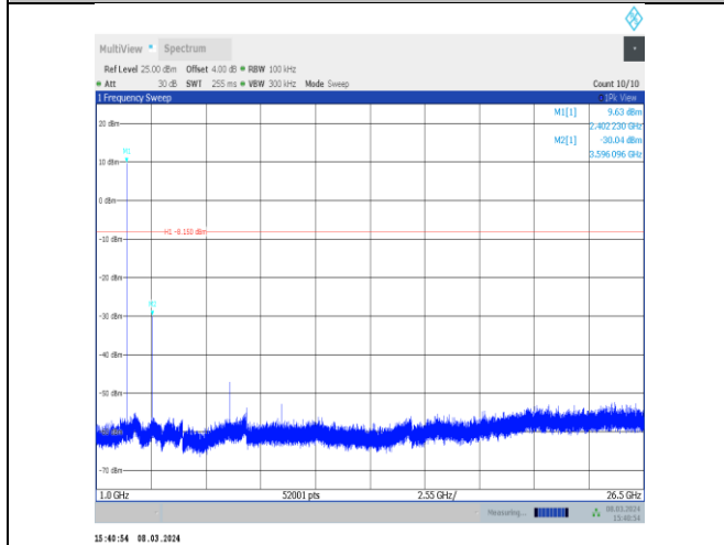
3DH5-Ant10-2402-1000~26500-PASS
