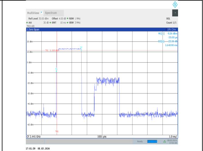
2DH3-Ant10-Hop-PASS
