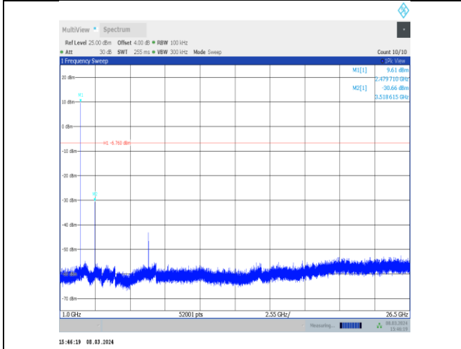
3DH5-Ant10-2480-1000~26500-PASS
