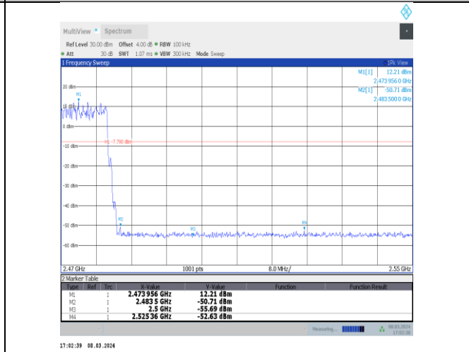
2DH5-Ant10-Hop_2480-PASS
