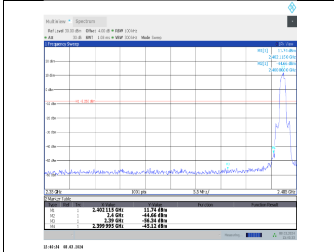
3DH5-Ant10-2402-PASS
