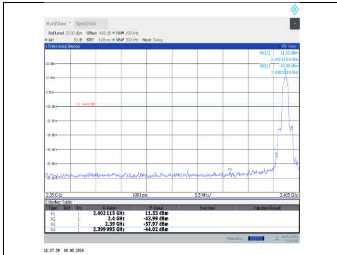
2DH5-Ant10-2402-PASS
