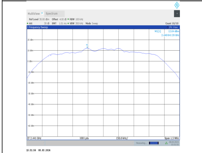
2DH5-Ant10-2441-0~Reference-PASS
