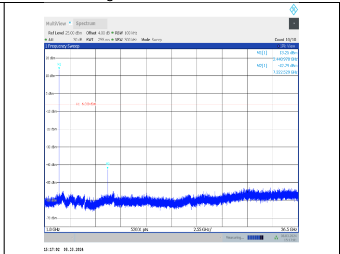
DH5-Ant10-2441-1000~26500-PASS
