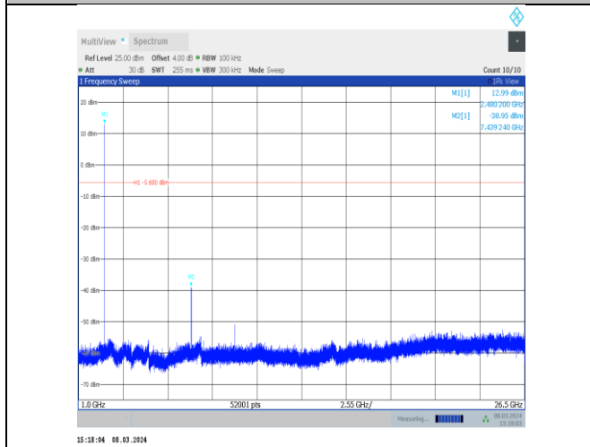
DH5-Ant10-2480-1000~26500-PASS
