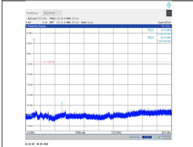
2DH5-Ant10-2441-1000~26500-PASS
