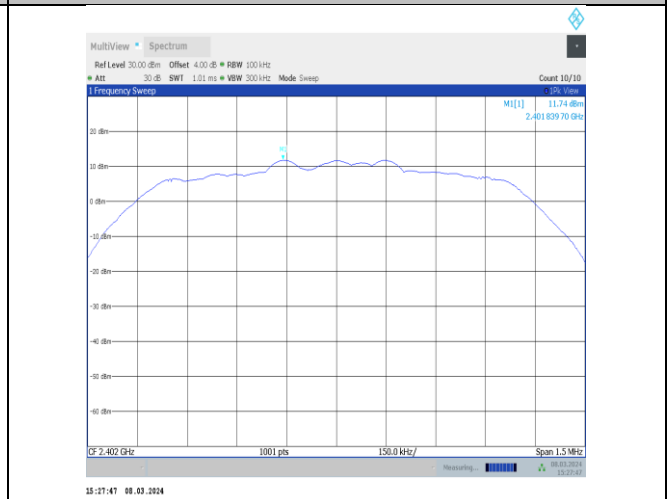
2DH5-Ant10-2402-0~Reference-PASS
