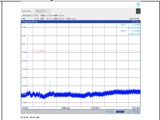
2DH5-Ant10-2402-1000~26500-PASS
