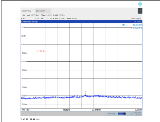
3DH5-Ant10-2441-30~1000-PASS
