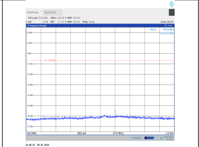
3DH5-Ant10-2480-30~1000-PASS
