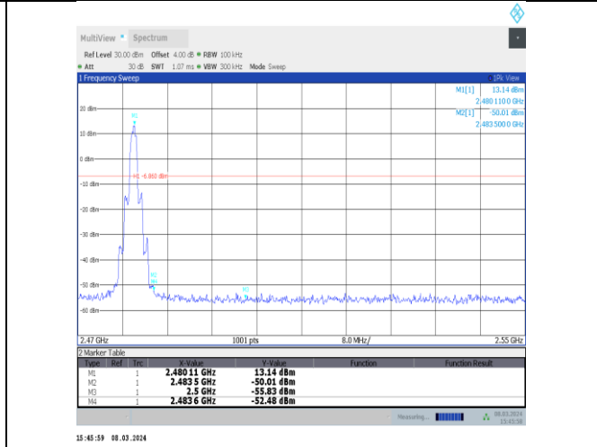
3DH5-Ant10-2480-PASS
