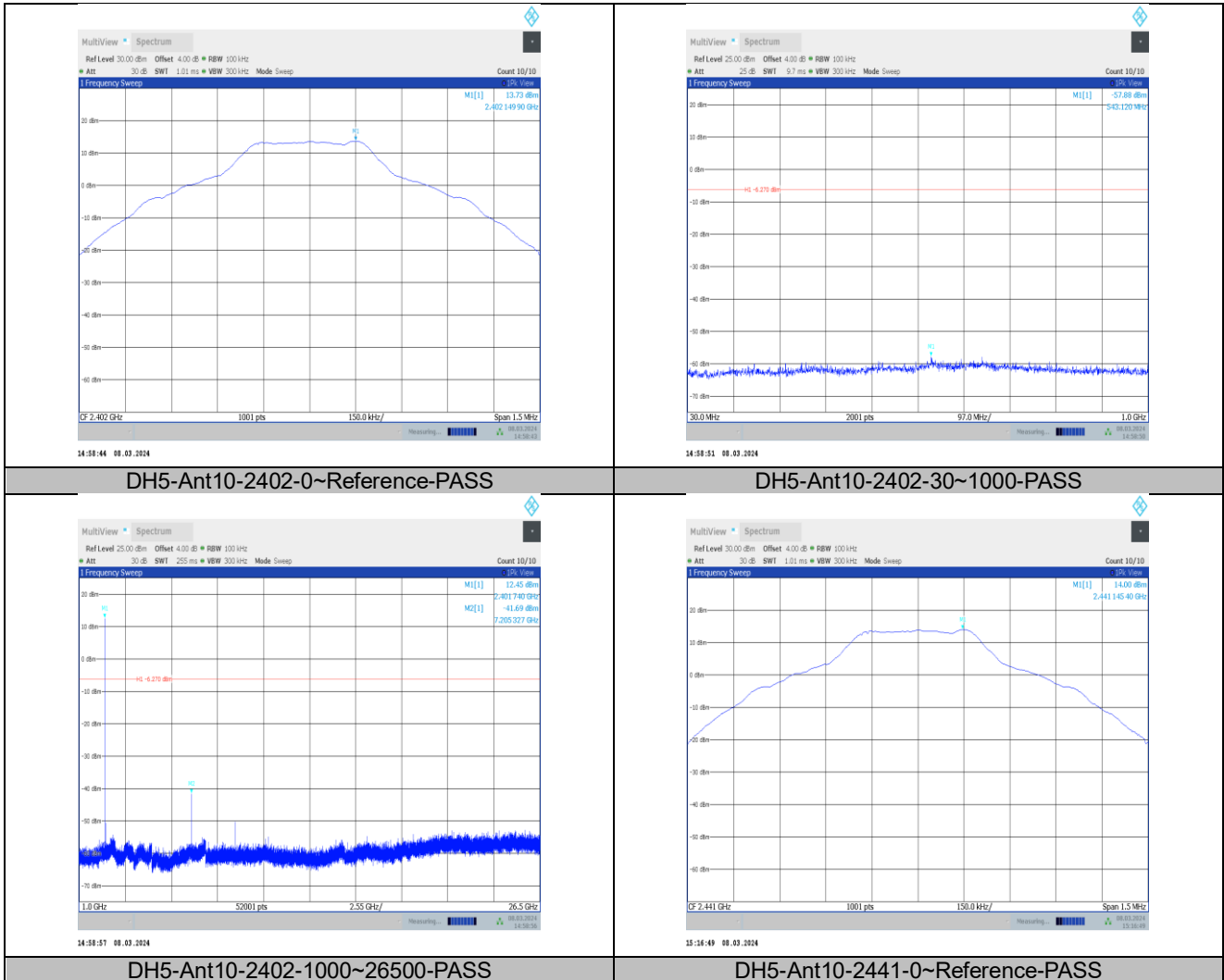
DH5-Ant10-2402-1000~26500-PASS
