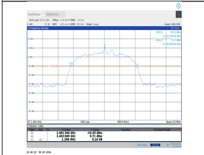
3DH5-Ant10-2402
