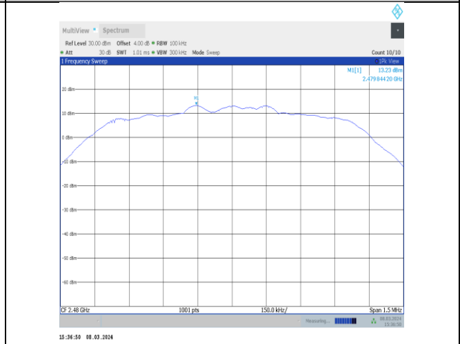
2DH5-Ant10-2480-0~Reference-PASS
