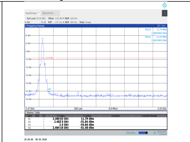
2DH5-Ant10-2480-PASS
