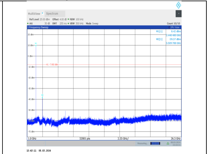
3DH5-Ant10-2441-1000~26500-PASS
