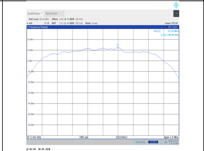
3DH5-Ant10-2441-0~Reference-PASS
