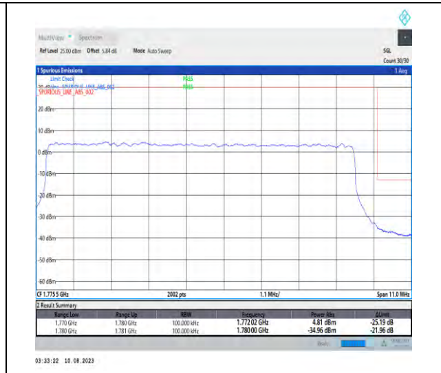
1-N66-PC3-15-10-H-3-DFT-PI2BPSK-Outer_Full-50@0-Ant1-1-seegraph-PASS-see graph
