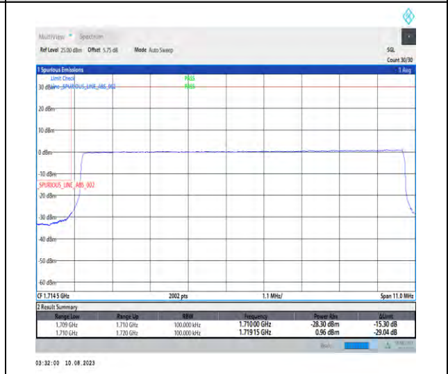
1-N66-PC3-15-10-L-6-CP-QPSK-Outer_Full-52@0-Ant1-1-seegraph-PASS-see graph
