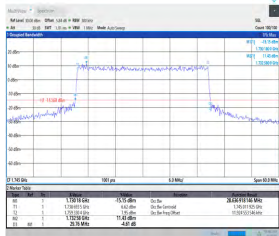
1-N66-PC3-15-30-M-8-CP-64QAM-Outer_Full-160 @0-Ant1-28.637-29.760-<30-PASS
