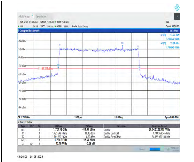
1-N66-PC3-15-40-M-8-CP-64QAM-Outer_Full-216 @0-Ant1-38.642-40.160-≤40-PASS
