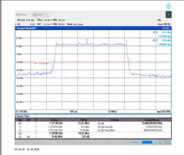
1-N66-PC3-15-15-M-1-DFT-QPSK-Outer_Full-75@ 0-Ant1-13.48-14.460-≤15-PASS
