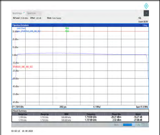
1-N66-PC3-15-40-L-6-CP-QPSK-Outer_Full-216@0-Ant1-1-seegraph-PASS-see graph
