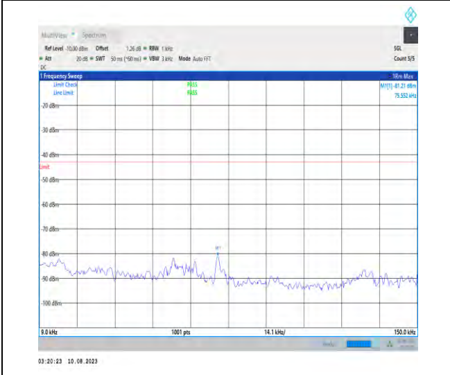
1-N66-PC3-15-40-L-1-N/A-DFT-PI2BPSK-Inner_1R B_Left-1@1-0.009-0.15-Ant1-0.02--81.21--43-PASS
