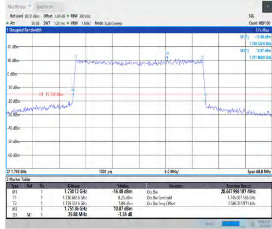
1-N66-PC3-15-30-M-6-CP-QPSK-Outer_Full-160@ -Ant1-28.648-29.880-<30-PASS
