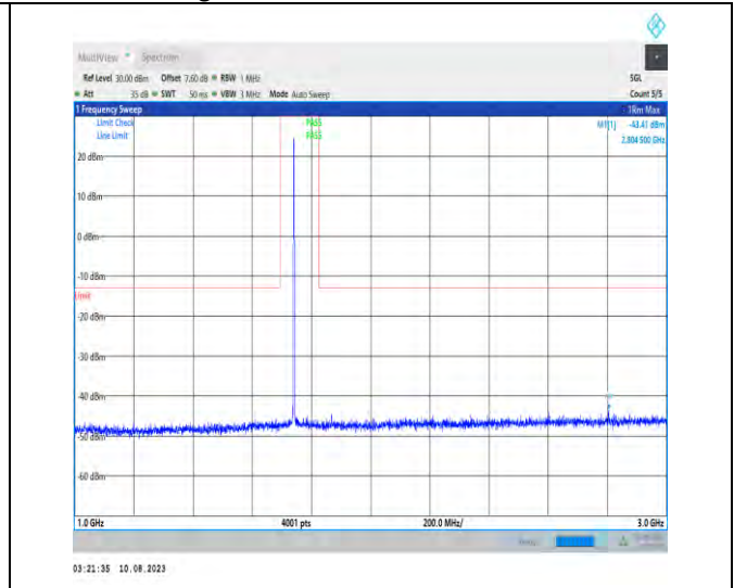
1-N66-PC3-15-40-H-1-N/A-DFT-PI2BPSK-Inner_1RB _Left-1@1-1000-3000-Ant1-2985.00--43.41--13-PASS
