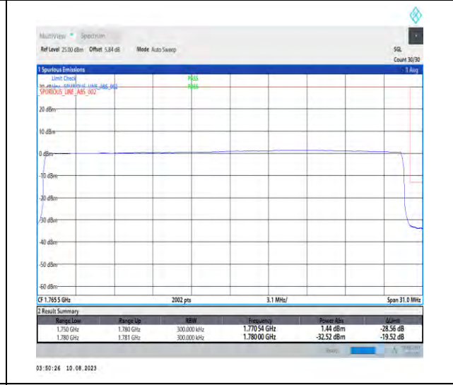
1-N66-PC3-15-30-H-6-CP-QPSK-Outer_Full-160@0-Ant1-1-seegraph-PASS-see graph
