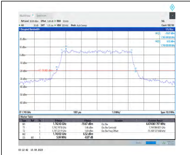
1-N66-PC3-15-5-M-9-CP-256QAM-Outer_Full-25@0-Ant1-4.474-5.040-≤5-PASS
