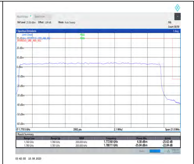
1-N66-PC3-15-20-H-3-DFT-PI2BPSK-Outer_Full-100@0-Ant1-1-seegraph-PASS-see graph
