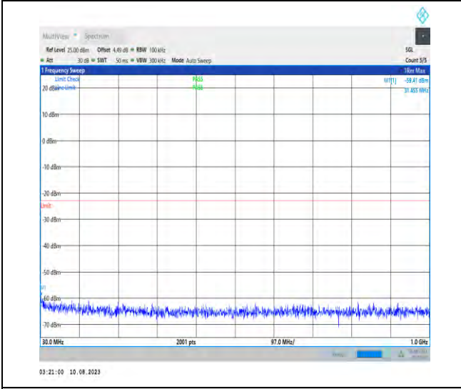
1-N66-PC3-15-40-M-1-N/A-DFT-PI2BPSK-Inner_1R B_Left-1@1-30-1000-Ant1-43.58--59.41--23-PASS
