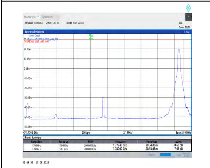
1-N66-PC3-15-20-H-5-CP-QPSK-Edge_1RB_Right-1@105-Ant1-1-seegraph-PASS-see graph
