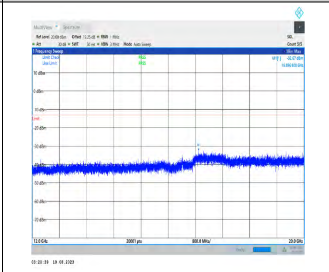
1-N66-PC3-15-40-L-1-N/A-DFT-PI2BPSK-Inner_1RB_Left-1@1-12000-20000-Ant1-19785.20--32.67--13-PASS
