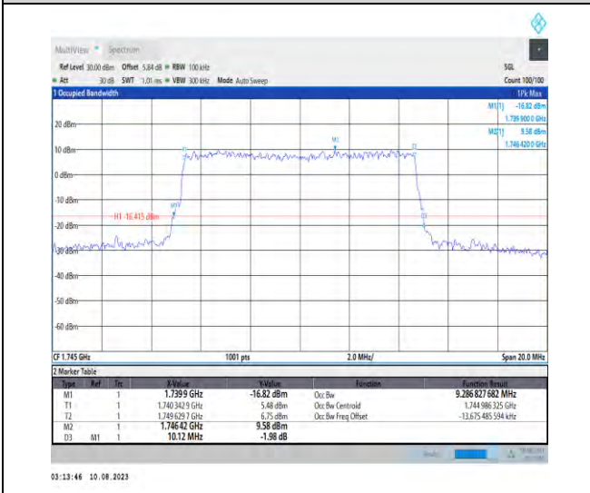
1-N66-PC3-15-10-M-6-CP-QPSK-Outer_Full-52@0- Ant1-9.287-10.120-≤10-PASS
