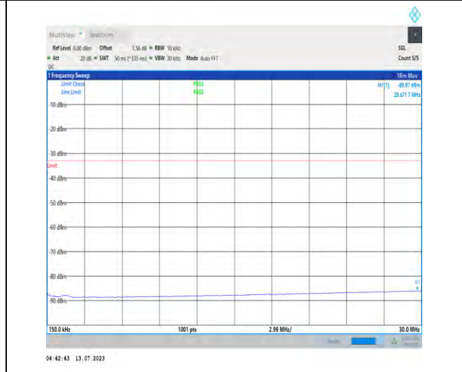
1-N66-PC3-15-30-M-1-N/A-DFT-PI2BPSK-Inner_1RB _Left-1@1-0.15-30-Ant1-29.67--85.97--33-PASS
