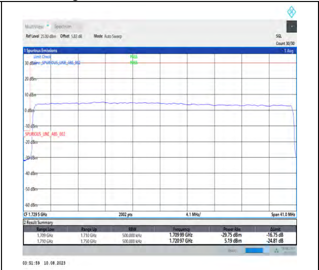
1-N66-PC3-15-40-L-3-DFT-PI2BPSK-Outer_Full-216@0-Ant1-1-seegraph-PASS-see graph
