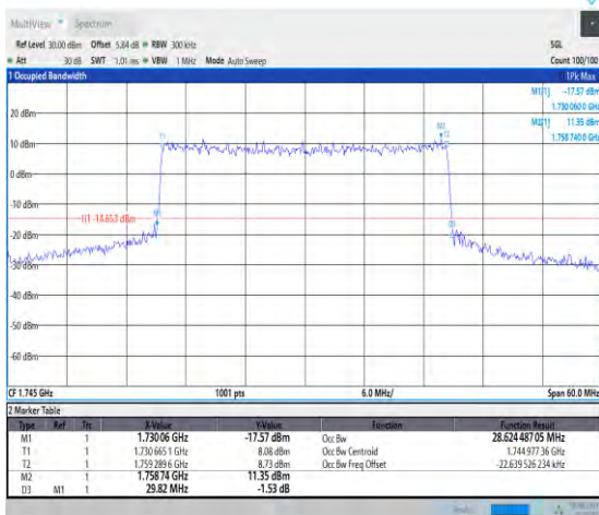
1-N66-PC3-15-30-M-7-CP-16QAM-Outer_Full-160@ 0-Ant1-28.624-29.820-<30-PASS
