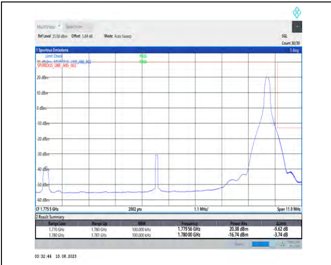
1-N66-PC3-15-10-H-2-DFT-PI2BPSK-Edge_1RB_Right-t-1@51-Ant1-1-seegraph-PASS-see graph
