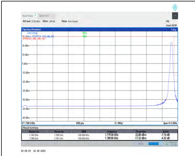
1-N66-PC3-15-40-H-2-DFT-PI2BPSK-Edge_1RB_Right-t-1@215-Ant1-1-seegraph-PASS-see graph
