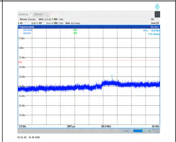
1-N66-PC3-15-40-H-1-N/A-DFT-PI2BPSK-Inner_1RB _Left-1@1-12000-20000-Ant1-17303.20--32.53--13-PASS
