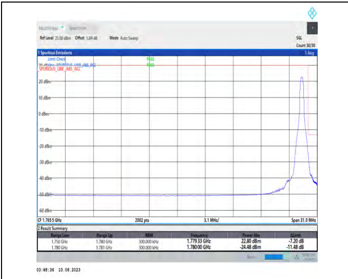
1-N66-PC3-15-30-H-2-DFT-PI2BPSK-Edge_1RB_Right-t-1@159-Ant1-1-seegraph-PASS-see graph
