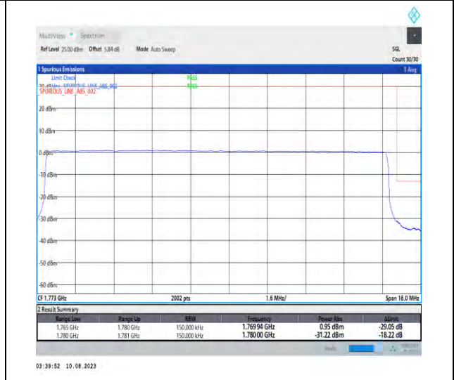
1-N66-PC3-15-15-H-6-CP-QPSK-Outer_Full-79@0-Ant1-1-seegraph-PASS-see graph
