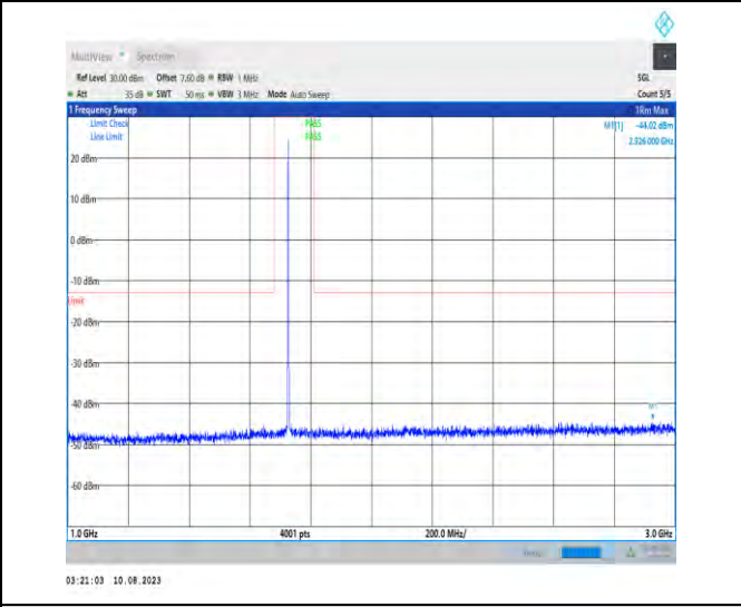
1-N66-PC3-15-40-M-1-N/A-DFT-PI2BPSK-Inner_1RB _Left-1@1-1000-3000-Ant1-2994.00--44.02--13-PASS
