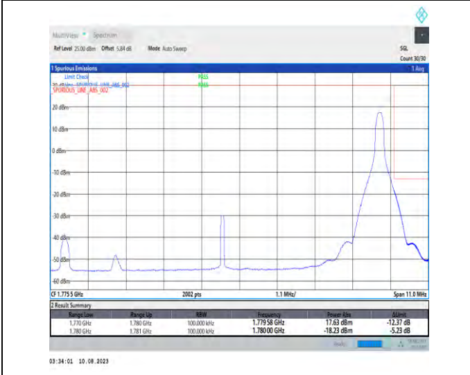
1-N66-PC3-15-10-H-5-CP-QPSK-Edge_1RB_Right-1@51-Ant1-1-seegraph-PASS-see graph
