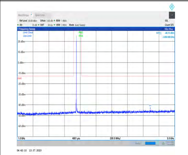
1-N66-PC3-15-30-H-1-N/A-DFT-PI2BPSK-Inner_1RB _Left-1@1-1000-3000-Ant1-2690.00--44.10--13-PASS
