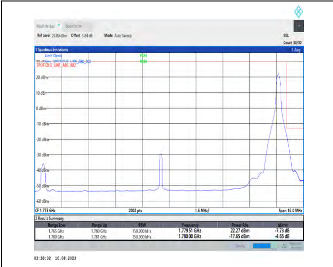
1-N66-PC3-15-15-H-2-DFT-PI2BPSK-Edge_1RB_Right-t-1@78-Ant1-1-seegraph-PASS-see graph
