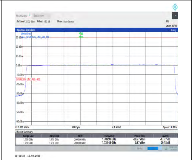
1-N66-PC3-15-20-L-6-CP-QPSK-Outer_Full-106@0-Ant1-1-seegraph-PASS-see graph
