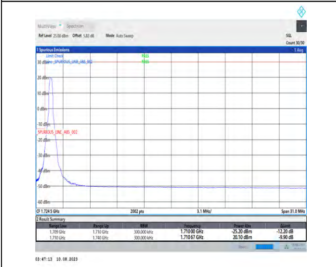
1-N66-PC3-15-30-L-4-CP-QPSK-Edge_1RB_Left-1@0-Ant1-1-seegraph-PASS-see graph
