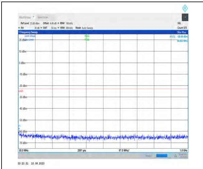
1-N66-PC3-15-40-L-1-N/A-DFT-PI2BPSK-Inner_1RB_Left-1@1-30-1000-Ant1-31.94--58.48--23-PASS
