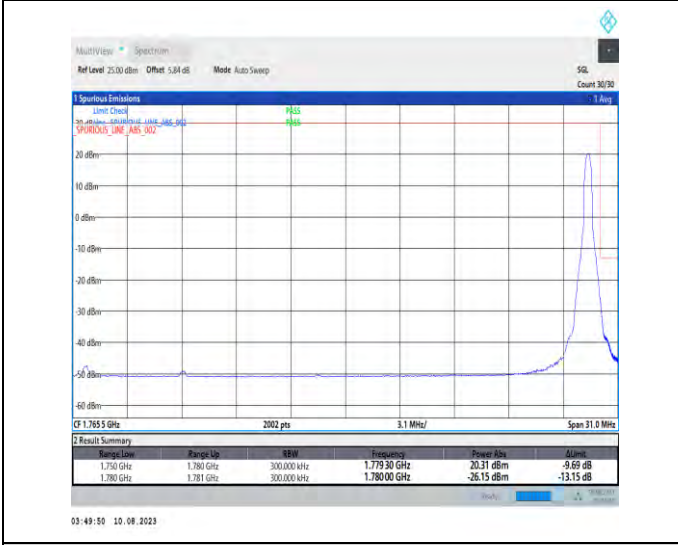
1-N66-PC3-15-30-H-5-CP-QPSK-Edge_1RB_Right-1@159-Ant1-1-seegraph-PASS-see graph
