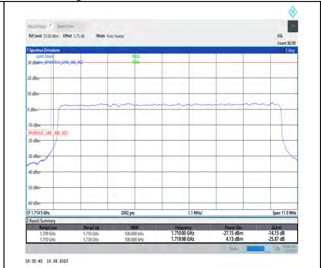
1-N66-PC3-15-10-L-3-DFT-PI2BPSK-Outer_Full-50@0-Ant1-1-seegraph-PASS-see graph
