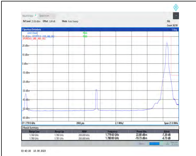
1-N66-PC3-15-20-H-2-DFT-PI2BPSK-Edge_1RB_Right-t-1@105-Ant1-1-seegraph-PASS-see graph
