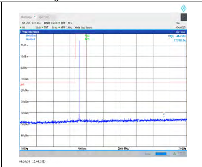
1-N66-PC3-15-40-L-1-N/A-DFT-PI2BPSK-Inner_1RB_Left-1@1-1000-3000-Ant1-2996.50--44.42--13-PASS
