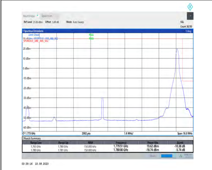
1-N66-PC3-15-15-H-5-CP-QPSK-Edge_1RB_Right-1@78-Ant1-1-seegraph-PASS-see graph
