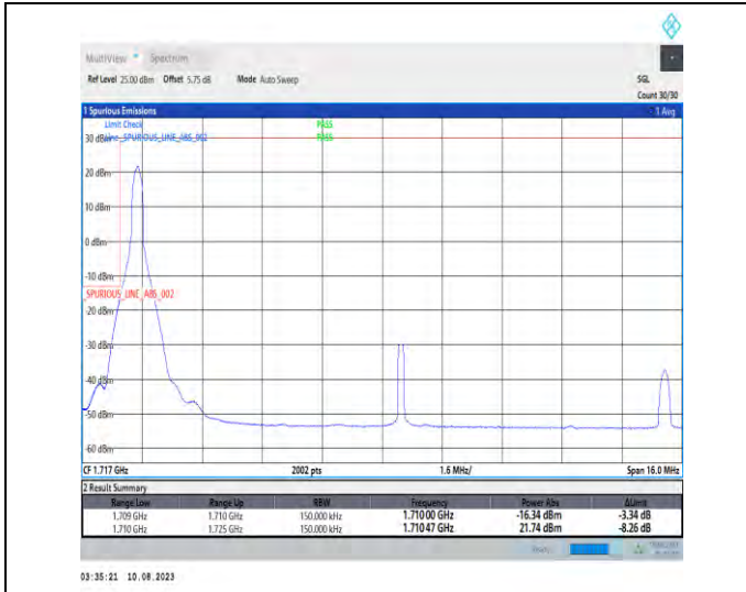
1-N66-PC3-15-15-L-1-DFT-PI2BPSK-Edge_1RB_Left-1@0-Ant1-1-seegraph-PASS-see graph
