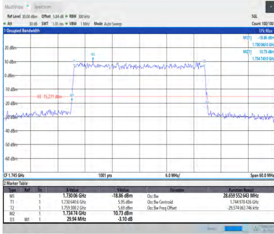
1-N66-PC3-15-30-M-5-DFT-256QAM-Outer_Full-160 @0-Ant1-28.66-29.940-<30-PASS
