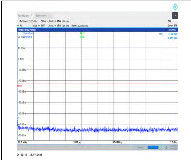
1-N66-PC3-15-30-M-1-N/A-DFT-PI2BPSK-Inner_1R B_Left-1@1-30-1000-Ant1-31.46--57.78--23-PASS
