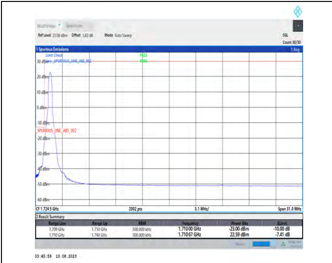
1-N66-PC3-15-30-L-1-DFT-PI2BPSK-Edge_1RB_Left-1@0-Ant1-1-seegraph-PASS-see graph
