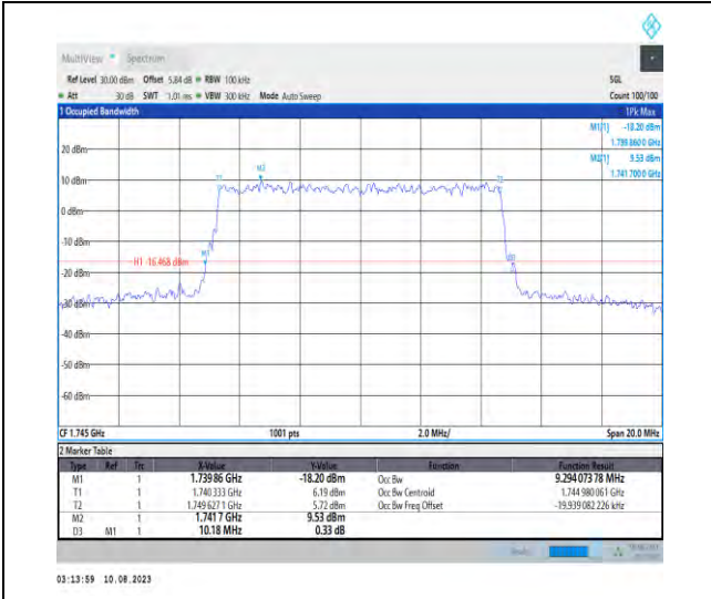
1-N66-PC3-15-10-M-8-CP-64QAM-Outer_Full-52@ 0-Ant1-9.294-10.180-≤10-PASS
