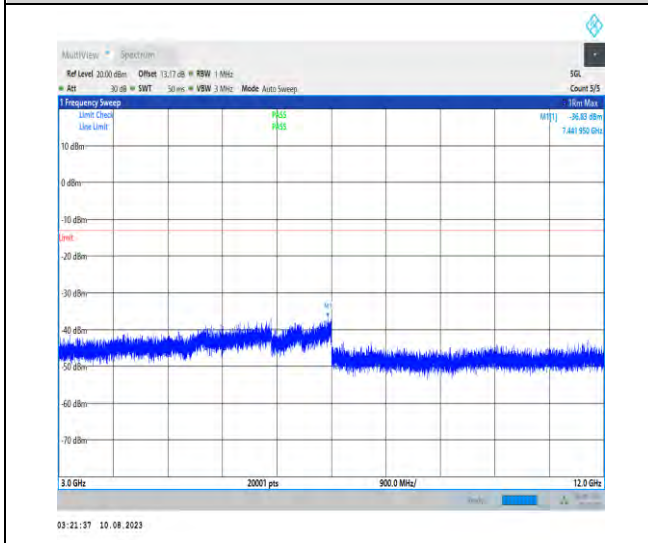
1-N66-PC3-15-40-H-1-N/A-DFT-PI2BPSK-Inner_1R B_Left-1@1-3000-12000-Ant1-7465.35--36.83--13-PASS
