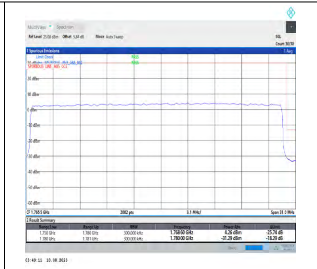
1-N66-PC3-15-30-H-3-DFT-PI2BPSK-Outer_Full-160@0-Ant1-1-seegraph-PASS-see graph
