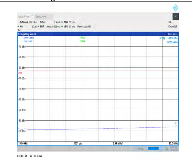
1-N66-PC3-15-30-H-1-N/A-DFT-PI2BPSK-Inner_1RB _Left-1@1-0.15-30-Ant1-29.55--85.95--33-PASS
