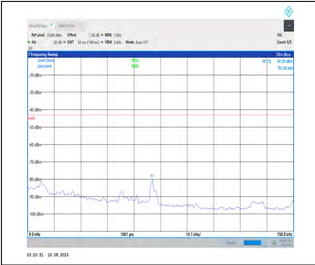
1-N66-PC3-15-40-M-1-N/A-DFT-PI2BPSK-Inner_1R B_Left-1@1-0.009-0.15-Ant1-0.02--81.33--43-PASS
