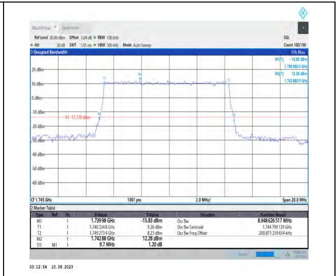
1-N66-PC3-15-10-M-1-DFT-QPSK-Outer_Full-50@0-Ant1-8.949-9.700-≤10-PASS
