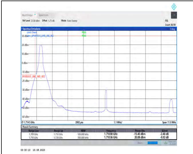
1-N66-PC3-15-10-L-1-DFT-PI2BPSK-Edge_1RB_Left-1@0-Ant1-1-seegraph-PASS-see graph
