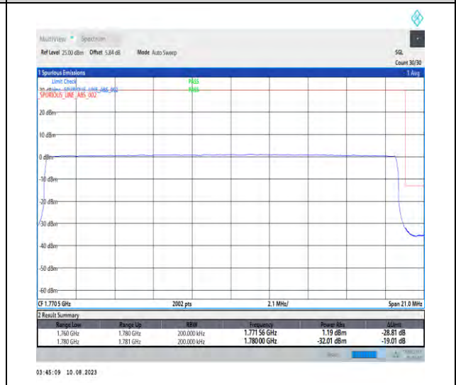
1-N66-PC3-15-20-H-6-CP-QPSK-Outer_Full-106@0-Ant1-1-seegraph-PASS-see graph
