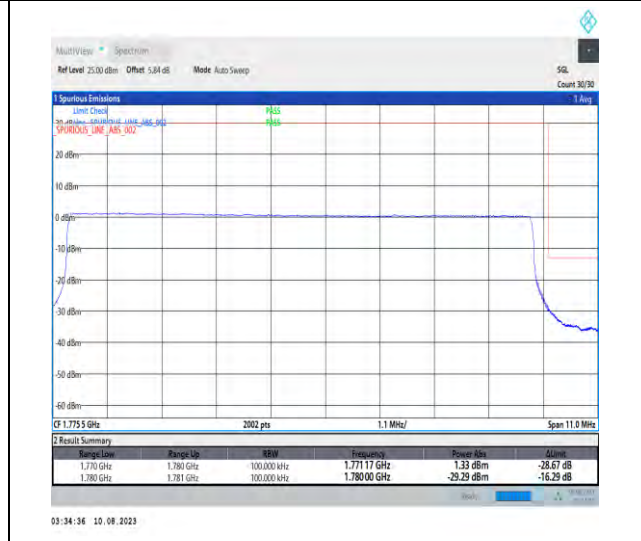
1-N66-PC3-15-10-H-6-CP-QPSK-Outer_Full-52@0-Ant1-1-seegraph-PASS-see graph
