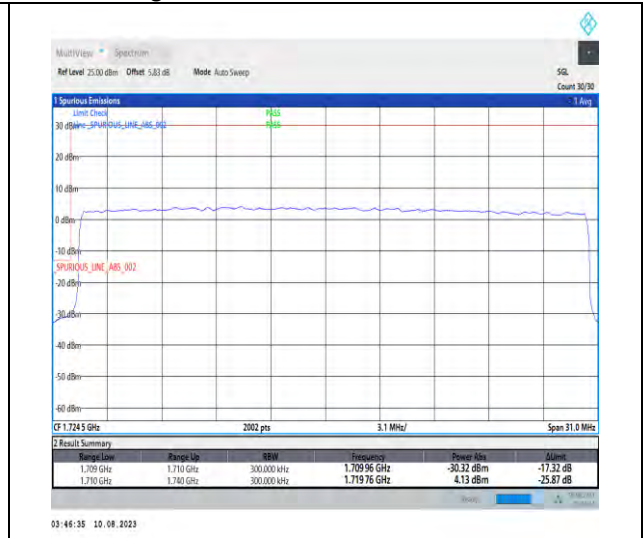
1-N66-PC3-15-30-L-3-DFT-PI2BPSK-Outer_Full-160@0-Ant1-1-seegraph-PASS-see graph
