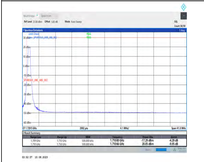
1-N66-PC3-15-40-L-4-CP-QPSK-Edge_1RB_Left-1@0-Ant1-1-seegraph-PASS-see graph
