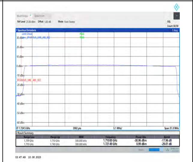
1-N66-PC3-15-30-L-6-CP-QPSK-Outer_Full-160@0-Ant1-1-seegraph-PASS-see graph
