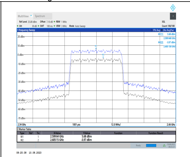
1-N38-PC3-30-40-H-2-CP-256QAM-Outer_Full-106 @0-Ant1-9.65-100%-0.00-9.65-PASS-≤13
