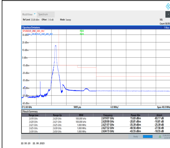
1-N38-PC3-30-10-H-5-CP-QPSK-Edge_1RB_Right1@23-Ant1-1--PASS-see graph
