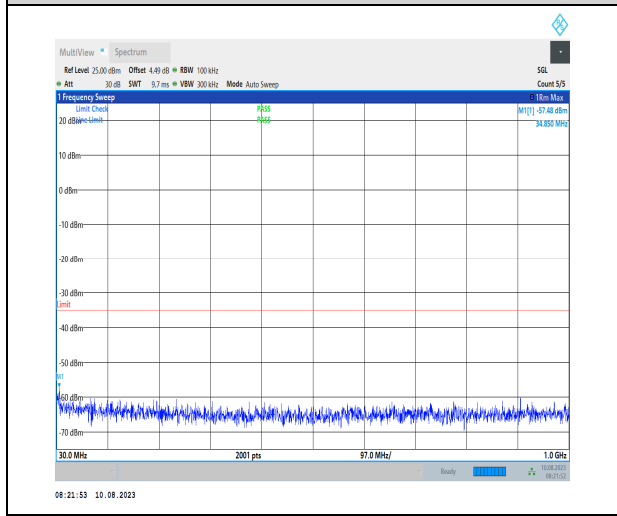
1-N38-PC3-30-40-L-1-N/A-DFT-PI2BPSK-Inner_1R B_Left-1@1-30-1000-Ant1-30.97--57.48--35-PASS
