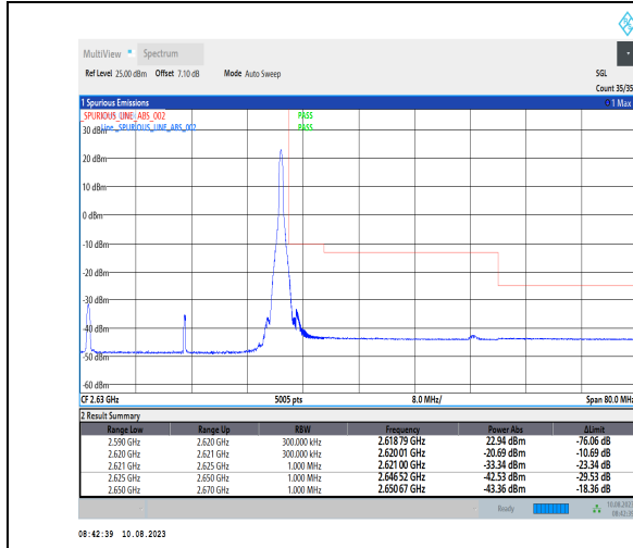
1-N38-PC3-30-30-H-2-DFT-PI2BPSK-Edge_1RB_Right-t-1@77-Ant1-1--PASS-see graph
