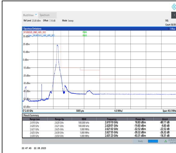
1-N38-PC3-30-10-H-2-DFT-PI2BPSK-Edge_1RB_Right-t1@23-Ant1-1--PASS-see graph
