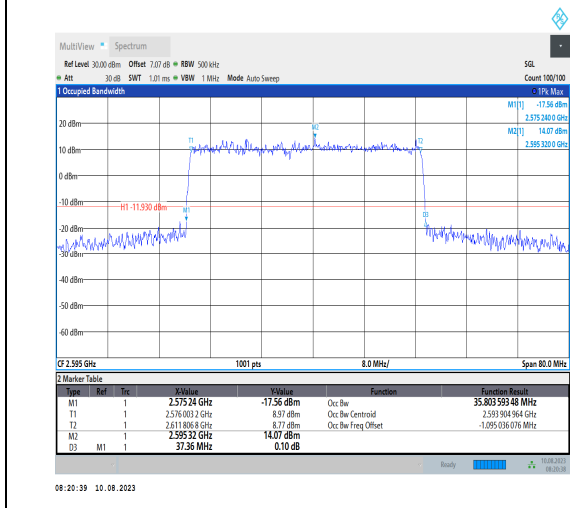
1-N38-PC3-30-40-M-3-DFT-16QAM-Outer_Full-100 @0-Ant1-35.804-37.360-≤40-PASS
