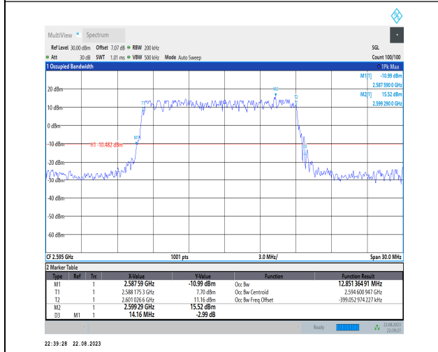
1-N38-PC3-30-15-M-2-DFT-PI2BPSK-Outer_Full-36 @0-Ant1-12.851-14.160-≤15-PASS
