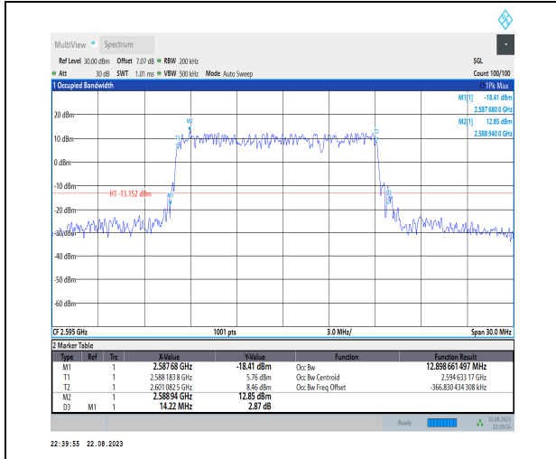
1-N38-PC3-30-15-M-4-DFT-64QAM-Outer_Full-36@ 0-Ant1-12.899-14.220-≤15-PASS
