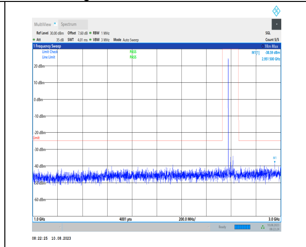
1-N38-PC3-30-40-M-1-N/A-DFT-PI2BPSK-Inner_1RB_Left-1@1-1000-3000-Ant1-2940.50--38.59--25-PASS
