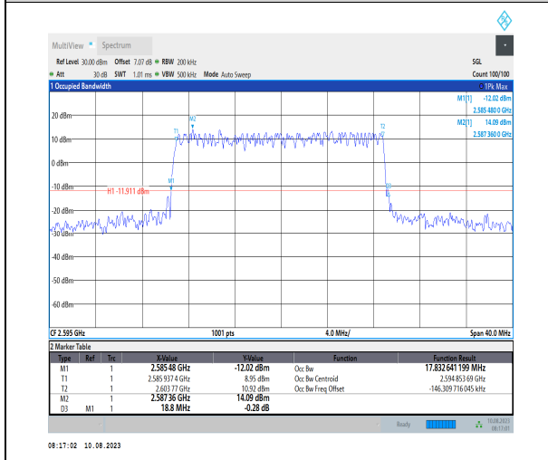
1-N38-PC3-30-20-M-1-DFT-QPSK-Outer_Full-50@ 0-Ant1-17.833-18.800-≤20-PASS
