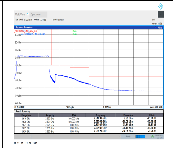
1-N38-PC3-30-10-H-6-CP-QPSK-Outer_Full-24@0-Ant1-1--PASS-see graph
