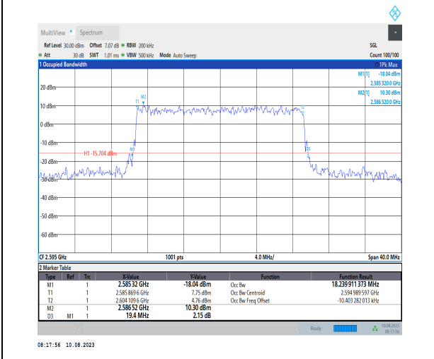
1-N38-PC3-30-20-M-6-CP-QPSK-Outer_Full-51@0- Ant1-18.24-19.400-≤20-PASS
