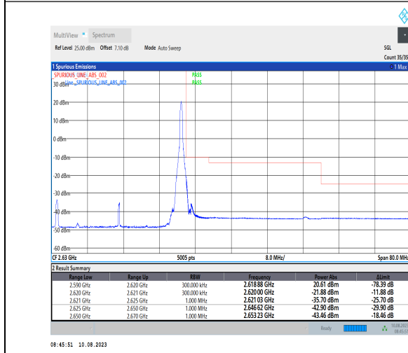
1-N38-PC3-30-30-H-5-CP-QPSK-Edge_1RB_Right-1@77-Ant1-1--PASS-see graph
