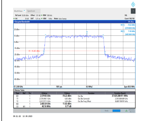
1-N38-PC3-30-40-M-8-CP-64QAM-Outer_Full-106 @0-Ant1-37.925-40.160-≤40-PASS
