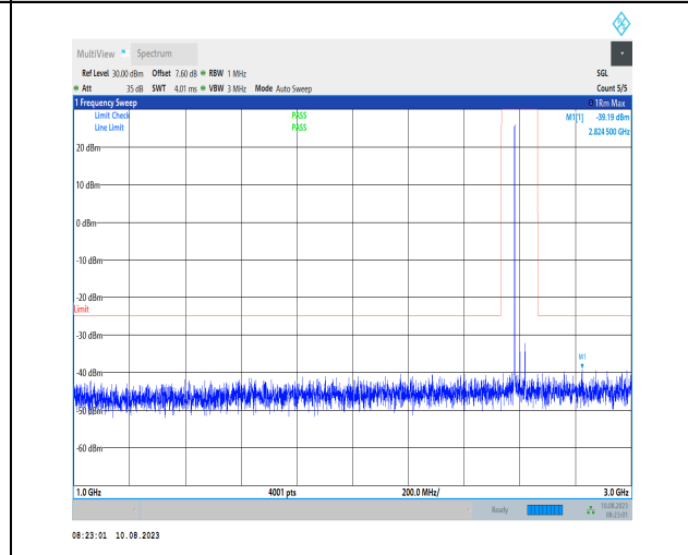
1-N38-PC3-30-40-H-1-N/A-DFT-PI2BPSK-Inner_1RB _Left-1@1-1000-3000-Ant1-2158.50--39.19--25-PAS S
