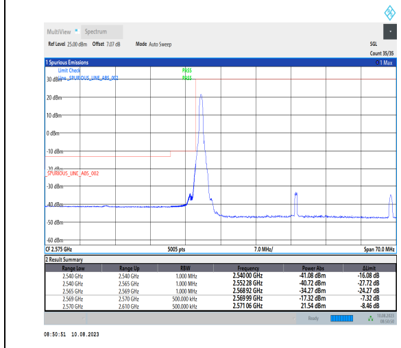
1-N38-PC3-30-40-L-4-CP-QPSK-Edge_1RB_Left-1@ 0-Ant1-1--PASS-see graph
