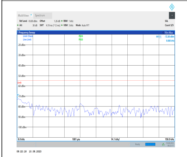
1-N38-PC3-30-40-M-1-N/A-DFT-PI2BPSK-Inner_1R B_Left-1@1-0.009-0.15-Ant1-0.01--72.30--55-PASS
