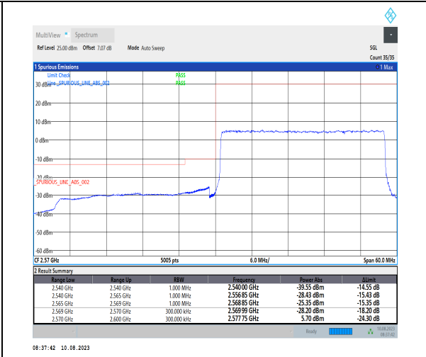
1-N38-PC3-30-30-L-3-DFT-PI2BPSK-Outer_Full-75@0-Ant1-1--PASS-see graph
