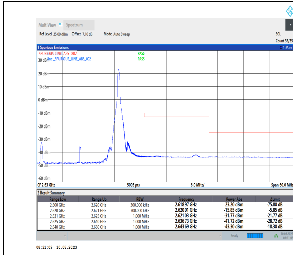
1-N38-PC3-30-20-H-2-DFT-PI2BPSK-Edge_1RB_Right-t-1@50-Ant1-1--PASS-see graph
