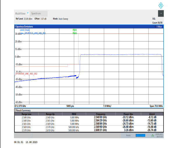
1-N38-PC3-30-40-L-6-CP-QPSK-Outer_Full-106@0 -Ant1-1--PASS-see graph
