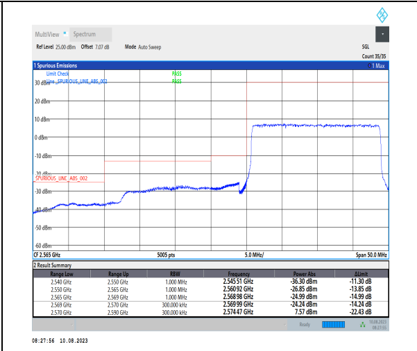
1-N38-PC3-30-20-L-3-DFT-PI2BPSK-Outer_Full-50@0-Ant1-1--PASS-see graph
