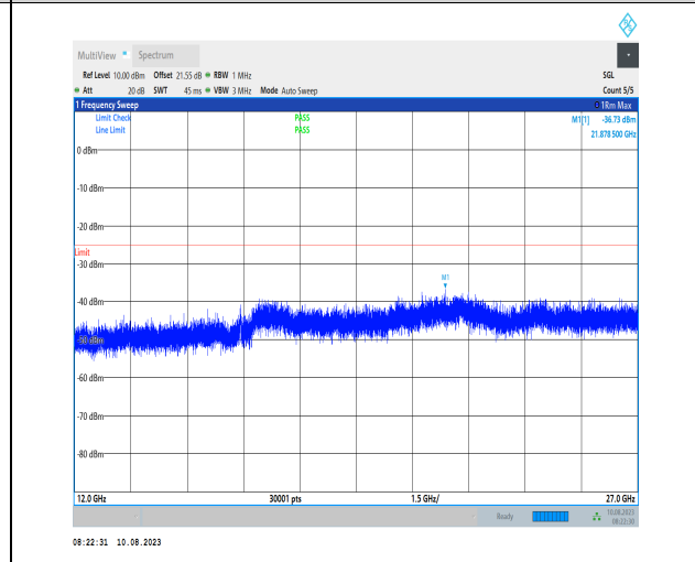
1-N38-PC3-30-40-M-1-N/A-DFT-PI2BPSK-Inner_1RB_Left-1@1-12000-27000-Ant1-22284.50--36.73--25-PASS
