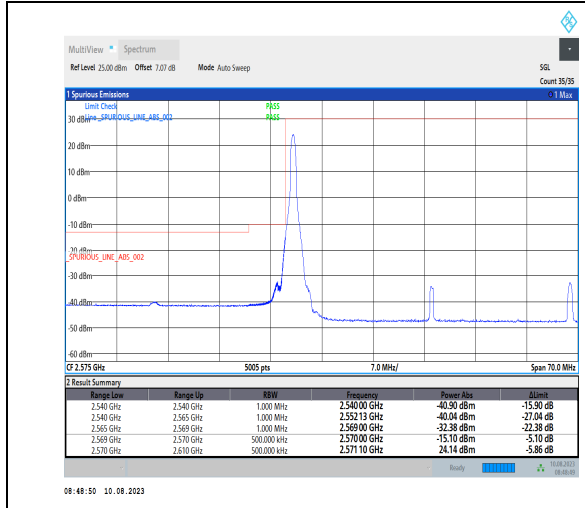
1-N38-PC3-30-40-L-1-DFT-PI2BPSK-Edge_1RB_Left -1@0-Ant1-1--PASS-see graph
