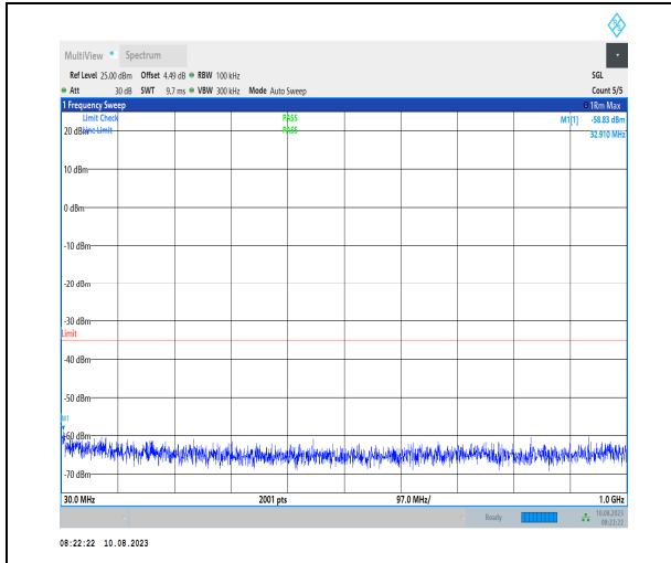
1-N38-PC3-30-40-M-1-N/A-DFT-PI2BPSK-Inner_1R_B_Left-1@1-30-1000-Ant1-32.91--58.83--35-PASS
