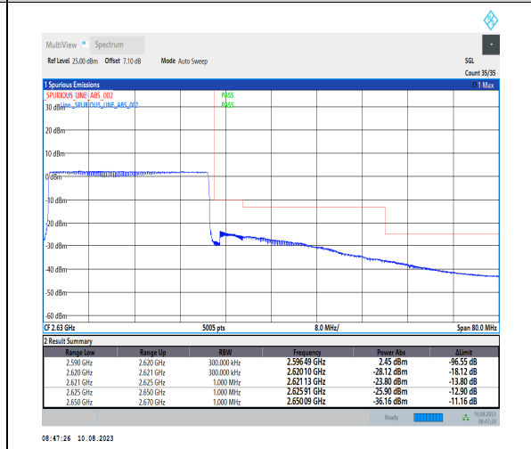
1-N38-PC3-30-30-H-6-CP-QPSK-Outer_Full-78@0-Ant1-1--PASS-see graph
