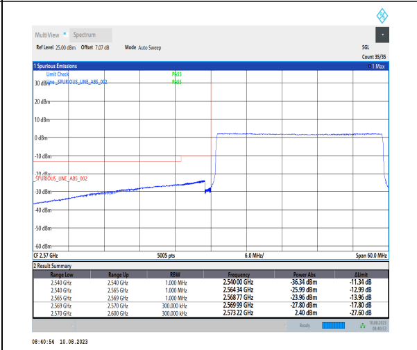
1-N38-PC3-30-30-L-6-CP-QPSK-Outer_Full-78@0-Ant1-1--PASS-see graph
