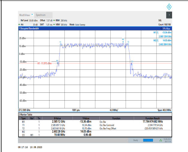
1-N38-PC3-30-20-M-2-DFT-PI2BPSK-Outer_Full-50 @0-Ant1-17.764-19.480-≤20-PASS
