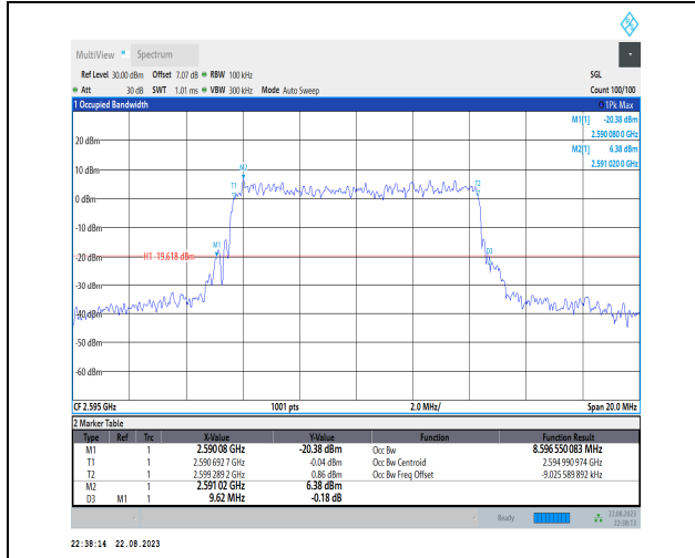
1-N38-PC3-30-10-M-9-CP-256QAM-Outer_Full-24@ 0-Ant1-8.597-9.620-≤10-PASS
