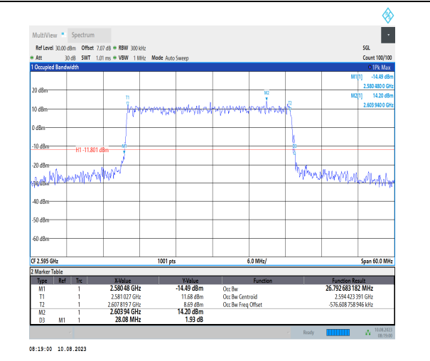
1-N38-PC3-30-30-M-3-DFT-16QAM-Outer_Full-75 @0-Ant1-26.793-28.080-≤30-PASS
