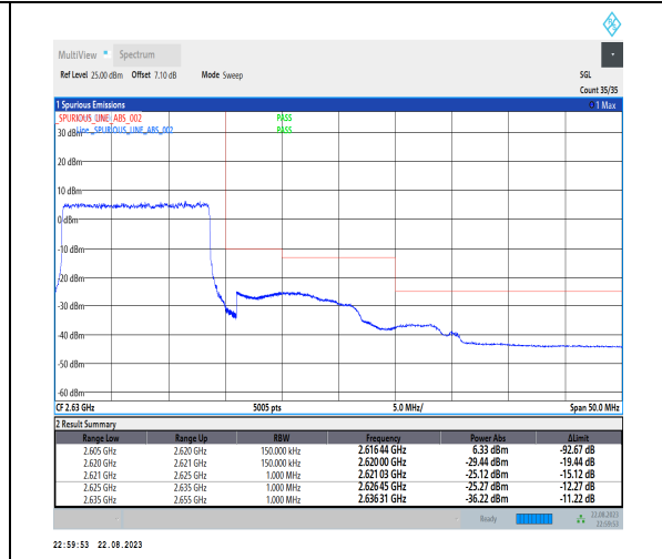
1-N38-PC3-30-15-H-3-DFT-PI2BPSK-Outer_Full-36@0-Ant1-1--PASS-see graph
