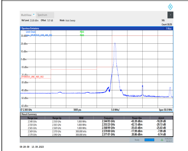
1-N38-PC3-30-20-L-4-CP-QPSK-Edge_1RB_Left-1@0-Ant1-1--PASS-see graph
