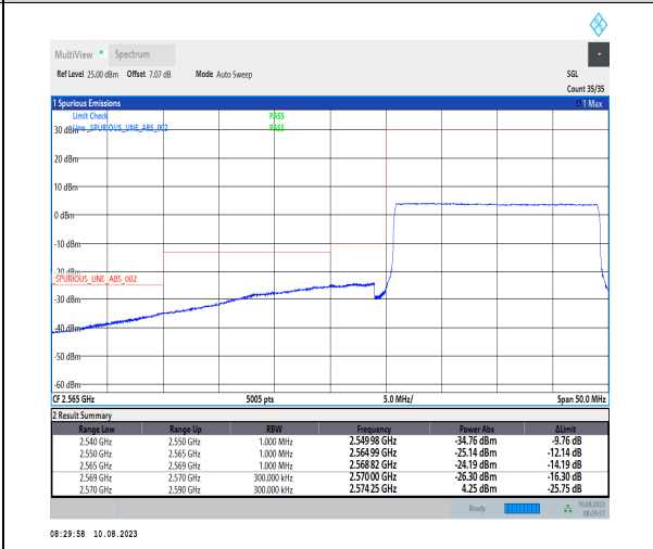
1-N38-PC3-30-20-L-6-CP-QPSK-Outer_Full-51@0-Ant1-1--PASS-see graph
