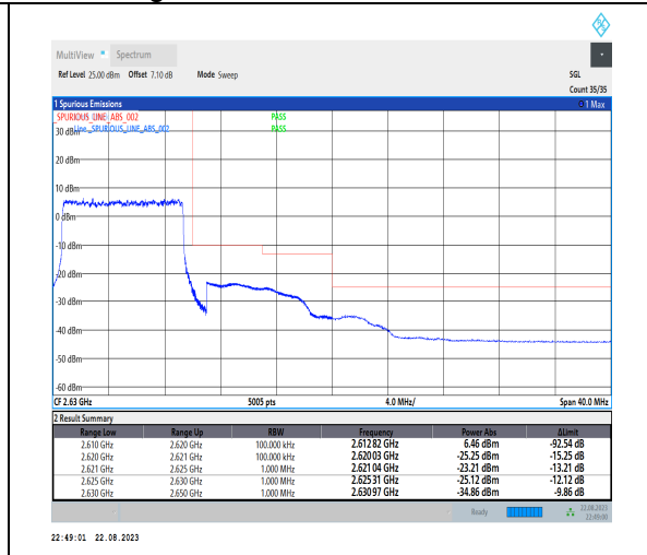
1-N38-PC3-30-10-H-3-DFT-PI2BPSK-Outer_Full-24@0-Ant1-1--PASS-see graph
