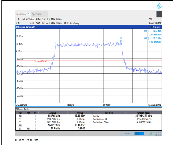
1-N38-PC3-30-15-M-8-CP-64QAM-Outer_Full-38@ 0-Ant1-13.571-14.700-≤15-PASS
