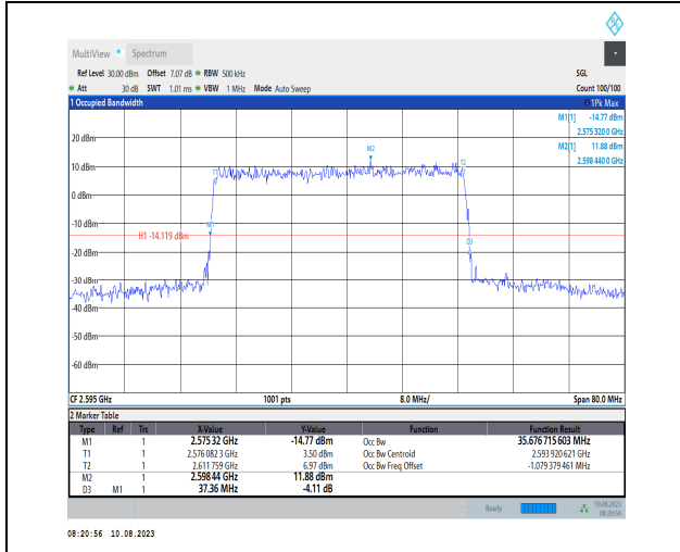
1-N38-PC3-30-40-M-5-DFT-256QAM-Outer_Full-100 @0-Ant1-35.677-37.360-≤40-PASS
