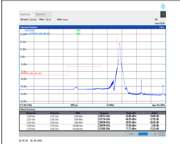
1-N38-PC3-30-15-L-4-CP-QPSK-Edge_1RB_Left-1@0-Ant1-1--PASS-see graph
