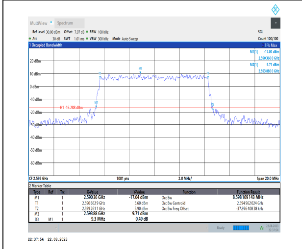
1-N38-PC3-30-10-M-7-CP-16QAM-Outer_Full-24@0 -Ant1-8.598-9.300-≤10-PASS
