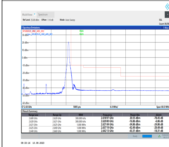
1-N38-PC3-30-20-H-5-CP-QPSK-Edge_1RB_Right-1@50-Ant1-1--PASS-see graph
