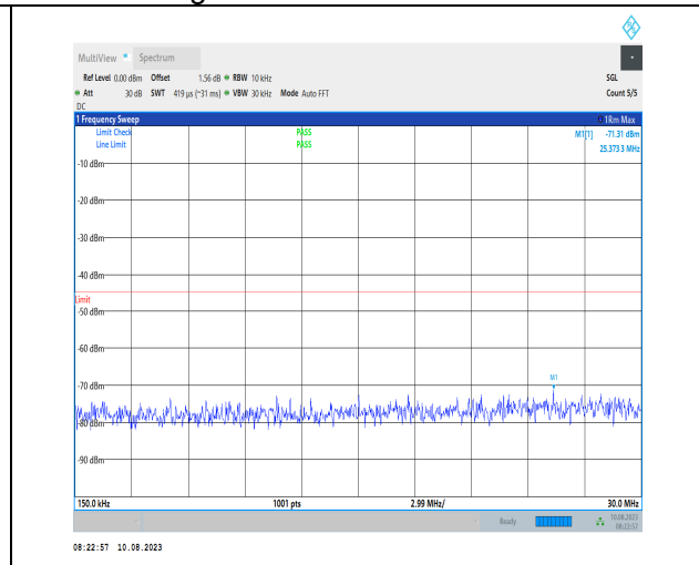
1-N38-PC3-30-40-H-1-N/A-DFT-PI2BPSK-Inner_1RB _Left-1@1-0.15-30-Ant1-30.00--71.31--45-PASS
