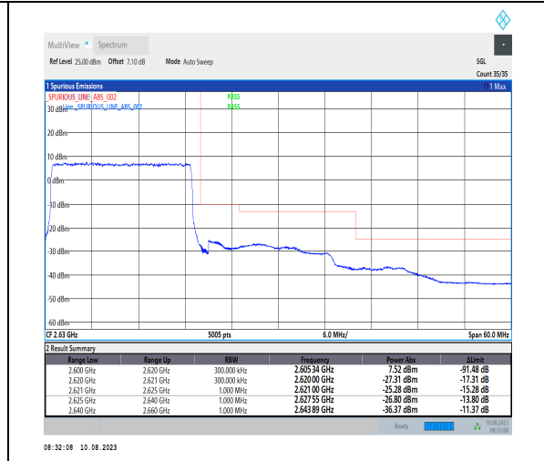
1-N38-PC3-30-20-H-3-DFT-PI2BPSK-Outer_Full-50@0-Ant1-1--PASS-see graph
