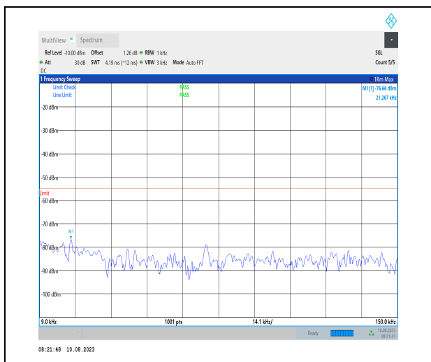
1-N38-PC3-30-40-L-1-N/A-DFT-PI2BPSK-Inner_1R B_Left-1@1-0.009-0.15-Ant1-0.01--76.66--55-PASS
