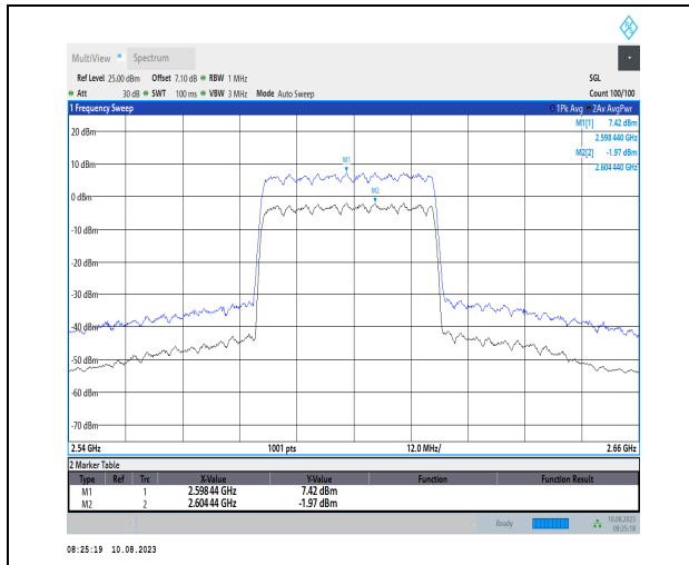
1-N38-PC3-30-40-H-1-DFT-256QAM-Outer_Full-100 @0-Ant1-9.39-100%-0.00-9.39-PASS-≤13
