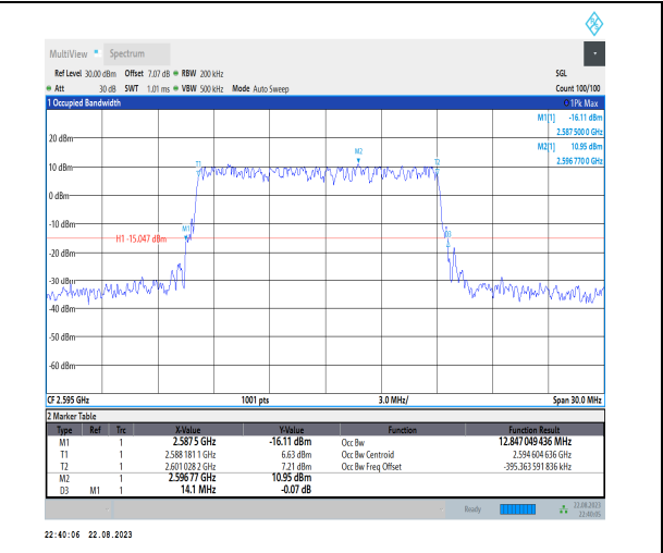
1-N38-PC3-30-15-M-5-DFT-256QAM-Outer_Full-36@ 0-Ant1-12.847-14.100-≤15-PASS
