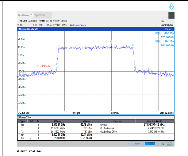
1-N38-PC3-30-40-M-6-CP-QPSK-Outer_Full-106@ 0-Ant1-37.859-39.680-≤40-PASS
