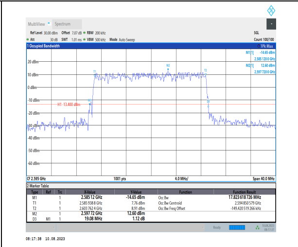
1-N38-PC3-30-20-M-4-DFT-64QAM-Outer_Full-50@ 0-Ant1-17.824-19.080-≤20-PASS
