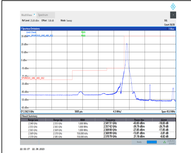
1-N38-PC3-30-15-L-1-DFT-PI2BPSK-Edge_1RB_Left-1@0-Ant1-1--PASS-see graph
