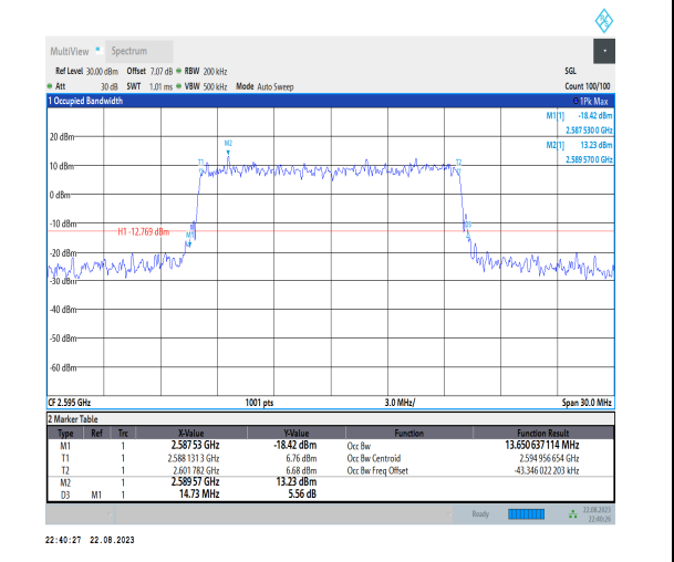
1-N38-PC3-30-15-M-7-CP-16QAM-Outer_Full-38@0- Ant1-13.651-14.730-≤15-PASS
