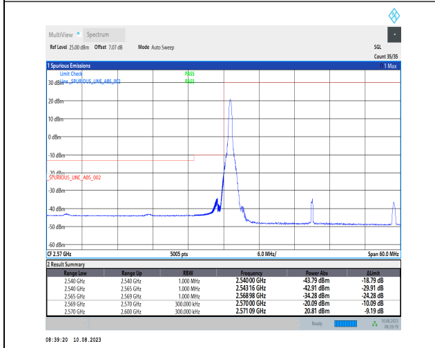
1-N38-PC3-30-30-L-4-CP-QPSK-Edge_1RB_Left-1@0-Ant1-1--PASS-see graph
