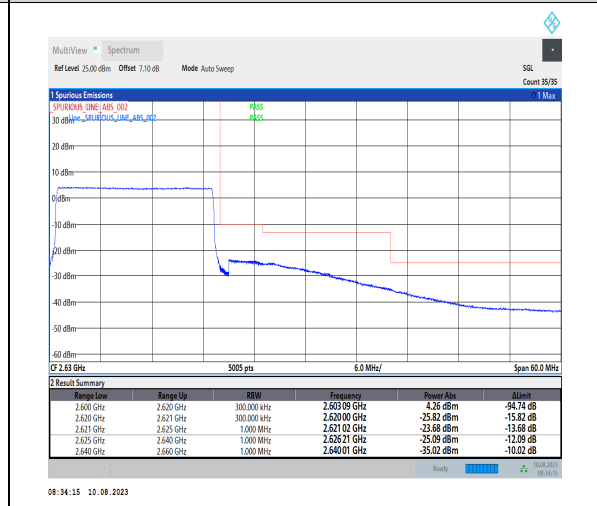
1-N38-PC3-30-20-H-6-CP-QPSK-Outer_Full-51@0-Ant1-1--PASS-see graph
