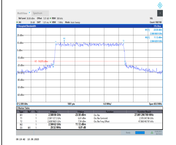
1-N38-PC3-30-30-M-8-CP-64QAM-Outer_Full-78@0-Ant1-27.841-29.520-<30-PASS
