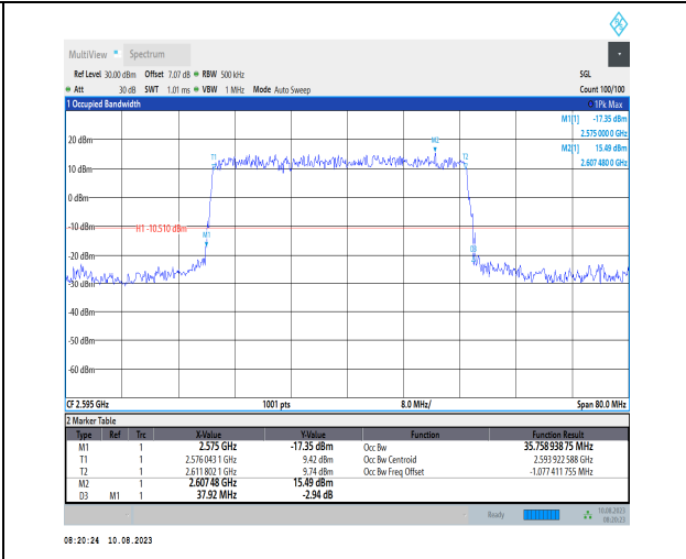
1-N38-PC3-30-40-M-2-DFT-PI2BPSK-Outer_Full-100 @0-Ant1-35.759-37.920-≤40-PASS
