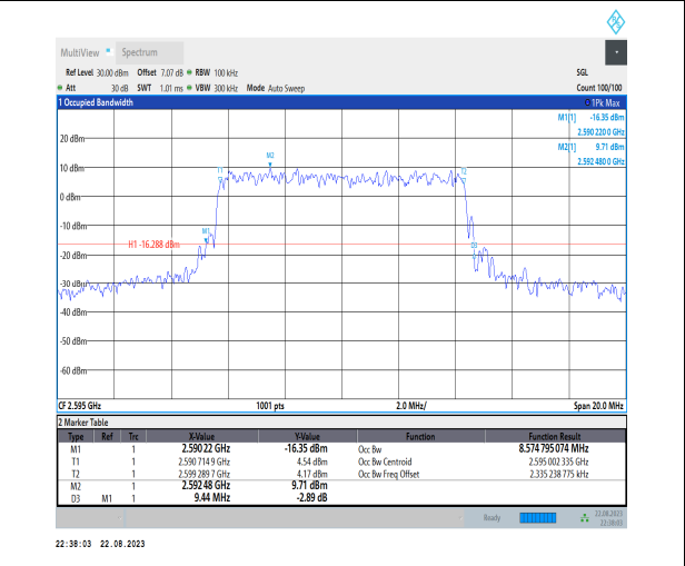
1-N38-PC3-30-10-M-8-CP-64QAM-Outer_Full-24@0 -Ant1-8.575-9.440-≤10-PASS
