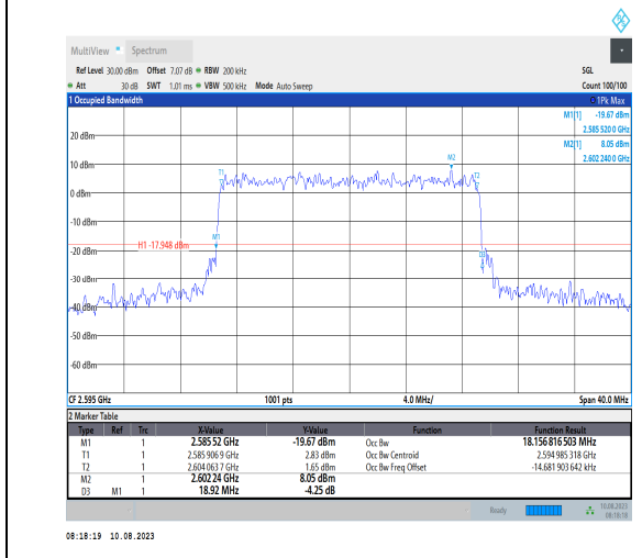
1-N38-PC3-30-20-M-9-CP-256QAM-Outer_Full-51@0-Ant1-18.157-18.920-≤20-PASS
