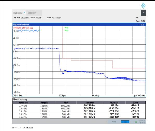
1-N38-PC3-30-30-H-3-DFT-PI2BPSK-Outer_Full-7@0-Ant1-1--PASS-see graph
