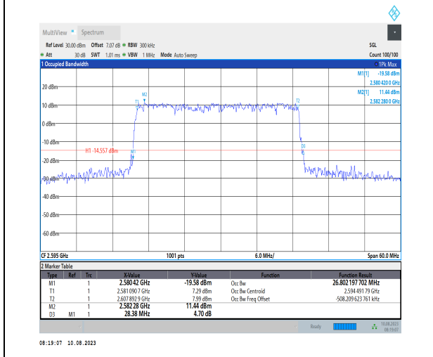
1-N38-PC3-30-30-M-4-DFT-64QAM-Outer_Full-75 @0-Ant1-26.802-28.380-≤30-PASS
