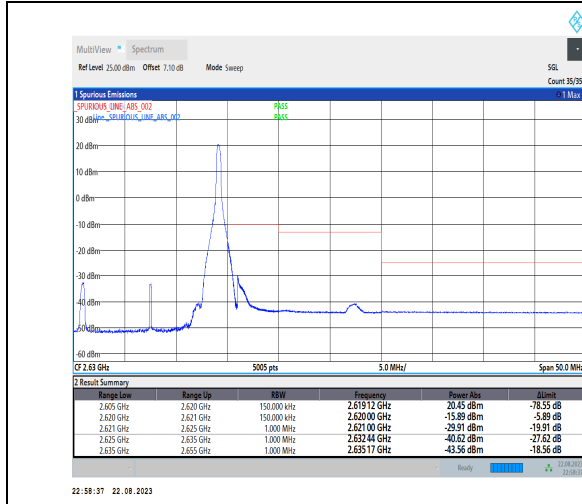
1-N38-PC3-30-15-H-2-DFT-PI2BPSK-Edge_1RB_Right-t1@37-Ant1-1--PASS-see graph
