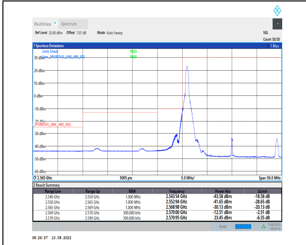
1-N38-PC3-30-20-L-1-DFT-PI2BPSK-Edge_1RB_Left-1@0-Ant1-1--PASS-see graph
