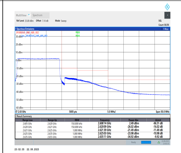
1-N38-PC3-30-15-H-6-CP-QPSK-Outer_Full-38@0-Ant1-1--PASS-see graph
