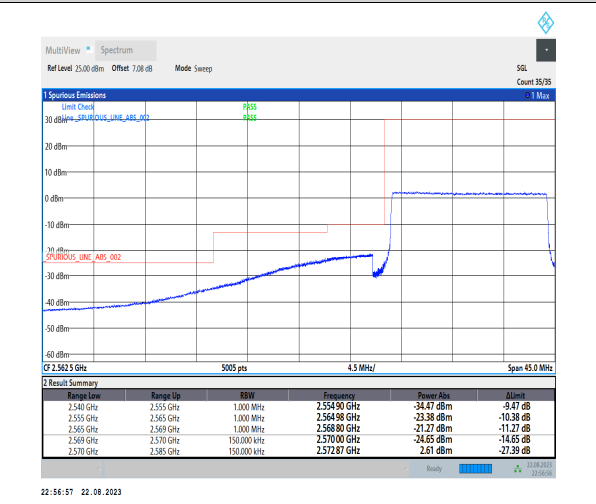
1-N38-PC3-30-15-L-6-CP-QPSK-Outer_Full-38@0-Ant1-1--PASS-see graph
