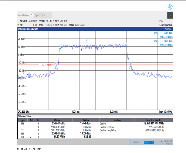
1-N38-PC3-30-15-M-3-DFT-16QAM-Outer_Full-36 @0-Ant1-12.87-14.370-≤15-PASS
