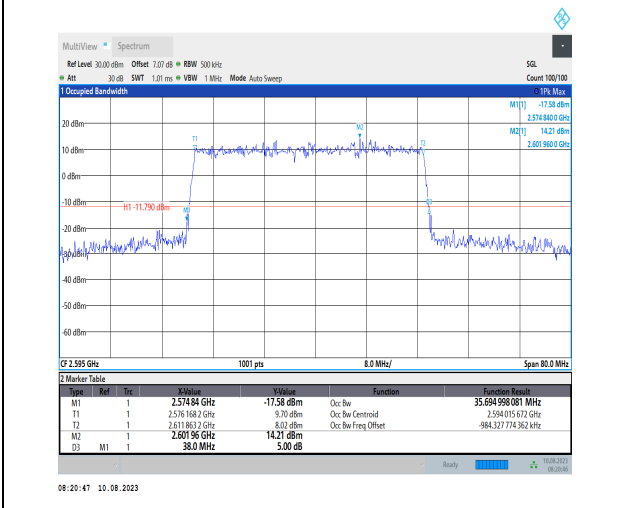
1-N38-PC3-30-40-M-4-DFT-64QAM-Outer_Full-100 @0-Ant1-35.695-38.000-≤40-PASS
