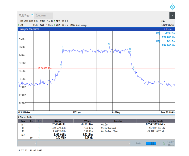
1-N38-PC3-30-10-M-5-DFT-256QAM-Outer_Full-24 @0-Ant1-8.594-9.220-≤10-PASS
