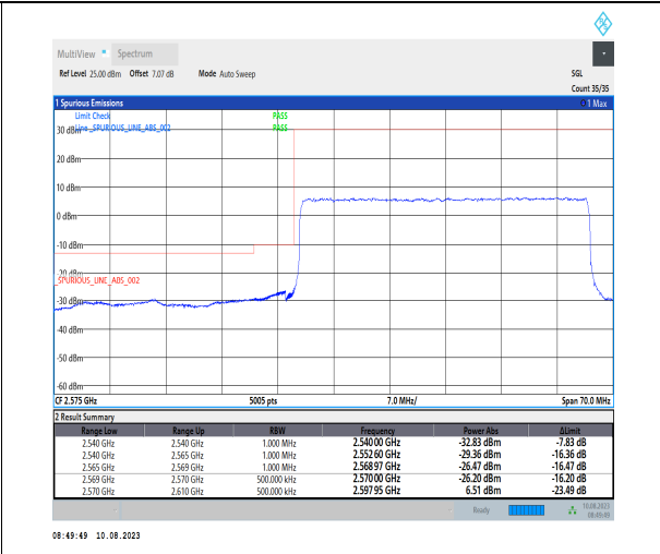
1-N38-PC3-30-40-L-3-DFT-PI2BPSK-Outer_Full-10 0@0-Ant1-1--PASS-see graph
