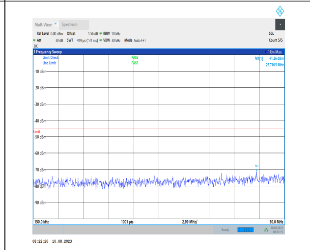
1-N38-PC3-30-40-M-1-N/A-DFT-PI2BPSK-Inner_1RB _Left-1@1-0.15-30-Ant1-20.00--71.26--45-PASS
