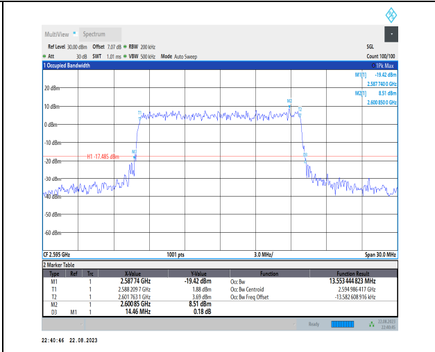
1-N38-PC3-30-15-M-9-CP-256QAM-Outer_Full-38@ 0-Ant1-13.553-14.460-≤15-PASS
