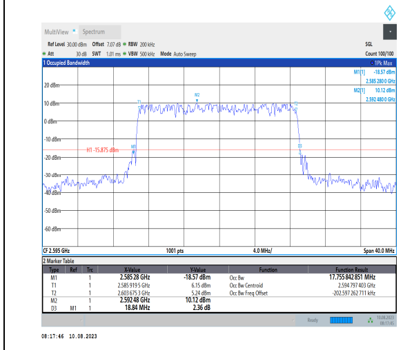
1-N38-PC3-30-20-M-5-DFT-256QAM-Outer_Full-50 @0-Ant1-17.756-18.840-≤20-PASS
