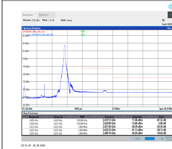
1-N38-PC3-30-15-H-5-CP-QPSK-Edge_1RB_Right-1@37-Ant1-1--PASS-see graph
