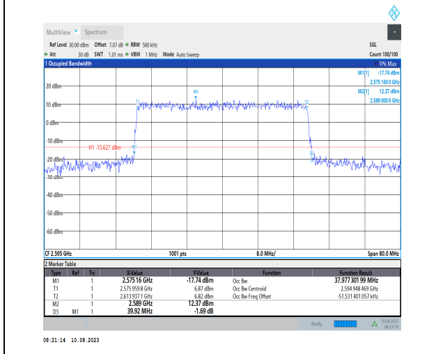
1-N38-PC3-30-40-M-7-CP-16QAM-Outer_Full-106@ 0-Ant1-37.977-39.920-≤40-PASS
