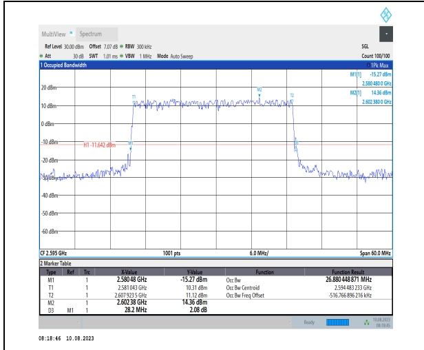
1-N38-PC3-30-30-M-2-DFT-PI2BPSK-Outer_Full-75 @0-Ant1-26.88-28.200-≤30-PASS
