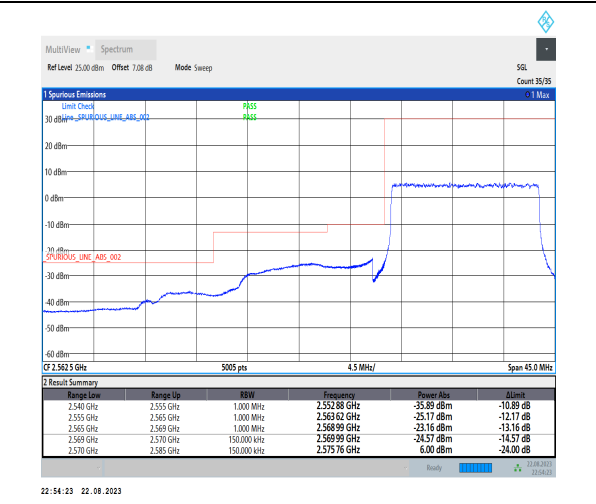
1-N38-PC3-30-15-L-3-DFT-PI2BPSK-Outer_Full-36@0-Ant1-1--PASS-see graph
