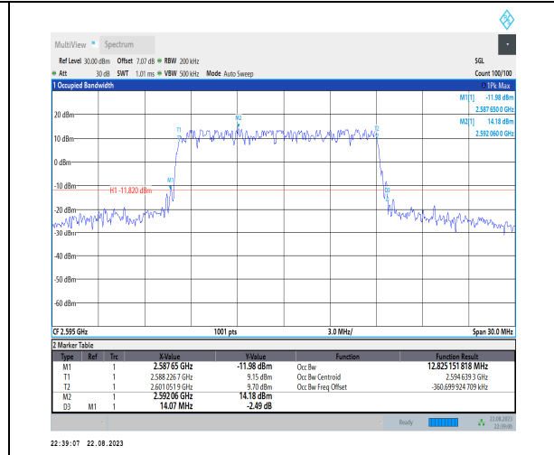
1-N38-PC3-30-15-M-1-DFT-QPSK-Outer_Full-36@ 0-Ant1-12.825-14.070-≤15-PASS
