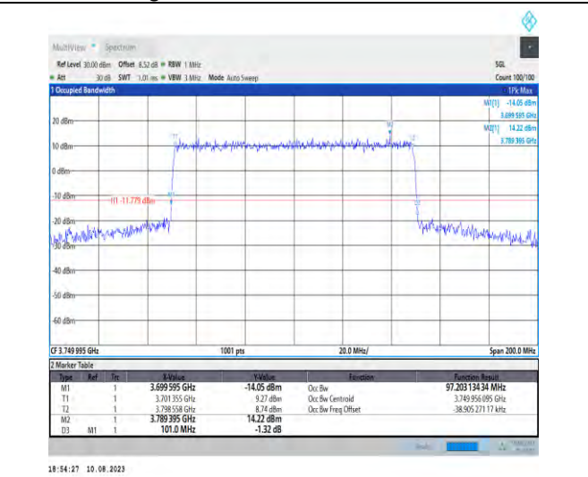
1-N78-3700-3800-PC2-30-100-M-8-CP-64QAM-Out er_Full-273@0-Ant1-97.203-101.000-≤100-PASS
