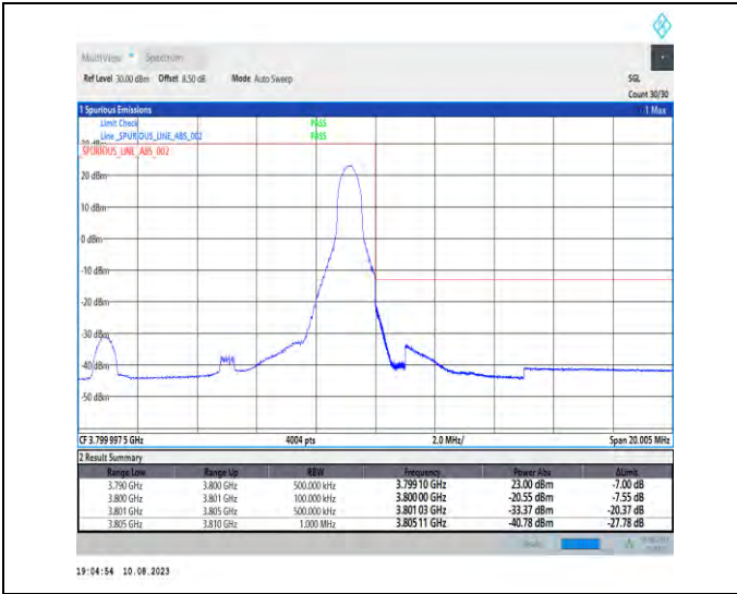
1-N78-3700-3800-PC2-30-10-H-2-DFT-PI2BPSK-Edge_1RB_Right-1@23-Ant1-1--PASS-see graph
