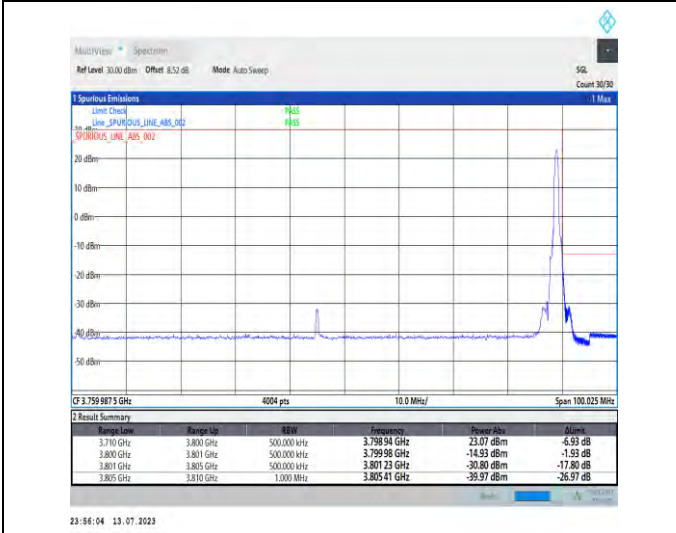
1-N78-3700-3800-PC2-30-90-H-5-CP-QPSK-Edge_1RB_Right-1@244-Ant1-1--PASS-see graph
