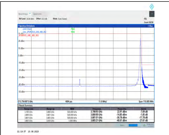
1-N78-3700-3800-PC2-30-100-H-2-DFT-PI2BPSK-Edge_1RB_Right-1@272-Ant1-1--PASS-see graph
