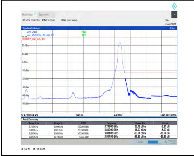
1-N78-3700-3800-PC2-30-20-H-5-CP-QPSK-Edge_1RB_Right-1@50-Ant1-1--PASS-see graph
