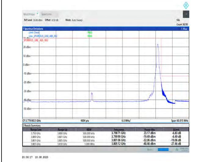
1-N78-3700-3800-PC2-30-50-H-5-CP-QPSK-Edge_1RB_Right-1@132-Ant1-1--PASS-see graph
