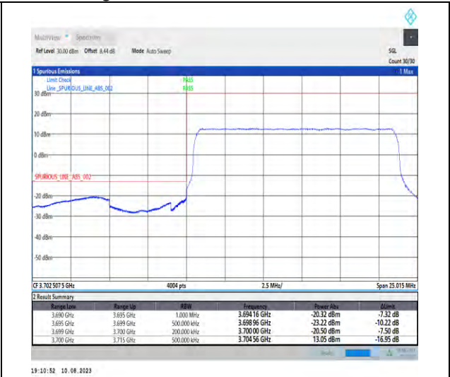
1-N78-3700-3800-PC2-30-15-L-3-DFT-PI2BPSK-Outer_Full-36@0-Ant1-1--PASS-see graph
