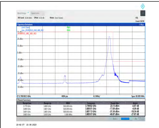
1-N78-3700-3800-PC2-30-30-H-2-DFT-PI2BPSK-Edge_1RB_Right-1@77-Ant1-1--PASS-see graph
