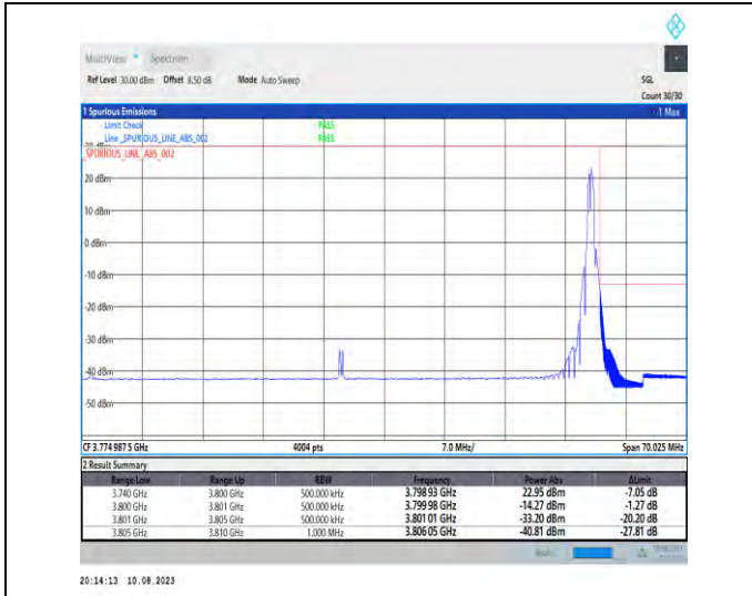
1-N78-3700-3800-PC2-30-60-H-2-DFT-PI2BPSK-Edge_1RB_Right-1@161-Ant1-1--PASS-see graph
