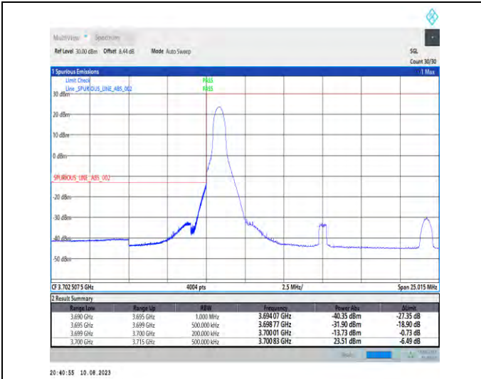
1-N78-3700-3800-PC2-30-15-L-1-DFT-PI2BPSK-Edge_1RB_Left-1@0-Ant1-1--PASS-see graph
