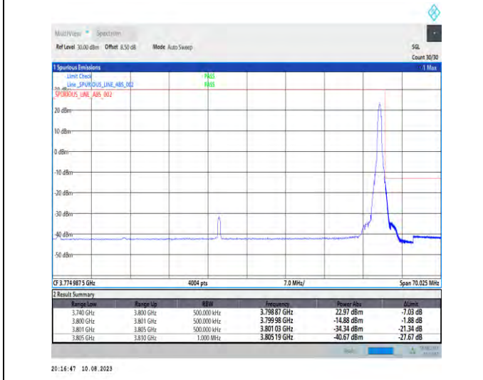
1-N78-3700-3800-PC2-30-60-H-5-CP-QPSK-Edge_1RB_Right-1@161-Ant1-1--PASS-see graph
