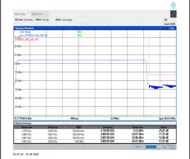
1-N78-3700-3800-PC2-30-50-H-6-CP-QPSK-Outer_Full-133@0-Ant1-1--PASS-see graph
