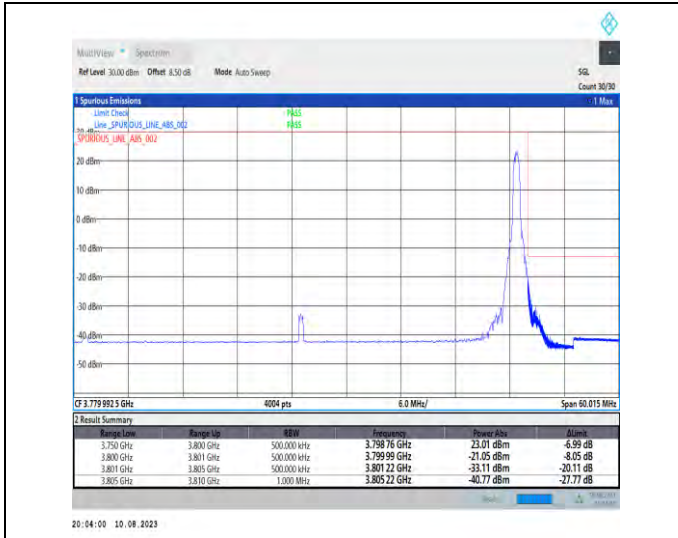
1-N78-3700-3800-PC2-30-50-H-2-DFT-PI2BPSK-Edge_1RB_Right-1@132-Ant1-1--PASS-see graph
