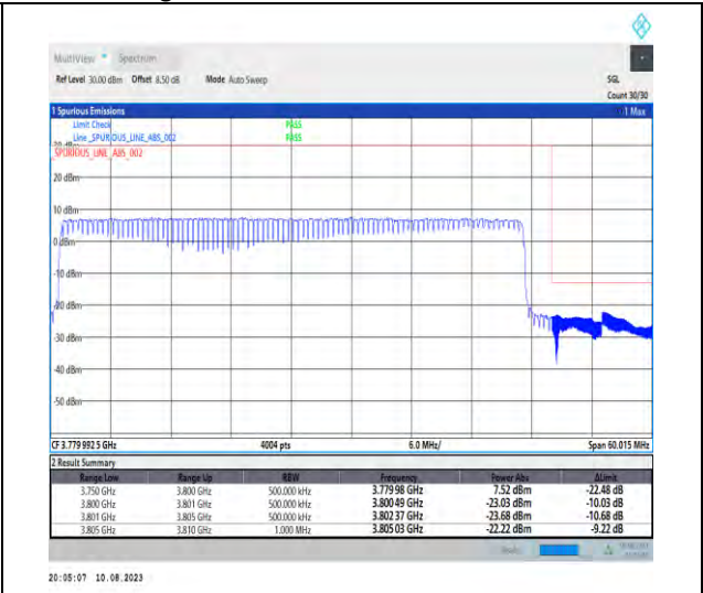
1-N78-3700-3800-PC2-30-50-H-3-DFT-PI2BPSK-Outer_Full-128@0-Ant1-1--PASS-see graph
