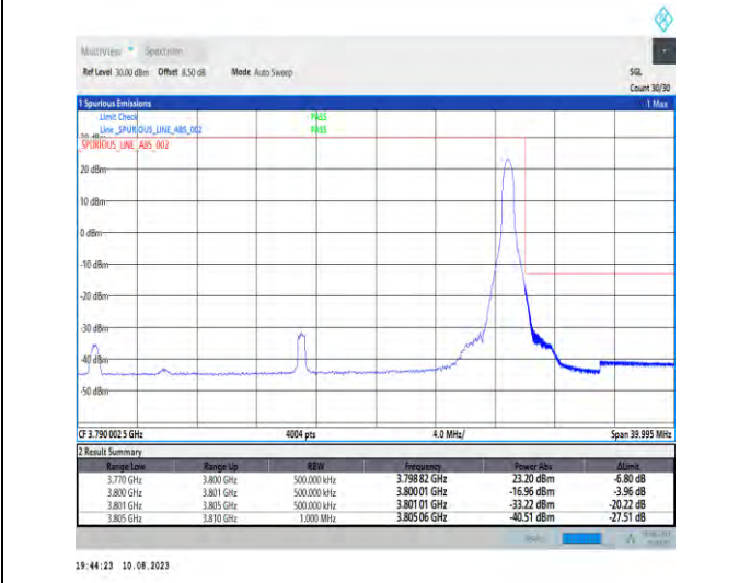
1-N78-3700-3800-PC2-30-30-H-5-CP-QPSK-Edge_1RB_Right-1@77-Ant1-1--PASS-see graph
