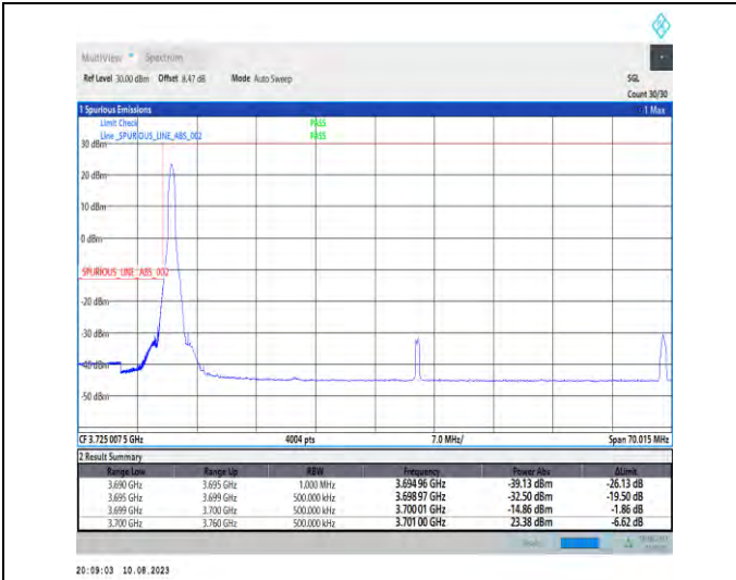
1-N78-3700-3800-PC2-30-60-L-1-DFT-PI2BPSK-Edge_1RB_Left-1@0-Ant1-1--PASS-see graph
