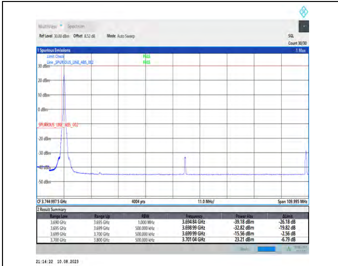
1-N78-3700-3800-PC2-30-100-L-1-DFT-PI2BPSK-Edge_e_1RB_Left-1@0-Ant1-1--PASS-see graph
