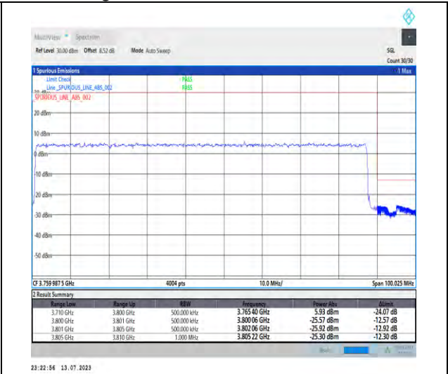
1-N78-3700-3800-PC2-30-90-H-3-DFT-PI2BPSK-Outer_Full-240@0-Ant1-1--PASS-see graph
