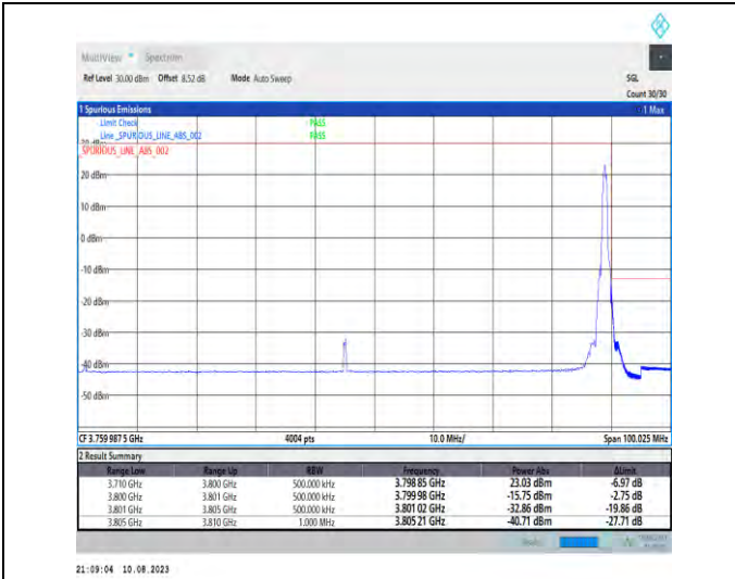
1-N78-3700-3800-PC2-30-90-H-2-DFT-PI2BPSK-Edge_1RB_Right-1@244-Ant1-1--PASS-see graph
