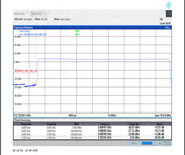
1-N78-3700-3800-PC2-30-60-L-6-CP-QPSK-Outer_Full-162@0-Ant1-1--PASS-see graph
