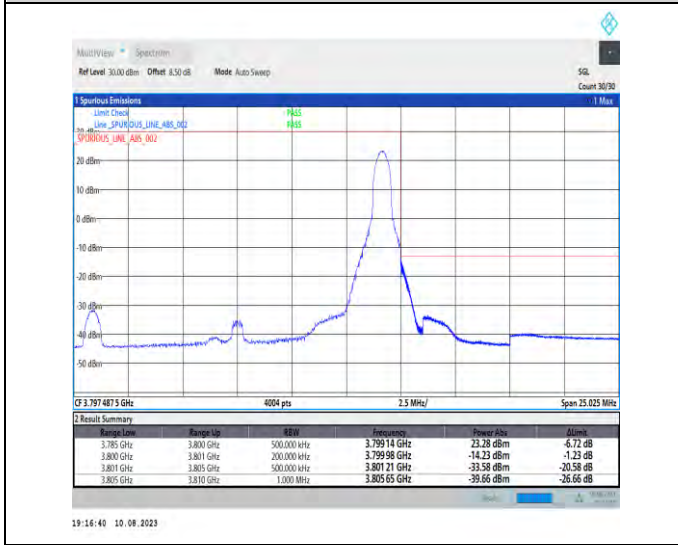
1-N78-3700-3800-PC2-30-15-H-5-CP-QPSK-Edge_1RB_Right-1@37-Ant1-1--PASS-see graph
