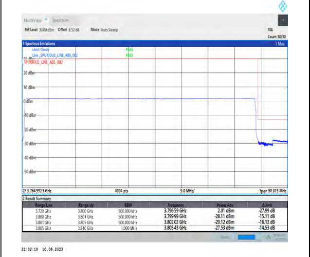
1-N78-3700-3800-PC2-30-80-H-6-CP-QPSK-Outer_Full-217@0-Ant1-1--PASS-see graph
