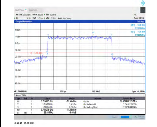
1-N78-3700-3800-PC2-30-70-M-8-CP-64QAM-Outer_Full-189@0-Ant1-67.478-69.440-≤70-PASS
