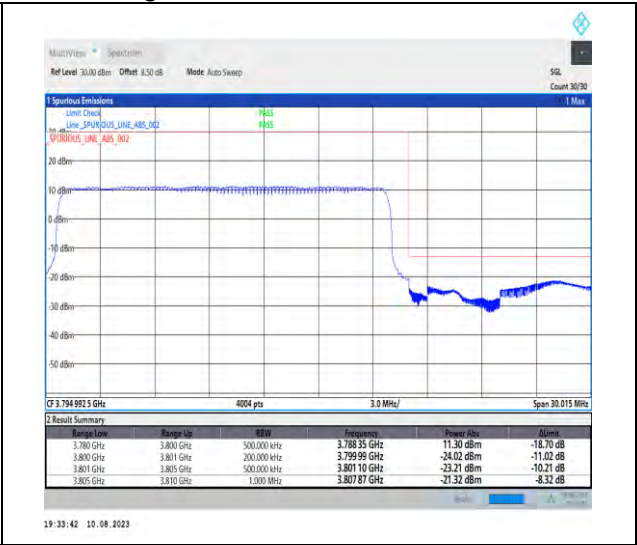
1-N78-3700-3800-PC2-30-20-H-3-DFT-PI2BPSK-Outer_Full-50@0-Ant1-1--PASS-see graph
