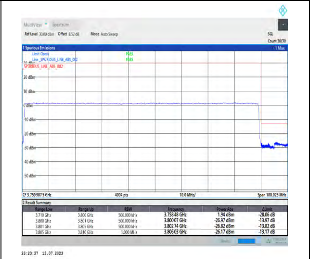
1-N78-3700-3800-PC2-30-90-H-6-CP-QPSK-Outer_Full-245@0-Ant1-1--PASS-see graph
