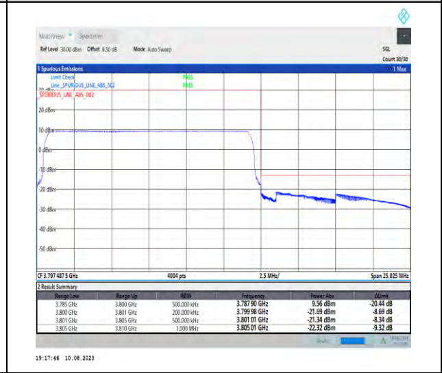
1-N78-3700-3800-PC2-30-15-H-6-CP-QPSK-Outer_Full-38@0-Ant1-1--PASS-see graph
