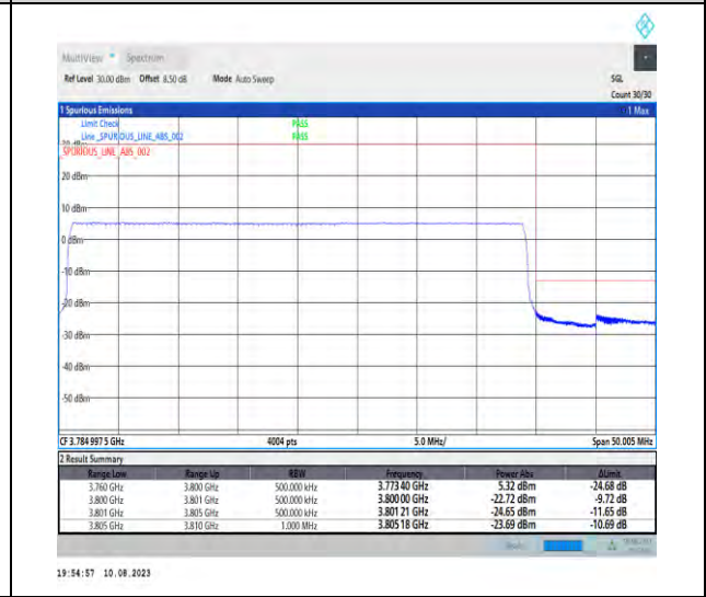
1-N78-3700-3800-PC2-30-40-H-6-CP-QPSK-Outer_Full-106@0-Ant1-1--PASS-see graph
