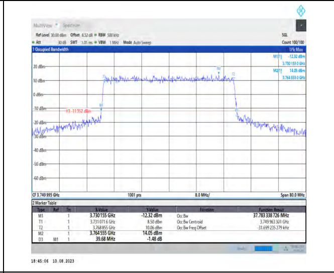
1-N78-3700-3800-PC2-30-40-M-8-CP-64QAM-Outer _Full-106@0-Ant1-37.783-39.680-≤40-PASS
