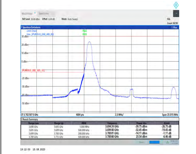
1-N78-3700-3800-PC2-30-15-L-4-CP-QPSK-Edge_1RB_Left-1@0-Ant1-1--PASS-see graph
