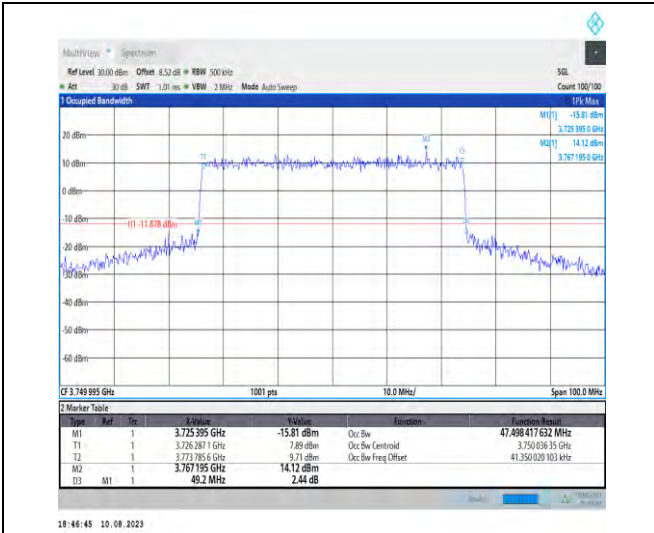
1-N78-3700-3800-PC2-30-50-M-8-CP-64QAM-Outer_Full-133@0-Ant1-47.498-49.200-≤50-PASS
