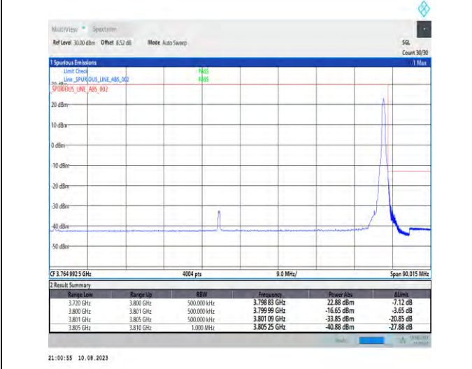
1-N78-3700-3800-PC2-30-80-H-5-CP-QPSK-Edge_1RB_Right-1@216-Ant1-1--PASS-see graph
