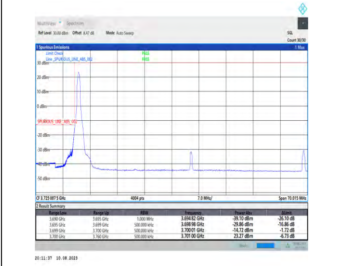
1-N78-3700-3800-PC2-30-60-L-4-CP-QPSK-Edge_1RB_Left-1@0-Ant1-1--PASS-see graph
