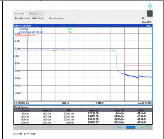
1-N78-3700-3800-PC2-30-40-H-3-DFT-PI2BPSK-Outer_Full-100@0-Ant1-1--PASS-see graph
