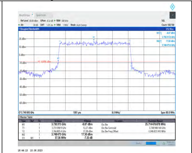
1-N78-3700-3800-PC2-30-40-M-2-DFT-PI2BPSK-Outer_Full-100@0-Ant1-35.714-37.360-≤40-PASS
