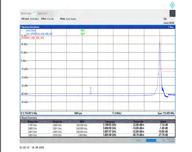
1-N78-3700-3800-PC2-30-100-H-5-CP-QPSK-Edge_1RB_Right-1@272-Ant1-1--PASS-see graph
