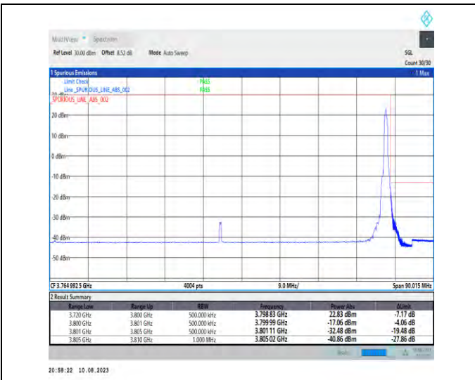
1-N78-3700-3800-PC2-30-80-H-2-DFT-PI2BPSK-Edge_1RB_Right-1@216-Ant1-1--PASS-see graph
