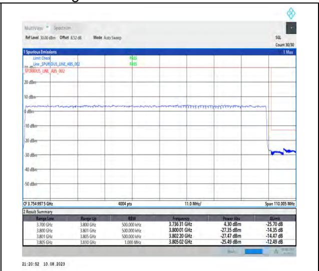
1-N78-3700-3800-PC2-30-100-H-3-DFT-PI2BPSK-Outer_Full-270@0-Ant1-1--PASS-see graph
