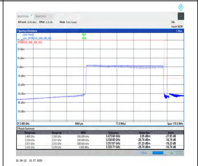
1-N78-3450-3550-PC2-30-80-H-6-CP-QPSK-Outer_Full-217@0-Ant1-1--PASS-see graph
