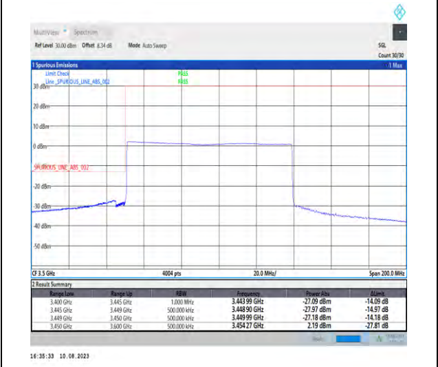
1-N78-3450-3550-PC2-30-90-L-6-CP-QPSK-Outer_Full-245@0-Ant1-1--PASS-see graph
