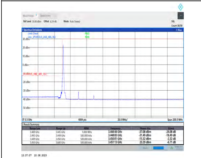
1-N78-3450-3550-PC2-30-40-L-4-CP-QPSK-Edge_1RB_Left-1@0-Ant1-1--PASS-see graph
