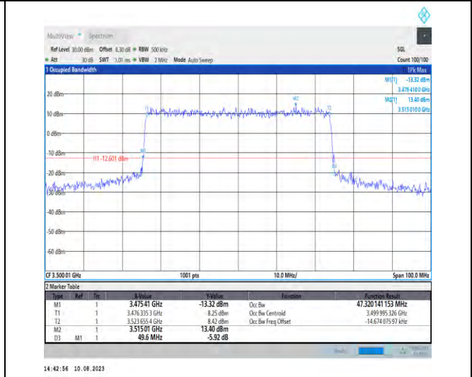
1-N78-3450-3550-PC2-30-50-M-7-CP-16QAM-Outer_Full-133@0-Ant1-47.32-49.600-≤50-PASS
