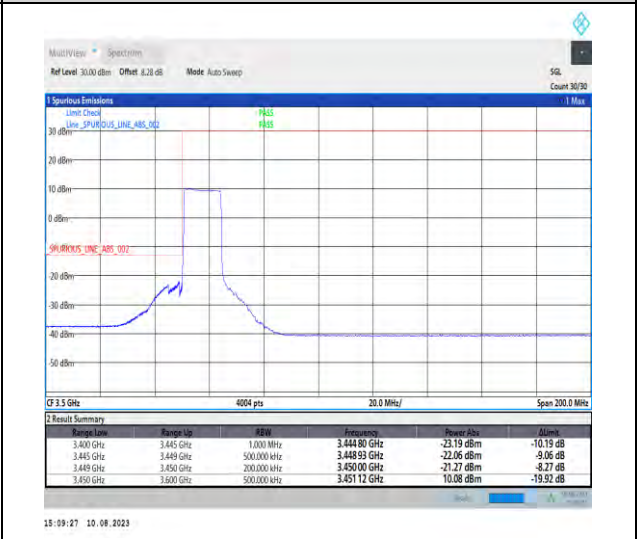
1-N78-3450-3550-PC2-30-15-L-6-CP-QPSK-Outer_Full-38@0-Ant1-1--PASS-see graph
