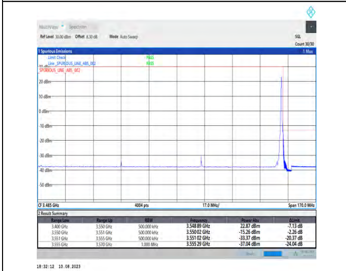
1-N78-3450-3550-PC2-30-100-H-5-CP-QPSK-Edge_1_RB_Right-1@272-Ant1-1--PASS-see graph
