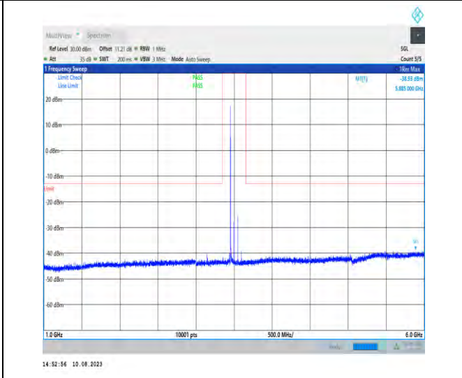
1-N78-3450-3550-PC2-30-100-H-1-N/A-DFT-PI2BPS K-Inner_1RB_Left-1@1-1000-6000-Ant1-5908.00--38 .93--13-PASS
