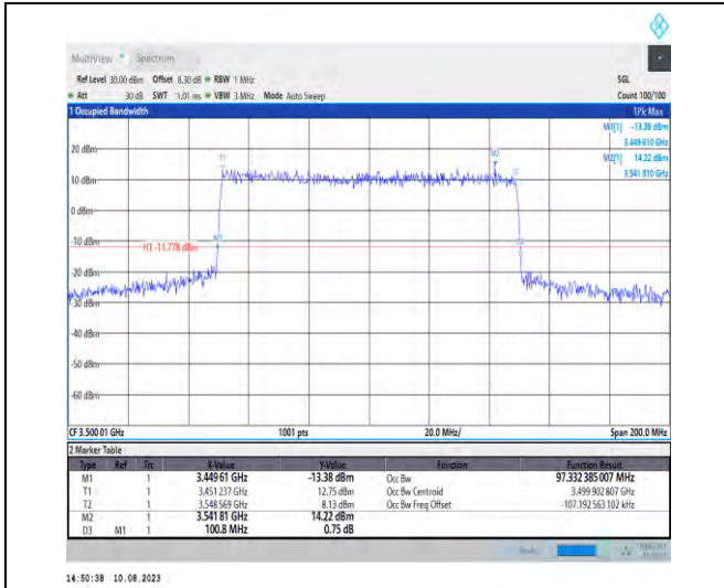
1-N78-3450-3550-PC2-30-100-M-7-CP-16QAM-Outer_Full-273@0-Ant1-97.332-100.800-≤100-PASS
