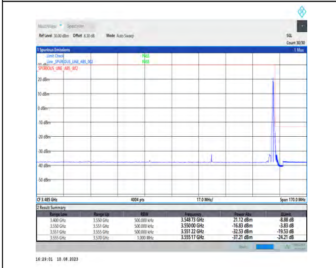
1-N78-3450-3550-PC2-30-80-H-5-CP-QPSK-Edge_1RB_Right-1@216-Ant1-1--PASS-see graph
