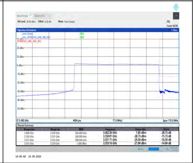
1-N78-3450-3550-PC2-30-90-H-6-CP-QPSK-Outer_Full-245@0-Ant1-1--PASS-see graph
