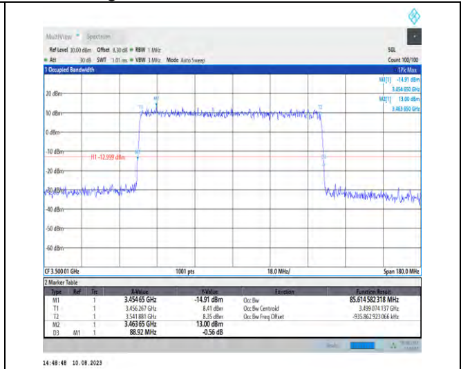
1-N78-3450-3550-PC2-30-90-M-5-DFT-256QAM-Outer_Full-240@0-Ant1-85.615-88.920-≤90-PASS
