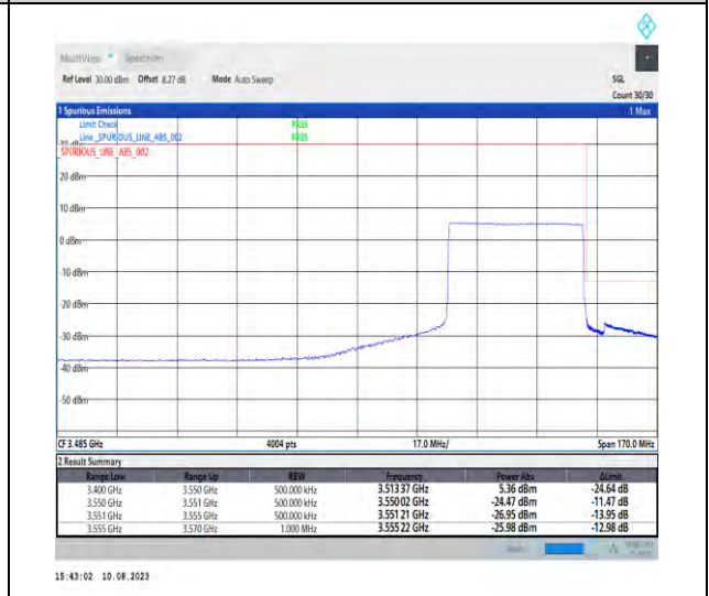
1-N78-3450-3550-PC2-30-40-H-6-CP-QPSK-Outer_Full-106@0-Ant1-1--PASS-see graph
