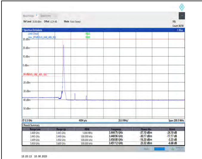
1-N78-3450-3550-PC2-30-30-L-1-DFT-PI2BPSK-Edge_1RB_Left-1@0-Ant1-1--PASS-see graph
