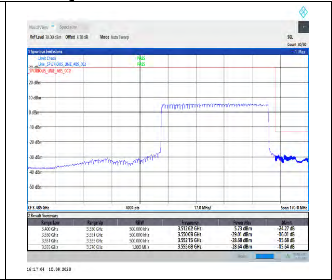
1-N78-3450-3550-PC2-30-70-H-3-DFT-PI2BPSK-Outer_Full-180@0-Ant1-1--PASS-see graph
