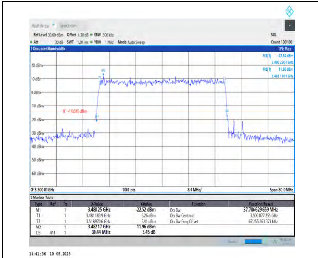
1-N78-3450-3550-PC2-30-40-M-9-CP-256QAM-Out er_Full-106@0-Ant1-37.787-39.440-≤40-PASS
