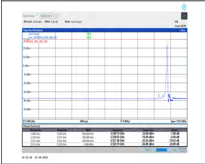
1-N78-3450-3550-PC2-30-10-H-5-CP-QPSK-Edge_1RB_Right-1@23-Ant1-1--PASS-see graph
