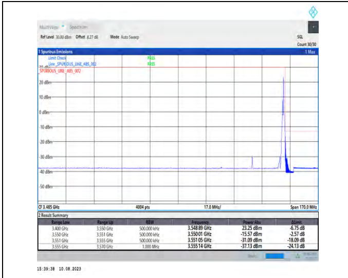
1-N78-3450-3550-PC2-30-40-H-2-DFT-PI2BPSK-Edge_1RB_Right-1@105-Ant1-1--PASS-see graph
