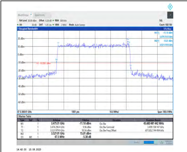
1-N78-3450-3550-PC2-30-50-M-4-DFT-64QAM-Outer_Full-128@0-Ant1-45.683-47.500-≤50-PASS
