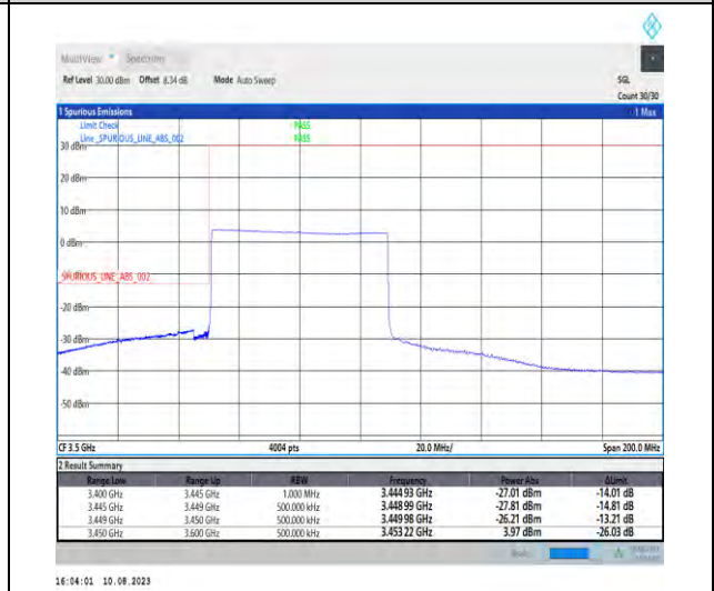
1-N78-3450-3550-PC2-30-60-L-6-CP-QPSK-Outer_Full-162@0-Ant1-1--PASS-see graph
