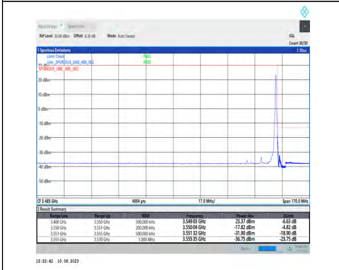
1-N78-3450-3550-PC2-30-20-H-5-CP-QPSK-Edge_1RB_Right-1@50-Ant1-1--PASS-see graph
