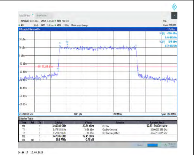
1-N78-3450-3550-PC2-30-60-M-6-CP-QPSK-Outer_Full-162@0-Ant1-57.631-60.600-≤60-PASS
