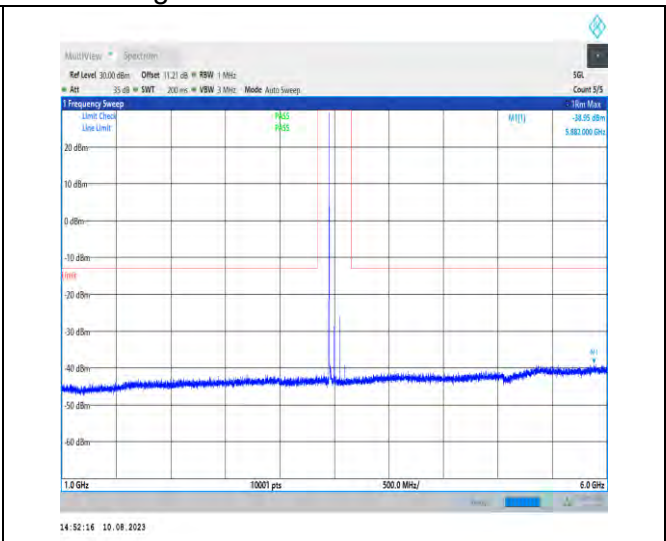
1-N78-3450-3550-PC2-30-100-M-1-N/A-DFT-PI2BPS K-Inner_1RB_Left-1@1-1000-6000-Ant1-5962.00--38.95--13-PASS
