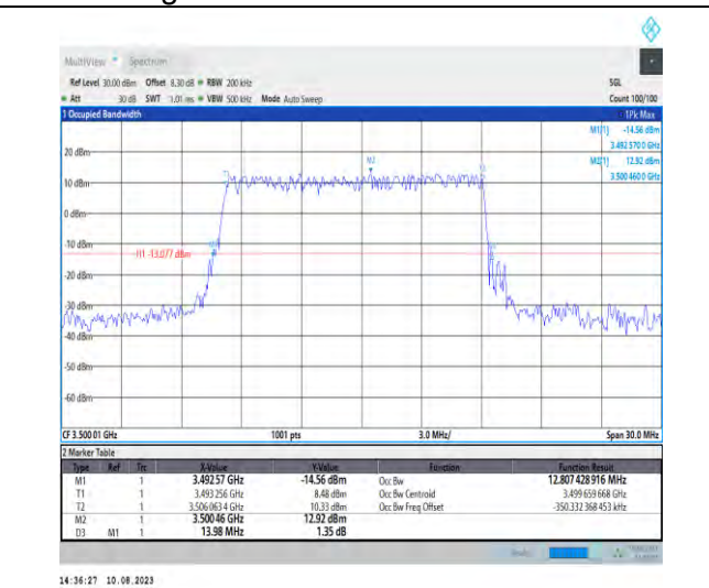
1-N78-3450-3550-PC2-30-15-M-5-DFT-256QAM-Outer_Full-36@0-Ant1-12.807-13.980-≤15-PASS
