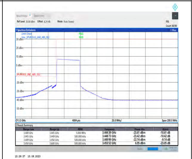
1-N78-3450-3550-PC2-30-30-L-6-CP-QPSK-Outer_Full-78@0-Ant1-1--PASS-see graph
