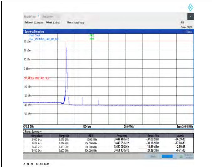
1-N78-3450-3550-PC2-30-40-L-1-DFT-PI2BPSK-Edge_1RB_Left-1@0-Ant1-1--PASS-see graph
