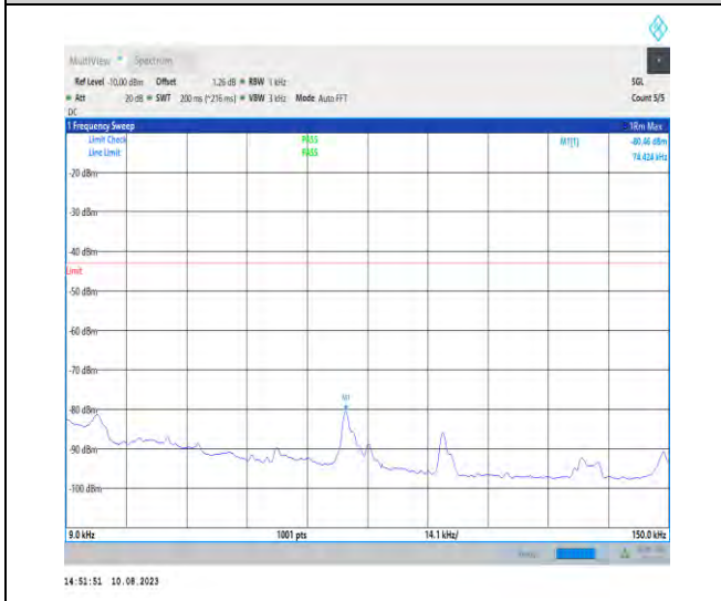
1-N78-3450-3550-PC2-30-100-M-1-N/A-DFT-PI2BP SK-Inner_1RB_Left-1@1-0.009-0.15-Ant1-0.07--80. 46--43-PASS
