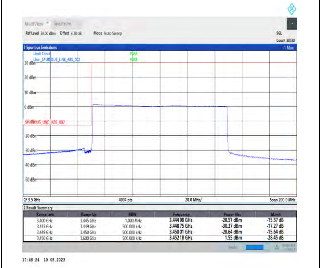
1-N78-3450-3550-PC2-30-100-L-6-CP-QPSK-Outer_Full-273@0-Ant1-1--PASS-see graph
