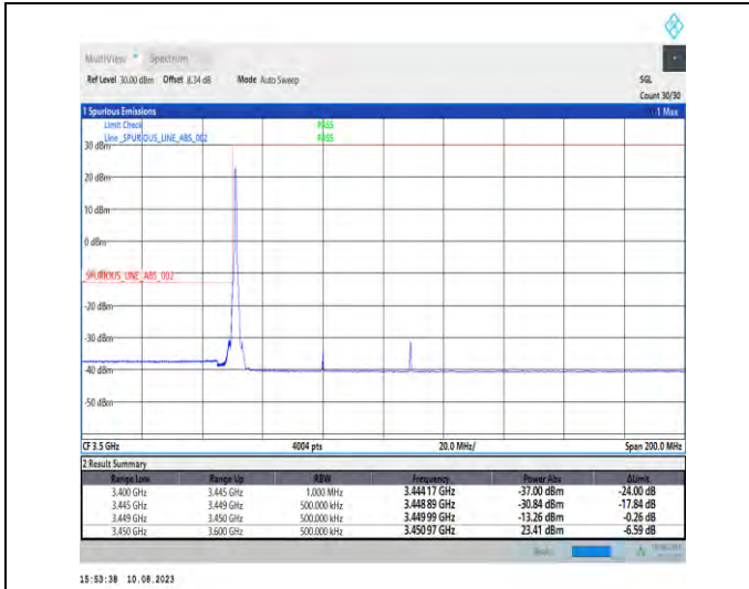
1-N78-3450-3550-PC2-30-60-L-1-DFT-PI2BPSK-Edge_1RB_Left-1@0-Ant1-1--PASS-see graph
