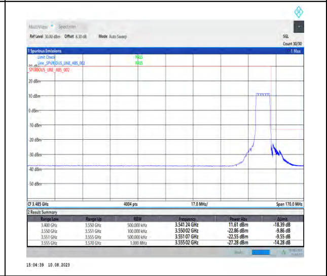
1-N78-3450-3550-PC2-30-10-H-6-CP-QPSK-Outer_Full-24@0-Ant1-1--PASS-see graph
