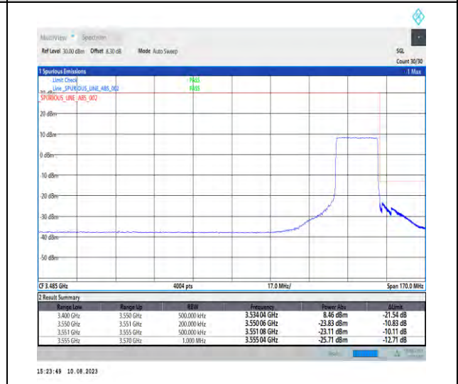
1-N78-3450-3550-PC2-30-20-H-6-CP-QPSK-Outer_Full-51@0-Ant1-1--PASS-see graph
