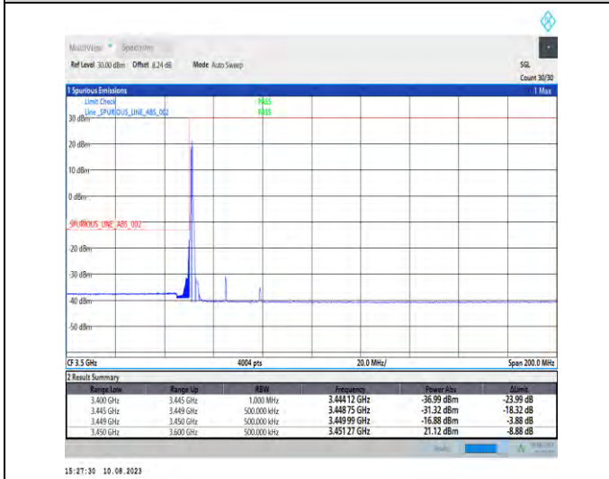
1-N78-3450-3550-PC2-30-30-L-4-CP-QPSK-Edge_1RB_Left-1@0-Ant1-1--PASS-see graph
