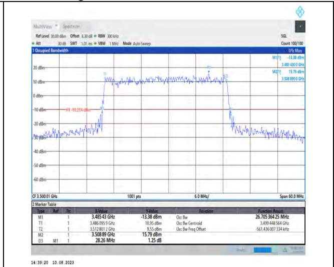
1-N78-3450-3550-PC2-30-30-M-3-DFT-16QAM-Outer_Full-75@0-Ant1-26.705-28.260-≤30-PASS
