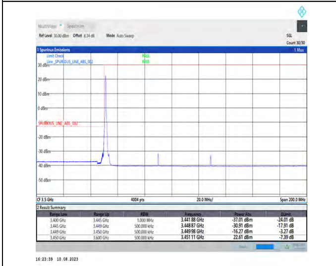
1-N78-3450-3550-PC2-30-80-L-4-CP-QPSK-Edge_1RB_Left-1@0-Ant1-1--PASS-see graph
