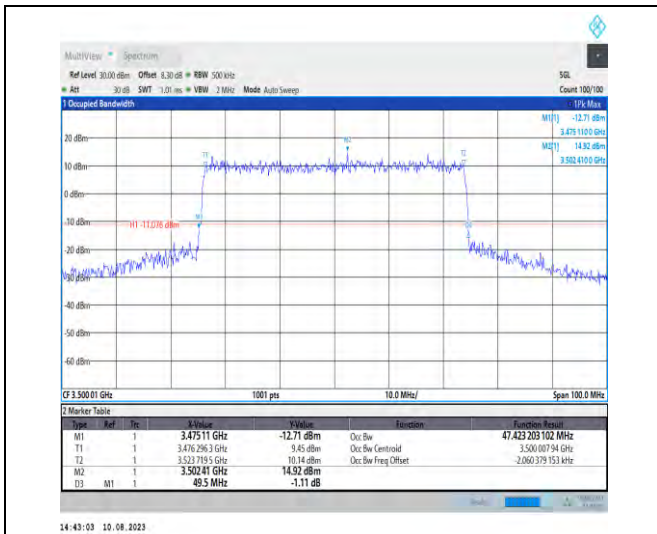
1-N78-3450-3550-PC2-30-50-M-8-CP-64QAM-Outer_Full-133@0-Ant1-47.423-49.500-≤50-PASS
