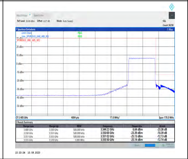
1-N78-3450-3550-PC2-30-30-H-6-CP-QPSK-Outer_Full-78@0-Ant1-1--PASS-see graph
