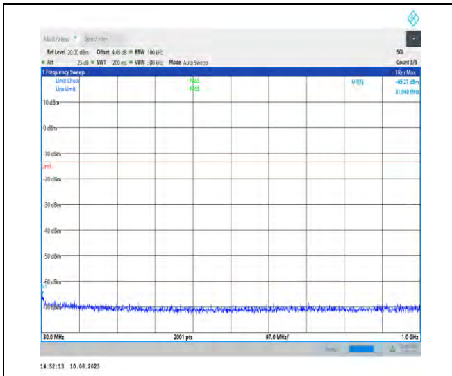
1-N78-3450-3550-PC2-30-100-M-1-N/A-DFT-PI2BP SK-Inner_1RB_Left-1@1-30-1000-Ant1-34.37--65.2 7--13-PASS
