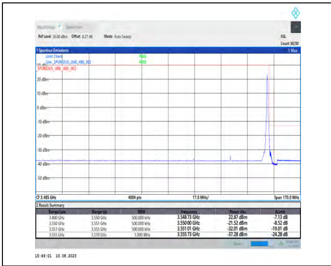
1-N78-3450-3550-PC2-30-50-H-2-DFT-PI2BPSK-Edge_1RB_Right-1@132-Ant1-1--PASS-see graph
