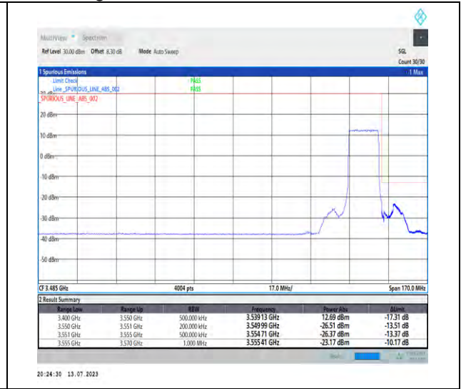
1-N78-3450-3550-PC2-30-15-H-3-DFT-PI2BPSK-Outer_Full-36@0-Ant1-1--PASS-see graph
