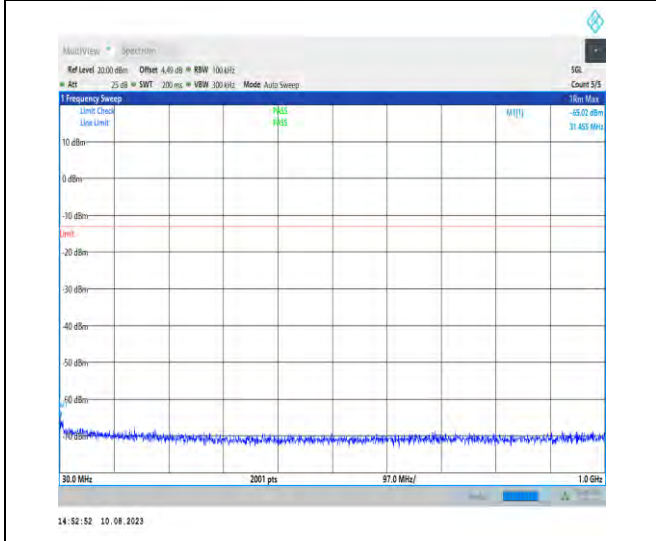
1-N78-3450-3550-PC2-30-100-H-1-N/A-DFT-PI2BP SK-Inner_1RB_Left-1@1-30-1000-Ant1-35.34--65.0 2--13-PASS
