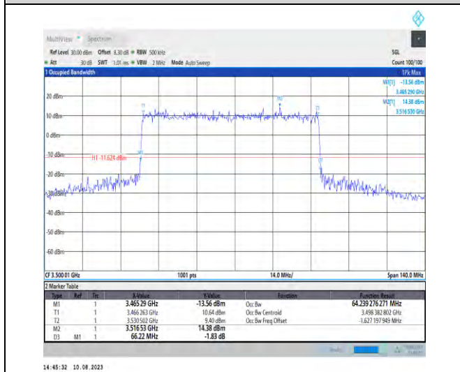
1-N78-3450-3550-PC2-30-70-M-4-DFT-64QAM-Outer_Full-180@0-Ant1-64.239-66.220-≤70-PASS
