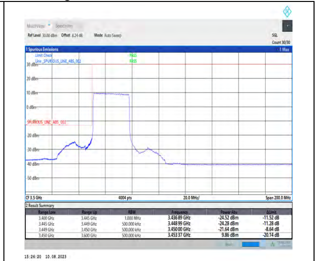
1-N78-3450-3550-PC2-30-30-L-3-DFT-PI2BPSK-Outer_Full-75@0-Ant1-1--PASS-see graph
