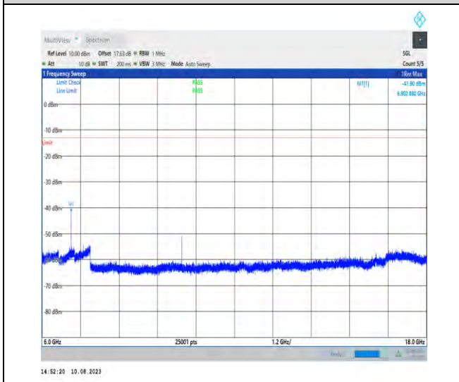
1-N78-3450-3550-PC2-30-100-M-1-N/A-DFT-PI2BP SK-Inner_1RB_Left-1@1-6000-18000-Ant1-7425.12 --41.90--13-PASS
