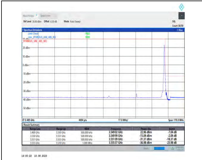
1-N78-3450-3550-PC2-30-60-H-2-DFT-PI2BPSK-Edge_1RB_Right-1@161-Ant1-1--PASS-see graph
