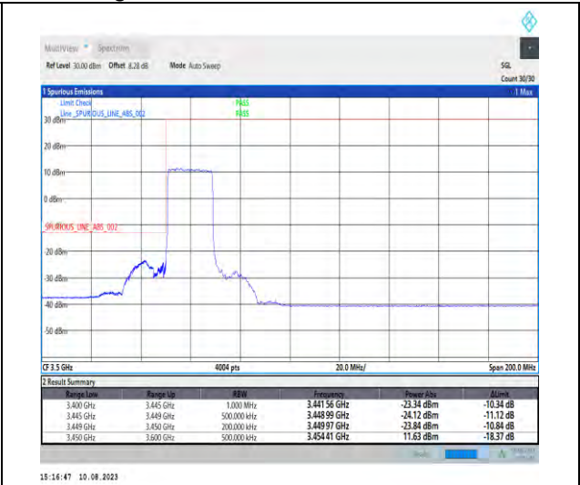
1-N78-3450-3550-PC2-30-20-L-3-DFT-PI2BPSK-Outer_Full-50@0-Ant1-1--PASS-see graph
