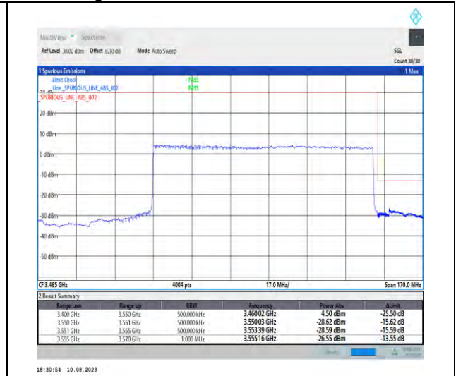
1-N78-3450-3550-PC2-30-100-H-3-DFT-PI2BPSK-Outer_Full-270@0-Ant1-1--PASS-see graph
