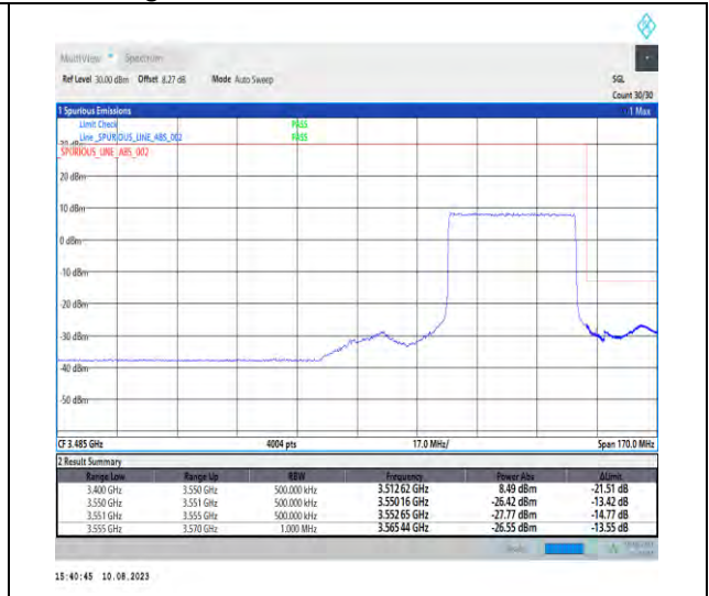
1-N78-3450-3550-PC2-30-40-H-3-DFT-PI2BPSK-Outer_Full-100@0-Ant1-1--PASS-see graph
