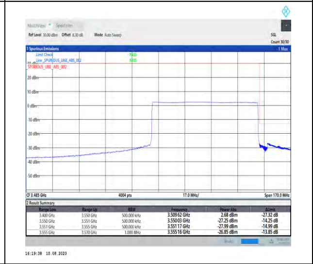
1-N78-3450-3550-PC2-30-70-H-6-CP-QPSK-Outer_Full-189@0-Ant1-1--PASS-see graph
