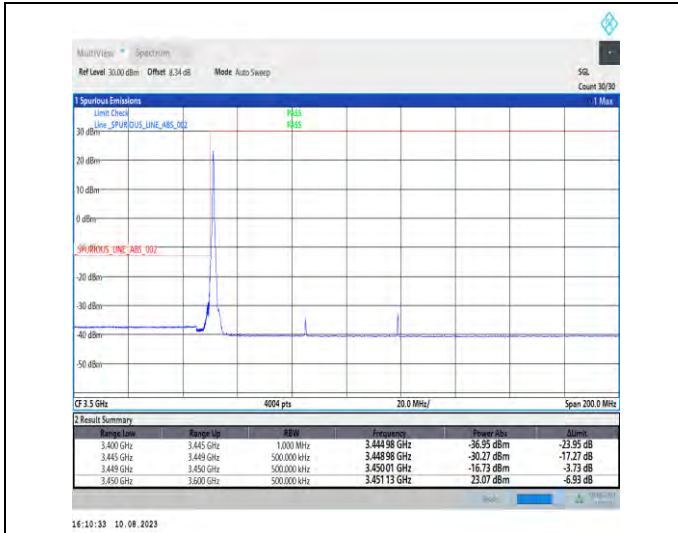
1-N78-3450-3550-PC2-30-70-L-1-DFT-PI2BPSK-Edge_1RB_Left-1@0-Ant1-1--PASS-see graph
