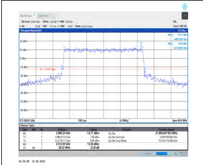
1-N78-3450-3550-PC2-30-30-M-8-CP-64QAM-Outer_Full-78@0-Ant1-27.846-29.520-≤30-PASS
