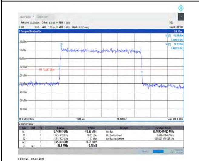
1-N78-3450-3550-PC2-30-100-M-5-DFT-256QAM-Out er_Full-270@0-Ant1-96.104-99.800-≤100-PASS
