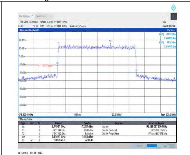
1-N78-3450-3550-PC2-30-100-M-4-DFT-64QAM-Out er_Full-270@0-Ant1-96.188-100.000-≤100-PASS
