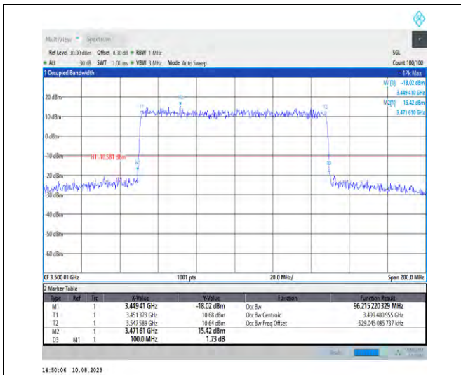
1-N78-3450-3550-PC2-30-100-M-3-DFT-16QAM-Out er_Full-270@0-Ant1-96.215-100.000-≤100-PASS
