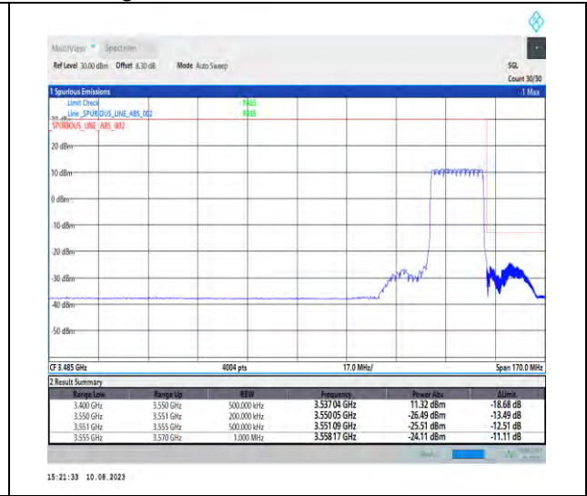
1-N78-3450-3550-PC2-30-20-H-3-DFT-PI2BPSK-Outer_Full-50@0-Ant1-1--PASS-see graph
