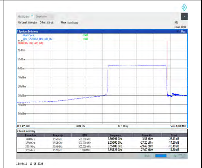
1-N78-3450-3550-PC2-30-60-H-6-CP-QPSK-Outer_Full-162@0-Ant1-1--PASS-see graph
