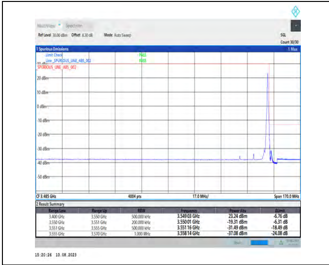
1-N78-3450-3550-PC2-30-20-H-2-DFT-PI2BPSK-Edge_1RB_Right-1@50-Ant1-1--PASS-see graph
