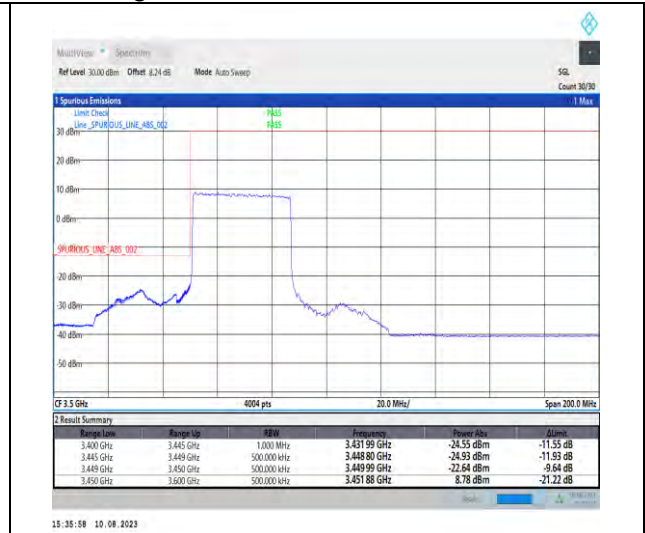
1-N78-3450-3550-PC2-30-40-L-3-DFT-PI2BPSK-Outer_Full-100@0-Ant1-1--PASS-see graph
