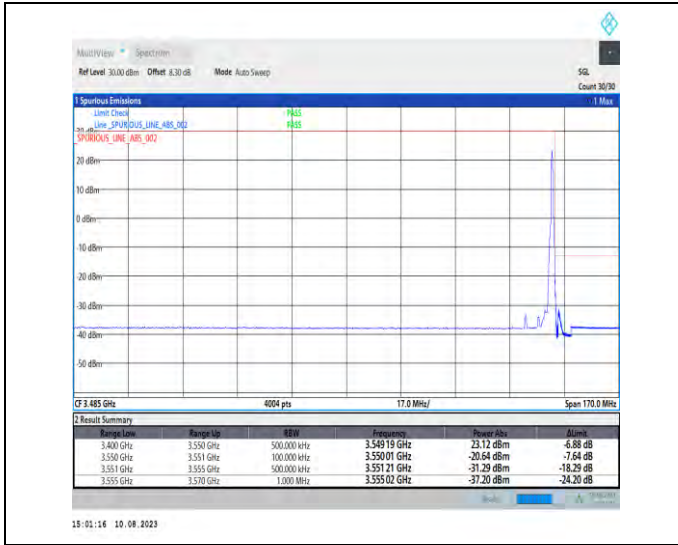
1-N78-3450-3550-PC2-30-10-H-2-DFT-PI2BPSK-Edge_1RB_Right-1@23-Ant1-1--PASS-see graph
