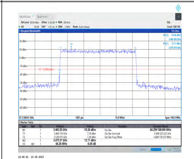
1-N78-3450-3550-PC2-30-70-M-5-DFT-256QAM-Outer_Full-180@0-Ant1-64.299-66.360-≤70-PASS
