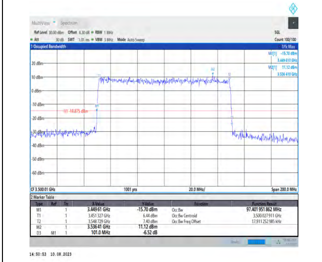
1-N78-3450-3550-PC2-30-100-M-9-CP-256QAM-Outer_Full-273@0-Ant1-97.402-101.000-≤100-PASS
