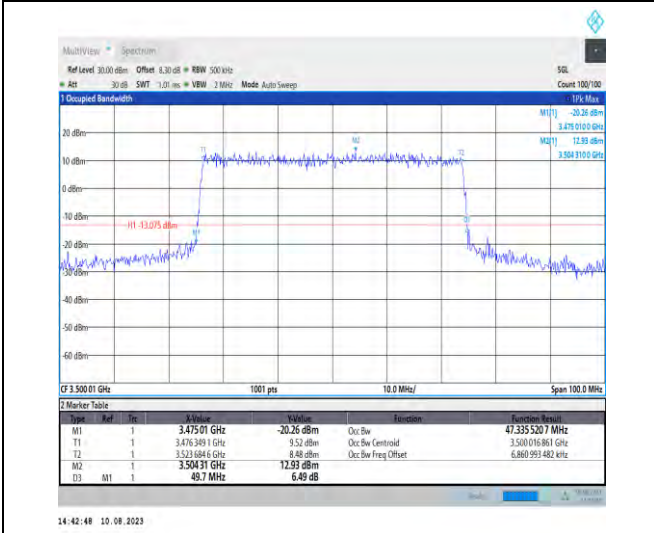
1-N78-3450-3550-PC2-30-50-M-6-CP-QPSK-Outer_Full-133@0-Ant1-47.336-49.700-≤50-PASS
