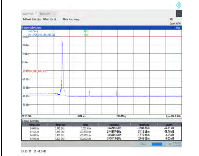
1-N78-3450-3550-PC2-30-70-L-4-CP-QPSK-Edge_1RB_Left-1@0-Ant1-1--PASS-see graph
