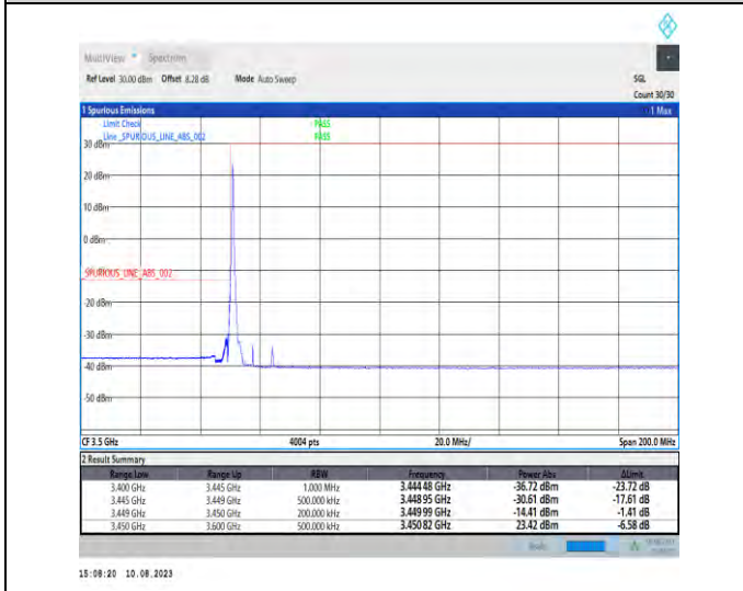
1-N78-3450-3550-PC2-30-15-L-4-CP-QPSK-Edge_1RB_Left-1@0-Ant1-1--PASS-see graph
