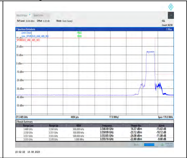
1-N78-3450-3550-PC2-30-10-H-3-DFT-PI2BPSK-Outer_Full-24@0-Ant1-1--PASS-see graph
