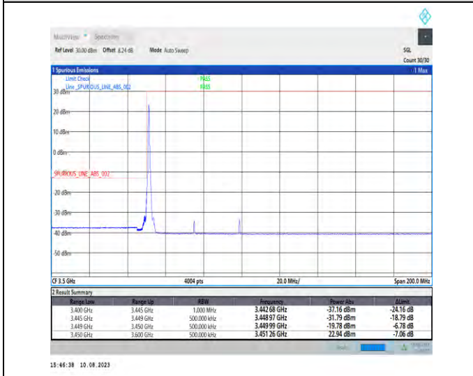
1-N78-3450-3550-PC2-30-50-L-4-CP-QPSK-Edge_1RB_Left-1@0-Ant1-1--PASS-see graph
