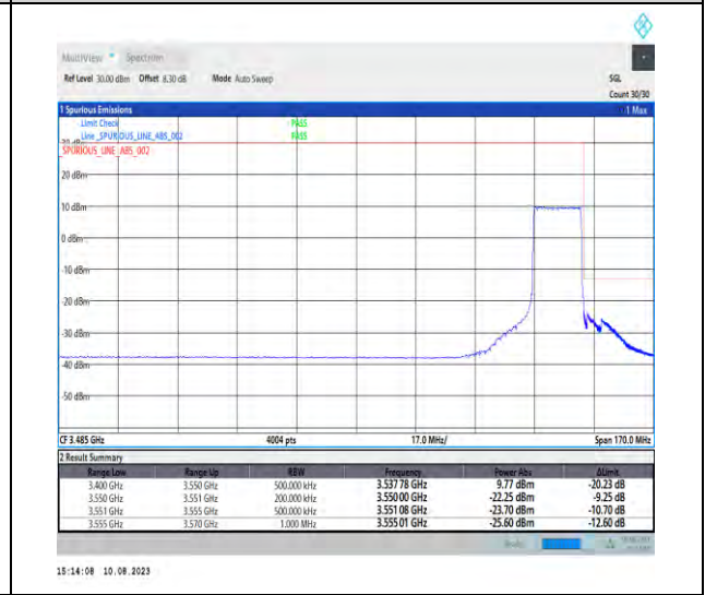
1-N78-3450-3550-PC2-30-15-H-6-CP-QPSK-Outer_Full-38@0-Ant1-1--PASS-see graph
