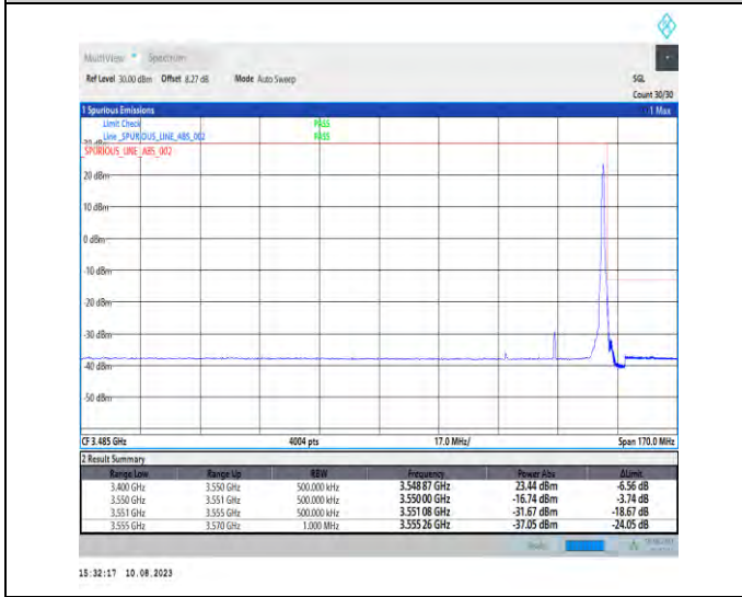
1-N78-3450-3550-PC2-30-30-H-5-CP-QPSK-Edge_1RB_Right-1@77-Ant1-1--PASS-see graph
