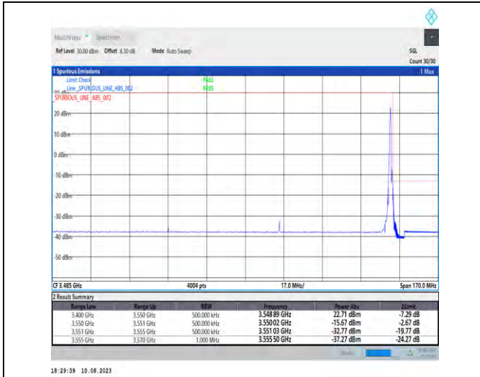
1-N78-3450-3550-PC2-30-100-H-2-DFT-PI2BPSK-Edge_1_RB_Right-1@272-Ant1-1--PASS-see graph
