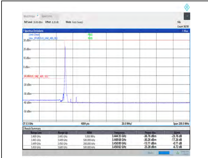
1-N78-3450-3550-PC2-30-15-L-1-DFT-PI2BPSK-Edge_1RB_Left-1@0-Ant1-1--PASS-see graph
