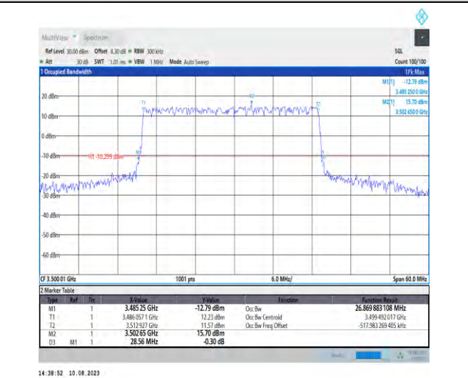
1-N78-3450-3550-PC2-30-30-M-1-DFT-QPSK-Outer_Full-75@0-Ant1-26.87-28.560-≤30-PASS
