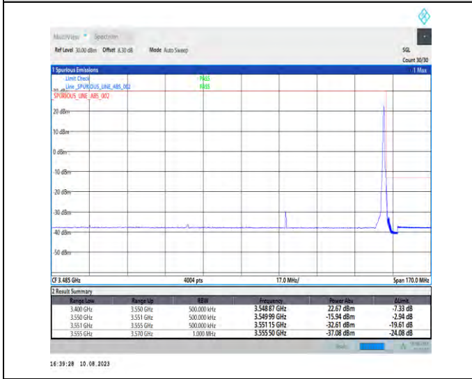
1-N78-3450-3550-PC2-30-90-H-5-CP-QPSK-Edge_1RB_Right-1@244-Ant1-1--PASS-see graph
