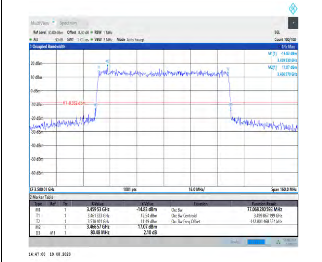
1-N78-3450-3550-PC2-30-80-M-3-DFT-16QAM-Outer_Full-216@0-Ant1-77.068-80.480-≤80-PASS
