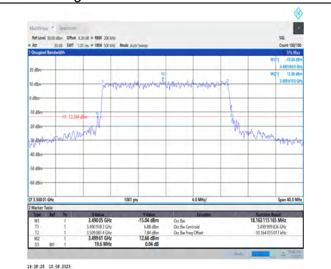
1-N78-3450-3550-PC2-30-20-M-8-CP-64QAM-Outer_Full-51@0-Ant1-18.163-19.600-≤20-PASS
