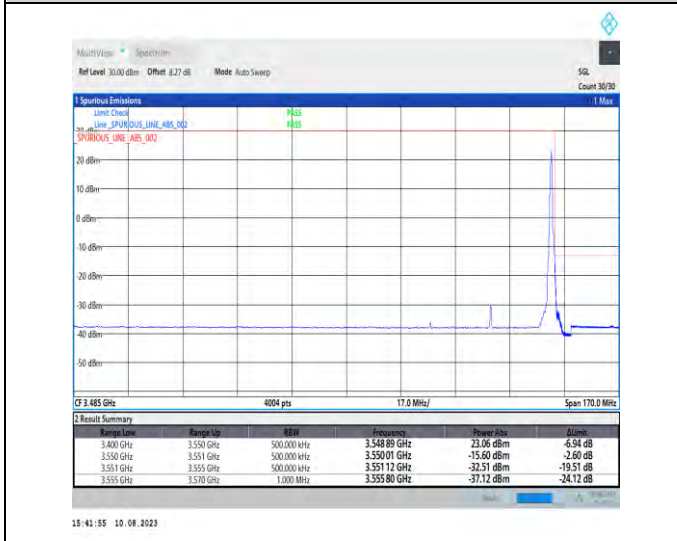
1-N78-3450-3550-PC2-30-40-H-5-CP-QPSK-Edge_1RB_Right-1@105-Ant1-1--PASS-see graph
