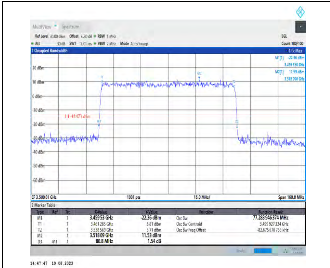
1-N78-3450-3550-PC2-30-80-M-9-CP-256QAM-Out er_Full-217@0-Ant1-77.284-80.800-<=80-PASS
