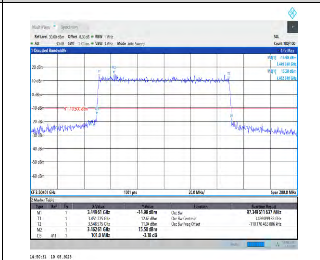
1-N78-3450-3550-PC2-30-100-M-6-CP-QPSK-Outer er_Full-273@0-Ant1-97.35-101.000-≤100-PASS
