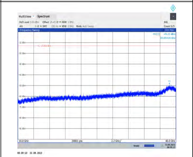
1-N78-3450-3550-PC2-30-100-M-1-N/A-DFT-PI2BPS K-Inner_1RB_Left-1@1-18000-40000-Ant1-18000.00 --57.99--13-PASS
