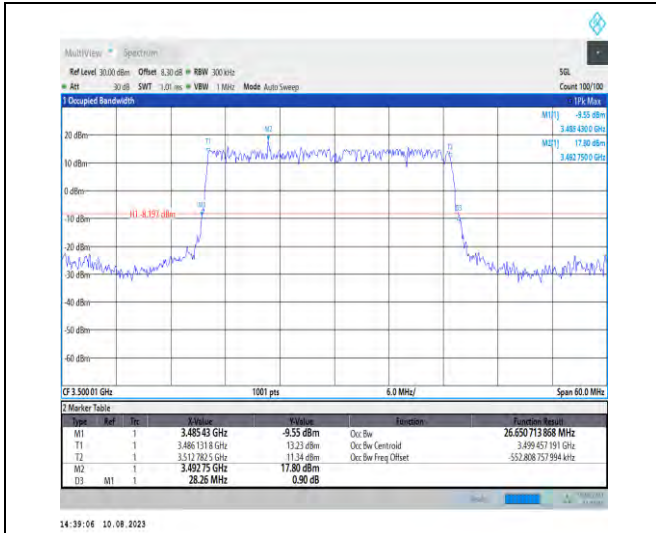
1-N78-3450-3550-PC2-30-30-M-2-DFT-PI2BPSK-Outer_Full-75@0-Ant1-26.651-28.260-≤30-PASS
