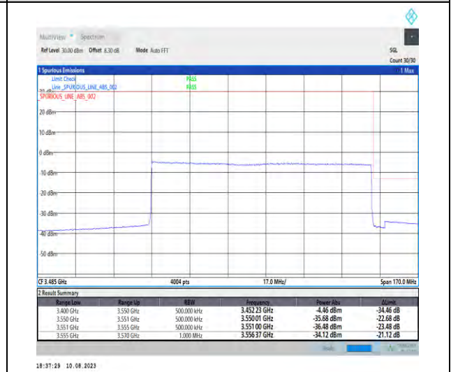
1-N78-3450-3550-PC2-30-100-H-6-CP-QPSK-Outer_Full-273@0-Ant1-1--PASS-see graph
