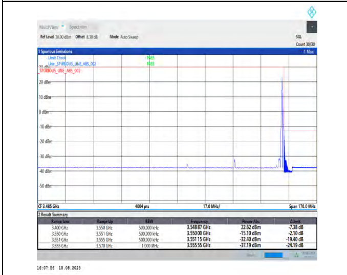
1-N78-3450-3550-PC2-30-60-H-5-CP-QPSK-Edge_1RB_Right-1@161-Ant1-1--PASS-see graph
