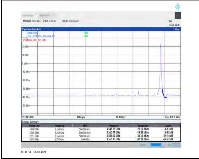
1-N78-3450-3550-PC2-30-50-H-5-CP-QPSK-Edge_1RB_Right-1@132-Ant1-1--PASS-see graph
