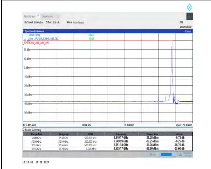
1-N78-3450-3550-PC2-30-15-H-5-CP-QPSK-Edge_1RB_Right-1@37-Ant1-1--PASS-see graph
