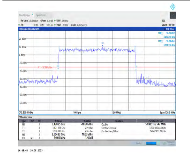
1-N78-3450-3550-PC2-30-60-M-9-CP-256QAM-Outer_Full-162@0-Ant1-57.815-59.640-≤60-PASS
