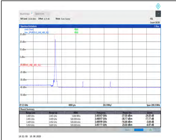
1-N78-3450-3550-PC2-30-80-L-1-DFT-PI2BPSK-Edge_1RB_Left-1@0-Ant1-1--PASS-see graph
