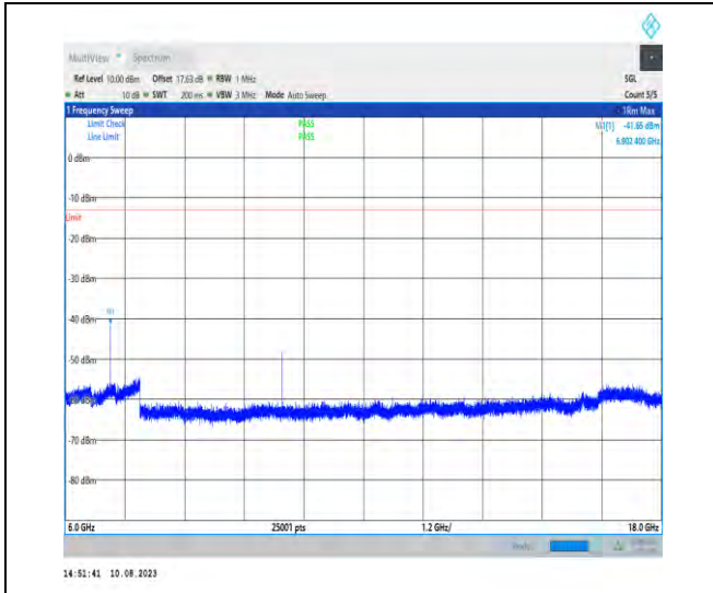
1-N78-3450-3550-PC2-30-100-L-1-N/A-DFT-PI2BP SK-Inner_1RB_Left-1@1-6000-18000-Ant1-7354.08 --41.65--13-PASS
