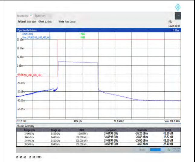
1-N78-3450-3550-PC2-30-50-L-6-CP-QPSK-Outer_Full-133@0-Ant1-1--PASS-see graph
