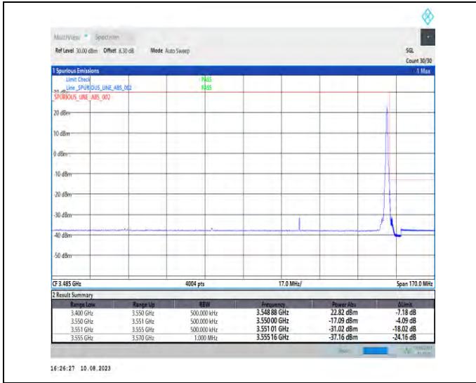
1-N78-3450-3550-PC2-30-80-H-2-DFT-PI2BPSK-Edge_1RB_Right-1@216-Ant1-1--PASS-see graph
