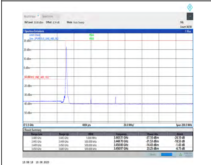
1-N78-3450-3550-PC2-30-60-L-4-CP-QPSK-Edge_1RB_Left-1@0-Ant1-1--PASS-see graph
