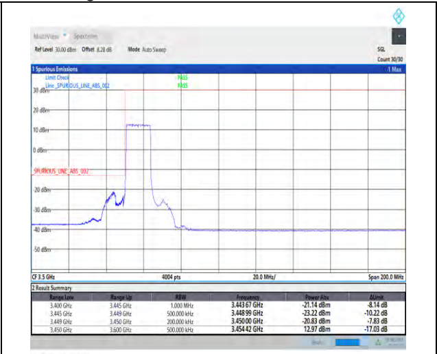
1-N78-3450-3550-PC2-30-15-L-3-DFT-PI2BPSK-Outer_Full-36@0-Ant1-1--PASS-see graph
