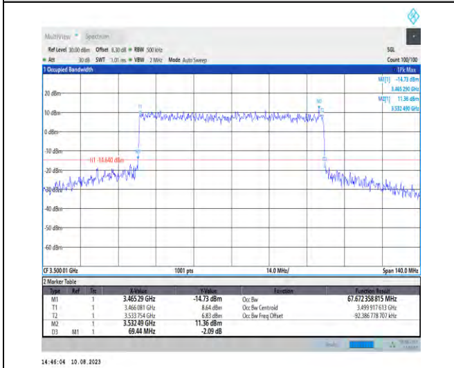
1-N78-3450-3550-PC2-30-70-M-8-CP-64QAM-Outer_Full-189@0-Ant1-67.672-69.440-≤70-PASS
