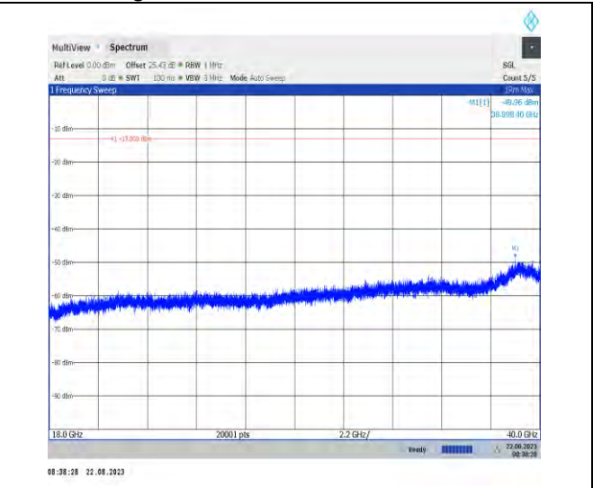
1-N77-3700-3980-PC2-30-100-L-1-N/A-DFT-PI2BPS K-Inner_1RB_Left-1@1-18000-40000-Ant1-18000.00 --56.06--13-PASS
