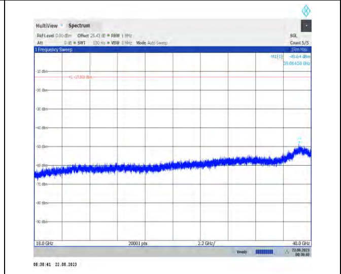
1-N77-3700-3980-PC2-30-100-M-1-N/A-DFT-PI2BPS K-Inner_1RB_Left-1@1-18000-40000-Ant1-18000.00 --56.66--13-PASS
