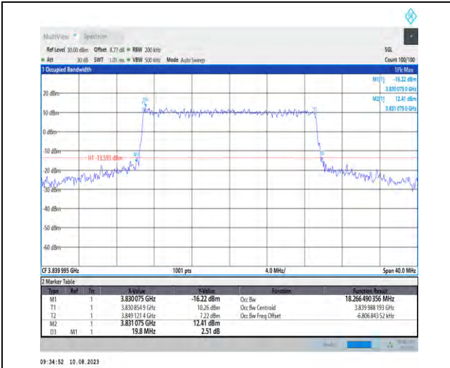
1-N77-3700-3980-PC2-30-20-M-7-CP-16QAM-Outer_Full-51@0-Ant1-18.266-19.800-≤20-PASS
