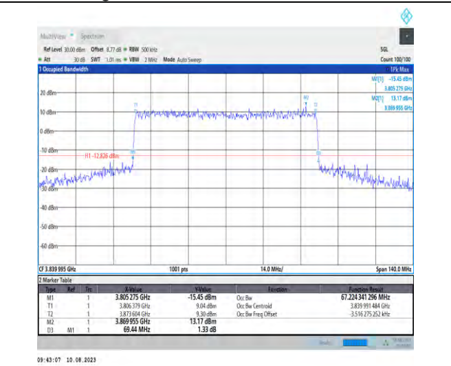
1-N77-3700-3980-PC2-30-70-M-7-CP-16QAM-Outer_Full-189@0-Ant1-67.224-69.440-≤70-PASS
