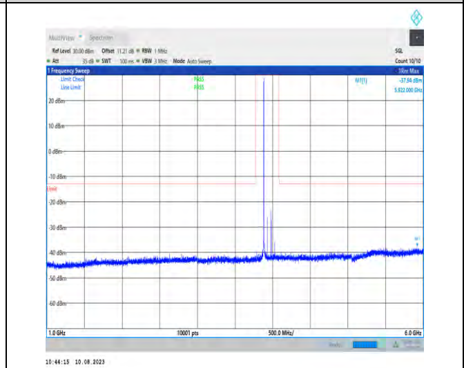
1-N77-3700-3980-PC2-30-100-H-1-N/A-DFT-PI2BPS K-Inner_1RB_Left-1@1-1000-6000-Ant1-5915.00--3 7.94--13-PASS
