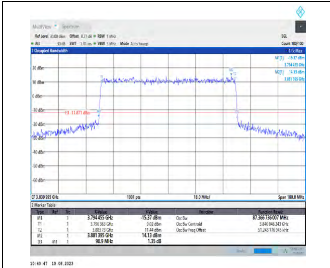
1-N77-3700-3980-PC2-30-90-M-8-CP-64QAM-Outer_Full-245@0-Ant1-87.367-90.900-≤90-PASS
