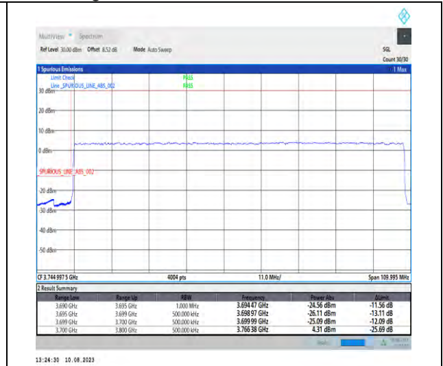
1-N77-3700-3980-PC2-30-100-L-3-DFT-PI2BPSK-Outer_Full-270@0-Ant1-1--PASS-see graph
