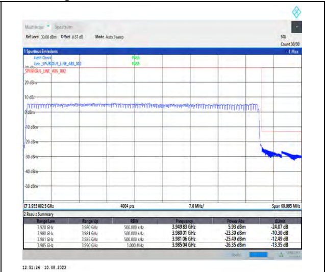
1-N77-3700-3980-PC2-30-60-H-3-DFT-PI2BPSK-Outer_Full-162@0-Ant1-1--PASS-see graph
