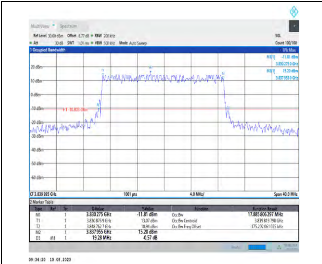
1-N77-3700-3980-PC2-30-20-M-3-DFT-16QAM-Outer_Full-50@0-Ant1-17.886-19.280-≤20-PASS
