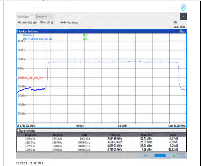
1-N77-3700-3980-PC2-30-50-L-3-DFT-PI2BPSK-Outer_Full-128@0-Ant1-1--PASS-see graph
