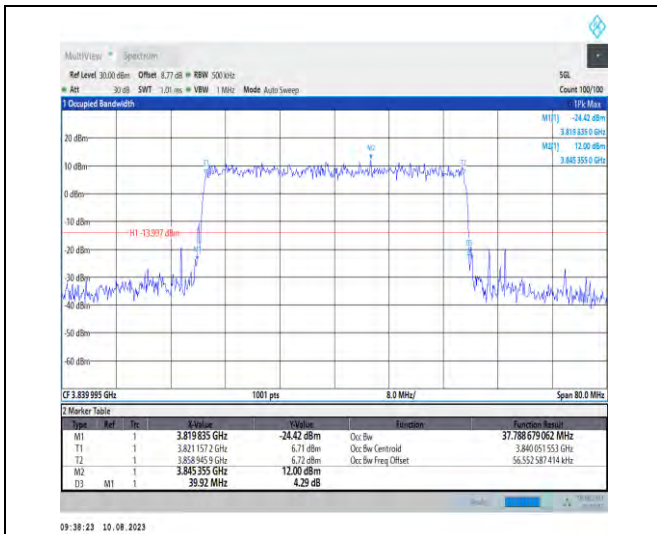
1-N77-3700-3980-PC2-30-40-M-9-CP-256QAM-Out er_Full-106@0-Ant1-37.789-39.920-≤40-PASS
