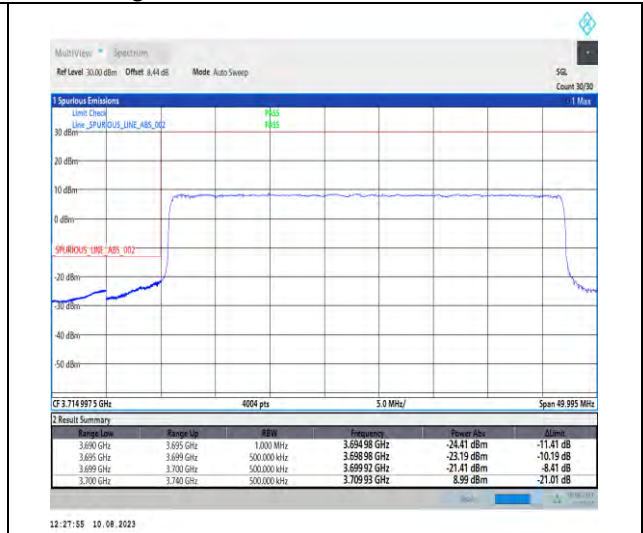
1-N77-3700-3980-PC2-30-40-L-3-DFT-PI2BPSK-Outer_Full-100@0-Ant1-1--PASS-see graph
