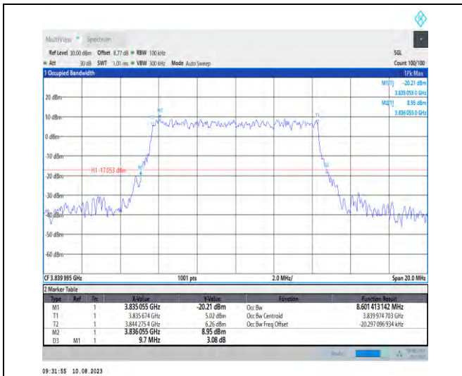
1-N77-3700-3980-PC2-30-10-M-9-CP-256QAM-Out er_Full-24@0-Ant1-8.601-9.700-≤10-PASS
