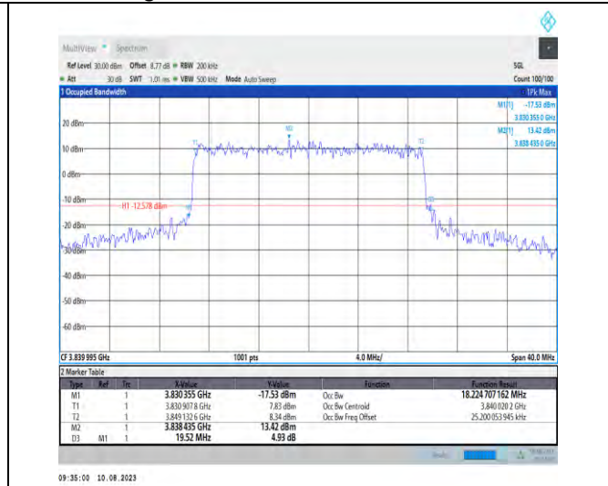
1-N77-3700-3980-PC2-30-20-M-8-CP-64QAM-Outer_Full-51@0-Ant1-18.225-19.520-≤20-PASS
