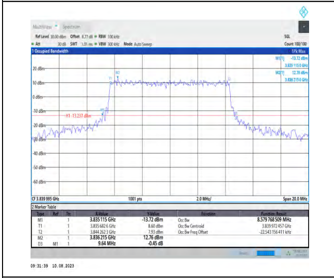
1-N77-3700-3980-PC2-30-10-M-7-CP-16QAM-Outer_Full-24@0-Ant1-8.58-9.640-≤10-PASS
