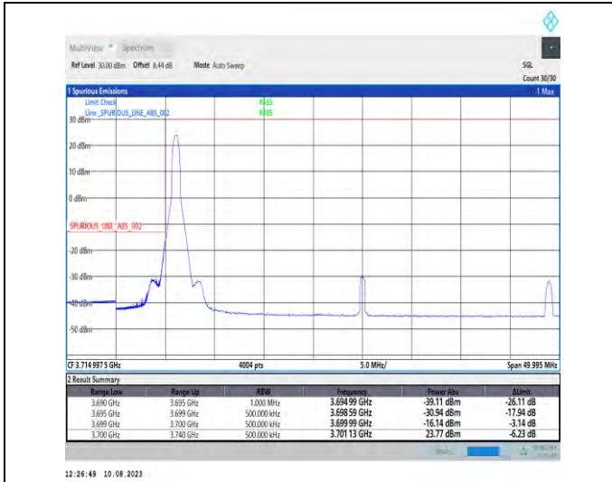
1-N77-3700-3980-PC2-30-40-L-1-DFT-PI2BPSK-Edge_1RB_Left-1@0-Ant1-1--PASS-see graph
