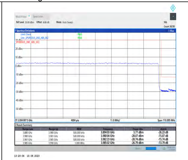
1-N77-3700-3980-PC2-30-100-H-3-DFT-PI2BPSK-Outer_Full-270@0-Ant1-1--PASS-see graph
