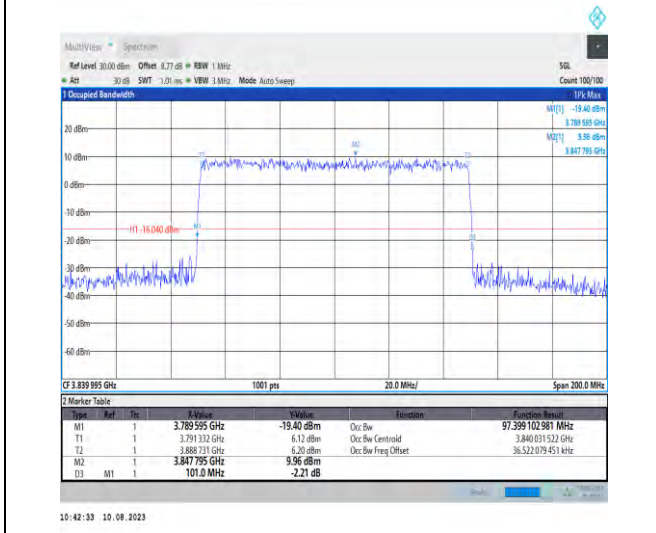
1-N77-3700-3980-PC2-30-100-M-9-CP-256QAM-Out ter_Full-273@0-Ant1-97.399-101.000-≤100-PASS
