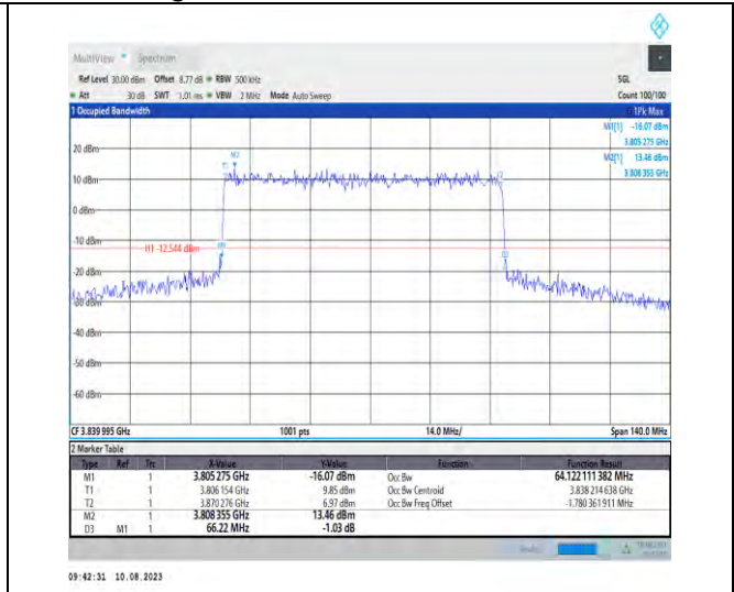
1-N77-3700-3980-PC2-30-70-M-3-DFT-16QAM-Outer_Full-180@0-Ant1-64.122-66.220-≤70-PASS
