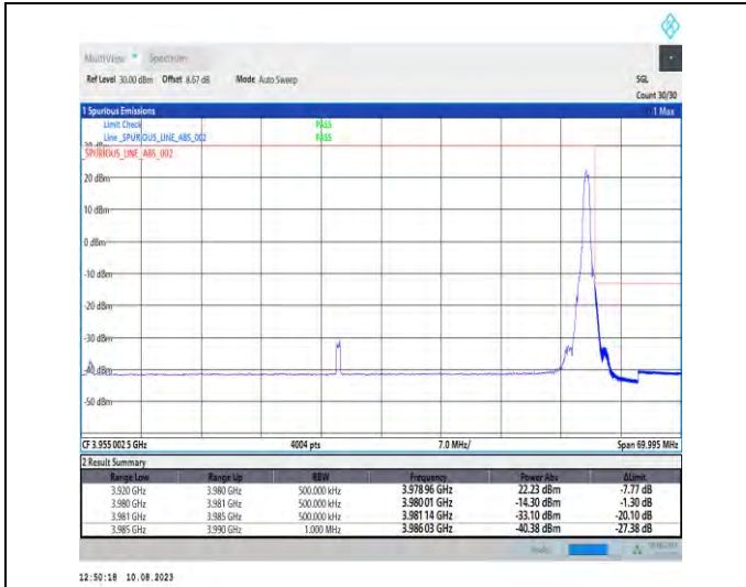
1-N77-3700-3980-PC2-30-60-H-2-DFT-PI2BPSK-Edge_1RB_Right-1@161-Ant1-1--PASS-see graph
