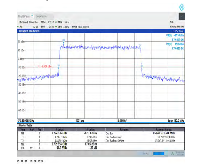
1-N77-3700-3980-PC2-30-90-M-1-DFT-QPSK-Outer_Full-240@0-Ant1-85.7-89.100-≤90-PASS
