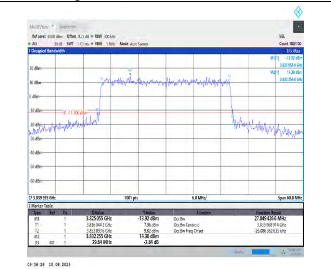
1-N77-3700-3980-PC2-30-30-M-7-CP-16QAM-Outer_Full-78@0-Ant1-27.849-29.640-≤30-PASS
