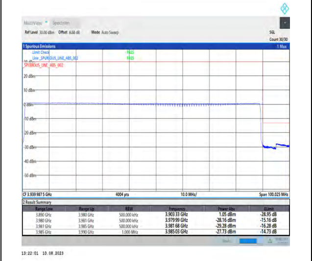
1-N77-3700-3980-PC2-30-90-H-6-CP-QPSK-Outer_Full-245@0-Ant1-1--PASS-see graph
