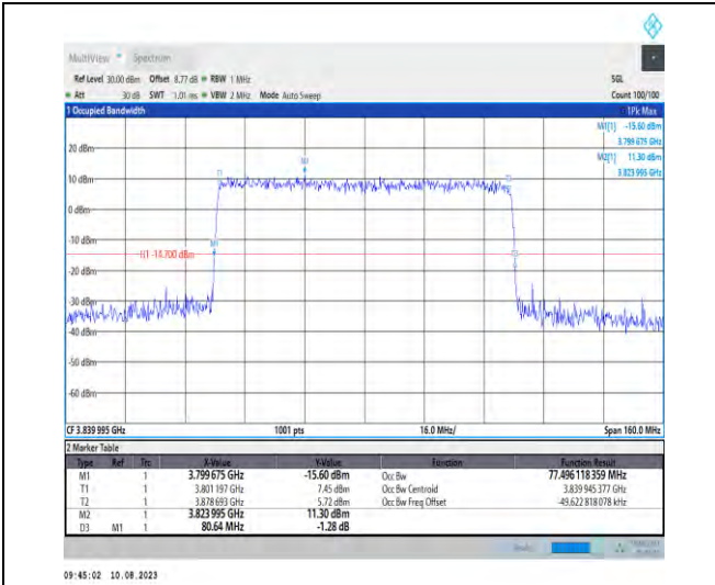
1-N77-3700-3980-PC2-30-80-M-9-CP-256QAM-Out er_Full-217@0-Ant1-77.496-80.640-≤80-PASS
