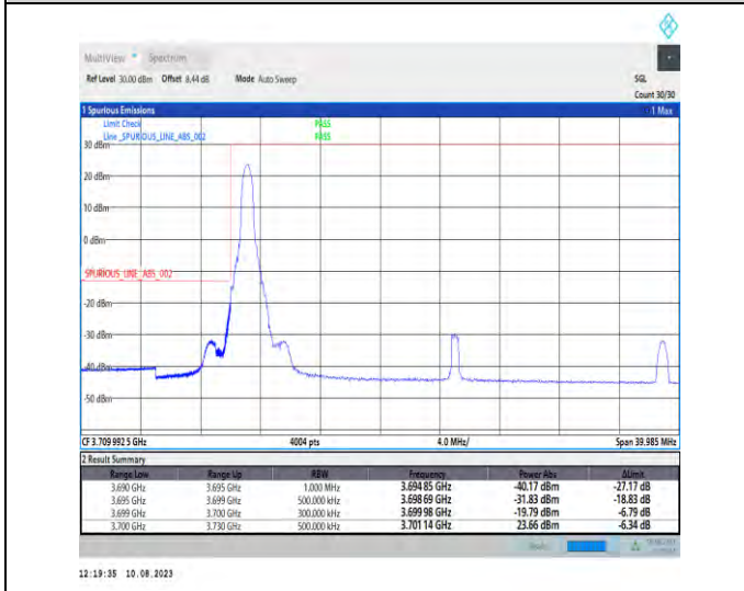
1-N77-3700-3980-PC2-30-30-L-4-CP-QPSK-Edge_1RB_Left-1@0-Ant1-1--PASS-see graph
