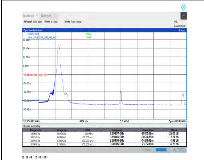
1-N77-3700-3980-PC2-30-40-L-4-CP-QPSK-Edge_1RB_Left-1@0-Ant1-1--PASS-see graph
