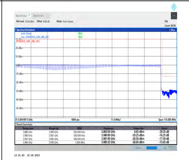
1-N77-3700-3980-PC2-30-100-H-6-CP-QPSK-Outer_Full-273@0-Ant1-1--PASS-see graph
