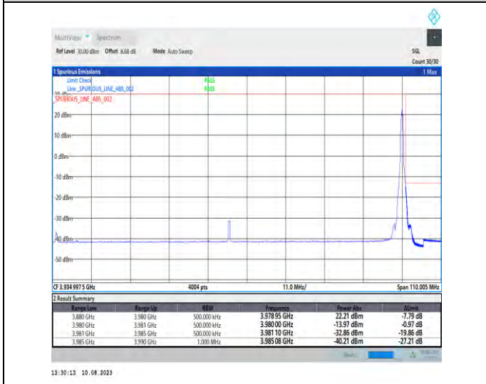
1-N77-3700-3980-PC2-30-100-H-5-CP-QPSK-Edge_1_RB_Right-1@272-Ant1-1--PASS-see graph
