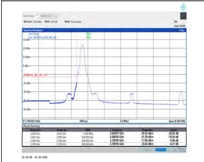
1-N77-3700-3980-PC2-30-20-L-4-CP-QPSK-Edge_1RB_Left-1@0-Ant1-1--PASS-see graph
