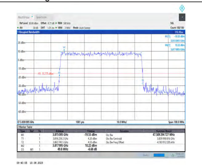
1-N77-3700-3980-PC2-30-50-M-9-CP-256QAM-Outer_Full-133@0-Ant1-47.509-49.800-≤50-PASS
