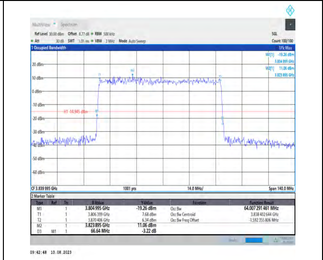
1-N77-3700-3980-PC2-30-70-M-5-DFT-256QAM-Outer_Full-180@0-Ant1-64.007-66.640-≤70-PASS
