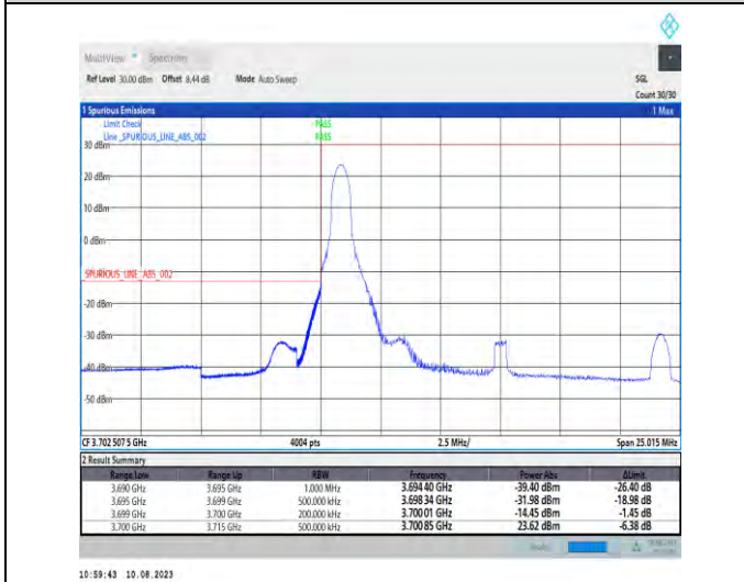
1-N77-3700-3980-PC2-30-15-L-4-CP-QPSK-Edge_1RB_Left-1@0-Ant1-1--PASS-see graph
