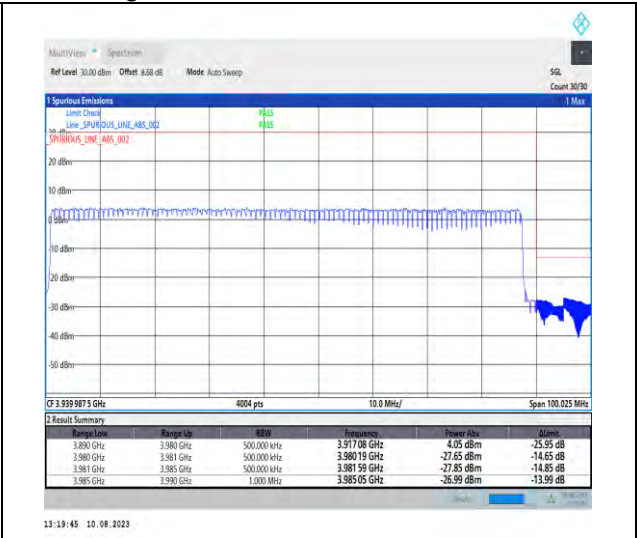
1-N77-3700-3980-PC2-30-90-H-3-DFT-PI2BPSK-Outer_Full-240@0-Ant1-1--PASS-see graph
