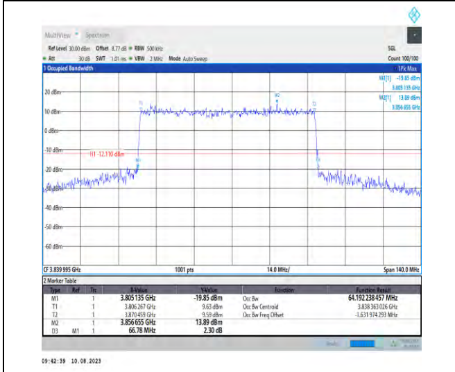
1-N77-3700-3980-PC2-30-70-M-4-DFT-64QAM-Outer_Full-180@0-Ant1-64.192-66.780-≤70-PASS
