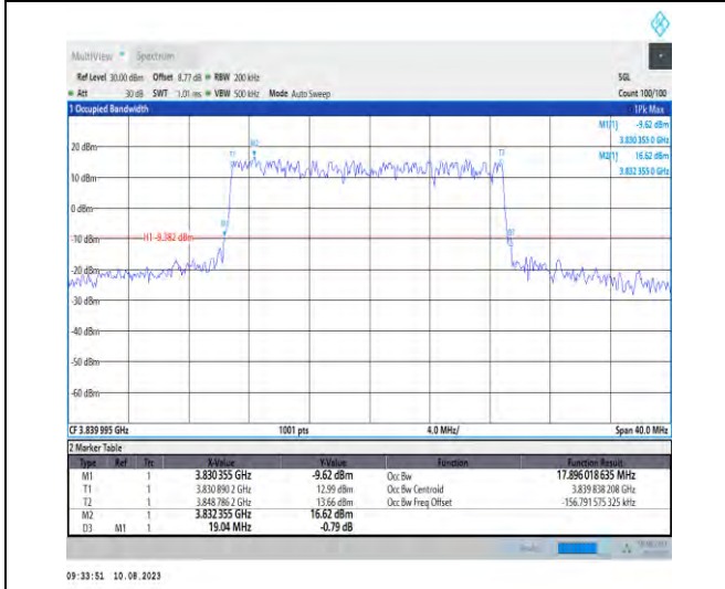
1-N77-3700-3980-PC2-30-20-M-1-DFT-QPSK-Outer_Full-50@0-Ant1-17.896-19.040-≤20-PASS
