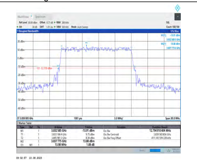
1-N77-3700-3980-PC2-30-15-M-5-DFT-256QAM-Outer_Full-36@0-Ant1-12.795-13.980-≤15-PASS
