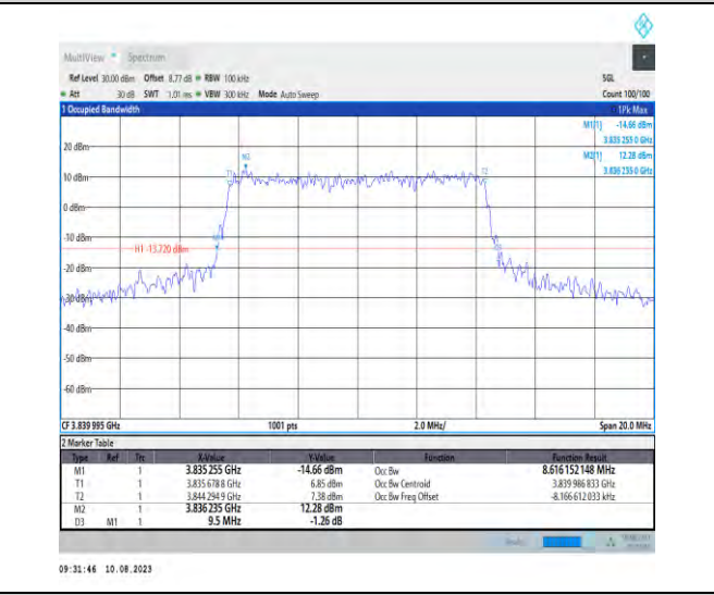
1-N77-3700-3980-PC2-30-10-M-8-CP-64QAM-Outer_Full-24@0-Ant1-8.616-9.500-≤10-PASS
