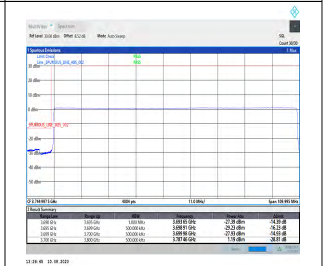
1-N77-3700-3980-PC2-30-100-L-6-CP-QPSK-Outer_Full-273@0-Ant1-1--PASS-see graph
