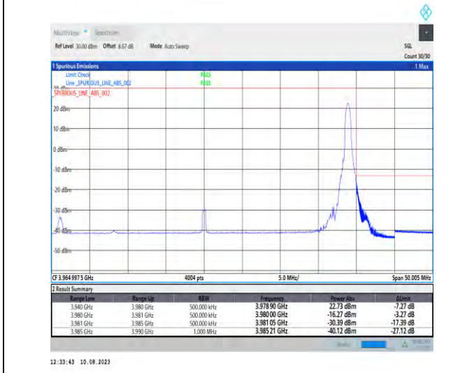
1-N77-3700-3980-PC2-30-40-H-5-CP-QPSK-Edge_1RB_Right-1@105-Ant1-1--PASS-see graph
