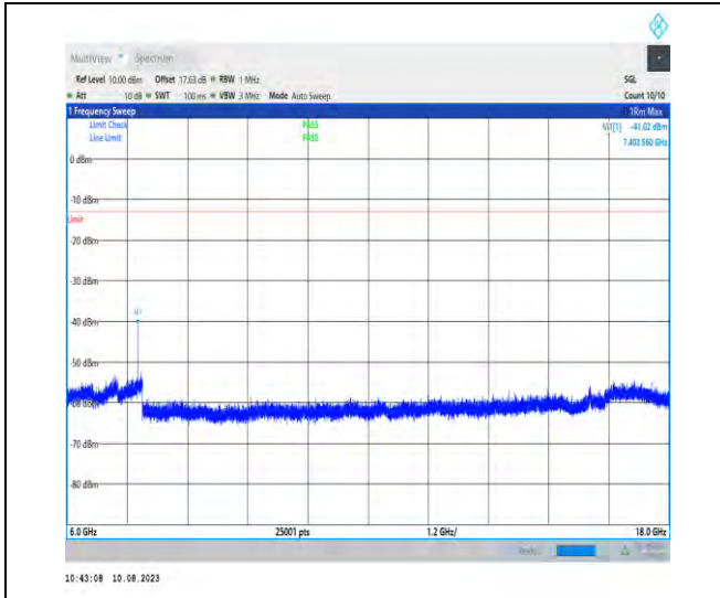
1-N77-3700-3980-PC2-30-100-L-1-N/A-DFT-PI2BPS K-Inner_1RB_Left-1@1-6000-18000-Ant1-11113.92- -41.02--13-PASS
