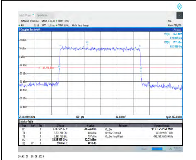
1-N77-3700-3980-PC2-30-100-M-5-DFT-256QAM-Out uter_Full-270@0-Ant1-96.531-99.800-≤100-PASS
