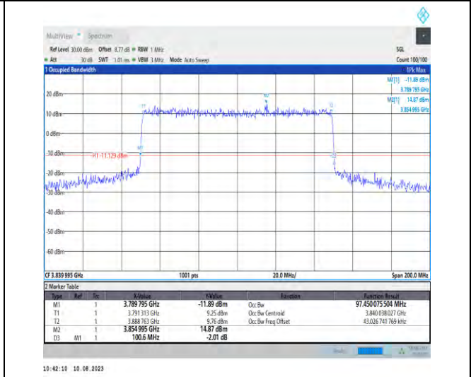
1-N77-3700-3980-PC2-30-100-M-6-CP-QPSK-Outer _Full-273@0-Ant1-97.45-100.600-≤100-PASS
