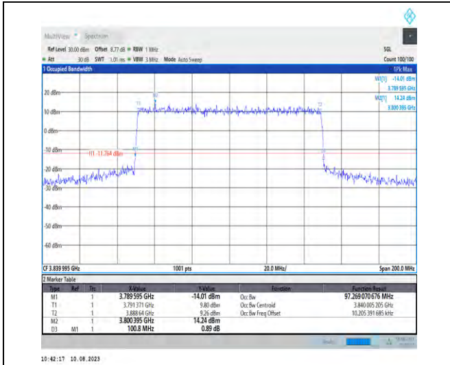
1-N77-3700-3980-PC2-30-100-M-7-CP-16QAM-Out er_Full-273@0-Ant1-97.269-100.800-≤100-PASS
