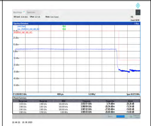
1-N77-3700-3980-PC2-30-50-H-6-CP-QPSK-Outer_Full-133@0-Ant1-1--PASS-see graph
