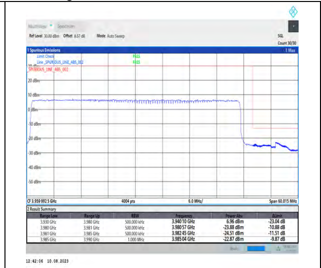
1-N77-3700-3980-PC2-30-50-H-3-DFT-PI2BPSK-Outer_Full-128@0-Ant1-1--PASS-see graph
