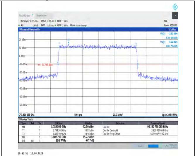
1-N77-3700-3980-PC2-30-100-M-4-DFT-64QAM-Out er_Full-270@0-Ant1-96.131-99.800-≤100-PASS
