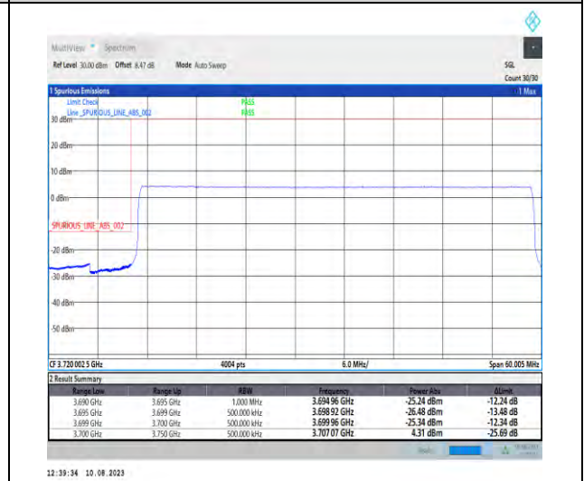
1-N77-3700-3980-PC2-30-50-L-6-CP-QPSK-Outer_Full-133@0-Ant1-1--PASS-see graph
