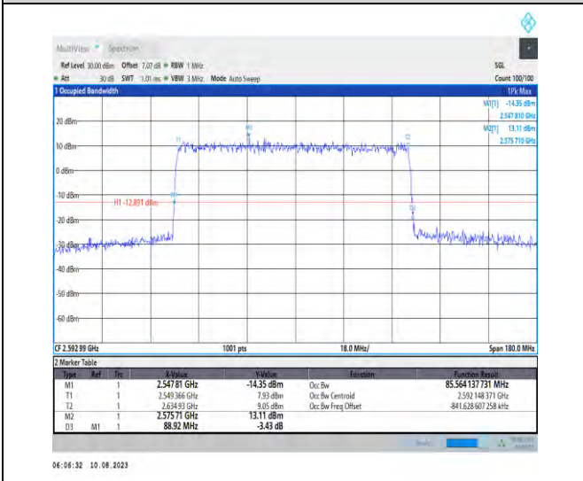
1-N41-PC3-30-90-M-4-DFT-64QAM-Outer_Full-240 @0-Ant1-85.564-88.920-<90-PASS
