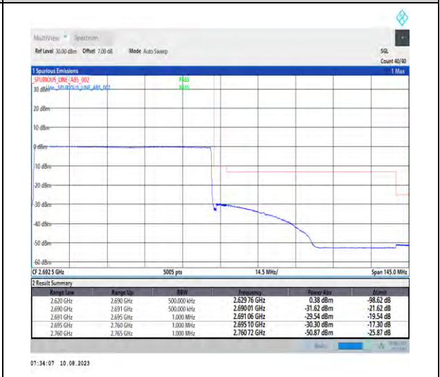
1-N41-PC3-30-70-H-6-CP-QPSK-Outer_Full-189@0-Ant1-1--PASS-see graph
