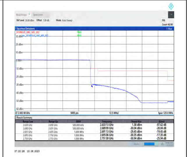
1-N41-PC3-30-60-H-6-CP-QPSK-Outer_Full-162@0-Ant1-1--PASS-see graph
