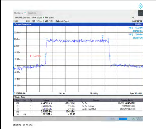
1-N41-PC3-30-90-M-5-DFT-256QAM-Outer_Full-240 @0-Ant1-85.551-89.280-<90-PASS
