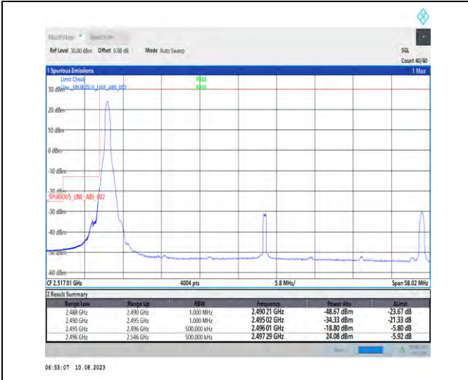
1-N41-PC3-30-50-L-1-DFT-PI2BPSK-Edge_1RB_Left-1@0-Ant1-1--PASS-see graph
