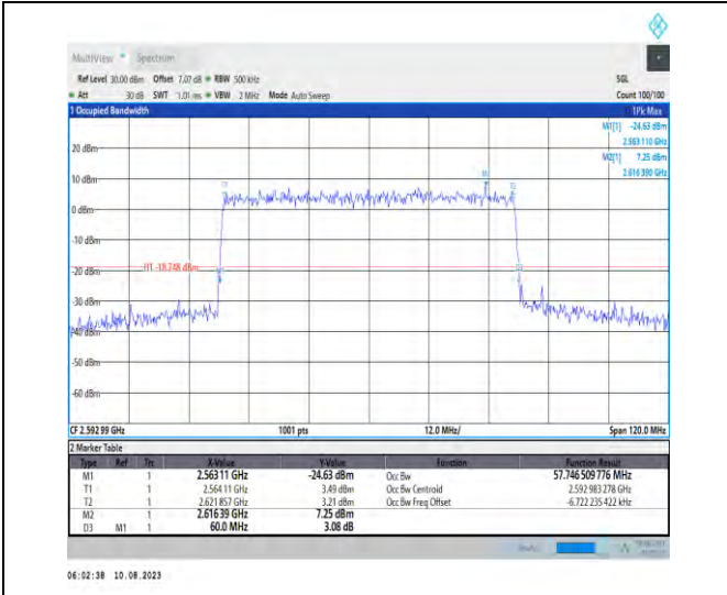
1-N41-PC3-30-60-M-9-CP-256QAM-Outer_Full-162 @0-Ant1-57.747-60.000-≤60-PASS
