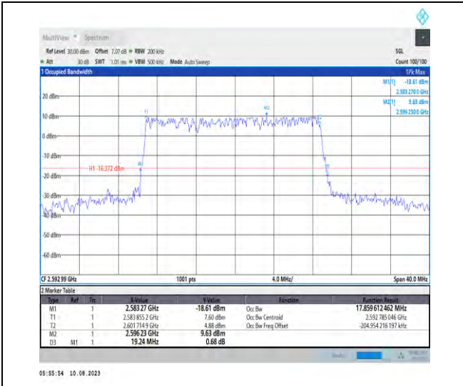
1-N41-PC3-30-20-M-5-DFT-256QAM-Outer_Full-50 @0-Ant1-17.86-19.240-≤20-PASS
