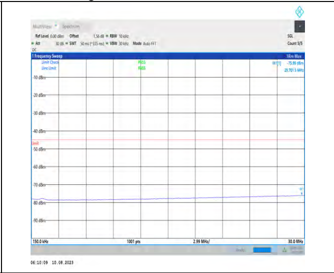
1-N41-PC3-30-100-H-1-N/A-DFT-PI2BPSK-Inner_1R B_Left-1@1-0.15-30-Ant1-30.00--75.99--45-PASS
