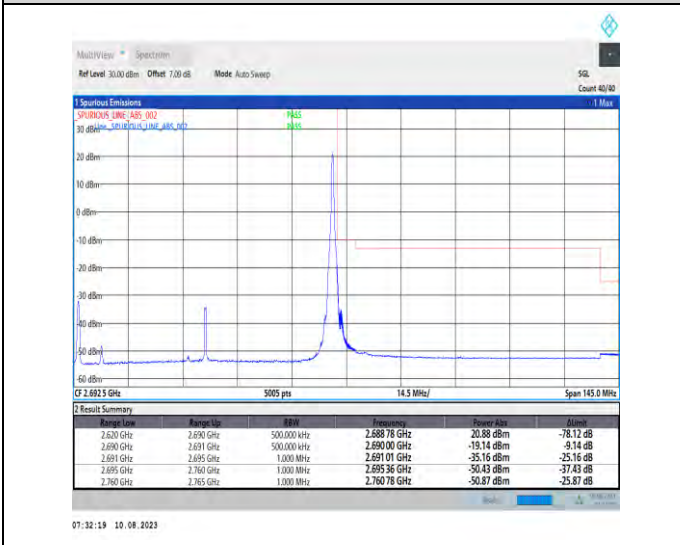
1-N41-PC3-30-70-H-5-CP-QPSK-Edge_1RB_Right-1@188-Ant1-1--PASS-see graph
