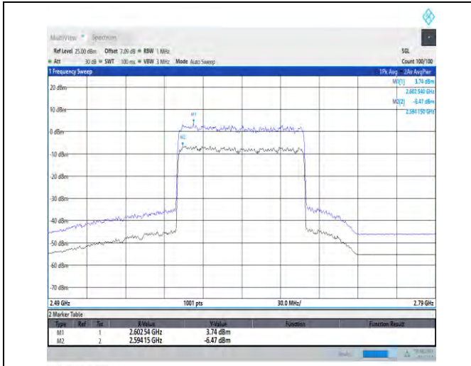
1-N41-PC3-30-100-H-1-DFT-256QAM-Outer_Full-270 @0-Ant1-10.21-100%-0.00-10.21-PASS-≤13
