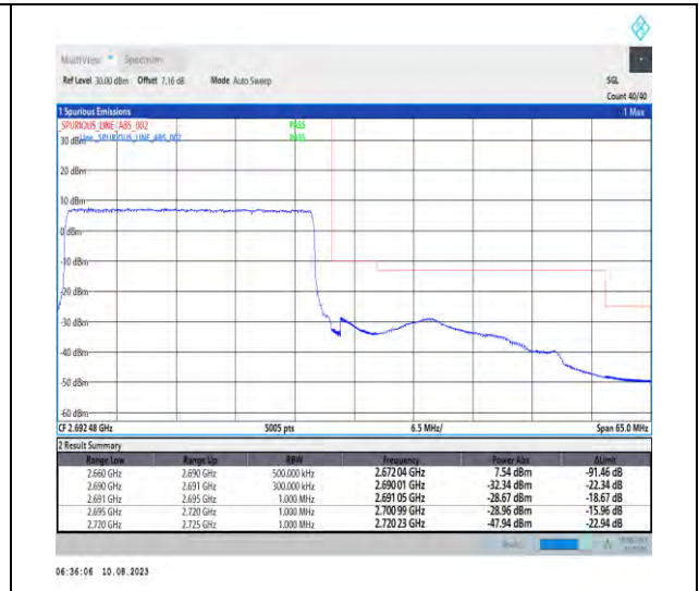
1-N41-PC3-30-30-H-3-DFT-PI2BPSK-Outer_Full-75@0-Ant1-1--PASS-see graph
