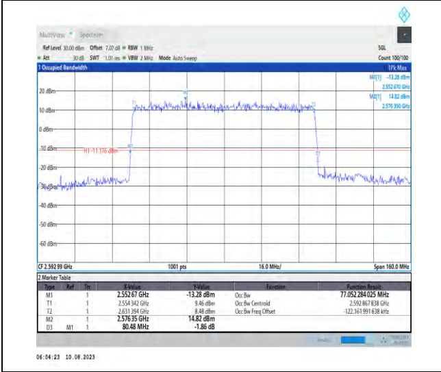
1-N41-PC3-30-80-M-1-DFT-QPSK-Outer_Full-216 @0-Ant1-77.052-80.480-<=80-PASS
