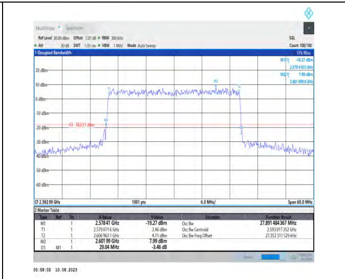
1-N41-PC3-30-30-M-9-CP-256QAM-Outer_Full-78@ 0-Ant1-27.891-29.040-≤30-PASS
