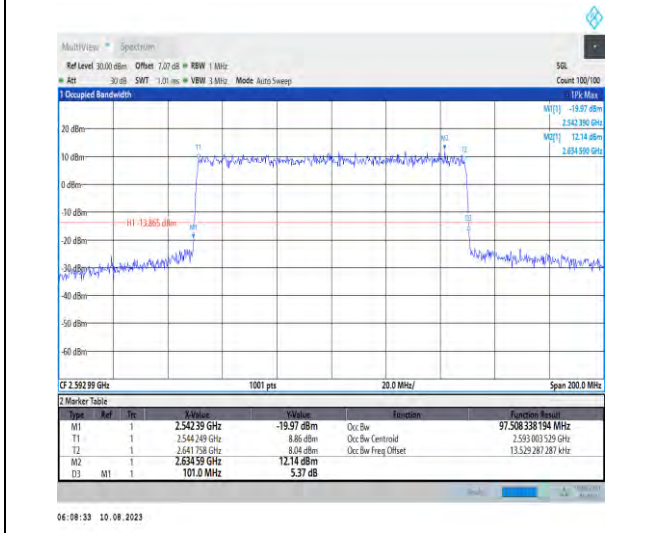
1-N41-PC3-30-100-M-7-CP-16QAM-Outer_Full-273@0-Ant1-97.508-101.000-≤100-PASS
