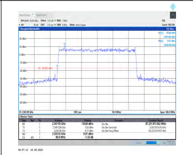
1-N41-PC3-30-90-M-9-CP-256QAM-Outer_Full-245 @0-Ant1-87.252-90.900-≤90-PASS
