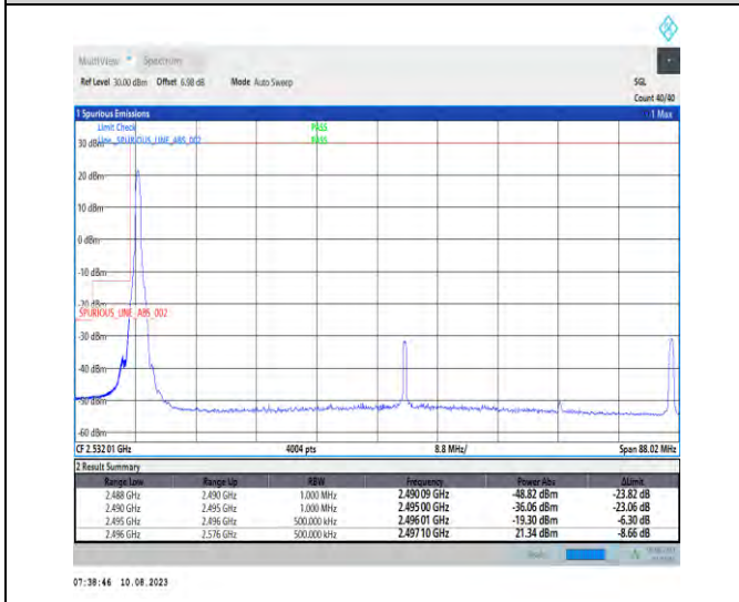
1-N41-PC3-30-80-L-4-CP-QPSK-Edge_1RB_Left-1@0-Ant1-1--PASS-see graph
