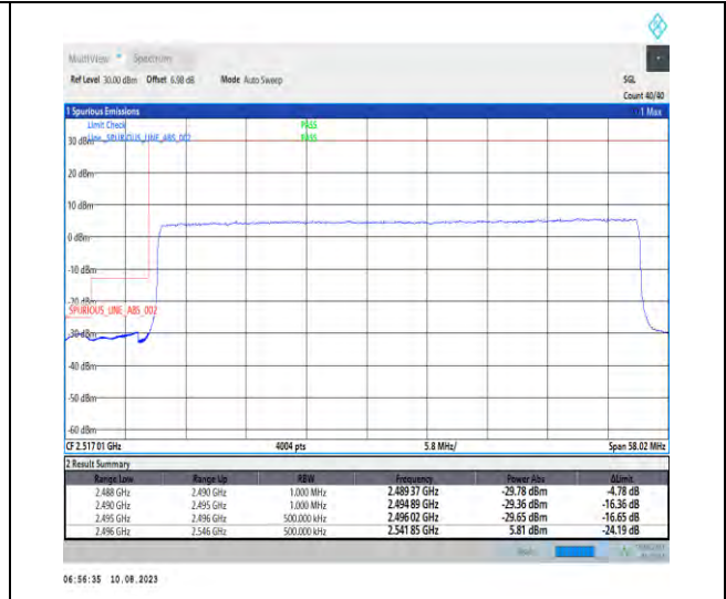
1-N41-PC3-30-50-L-3-DFT-PI2BPSK-Outer_Full-128@0-Ant1-1--PASS-see graph
