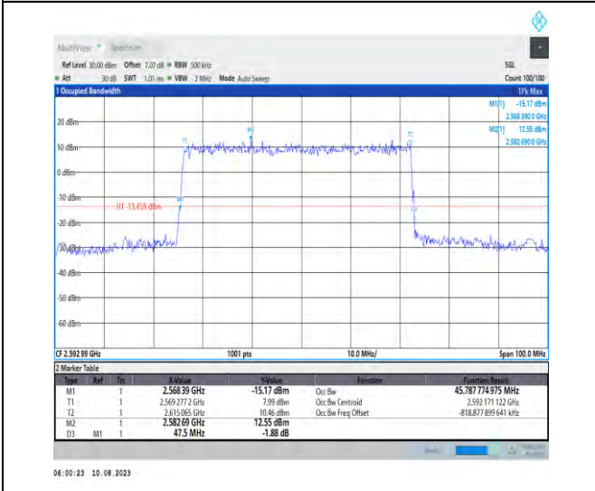
1-N41-PC3-30-50-M-4-DFT-64QAM-Outer_Full-128 @0-Ant1-45.788-47.500-≤50-PASS
