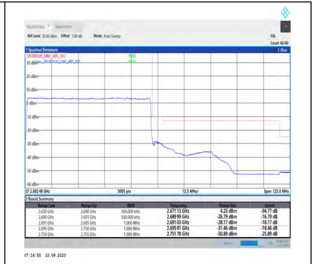
1-N41-PC3-30-60-H-3-DFT-PI2BPSK-Outer_Full-162@0-Ant1-1--PASS-see graph
