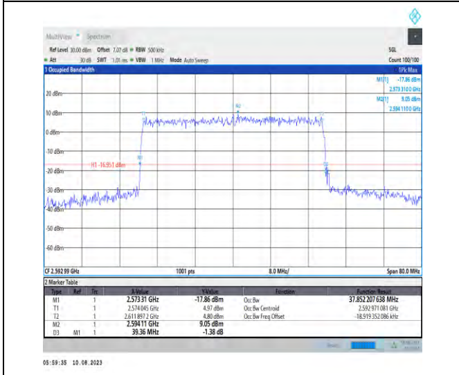
1-N41-PC3-30-40-M-9-CP-256QAM-Outer_Full-106@ @0-Ant1-37.852-39.360-<40-PASS
