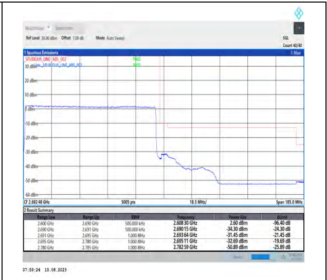
1-N41-PC3-30-90-H-3-DFT-PI2BPSK-Outer_Full-240@0-Ant1-1--PASS-see graph
