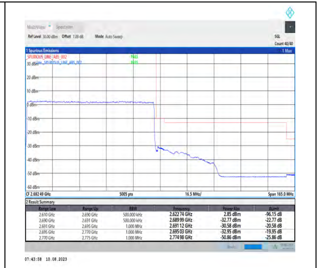
1-N41-PC3-30-80-H-3-DFT-PI2BPSK-Outer_Full-216@0-Ant1-1--PASS-see graph
