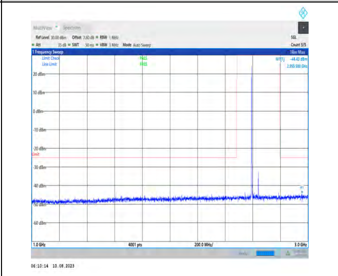
1-N41-PC3-30-100-H-1-N/A-DFT-PI2BPSK-Inner_1R B_Left-1@1-1000-3000-Ant1-2931.50--44.43--25-PA SS
