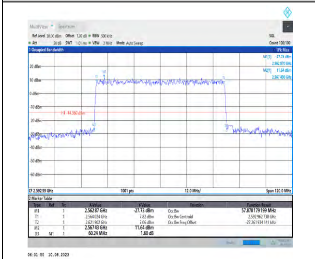
1-N41-PC3-30-60-M-3-DFT-16QAM-Outer_Full-162 @0-Ant1-57.878-60.240-≤60-PASS
