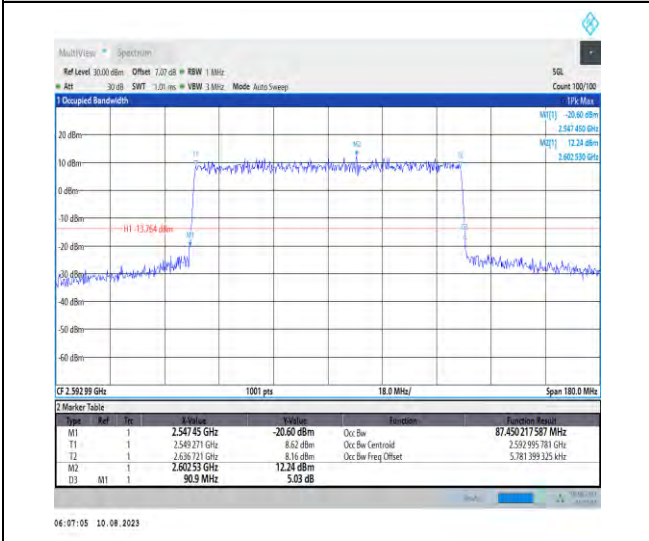
1-N41-PC3-30-90-M-8-CP-64QAM-Outer_Full-245 @0-Ant1-87.45-90.900-≤90-PASS
