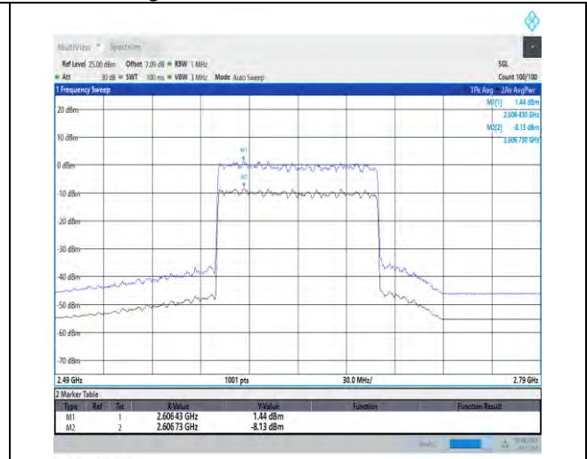
1-N41-PC3-30-100-H-2-CP-256QAM-Outer_Full-27 3@0-Ant1-9.57-100%-0.00-9.57-PASS-≤13
