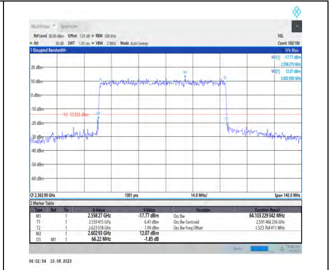
1-N41-PC3-30-70-M-1-DFT-QPSK-Outer_Full-180@ 0-Ant1-64.103-66.220-≤70-PASS
