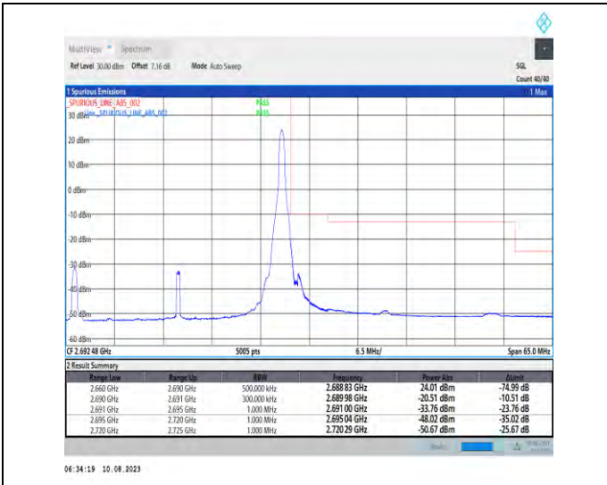
1-N41-PC3-30-30-H-2-DFT-PI2BPSK-Edge_1RB_Right-t1@77-Ant1-1--PASS-see graph
