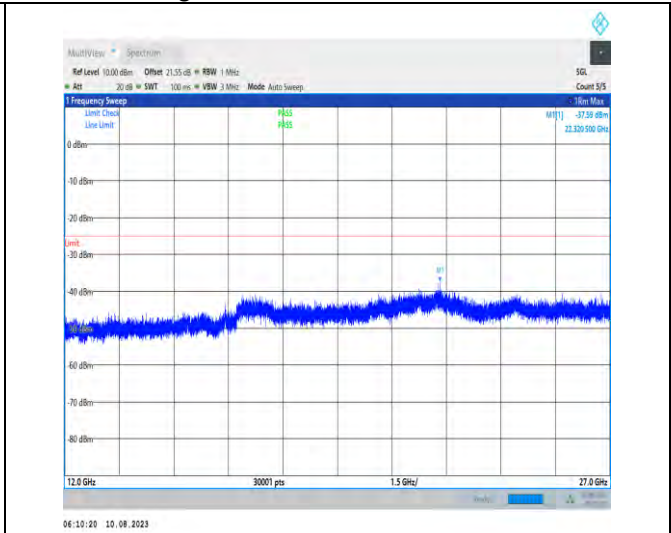
1-N41-PC3-30-100-H-1-N/A-DFT-PI2BPSK-Inner_1R B_Left-1@1-12000-27000-Ant1-22349.00--37.59--25 PASS
