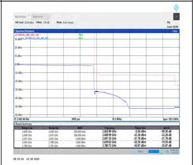
1-N41-PC3-30-90-H-6-CP-QPSK-Outer_Full-245@0-Ant1-1--PASS-see graph
