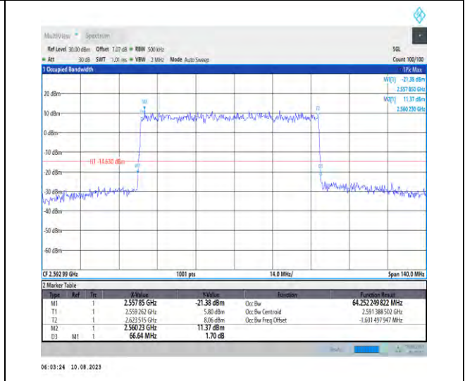
1-N41-PC3-30-70-M-3-DFT-16QAM-Outer_Full-180 @0-Ant1-64.252-66.640-≤70-PASS
