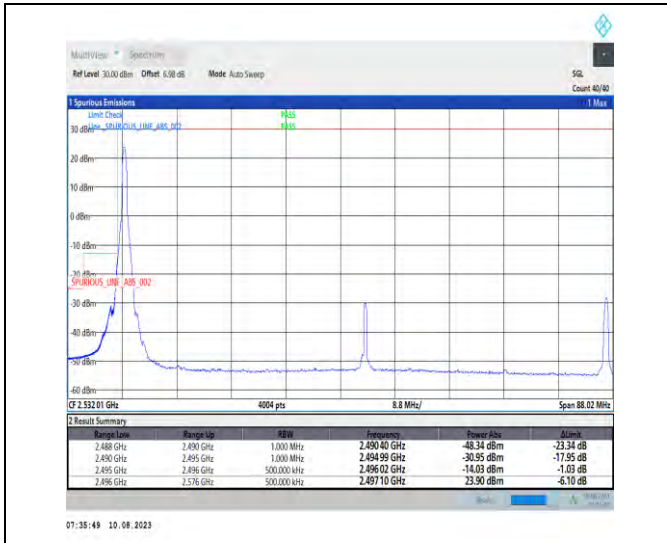
1-N41-PC3-30-80-L-1-DFT-PI2BPSK-Edge_1RB_Left-1@0-Ant1-1--PASS-see graph
