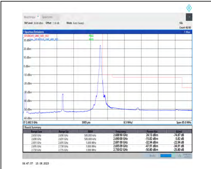
1-N41-PC3-30-40-H-2-DFT-PI2BPSK-Edge_1RB_Right-t-1@105-Ant1-1--PASS-see graph
