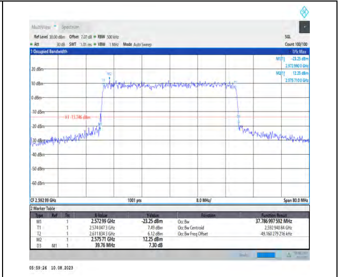
1-N41-PC3-30-40-M-8-CP-64QAM-Outer_Full-106@ @0-Ant1-37.787-39.760-<40-PASS
