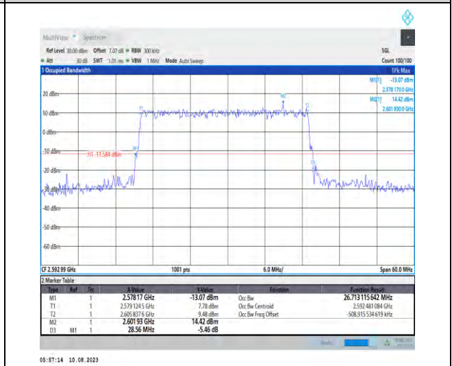
1-N41-PC3-30-30-M-3-DFT-16QAM-Outer_Full-75 @0-Ant1-26.713-28.560-<30-PASS
