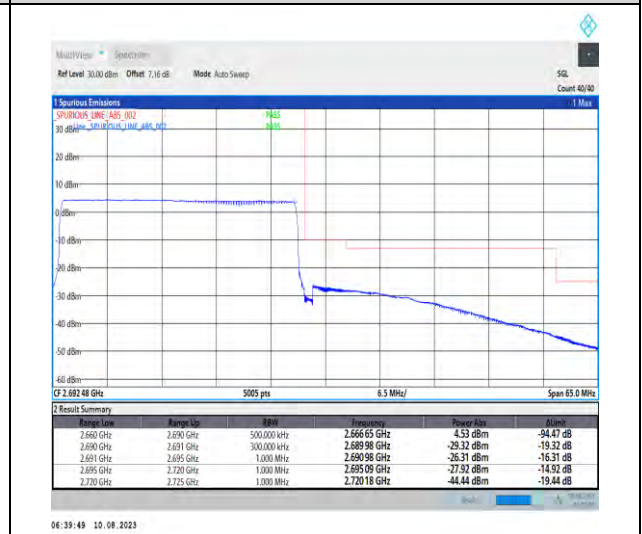
1-N41-PC3-30-30-H-6-CP-QPSK-Outer_Full-78@0-Ant1-1--PASS-see graph
