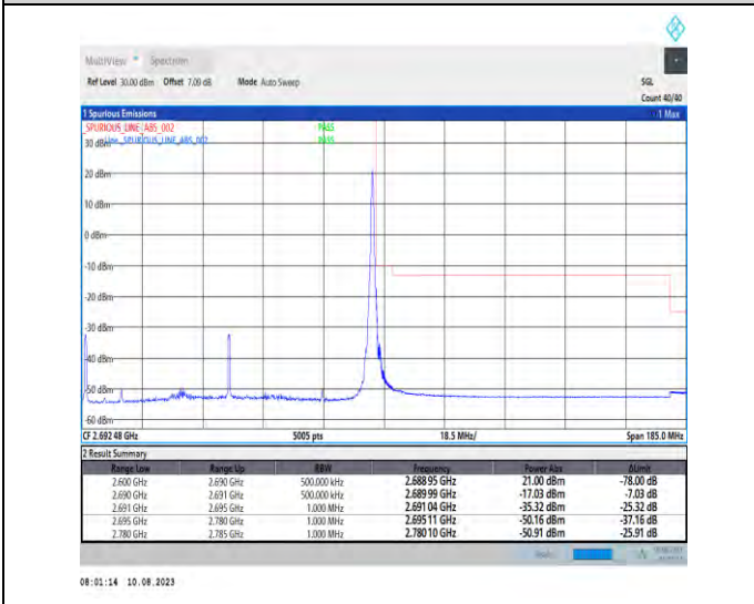
1-N41-PC3-30-90-H-5-CP-QPSK-Edge_1RB_Right-1@244-Ant1-1--PASS-see graph
