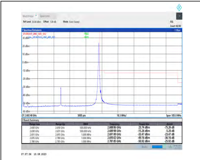
1-N41-PC3-30-90-H-2-DFT-PI2BPSK-Edge_1RB_Right-t-1@244-Ant1-1--PASS-see graph
