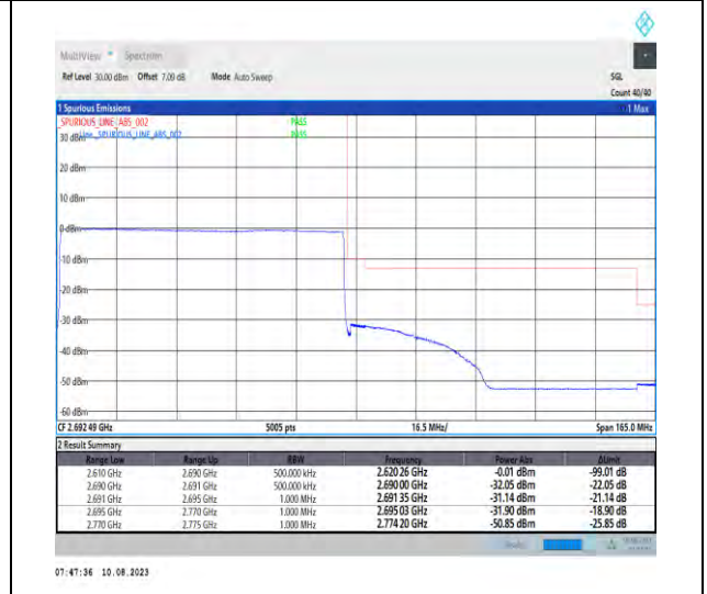
1-N41-PC3-30-80-H-6-CP-QPSK-Outer_Full-217@0-Ant1-1--PASS-see graph
