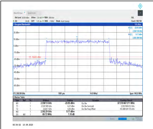
1-N41-PC3-30-70-M-8-CP-64QAM-Outer_Full-189 @0-Ant1-67.51-69.720-<=70-PASS
