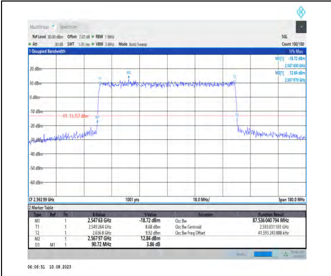
1-N41-PC3-30-90-M-6-CP-QPSK-Outer_Full-245@ 0-Ant1-87.536-90.720-≤90-PASS
