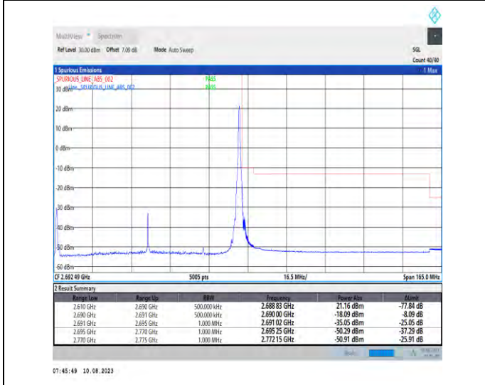
1-N41-PC3-30-80-H-5-CP-QPSK-Edge_1RB_Right-1@216-Ant1-1--PASS-see graph
