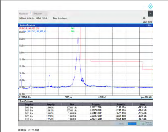
1-N41-PC3-30-30-H-5-CP-QPSK-Edge_1RB_Right-1@77-Ant1-1--PASS-see graph
