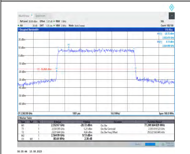
1-N41-PC3-30-80-M-9-CP-256QAM-Outer_Full-217 @0-Ant1-77.249-80.640-<80-PASS
