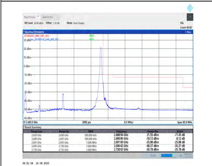
1-N41-PC3-30-40-H-5-CP-QPSK-Edge_1RB_Right-1@105-Ant1-1--PASS-see graph
