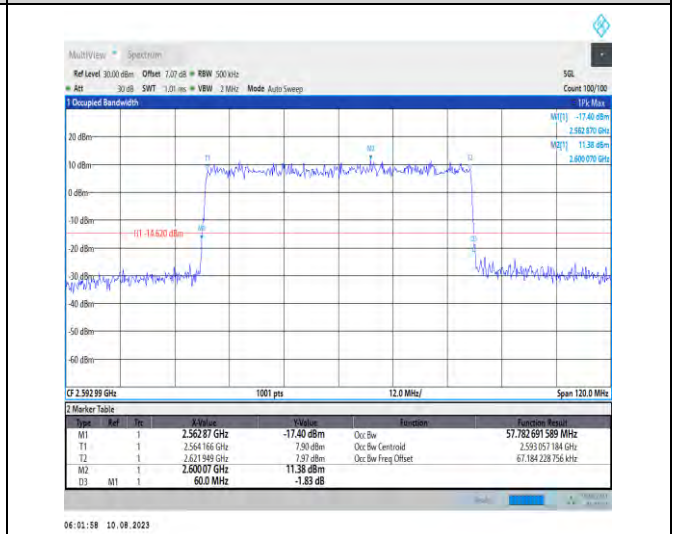
1-N41-PC3-30-60-M-4-DFT-64QAM-Outer_Full-162 @0-Ant1-57.783-60.000-≤60-PASS
