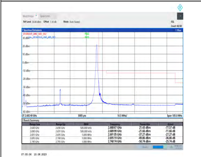
1-N41-PC3-30-50-H-5-CP-QPSK-Edge_1RB_Right-1@132-Ant1-1--PASS-see graph
