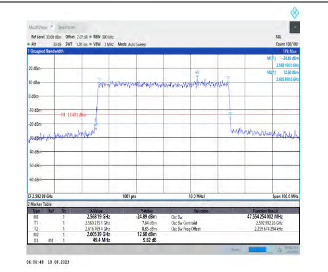
1-N41-PC3-30-50-M-7-CP-16QAM-Outer_Full-133@0-Ant1-47.554-49.400-<=50-PASS
