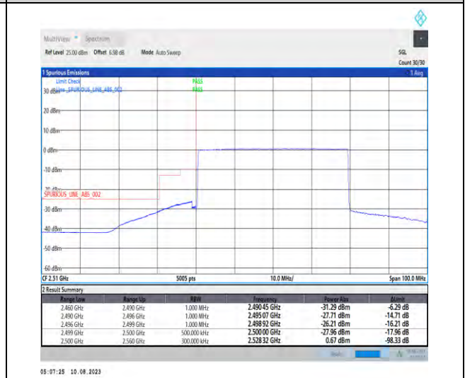
1-N7-PC3-15-40-L-6-CP-QPSK-Outer_Full-216@0-Ant1-1--PASS-see graph
