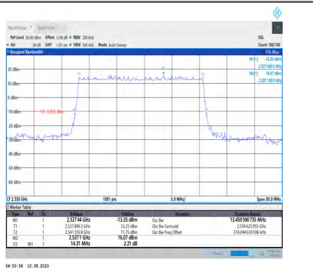
1-N7-PC3-15-15-M-2-DFT-PI2BPSK-Outer_Full-75@0 Ant1-13.46-14.310-≤15-PASS
