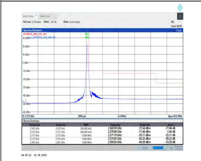
1-N7-PC3-15-25-H-5-CP-QPSK-Edge_1RB_Right-1@132-Ant1-1--PASS-see graph
