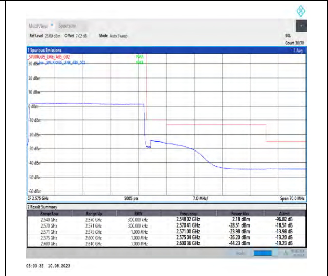
1-N7-PC3-15-30-H-6-CP-QPSK-Outer_Full-160@0-Ant1-1--PASS-see graph
