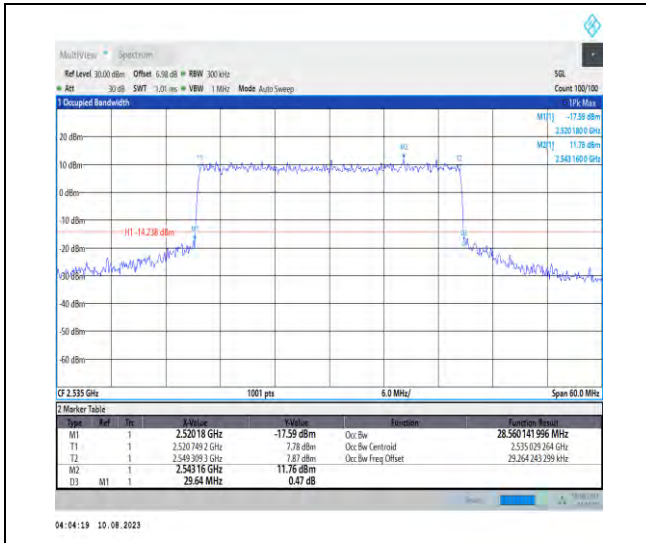
1-N7-PC3-15-30-M-8-CP-64QAM-Outer_Full-160@ 0-Ant1-28.56-29.640-≤30-PASS
