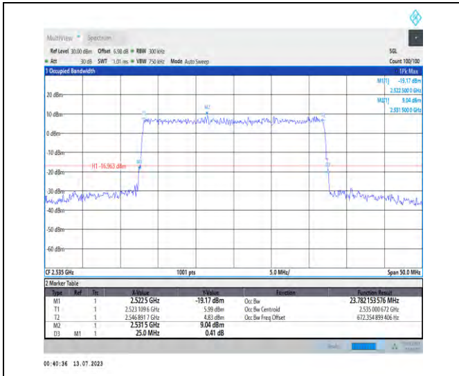
1-N7-PC3-15-25-M-9-CP-256QAM-Outer_Full-133@ 0-Ant1-23.782-25.000-≤25-PASS
