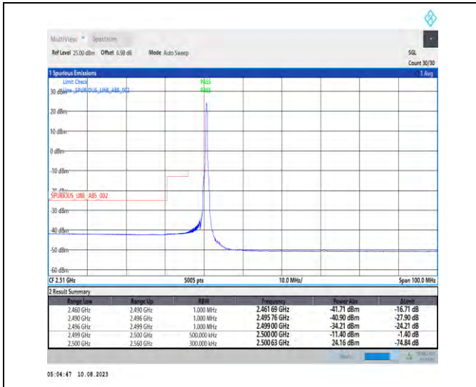
1-N7-PC3-15-40-L-1-DFT-PI2BPSK-Edge_1RB_Left-1@0-Ant1-1--PASS-see graph
