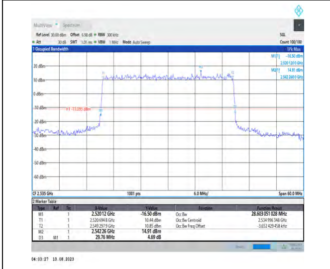
1-N7-PC3-15-30-M-2-DFT-PI2BPSK-Outer_Full-160 @0-Ant1-28.603-29.760-≤30-PASS
