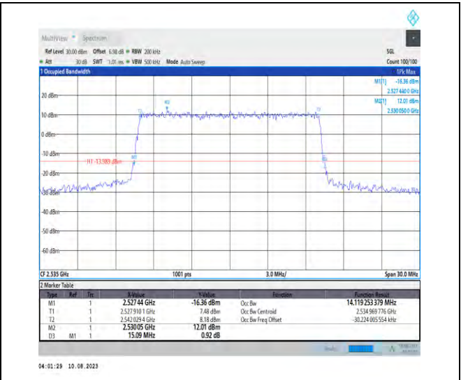
1-N7-PC3-15-15-M-8-CP-64QAM-Outer_Full-79@0- Ant1-14.119-15.090-≤15-PASS
