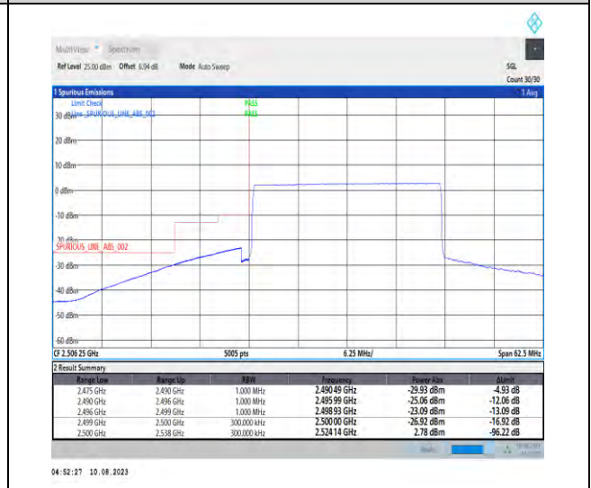
1-N7-PC3-15-25-L-6-CP-QPSK-Outer_Full-133@0-Ant1-1--PASS-see graph
