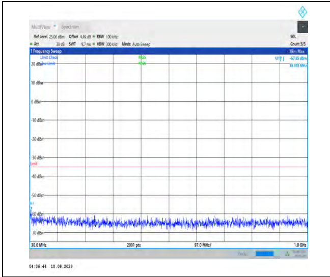
1-N7-PC3-15-40-M-1-N/A-DFT-PI2BPSK-Inner_1RB _Left-1@1-30-1000-Ant1-34.85--57.85--35-PASS
