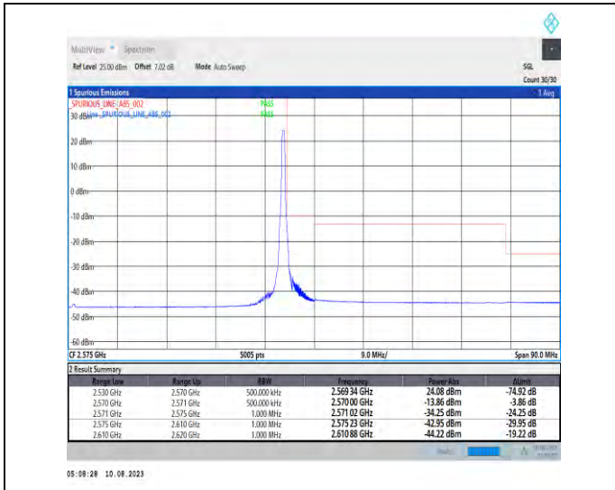
1-N7-PC3-15-40-H-2-DFT-PI2BPSK-Edge_1RB_Right-1@215-Ant1-1--PASS-see graph
