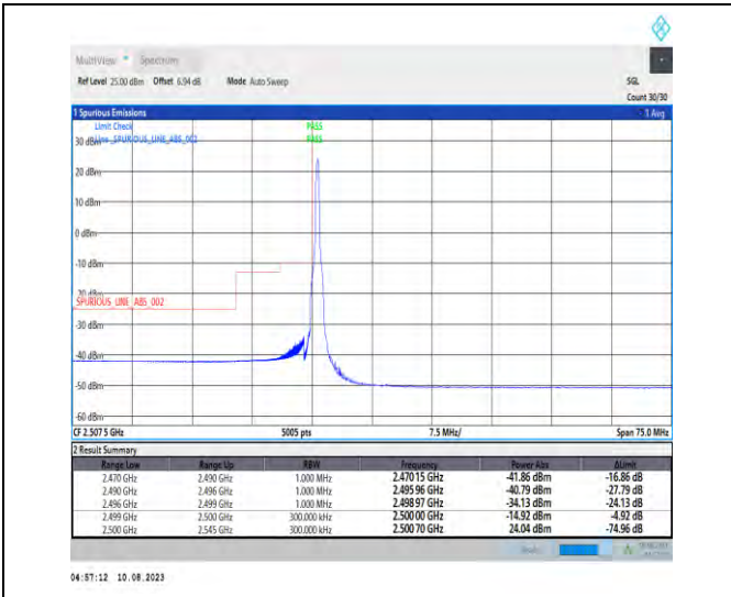
1-N7-PC3-15-30-L-1-DFT-PI2BPSK-Edge_1RB_Left-1@0-Ant1-1--PASS-see graph
