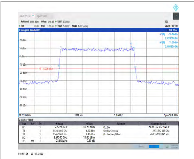
1-N7-PC3-15-25-M-5-DFT-256QAM-Outer_Full-128 @0-Ant1-22.884-23.850-≤25-PASS
