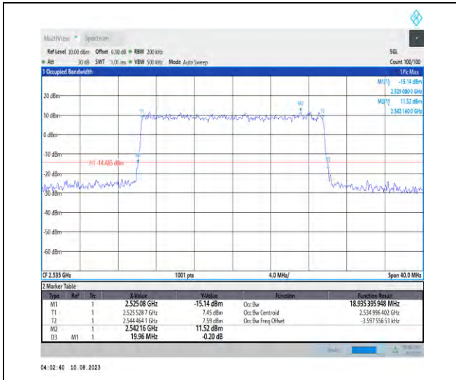
1-N7-PC3-15-20-M-6-CP-QPSK-Outer_Full-106@0-Ant1-18.935-19.960-<20-PASS
