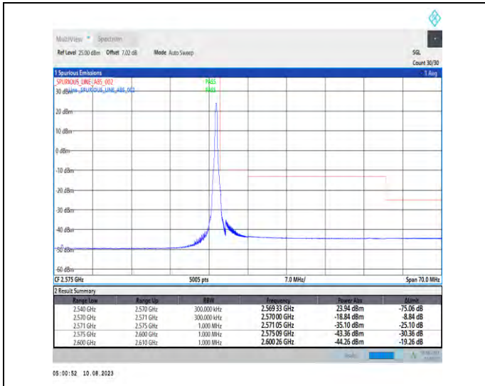
1-N7-PC3-15-30-H-2-DFT-PI2BPSK-Edge_1RB_Right-1@159-Ant1-1--PASS-see graph
