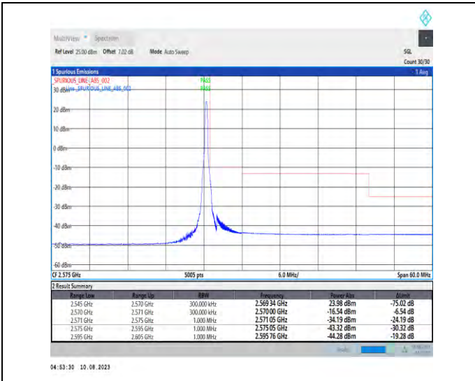
1-N7-PC3-15-25-H-2-DFT-PI2BPSK-Edge_1RB_Right-1@132-Ant1-1--PASS-see graph
