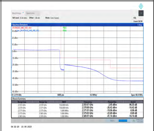
1-N7-PC3-15-15-H-6-CP-QPSK-Outer_Full-79@0-Ant1-1--PASS-see graph
