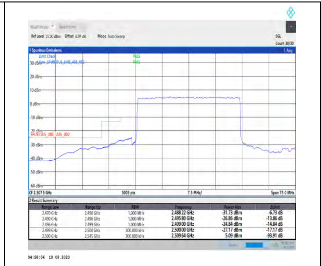
1-N7-PC3-15-30-L-3-DFT-PI2BPSK-Outer_Full-160@0-Ant1-1--PASS-see graph
