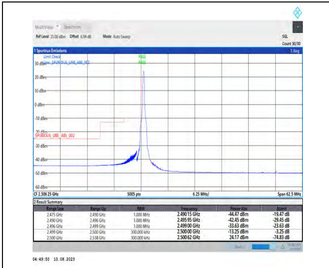
1-N7-PC3-15-25-L-1-DFT-PI2BPSK-Edge_1RB_Left-1@0-Ant1-1--PASS-see graph
