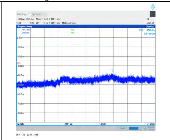
1-N7-PC3-15-40-H-1-N/A-DFT-PI2BPSK-Inner_1RB Left-1@1-12000-27000-Ant1-22296.00--37.49--25-PA SS
