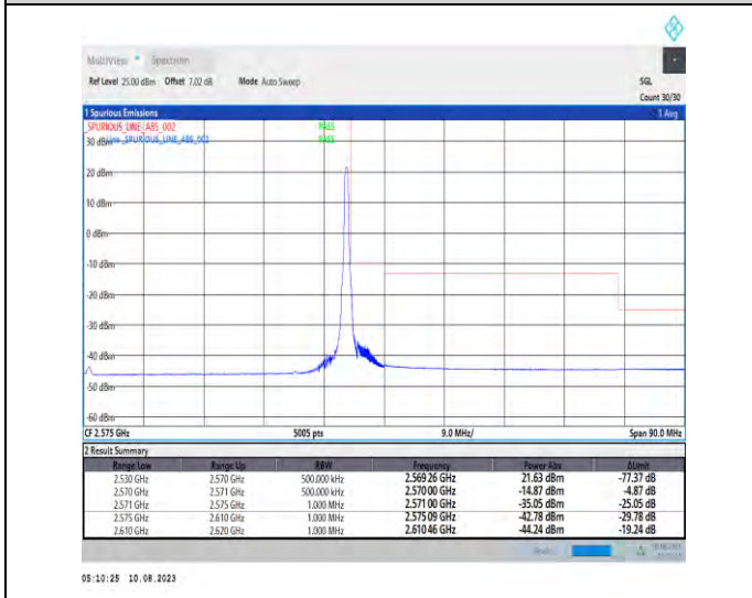
1-N7-PC3-15-40-H-5-CP-QPSK-Edge_1RB_Right-1@215-Ant1-1--PASS-see graph
