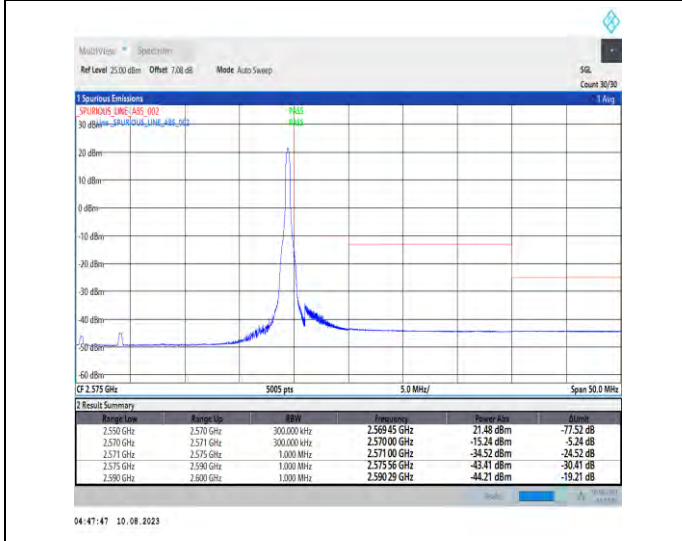
1-N7-PC3-15-20-H-5-CP-QPSK-Edge_1RB_Right-1@105-Ant1-1--PASS-see graph
