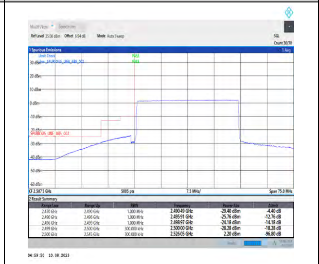
1-N7-PC3-15-30-L-6-CP-QPSK-Outer_Full-160@0-Ant1-1--PASS-see graph
