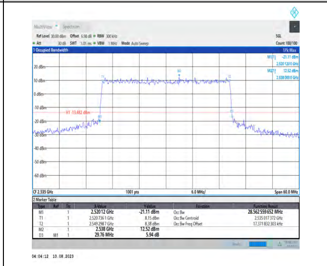
1-N7-PC3-15-30-M-7-CP-16QAM-Outer_Full-160@0- Ant1-28.563-29.760-≤30-PASS
