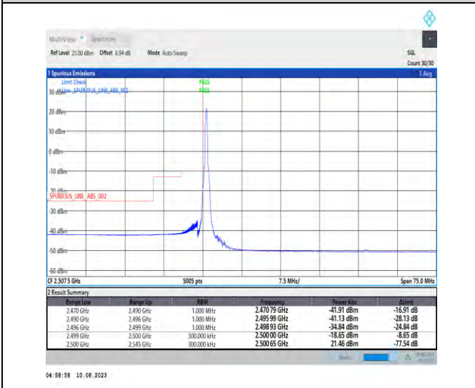
1-N7-PC3-15-30-L-4-CP-QPSK-Edge_1RB_Left-1@0-Ant1-1--PASS-see graph
