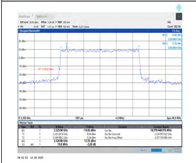
1-N7-PC3-15-20-M-8-CP-64QAM-Outer_Full-106@0-Ant1-18.978-19.800-<20-PASS
