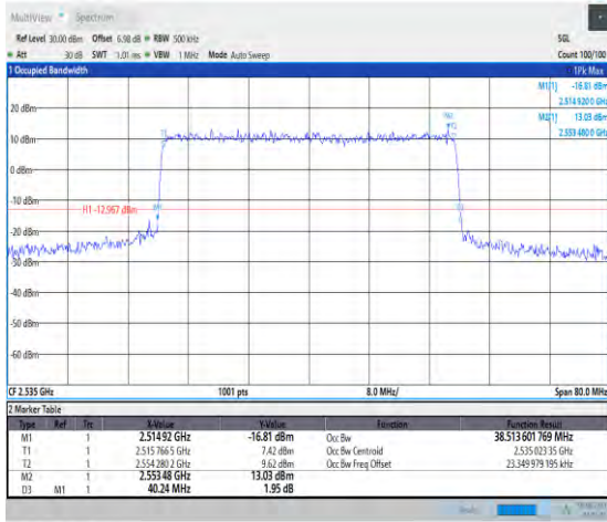
1-N7-PC3-15-40-M-7-CP-16QAM-Outer_Full-216@0 -Ant1-38.514-40.240-≤40-PASS
