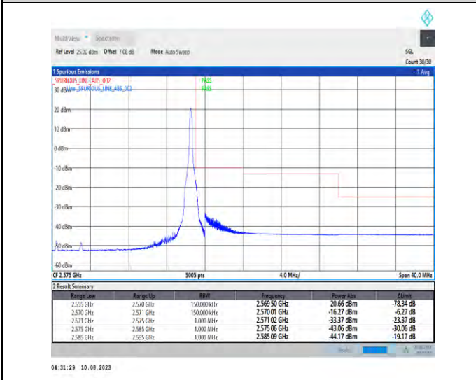
1-N7-PC3-15-15-H-5-CP-QPSK-Edge_1RB_Right-1@78-Ant1-1--PASS-see graph
