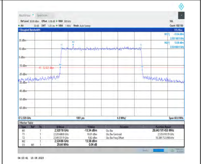
1-N7-PC3-15-30-M-3-DFT-16QAM-Outer_Full-160 @0-Ant1-28.643-29.640-≤30-PASS
