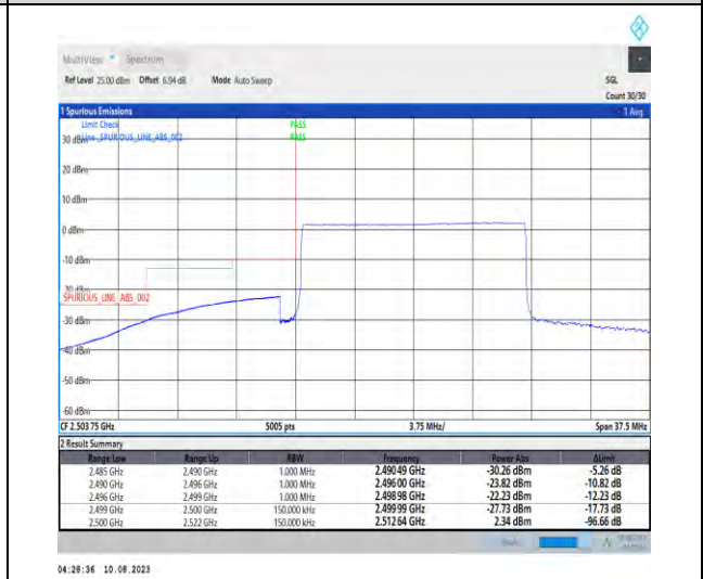
1-N7-PC3-15-15-L-6-CP-QPSK-Outer_Full-79@0- Ant1-1--PASS-see graph
