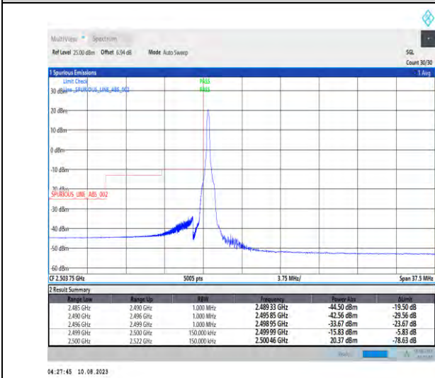
1-N7-PC3-15-15-L-4-CP-QPSK-Edge_1RB_Left-1@0- Ant1-1--PASS-see graph
