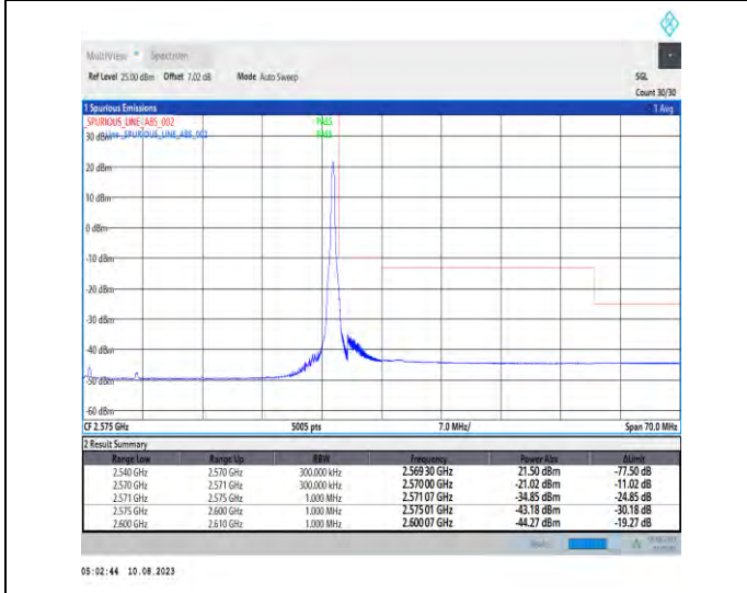
1-N7-PC3-15-30-H-5-CP-QPSK-Edge_1RB_Right-1@159-Ant1-1--PASS-see graph
