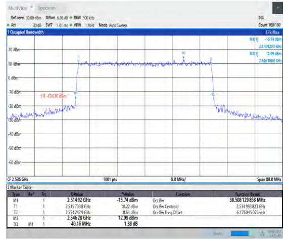
1-N7-PC3-15-40-M-8-CP-64QAM-Outer_Full-216@0 0-Ant1-38.508-40.160-≤40-PASS
