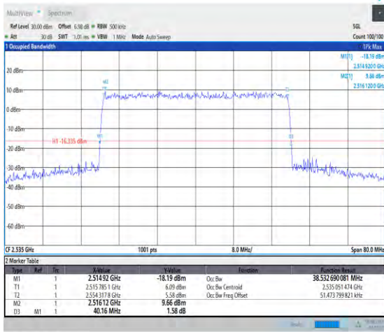
1-N7-PC3-15-40-M-9-CP-256QAM-Outer_Full-216@0 0-Ant1-38.533-40.160-≤40-PASS
