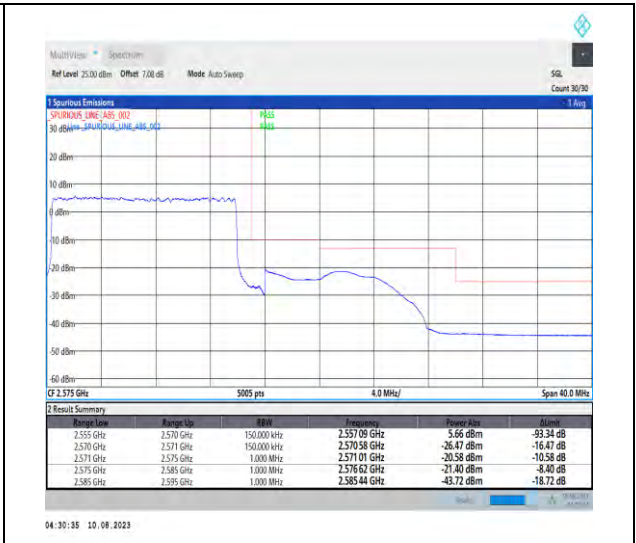
1-N7-PC3-15-15-H-3-DFT-PI2BPSK-Outer_Full-75@0-Ant1-1--PASS-see graph
