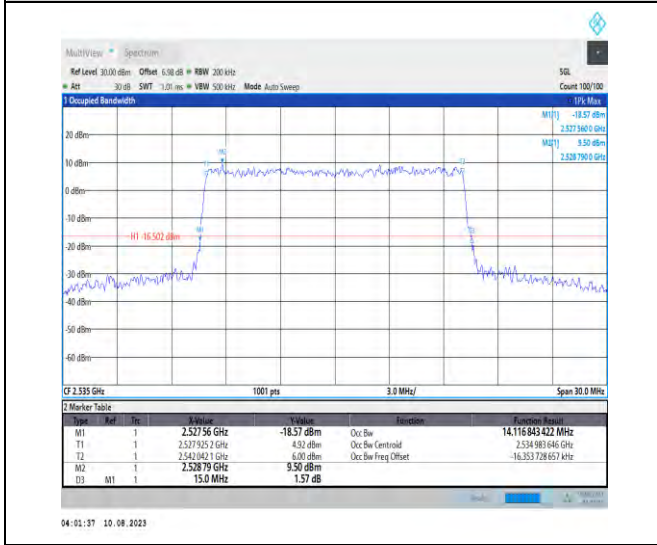
1-N7-PC3-15-15-M-9-CP-256QAM-Outer_Full-79@0 -Ant1-14.117-15.000-≤15-PASS
