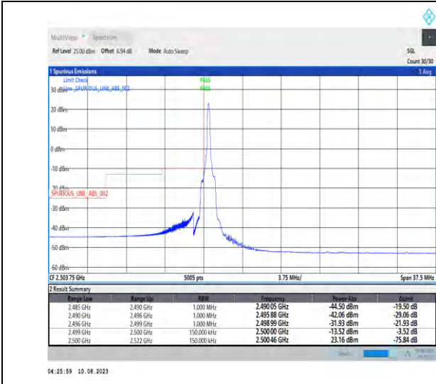
1-N7-PC3-15-15-L-1-DFT-PI2BPSK-Edge_1RB_Left-1 @0-Ant1-1--PASS-see graph
