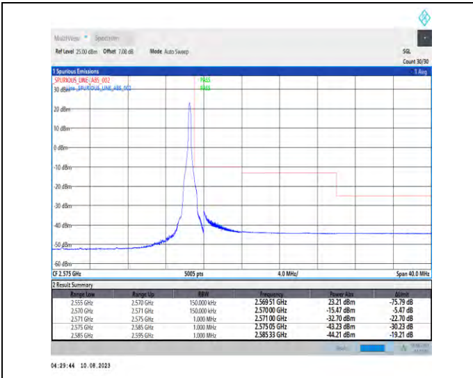
1-N7-PC3-15-15-H-2-DFT-PI2BPSK-Edge_1RB_Right-1@78-Ant1-1--PASS-see graph
