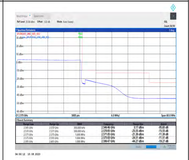
1-N7-PC3-15-25-H-6-CP-QPSK-Outer_Full-133@0-Ant1-1--PASS-see graph
