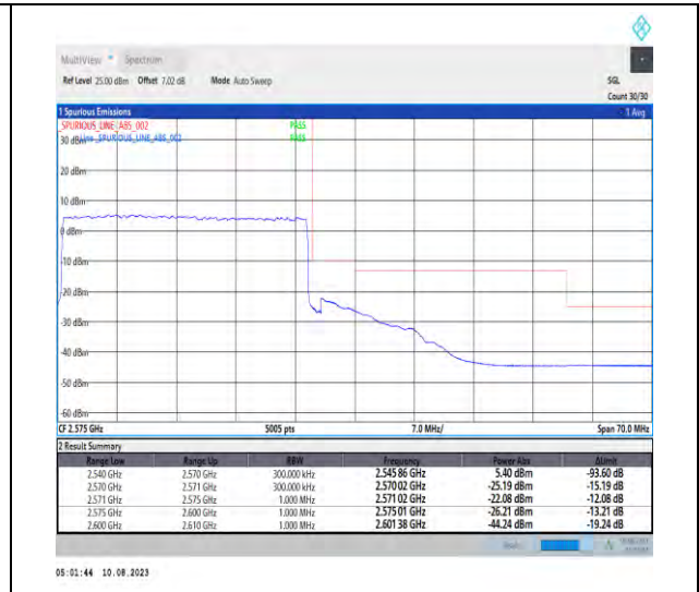
1-N7-PC3-15-30-H-3-DFT-PI2BPSK-Outer_Full-160@0-Ant1-1--PASS-see graph
