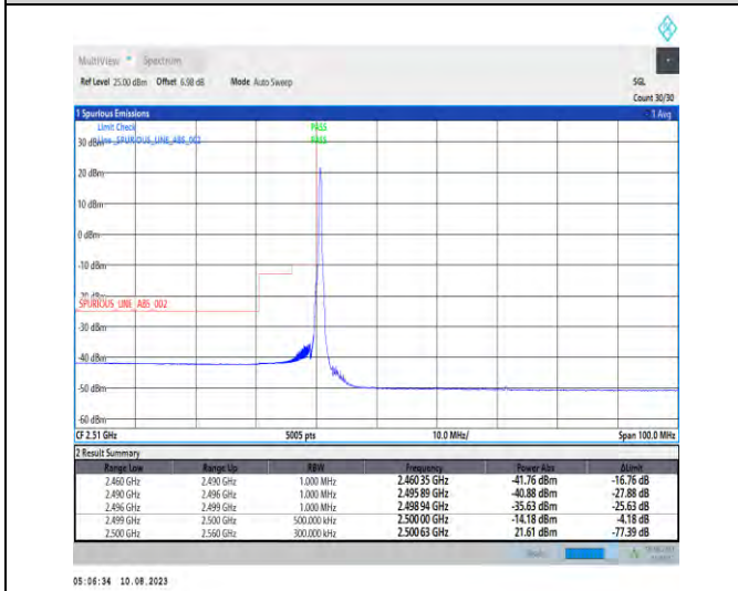
1-N7-PC3-15-40-L-4-CP-QPSK-Edge_1RB_Left-1@0-Ant1-1--PASS-see graph
