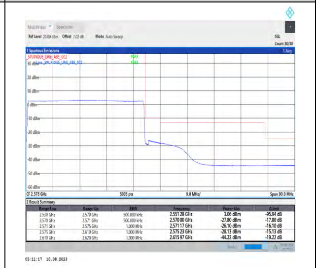
1-N7-PC3-15-40-H-6-CP-QPSK-Outer_Full-216@0-Ant1-1--PASS-see graph
