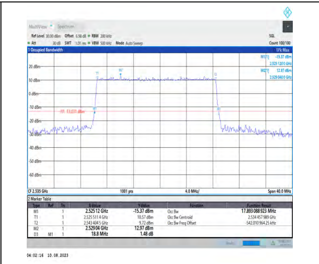
1-N7-PC3-15-20-M-3-DFT-16QAM-Outter_Full-100@ 0-Ant1-17.893-18.800-<=20-PASS
