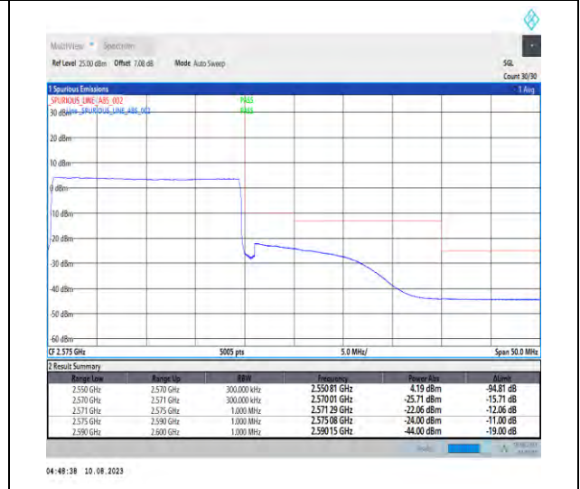
1-N7-PC3-15-20-H-6-CP-QPSK-Outer_Full-106@0-Ant1-1--PASS-see graph
