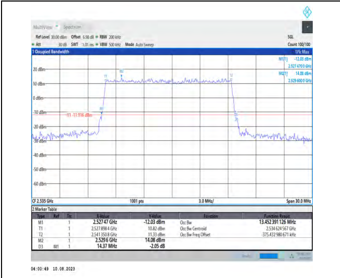
1-N7-PC3-15-15-M-3-DFT-16QAM-Outer_Full-75@0-Ant1-13.452-14.370-≤15-PASS
