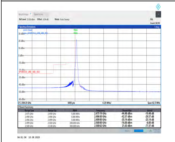
1-N7-PC3-15-25-L-4-CP-QPSK-Edge_1RB_Left-1@0-Ant1-1--PASS-see graph
