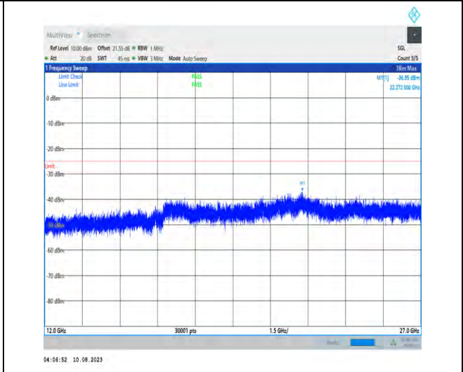
1-N7-PC3-15-40-M-1-N/A-DFT-PI2BPSK-Inner_1RB Left-1@1-12000-27000-Ant1-25855.00--36.95--25-PA
