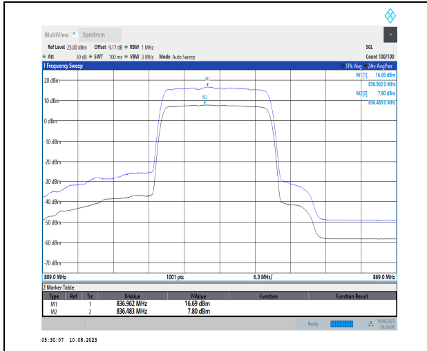
1-N5-PC3-15-20-H-1-DFT-256QAM-Outer_Full-100 @0-Ant1-8.89-100%-0.00-8.89-PASS-≤13
