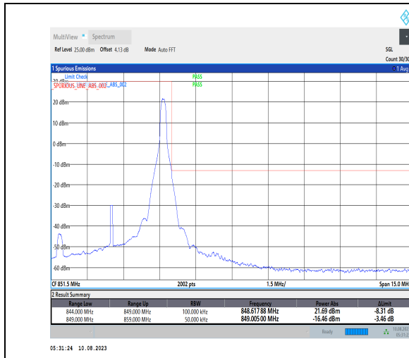
1-N5-PC3-15-5-H-2-DFT-PI2BPSK-Edge_1RB_Right-1 @24-Ant1-1-seegraph-PASS-see graph
