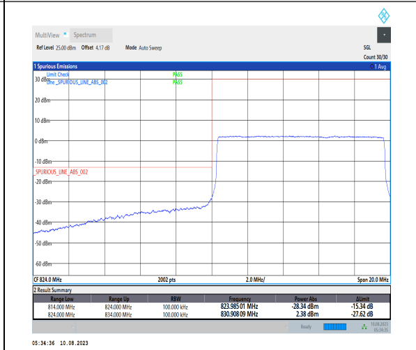
1-N5-PC3-15-10-L-6-CP-QPSK-Outer_Full-52@0-Ant1-1-seegraph-PASS-see graph
