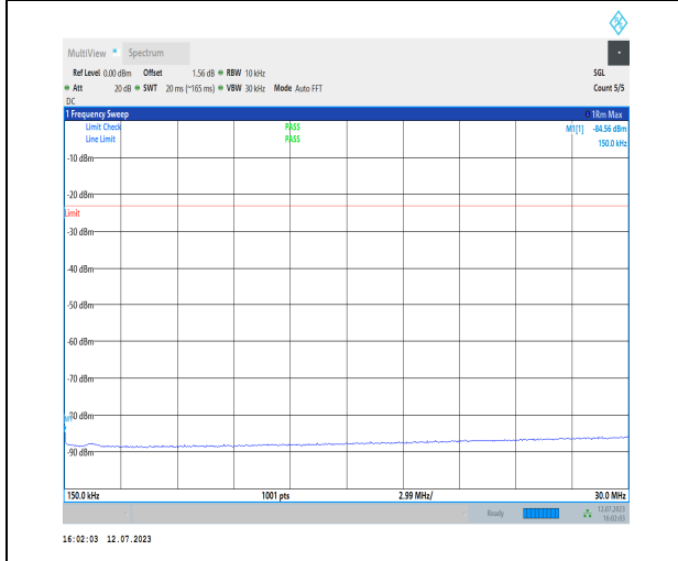
1-N5-PC3-15-20-M-1-N/A-DFT-PI2BPSK-Inner_1RB_Left-1@1-0.15-30-Ant1-0.15--84.56--23-PASS
