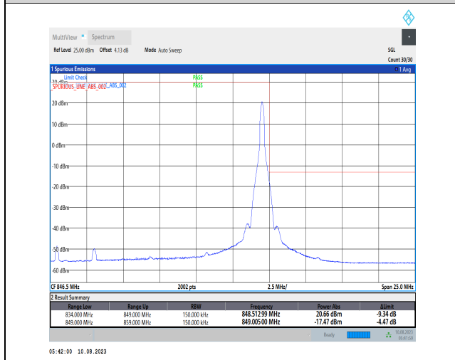
1-N5-PC3-15-15-H-5-CP-QPSK-Edge_1RB_Right-1@78-Ant1-1-seegraph-PASS-see graph
