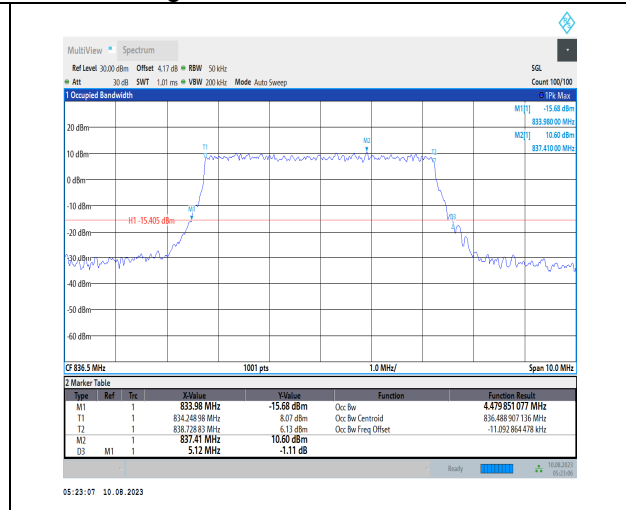
1-N5-PC3-15-5-M-6-CP-QPSK-Outer_Full-25@0-Ant 1-4.48-5.120-≤5-PASS
