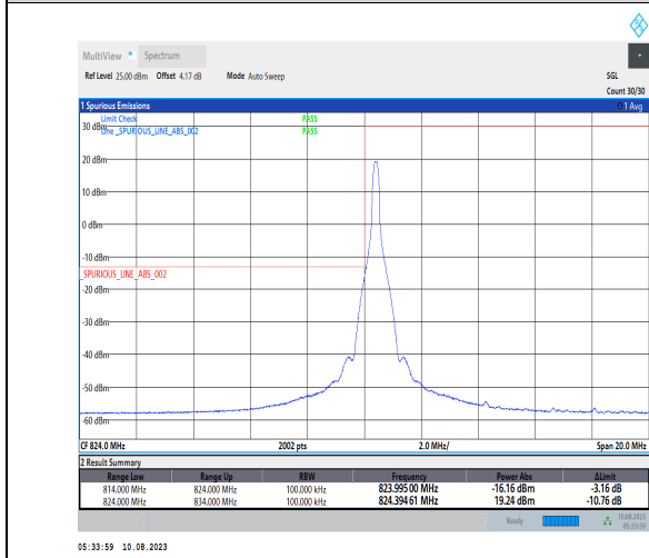
1-N5-PC3-15-10-L-4-CP-QPSK-Edge_1RB_Left-1@0-Ant1-1-seegraph-PASS-see graph
