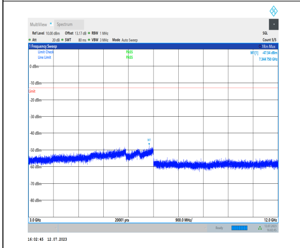
1-N5-PC3-15-20-H-1-N/A-DFT-PI2BPSK-Inner_1RB _Left-1@1-3000-12000-Ant1-7344.75--47.54--13-PA SS
