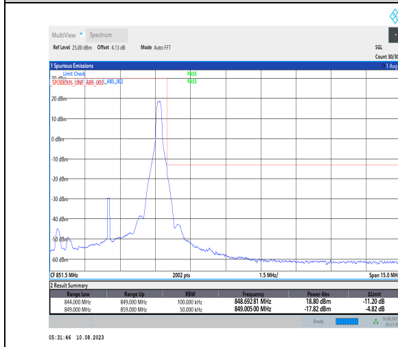
1-N5-PC3-15-5-H-5-CP-QPSK-Edge_1RB_Right-1@2 4-Ant1-1-seegraph-PASS-see graph
