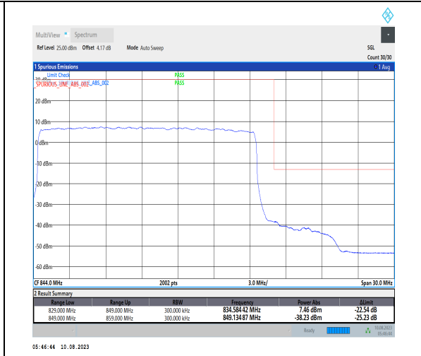
1-N5-PC3-15-20-H-3-DFT-PI2BPSK-Outer_Full-100@0-Ant1-1-seegraph-PASS-see graph
