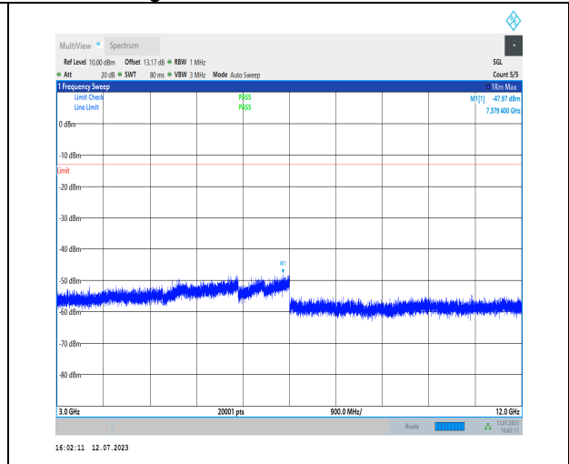
1-N5-PC3-15-20-M-1-N/A-DFT-PI2BPSK-Inner_1RB_Left-1@1-3000-12000-Ant1-7379.40--47.97--13-PA SS
