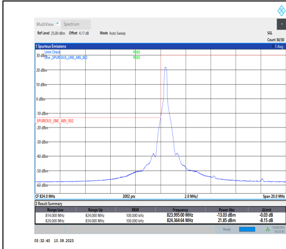
1-N5-PC3-15-10-L-1-DFT-PI2BPSK-Edge_1RB_Left-1@0-Ant1-1-seegraph-PASS-see graph
