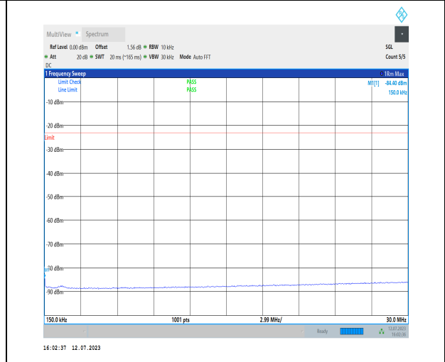
1-N5-PC3-15-20-H-1-N/A-DFT-PI2BPSK-Inner_1RB_Left-1@1-0.15-30-Ant1-0.15--84.40--23-PASS
