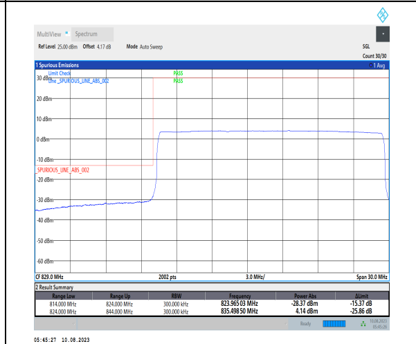
1-N5-PC3-15-20-L-6-CP-QPSK-Outer_Full-106@0-Ant1-1-seegraph-PASS-see graph
