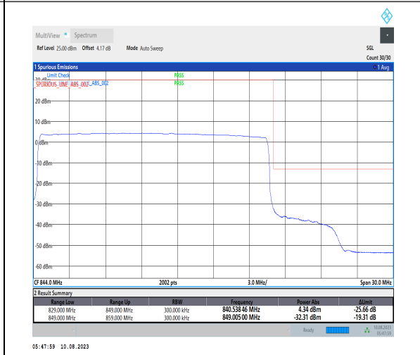
1-N5-PC3-15-20-H-6-CP-QPSK-Outer_Full-106@0-Ant1-1-seegraph-PASS-see graph
