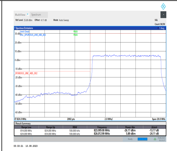
1-N5-PC3-15-10-L-3-DFT-PI2BPSK-Outer_Full-50@0-Ant1-1-seegraph-PASS-see graph
