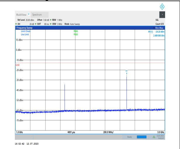
1-N5-PC3-15-20-H-1-N/A-DFT-PI2BPSK-Inner_1RB _Left-1@1-1000-3000-Ant1-2489.50--24.20--13-PAS S
