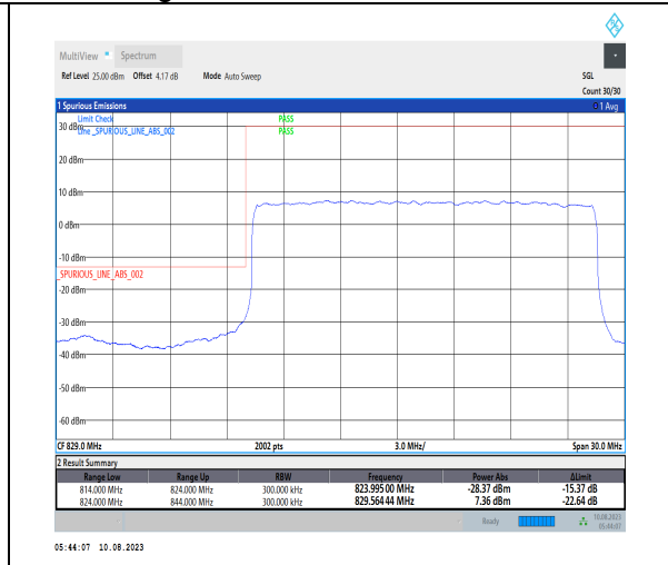
1-N5-PC3-15-20-L-3-DFT-PI2BPSK-Outer_Full-10@0-Ant1-1-seegraph-PASS-see graph
