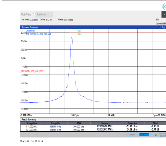
1-N5-PC3-15-20-L-1-DFT-PI2BPSK-Edge_1RB_Left-1@0-Ant1-1-seegraph-PASS-see graph
