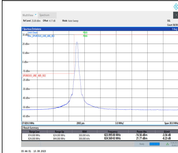
1-N5-PC3-15-20-L-4-CP-QPSK-Edge_1RB_Left-1@0-Ant1-1-seegraph-PASS-see graph
