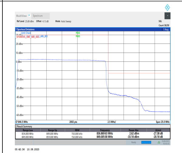
1-N5-PC3-15-15-H-6-CP-QPSK-Outer_Full-79@0-Ant1-1-seegraph-PASS-see graph
