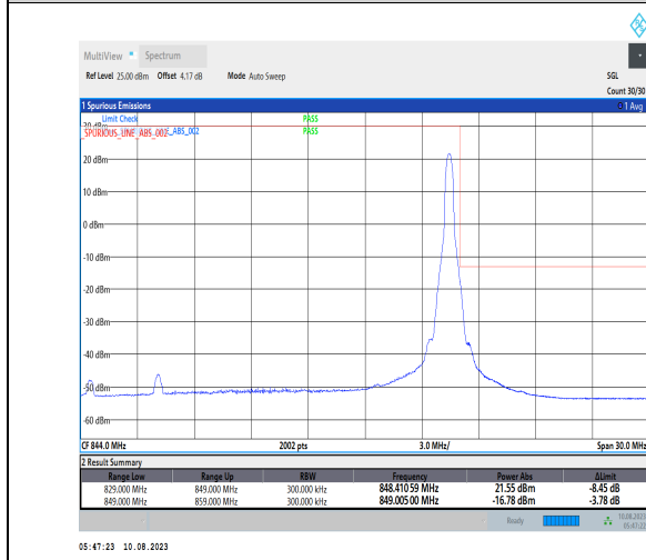
1-N5-PC3-15-20-H-5-CP-QPSK-Edge_1RB_Right-1@105-Ant1-1-seegraph-PASS-see graph
