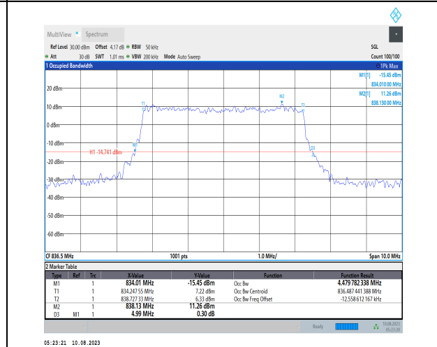
1-N5-PC3-15-5-M-8-CP-64QAM-Outer_Full-25@0-A nt1-4.48-4.990-≤5-PASS
