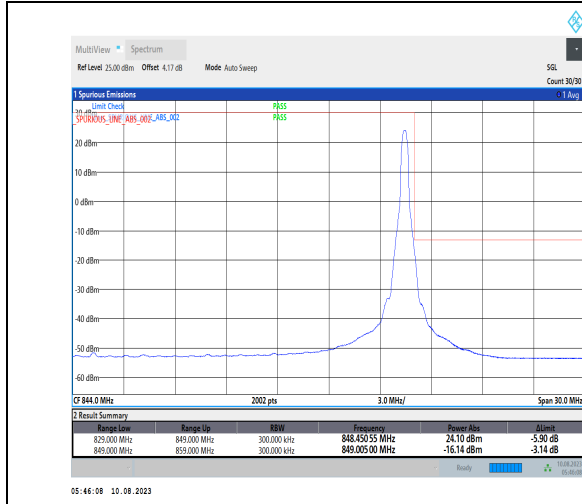
1-N5-PC3-15-20-H-2-DFT-PI2BPSK-Edge_1RB_Right-1@105-Ant1-1-seegraph-PASS-see graph
