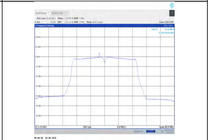
11ac40MIMO-Ant12-5190
