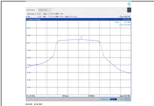
11a-CDD-Ant11-5260
