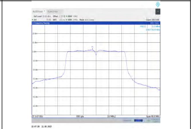
11ac40MIMO-Ant12-5670
