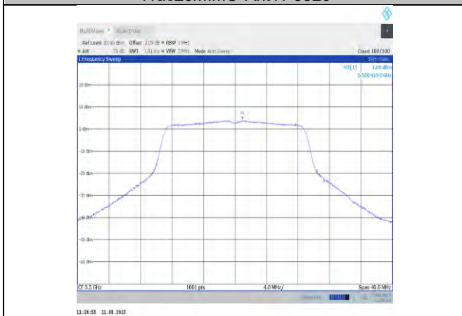
11ac20MIMO-Ant11-5500
