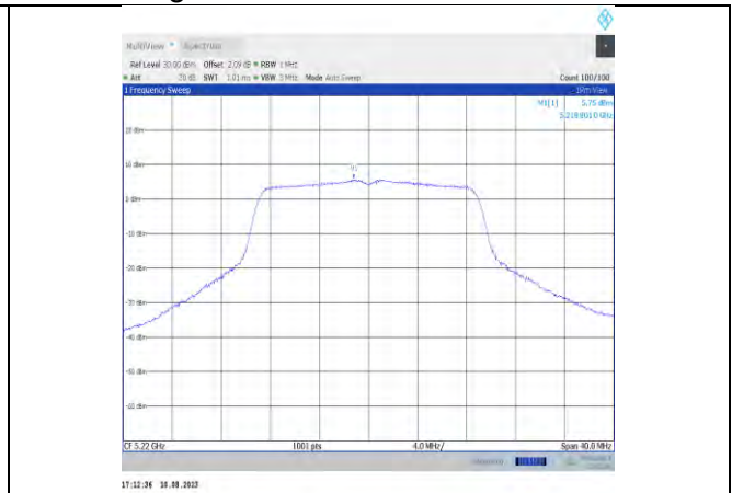
11ac20MIMO-Ant12-5220
