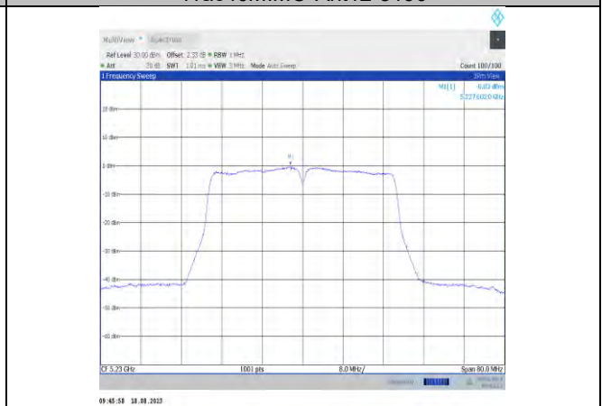
11ac40MIMO-Ant12-5230
