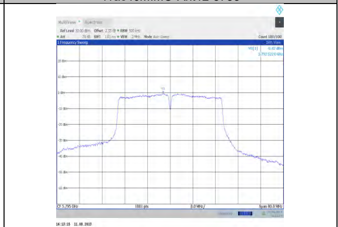
11ac40MIMO-Ant12-5795
