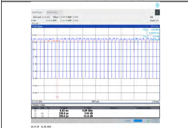
NTVN-11ac80MIMO-Ant11-5210
