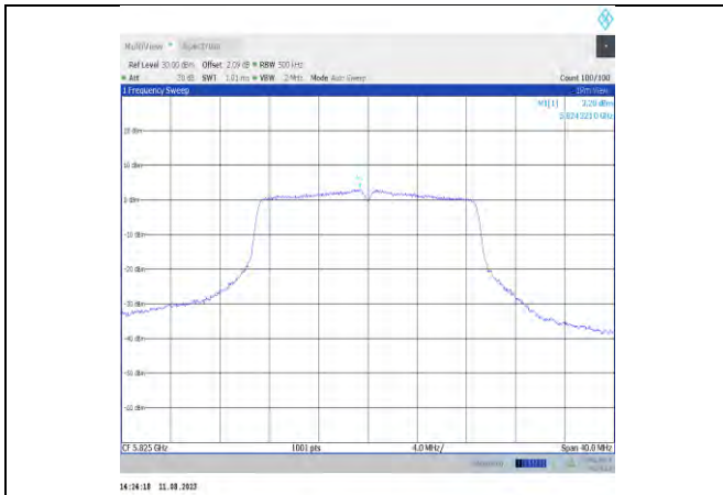
11ac20MIMO-Ant11-5825
