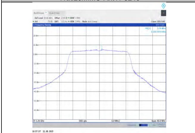
11ac20MIMO-Ant11-5260
