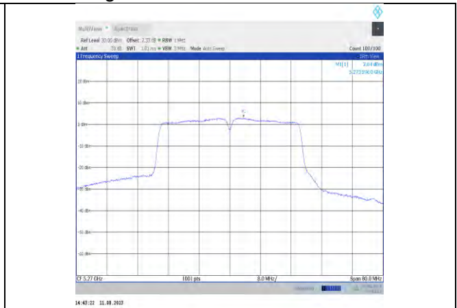
11ac40MIMO-Ant12-5270
