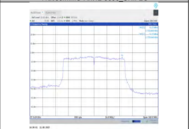
11ac80MIMO-Ant12-5690 UNII-3
