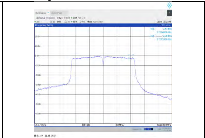
11ac40MIMO-Ant12-5710 UNII-3
