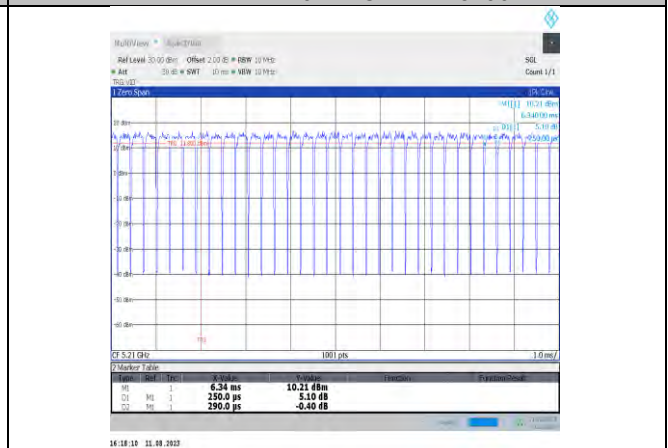
NTVN-11ac80MIMO-Ant12-5210
