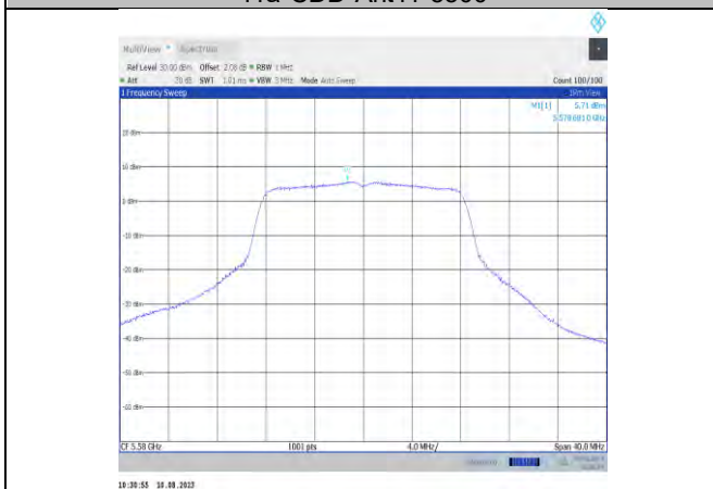
11a-CDD-Ant11-5580
