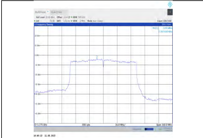
11ac80MIMO-Ant11-5775
