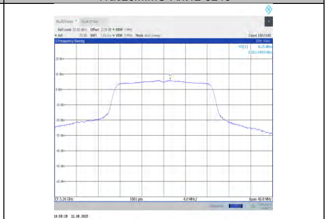
11ac20MIMO-Ant12-5260
