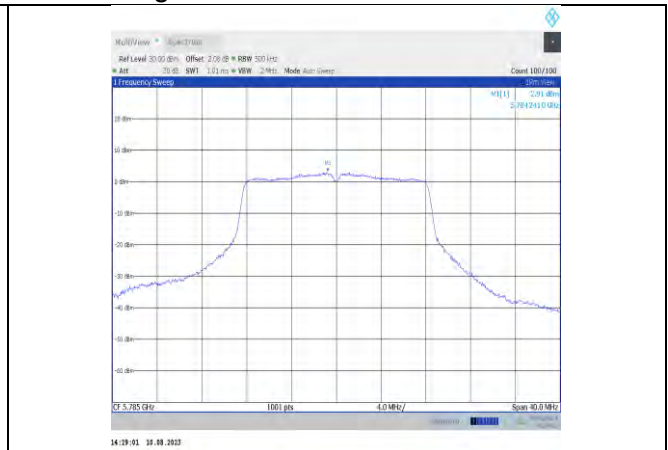
11a-CDD-Ant12-5785
