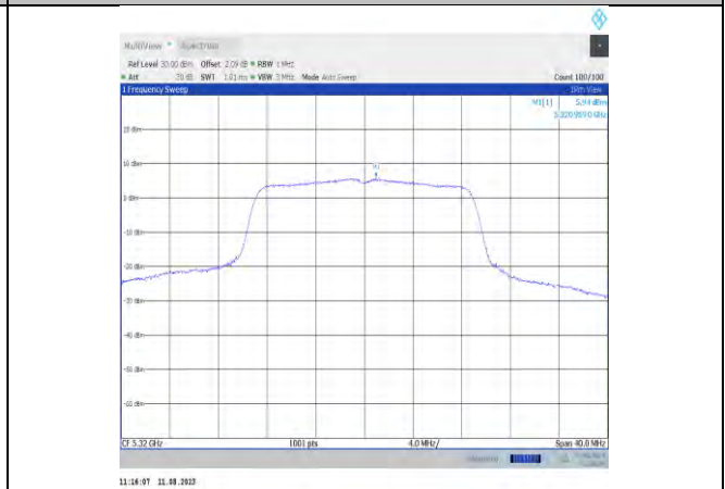
11ac20MIMO-Ant12-5320
