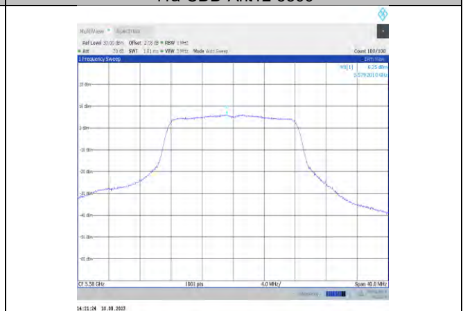
11a-CDD-Ant12-5580
