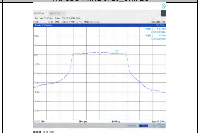
11a-CDD-Ant12-5720_UNII-3
