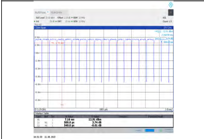
NTVN-11ac40MIMO-Ant11-5190
