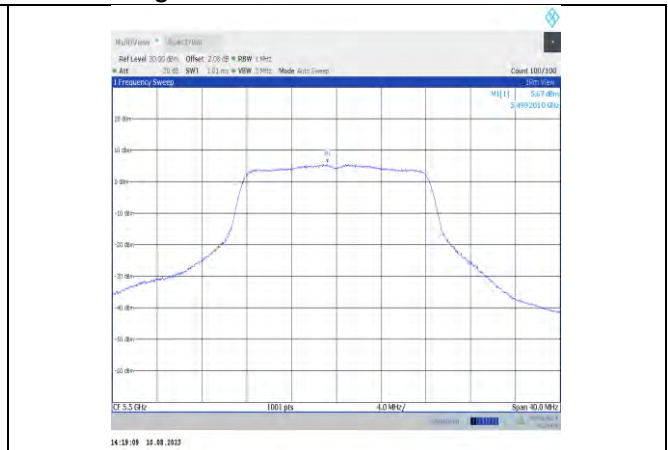
11a-CDD-Ant12-5500
