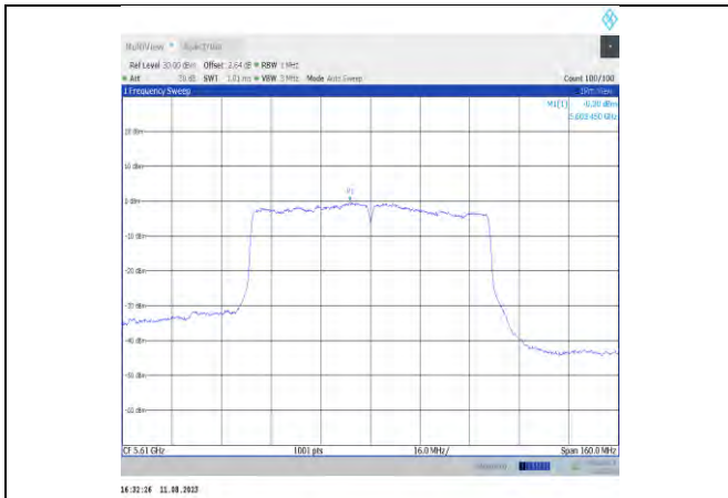
11ac80MIMO-Ant11-5610
