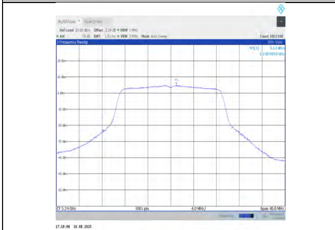
11ac20MIMO-Ant11-5240
