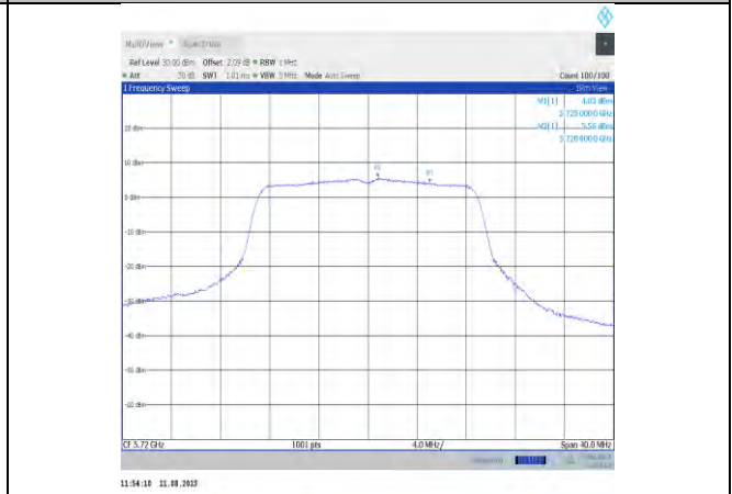
11ac20MIMO-Ant12-5720 UNII-2C
