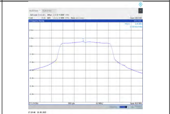
11ac20MIMO-Ant12-5240
