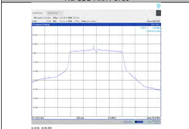
11a-CDD-Ant11-5825
