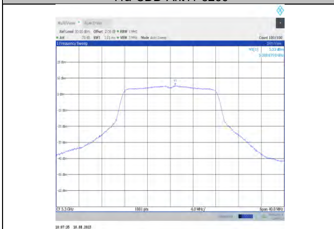
11a-CDD-Ant11-5300
