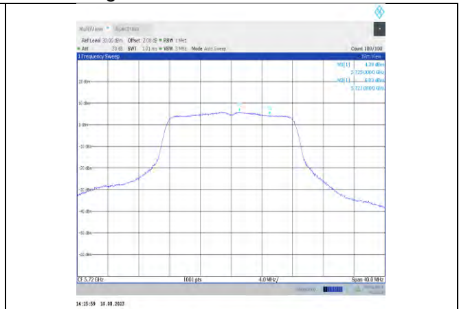
11a-CDD-Ant12-5720_UNII-2C
