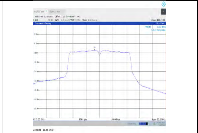
11ac40MIMO-Ant12-5550
