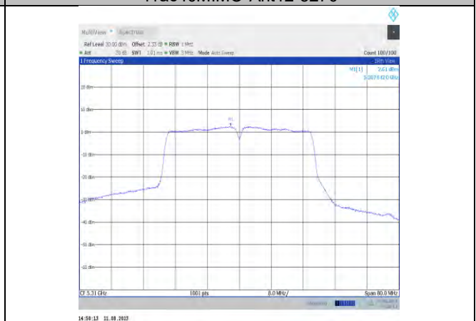
11ac40MIMO-Ant12-5310
