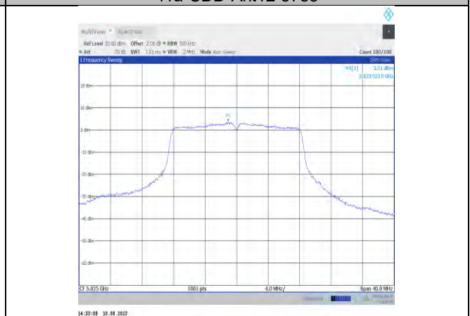
11a-CDD-Ant12-5825
