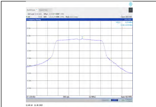
11ac20MIMO-Ant11-5580
