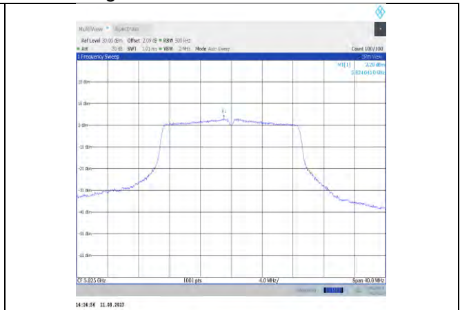
11ac20MIMO-Ant12-5825
