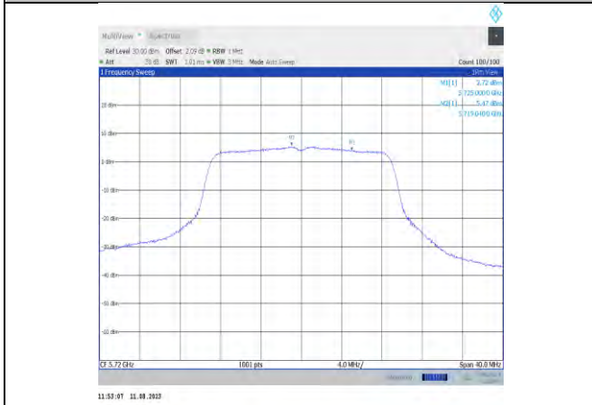
11ac20MIMO-Ant11-5720 UNII-2C
