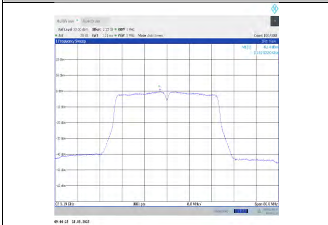
11ac40MIMO-Ant11-5190
