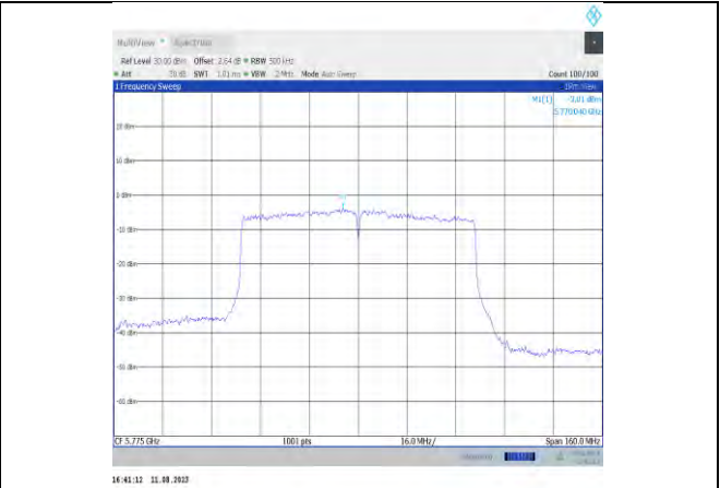
11ac80MIMO-Ant12-5775
