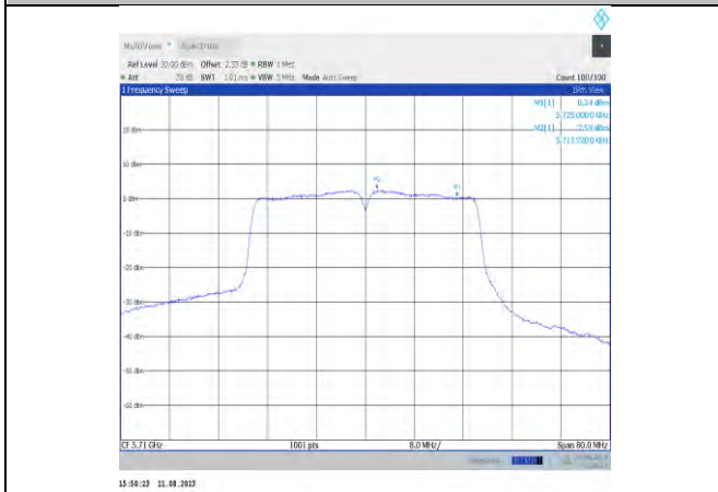
11ac40MIMO-Ant11-5710 UNII-2C
