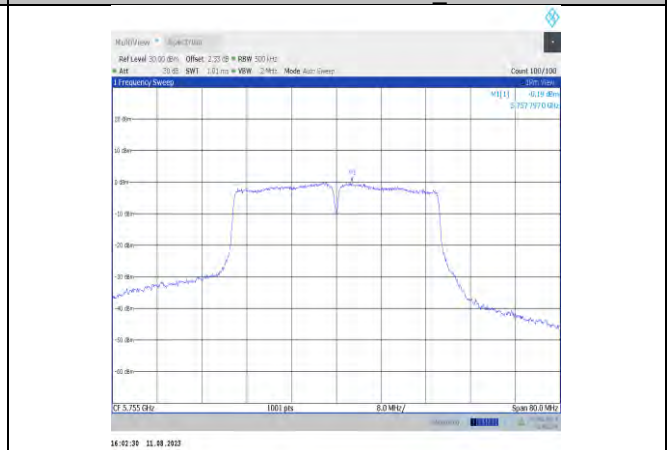
11ac40MIMO-Ant12-5755
