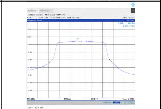
11ac20MIMO-Ant12-5500
