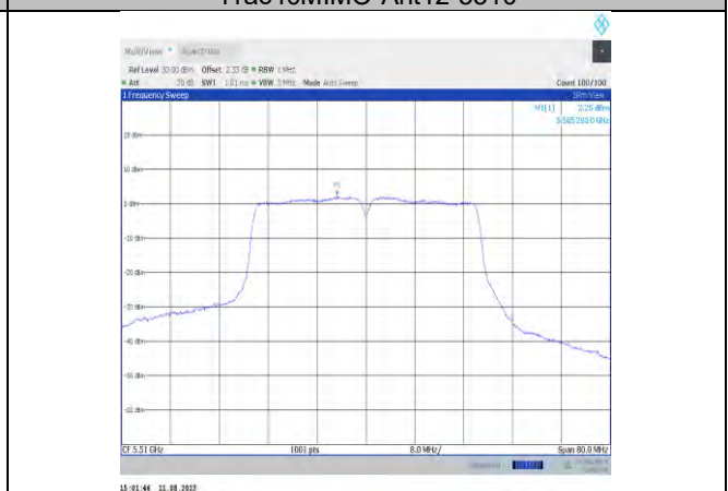
11ac40MIMO-Ant12-5510
