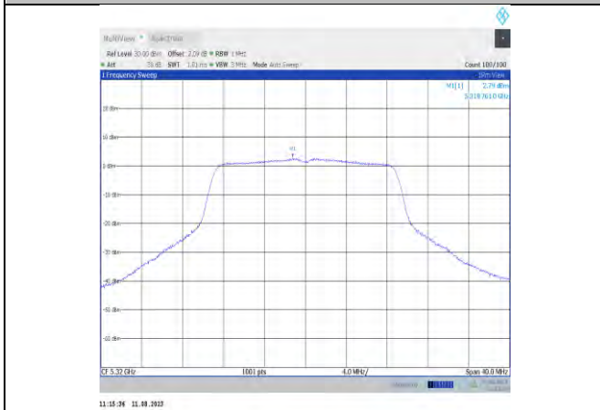
11ac20MIMO-Ant11-5320
