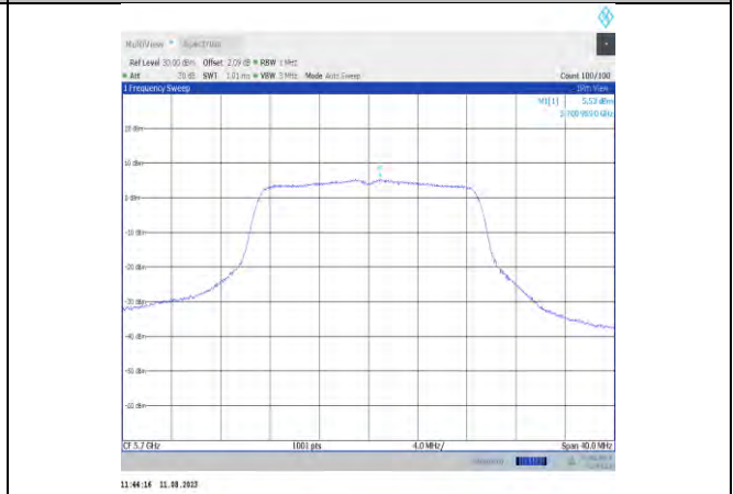
11ac20MIMO-Ant12-5700
