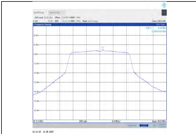
11ac20MIMO-Ant11-5300
