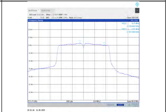
11ac40MIMO-Ant12-5710 UNII-2C
