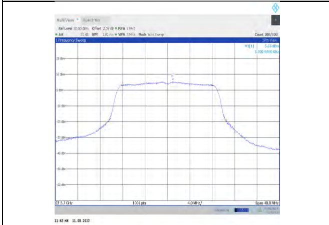
11ac20MIMO-Ant11-5700
