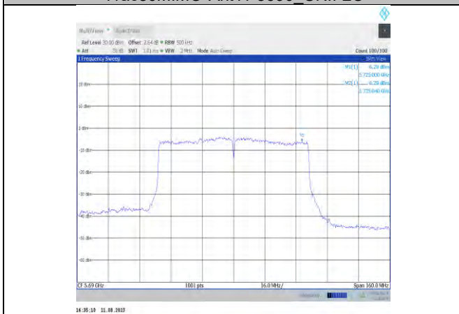
11ac80MIMO-Ant11-5690 UNII-3
