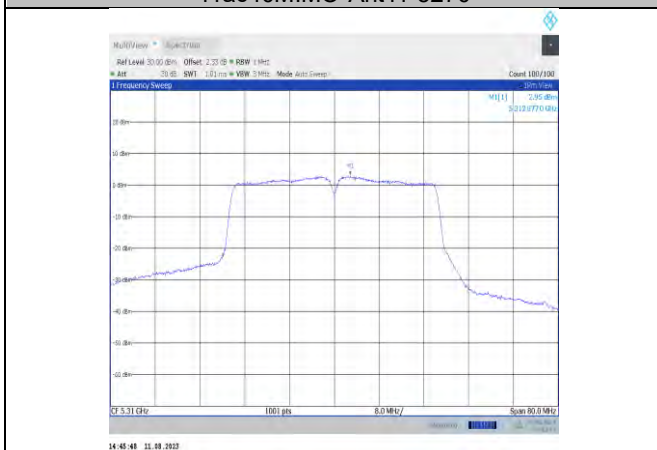
11ac40MIMO-Ant11-5310
