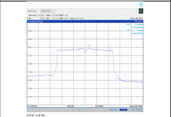
11ac80MIMO-Ant12-5690 UNII-2C
