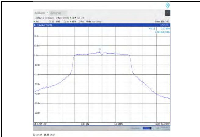
11a-CDD-Ant11-5785
