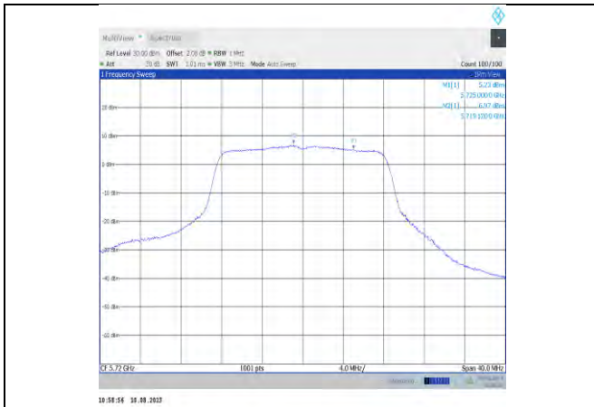
11a-CDD-Ant11-5720_UNII-2C
