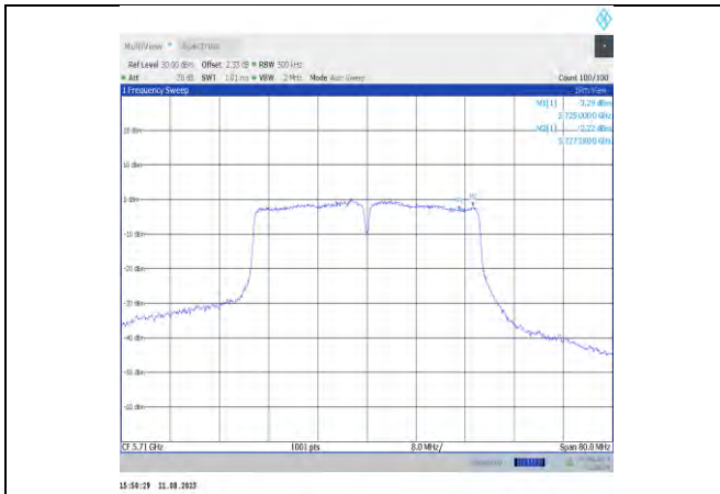
11ac40MIMO-Ant11-5710 UNII-3
