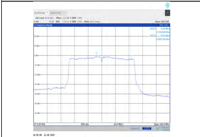
11ac80MIMO-Ant11-5690 UNII-2C
