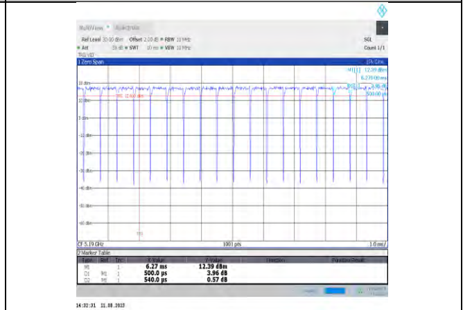
NTVN-11ac40MIMO-Ant12-5190
