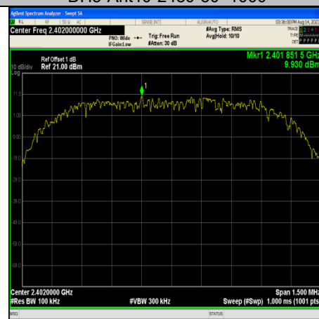
2DH5-Ant10-2402-0~Reference
