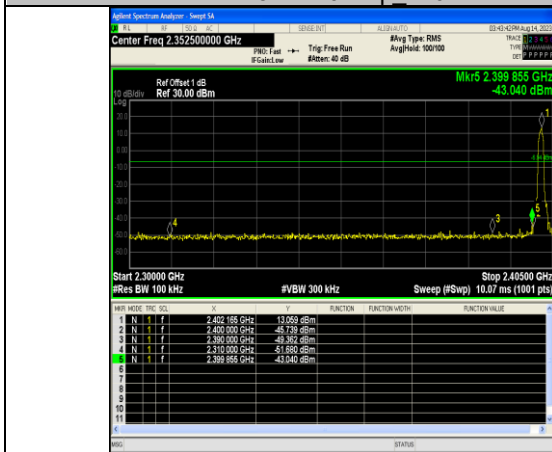
3DH5-Ant10-2402
