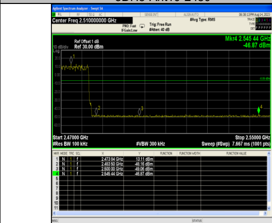
3DH5-Ant10-Hop_2480
