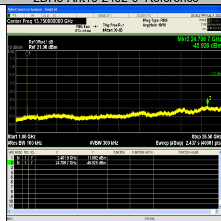
2DH5-Ant10-2402-1000~26500
