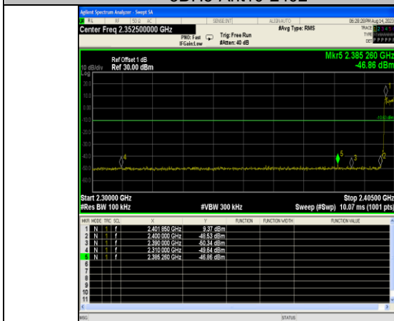
3DH5-Ant10-Hop_2402
