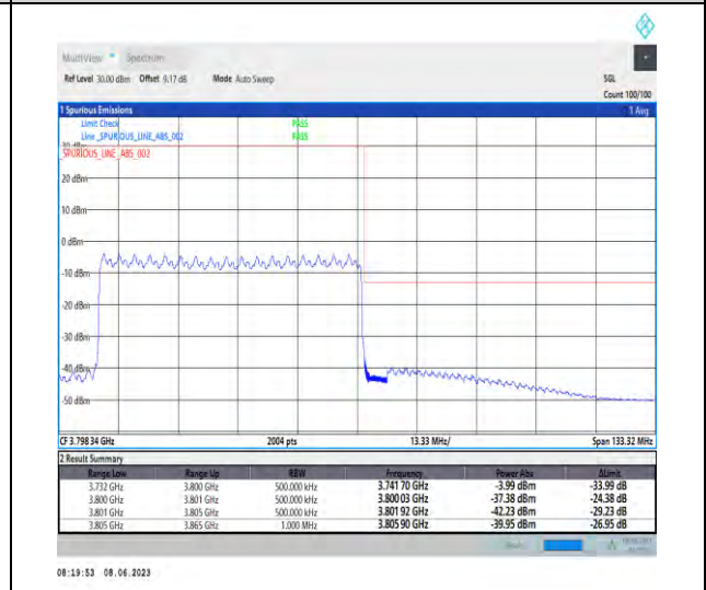
1-N78-3700-3800-PC3-30-60-H-6-CP-QPSK-Outer_Full-162@0-Ant1-1--PASS-see graph
