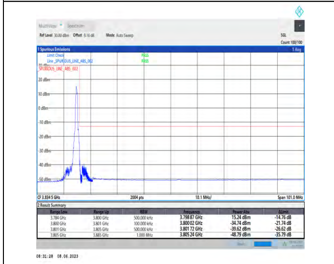
1-N78-3700-3800-PC3-30-80-H-5-CP-QPSK-Edge_1RB_Right-1@216-Ant1-1--PASS-see graph
