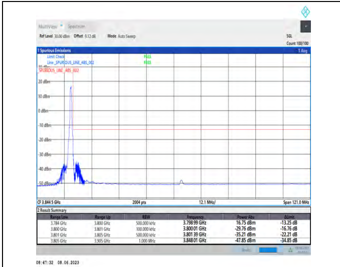
1-N78-3700-3800-PC3-30-100-H-2-DFT-PI2BPSK-Edge_1_RB_Right-1@272-Ant1-1--PASS-see graph
