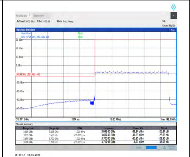
1-N78-3700-3800-PC3-30-90-L-6-CP-QPSK-Outer_Full-245@0-Ant1-1--PASS-see graph
