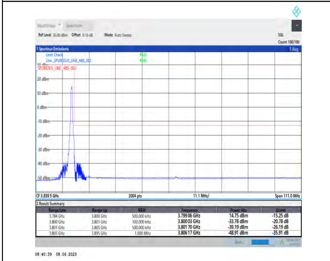
1-N78-3700-3800-PC3-30-90-H-5-CP-QPSK-Edge_1RB_Right-1@244-Ant1-1--PASS-see graph
