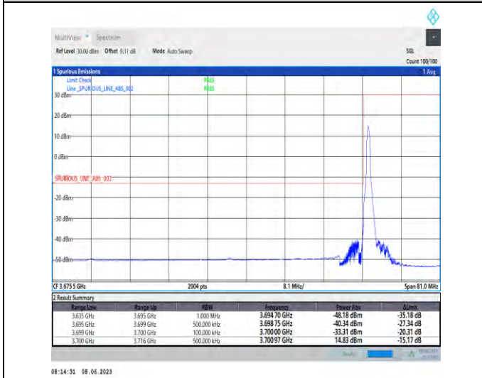
1-N78-3700-3800-PC3-30-60-L-4-CP-QPSK-Edge_1RB_Left-1@0-Ant1-1--PASS-see graph
