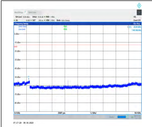
1-N78-3700-3800-PC3-30-100-L-1-N/A-DFT-PI2BP SK-Inner_1RB_Left-1@1-6000-18000-Ant1-7402.56 --53.09--13-PASS
