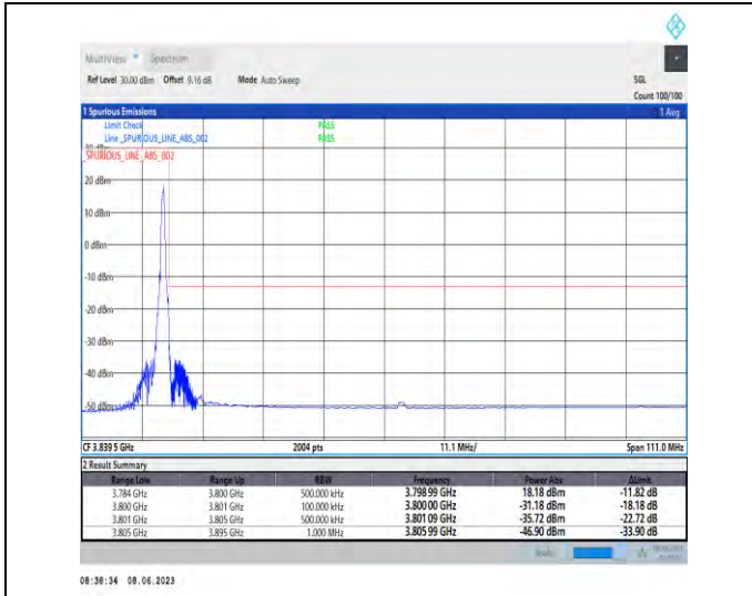
1-N78-3700-3800-PC3-30-90-H-2-DFT-PI2BPSK-Edge_1RB_Right-1@244-Ant1-1--PASS-see graph
