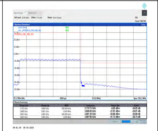
1-N78-3700-3800-PC3-30-90-H-6-CP-QPSK-Outer_Full-245@0-Ant1-1--PASS-see graph
