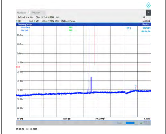
1-N78-3700-3800-PC3-30-100-H-1-N/A-DFT-PI2BPS K-Inner_1RB_Left-1@1-1000-6000-Ant1-5434.50--38 .97--13-PASS
