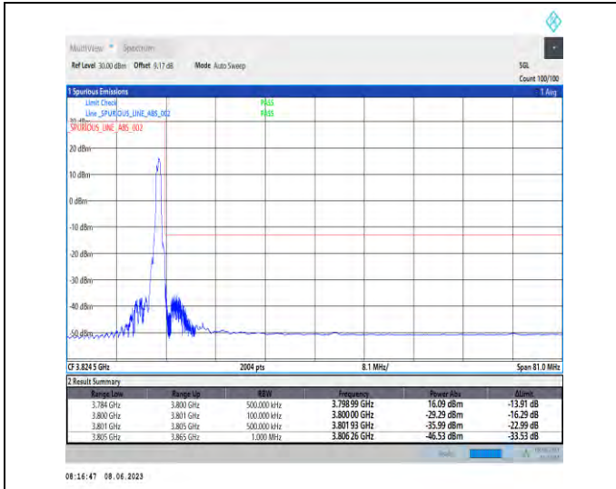
1-N78-3700-3800-PC3-30-60-H-2-DFT-PI2BPSK-Edge_1RB_Right-1@161-Ant1-1--PASS-see graph
