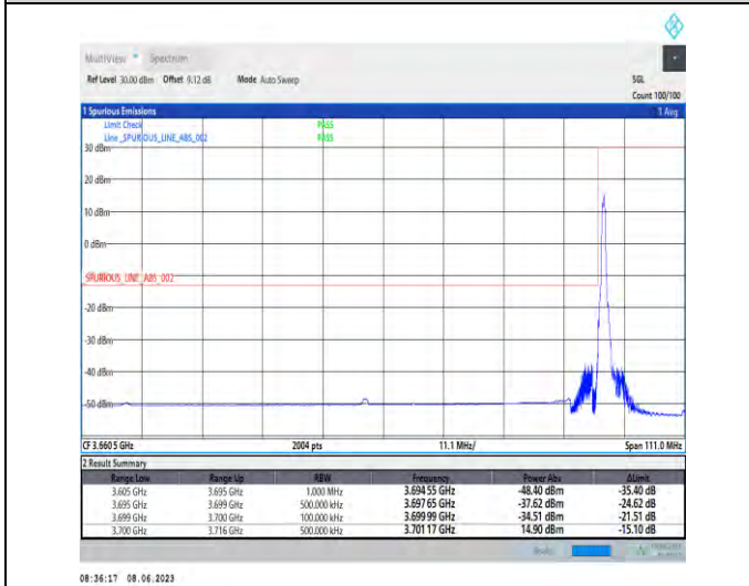
1-N78-3700-3800-PC3-30-90-L-4-CP-QPSK-Edge_1RB_Left-1@0-Ant1-1--PASS-see graph
