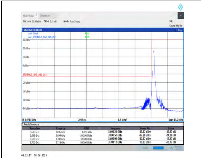
1-N78-3700-3800-PC3-30-60-L-1-DFT-PI2BPSK-Edge_1RB_Left-1@0-Ant1-1--PASS-see graph
