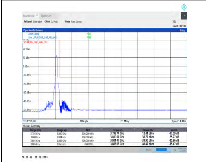
1-N78-3700-3800-PC3-30-50-H-5-CP-QPSK-Edge_1RB_Right-1@132-Ant1-1--PASS-see graph
