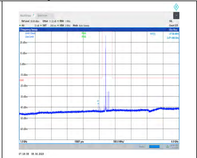
1-N78-3700-3800-PC3-30-100-M-1-N/A-DFT-PI2BPS K-Inner_1RB_Left-1@1-1000-6000-Ant1-3471.00--37.58--13-PASS
