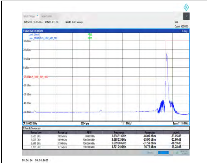
1-N78-3700-3800-PC3-30-90-L-1-DFT-PI2BPSK-Edge_1RB_Left-1@0-Ant1-1--PASS-see graph
