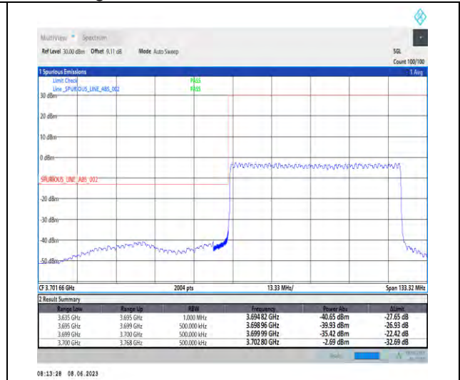
1-N78-3700-3800-PC3-30-60-L-3-DFT-PI2BPSK-Outer_Full-162@0-Ant1-1--PASS-see graph
