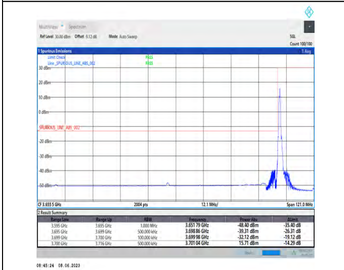
1-N78-3700-3800-PC3-30-100-L-4-CP-QPSK-Edge_1RB_Left-1@0-Ant1-1--PASS-see graph
