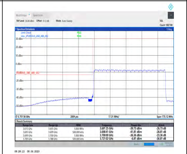
1-N78-3700-3800-PC3-30-80-L-6-CP-QPSK-Outer_Full-217@0-Ant1-1--PASS-see graph
