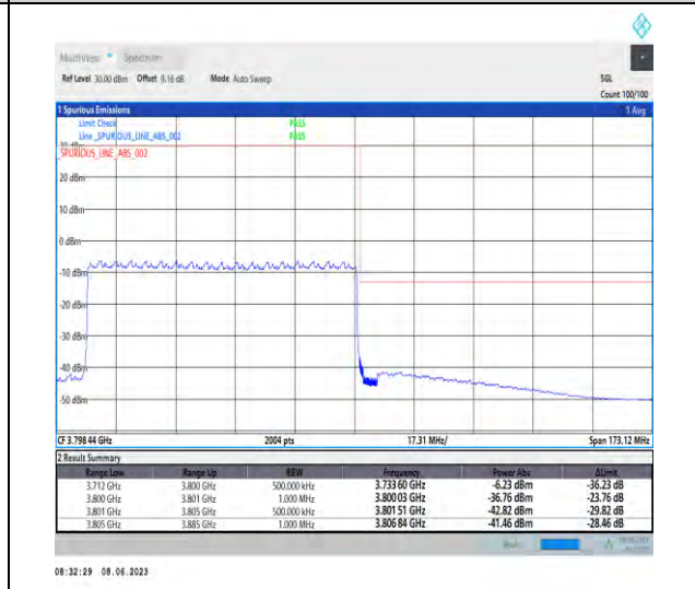
1-N78-3700-3800-PC3-30-80-H-6-CP-QPSK-Outer_Full-217@0-Ant1-1--PASS-see graph
