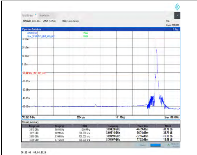
1-N78-3700-3800-PC3-30-80-L-1-DFT-PI2BPSK-Edge_1RB_Left-1@0-Ant1-1--PASS-see graph
