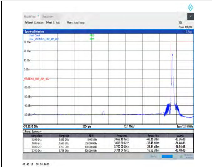
1-N78-3700-3800-PC3-30-100-L-1-DFT-PI2BPSK-Edge_e_1RB_Left-1@0-Ant1-1--PASS-see graph
