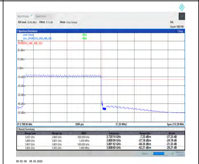
1-N78-3700-3800-PC3-30-100-H-6-CP-QPSK-Outer_Full-273@0-Ant1-1--PASS-see graph
