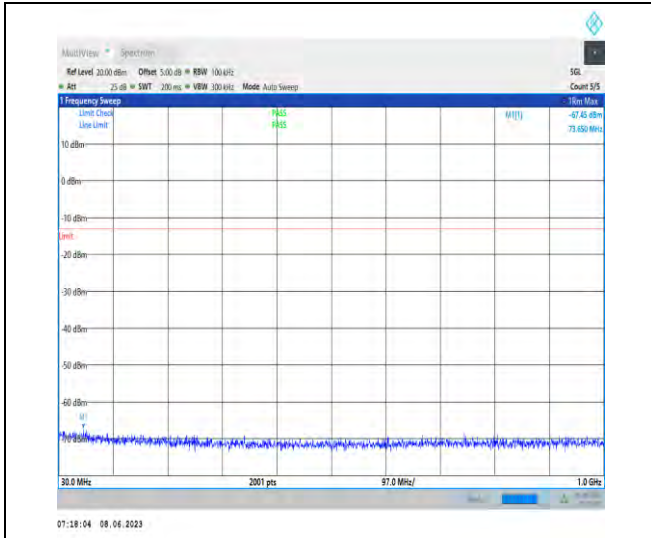
1-N78-3700-3800-PC3-30-100-M-1-N/A-DFT-PI2BP SK-Inner_1RB_Left-1@1-30-1000-Ant1-73.65--67.4 5--13-PASS
