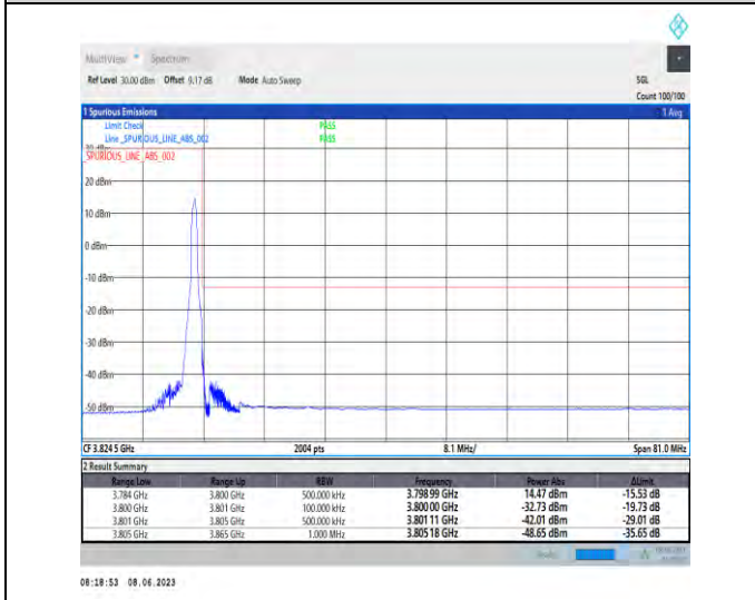
1-N78-3700-3800-PC3-30-60-H-5-CP-QPSK-Edge_1RB_Right-1@161-Ant1-1--PASS-see graph
