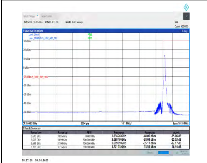
1-N78-3700-3800-PC3-30-80-L-4-CP-QPSK-Edge_1RB_Left-1@0-Ant1-1--PASS-see graph
