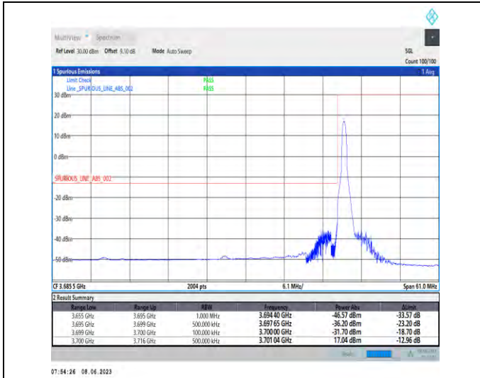
1-N78-3700-3800-PC3-30-40-L-1-DFT-PI2BPSK-Edge_1RB_Left-1@0-Ant1-1--PASS-see graph
