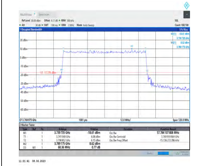
1-N78-3700-3800-PC3-30-60-H-9-CP-256QAM-Outer_Full-162@0-Ant1-57.784-60.360-≤60-PASS
