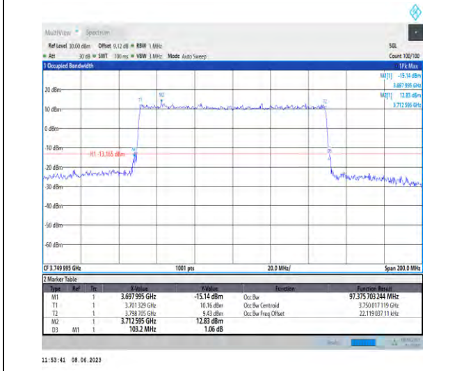
1-N78-3700-3800-PC3-30-100-L-6-CP-QPSK-Outer _Full-273@0-Ant1-97.376-103.200-≤100-PASS
