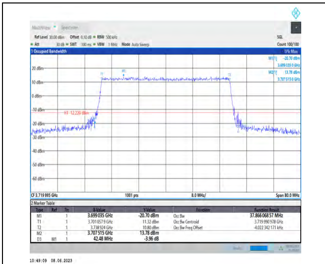
1-N78-3700-3800-PC3-30-40-L-7-CP-16QAM-Outer_Full-106@0-Ant1-37.866-42.480-≤40-PASS
