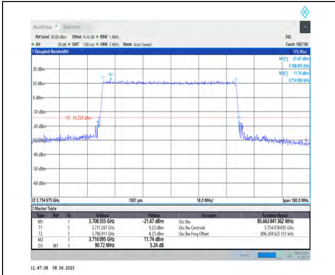
1-N78-3700-3800-PC3-30-90-H-5-DFT-256QAM-Out er_Full-240@0-Ant1-85.664-90.720-≤90-PASS
