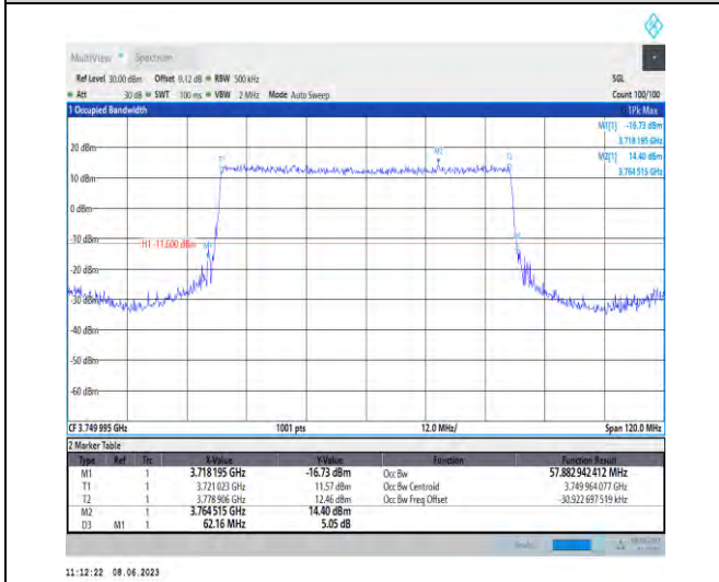
1-N78-3700-3800-PC3-30-60-M-2-DFT-PI2BPSK-Outer_Full-162@0-Ant1-57.883-62.160-≤60-PASS
