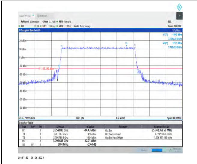
1-N78-3700-3800-PC3-30-40-H-5-DFT-256QAM-Out er_Full-100@0-Ant1-35.742-38.400-≤40-PASS
