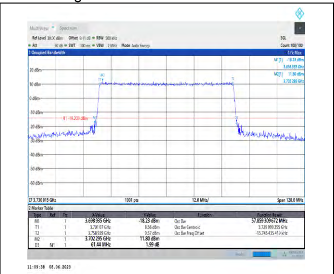
1-N78-3700-3800-PC3-30-60-L-6-CP-QPSK-Outer_Full-162@0-Ant1-57.859-61.440-≤60-PASS
