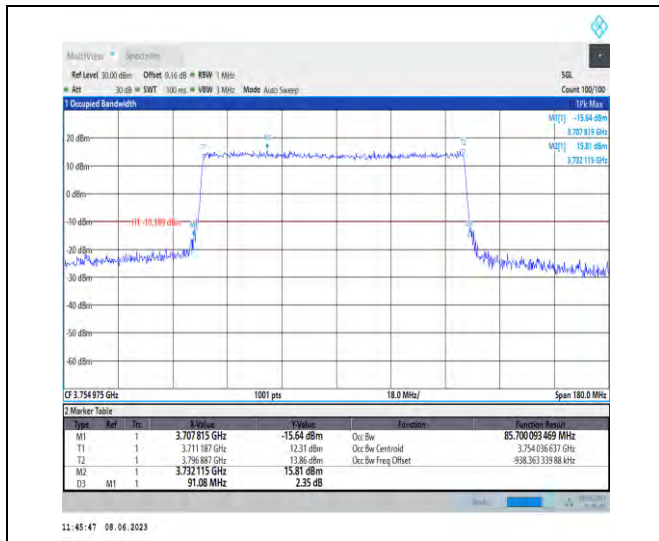
1-N78-3700-3800-PC3-30-90-H-1-DFT-QPSK-Outer_Full-240@0-Ant1-85.7-91.080-≤90-PASS
