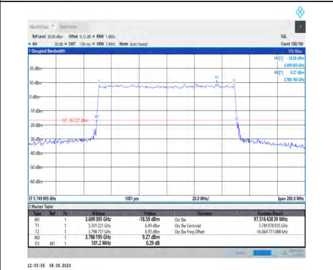
1-N78-3700-3800-PC3-30-100-H-9-CP-256QAM-Outer_Full-273@0-Ant1-97.516-101.200-≤100-PASS
