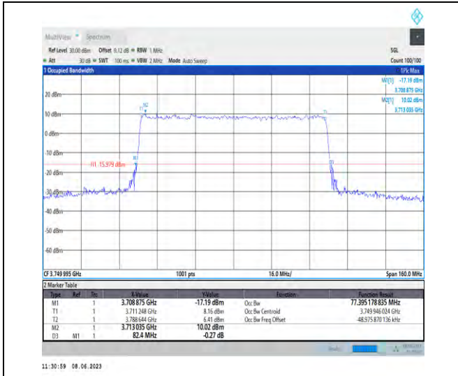
1-N78-3700-3800-PC3-30-80-M-9-CP-256QAM-Out er_Full-217@0-Ant1-77.395-82.400-≤80-PASS
