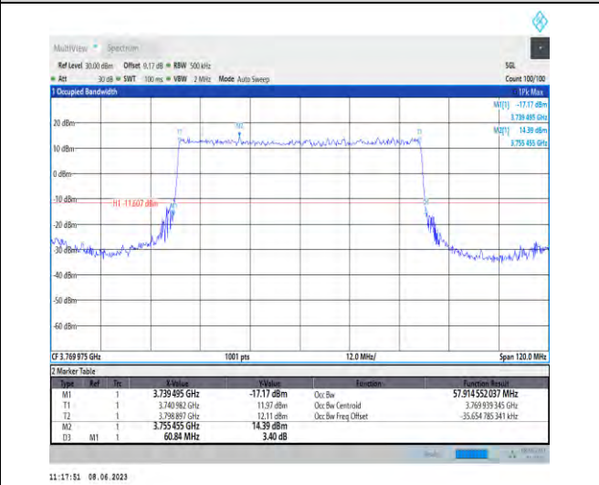
1-N78-3700-3800-PC3-30-60-H-2-DFT-PI2BPSK-Outer_Full-162@0-Ant1-57.915-60.840-≤60-PASS
