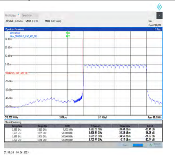
1-N78-3700-3800-PC3-30-40-L-3-DFT-PI2BPSK-Outer_Full-100@0-Ant1-1--PASS-see graph
