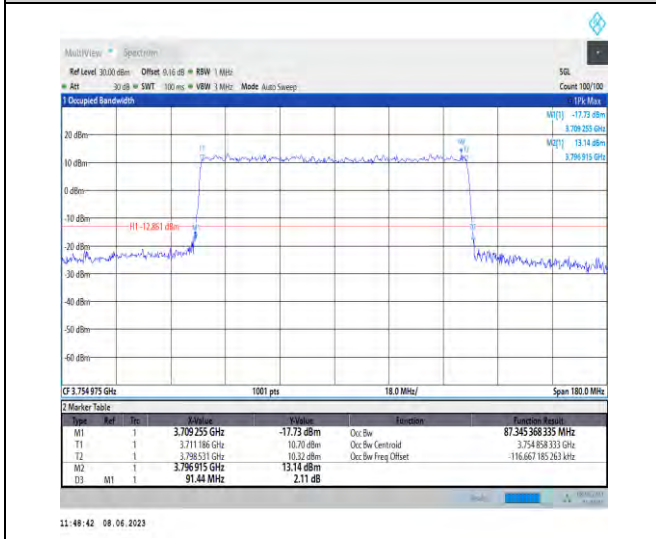
1-N78-3700-3800-PC3-30-90-H-7-CP-16QAM-Outer _Full-245@0-Ant1-87.345-91.440-≤90-PASS
