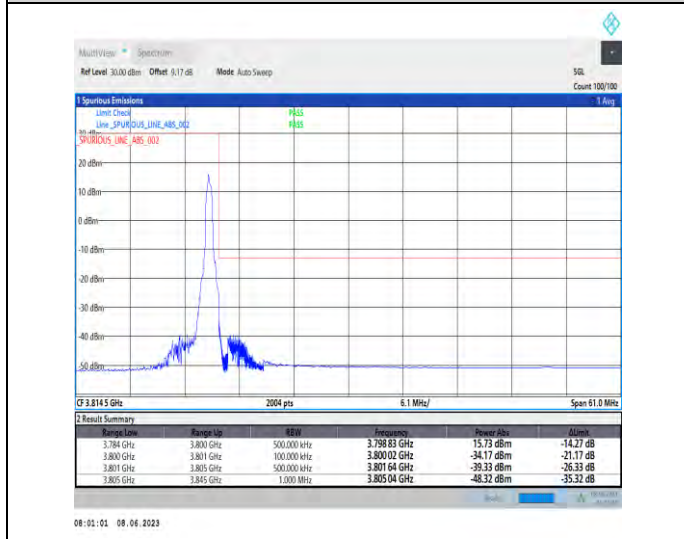
1-N78-3700-3800-PC3-30-40-H-5-CP-QPSK-Edge_1RB_Right-1@105-Ant1-1--PASS-see graph
