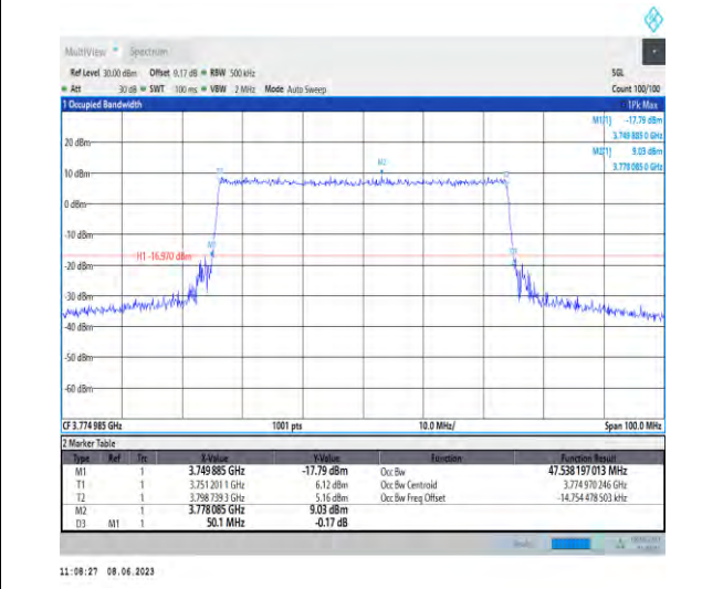
1-N78-3700-3800-PC3-30-50-H-9-CP-256QAM-Outer_Full-133@0-Ant1-47.538-50.100-≤50-PASS
