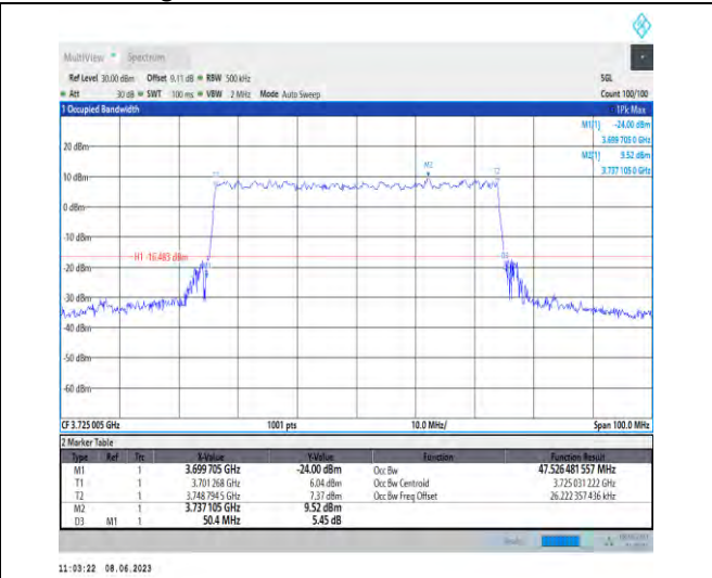
1-N78-3700-3800-PC3-30-50-L-9-CP-256QAM-Outer_Full-133@0-Ant1-47.526-50.400-≤50-PASS
