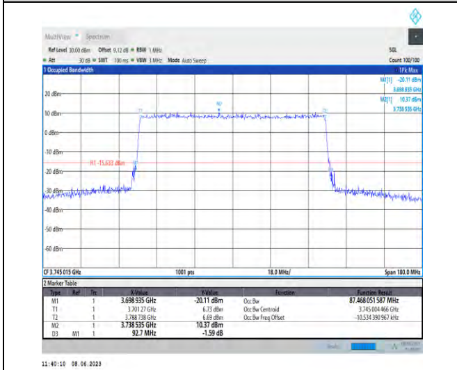
1-N78-3700-3800-PC3-30-90-L-9-CP-256QAM-Outer_Full-245@0-Ant1-87.468-92.700-≤90-PASS
