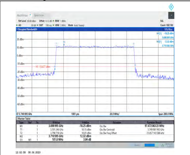
1-N78-3700-3800-PC3-30-100-H-7-CP-16QAM-Outer_Full-273@0-Ant1-97.472-101.800-≤100-PASS
