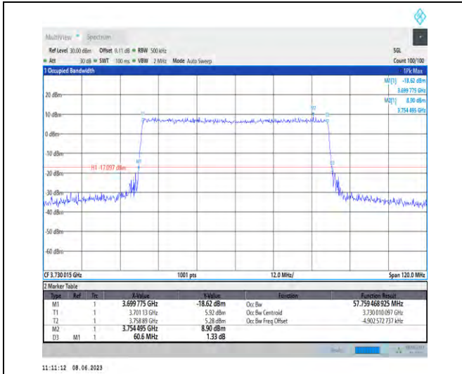
1-N78-3700-3800-PC3-30-60-L-9-CP-256QAM-Outer_Full-162@0-Ant1-57.759-60.600-≤60-PASS
