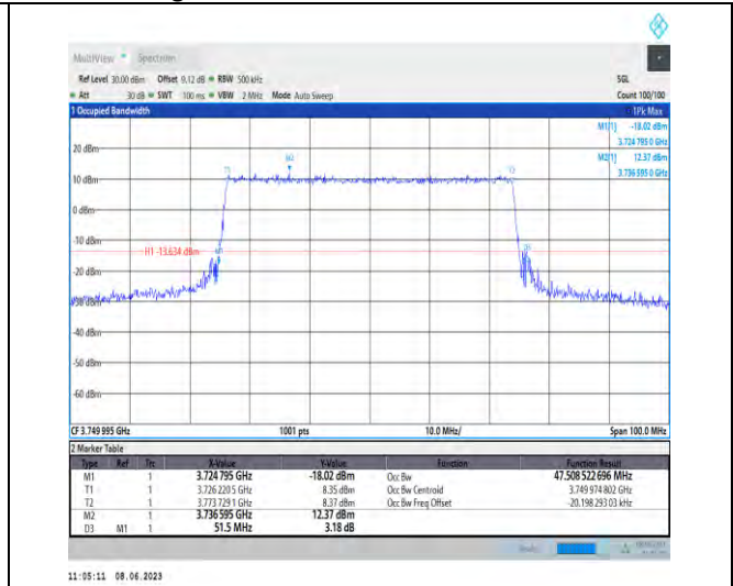
1-N78-3700-3800-PC3-30-50-M-8-CP-64QAM-Outer _Full-133@0-Ant1-47.509-51.500-≤50-PASS
