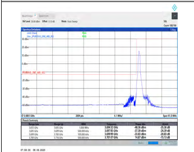
1-N78-3700-3800-PC3-30-40-L-4-CP-QPSK-Edge_1RB_Left-1@0-Ant1-1--PASS-see graph
