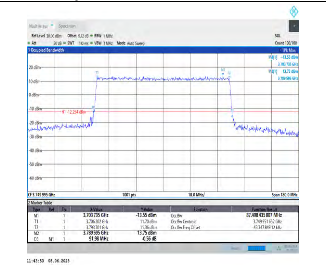
1-N78-3700-3800-PC3-30-90-M-7-CP-16QAM-Outer_Full-245@0-Ant1-87.498-91.980-≤90-PASS
