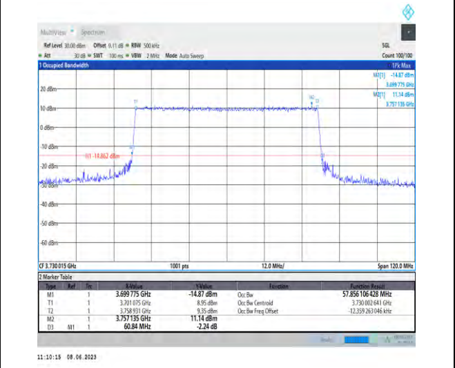
1-N78-3700-3800-PC3-30-60-L-8-CP-64QAM-Outer_Full-162@0-Ant1-57.856-60.840-≤60-PASS
