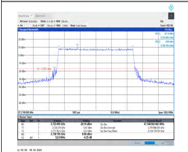
1-N78-3700-3800-PC3-30-50-M-9-CP-256QAM-Outer _Full-133@0-Ant1-47.549-52.800-≤50-PASS
