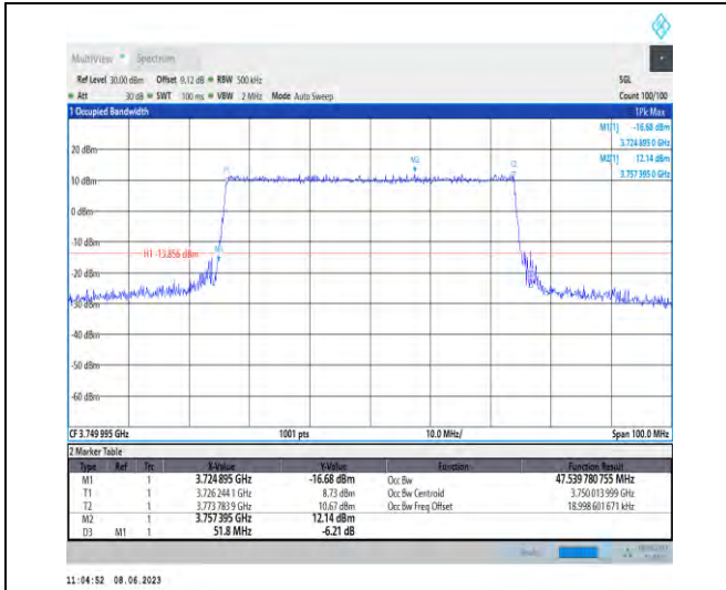
1-N78-3700-3800-PC3-30-50-M-7-CP-16QAM-Outer _Full-133@0-Ant1-47.54-51.800-≤50-PASS
