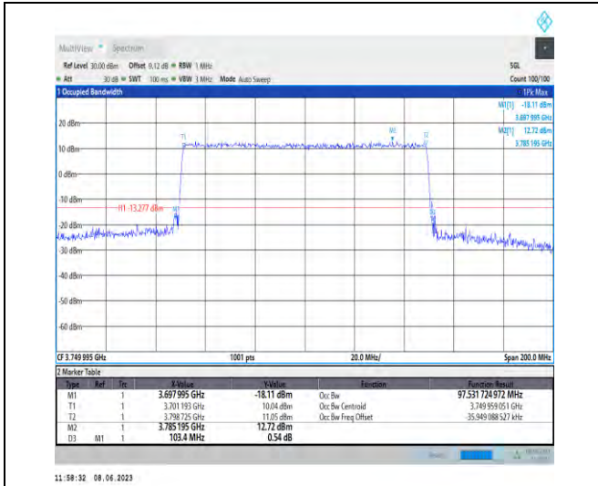
1-N78-3700-3800-PC3-30-100-M-7-CP-16QAM-Outer_Full-273@0-Ant1-97.532-103.400-≤100-PASS
