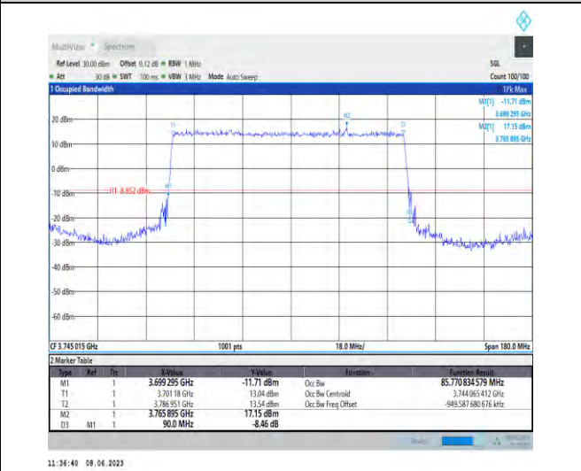
1-N78-3700-3800-PC3-30-90-L-2-DFT-PI2BPSK-Outer_Full-240@0-Ant1-85.771-90.000-≤90-PASS
