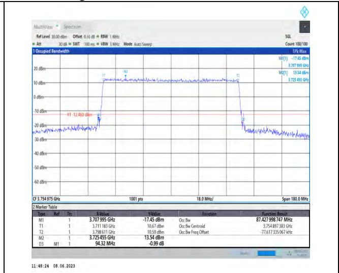
1-N78-3700-3800-PC3-30-90-H-6-CP-QPSK-Outer Full-245@0-Ant1-87.428-94.320-≤90-PASS
