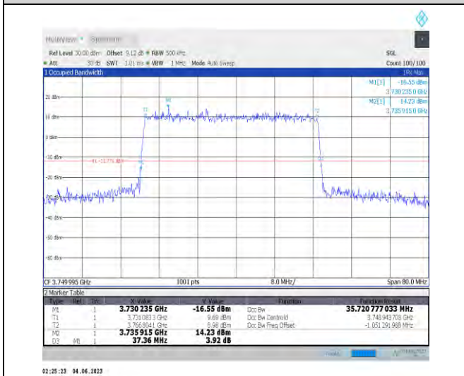
1-N78-3700-3800-PC3-30-40-M-4-DFT-64QAM-Outer_r_Full-100@0-Ant1-35.721-37.360-≤40-PASS
