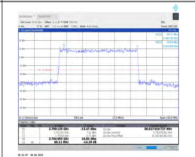
1-N78-3700-3800-PC3-30-60-L-4-DFT-64QAM-Outer_Full-162@0-Ant1-58.027-60.120-≤60-PASS
