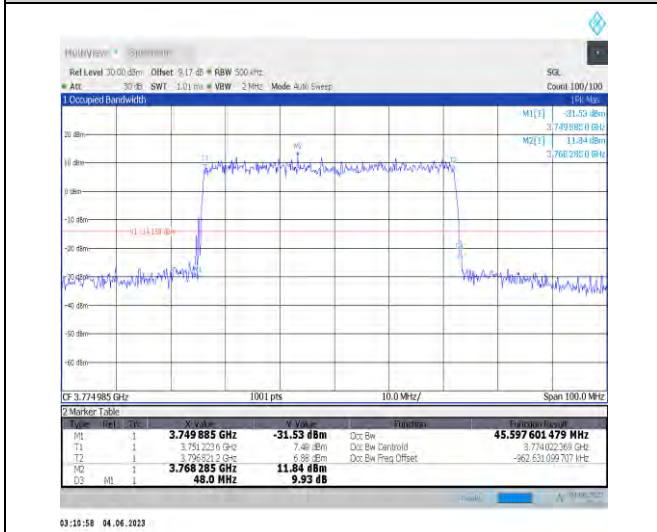
1-N78-3700-3800-PC3-30-50-H-4-DFT-64QAM-Outer_Full-128@0-Ant1-45.598-48.000-≤50-PASS
