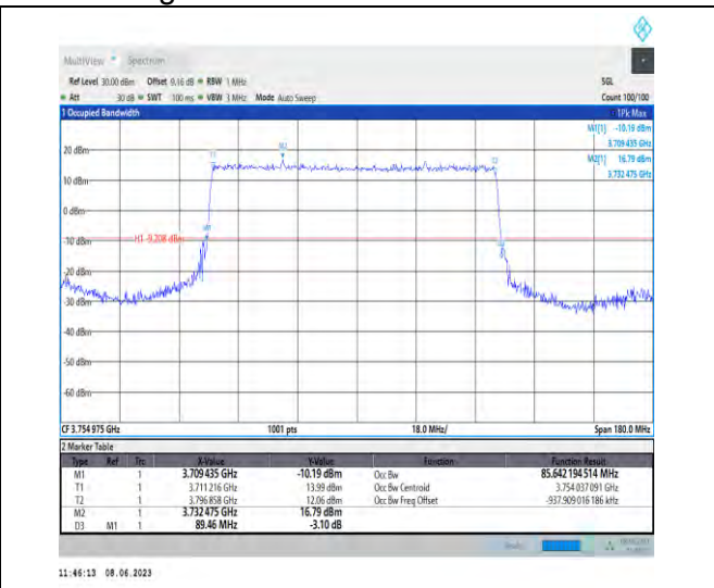
1-N78-3700-3800-PC3-30-90-H-2-DFT-PI2BPSK-Outer_Full-240@0-Ant1-85.642-89.460-≤90-PASS
