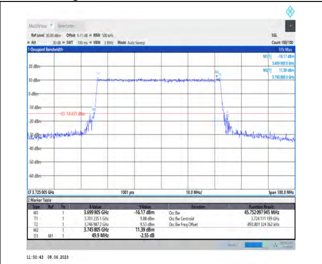
1-N78-3700-3800-PC3-30-50-L-5-DFT-256QAM-Outer_Full-128@0-Ant1-45.752-49.900-≤50-PASS
