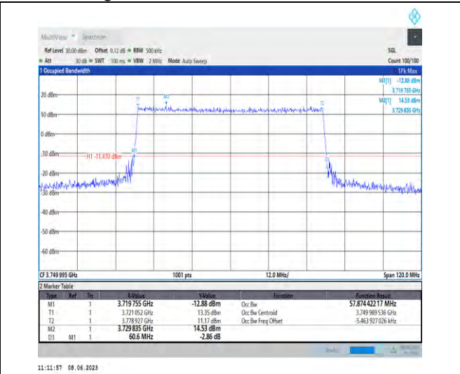
1-N78-3700-3800-PC3-30-60-M-1-DFT-QPSK-Outer_Full-162@0-Ant1-57.874-60.600-≤60-PASS
