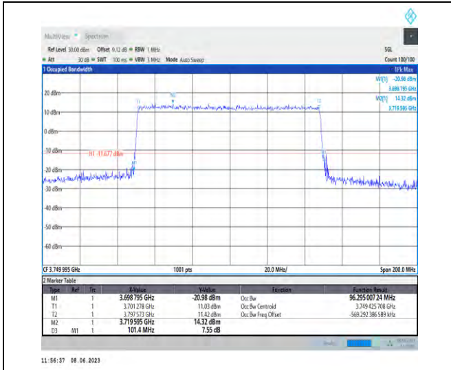
1-N78-3700-3800-PC3-30-100-M-3-DFT-16QAM-Out er_Full-270@0-Ant1-96.295-101.400-≤100-PASS
