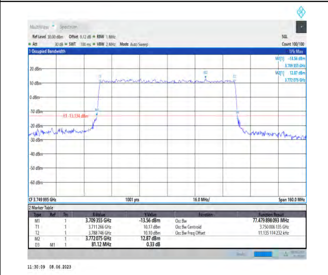
1-N78-3700-3800-PC3-30-80-M-8-CP-64QAM-Outer_Full-217@0-Ant1-77.48-81.120-<80-PASS
