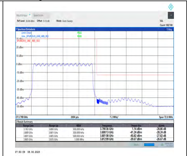
1-N78-3700-3800-PC3-30-30-H-3-DFT-PI2BPSK-Outer_Full-75@0-Ant1-1--PASS-see graph
