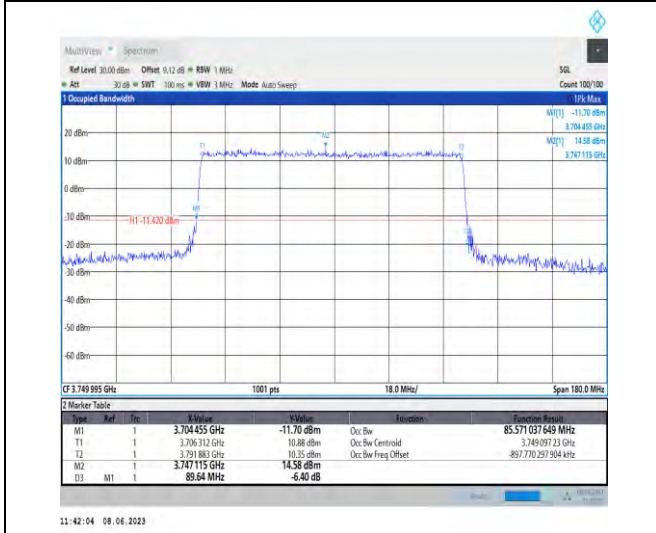
1-N78-3700-3800-PC3-30-90-M-4-DFT-64QAM-Outer_Full-240@0-Ant1-85.571-89.640-≤90-PASS
