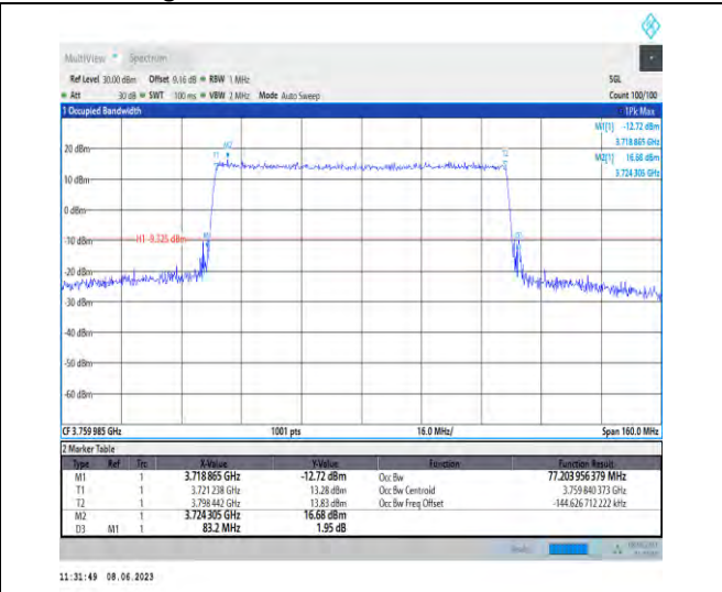
1-N78-3700-3800-PC3-30-80-H-1-DFT-QPSK-Outer_Full-216@0-Ant1-77.204-83.200-≤80-PASS
