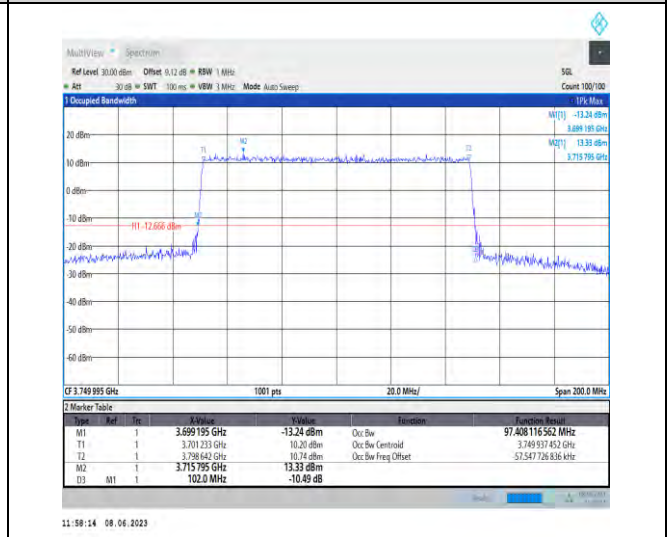
1-N78-3700-3800-PC3-30-100-M-6-CP-QPSK-Outer _Full-273@0-Ant1-97.408-102.000-≤100-PASS
