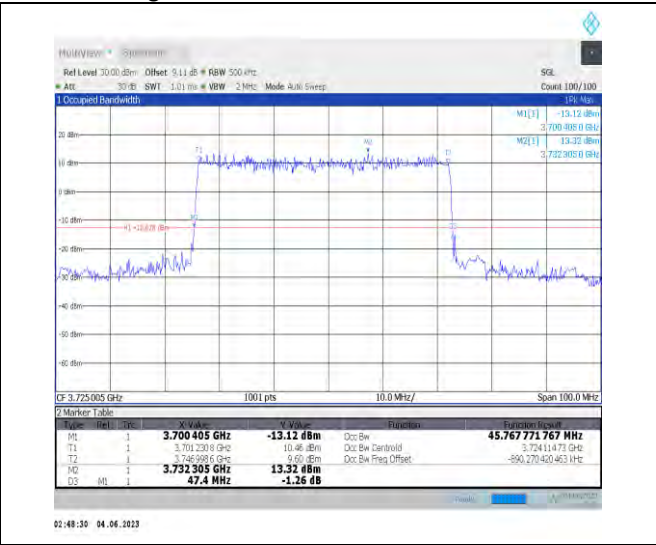
1-N78-3700-3800-PC3-30-50-L-1-DFT-QPSK-Outer_Full-128@0-Ant1-45.768-47.400-≤50-PASS
