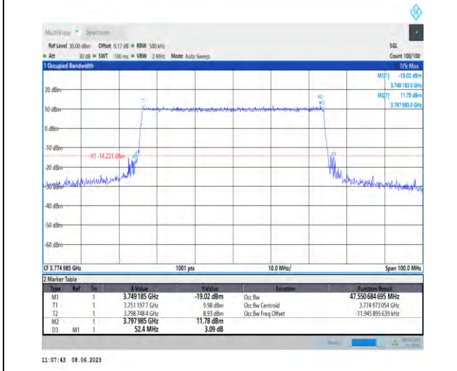
1-N78-3700-3800-PC3-30-50-H-8-CP-64QAM-Outer_Full-133@0-Ant1-47.551-52.400-≤50-PASS
