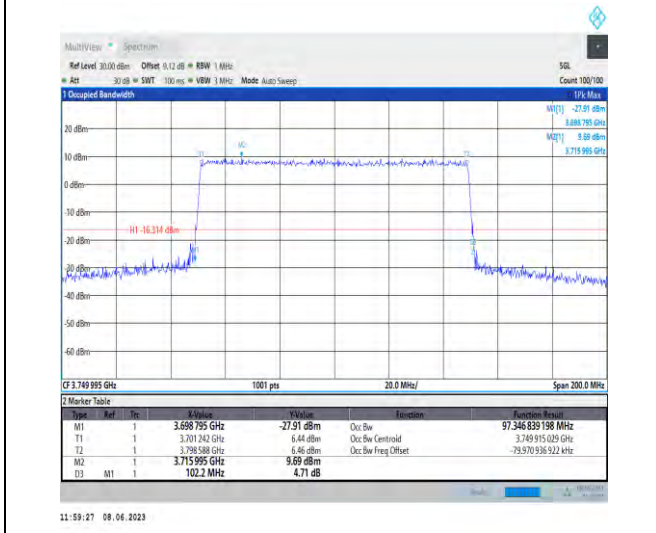
1-N78-3700-3800-PC3-30-100-M-9-CP-256QAM-Outer_Full-273@0-Ant1-97.347-102.200-≤100-PASS
