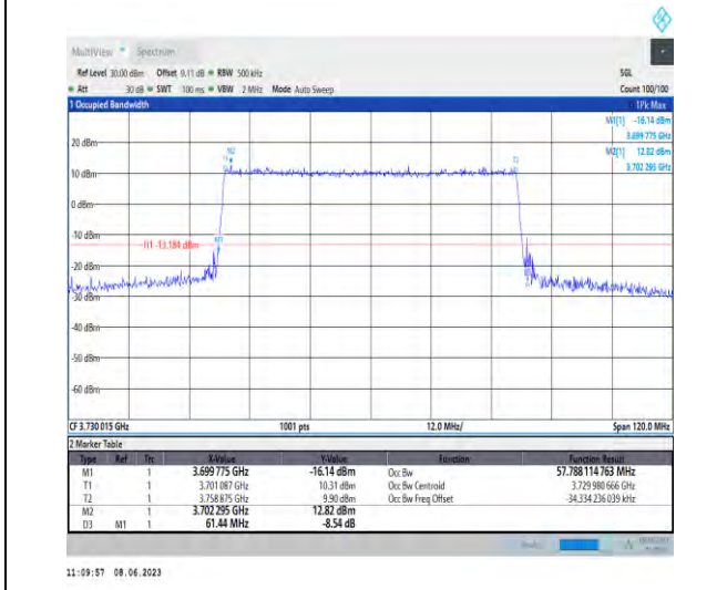
1-N78-3700-3800-PC3-30-60-L-7-CP-16QAM-Outer_Full-162@0-Ant1-57.788-61.440-≤60-PASS
