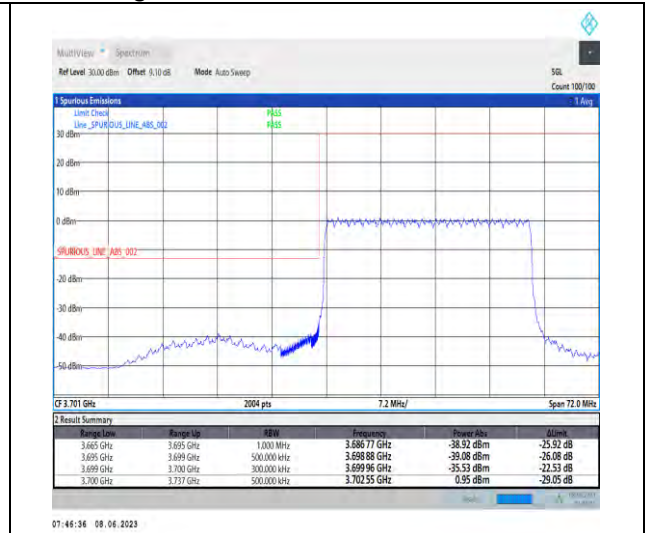
1-N78-3700-3800-PC3-30-30-L-3-DFT-PI2BPSK-Outer_Full-75@0-Ant1-1--PASS-see graph
