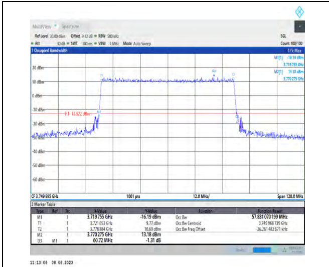
1-N78-3700-3800-PC3-30-60-M-4-DFT-64QAM-Outer_Full-162@0-Ant1-57.831-60.720-≤60-PASS
