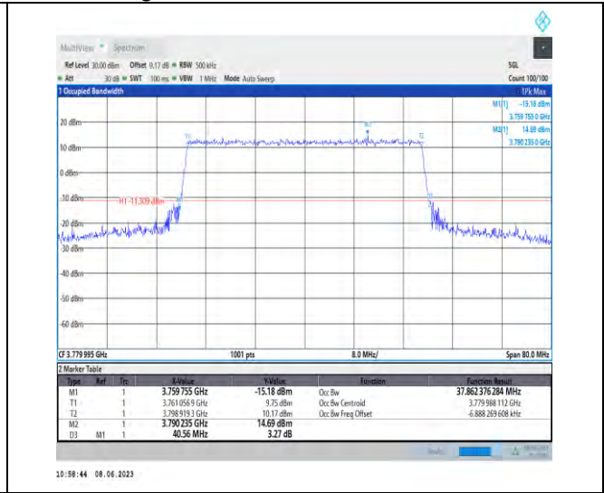
1-N78-3700-3800-PC3-30-40-H-6-CP-QPSK-Outer Full-106@0-Ant1-37.862-40.560-≤40-PASS
