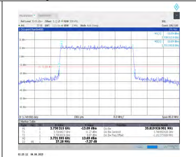
1-N78-3700-3800-PC3-30-40-M-3-DFT-16QAM-Outer_r_Full-100@0-Ant1-35.82-37.280-≤40-PASS
