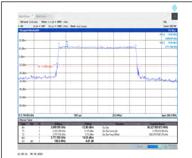
1-N78-3700-3800-PC3-30-100-L-4-DFT-64QAM-Out er_Full-270@0-Ant1-96.327-100.600-≤100-PASS
