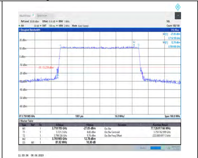
1-N78-3700-3800-PC3-30-80-H-5-DFT-256QAM-Outer_Full-216@0-Ant1-77.127-81.920-≤80-PASS
