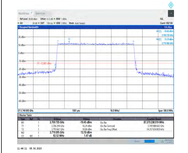
1-N78-3700-3800-PC3-30-90-M-8-CP-64QAM-Outer_Full-245@0-Ant1-87.373-92.520-≤90-PASS
