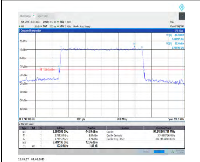
1-N78-3700-3800-PC3-30-100-H-8-CP-64QAM-Outer_Full-273@0-Ant1-97.249-102.000-≤100-PASS
