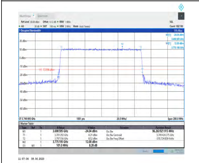
1-N78-3700-3800-PC3-30-100-M-5-DFT-256QAM-Out uter_Full-270@0-Ant1-96.264-101.000-≤100-PASS
