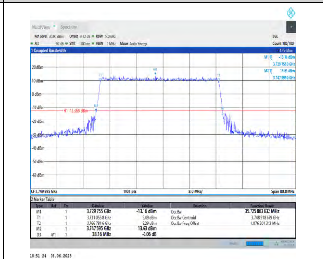
1-N78-3700-3800-PC3-30-40-M-5-DFT-256QAM-Outer_r_Full-100@0-Ant1-35.726-38.160-≤40-PASS
