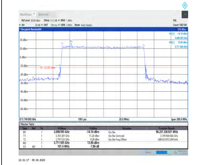
1-N78-3700-3800-PC3-30-100-H-4-DFT-64QAM-Outer_Full-270@0-Ant1-96.251-101.400-≤100-PASS
