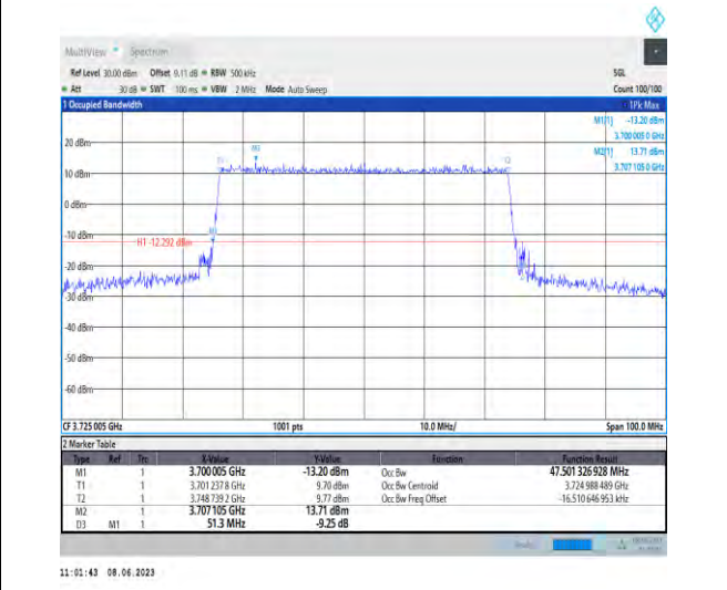
1-N78-3700-3800-PC3-30-50-L-7-CP-16QAM-Outer_Full-133@0-Ant1-47.501-51.300-≤50-PASS
