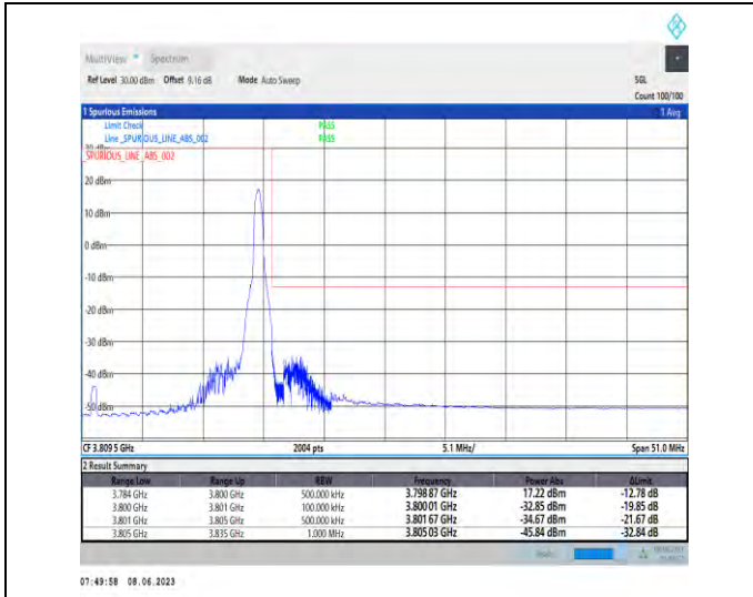
1-N78-3700-3800-PC3-30-30-H-2-DFT-PI2BPSK-Edge_1RB_Right-1@77-Ant1-1--PASS-see graph
