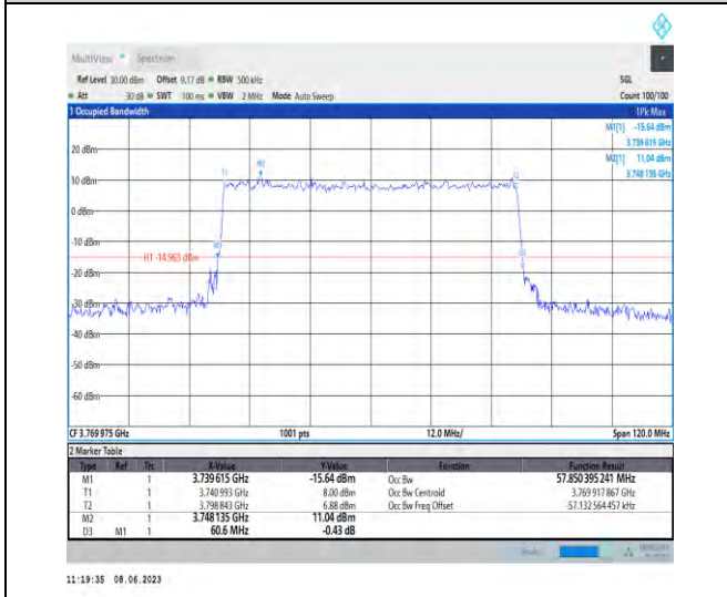
1-N78-3700-3800-PC3-30-60-H-5-DFT-256QAM-Outer_Full-162@0-Ant1-57.85-60.600-≤60-PASS
