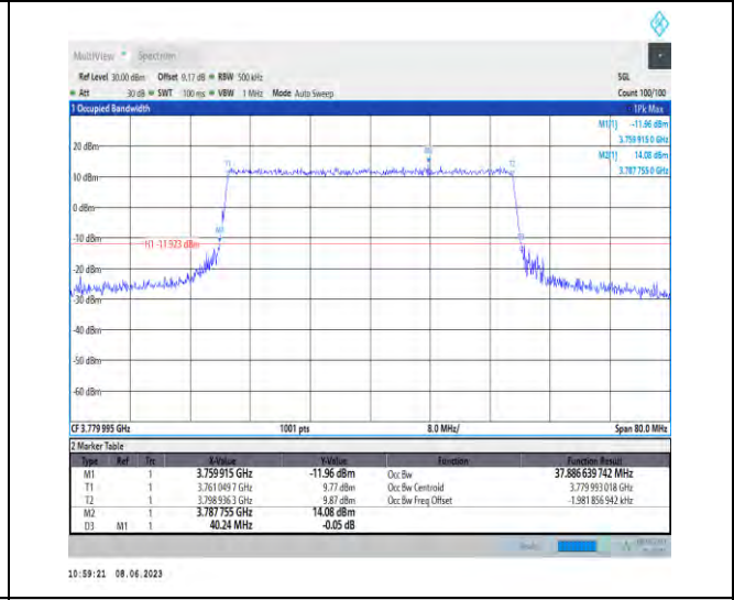
1-N78-3700-3800-PC3-30-40-H-8-CP-64QAM-Outer _Full-106@0-Ant1-37.887-40.240-≤40-PASS
