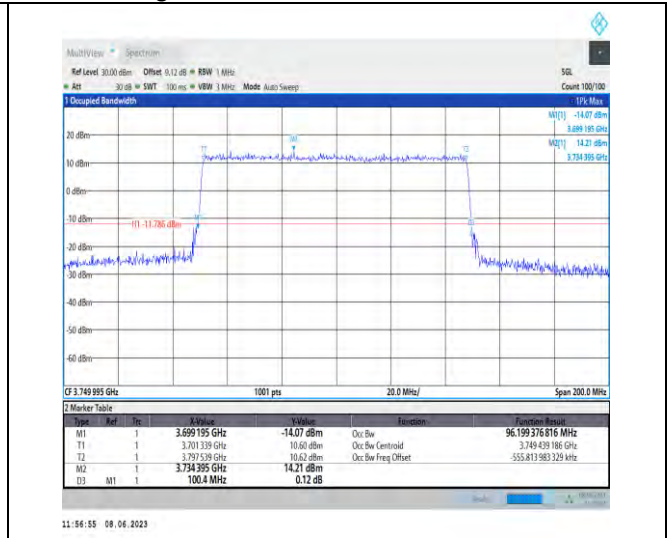
1-N78-3700-3800-PC3-30-100-M-4-DFT-64QAM-Out er_Full-270@0-Ant1-96.199-100.400-≤100-PASS
