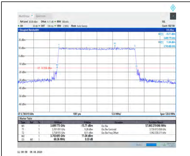
1-N78-3700-3800-PC3-30-60-L-5-DFT-256QAM-Out_er_Full-162@0-Ant1-57.843-60.360-≤60-PASS
