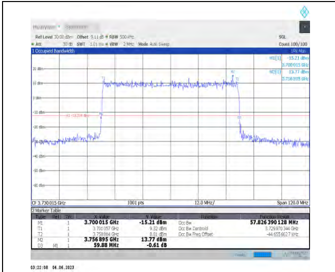
1-N78-3700-3800-PC3-30-60-L-1-DFT-QPSK-Outer_Full-162@0-Ant1-57.826-59.880-≤60-PASS
