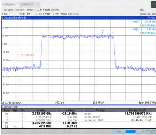
1-N78-3700-3800-PC3-30-50-M-3-DFT-16QAM-Outer_Full-128@0-Ant1-45.776-47.800-≤50-PASS
