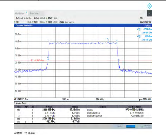
1-N78-3700-3800-PC3-30-100-L-9-CP-256QAM-Outer_Full-273@0-Ant1-97.54-102.200-≤100-PASS
