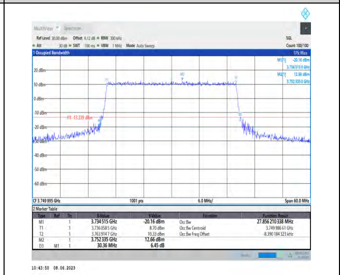
1-N78-3700-3800-PC3-30-30-M-8-CP-64QAM-Outer _Full-78@0-Ant1-27.856-30.360-≤30-PASS
