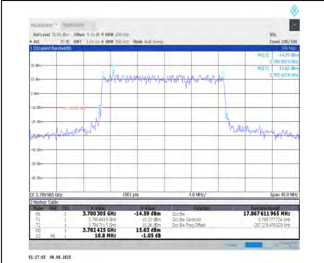
1-N78-3700-3800-PC3-30-20-H-1-DFT-QPSK-Outer_Full-50@0-Ant1-17.868-18.800-≤20-PASS
