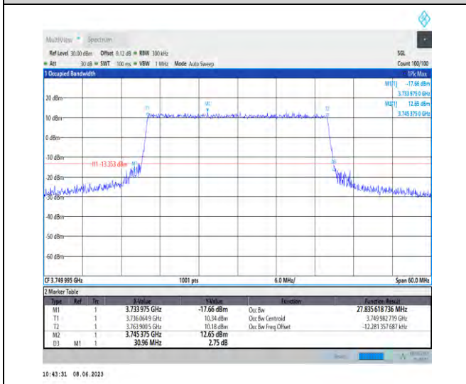
1-N78-3700-3800-PC3-30-30-M-7-CP-16QAM-Outer _Full-78@0-Ant1-27.836-30.960-≤30-PASS
