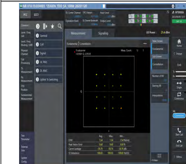
1-N78-3700-3800-PC3-30-100-M-3-DFT-16QAM-Out er_Full-270@0-Ant1-see graph-PASS
