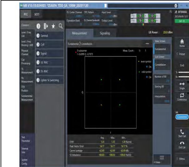
1-N78-3700-3800-PC3-30-100-M-1-DFT-PI2BPSK-Outer_Full-270@0-Ant1-see graph-PASS
