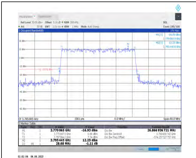
1-N78-3700-3800-PC3-30-30-H-4-DFT-64QAM-Outer_Full-75@0-Ant1-26.867-28.680-≤30-PASS
