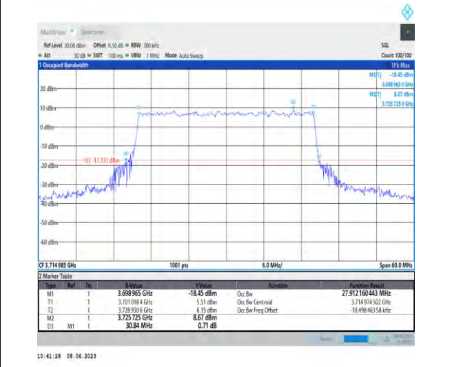
1-N78-3700-3800-PC3-30-30-L-9-CP-256QAM-Outer_Full-78@0-Ant1-27.912-30.840-≤30-PASS
