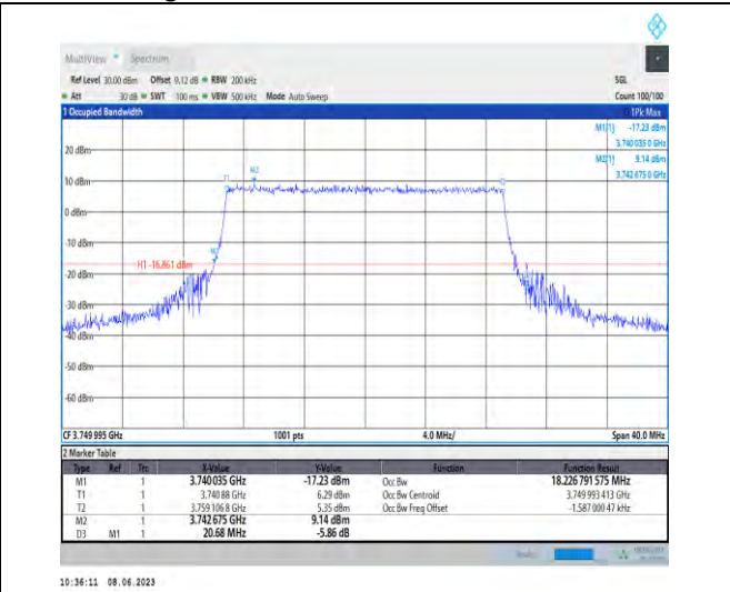
1-N78-3700-3800-PC3-30-20-M-9-CP-256QAM-Outer_Full-51@0-Ant1-18.227-20.680-≤20-PASS
