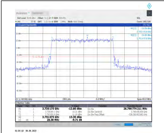
1-N78-3700-3800-PC3-30-30-M-1-DFT-QPSK-Outer_Full-75@0-Ant1-26.791-28.380-≤30-PASS
