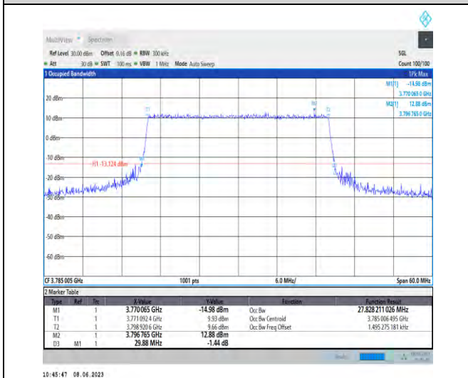
1-N78-3700-3800-PC3-30-30-H-6-CP-QPSK-Outer_Full-78@0-Ant1-27.828-29.880-≤30-PASS
