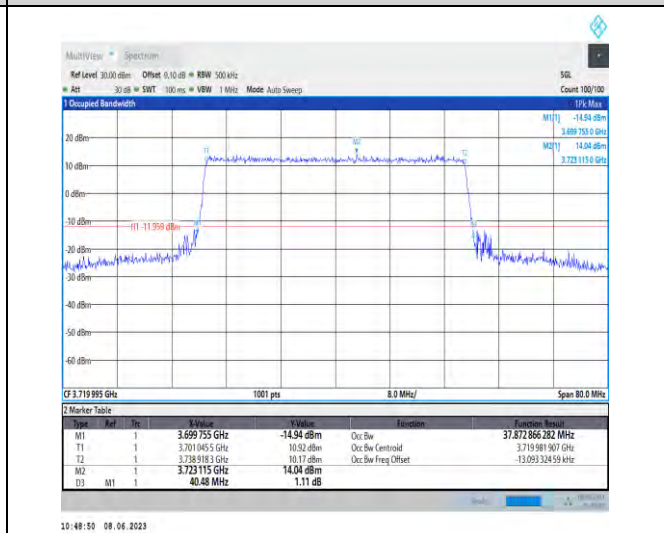
1-N78-3700-3800-PC3-30-40-L-6-CP-QPSK-Outer_Full-106@0-Ant1-37.873-40.480-≤40-PASS
