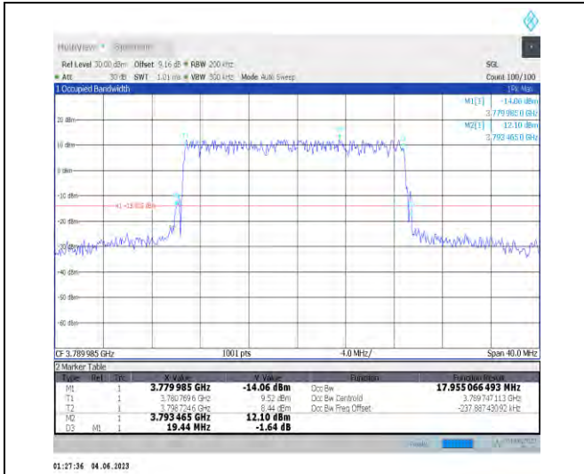
1-N78-3700-3800-PC3-30-20-H-3-DFT-16QAM-Outer_Full-50@0-Ant1-17.955-19.440-≤20-PASS
