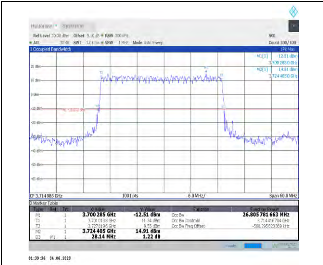
1-N78-3700-3800-PC3-30-30-L-2-DFT-PI2BPSK-Out er_Full-75@0-Ant1-26.806-28.140-≤30-PASS
