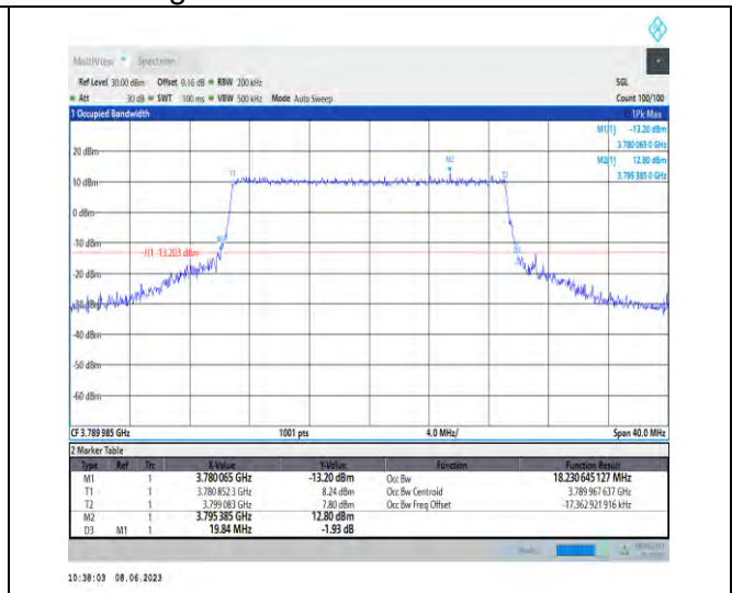
1-N78-3700-3800-PC3-30-20-H-8-CP-64QAM-Outer_Full-51@0-Ant1-18.231-19.840-≤20-PASS
