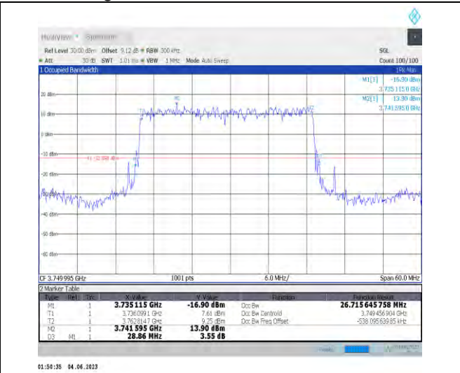
1-N78-3700-3800-PC3-30-30-M-2-DFT-PI2BPSK-Outer_Full-75@0-Ant1-26.716-28.860-≤30-PASS
