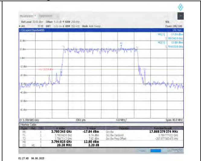
1-N78-3700-3800-PC3-30-20-H-4-DFT-64QAM-Outer_Full-50@0-Ant1-17.868-20.280-≤20-PASS
