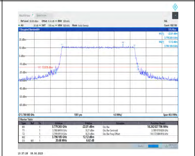
1-N78-3700-3800-PC3-30-20-H-6-CP-QPSK-Outer_Full-51@0-Ant1-18.242-20.680-≤20-PASS
