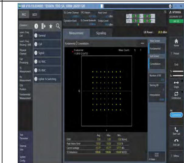
1-N78-3700-3800-PC3-30-100-M-4-DFT-64QAM-Out er_Full-270@0-Ant1-see graph-PASS
