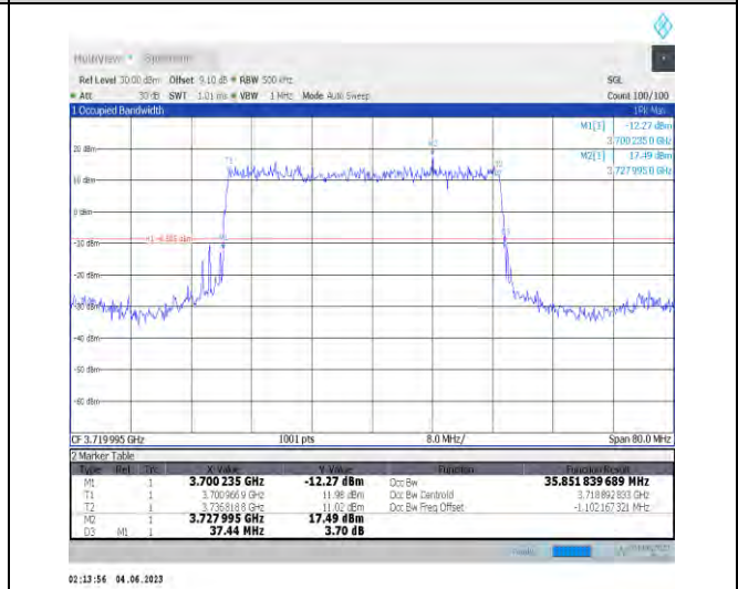
1-N78-3700-3800-PC3-30-40-L-2-DFT-PI2BPSK-Outer_Full-100@0-Ant1-35.852-37.440-≤40-PASS
