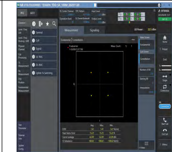
1-N78-3700-3800-PC3-30-100-M-2-DFT-QPSK-Out er_Full-270@0-Ant1-see graph-PASS
