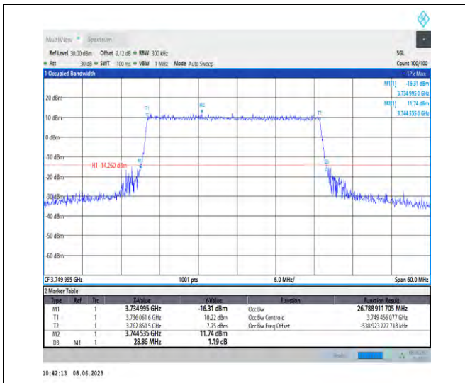
1-N78-3700-3800-PC3-30-30-M-5-DFT-256QAM-Out _Full-75@0-Ant1-26.789-28.860-≤30-PASS
