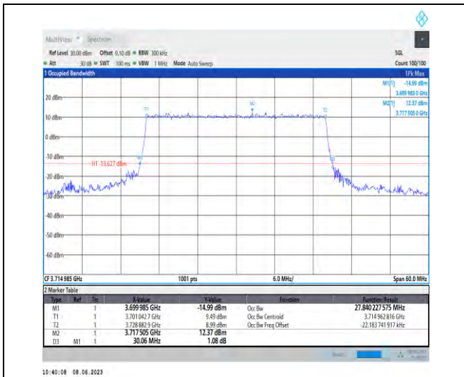
1-N78-3700-3800-PC3-30-30-L-6-CP-QPSK-Outer_Full-78@0-Ant1-27.84-30.060-≤30-PASS
