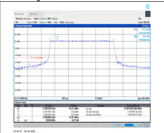
1-N78-3700-3800-PC3-30-30-L-7-CP-16QAM-Outer_Full-78@0-Ant1-27.874-29.880-≤30-PASS
