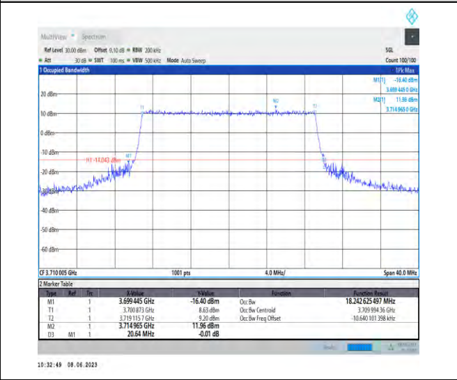
1-N78-3700-3800-PC3-30-20-L-8-CP-64QAM-Outer_Full-51@0-Ant1-18.243-20.640-≤20-PASS
