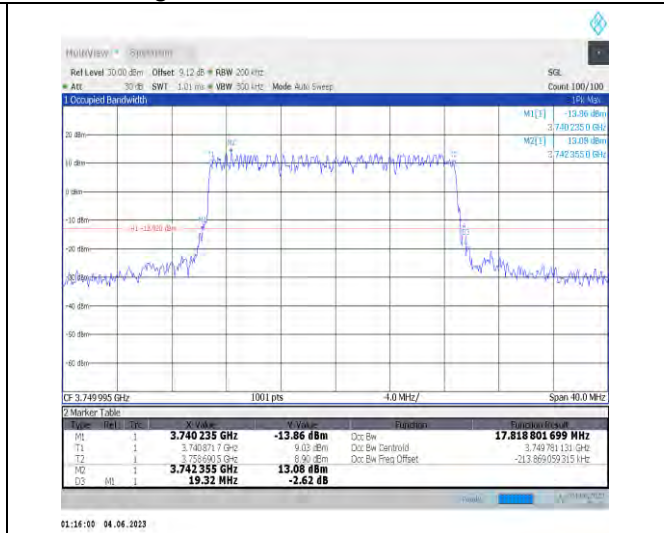
1-N78-3700-3800-PC3-30-20-M-1-DFT-QPSK-Outer_Full-50@0-Ant1-17.819-19.320-≤20-PASS
