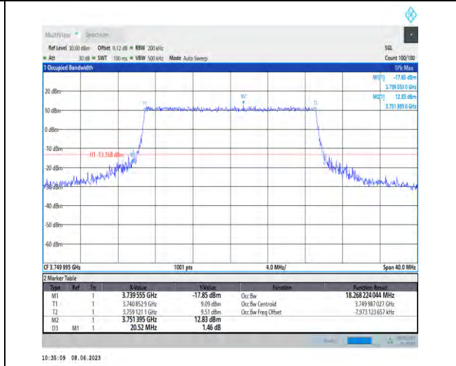
1-N78-3700-3800-PC3-30-20-M-7-CP-16QAM-Outer_Full-51@0-Ant1-18.268-20.520-≤20-PASS
