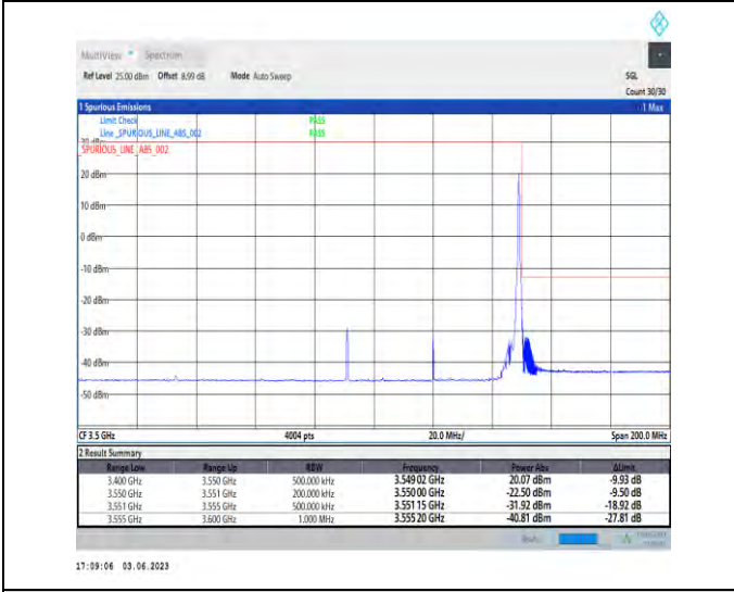
1-N78-3450-3550-PC3-30-60-H-5-CP-QPSK-Edge_1RB_Right-1@161-Ant1-1--PASS-see graph
