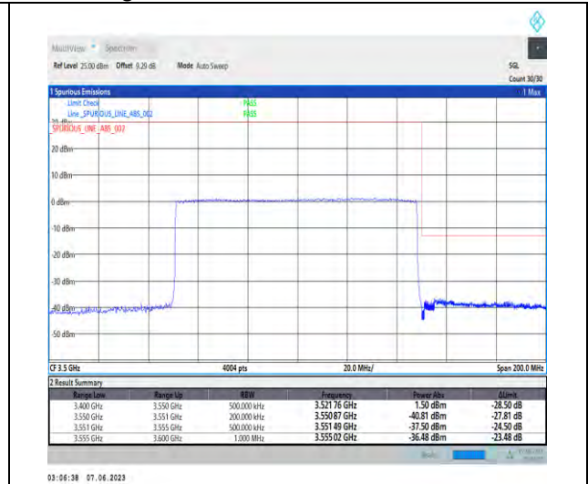
1-N78-3450-3550-PC3-30-100-H-3-DFT-PI2BPSK-Outer_Full-270@0-Ant1-1--PASS-see graph
