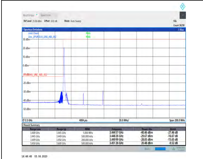
1-N78-3450-3550-PC3-30-50-L-4-CP-QPSK-Edge_1RB_Left-1@0-Ant1-1--PASS-see graph
