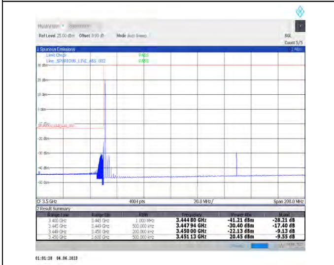
1-N78-3450-3550-PC3-30-100-L-4-CP-QPSK-Edge_1_RB_Left-1@0-Ant1-1--PASS-see graph
