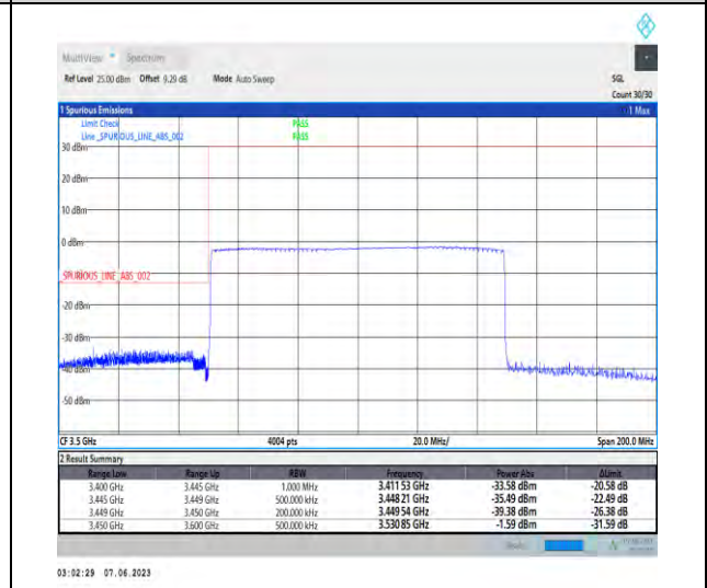
1-N78-3450-3550-PC3-30-100-L-6-CP-QPSK-Outer_Full-273@0-Ant1-1--PASS-see graph
