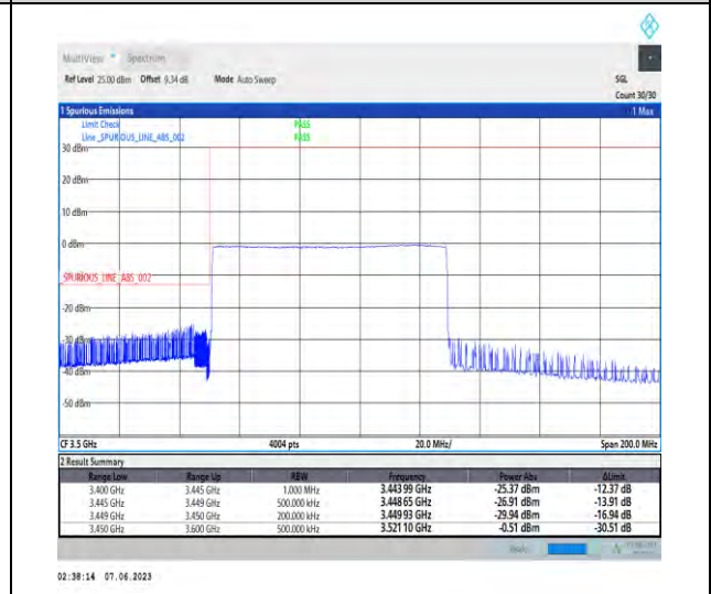
1-N78-3450-3550-PC3-30-80-L-6-CP-QPSK-Outer_Full-217@0-Ant1-1--PASS-see graph
