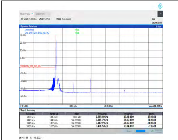
1-N78-3450-3550-PC3-30-50-L-1-DFT-PI2BPSK-Edge_1RB_Left-1@0-Ant1-1--PASS-see graph
