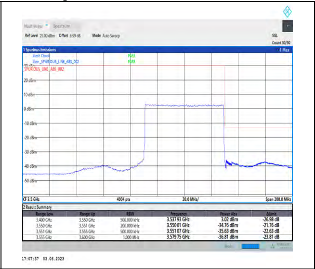
1-N78-3450-3550-PC3-30-60-H-3-DFT-PI2BPSK-Outer_Full-162@0-Ant1-1--PASS-see graph
