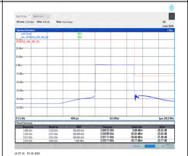
1-N78-3450-3550-PC3-30-50-H-6-CP-QPSK-Outer_Full-133@0-Ant1-1--PASS-see graph
