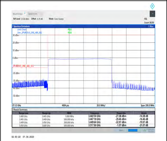
1-N78-3450-3550-PC3-30-90-L-6-CP-QPSK-Outer_Full-245@0-Ant1-1--PASS-see graph
