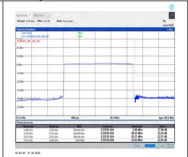
1-N78-3450-3550-PC3-30-90-H-3-DFT-PI2BPSK-Outer_Full-240@0-Ant1-1--PASS-see graph
