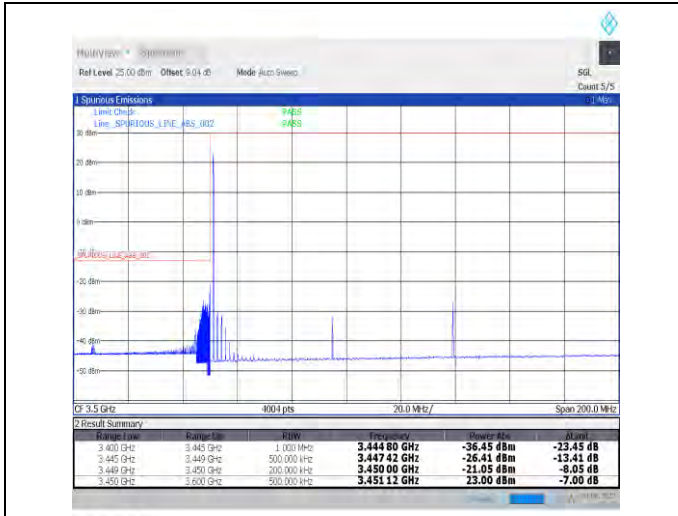
1-N78-3450-3550-PC3-30-90-L-1-DFT-PI2BPSK-Edge_1RB_Left-1@0-Ant1-1--PASS-see graph
