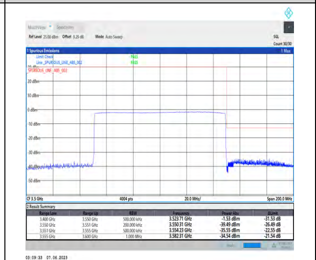
1-N78-3450-3550-PC3-30-100-H-6-CP-QPSK-Outer_Full-273@0-Ant1-1--PASS-see graph
