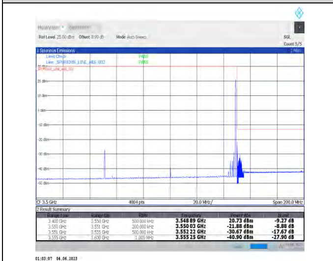
1-N78-3450-3550-PC3-30-100-H-5-CP-QPSK-Edge_1RB_Right-1@272-Ant1-1--PASS-see graph
