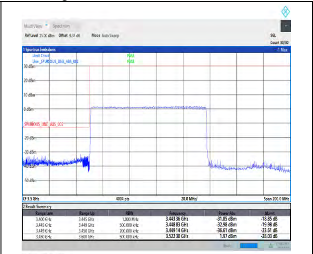
1-N78-3450-3550-PC3-30-90-L-3-DFT-PI2BPSK-Outer_Full-240@0-Ant1-1--PASS-see graph
