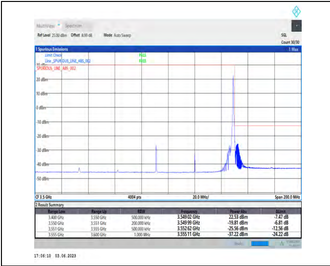
1-N78-3450-3550-PC3-30-60-H-2-DFT-PI2BPSK-Edge_1RB_Right-1@161-Ant1-1--PASS-see graph
