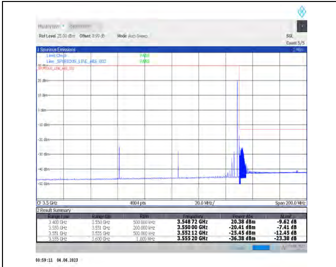
1-N78-3450-3550-PC3-30-90-H-2-DFT-PI2BPSK-Edge_1RB_Right-1@244-Ant1-1--PASS-see graph
