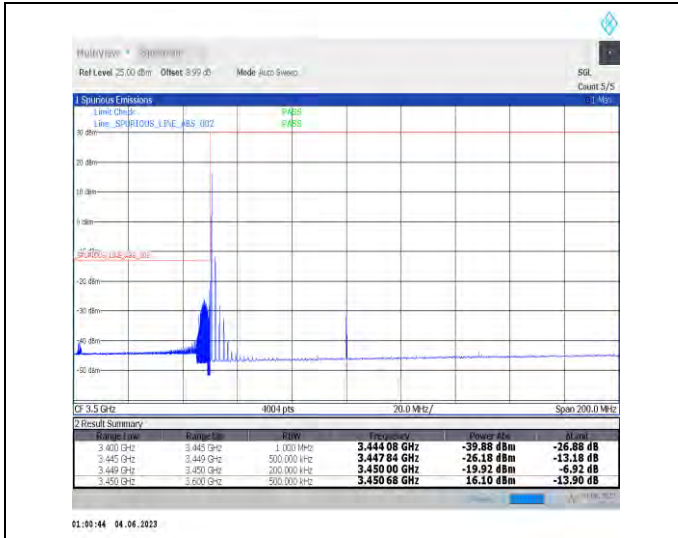
1-N78-3450-3550-PC3-30-100-L-1-DFT-PI2BPSK-Edge_1_RB_Left-1@0-Ant1-1--PASS-see graph
