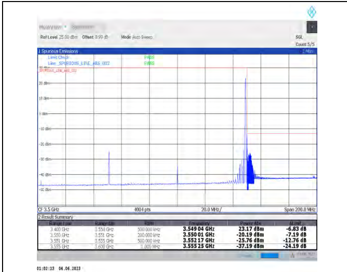
1-N78-3450-3550-PC3-30-100-H-2-DFT-PI2BPSK-Edge_1RB_Right-1@272-Ant1-1--PASS-see graph
