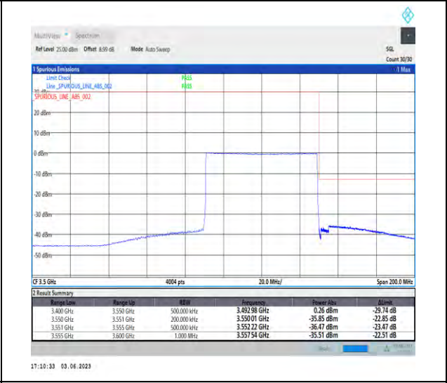
1-N78-3450-3550-PC3-30-60-H-6-CP-QPSK-Outer_Full-162@0-Ant1-1--PASS-see graph
