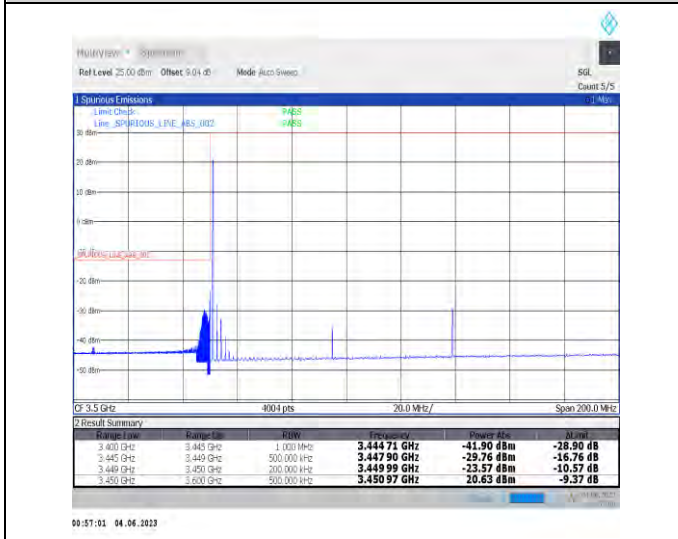
1-N78-3450-3550-PC3-30-90-L-4-CP-QPSK-Edge_1RB_Left-1@0-Ant1-1--PASS-see graph
