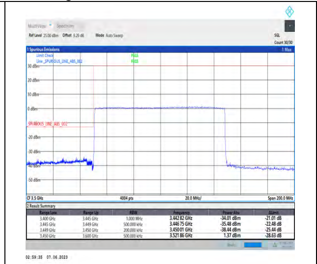
1-N78-3450-3550-PC3-30-100-L-3-DFT-PI2BPSK-Outer_Full-270@0-Ant1-1--PASS-see graph
