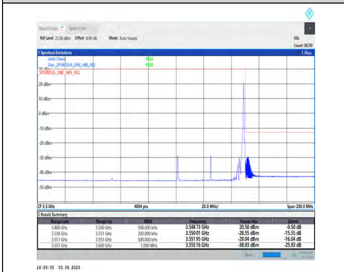
1-N78-3450-3550-PC3-30-50-H-5-CP-QPSK-Edge_1RB_Right-1@132-Ant1-1--PASS-see graph
